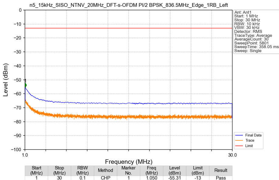
n5_15kHz_SISO_NTNV_20MHz_DFT-s-OFDM PI/2 BPSK_836.5MHz_Edge_1RB_Left
