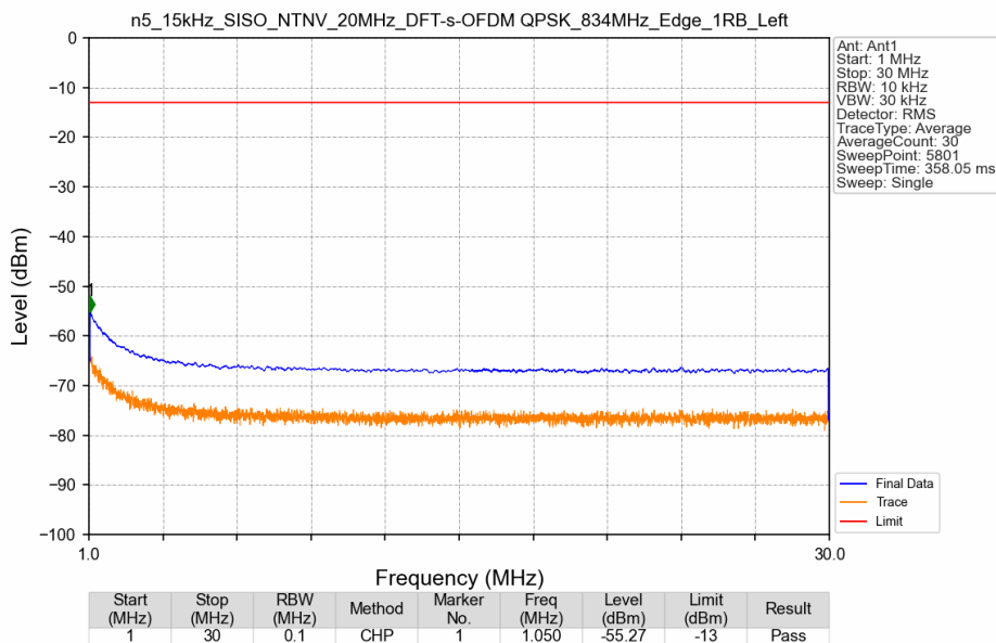
n5_15kHz_SISO_NTNV_20MHz_DFT-s-OFDM QPSK_834MHz_Edge_1RB_Left
