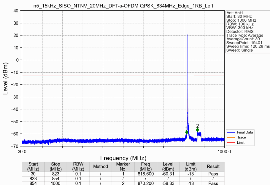
n5_15kHz_SISO_NTNV_20MHz_DFT-s-OFDM QPSK_834MHz_Edge_1RB_Left
