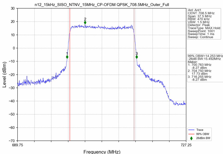
n12_15kHz_SISO_NTNV_15MHz_CP-OFDM QPSK_708.5MHz_Outer_Full
