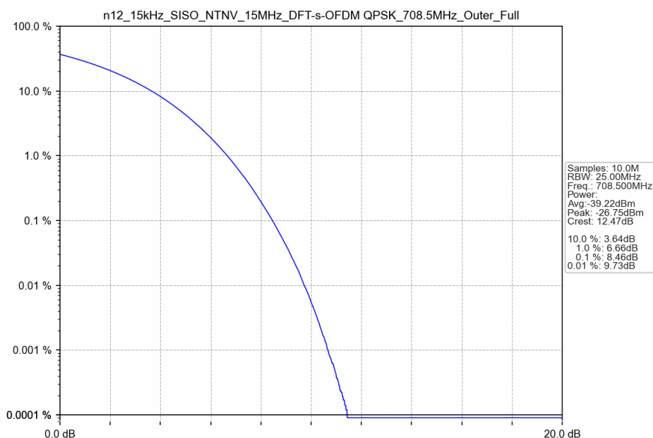
n12_15kHz_SISO_NTNV_15MHz_DFT-s-OFDM QPSK_708.5MHz_Outer_Full
