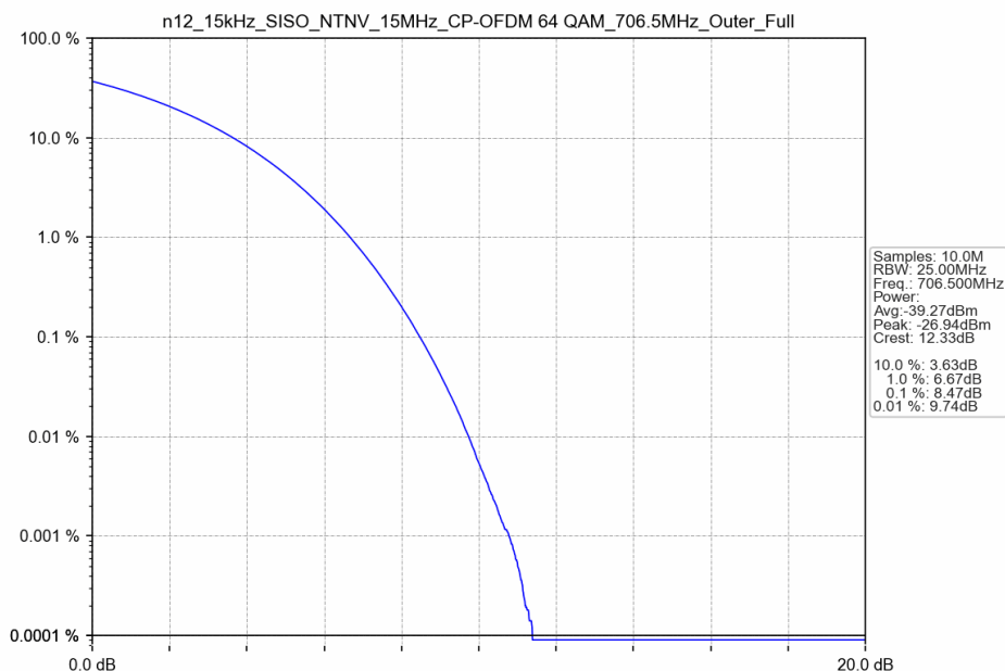
n12_15kHz_SISO_NTNV_15MHz_CP-OFDM 64 QAM_706.5MHz_Outer_Full
