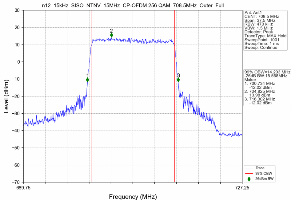
n12_15kHz_SISO_NTNV_15MHz_CP-OFDM 256 QAM_708.5MHz_Outer_Full
