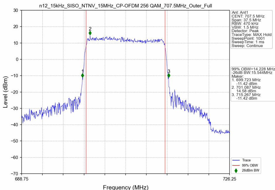
n12_15kHz_SISO_NTNV_15MHz_CP-OFDM 256 QAM_707.5MHz_Outer_Full
