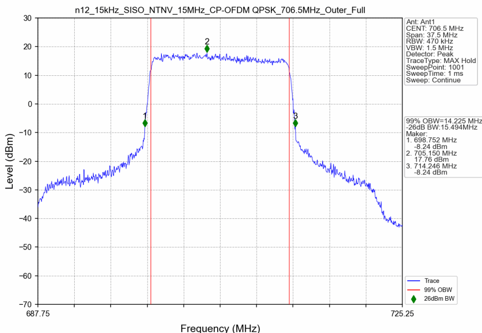
n12_15kHz_SISO_NTNV_15MHz_CP-OFDM QPSK_706.5MHz_Outer_Full
