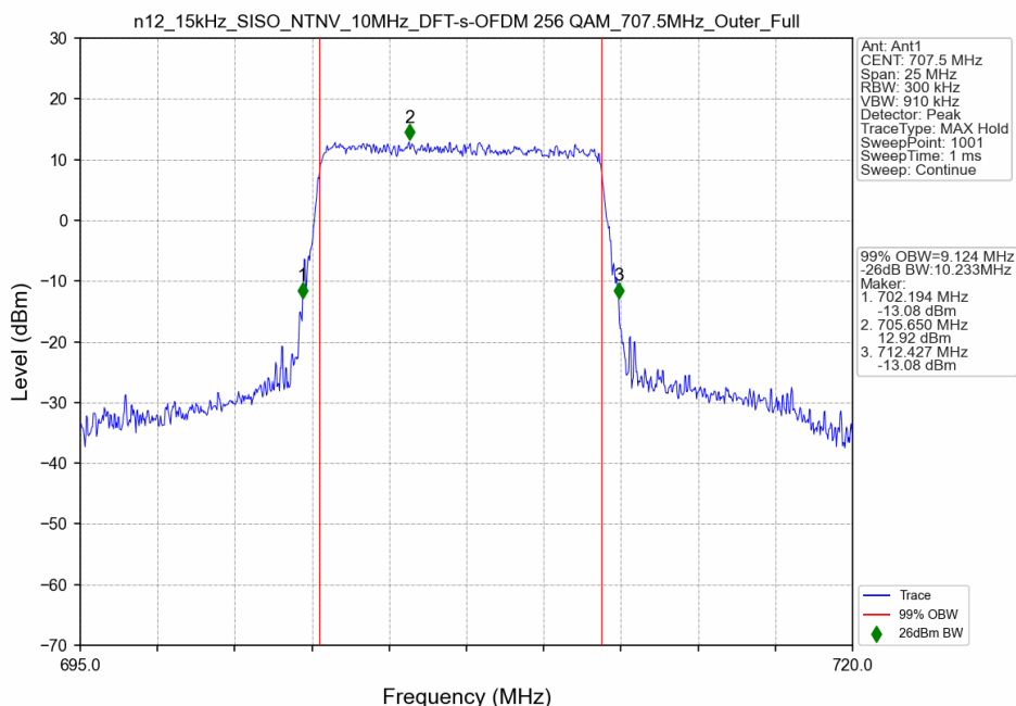
n12_15kHz_SISO_NTNV_10MHz_DFT-s-OFDM 256 QAM_707.5MHz_Outer_Full
