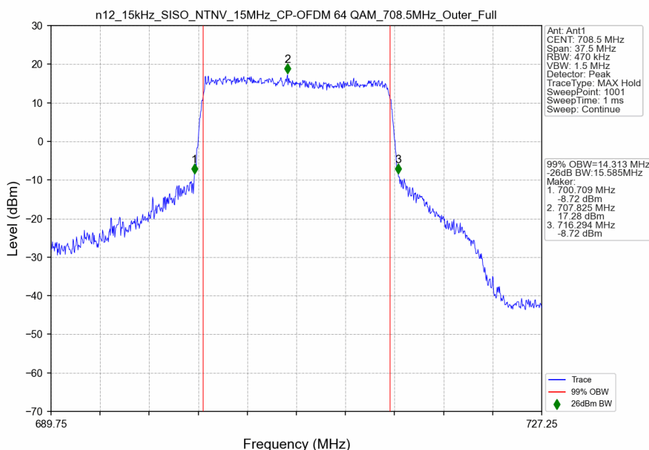
n12_15kHz_SISO_NTNV_15MHz_CP-OFDM 64 QAM_708.5MHz_Outer_Full
