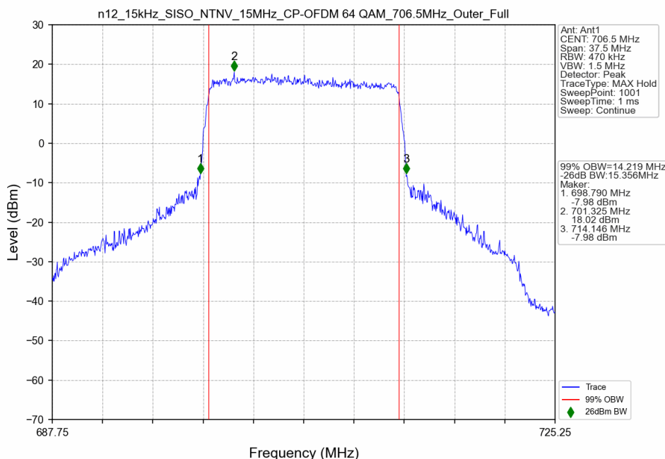
n12_15kHz_SISO_NTNV_15MHz_CP-OFDM 64 QAM_706.5MHz_Outer_Full
