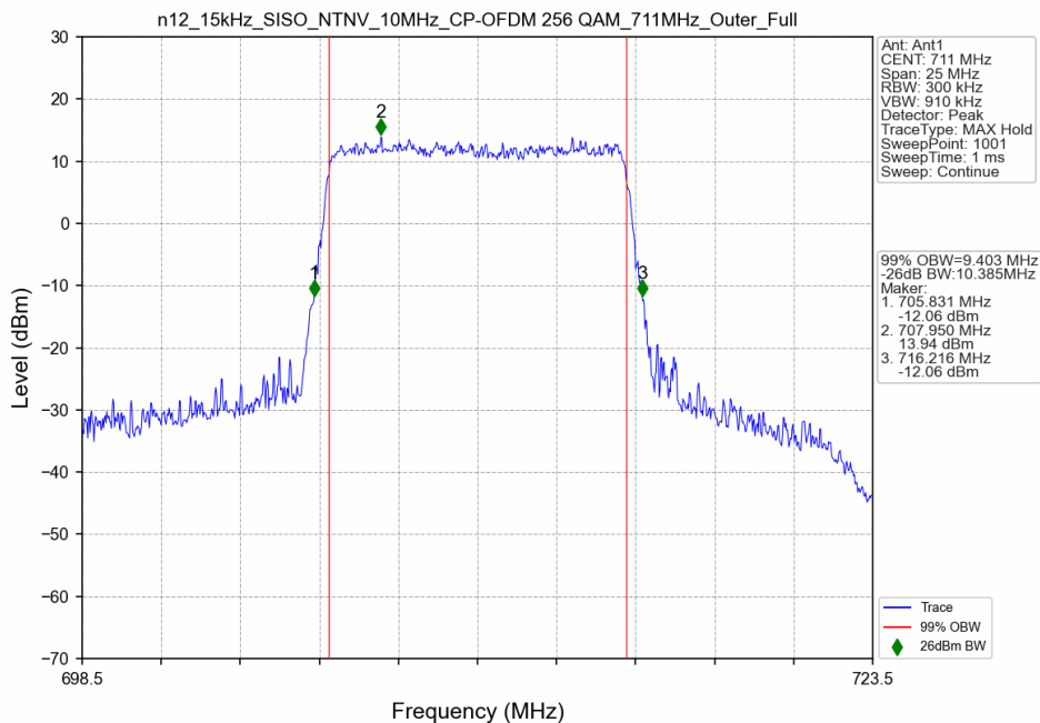
n12_15kHz_SISO_NTNV_10MHz_CP-OFDM 256 QAM_711MHz_Outer_Full
