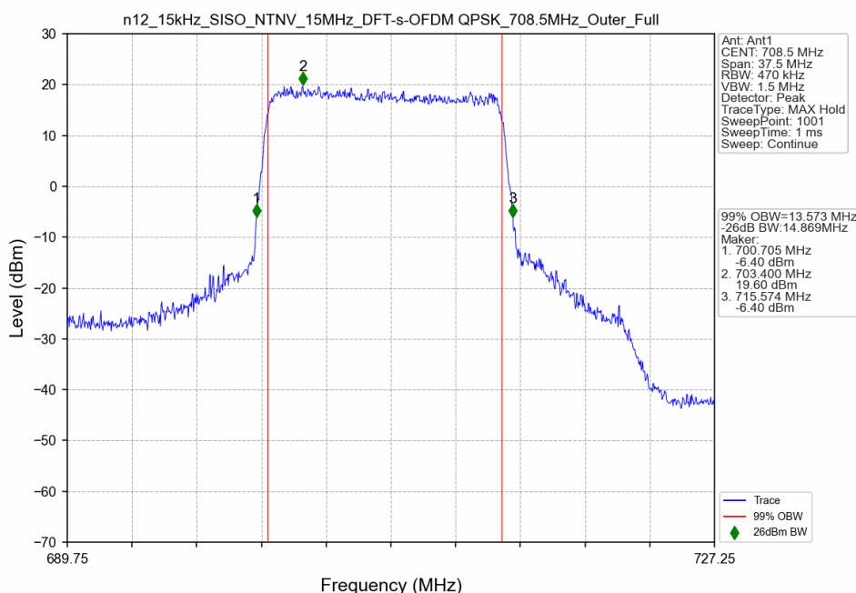
n12_15kHz_SISO_NTNV_15MHz_DFT-s-OFDM QPSK_708.5MHz_Outer_Full
