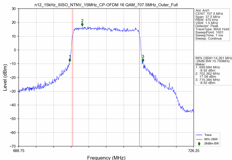
n12_15kHz_SISO_NTNV_15MHz_CP-OFDM 16 QAM_707.5MHz_Outer_Full
