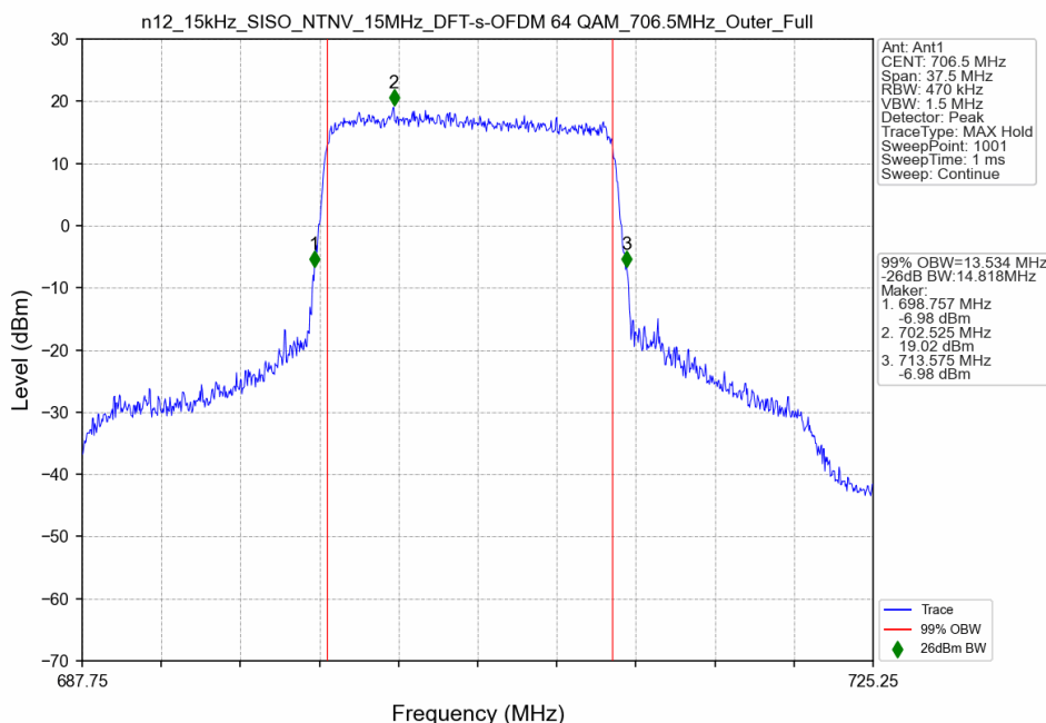
n12_15kHz_SISO_NTNV_15MHz_DFT-s-OFDM 64 QAM_706.5MHz_Outer_Full
