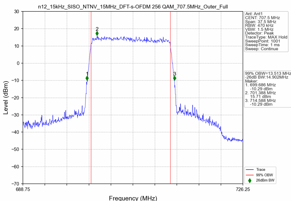
n12_15kHz_SISO_NTNV_15MHz_DFT-s-OFDM 256 QAM_707.5MHz_Outer_Full
