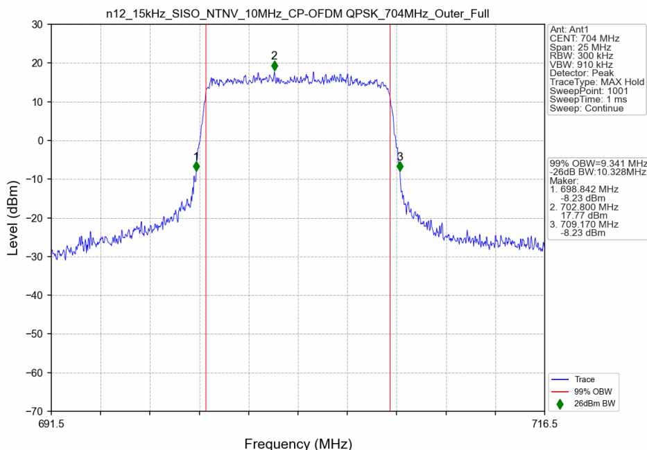
n12_15kHz_SISO_NTNV_10MHz_CP-OFDM QPSK_704MHz_Outer_Full
