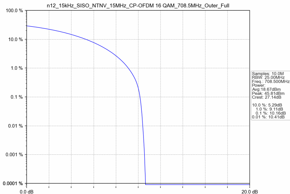
n12_15kHz_SISO_NTNV_15MHz_CP-OFDM 16 QAM_708.5MHz_Outer_Full
