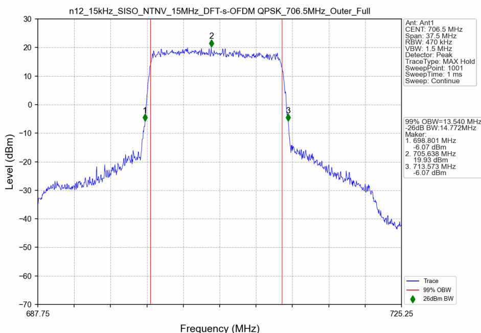
n12_15kHz_SISO_NTNV_15MHz_DFT-s-OFDM QPSK_706.5MHz_Outer_Full
