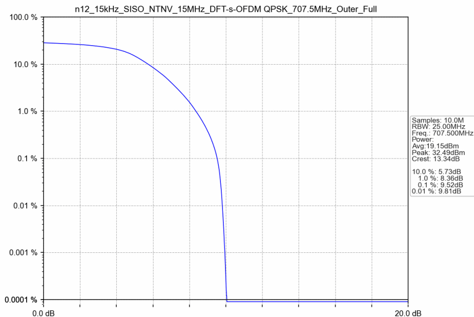
n12_15kHz_SISO_NTNV_15MHz_DFT-s-OFDM QPSK_707.5MHz_Outer_Full
