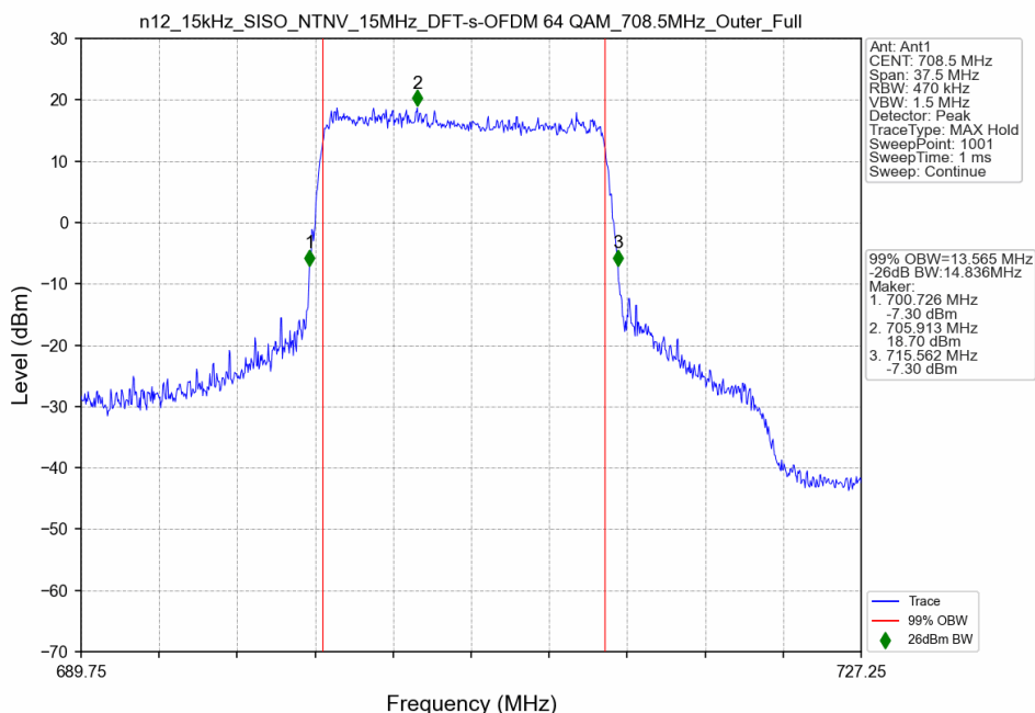
n12_15kHz_SISO_NTNV_15MHz_DFT-s-OFDM 64 QAM_708.5MHz_Outer_Full
