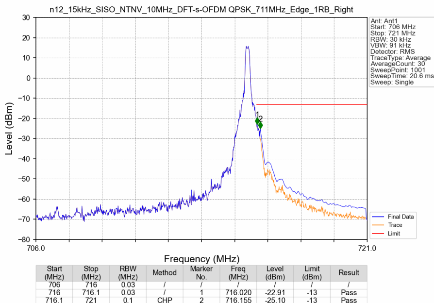
n12_15kHz_SISO_NTNV_10MHz_DFT-s-OFDM QPSK_711MHz_Edge_1RB_Right
