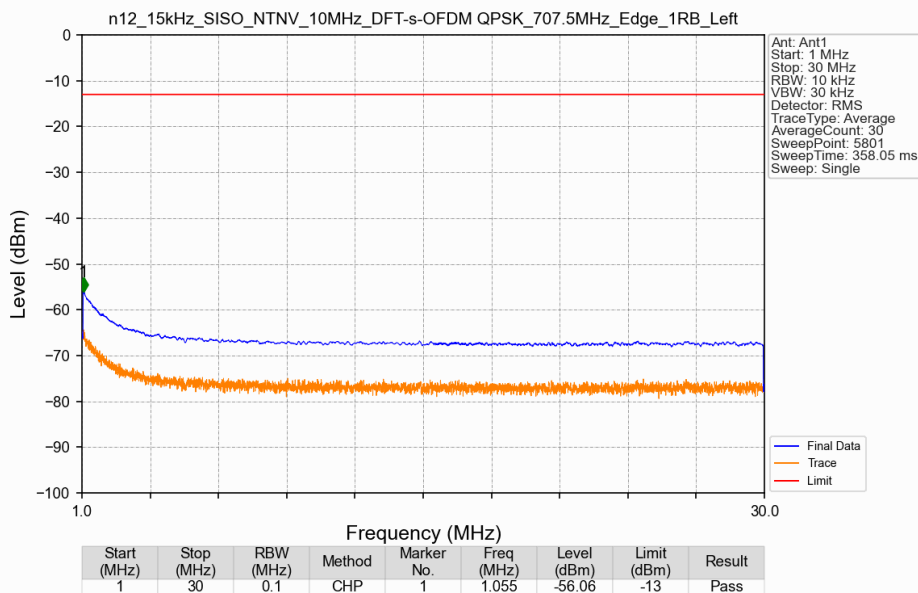
n12_15kHz_SISO_NTNV_10MHz_DFT-s-OFDM QPSK_707.5MHz_Edge_1RB_Left
