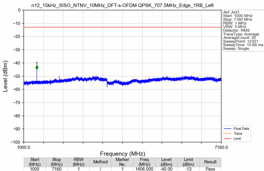
n12_15kHz_SISO_NTNV_10MHz_DFT-s-OFDM QPSK_707.5MHz_Edge_1RB_Left
