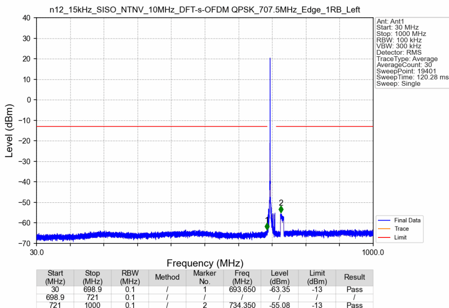
n12_15kHz_SISO_NTNV_10MHz_DFT-s-OFDM QPSK_707.5MHz_Edge_1RB_Left
