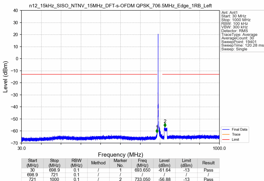
n12_15kHz_SISO_NTNV_15MHz_DFT-s-OFDM QPSK_706.5MHz_Edge_1RB_Left
