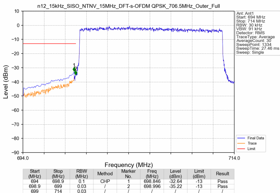
n12_15kHz_SISO_NTNV_15MHz_DFT-s-OFDM QPSK_706.5MHz_Outer_Full
