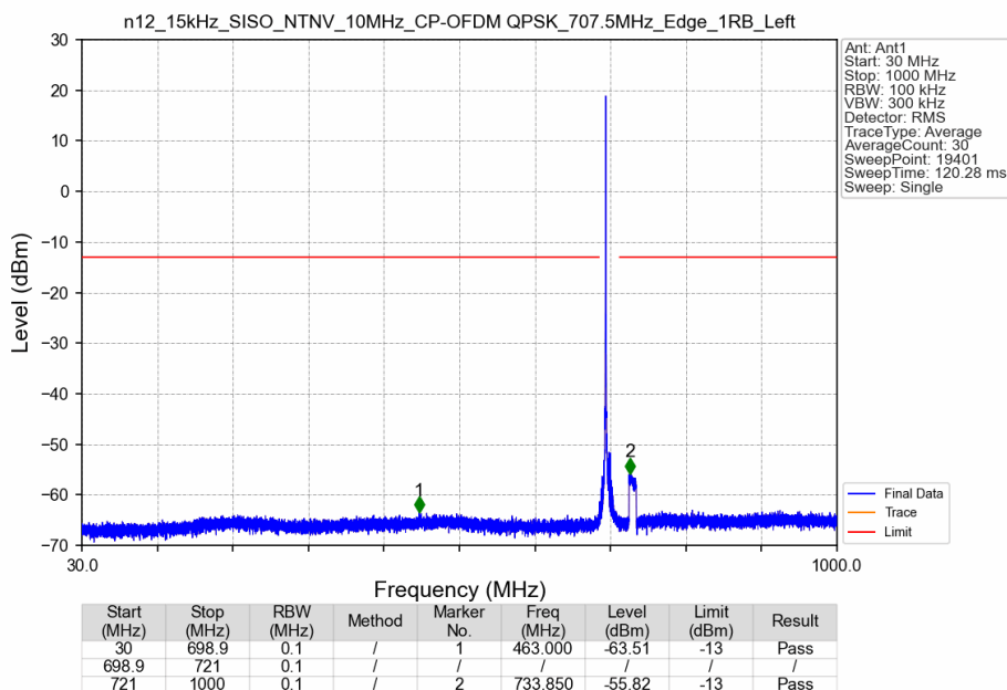
n12_15kHz_SISO_NTNV_10MHz_CP-OFDM QPSK_707.5MHz_Edge_1RB_Left
