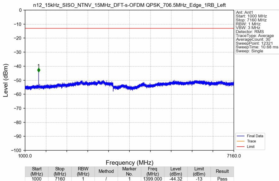
n12_15kHz_SISO_NTNV_15MHz_DFT-s-OFDM QPSK_706.5MHz_Edge_1RB_Left
