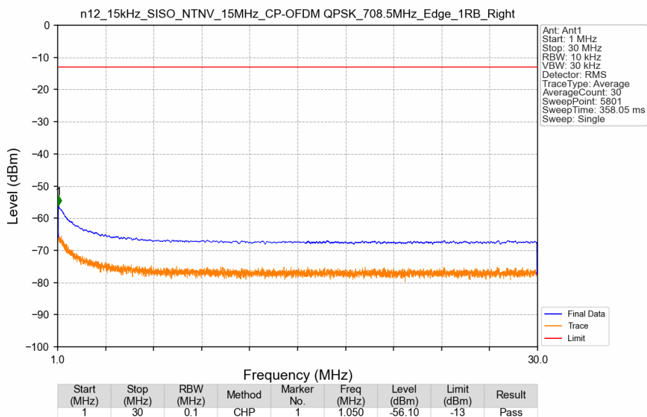
n12_15kHz_SISO_NTNV_15MHz_CP-OFDM QPSK_708.5MHz_Edge_1RB_Right
