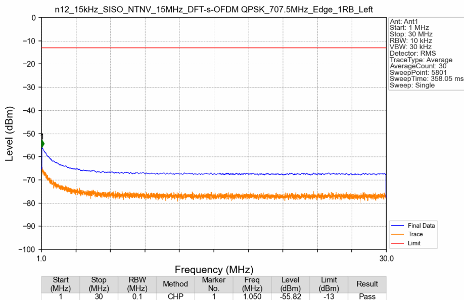
n12_15kHz_SISO_NTNV_15MHz_DFT-s-OFDM QPSK_707.5MHz_Edge_1RB_Left
