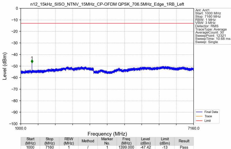
n12_15kHz_SISO_NTNV_15MHz_CP-OFDM QPSK_706.5MHz_Edge_1RB_Left
