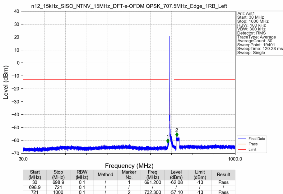
n12_15kHz_SISO_NTNV_15MHz_DFT-s-OFDM QPSK_707.5MHz_Edge_1RB_Left
