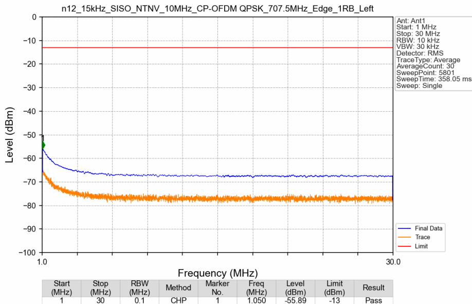
n12_15kHz_SISO_NTNV_10MHz_CP-OFDM QPSK_707.5MHz_Edge_1RB_Left
