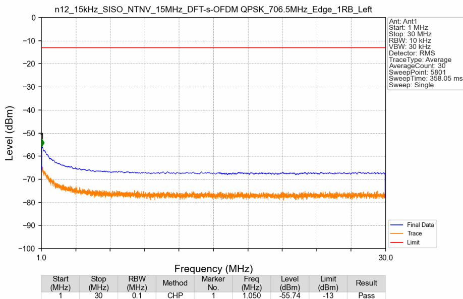
n12_15kHz_SISO_NTNV_15MHz_DFT-s-OFDM QPSK_706.5MHz_Edge_1RB_Left
