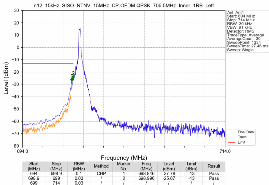
n12_15kHz_SISO_NTNV_15MHz_CP-OFDM QPSK_706.5MHz_Inner_1RB_Left
