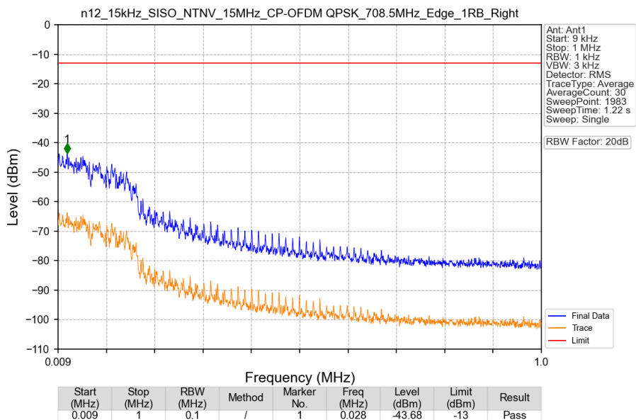
n12_15kHz_SISO_NTNV_15MHz_CP-OFDM QPSK_708.5MHz_Edge_1RB_Right
