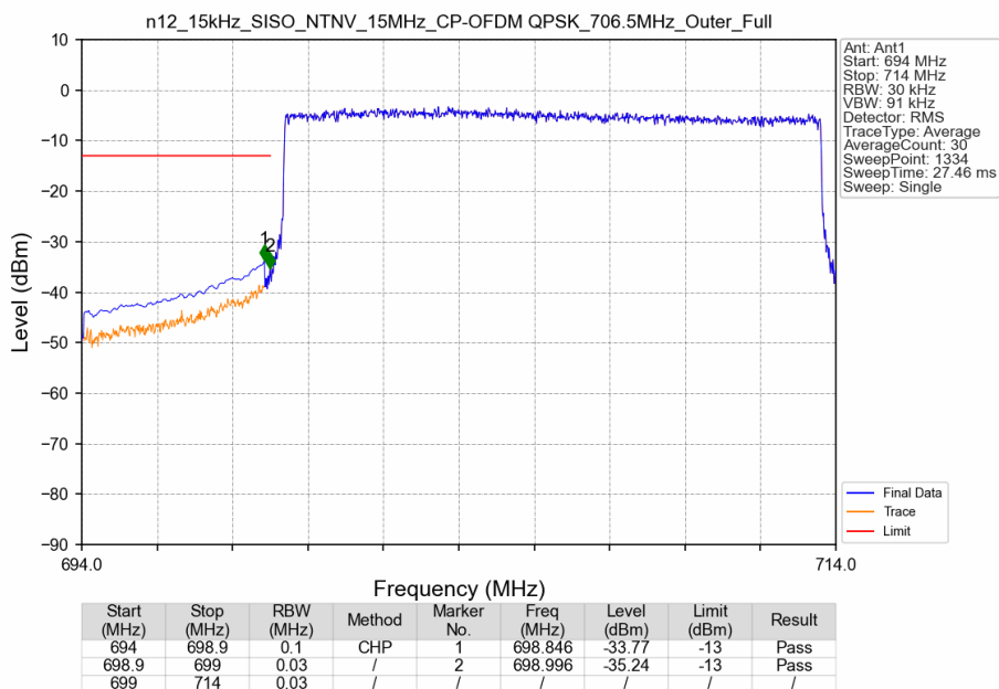
n12_15kHz_SISO_NTNV_15MHz_CP-OFDM QPSK_706.5MHz_Outer_Full
