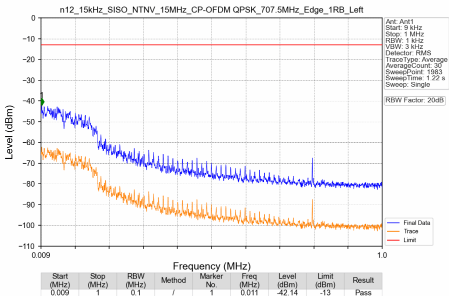
n12_15kHz_SISO_NTNV_15MHz_CP-OFDM QPSK_707.5MHz_Edge_1RB_Left
