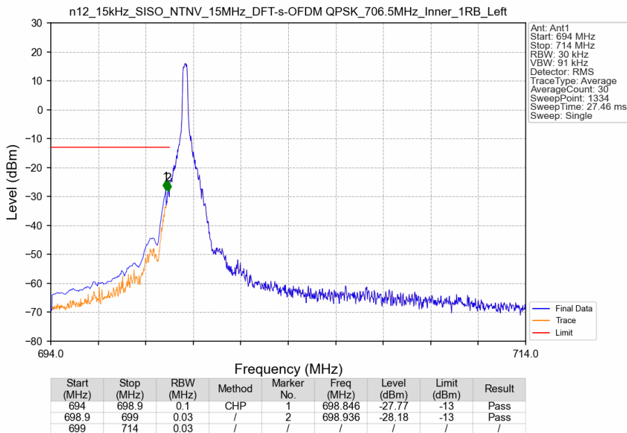
n12_15kHz_SISO_NTNV_15MHz_DFT-s-OFDM QPSK_706.5MHz_Inner_1RB_Left
