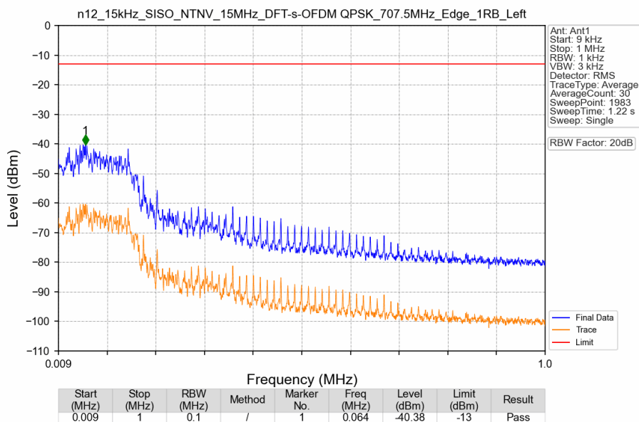
n12_15kHz_SISO_NTNV_15MHz_DFT-s-OFDM QPSK_707.5MHz_Edge_1RB_Left
