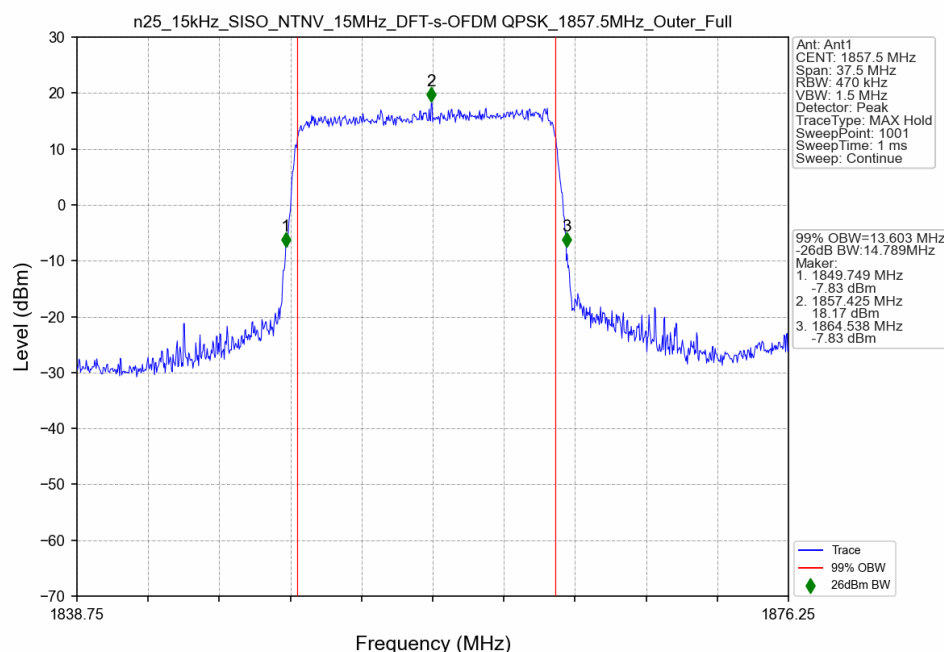
n25_15kHz_SISO_NTNV_15MHz_DFT-s-OFDM QPSK_1857.5MHz_Outer_Full
