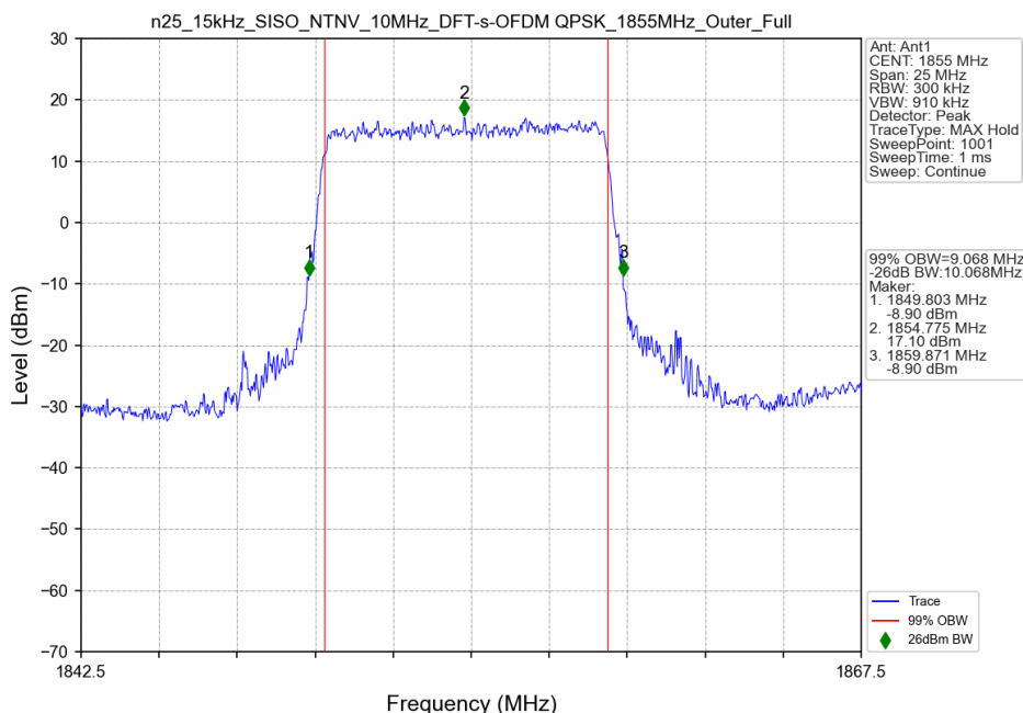
n25_15kHz_SISO_NTNV_10MHz_DFT-s-OFDM QPSK_1855MHz_Outer_Full
