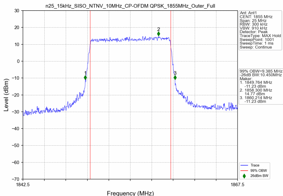
n25_15kHz_SISO_NTNV_10MHz_CP-OFDM QPSK_1855MHz_Outer_Full
