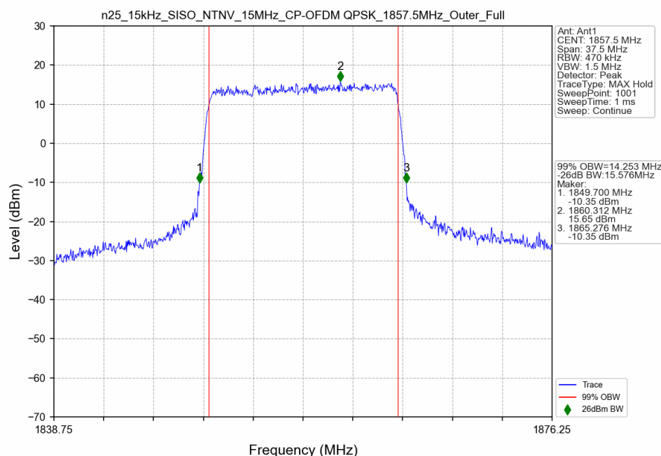
n25_15kHz_SISO_NTNV_15MHz_CP-OFDM QPSK_1857.5MHz_Outer_Full
