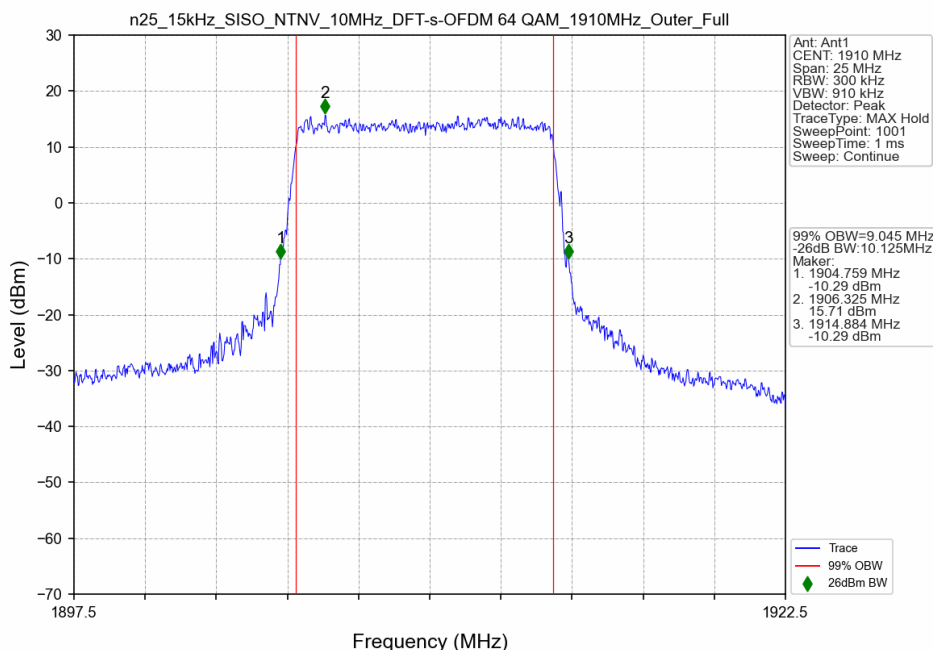
n25_15kHz_SISO_NTNV_10MHz_DFT-s-OFDM 64 QAM_1910MHz_Outer_Full
