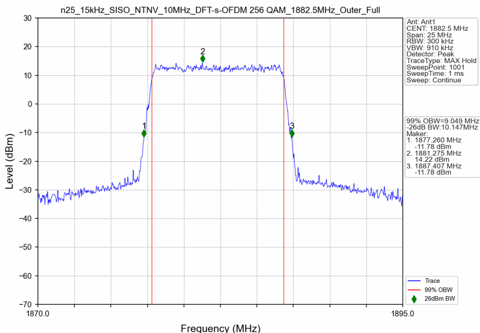
n25_15kHz_SISO_NTNV_10MHz_DFT-s-OFDM 256 QAM_1882.5MHz_Outer_Full
