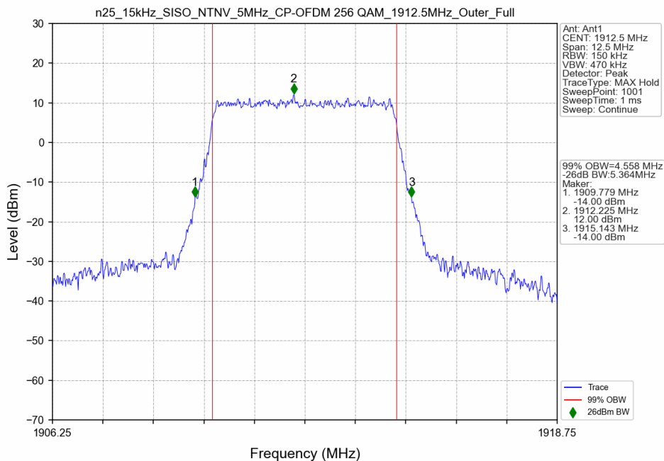
n25_15kHz_SISO_NTNV_5MHz_CP-OFDM 256 QAM_1912.5MHz_Outer_Full
