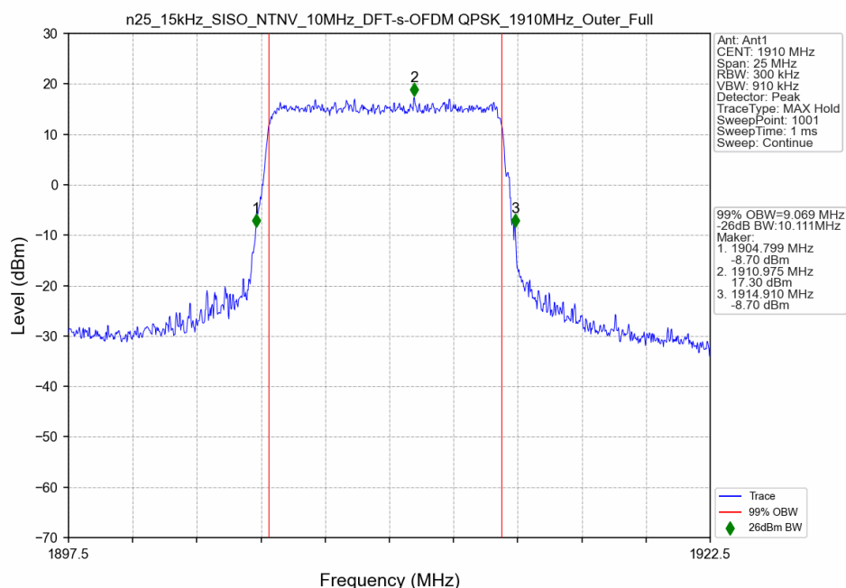
n25_15kHz_SISO_NTNV_10MHz_DFT-s-OFDM QPSK_1910MHz_Outer_Full
