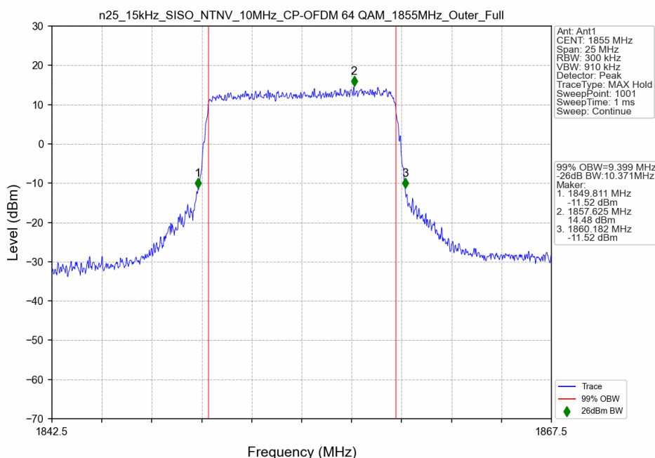
n25_15kHz_SISO_NTNV_10MHz_CP-OFDM 64 QAM_1855MHz_Outer_Full
