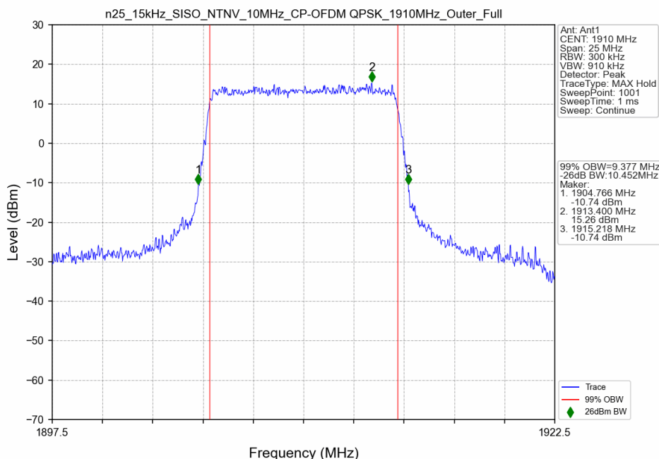
n25_15kHz_SISO_NTNV_10MHz_CP-OFDM QPSK_1910MHz_Outer_Full
