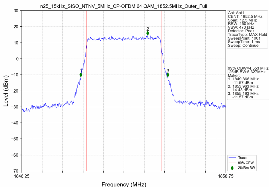
n25_15kHz_SISO_NTNV_5MHz_CP-OFDM 64 QAM_1852.5MHz_Outer_Full
