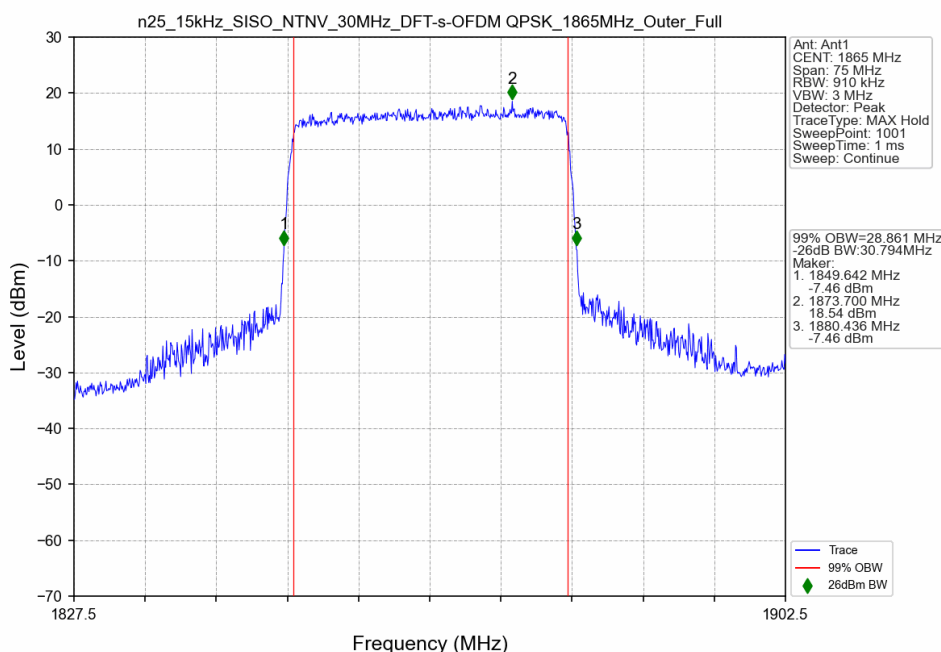
n25_15kHz_SISO_NTNV_30MHz_DFT-s-OFDM QPSK_1865MHz_Outer_Full
