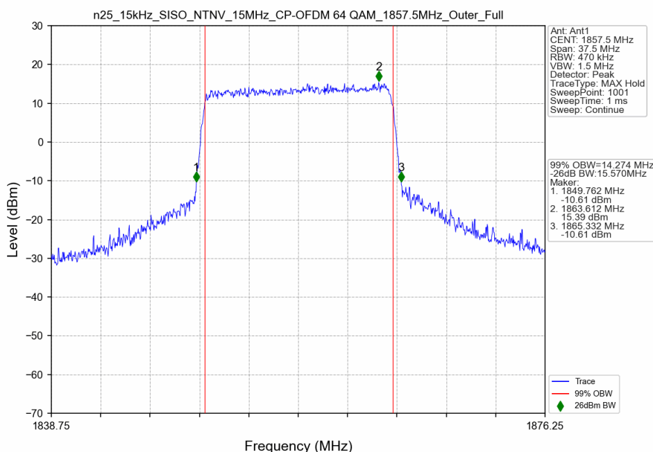
n25_15kHz_SISO_NTNV_15MHz_CP-OFDM 64 QAM_1857.5MHz_Outer_Full
