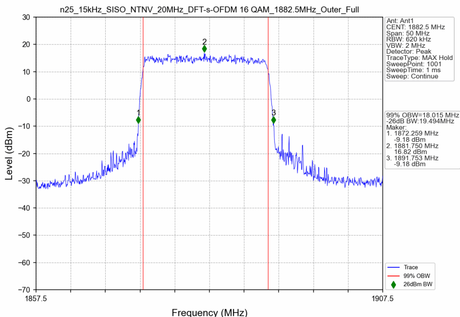
n25_15kHz_SISO_NTNV_20MHz_DFT-s-OFDM 16 QAM_1882.5MHz_Outer_Full
