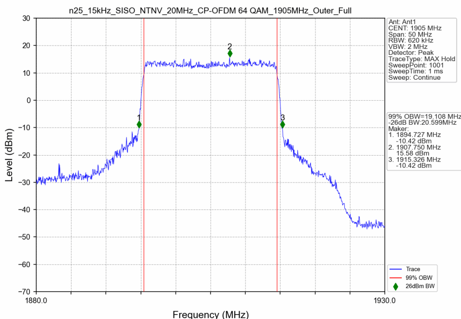
n25_15kHz_SISO_NTNV_20MHz_CP-OFDM 64 QAM_1905MHz_Outer_Full
