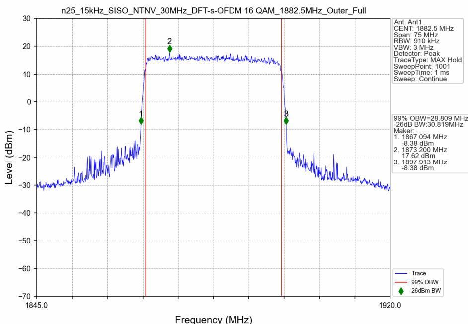
n25_15kHz_SISO_NTNV_30MHz_DFT-s-OFDM 16 QAM_1882.5MHz_Outer_Full
