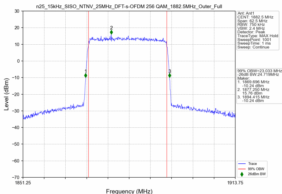
n25_15kHz_SISO_NTNV_25MHz_DFT-s-OFDM 256 QAM_1882.5MHz_Outer_Full
