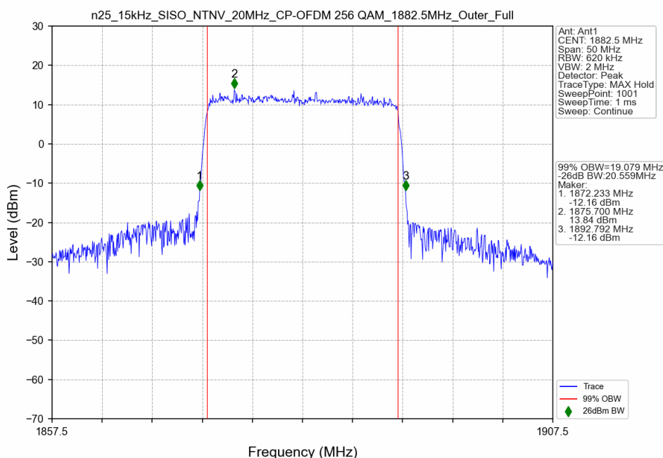
n25_15kHz_SISO_NTNV_20MHz_CP-OFDM 256 QAM_1882.5MHz_Outer_Full
