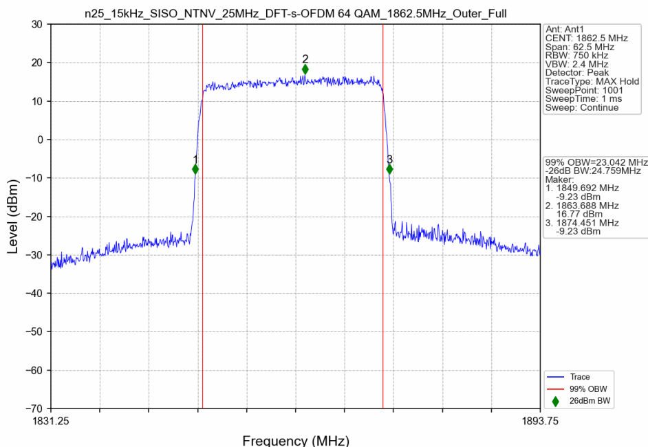
n25_15kHz_SISO_NTNV_25MHz_DFT-s-OFDM 64 QAM_1862.5MHz_Outer_Full
