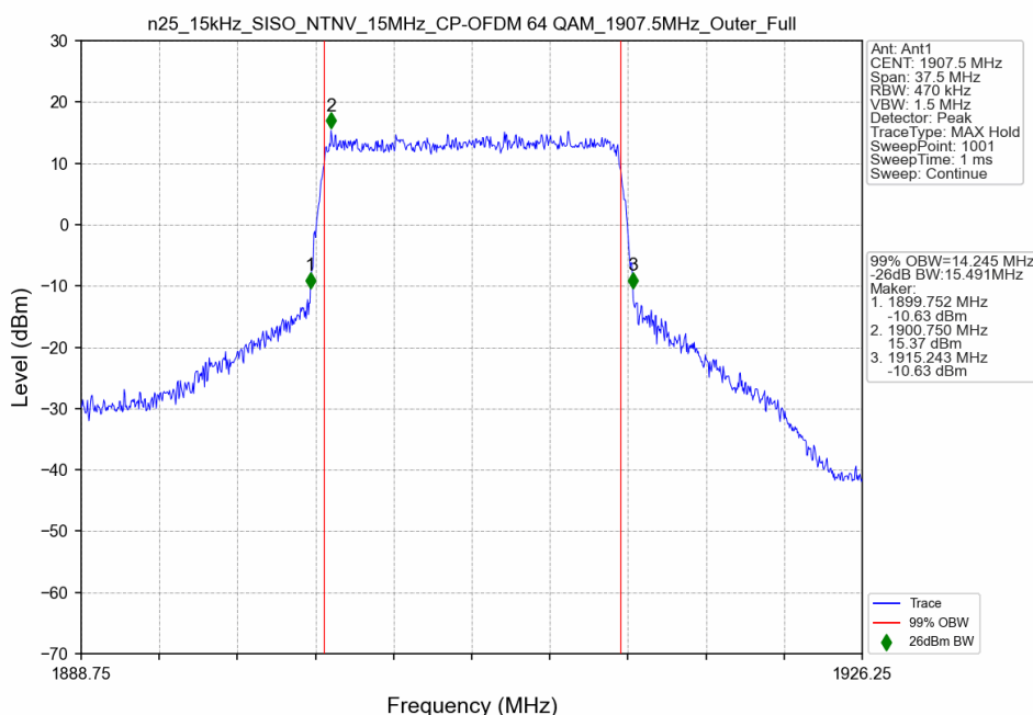
n25_15kHz_SISO_NTNV_15MHz_CP-OFDM 64 QAM_1907.5MHz_Outer_Full
