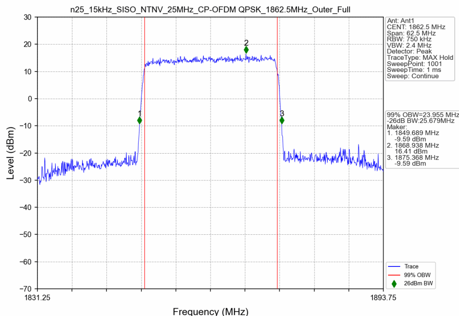
n25_15kHz_SISO_NTNV_25MHz_CP-OFDM QPSK_1862.5MHz_Outer_Full
