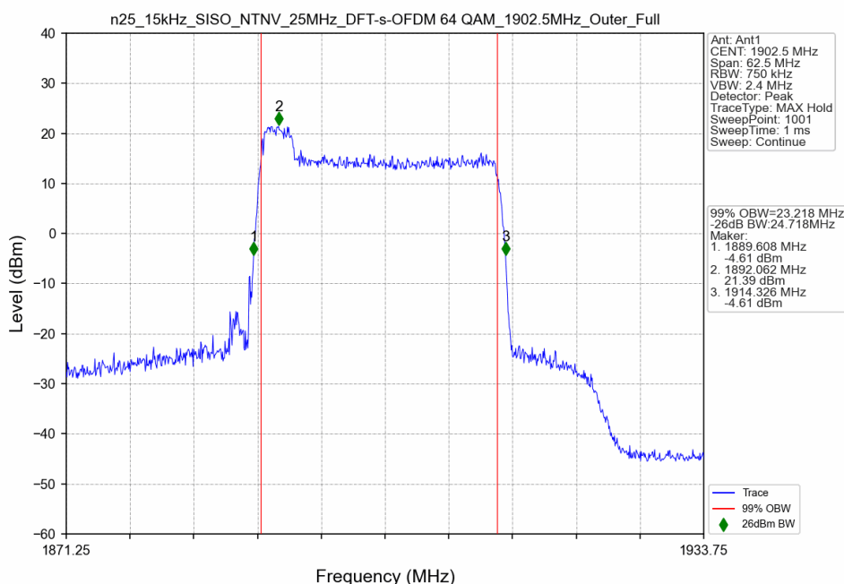
n25_15kHz_SISO_NTNV_25MHz_DFT-s-OFDM 64 QAM_1902.5MHz_Outer_Full
