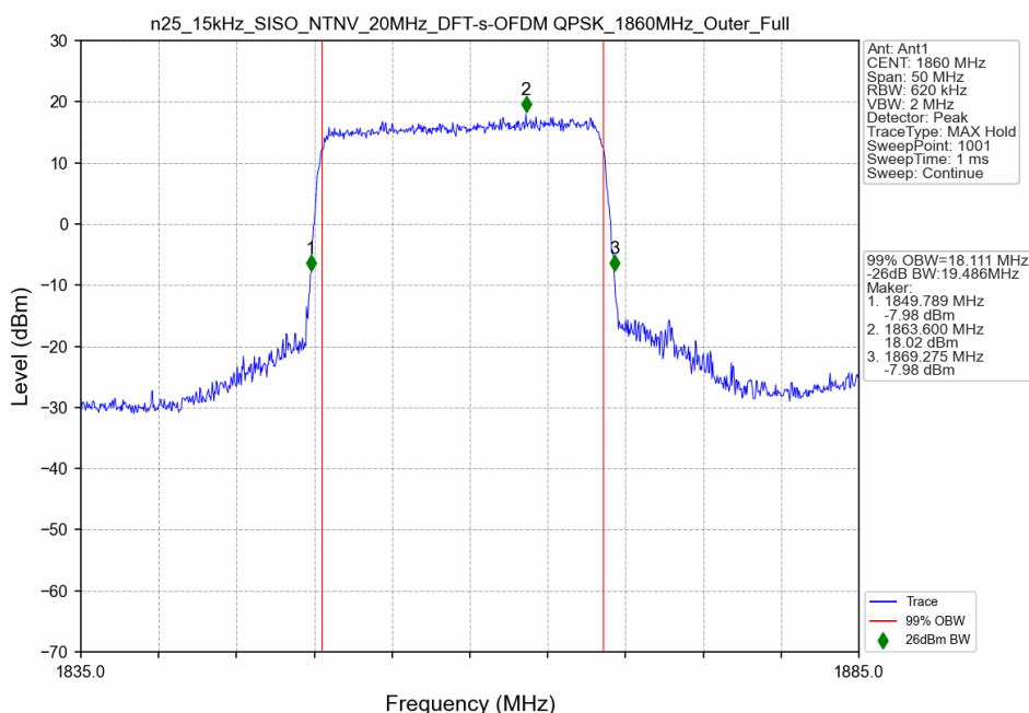
n25_15kHz_SISO_NTNV_20MHz_DFT-s-OFDM QPSK_1860MHz_Outer_Full
