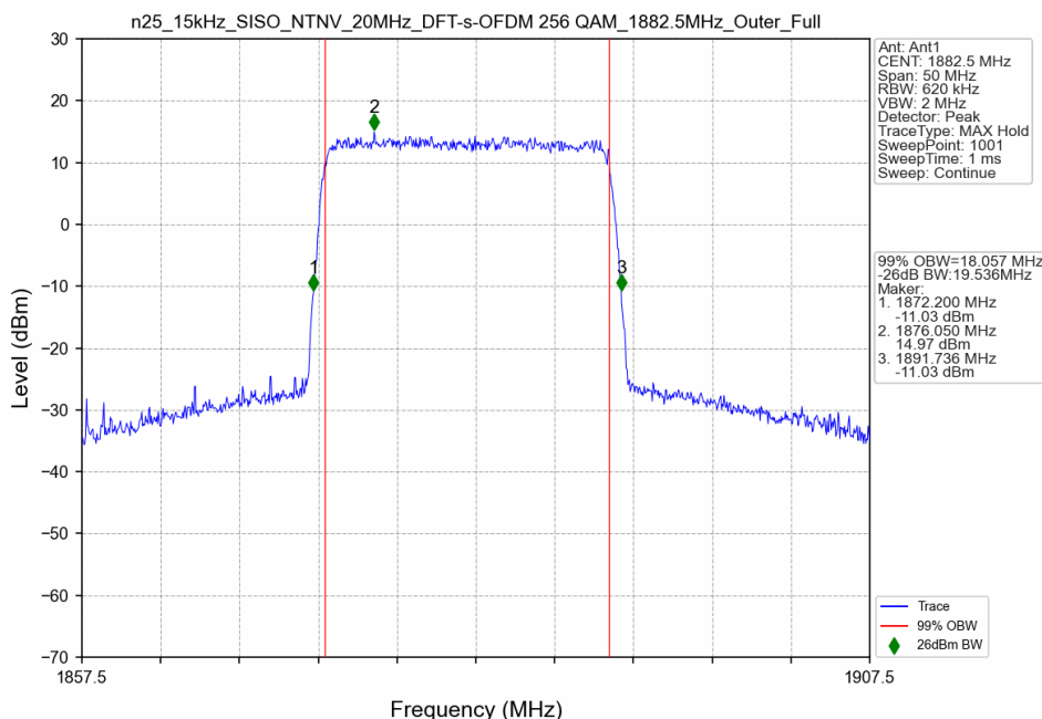
n25_15kHz_SISO_NTNV_20MHz_DFT-s-OFDM 256 QAM_1882.5MHz_Outer_Full
