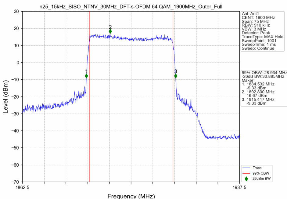
n25_15kHz_SISO_NTNV_30MHz_DFT-s-OFDM 64 QAM_1900MHz_Outer_Full
