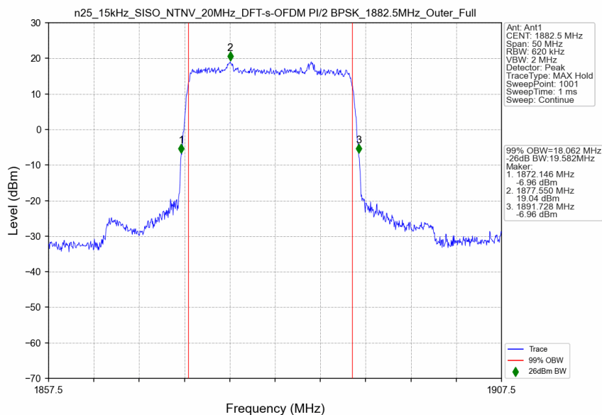
n25_15kHz_SISO_NTNV_20MHz_DFT-s-OFDM PI/2 BPSK_1882.5MHz_Outer_Full
