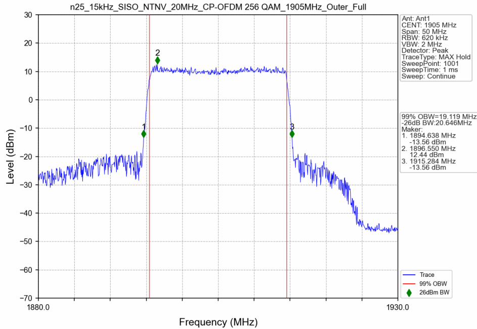
n25_15kHz_SISO_NTNV_20MHz_CP-OFDM 256 QAM_1905MHz_Outer_Full
