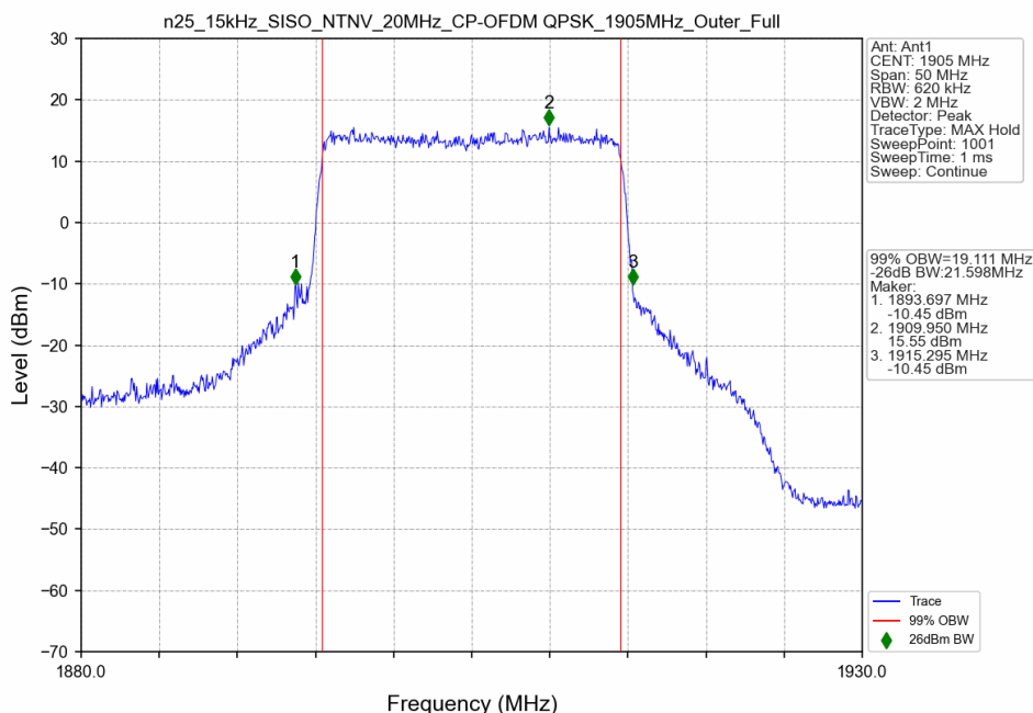
n25_15kHz_SISO_NTNV_20MHz_CP-OFDM QPSK_1905MHz_Outer_Full
