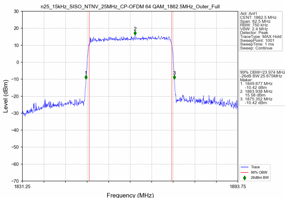
n25_15kHz_SISO_NTNV_25MHz_CP-OFDM 64 QAM_1862.5MHz_Outer_Full
