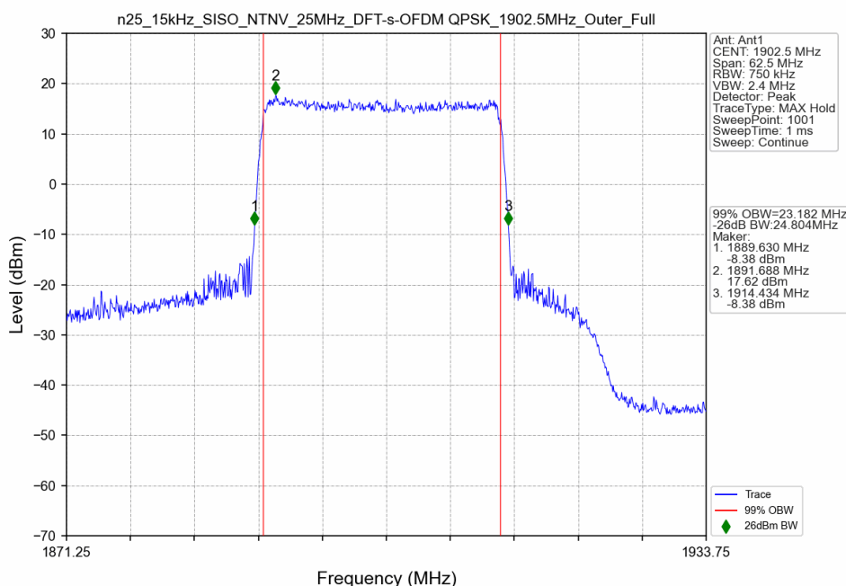
n25_15kHz_SISO_NTNV_25MHz_DFT-s-OFDM QPSK_1902.5MHz_Outer_Full
