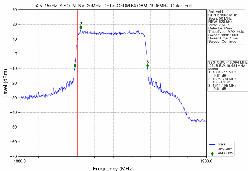
n25_15kHz_SISO_NTNV_20MHz_DFT-s-OFDM 64 QAM_1905MHz_Outer_Full
