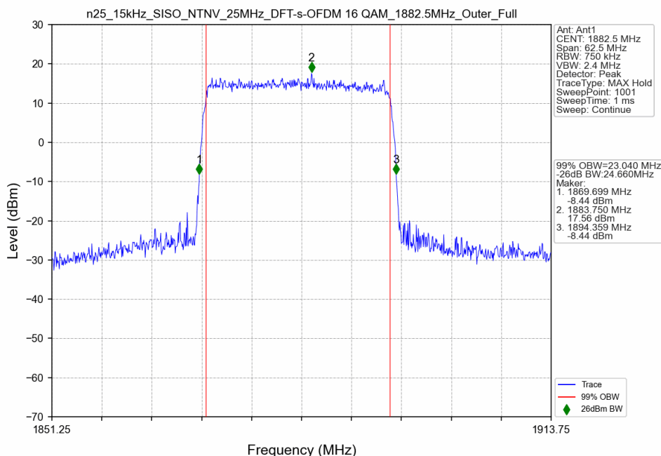
n25_15kHz_SISO_NTNV_25MHz_DFT-s-OFDM 16 QAM_1882.5MHz_Outer_Full
