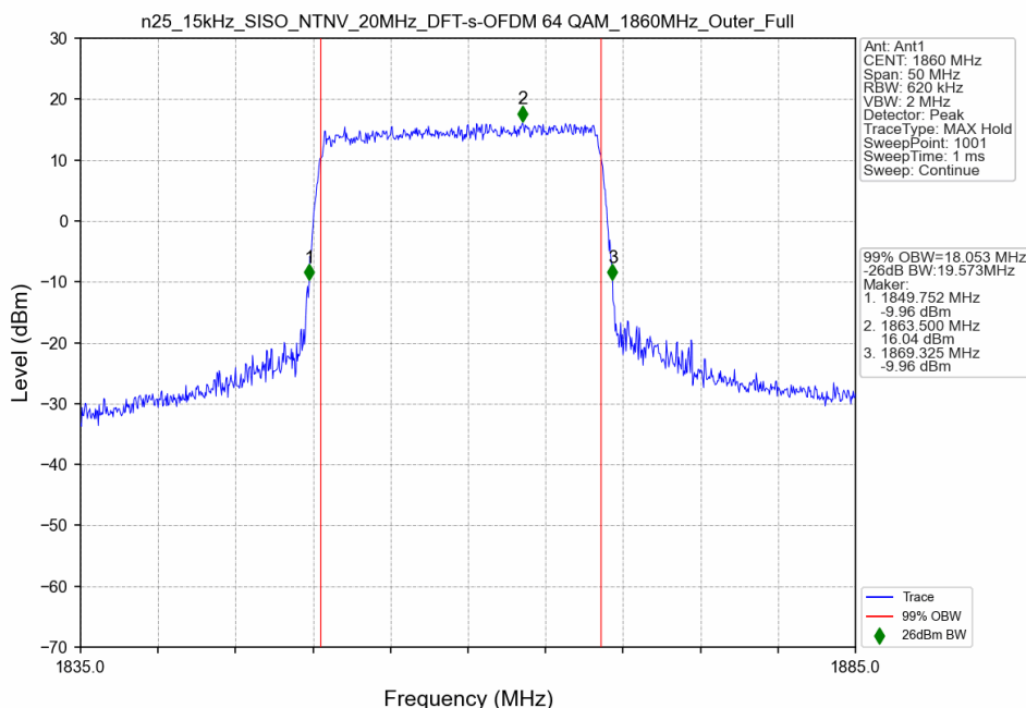
n25_15kHz_SISO_NTNV_20MHz_DFT-s-OFDM 64 QAM_1860MHz_Outer_Full
