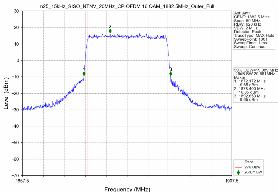
n25_15kHz_SISO_NTNV_20MHz_CP-OFDM 16 QAM_1882.5MHz_Outer_Full
