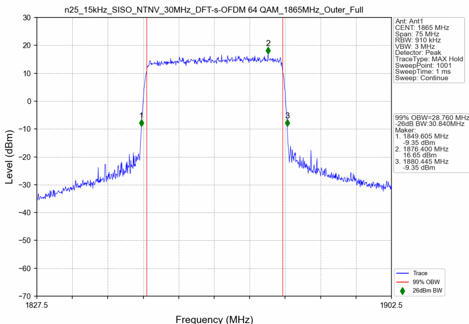
n25_15kHz_SISO_NTNV_30MHz_DFT-s-OFDM 64 QAM_1865MHz_Outer_Full
