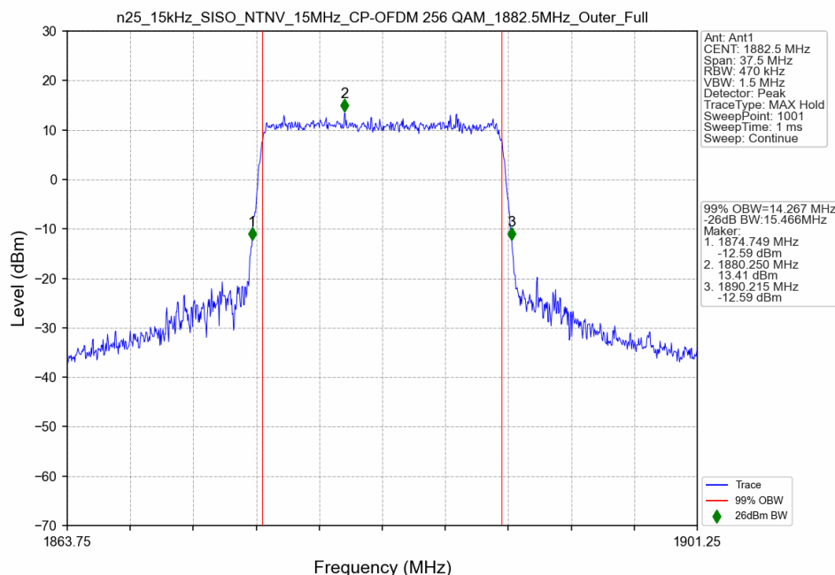
n25_15kHz_SISO_NTNV_15MHz_CP-OFDM 256 QAM_1882.5MHz_Outer_Full
