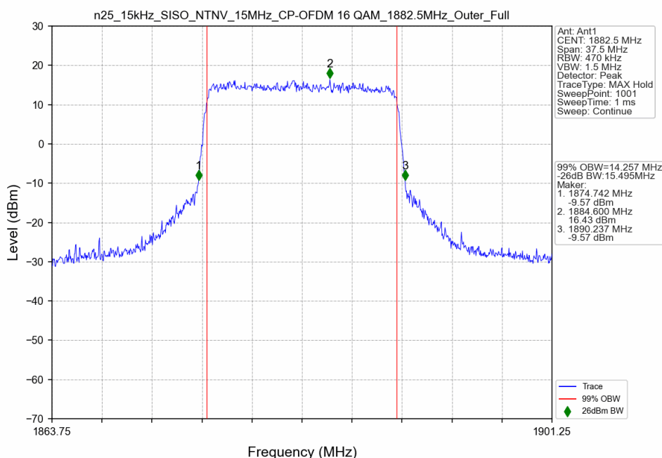
n25_15kHz_SISO_NTNV_15MHz_CP-OFDM 16 QAM_1882.5MHz_Outer_Full
