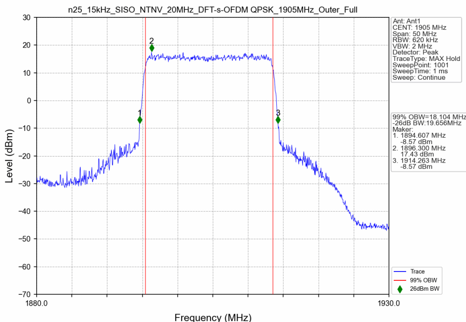
n25_15kHz_SISO_NTNV_20MHz_DFT-s-OFDM QPSK_1905MHz_Outer_Full
