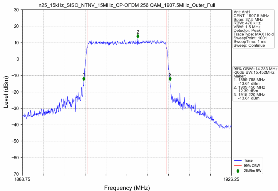
n25_15kHz_SISO_NTNV_15MHz_CP-OFDM 256 QAM_1907.5MHz_Outer_Full
