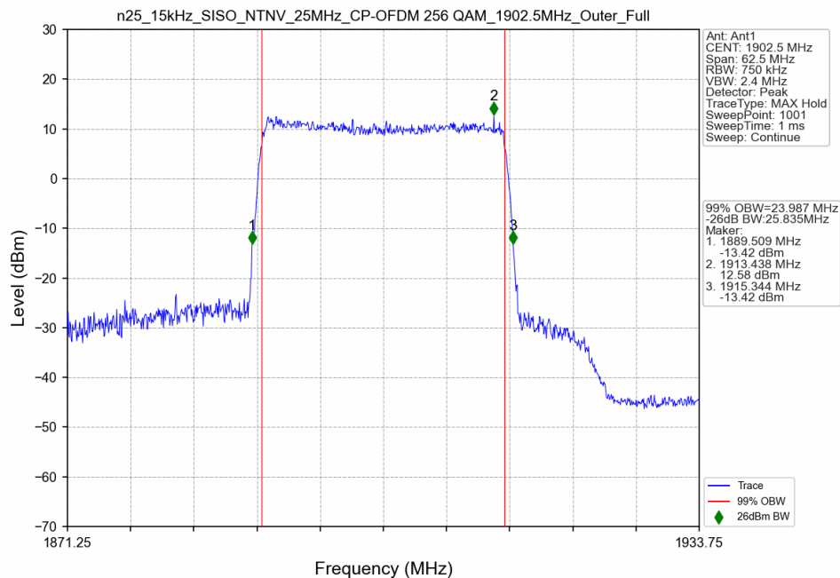
n25_15kHz_SISO_NTNV_25MHz_CP-OFDM 256 QAM_1902.5MHz_Outer_Full
