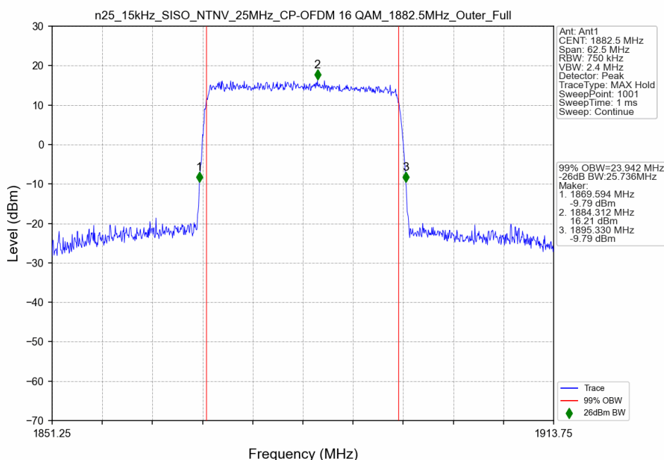
n25_15kHz_SISO_NTNV_25MHz_CP-OFDM 16 QAM_1882.5MHz_Outer_Full
