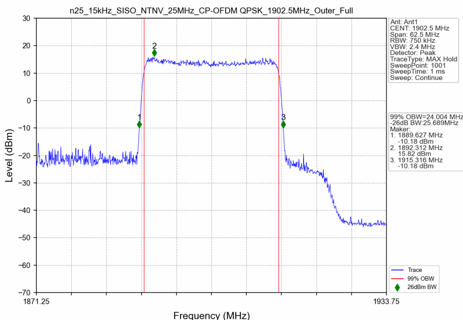
n25_15kHz_SISO_NTNV_25MHz_CP-OFDM QPSK_1902.5MHz_Outer_Full
