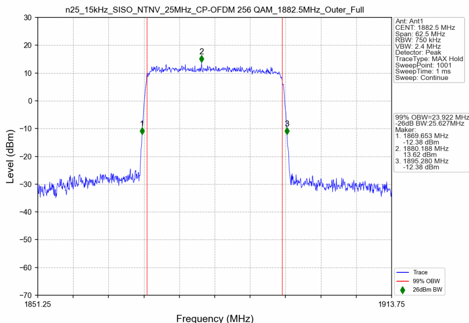
n25_15kHz_SISO_NTNV_25MHz_CP-OFDM 256 QAM_1882.5MHz_Outer_Full
