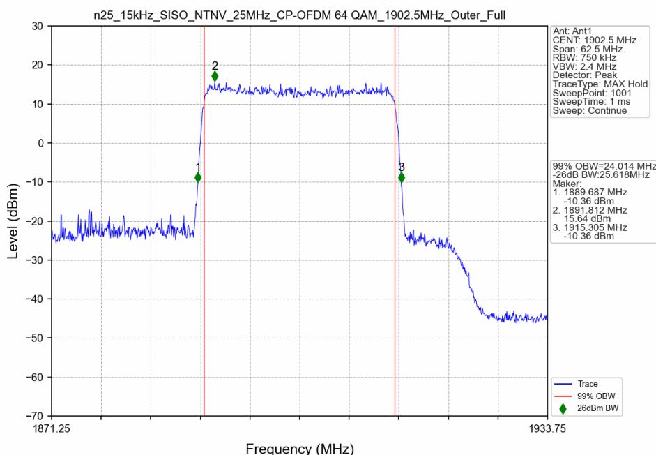
n25_15kHz_SISO_NTNV_25MHz_CP-OFDM 64 QAM_1902.5MHz_Outer_Full
