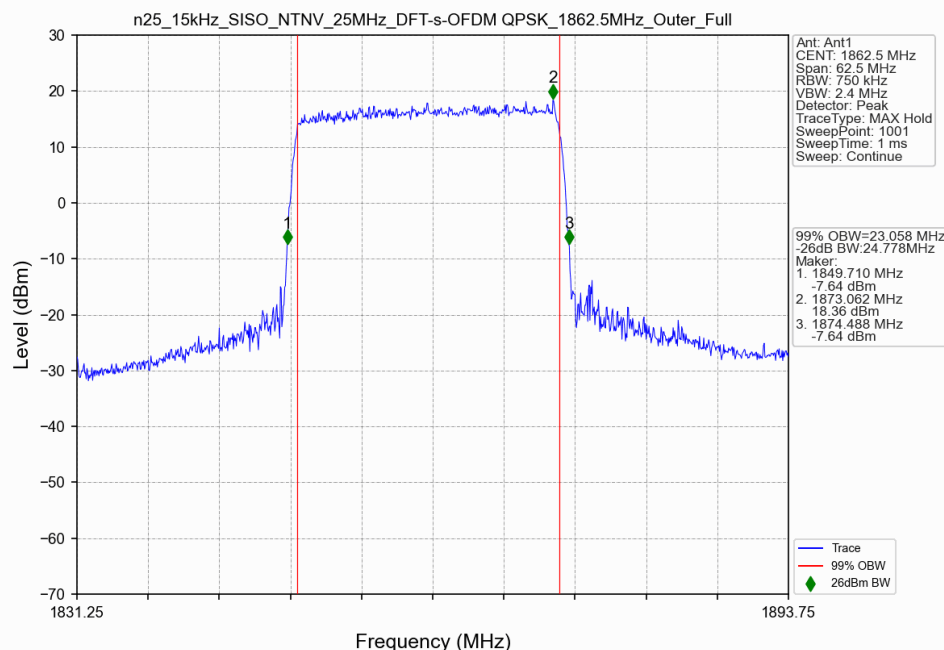
n25_15kHz_SISO_NTNV_25MHz_DFT-s-OFDM QPSK_1862.5MHz_Outer_Full
