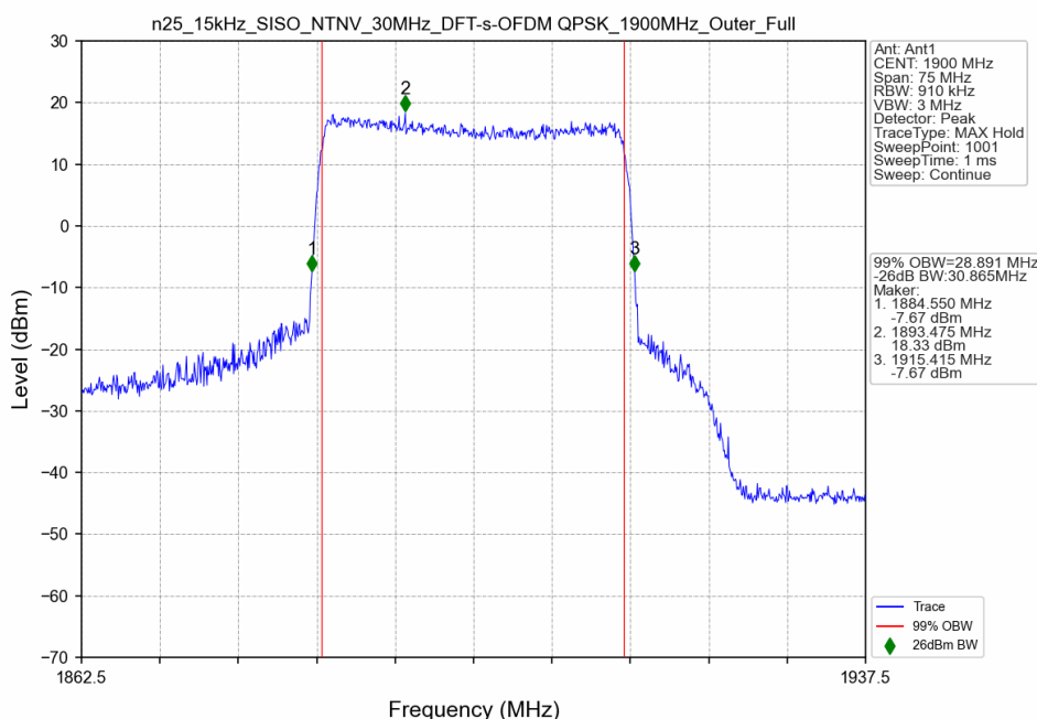
n25_15kHz_SISO_NTNV_30MHz_DFT-s-OFDM QPSK_1900MHz_Outer_Full
