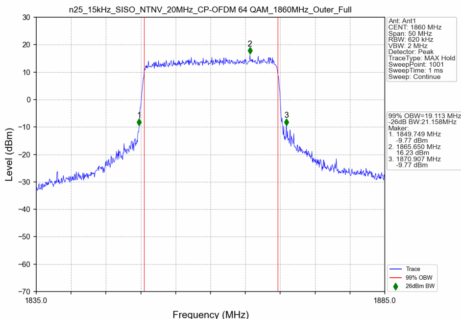
n25_15kHz_SISO_NTNV_20MHz_CP-OFDM 64 QAM_1860MHz_Outer_Full
