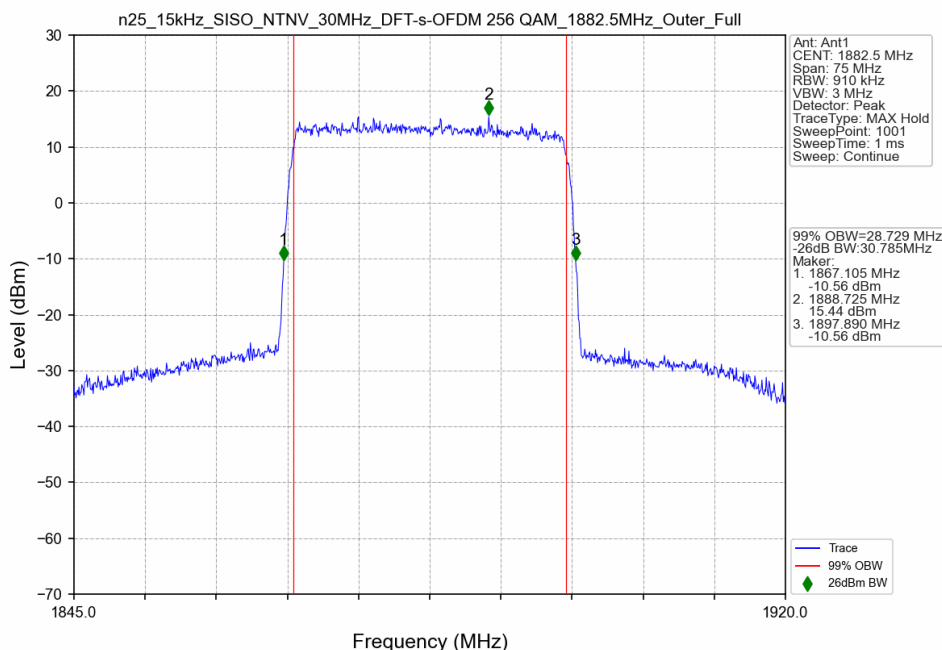
n25_15kHz_SISO_NTNV_30MHz_DFT-s-OFDM 256 QAM_1882.5MHz_Outer_Full
