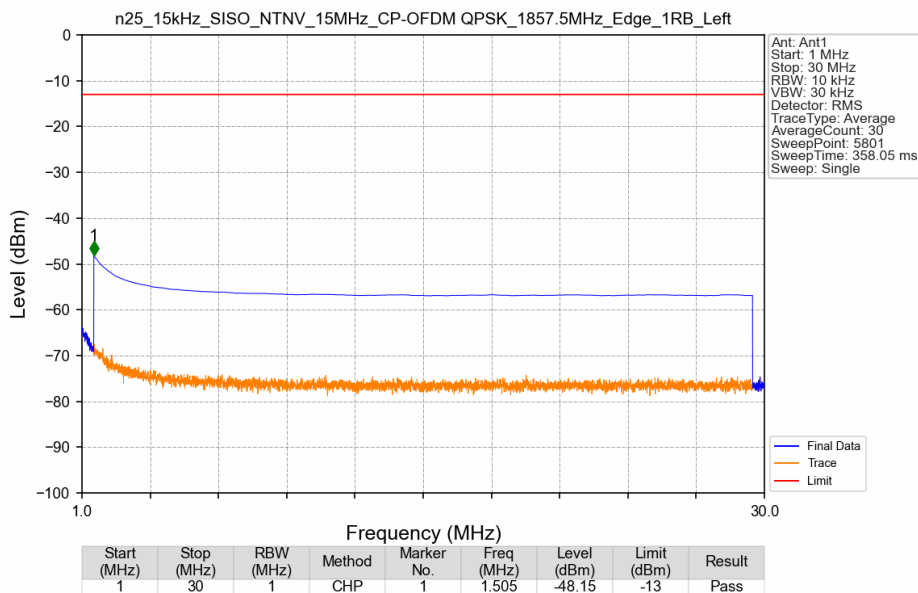
n25_15kHz_SISO_NTNV_15MHz_CP-OFDM QPSK_1857.5MHz_Edge_1RB_Left
