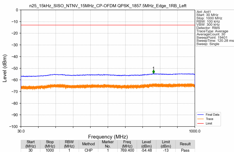
n25_15kHz_SISO_NTNV_15MHz_CP-OFDM QPSK_1857.5MHz_Edge_1RB_Left
