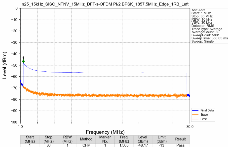
n25_15kHz_SISO_NTNV_15MHz_DFT-s-OFDM PI/2 BPSK_1857.5MHz_Edge_1RB_Left
