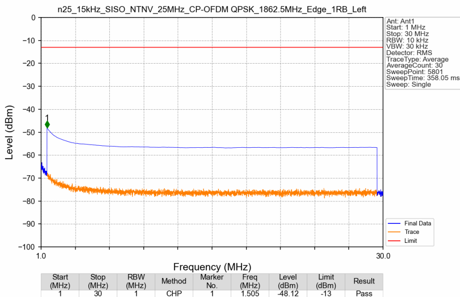
n25_15kHz_SISO_NTNV_25MHz_CP-OFDM QPSK_1862.5MHz_Edge_1RB_Left
