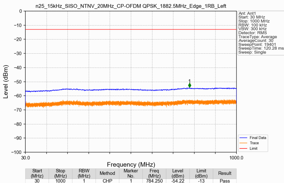
n25_15kHz_SISO_NTNV_20MHz_CP-OFDM QPSK_1882.5MHz_Edge_1RB_Left
