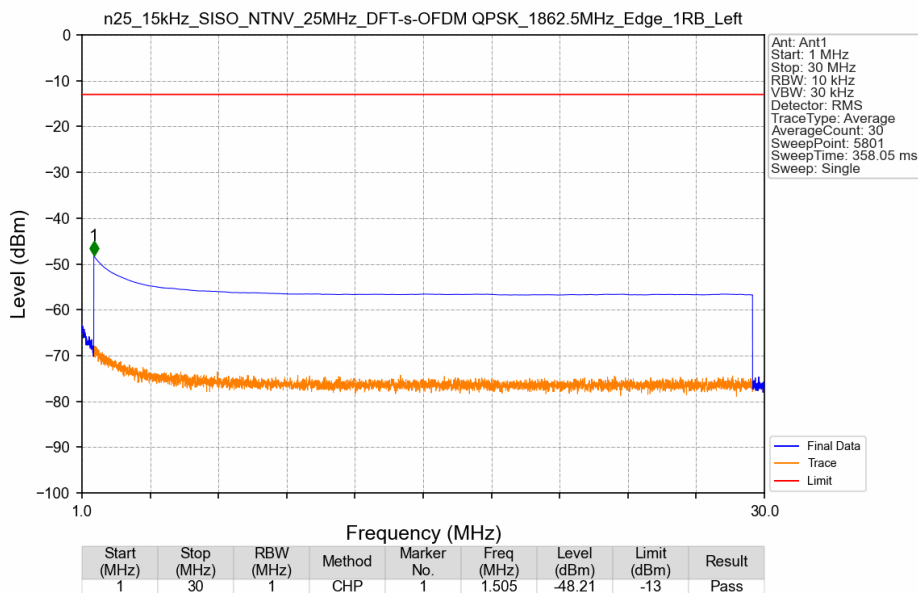
n25_15kHz_SISO_NTNV_25MHz_DFT-s-OFDM QPSK_1862.5MHz_Edge_1RB_Left
