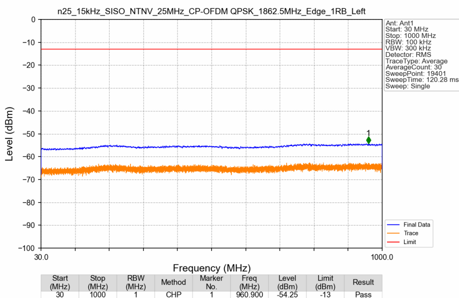
n25_15kHz_SISO_NTNV_25MHz_CP-OFDM QPSK_1862.5MHz_Edge_1RB_Left
