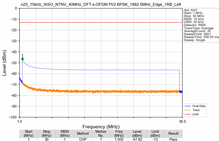
n25_15kHz_SISO_NTNV_40MHz_DFT-s-OFDM PI/2 BPSK_1882.5MHz_Edge_1RB_Left
