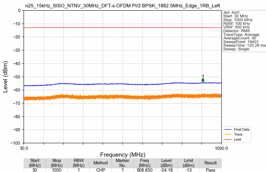
n25_15kHz_SISO_NTNV_30MHz_DFT-s-OFDM PI/2 BPSK_1882.5MHz_Edge_1RB_Left
