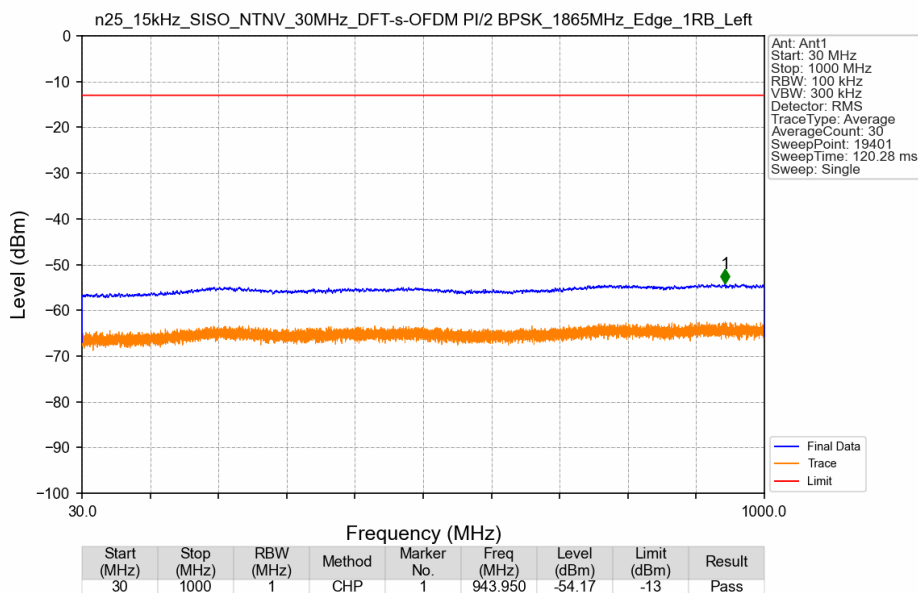
n25_15kHz_SISO_NTNV_30MHz_DFT-s-OFDM PI/2 BPSK_1865MHz_Edge_1RB_Left
