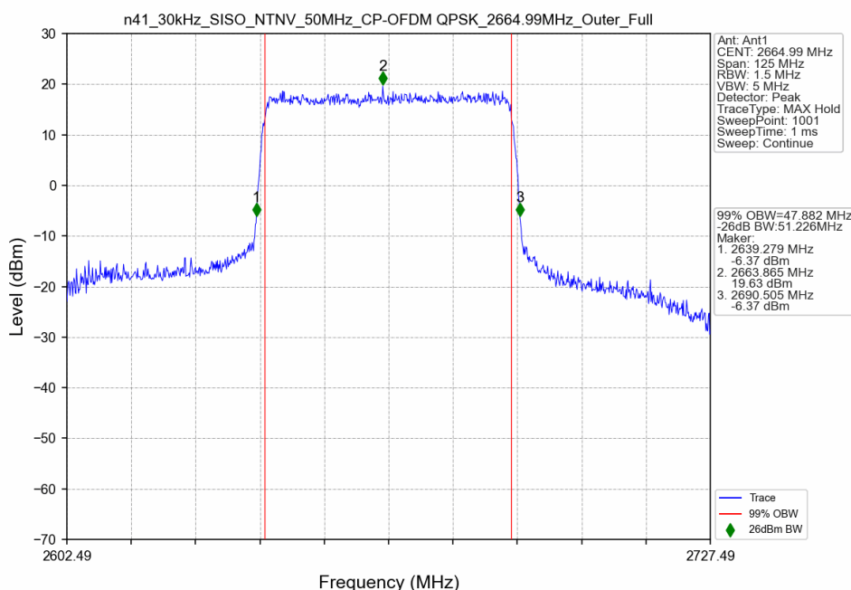
n41_30kHz_SISO_NTNV_50MHz_CP-OFDM QPSK_2664.99MHz_Outer_Full
