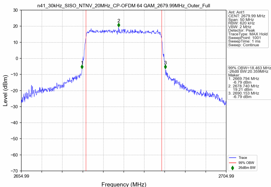
n41_30kHz_SISO_NTNV_20MHz_CP-OFDM 64 QAM_2679.99MHz_Outer_Full
