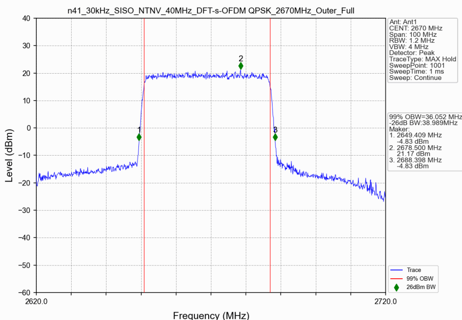
n41_30kHz_SISO_NTNV_40MHz_DFT-s-OFDM QPSK_2670MHz_Outer_Full
