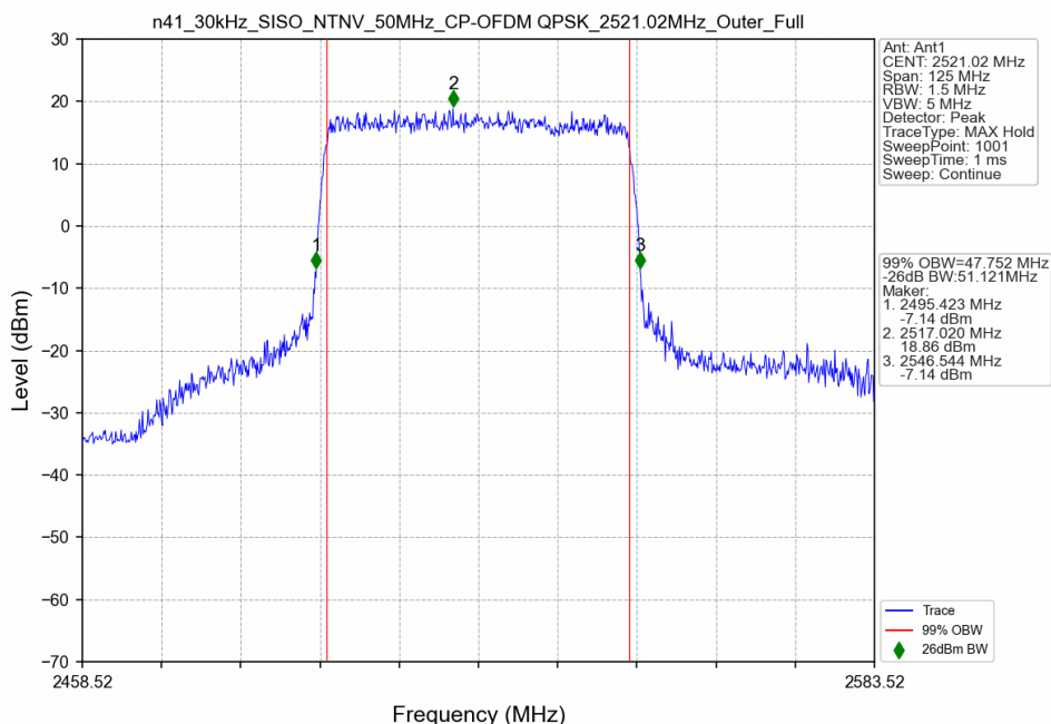
n41_30kHz_SISO_NTNV_50MHz_CP-OFDM QPSK_2521.02MHz_Outer_Full
