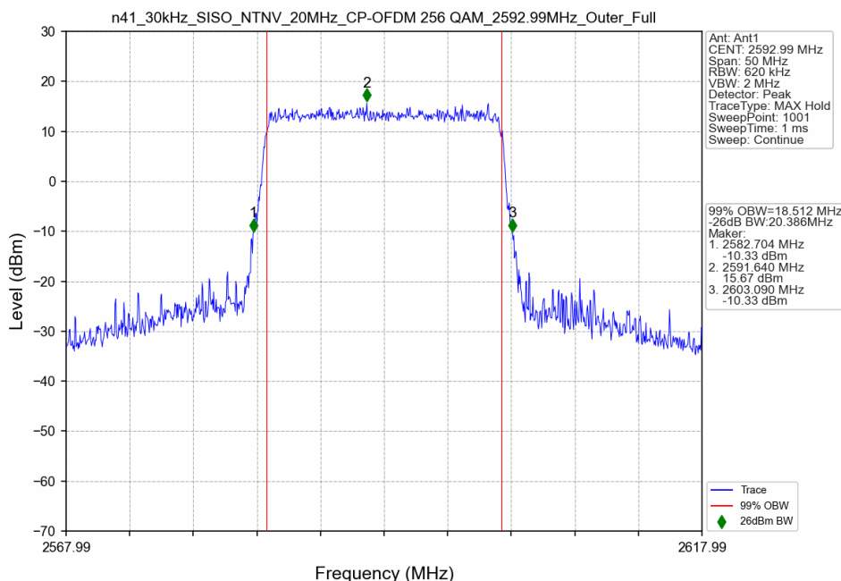
n41_30kHz_SISO_NTNV_20MHz_CP-OFDM 256 QAM_2592.99MHz_Outer_Full
