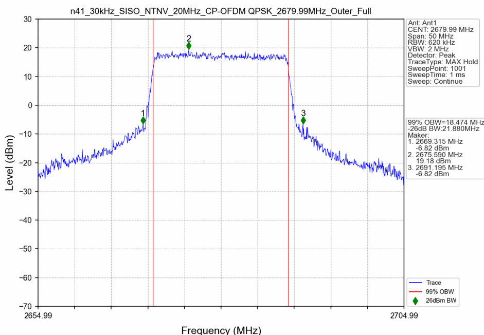
n41_30kHz_SISO_NTNV_20MHz_CP-OFDM QPSK_2679.99MHz_Outer_Full
