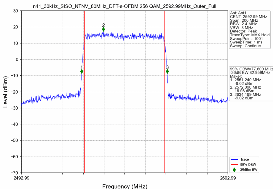
n41_30kHz_SISO_NTNV_80MHz_DFT-s-OFDM 256 QAM_2592.99MHz_Outer_Full
