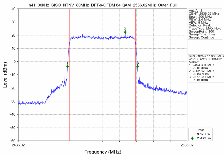
n41_30kHz_SISO_NTNV_80MHz_DFT-s-OFDM 64 QAM_2536.02MHz_Outer_Full
