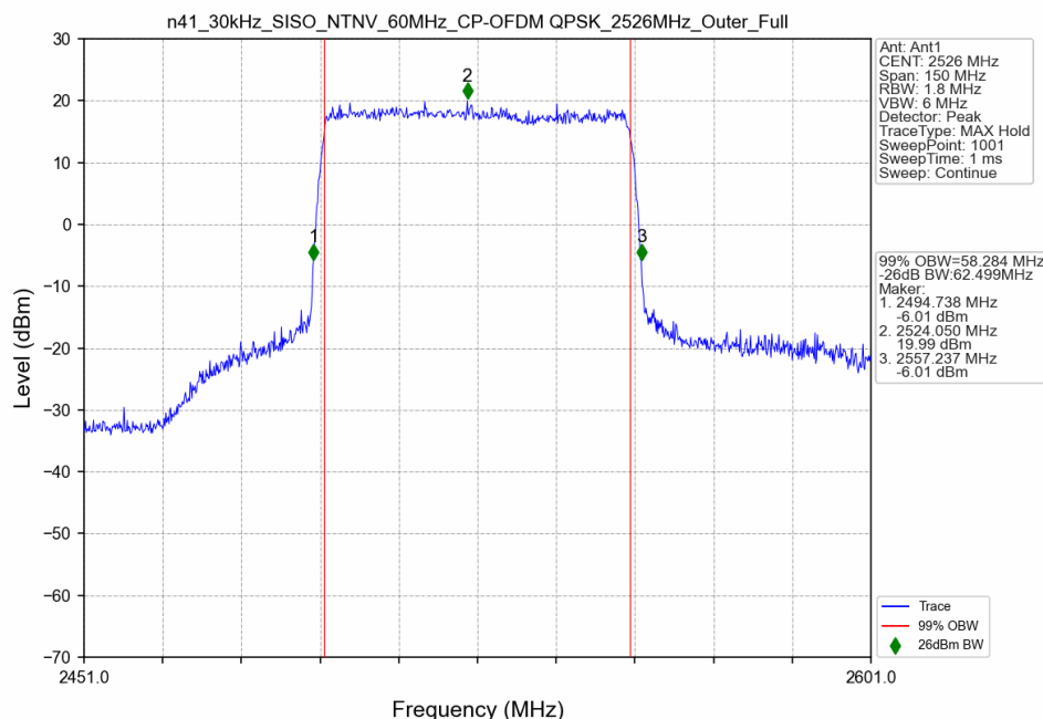
n41_30kHz_SISO_NTNV_60MHz_CP-OFDM QPSK_2526MHz_Outer_Full
