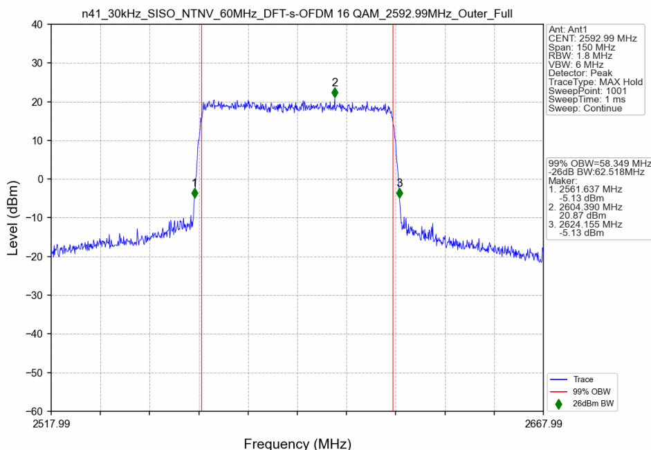
n41_30kHz_SISO_NTNV_60MHz_DFT-s-OFDM 16 QAM_2592.99MHz_Outer_Full
