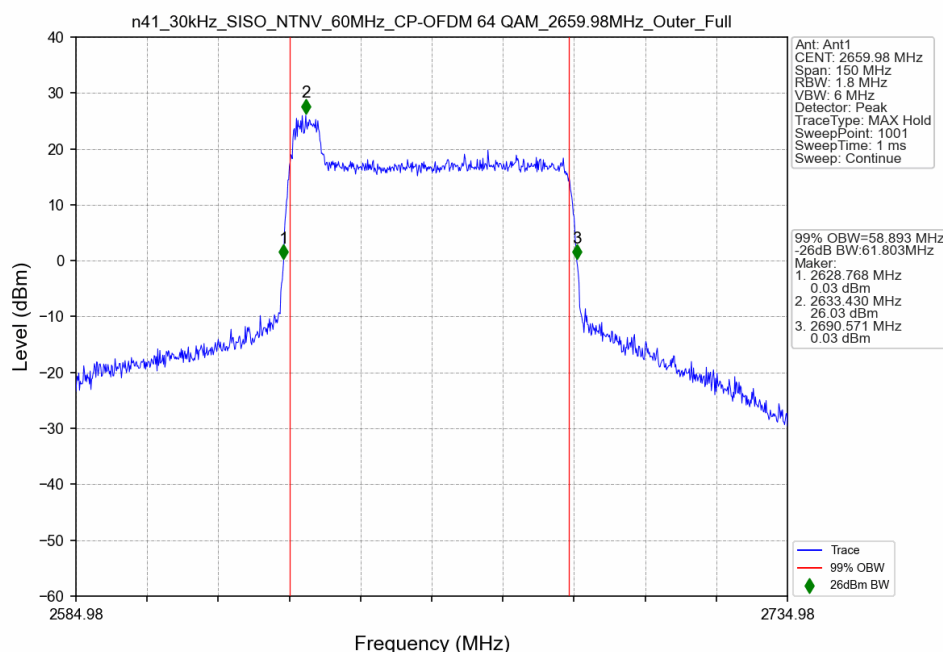
n41_30kHz_SISO_NTNV_60MHz_CP-OFDM 64 QAM_2659.98MHz_Outer_Full
