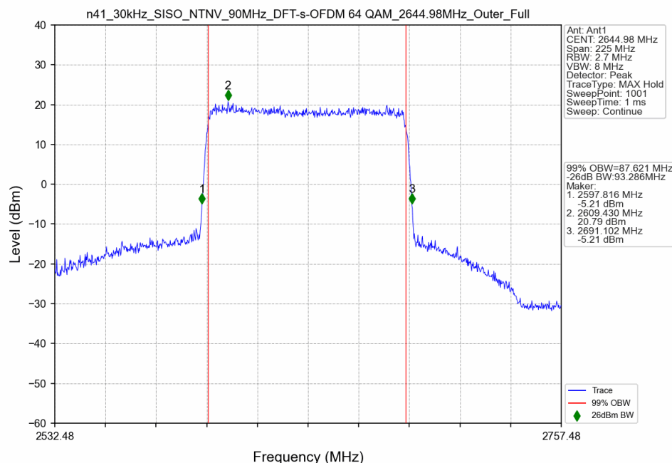
n41_30kHz_SISO_NTNV_90MHz_DFT-s-OFDM 64 QAM_2644.98MHz_Outer_Full
