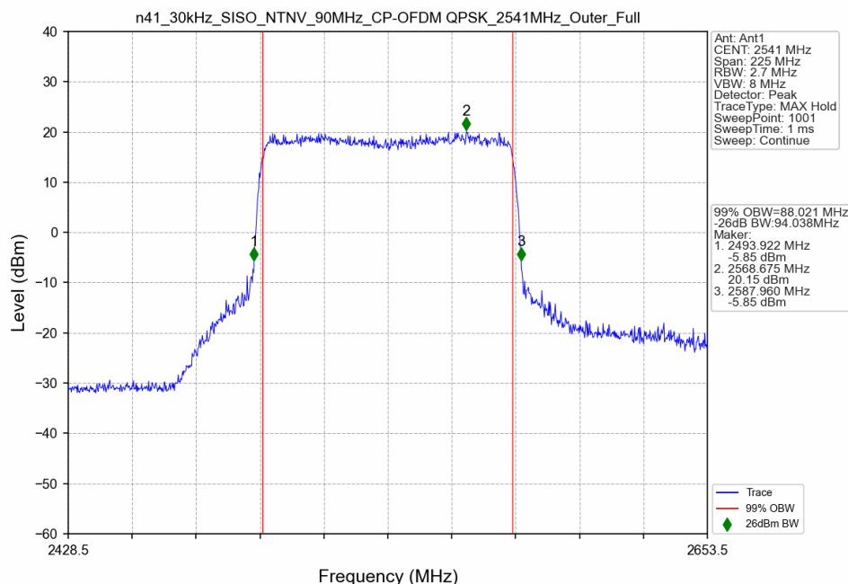
n41_30kHz_SISO_NTNV_90MHz_CP-OFDM QPSK_2541MHz_Outer_Full
