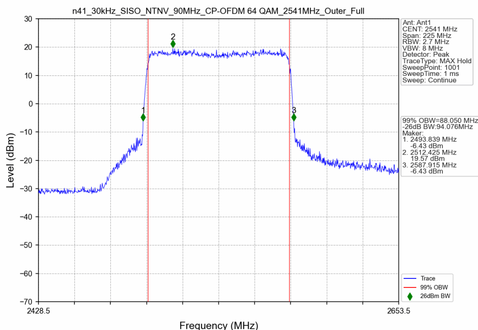
n41_30kHz_SISO_NTNV_90MHz_CP-OFDM 64 QAM_2541MHz_Outer_Full
