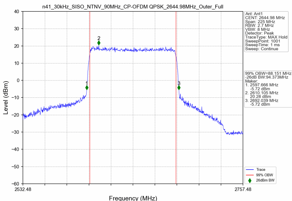
n41_30kHz_SISO_NTNV_90MHz_CP-OFDM QPSK_2644.98MHz_Outer_Full
