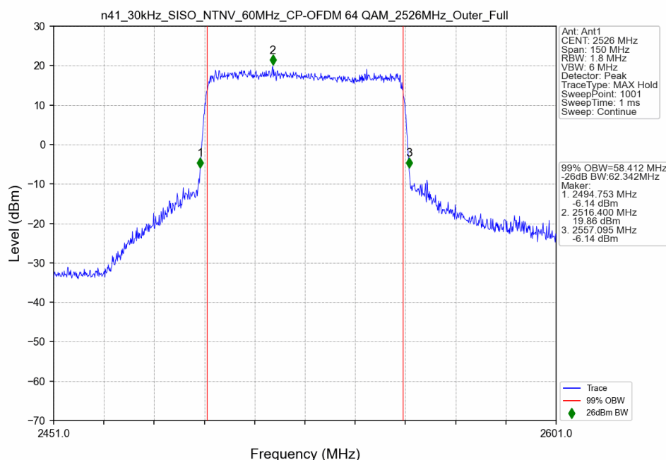
n41_30kHz_SISO_NTNV_60MHz_CP-OFDM 64 QAM_2526MHz_Outer_Full
