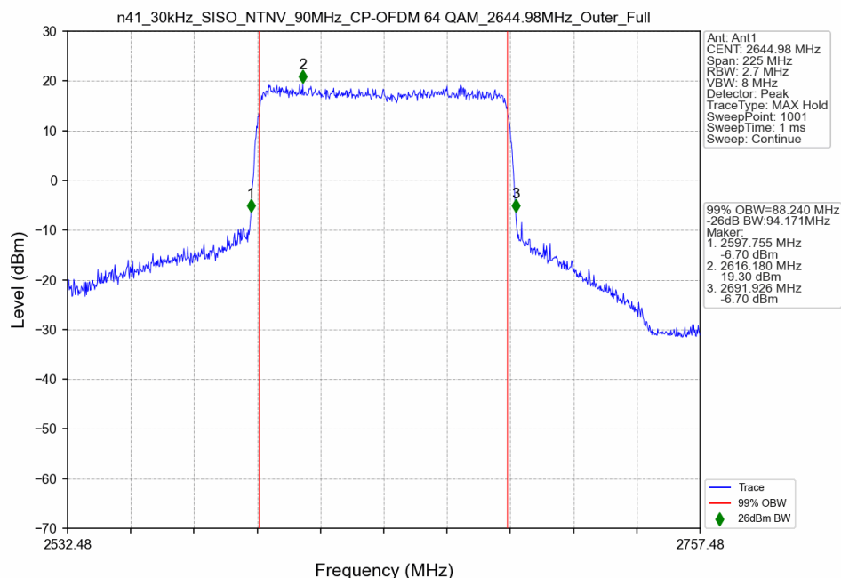
n41_30kHz_SISO_NTNV_90MHz_CP-OFDM 64 QAM_2644.98MHz_Outer_Full
