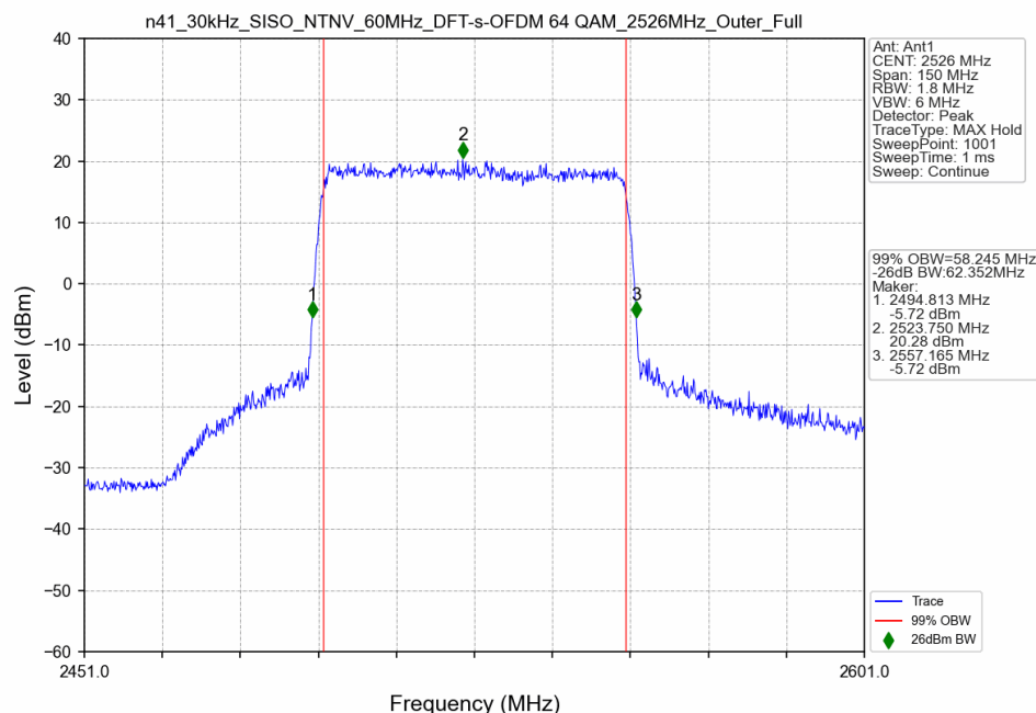
n41_30kHz_SISO_NTNV_60MHz_DFT-s-OFDM 64 QAM_2526MHz_Outer_Full
