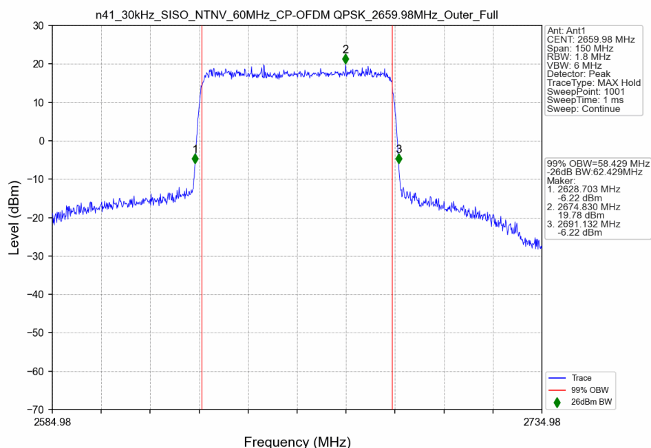
n41_30kHz_SISO_NTNV_60MHz_CP-OFDM QPSK_2659.98MHz_Outer_Full
