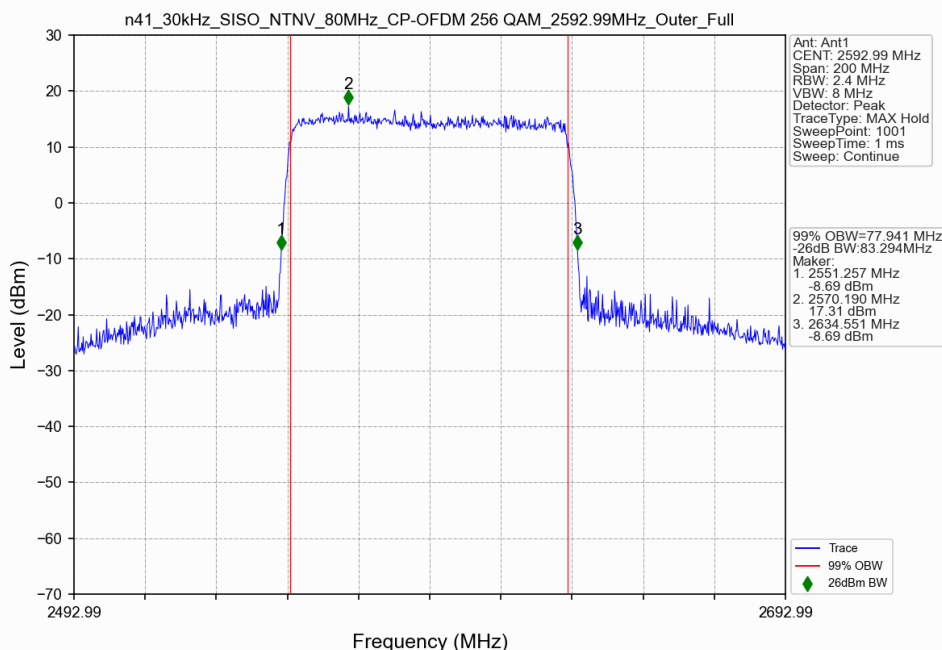
n41_30kHz_SISO_NTNV_80MHz_CP-OFDM 256 QAM_2592.99MHz_Outer_Full
