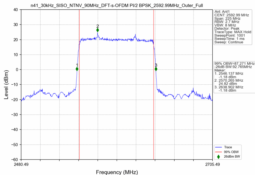
n41_30kHz_SISO_NTNV_90MHz_DFT-s-OFDM PI/2 BPSK_2592.99MHz_Outer_Full
