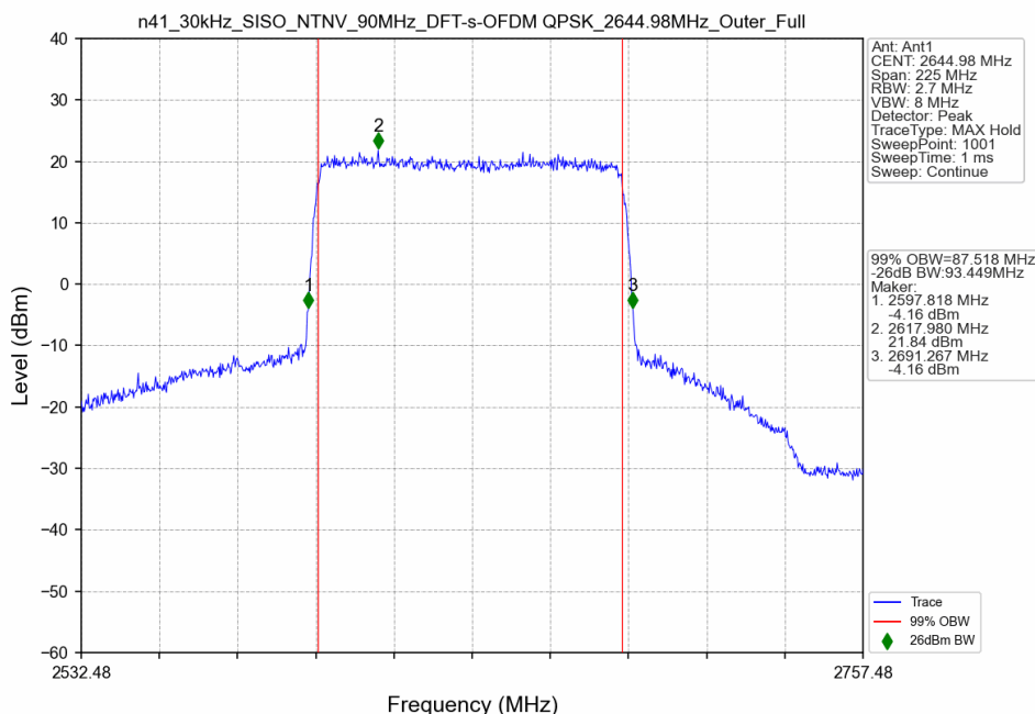
n41_30kHz_SISO_NTNV_90MHz_DFT-s-OFDM QPSK_2644.98MHz_Outer_Full
