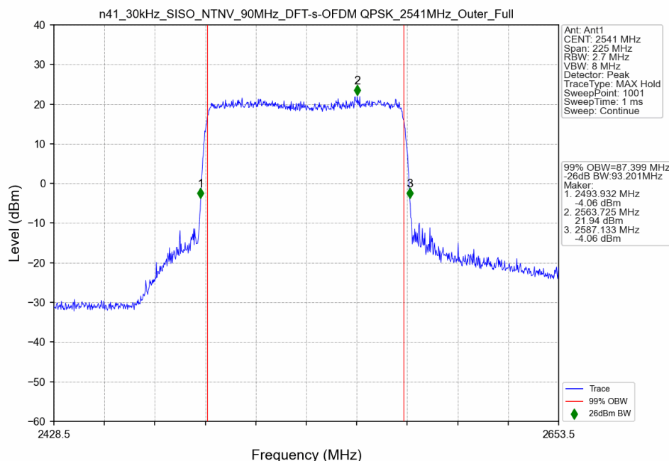
n41_30kHz_SISO_NTNV_90MHz_DFT-s-OFDM QPSK_2541MHz_Outer_Full
