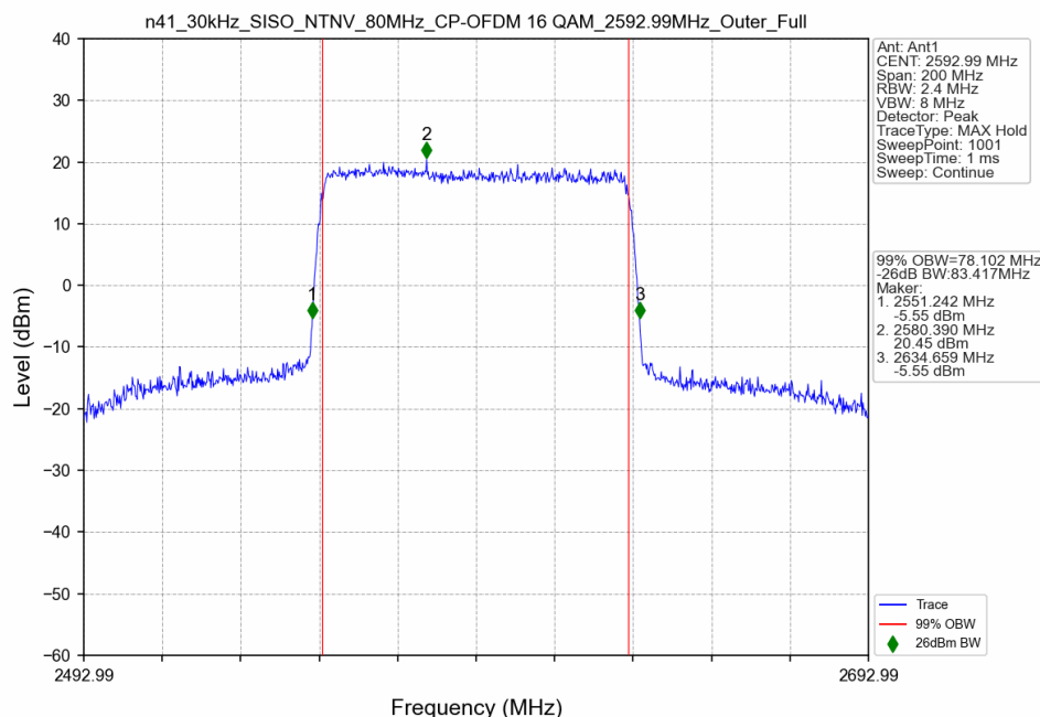
n41_30kHz_SISO_NTNV_80MHz_CP-OFDM 16 QAM_2592.99MHz_Outer_Full
