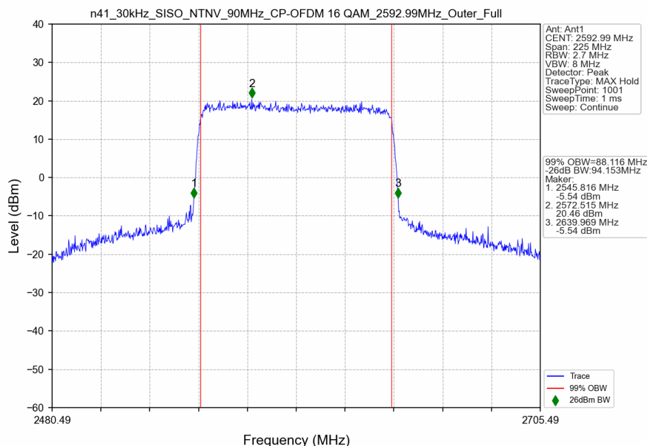
n41_30kHz_SISO_NTNV_90MHz_CP-OFDM 16 QAM_2592.99MHz_Outer_Full
