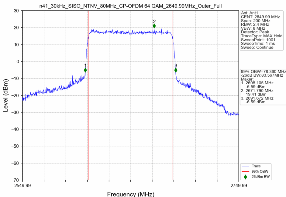
n41_30kHz_SISO_NTNV_80MHz_CP-OFDM 64 QAM_2649.99MHz_Outer_Full
