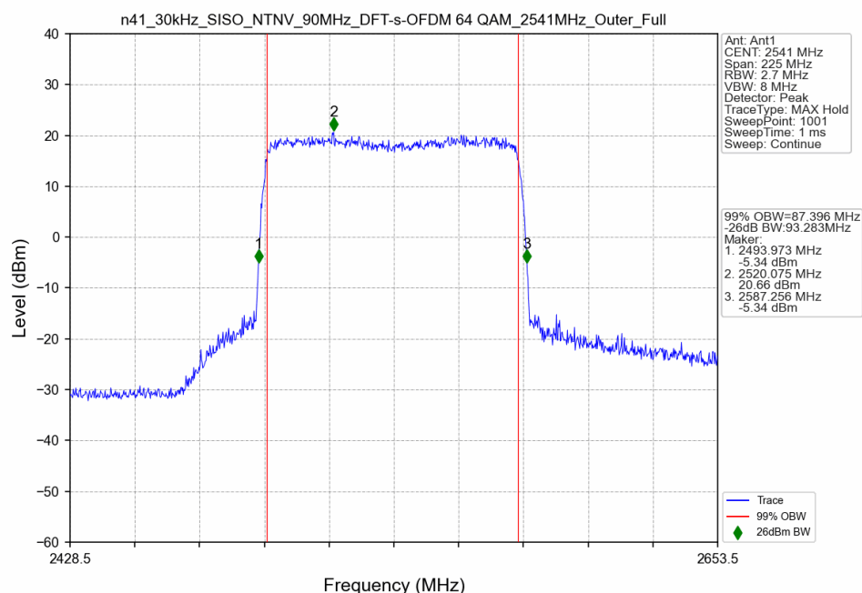
n41_30kHz_SISO_NTNV_90MHz_DFT-s-OFDM 64 QAM_2541MHz_Outer_Full
