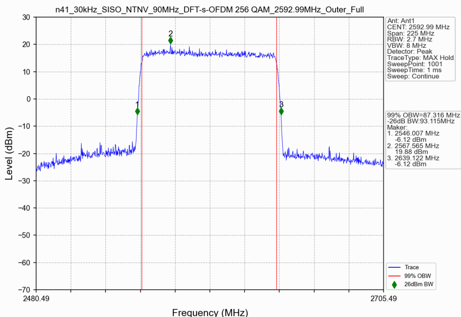
n41_30kHz_SISO_NTNV_90MHz_DFT-s-OFDM 256 QAM_2592.99MHz_Outer_Full
