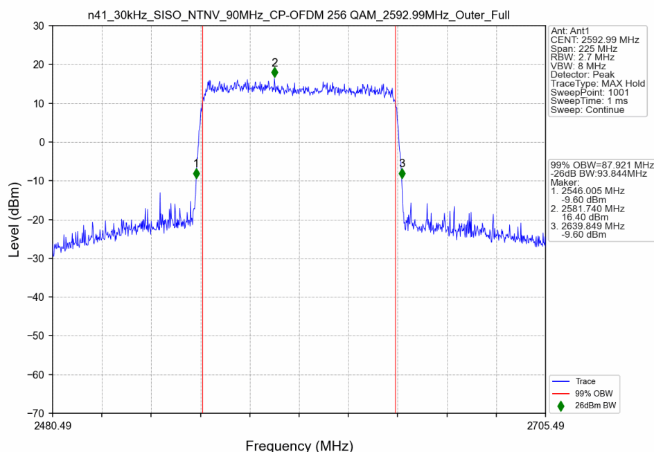
n41_30kHz_SISO_NTNV_90MHz_CP-OFDM 256 QAM_2592.99MHz_Outer_Full
