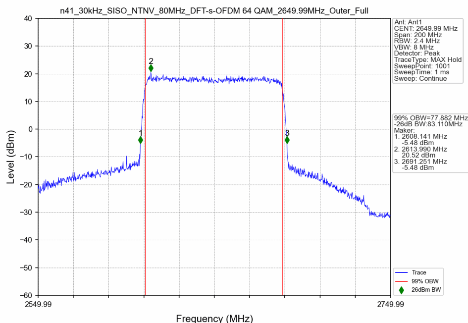
n41_30kHz_SISO_NTNV_80MHz_DFT-s-OFDM 64 QAM_2649.99MHz_Outer_Full
