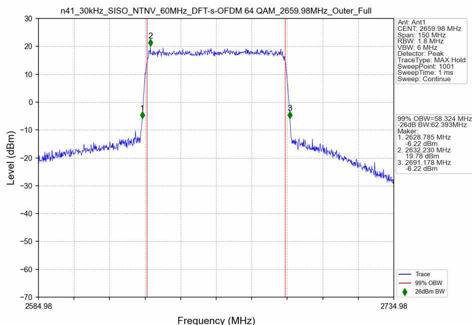
n41_30kHz_SISO_NTNV_60MHz_DFT-s-OFDM 64 QAM_2659.98MHz_Outer_Full
