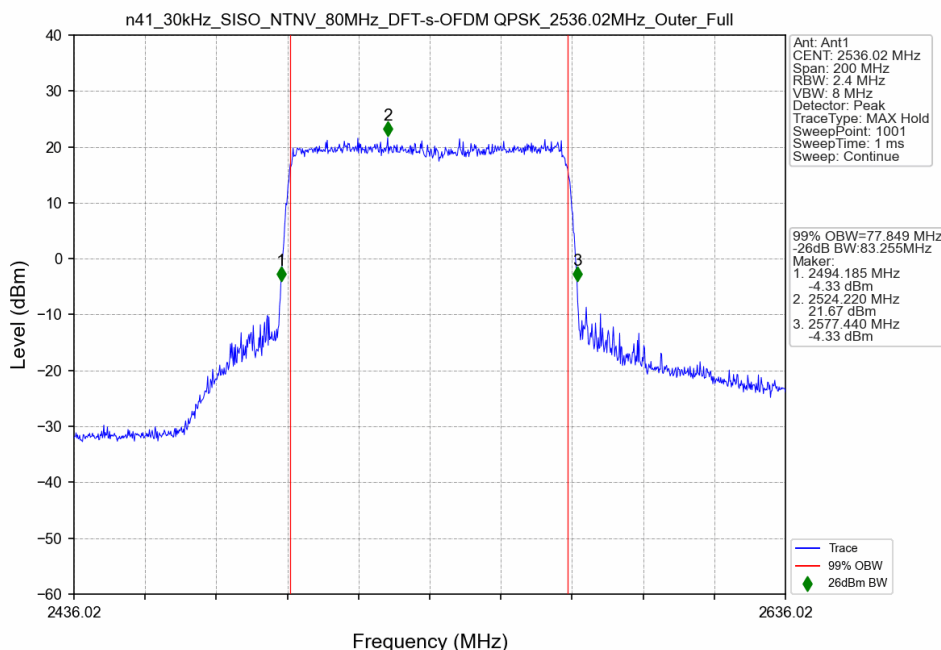
n41_30kHz_SISO_NTNV_80MHz_DFT-s-OFDM QPSK_2536.02MHz_Outer_Full
