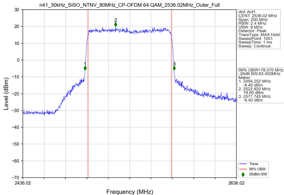
n41_30kHz_SISO_NTNV_80MHz_CP-OFDM 64 QAM_2536.02MHz_Outer_Full
