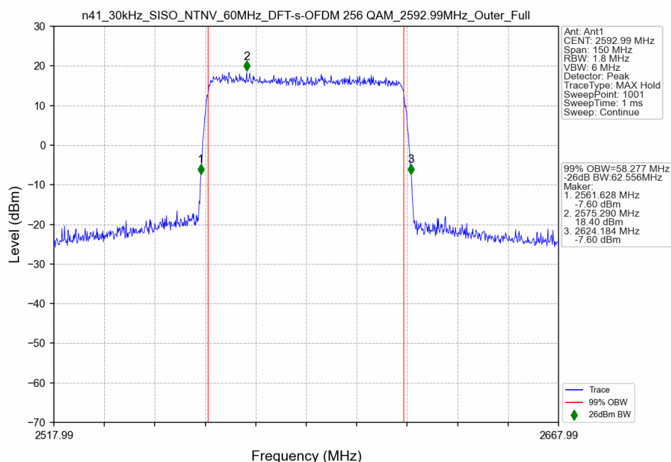
n41_30kHz_SISO_NTNV_60MHz_DFT-s-OFDM 256 QAM_2592.99MHz_Outer_Full
