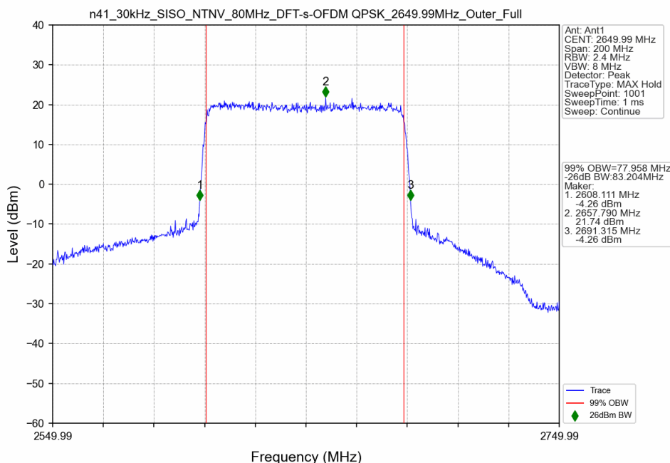
n41_30kHz_SISO_NTNV_80MHz_DFT-s-OFDM QPSK_2649.99MHz_Outer_Full
