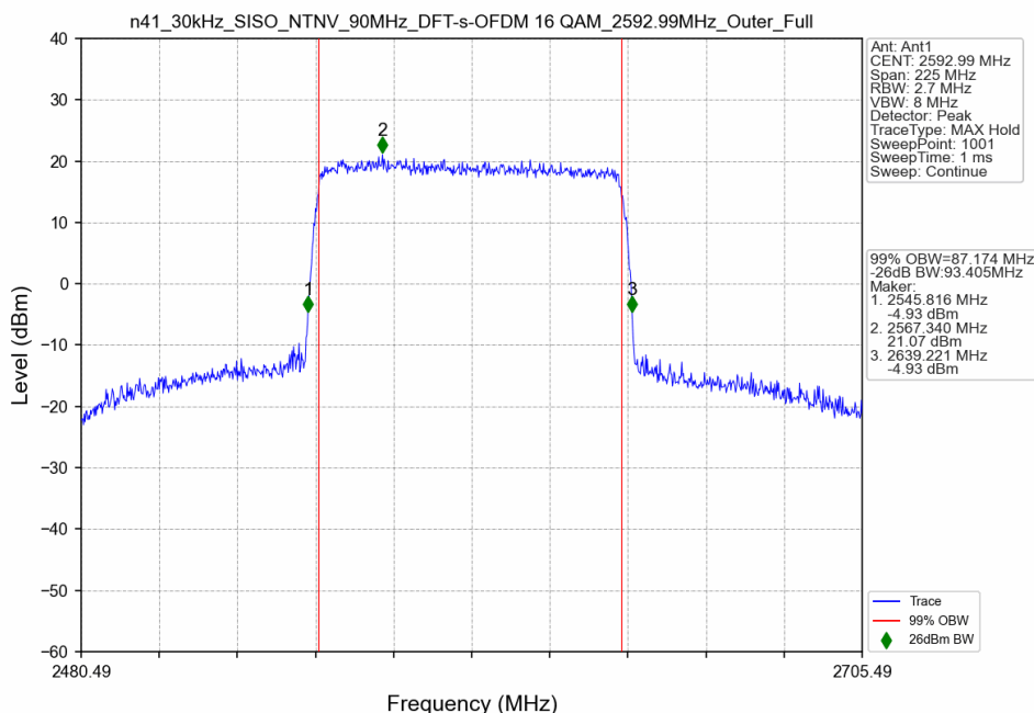
n41_30kHz_SISO_NTNV_90MHz_DFT-s-OFDM 16 QAM_2592.99MHz_Outer_Full
