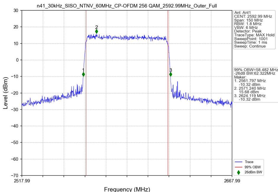
n41_30kHz_SISO_NTNV_60MHz_CP-OFDM 256 QAM_2592.99MHz_Outer_Full
