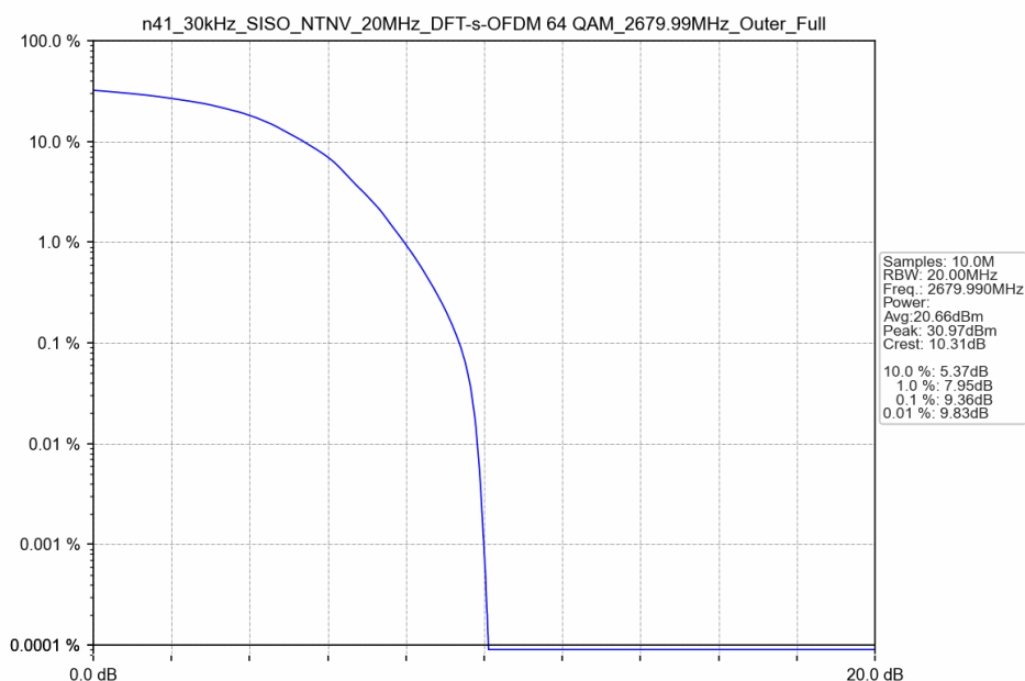
n41_30kHz_SISO_NTNV_20MHz_DFT-s-OFDM 64 QAM_2679.99MHz_Outer_Full
