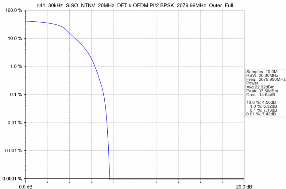
n41_30kHz_SISO_NTNV_20MHz_DFT-s-OFDM PI/2 BPSK_2679.99MHz_Outer_Full
