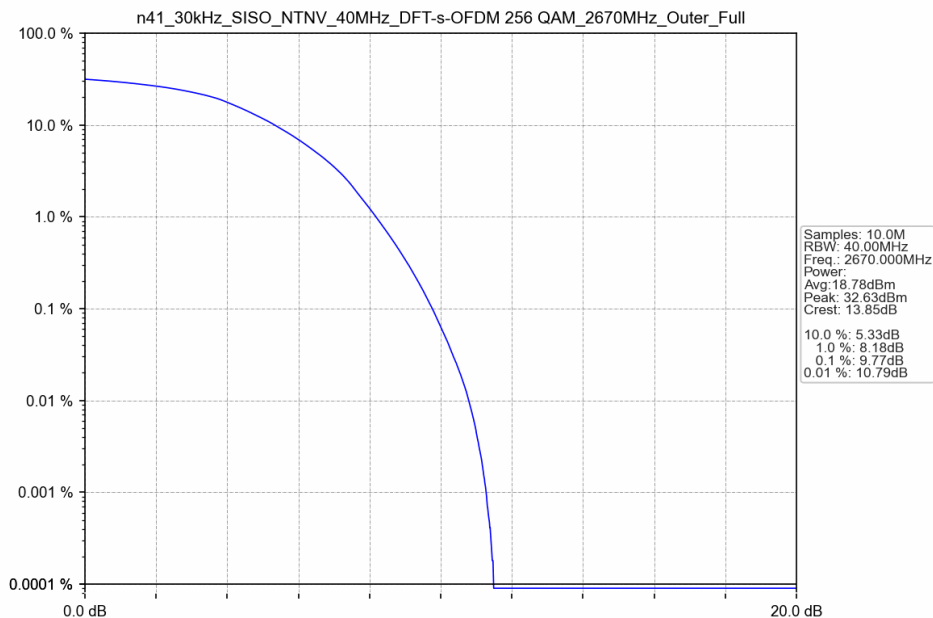
n41_30kHz_SISO_NTNV_40MHz_DFT-s-OFDM 256 QAM_2670MHz_Outer_Full
