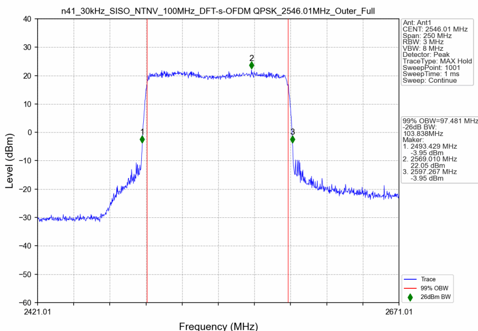
n41_30kHz_SISO_NTNV_100MHz_DFT-s-OFDM QPSK_2546.01MHz_Outer_Full
