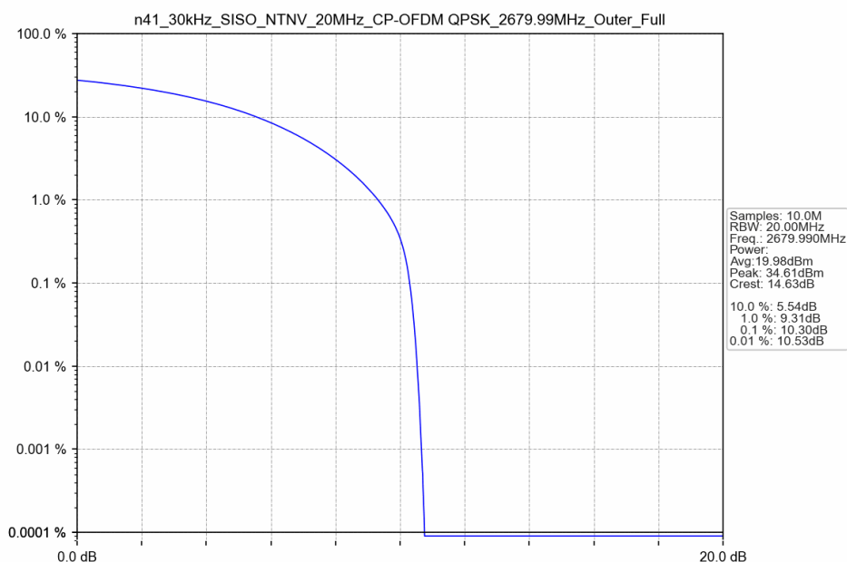
n41_30kHz_SISO_NTNV_20MHz_CP-OFDM QPSK_2679.99MHz_Outer_Full
