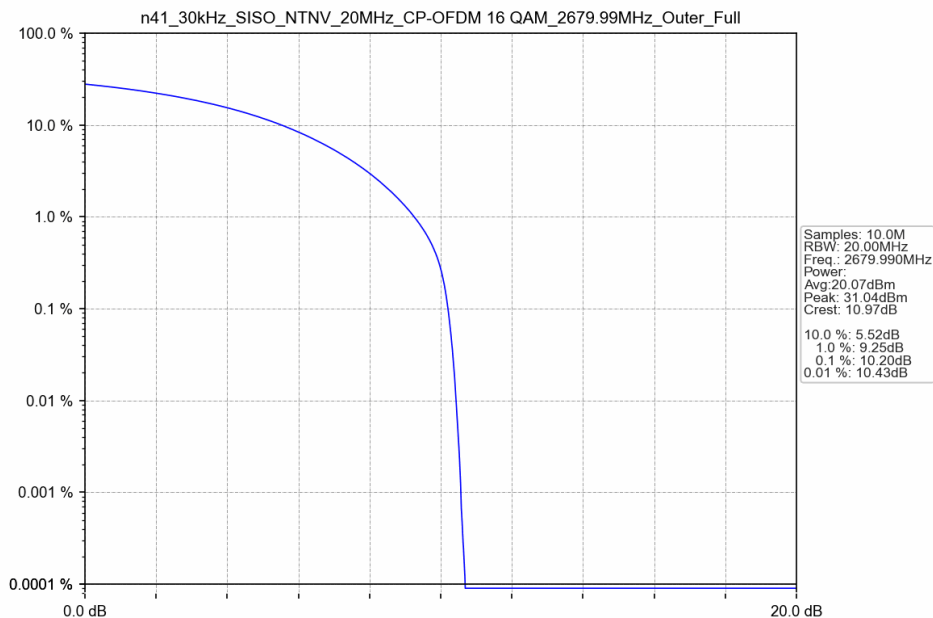
n41_30kHz_SISO_NTNV_20MHz_CP-OFDM 16 QAM_2679.99MHz_Outer_Full
