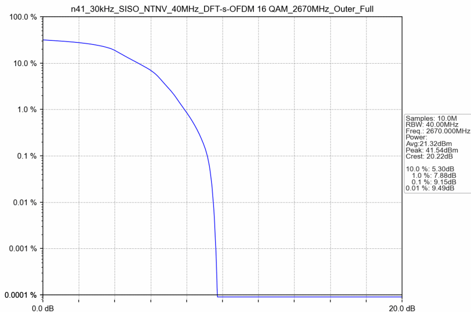
n41_30kHz_SISO_NTNV_40MHz_DFT-s-OFDM 16 QAM_2670MHz_Outer_Full
