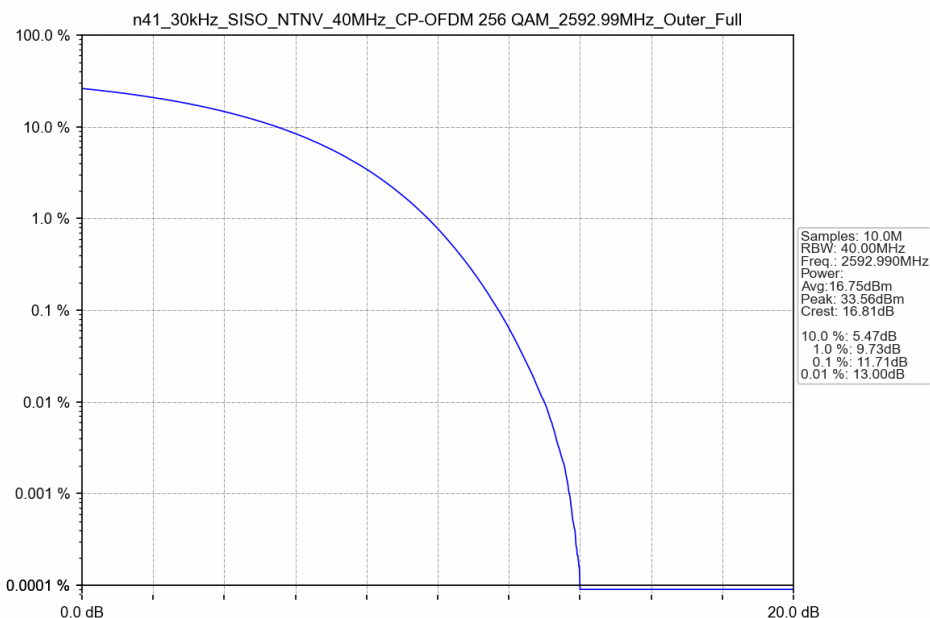
n41_30kHz_SISO_NTNV_40MHz_CP-OFDM 256 QAM_2592.99MHz_Outer_Full
