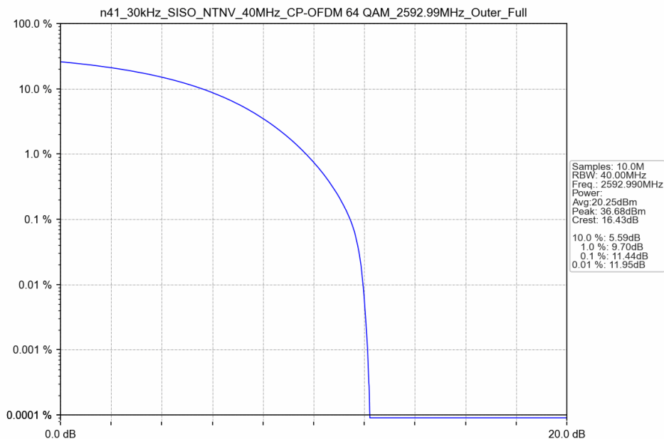
n41_30kHz_SISO_NTNV_40MHz_CP-OFDM 64 QAM_2592.99MHz_Outer_Full
