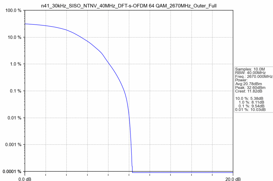
n41_30kHz_SISO_NTNV_40MHz_DFT-s-OFDM 64 QAM_2670MHz_Outer_Full
