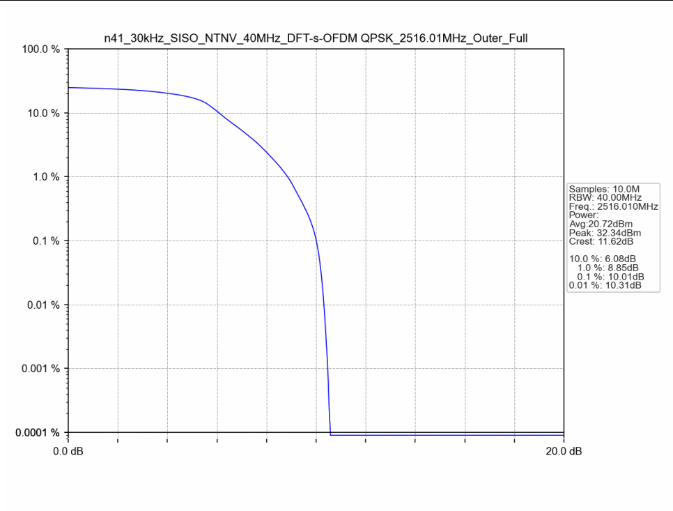
n41_30kHz_SISO_NTNV_40MHz_DFT-s-OFDM QPSK_2516.01MHz_Outer_Full
