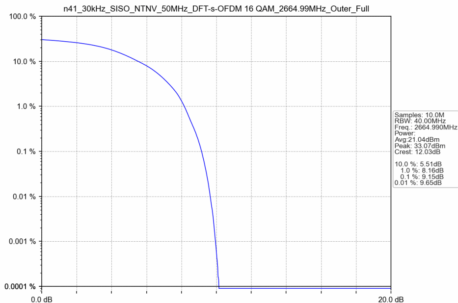
n41_30kHz_SISO_NTNV_50MHz_DFT-s-OFDM 16 QAM_2664.99MHz_Outer_Full
