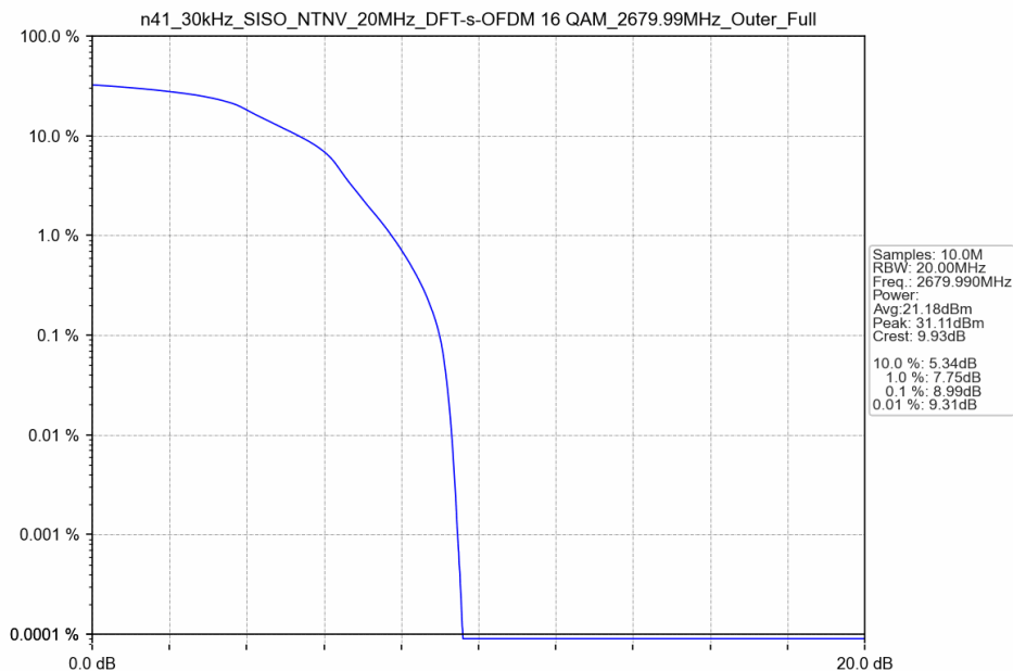
n41_30kHz_SISO_NTNV_20MHz_DFT-s-OFDM 16 QAM_2679.99MHz_Outer_Full
