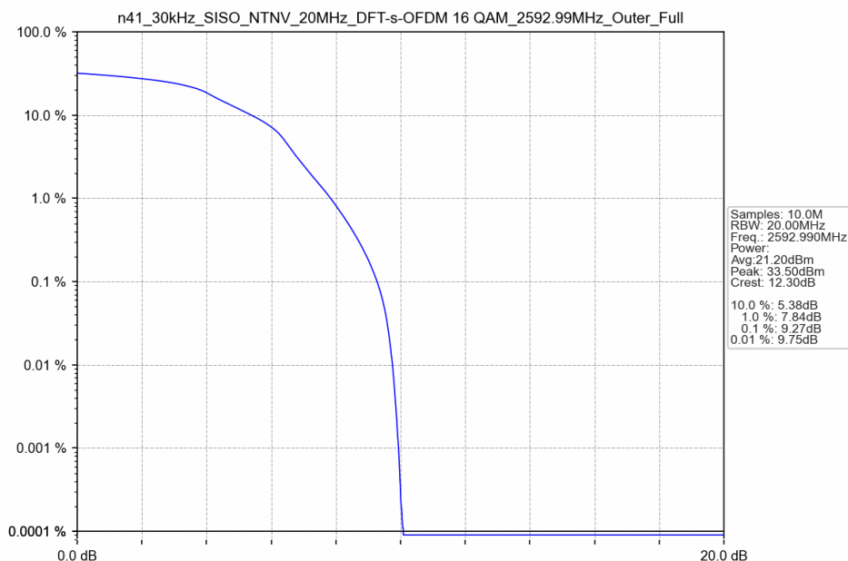
n41_30kHz_SISO_NTNV_20MHz_DFT-s-OFDM 16 QAM_2592.99MHz_Outer_Full
