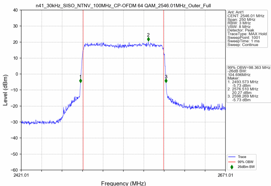
n41_30kHz_SISO_NTNV_100MHz_CP-OFDM 64 QAM_2546.01MHz_Outer_Full
