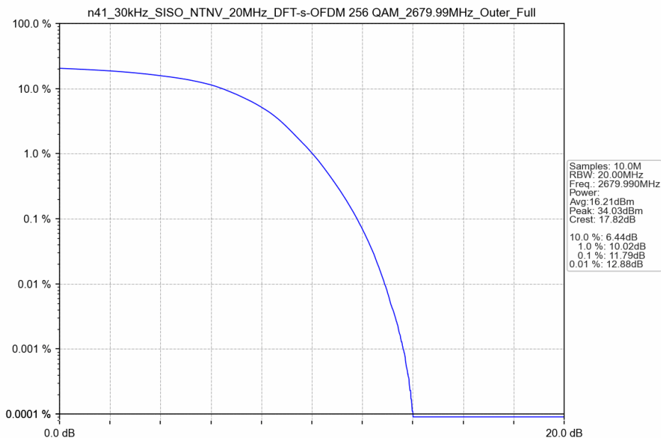
n41_30kHz_SISO_NTNV_20MHz_DFT-s-OFDM 256 QAM_2679.99MHz_Outer_Full
