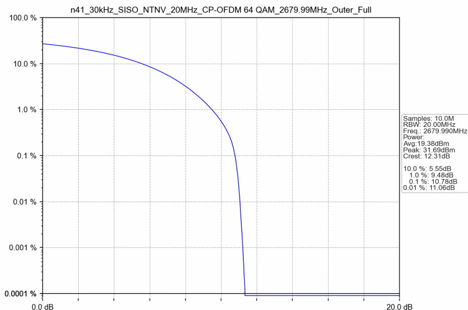
n41_30kHz_SISO_NTNV_20MHz_CP-OFDM 64 QAM_2679.99MHz_Outer_Full
