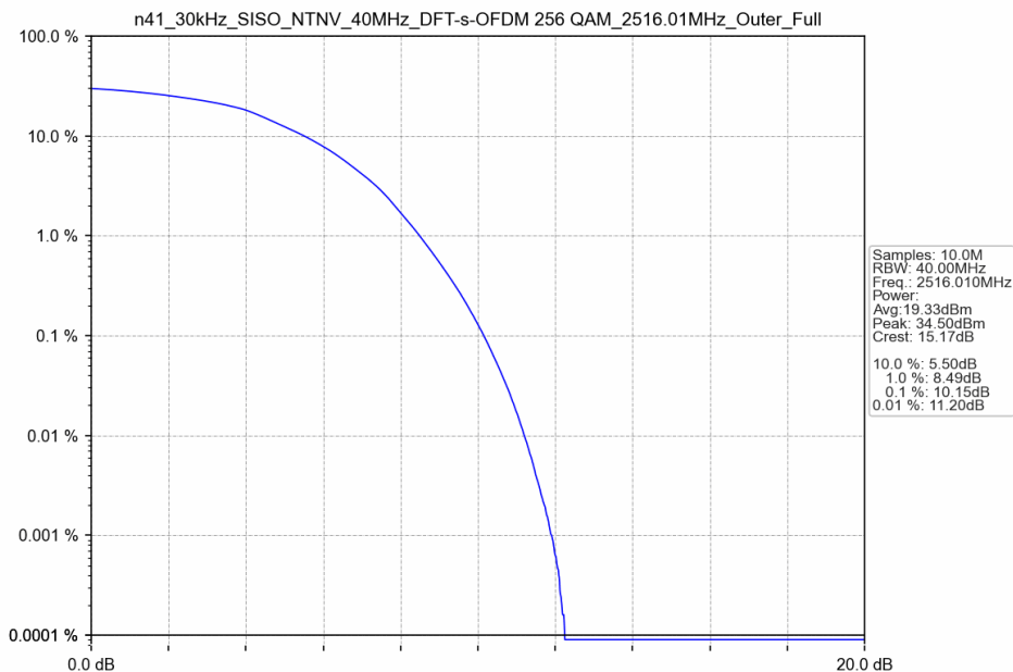
n41_30kHz_SISO_NTNV_40MHz_DFT-s-OFDM 256 QAM_2516.01MHz_Outer_Full
