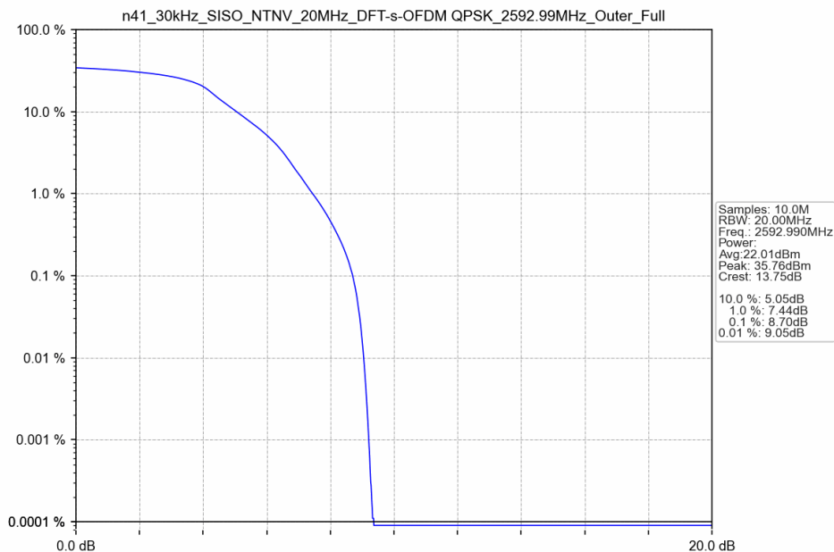
n41_30kHz_SISO_NTNV_20MHz_DFT-s-OFDM QPSK_2592.99MHz_Outer_Full
