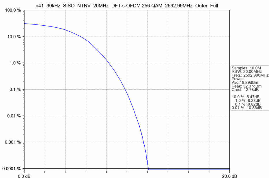
n41_30kHz_SISO_NTNV_20MHz_DFT-s-OFDM 256 QAM_2592.99MHz_Outer_Full
