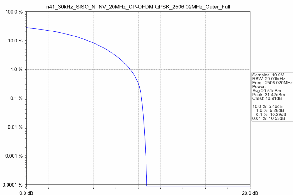
n41_30kHz_SISO_NTNV_20MHz_CP-OFDM QPSK_2506.02MHz_Outer_Full
