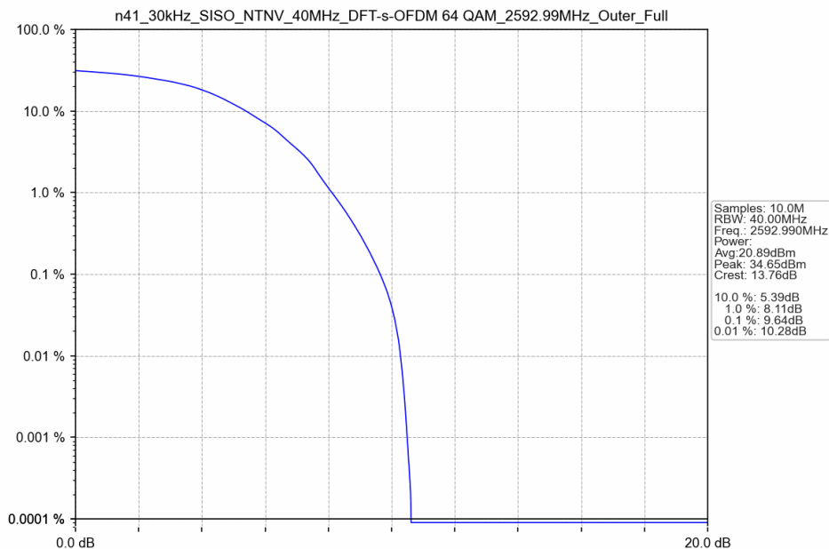
n41_30kHz_SISO_NTNV_40MHz_DFT-s-OFDM 64 QAM_2592.99MHz_Outer_Full
