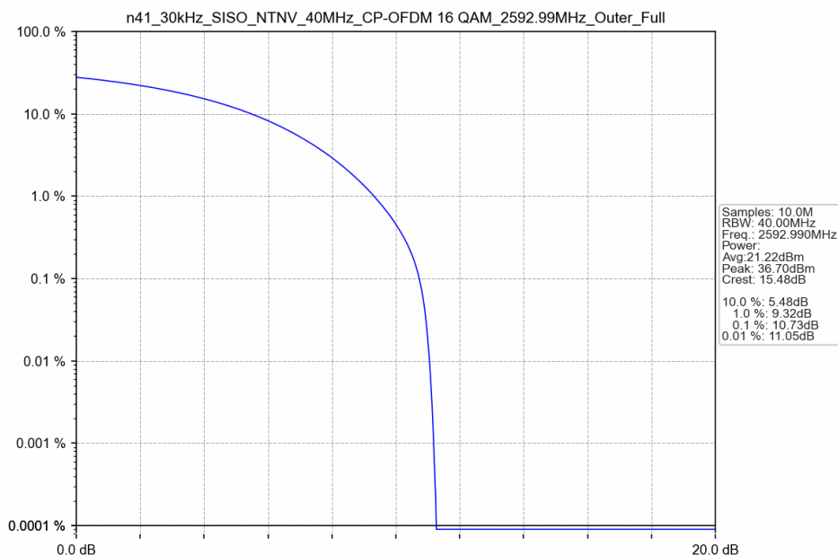
n41_30kHz_SISO_NTNV_40MHz_CP-OFDM 16 QAM_2592.99MHz_Outer_Full
