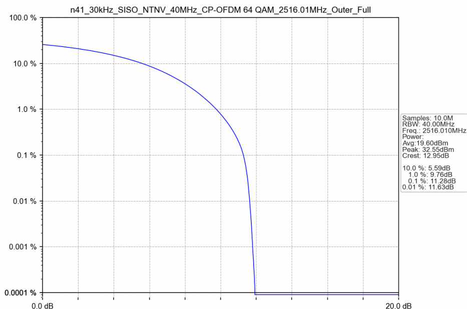
n41_30kHz_SISO_NTNV_40MHz_CP-OFDM 64 QAM_2516.01MHz_Outer_Full
