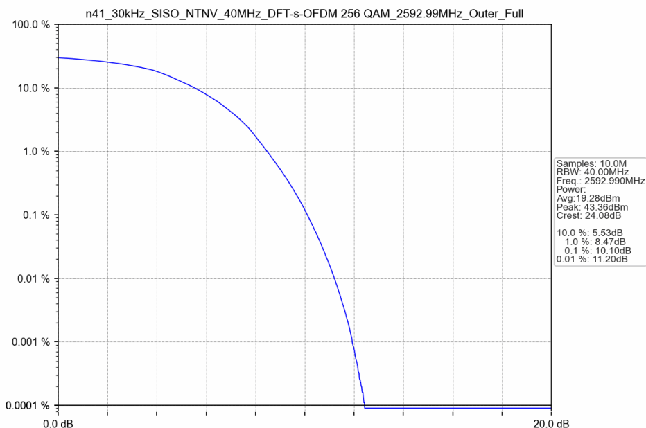
n41_30kHz_SISO_NTNV_40MHz_DFT-s-OFDM 256 QAM_2592.99MHz_Outer_Full
