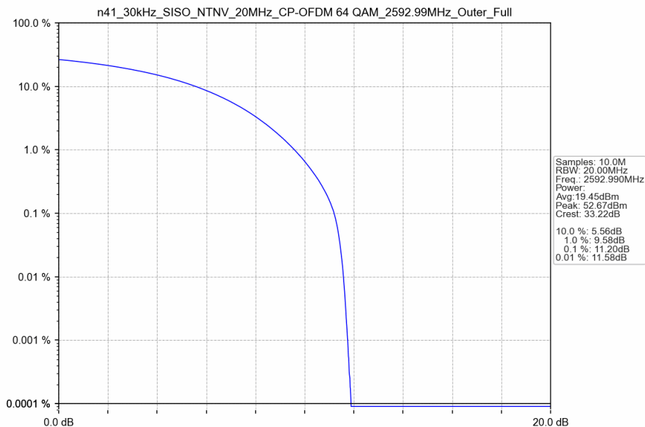
n41_30kHz_SISO_NTNV_20MHz_CP-OFDM 64 QAM_2592.99MHz_Outer_Full
