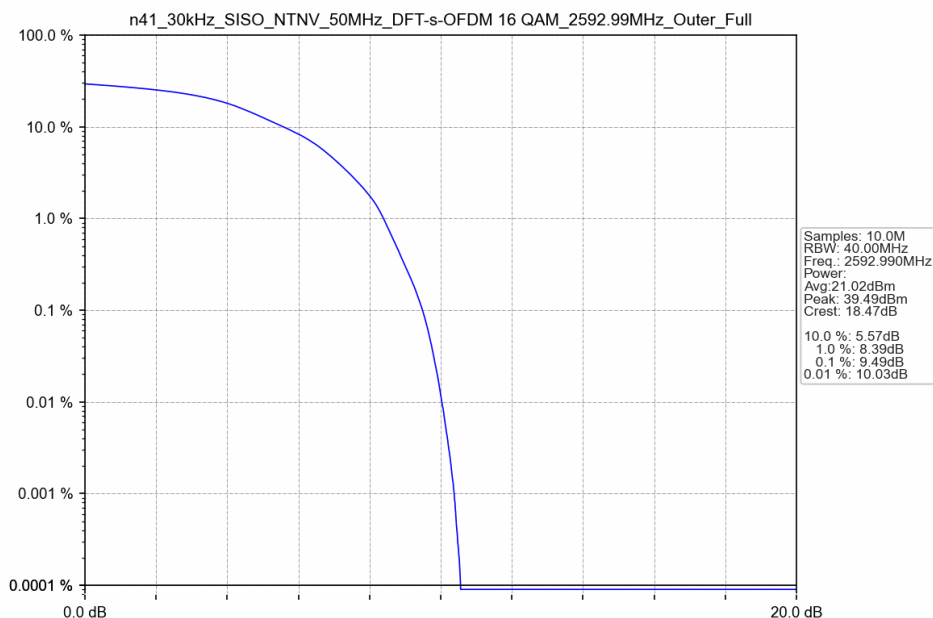
n41_30kHz_SISO_NTNV_50MHz_DFT-s-OFDM 16 QAM_2592.99MHz_Outer_Full
