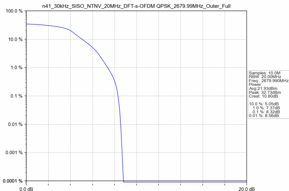
n41_30kHz_SISO_NTNV_20MHz_DFT-s-OFDM QPSK_2679.99MHz_Outer_Full
