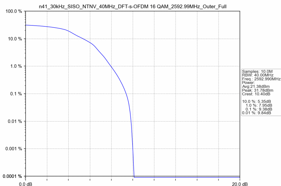
n41_30kHz_SISO_NTNV_40MHz_DFT-s-OFDM 16 QAM_2592.99MHz_Outer_Full
