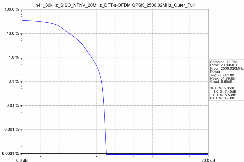
n41_30kHz_SISO_NTNV_20MHz_DFT-s-OFDM QPSK_2506.02MHz_Outer_Full
