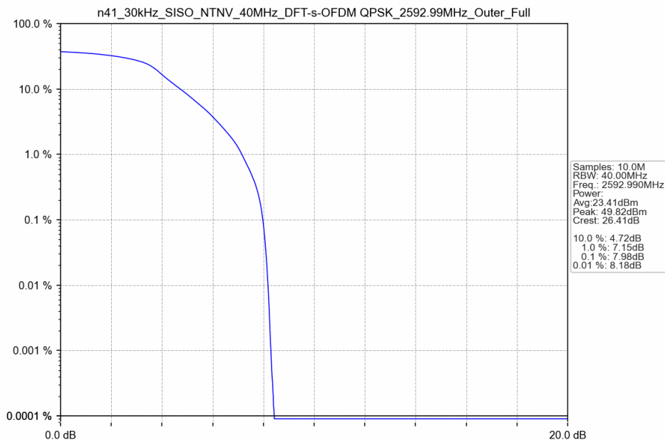
n41_30kHz_SISO_NTNV_40MHz_DFT-s-OFDM QPSK_2592.99MHz_Outer_Full
