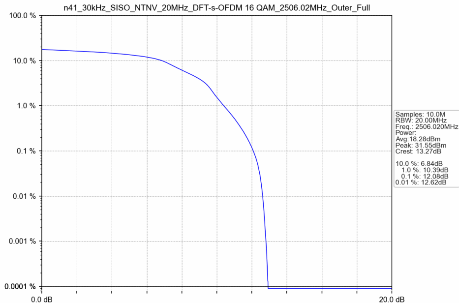
n41_30kHz_SISO_NTNV_20MHz_DFT-s-OFDM 16 QAM_2506.02MHz_Outer_Full
