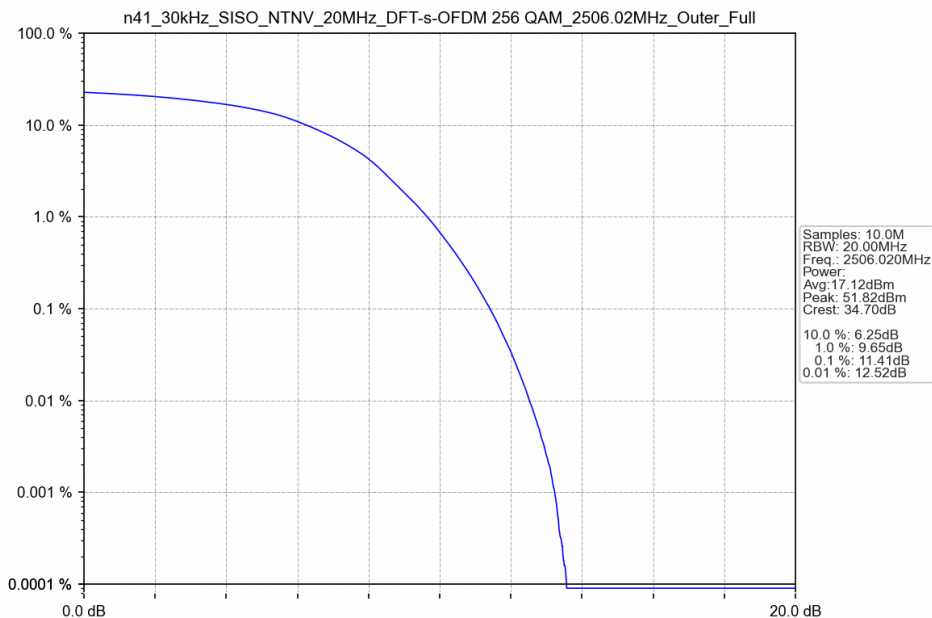
n41_30kHz_SISO_NTNV_20MHz_DFT-s-OFDM 256 QAM_2506.02MHz_Outer_Full
