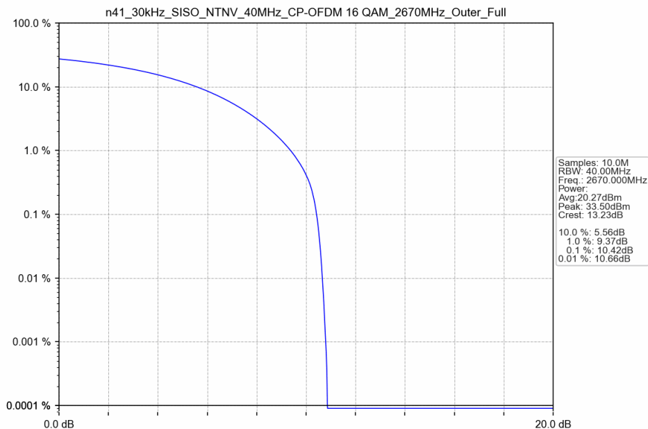
n41_30kHz_SISO_NTNV_40MHz_CP-OFDM 16 QAM_2670MHz_Outer_Full
