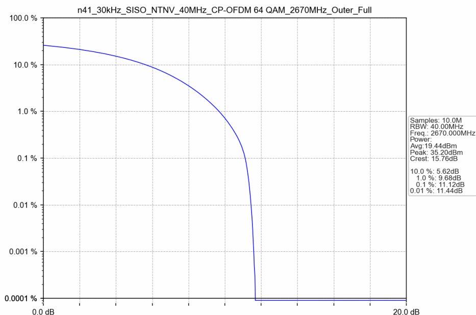
n41_30kHz_SISO_NTNV_40MHz_CP-OFDM 64 QAM_2670MHz_Outer_Full
