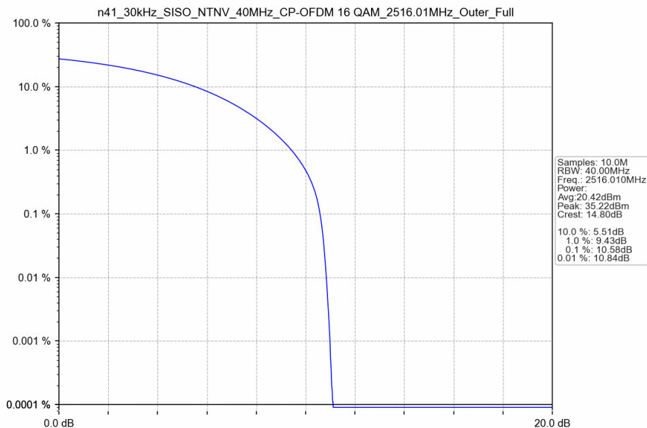
n41_30kHz_SISO_NTNV_40MHz_CP-OFDM 16 QAM_2516.01MHz_Outer_Full
