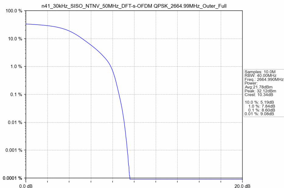
n41_30kHz_SISO_NTNV_50MHz_DFT-s-OFDM QPSK_2664.99MHz_Outer_Full
