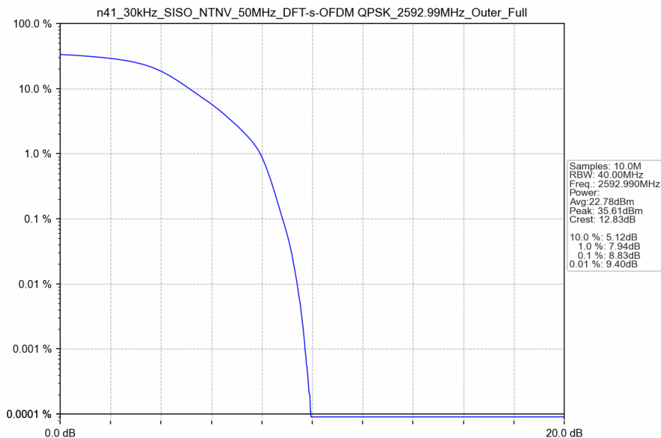
n41_30kHz_SISO_NTNV_50MHz_DFT-s-OFDM QPSK_2592.99MHz_Outer_Full
