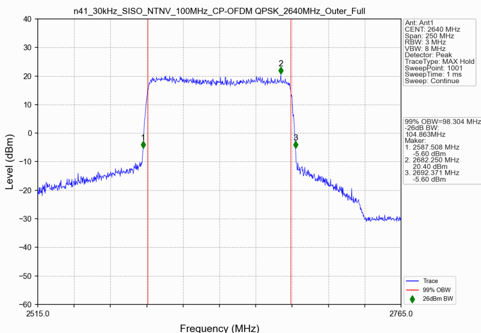
n41_30kHz_SISO_NTNV_100MHz_CP-OFDM QPSK_2640MHz_Outer_Full
