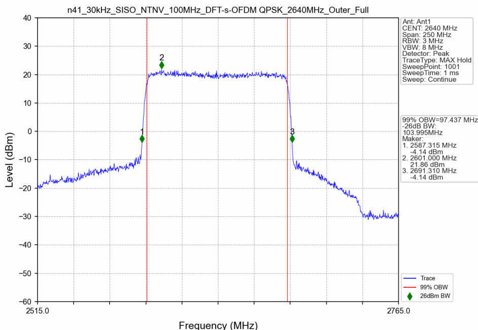
n41_30kHz_SISO_NTNV_100MHz_DFT-s-OFDM QPSK_2640MHz_Outer_Full
