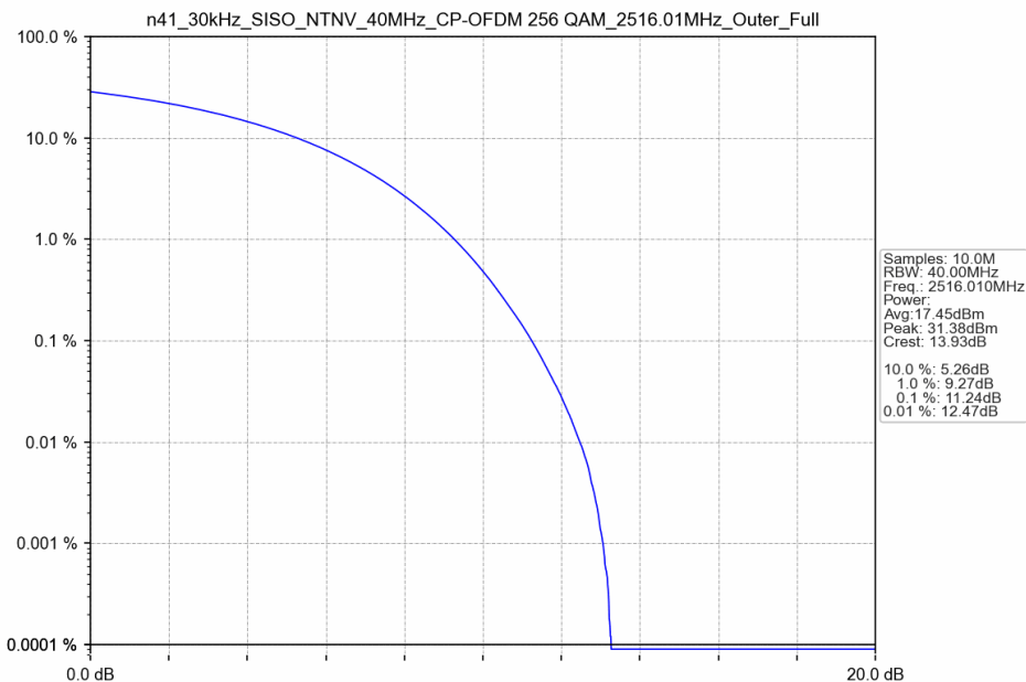
n41_30kHz_SISO_NTNV_40MHz_CP-OFDM 256 QAM_2516.01MHz_Outer_Full
