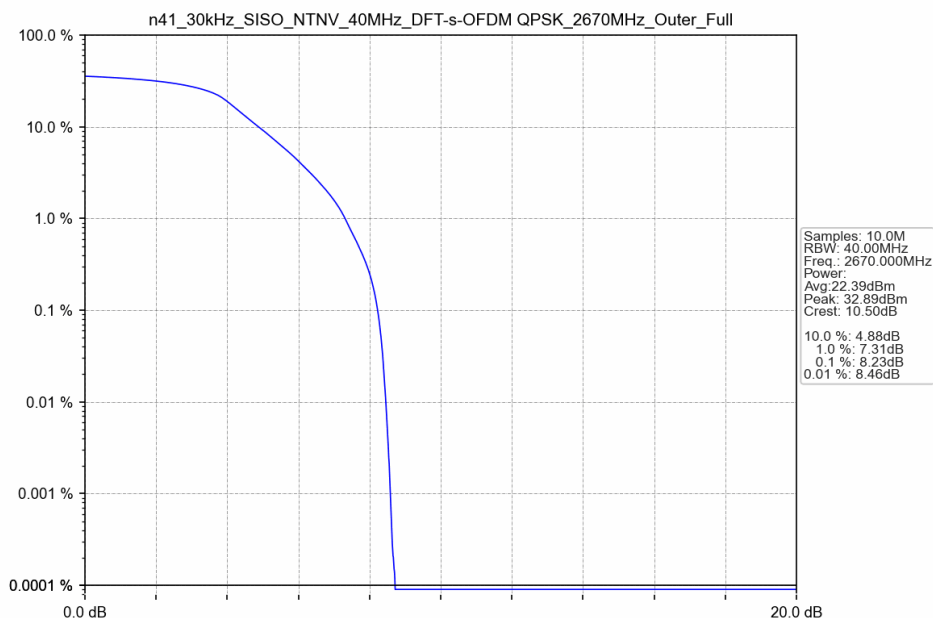
n41_30kHz_SISO_NTNV_40MHz_DFT-s-OFDM QPSK_2670MHz_Outer_Full
