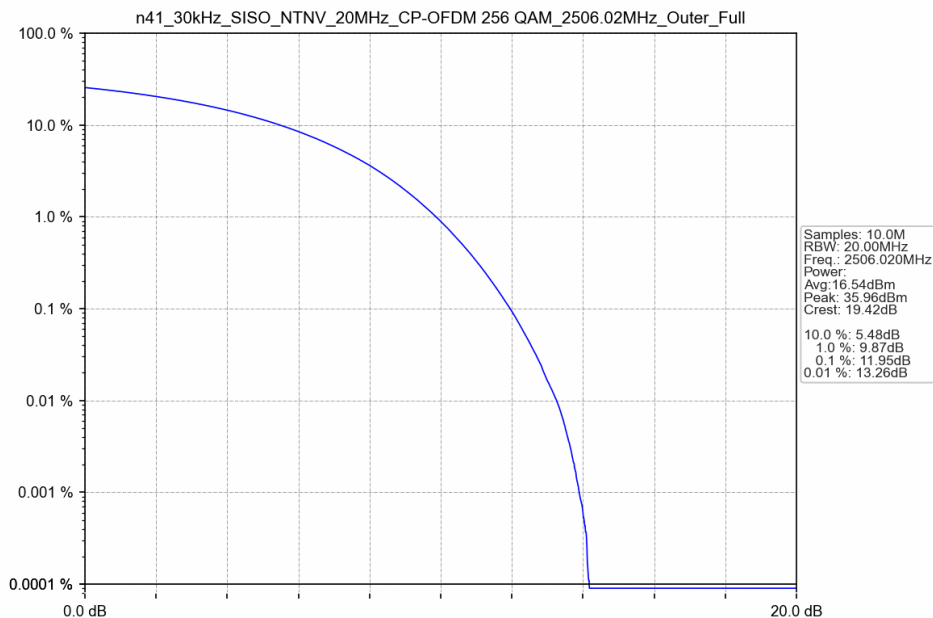
n41_30kHz_SISO_NTNV_20MHz_CP-OFDM 256 QAM_2506.02MHz_Outer_Full
