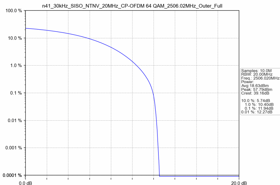
n41_30kHz_SISO_NTNV_20MHz_CP-OFDM 64 QAM_2506.02MHz_Outer_Full
