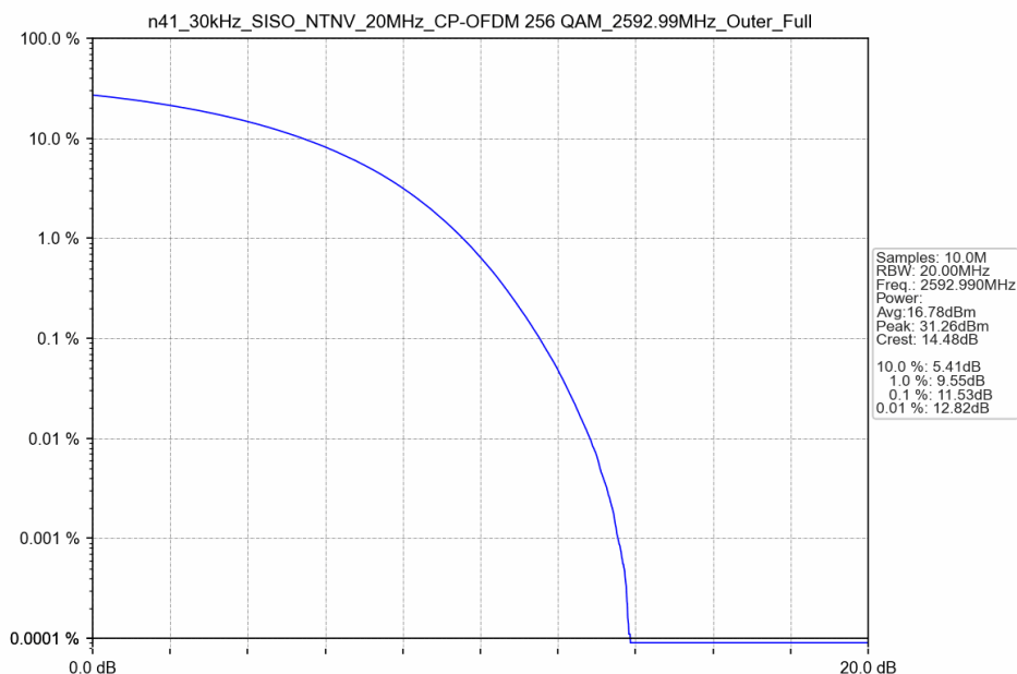
n41_30kHz_SISO_NTNV_20MHz_CP-OFDM 256 QAM_2592.99MHz_Outer_Full
