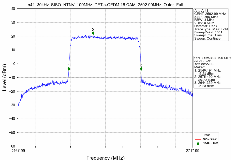
n41_30kHz_SISO_NTNV_100MHz_DFT-s-OFDM 16 QAM_2592.99MHz_Outer_Full
