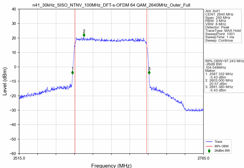
n41_30kHz_SISO_NTNV_100MHz_DFT-s-OFDM 64 QAM_2640MHz_Outer_Full
