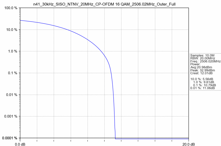
n41_30kHz_SISO_NTNV_20MHz_CP-OFDM 16 QAM_2506.02MHz_Outer_Full
