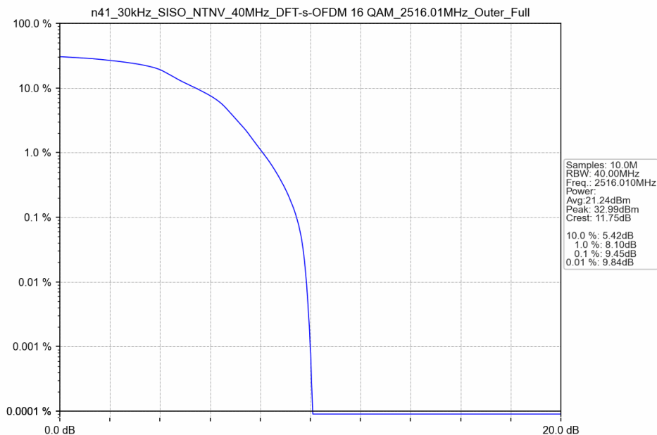
n41_30kHz_SISO_NTNV_40MHz_DFT-s-OFDM 16 QAM_2516.01MHz_Outer_Full
