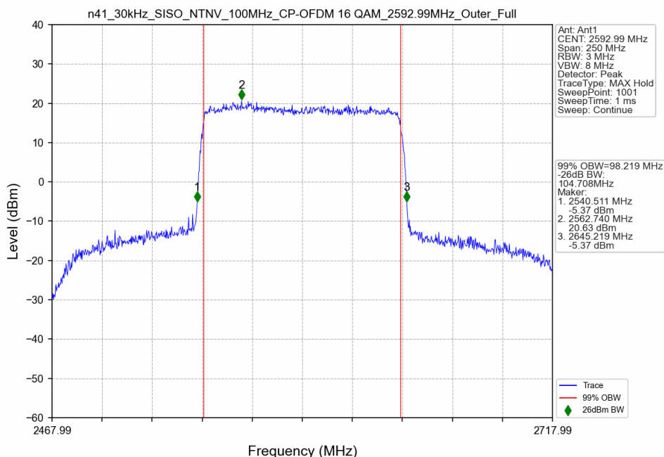
n41_30kHz_SISO_NTNV_100MHz_CP-OFDM 16 QAM_2592.99MHz_Outer_Full
