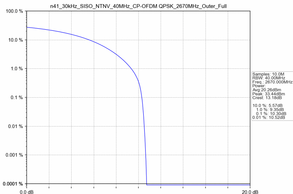
n41_30kHz_SISO_NTNV_40MHz_CP-OFDM QPSK_2670MHz_Outer_Full
