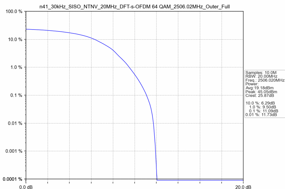
n41_30kHz_SISO_NTNV_20MHz_DFT-s-OFDM 64 QAM_2506.02MHz_Outer_Full
