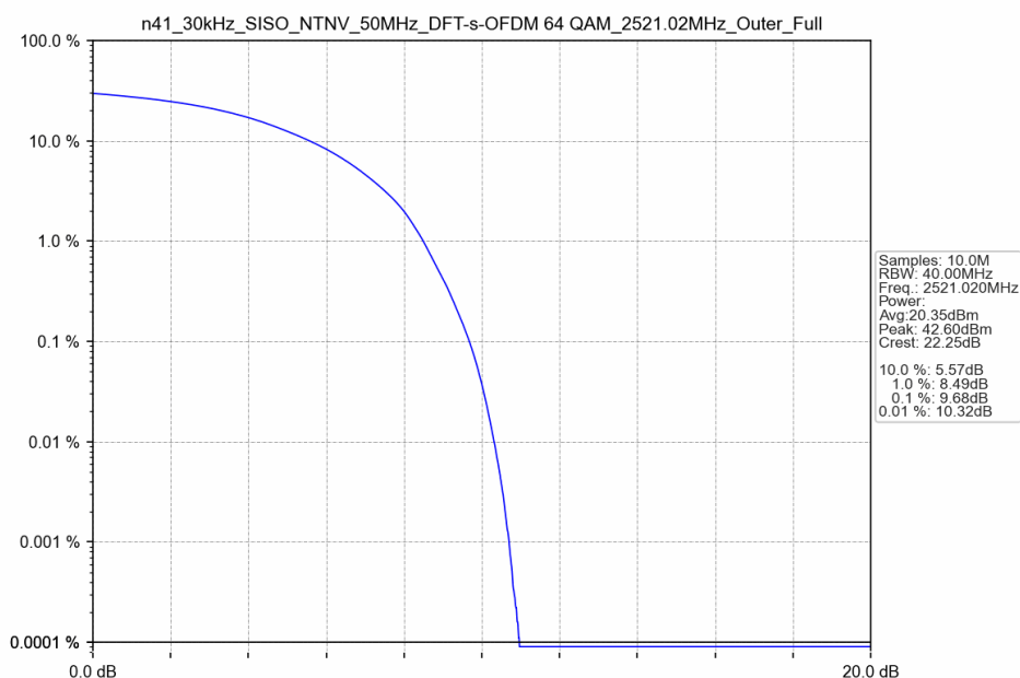
n41_30kHz_SISO_NTNV_50MHz_DFT-s-OFDM 64 QAM_2521.02MHz_Outer_Full
