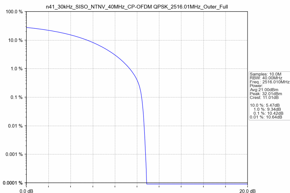
n41_30kHz_SISO_NTNV_40MHz_CP-OFDM QPSK_2516.01MHz_Outer_Full
