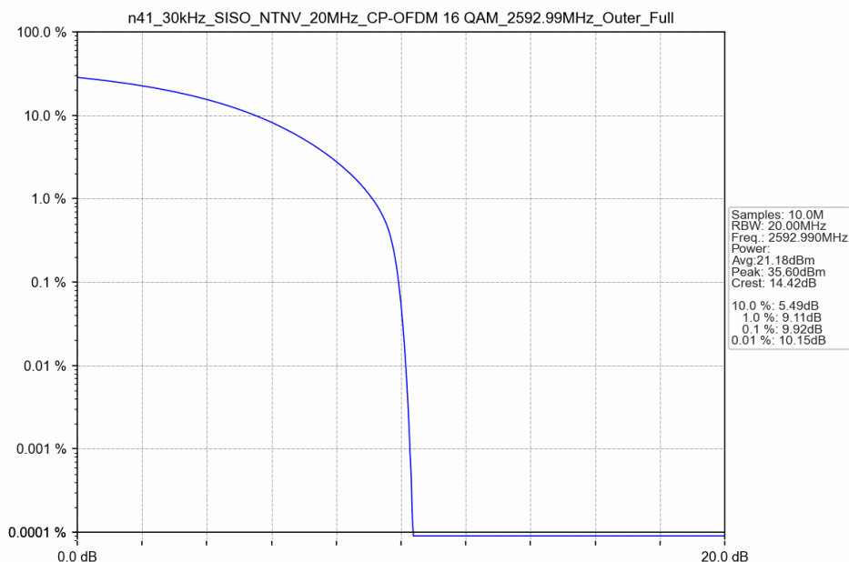
n41_30kHz_SISO_NTNV_20MHz_CP-OFDM 16 QAM_2592.99MHz_Outer_Full
