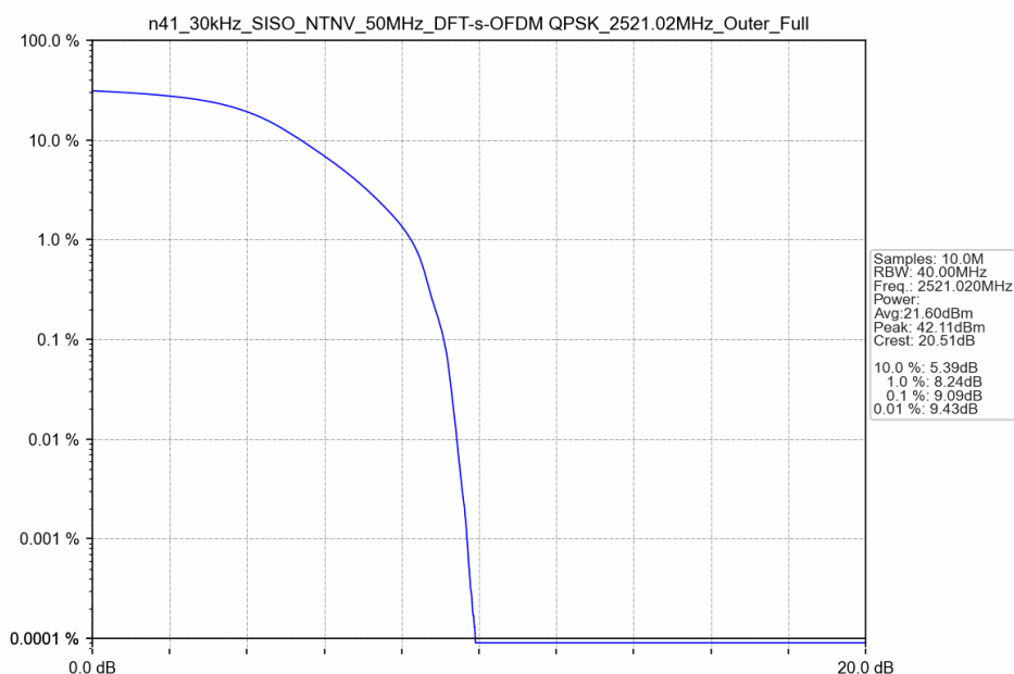
n41_30kHz_SISO_NTNV_50MHz_DFT-s-OFDM QPSK_2521.02MHz_Outer_Full
