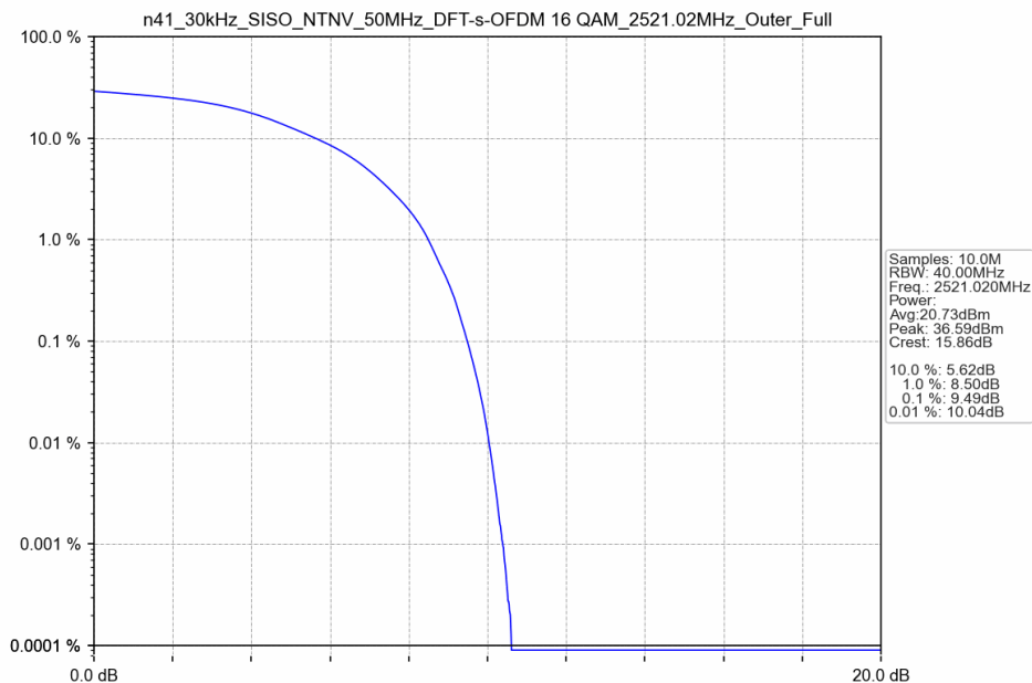
n41_30kHz_SISO_NTNV_50MHz_DFT-s-OFDM 16 QAM_2521.02MHz_Outer_Full
