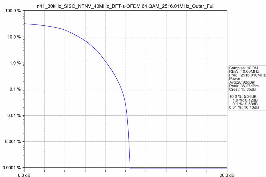
n41_30kHz_SISO_NTNV_40MHz_DFT-s-OFDM 64 QAM_2516.01MHz_Outer_Full
