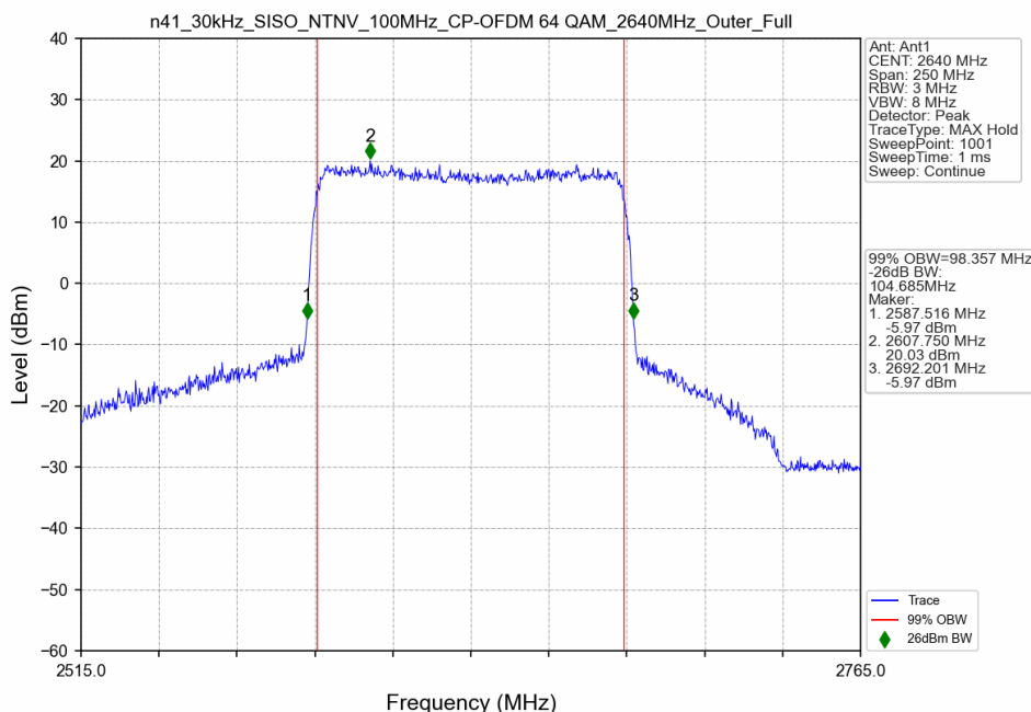
n41_30kHz_SISO_NTNV_100MHz_CP-OFDM 64 QAM_2640MHz_Outer_Full
