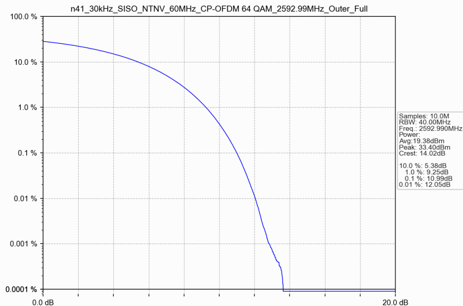
n41_30kHz_SISO_NTNV_60MHz_CP-OFDM 64 QAM_2592.99MHz_Outer_Full
