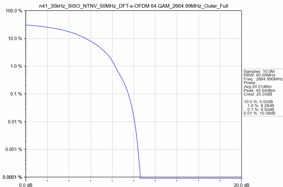
n41_30kHz_SISO_NTNV_50MHz_DFT-s-OFDM 64 QAM_2664.99MHz_Outer_Full
