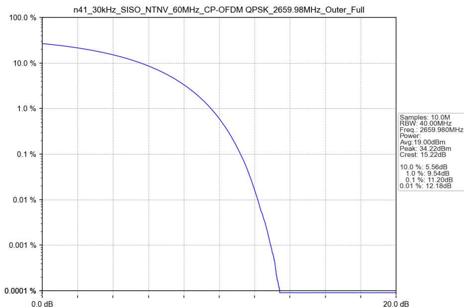
n41_30kHz_SISO_NTNV_60MHz_CP-OFDM QPSK_2659.98MHz_Outer_Full
