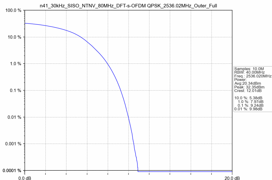
n41_30kHz_SISO_NTNV_80MHz_DFT-s-OFDM QPSK_2536.02MHz_Outer_Full
