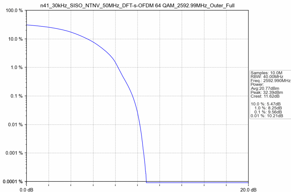
n41_30kHz_SISO_NTNV_50MHz_DFT-s-OFDM 64 QAM_2592.99MHz_Outer_Full
