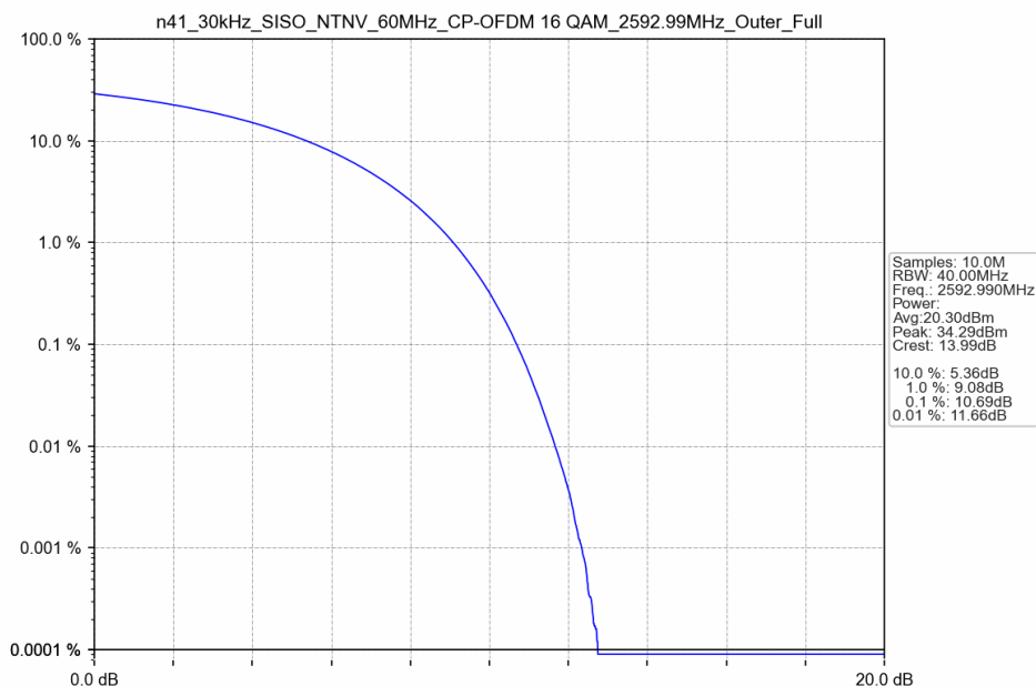
n41_30kHz_SISO_NTNV_60MHz_CP-OFDM 16 QAM_2592.99MHz_Outer_Full
