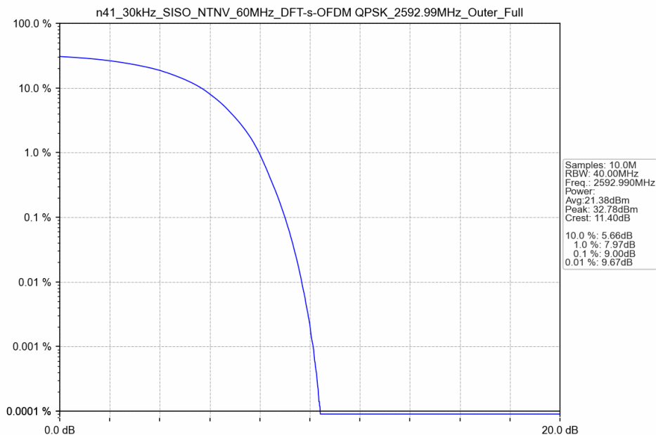
n41_30kHz_SISO_NTNV_60MHz_DFT-s-OFDM QPSK_2592.99MHz_Outer_Full
