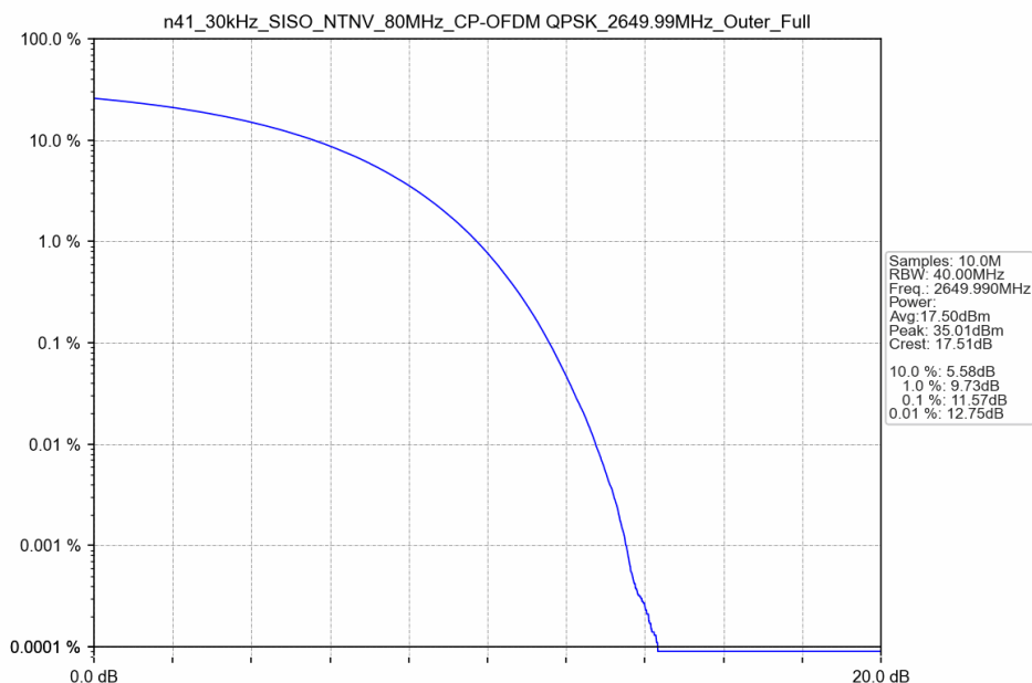
n41_30kHz_SISO_NTNV_80MHz_CP-OFDM QPSK_2649.99MHz_Outer_Full
