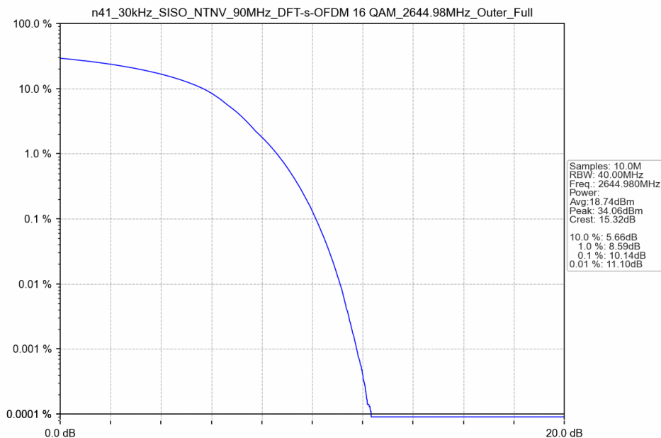
n41_30kHz_SISO_NTNV_90MHz_DFT-s-OFDM 16 QAM_2644.98MHz_Outer_Full
