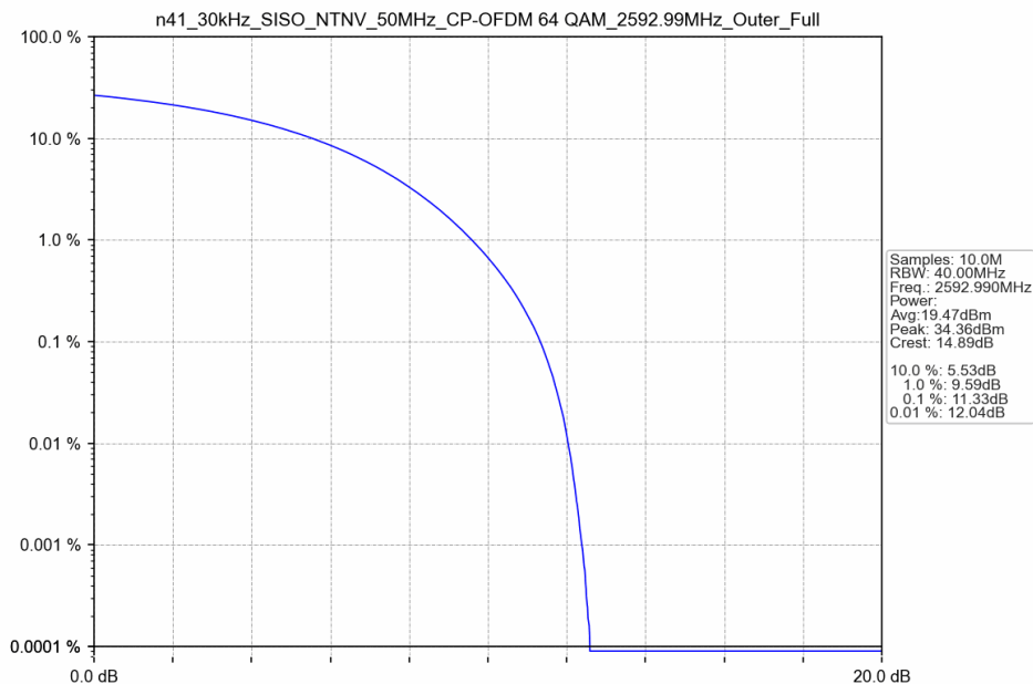
n41_30kHz_SISO_NTNV_50MHz_CP-OFDM 64 QAM_2592.99MHz_Outer_Full
