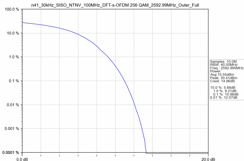
n41_30kHz_SISO_NTNV_100MHz_DFT-s-OFDM 256 QAM_2592.99MHz_Outer_Full
