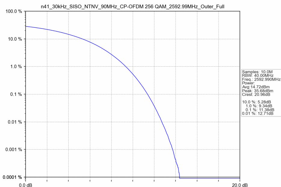
n41_30kHz_SISO_NTNV_90MHz_CP-OFDM 256 QAM_2592.99MHz_Outer_Full
