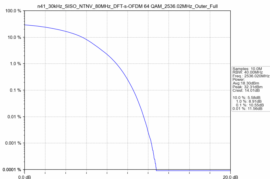
n41_30kHz_SISO_NTNV_80MHz_DFT-s-OFDM 64 QAM_2536.02MHz_Outer_Full
