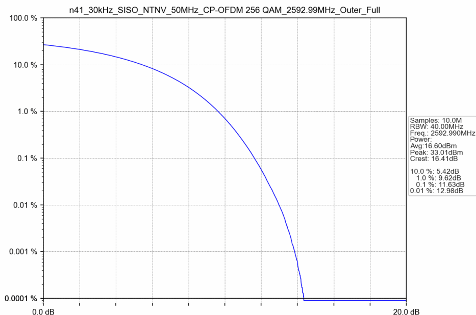
n41_30kHz_SISO_NTNV_50MHz_CP-OFDM 256 QAM_2592.99MHz_Outer_Full
