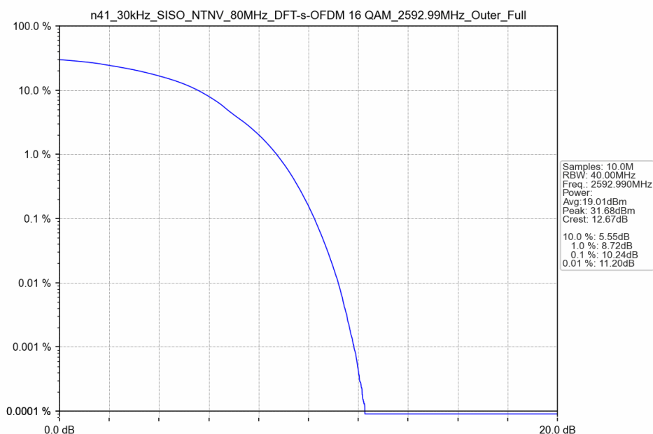
n41_30kHz_SISO_NTNV_80MHz_DFT-s-OFDM 16 QAM_2592.99MHz_Outer_Full
