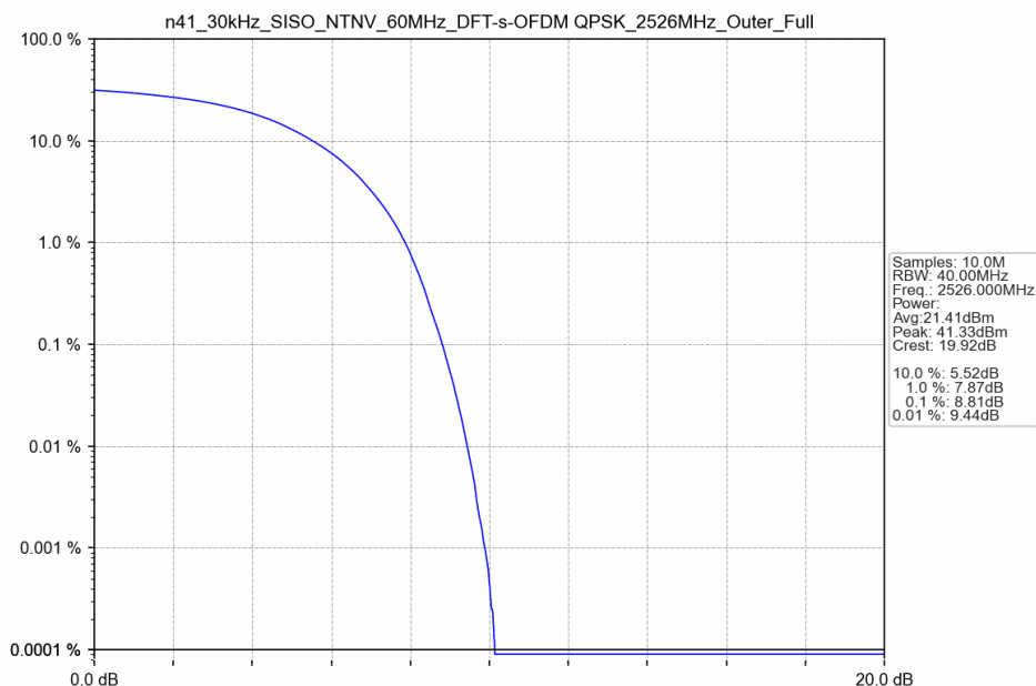
n41_30kHz_SISO_NTNV_60MHz_DFT-s-OFDM QPSK_2526MHz_Outer_Full
