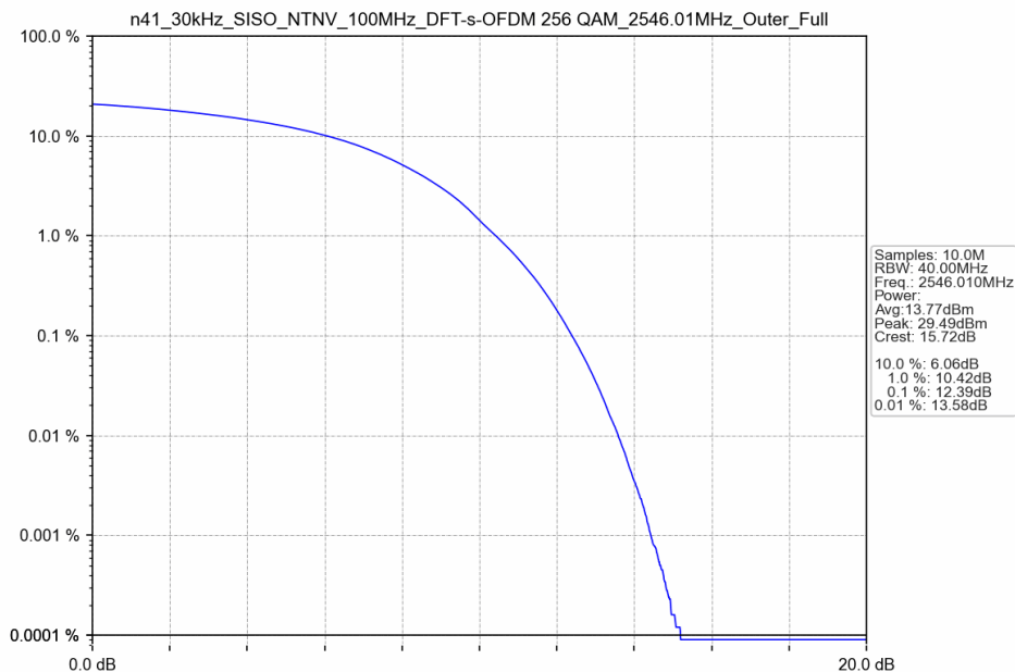
n41_30kHz_SISO_NTNV_100MHz_DFT-s-OFDM 256 QAM_2546.01MHz_Outer_Full
