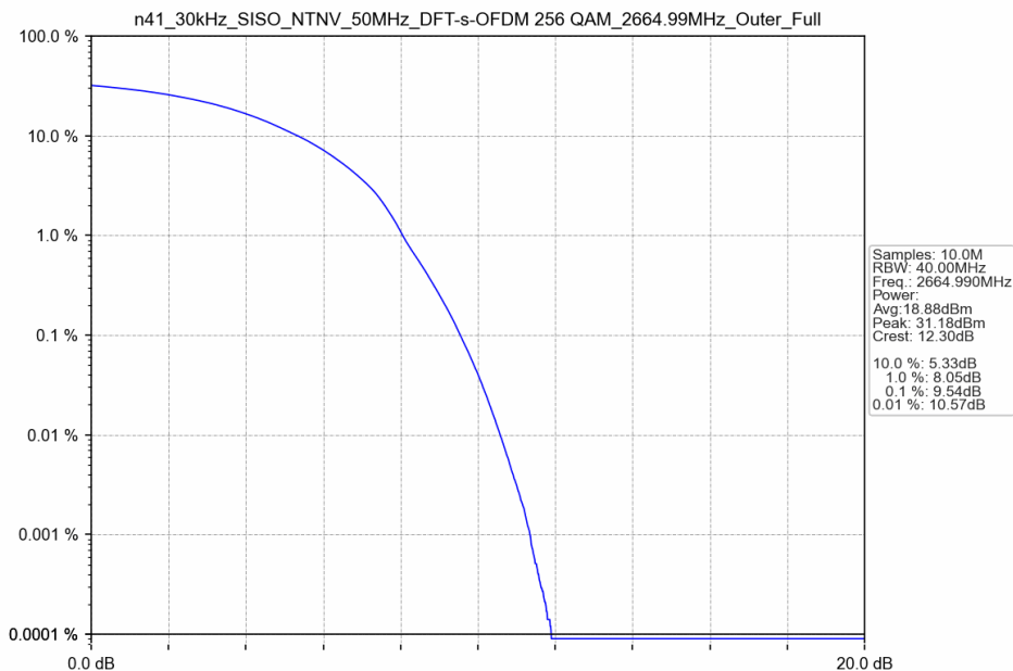
n41_30kHz_SISO_NTNV_50MHz_DFT-s-OFDM 256 QAM_2664.99MHz_Outer_Full
