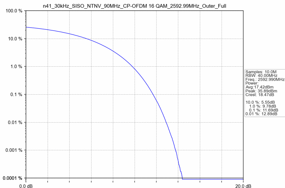
n41_30kHz_SISO_NTNV_90MHz_CP-OFDM 16 QAM_2592.99MHz_Outer_Full
