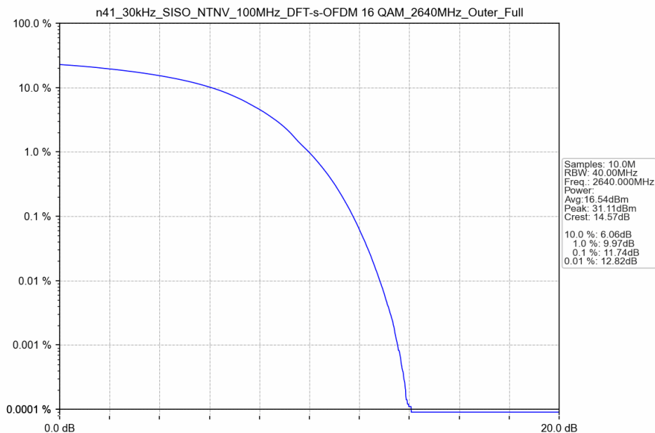
n41_30kHz_SISO_NTNV_100MHz_DFT-s-OFDM 16 QAM_2640MHz_Outer_Full
