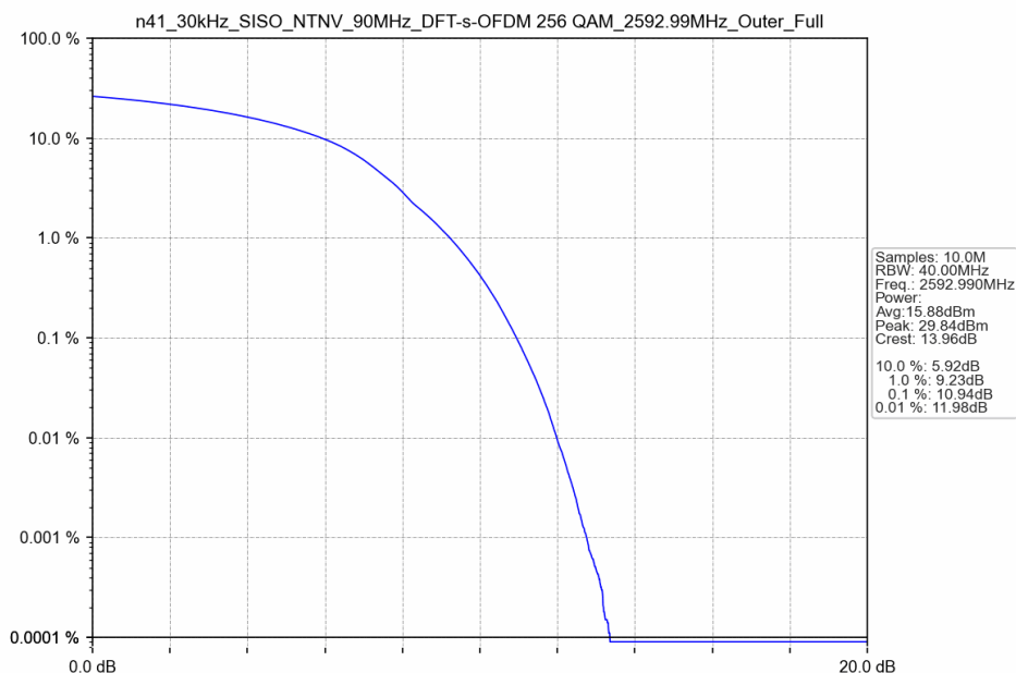
n41_30kHz_SISO_NTNV_90MHz_DFT-s-OFDM 256 QAM_2592.99MHz_Outer_Full
