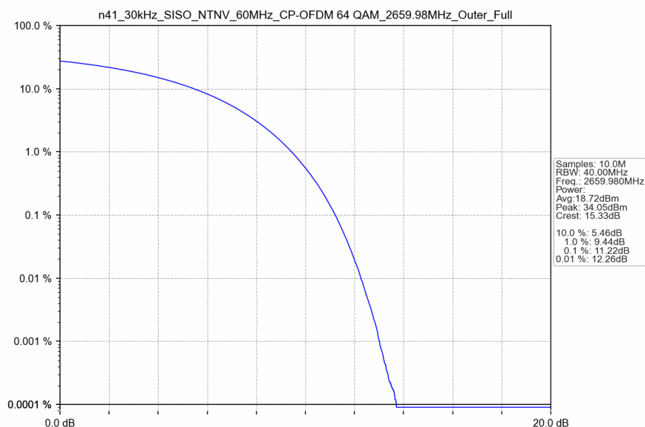
n41_30kHz_SISO_NTNV_60MHz_CP-OFDM 64 QAM_2659.98MHz_Outer_Full
