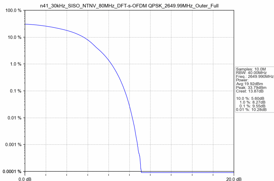
n41_30kHz_SISO_NTNV_80MHz_DFT-s-OFDM QPSK_2649.99MHz_Outer_Full
