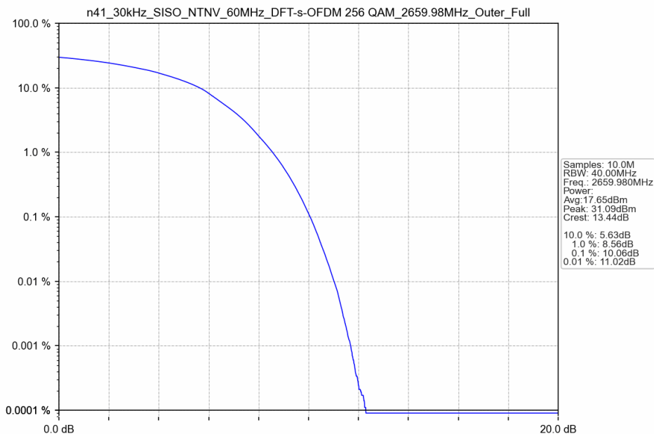
n41_30kHz_SISO_NTNV_60MHz_DFT-s-OFDM 256 QAM_2659.98MHz_Outer_Full
