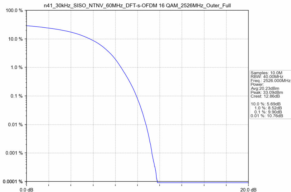
n41_30kHz_SISO_NTNV_60MHz_DFT-s-OFDM 16 QAM_2526MHz_Outer_Full
