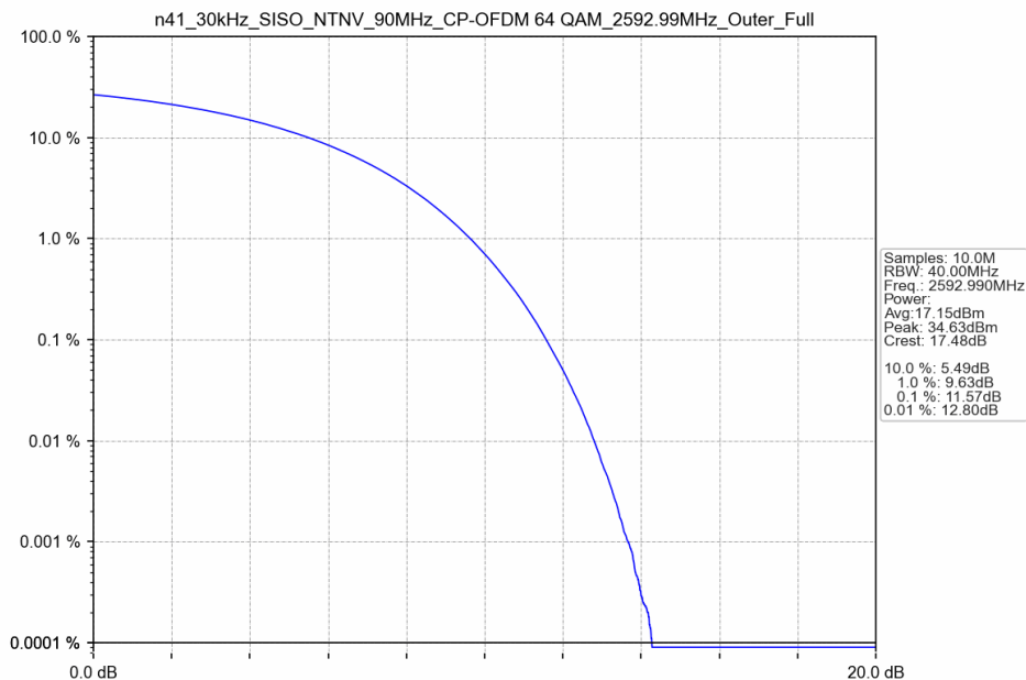
n41_30kHz_SISO_NTNV_90MHz_CP-OFDM 64 QAM_2592.99MHz_Outer_Full
