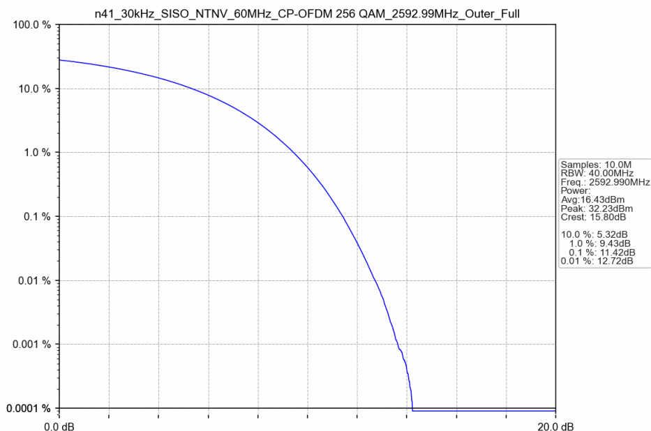
n41_30kHz_SISO_NTNV_60MHz_CP-OFDM 256 QAM_2592.99MHz_Outer_Full
