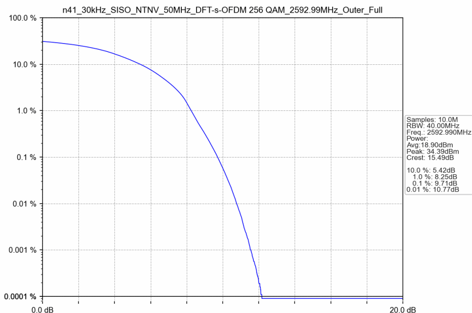
n41_30kHz_SISO_NTNV_50MHz_DFT-s-OFDM 256 QAM_2592.99MHz_Outer_Full
