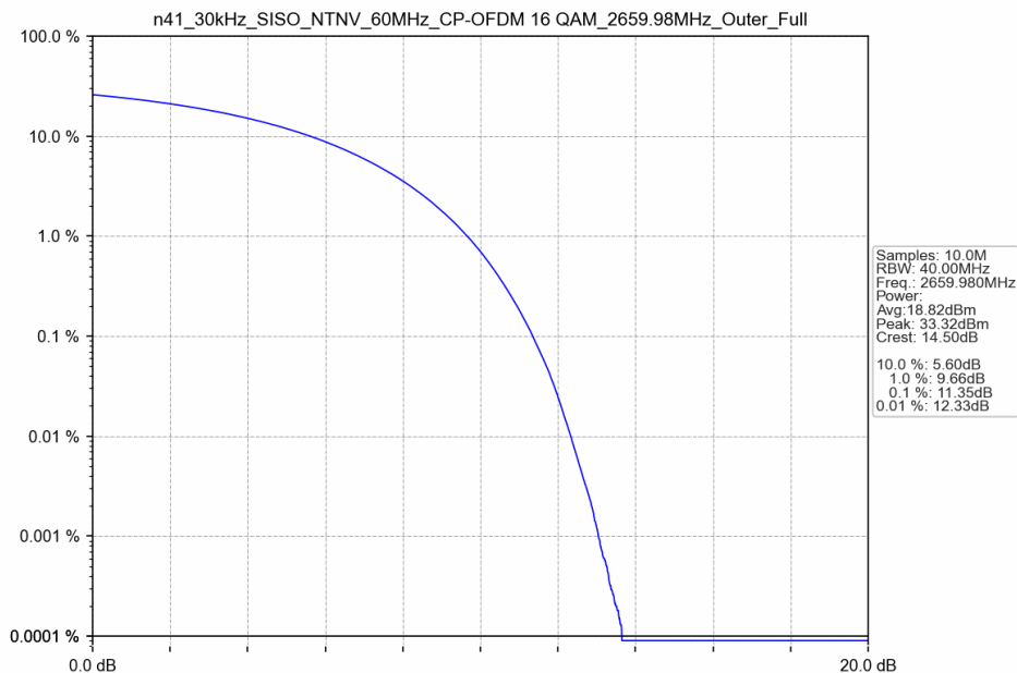
n41_30kHz_SISO_NTNV_60MHz_CP-OFDM 16 QAM_2659.98MHz_Outer_Full
