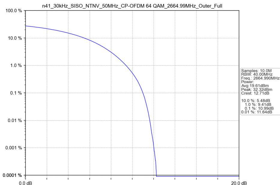
n41_30kHz_SISO_NTNV_50MHz_CP-OFDM 64 QAM_2664.99MHz_Outer_Full
