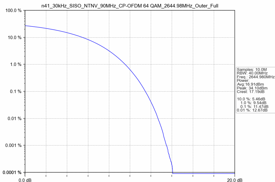
n41_30kHz_SISO_NTNV_90MHz_CP-OFDM 64 QAM_2644.98MHz_Outer_Full
