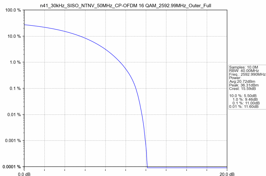
n41_30kHz_SISO_NTNV_50MHz_CP-OFDM 16 QAM_2592.99MHz_Outer_Full
