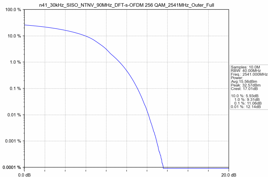
n41_30kHz_SISO_NTNV_90MHz_DFT-s-OFDM 256 QAM_2541MHz_Outer_Full
