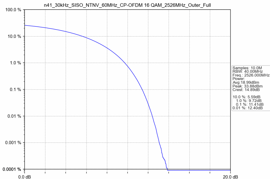
n41_30kHz_SISO_NTNV_60MHz_CP-OFDM 16 QAM_2526MHz_Outer_Full
