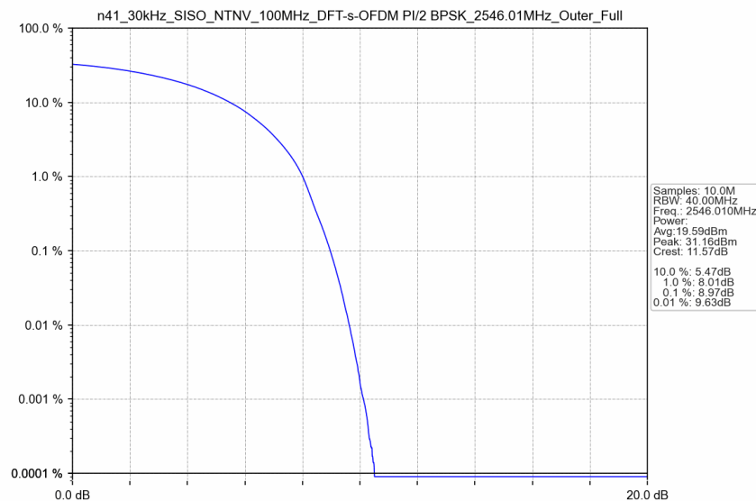
n41_30kHz_SISO_NTNV_100MHz_DFT-s-OFDM PI/2 BPSK_2546.01MHz_Outer_Full
