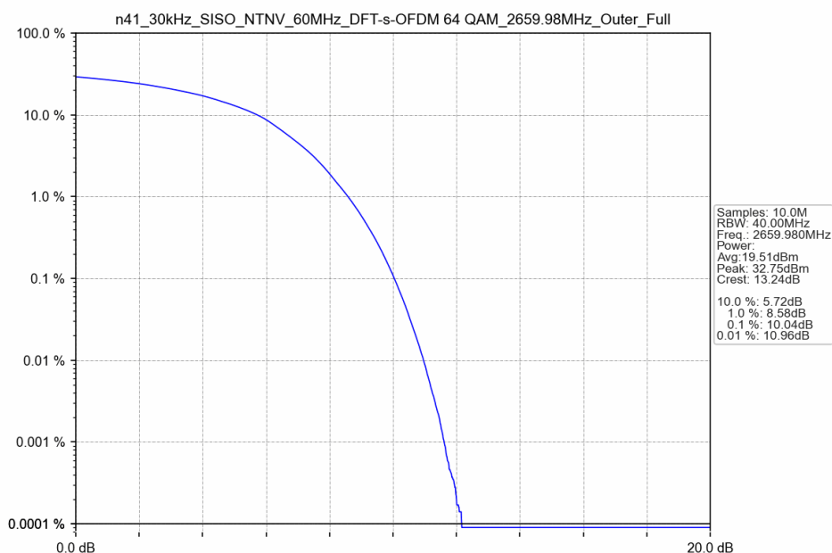
n41_30kHz_SISO_NTNV_60MHz_DFT-s-OFDM 64 QAM_2659.98MHz_Outer_Full
