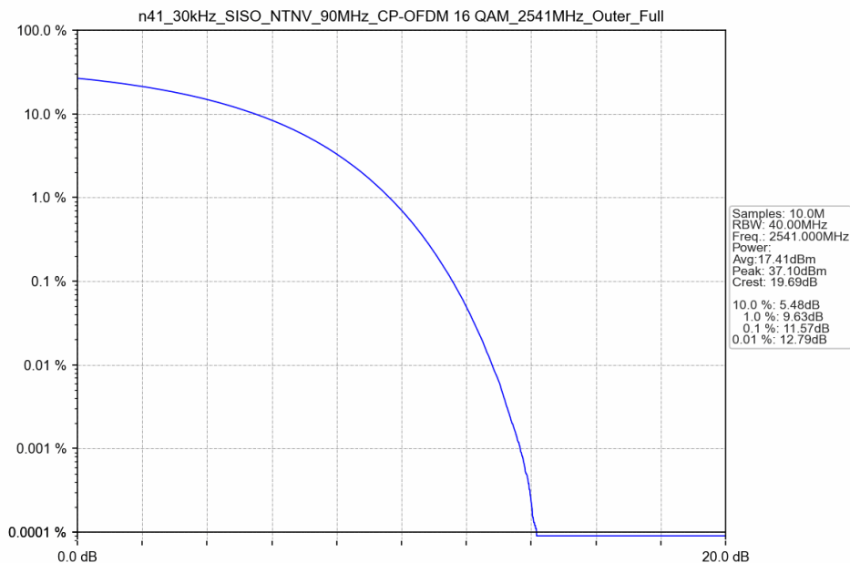
n41_30kHz_SISO_NTNV_90MHz_CP-OFDM 16 QAM_2541MHz_Outer_Full
