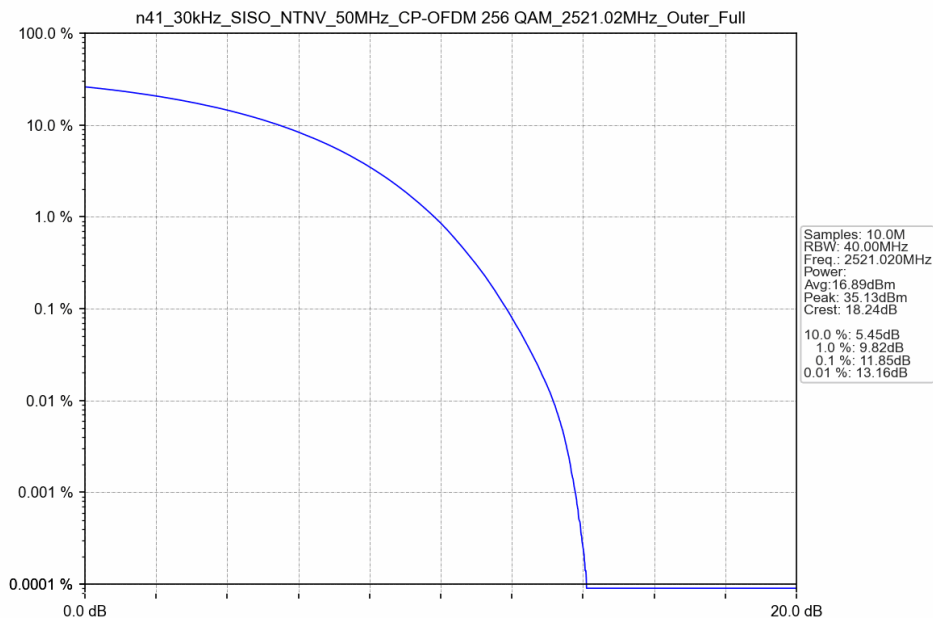
n41_30kHz_SISO_NTNV_50MHz_CP-OFDM 256 QAM_2521.02MHz_Outer_Full
