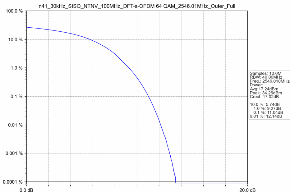
n41_30kHz_SISO_NTNV_100MHz_DFT-s-OFDM 64 QAM_2546.01MHz_Outer_Full
