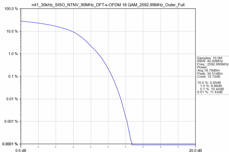
n41_30kHz_SISO_NTNV_90MHz_DFT-s-OFDM 16 QAM_2592.99MHz_Outer_Full
