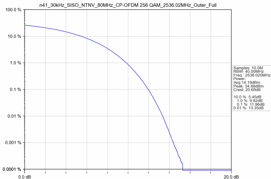
n41_30kHz_SISO_NTNV_80MHz_CP-OFDM 256 QAM_2536.02MHz_Outer_Full
