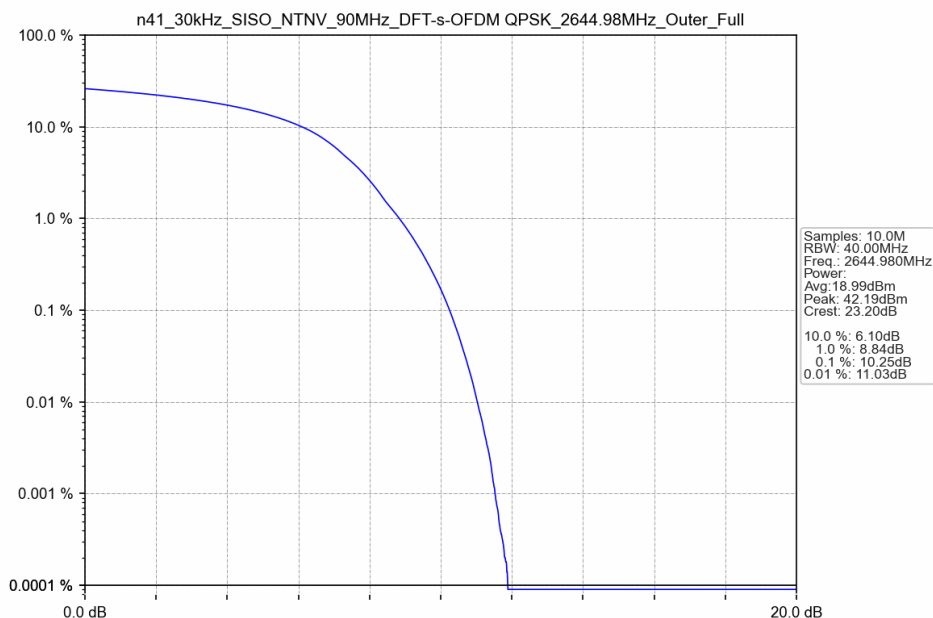
n41_30kHz_SISO_NTNV_90MHz_DFT-s-OFDM QPSK_2644.98MHz_Outer_Full
