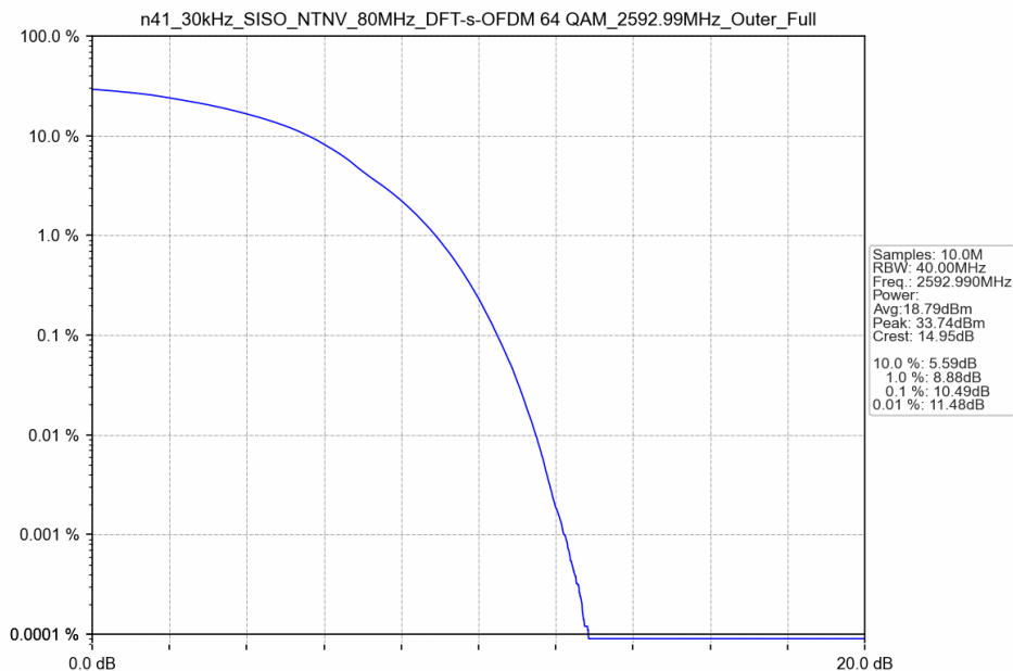
n41_30kHz_SISO_NTNV_80MHz_DFT-s-OFDM 64 QAM_2592.99MHz_Outer_Full
