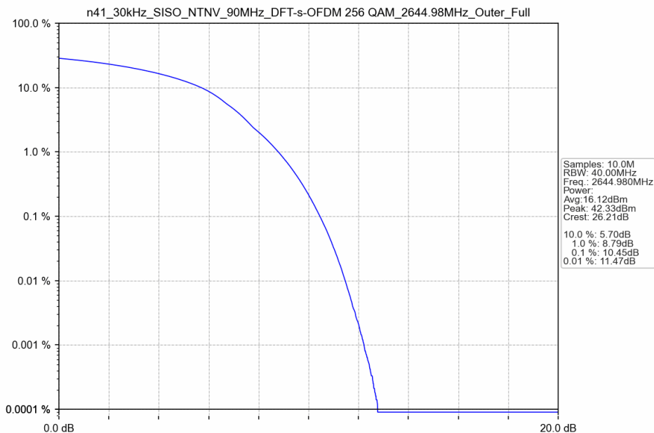
n41_30kHz_SISO_NTNV_90MHz_DFT-s-OFDM 256 QAM_2644.98MHz_Outer_Full
