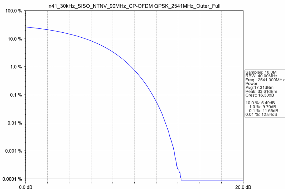
n41_30kHz_SISO_NTNV_90MHz_CP-OFDM QPSK_2541MHz_Outer_Full
