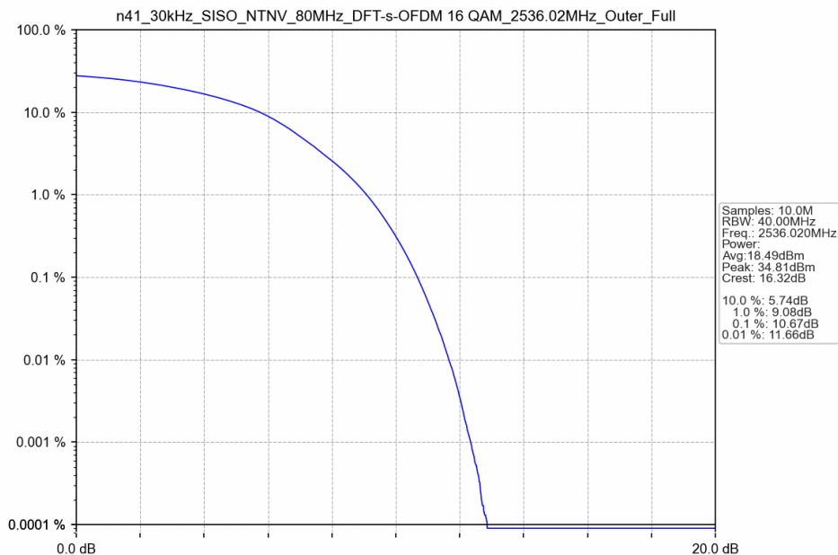
n41_30kHz_SISO_NTNV_80MHz_DFT-s-OFDM 16 QAM_2536.02MHz_Outer_Full
