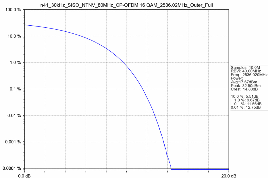
n41_30kHz_SISO_NTNV_80MHz_CP-OFDM 16 QAM_2536.02MHz_Outer_Full
