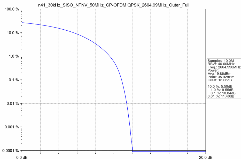
n41_30kHz_SISO_NTNV_50MHz_CP-OFDM QPSK_2664.99MHz_Outer_Full
