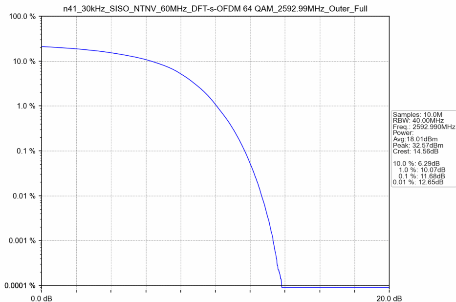
n41_30kHz_SISO_NTNV_60MHz_DFT-s-OFDM 64 QAM_2592.99MHz_Outer_Full
