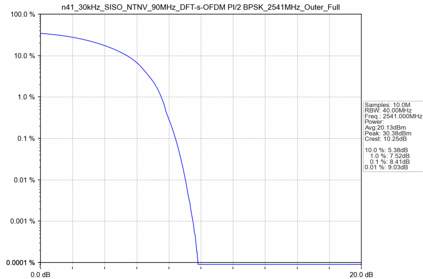
n41_30kHz_SISO_NTNV_90MHz_DFT-s-OFDM PI/2 BPSK_2541MHz_Outer_Full
