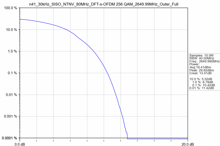
n41_30kHz_SISO_NTNV_80MHz_DFT-s-OFDM 256 QAM_2649.99MHz_Outer_Full
