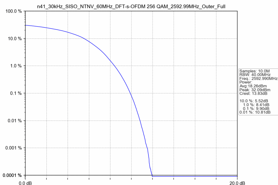
n41_30kHz_SISO_NTNV_60MHz_DFT-s-OFDM 256 QAM_2592.99MHz_Outer_Full
