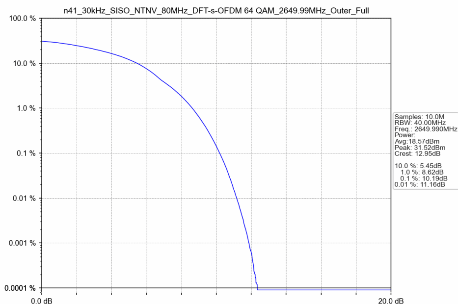
n41_30kHz_SISO_NTNV_80MHz_DFT-s-OFDM 64 QAM_2649.99MHz_Outer_Full
