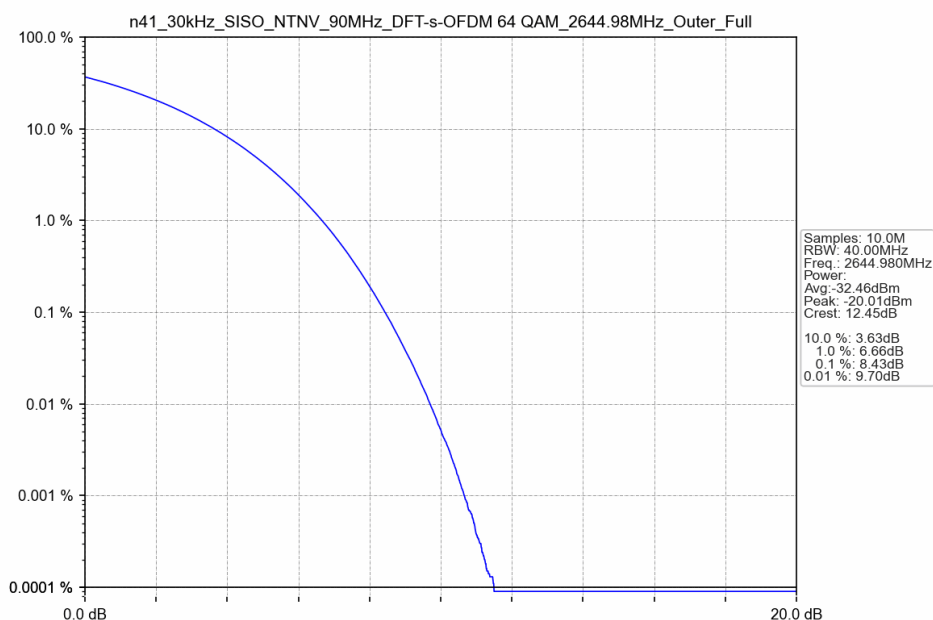
n41_30kHz_SISO_NTNV_90MHz_DFT-s-OFDM 64 QAM_2644.98MHz_Outer_Full
