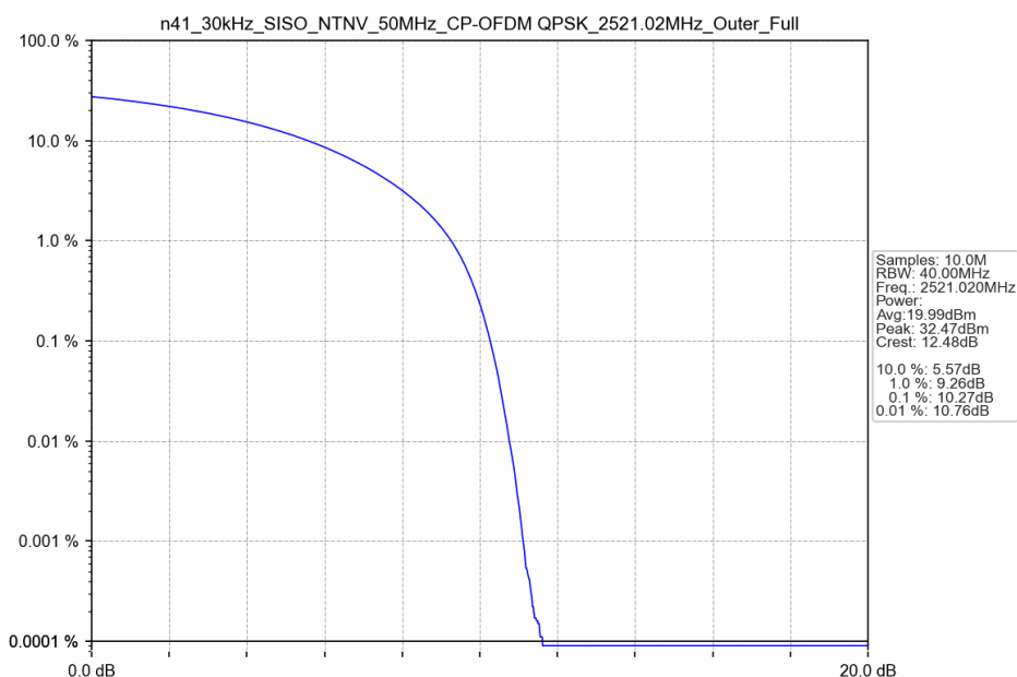
n41_30kHz_SISO_NTNV_50MHz_CP-OFDM QPSK_2521.02MHz_Outer_Full
