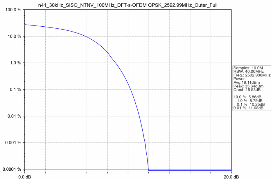
n41_30kHz_SISO_NTNV_100MHz_DFT-s-OFDM QPSK_2592.99MHz_Outer_Full
