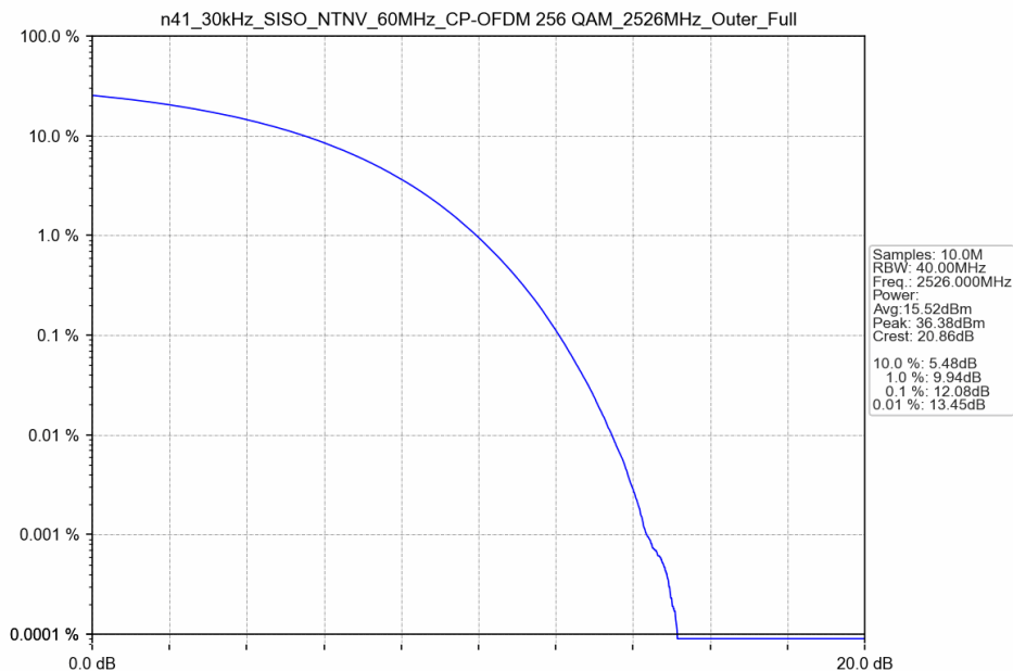
n41_30kHz_SISO_NTNV_60MHz_CP-OFDM 256 QAM_2526MHz_Outer_Full
