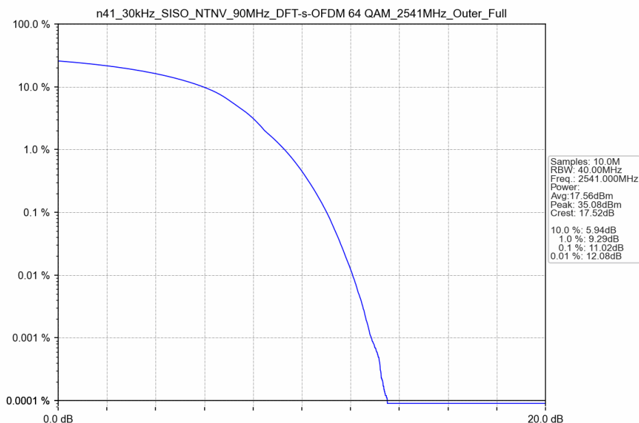
n41_30kHz_SISO_NTNV_90MHz_DFT-s-OFDM 64 QAM_2541MHz_Outer_Full
