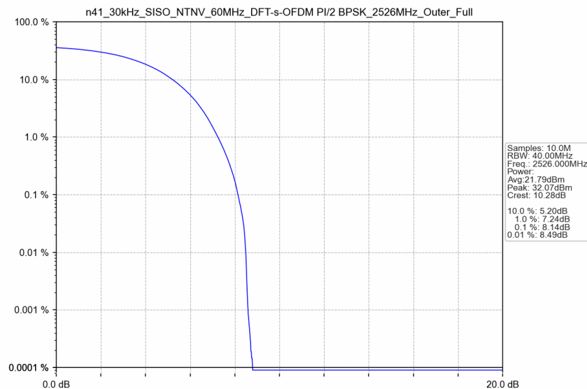
n41_30kHz_SISO_NTNV_60MHz_DFT-s-OFDM PI/2 BPSK_2526MHz_Outer_Full
