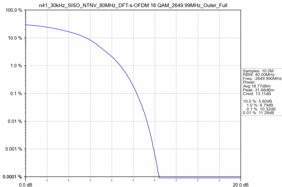
n41_30kHz_SISO_NTNV_80MHz_DFT-s-OFDM 16 QAM_2649.99MHz_Outer_Full
