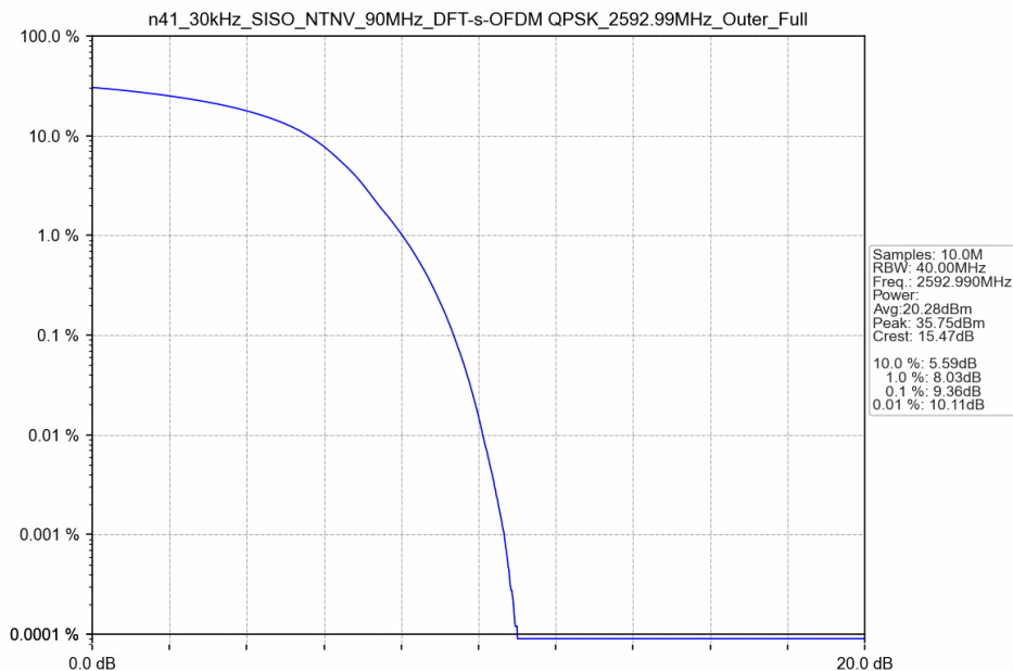
n41_30kHz_SISO_NTNV_90MHz_DFT-s-OFDM QPSK_2592.99MHz_Outer_Full
