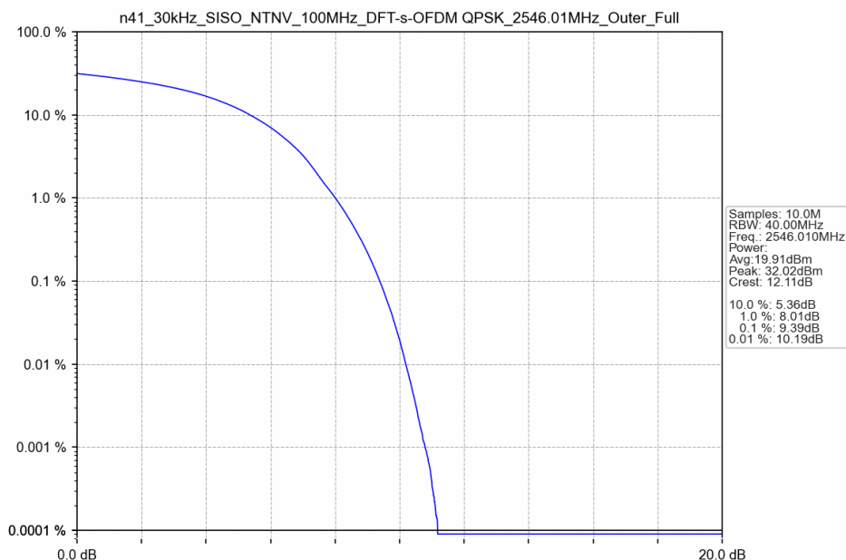
n41_30kHz_SISO_NTNV_100MHz_DFT-s-OFDM QPSK_2546.01MHz_Outer_Full
