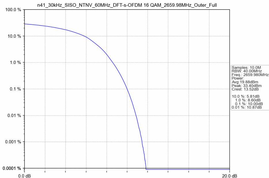
n41_30kHz_SISO_NTNV_60MHz_DFT-s-OFDM 16 QAM_2659.98MHz_Outer_Full
