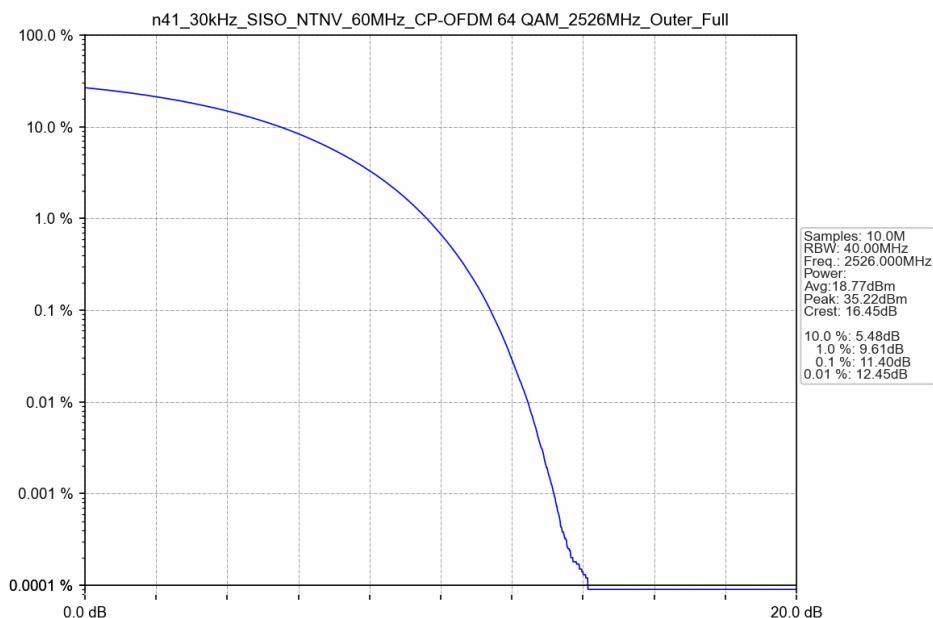
n41_30kHz_SISO_NTNV_60MHz_CP-OFDM 64 QAM_2526MHz_Outer_Full
