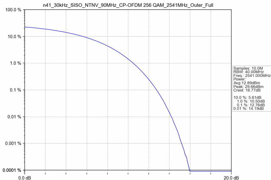
n41_30kHz_SISO_NTNV_90MHz_CP-OFDM 256 QAM_2541MHz_Outer_Full
