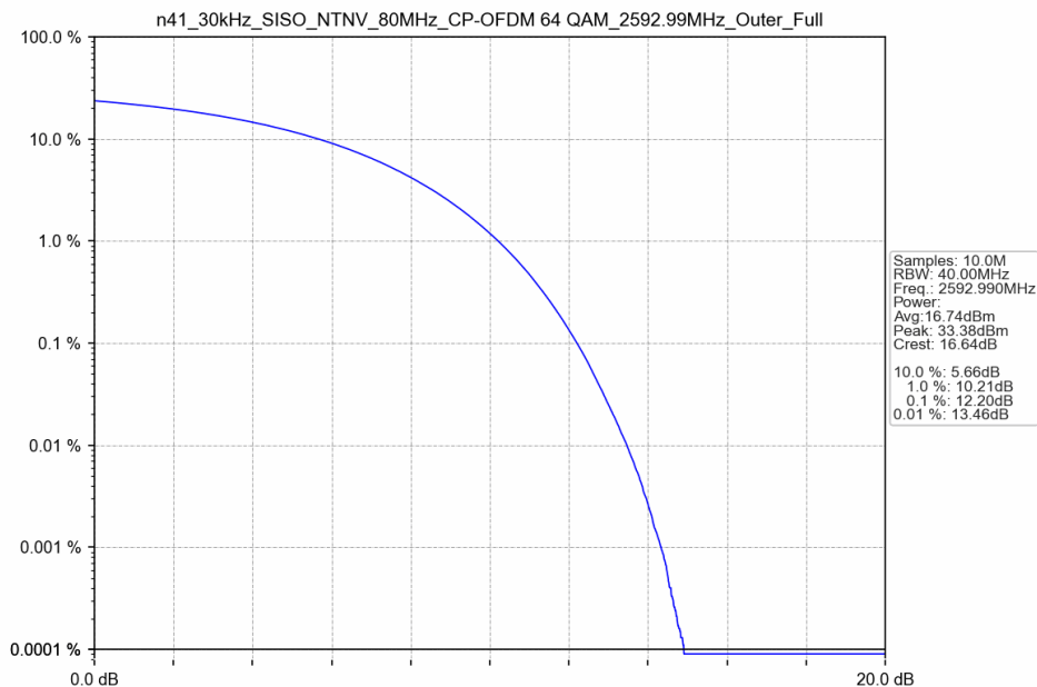
n41_30kHz_SISO_NTNV_80MHz_CP-OFDM 64 QAM_2592.99MHz_Outer_Full
