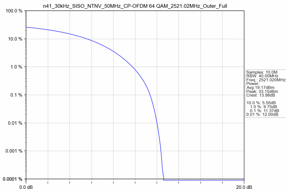
n41_30kHz_SISO_NTNV_50MHz_CP-OFDM 64 QAM_2521.02MHz_Outer_Full
