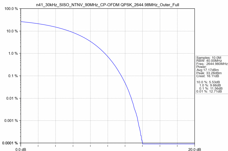
n41_30kHz_SISO_NTNV_90MHz_CP-OFDM QPSK_2644.98MHz_Outer_Full
