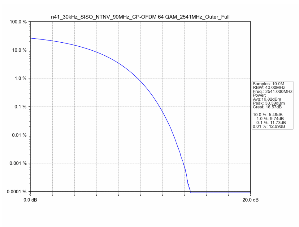
n41_30kHz_SISO_NTNV_90MHz_CP-OFDM 64 QAM_2541MHz_Outer_Full
