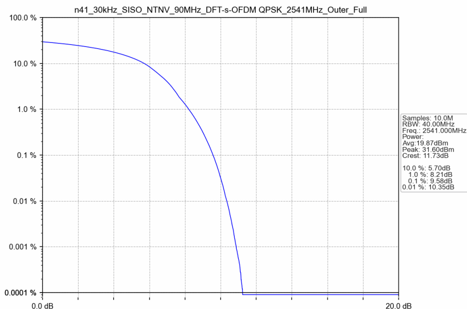
n41_30kHz_SISO_NTNV_90MHz_DFT-s-OFDM QPSK_2541MHz_Outer_Full
