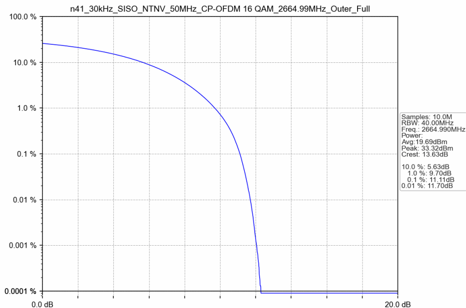
n41_30kHz_SISO_NTNV_50MHz_CP-OFDM 16 QAM_2664.99MHz_Outer_Full
