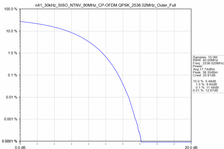
n41_30kHz_SISO_NTNV_80MHz_CP-OFDM QPSK_2536.02MHz_Outer_Full
