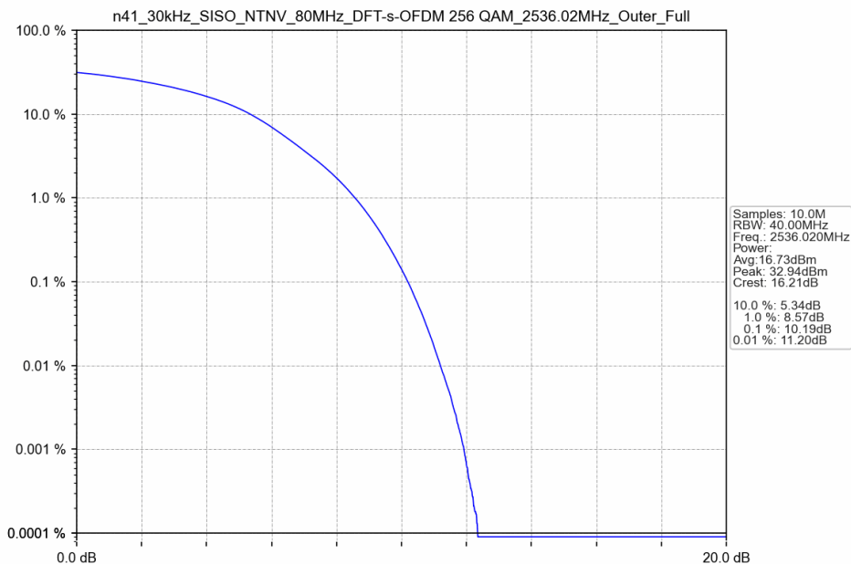
n41_30kHz_SISO_NTNV_80MHz_DFT-s-OFDM 256 QAM_2536.02MHz_Outer_Full
