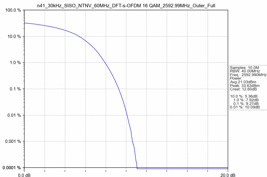
n41_30kHz_SISO_NTNV_60MHz_DFT-s-OFDM 16 QAM_2592.99MHz_Outer_Full
