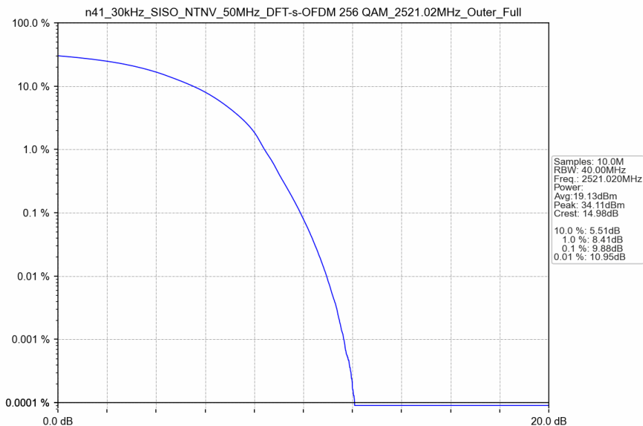
n41_30kHz_SISO_NTNV_50MHz_DFT-s-OFDM 256 QAM_2521.02MHz_Outer_Full
