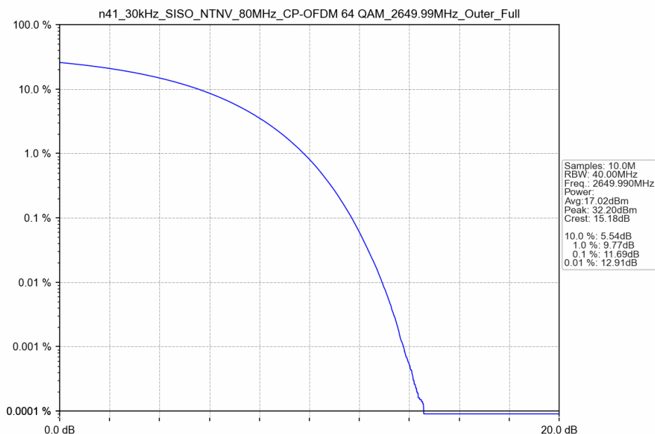
n41_30kHz_SISO_NTNV_80MHz_CP-OFDM 64 QAM_2649.99MHz_Outer_Full
