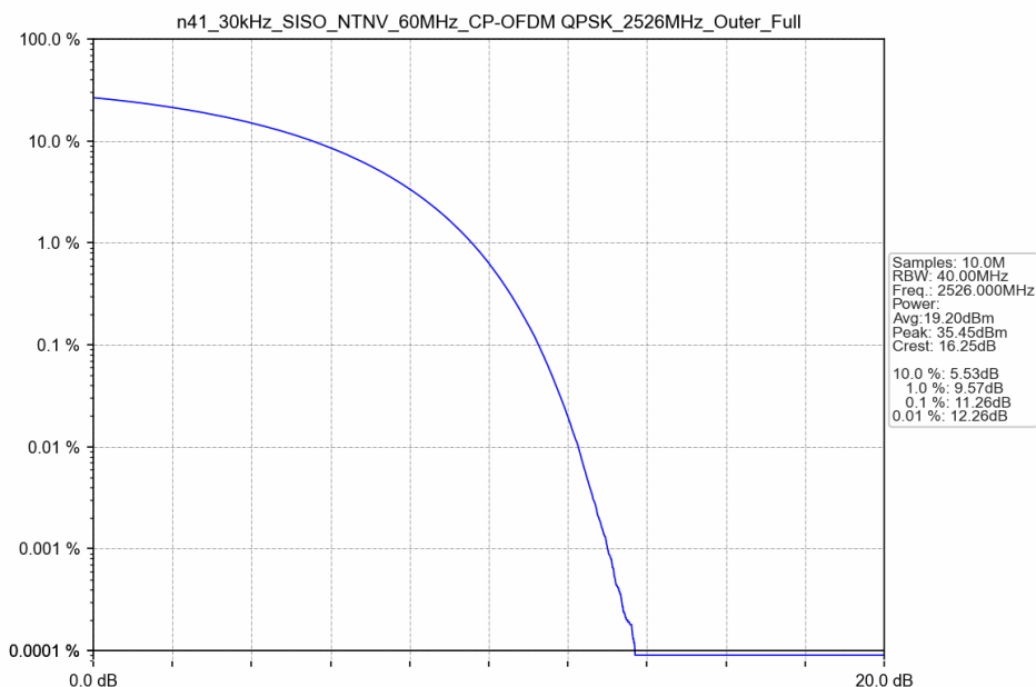
n41_30kHz_SISO_NTNV_60MHz_CP-OFDM QPSK_2526MHz_Outer_Full
