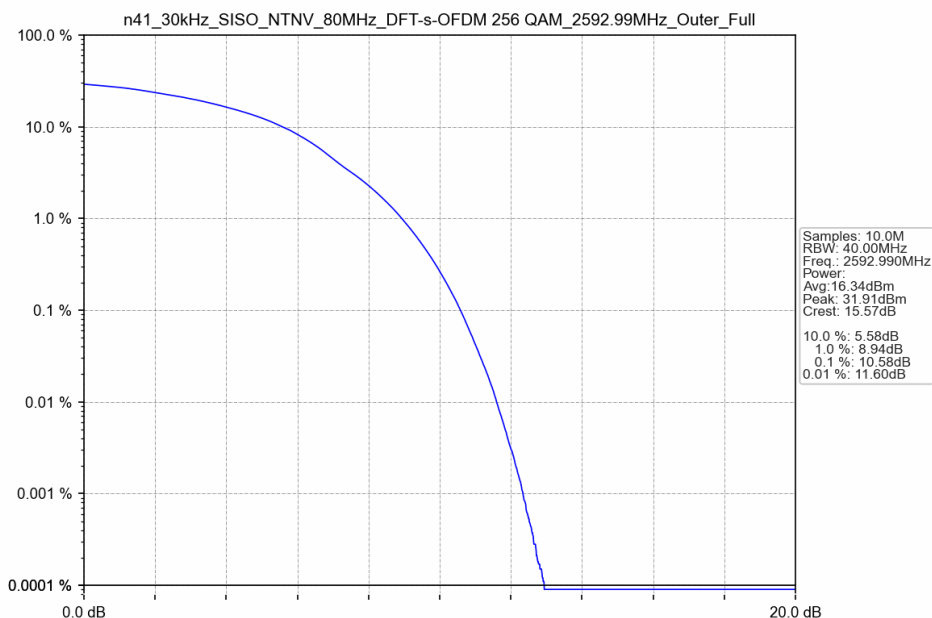
n41_30kHz_SISO_NTNV_80MHz_DFT-s-OFDM 256 QAM_2592.99MHz_Outer_Full
