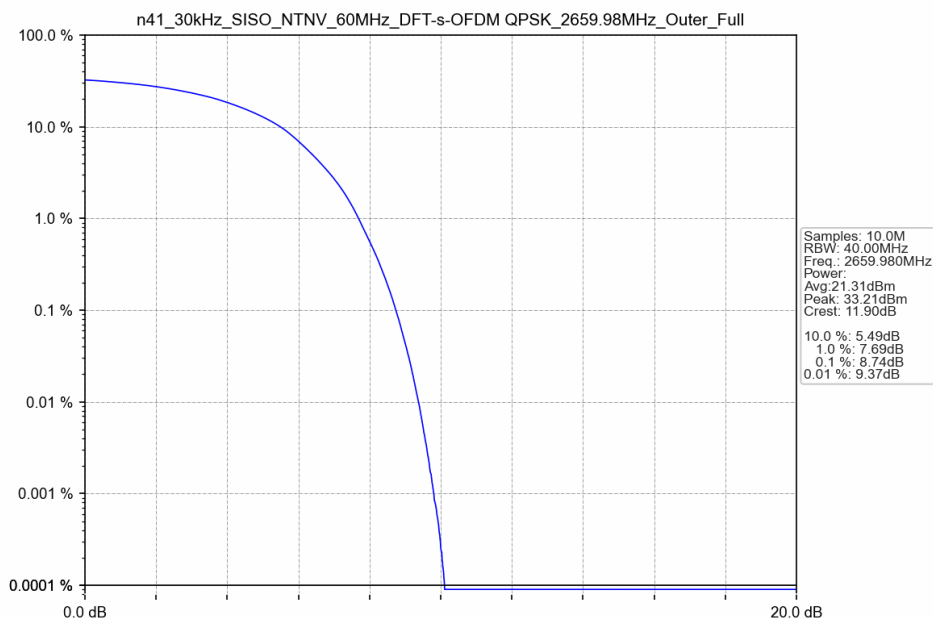
n41_30kHz_SISO_NTNV_60MHz_DFT-s-OFDM QPSK_2659.98MHz_Outer_Full
