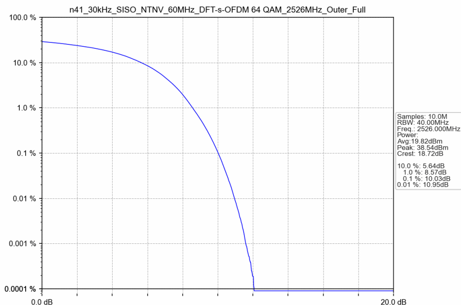
n41_30kHz_SISO_NTNV_60MHz_DFT-s-OFDM 64 QAM_2526MHz_Outer_Full
