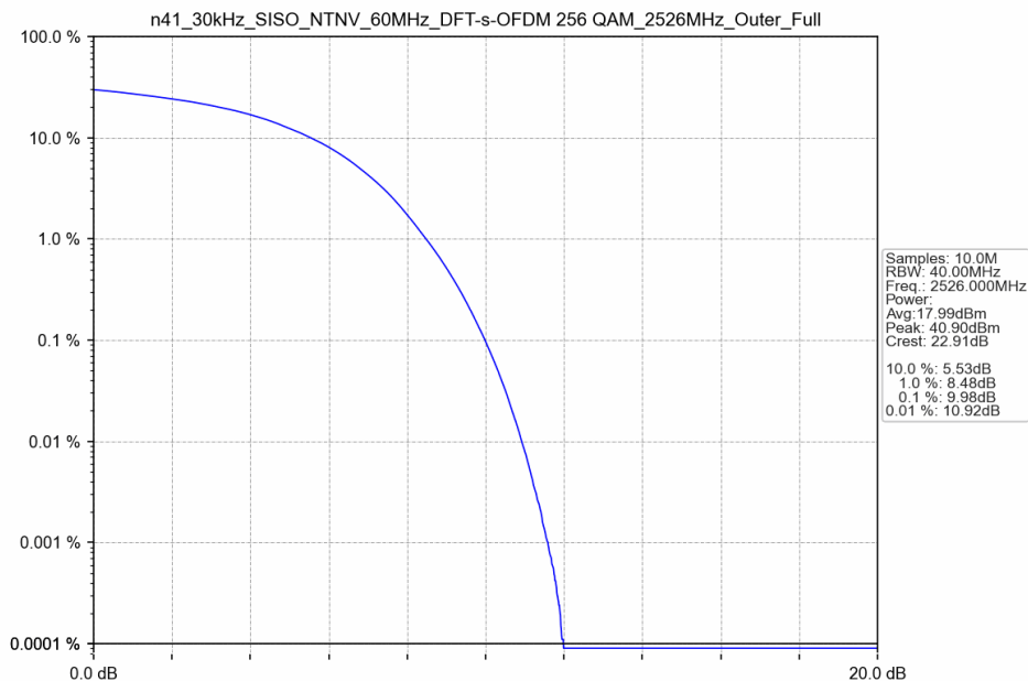
n41_30kHz_SISO_NTNV_60MHz_DFT-s-OFDM 256 QAM_2526MHz_Outer_Full
