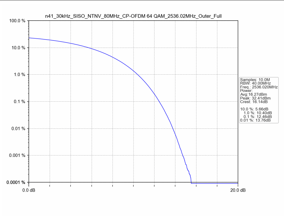
n41_30kHz_SISO_NTNV_80MHz_CP-OFDM 64 QAM_2536.02MHz_Outer_Full
