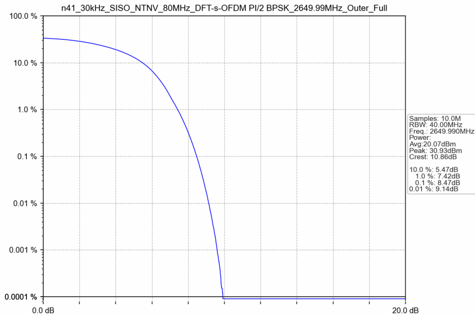
n41_30kHz_SISO_NTNV_80MHz_DFT-s-OFDM PI/2 BPSK_2649.99MHz_Outer_Full
