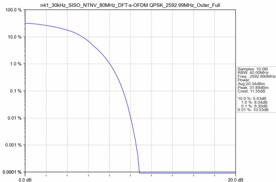
n41_30kHz_SISO_NTNV_80MHz_DFT-s-OFDM QPSK_2592.99MHz_Outer_Full
