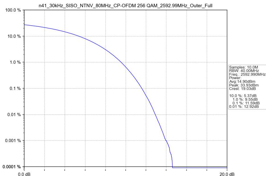
n41_30kHz_SISO_NTNV_80MHz_CP-OFDM 256 QAM_2592.99MHz_Outer_Full
