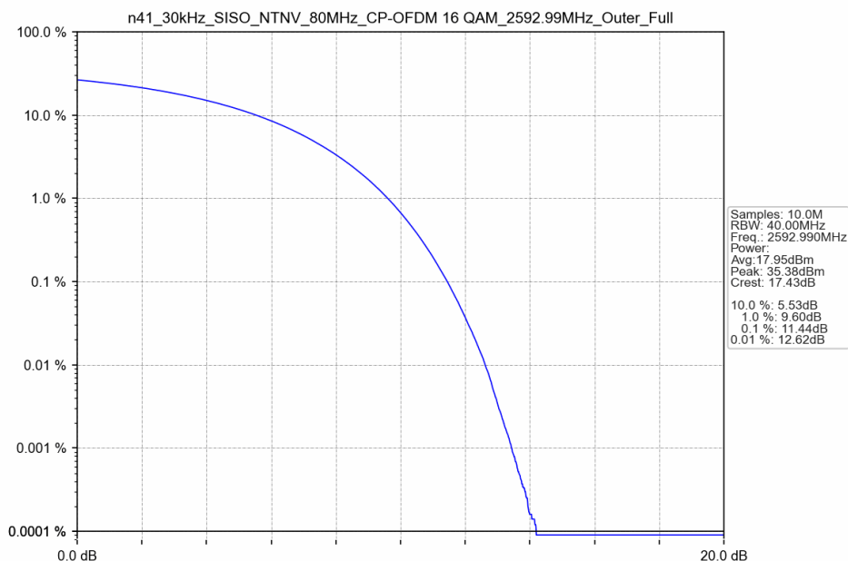
n41_30kHz_SISO_NTNV_80MHz_CP-OFDM 16 QAM_2592.99MHz_Outer_Full
