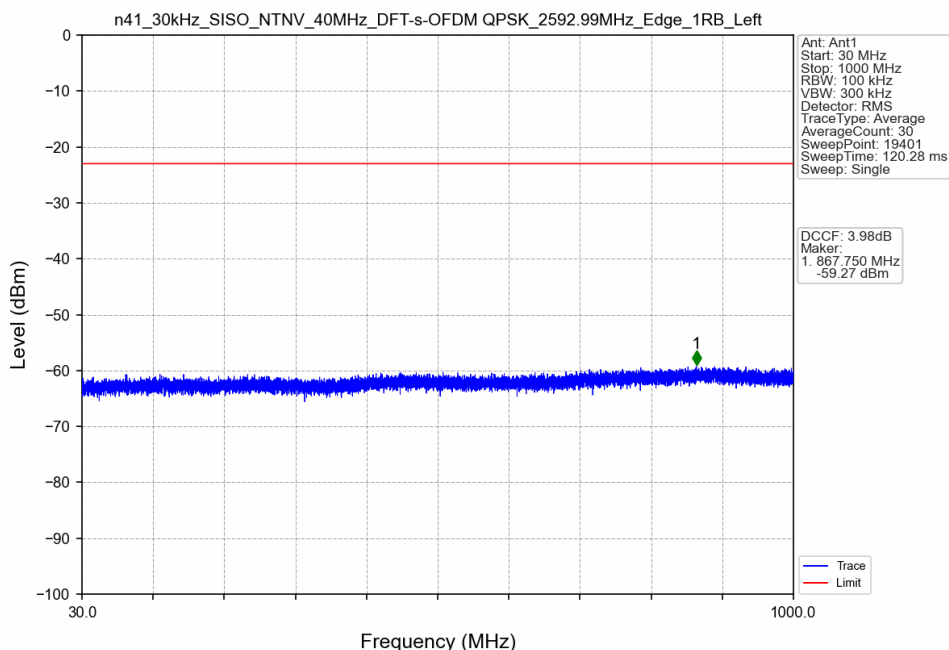
n41_30kHz_SISO_NTNV_40MHz_DFT-s-OFDM QPSK_2592.99MHz_Edge_1RB_Left
