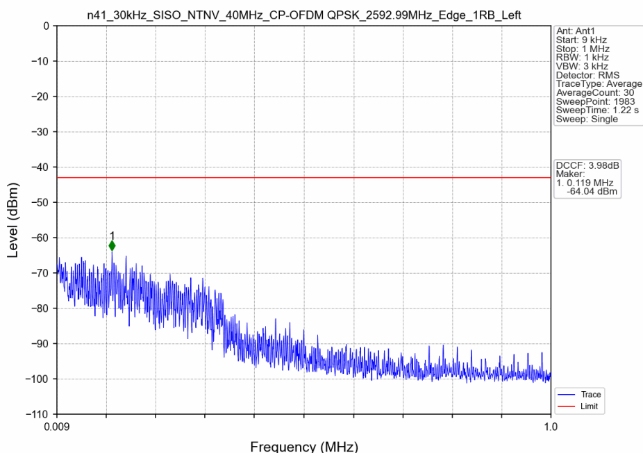
n41_30kHz_SISO_NTNV_40MHz_CP-OFDM QPSK_2592.99MHz_Edge_1RB_Left
