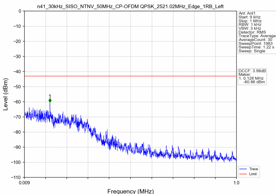
n41_30kHz_SISO_NTNV_50MHz_CP-OFDM QPSK_2521.02MHz_Edge_1RB_Left
