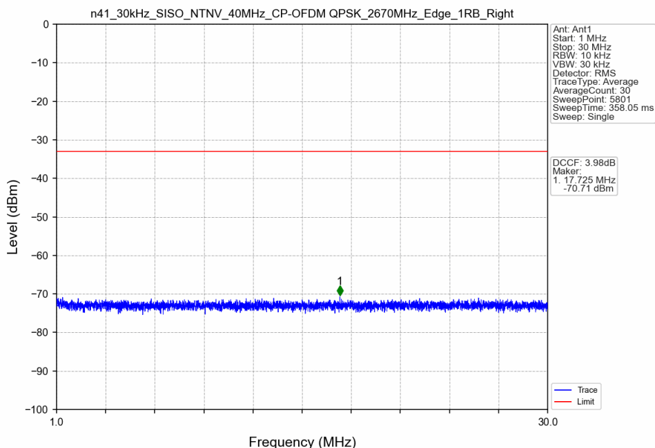
n41_30kHz_SISO_NTNV_40MHz_CP-OFDM QPSK_2670MHz_Edge_1RB_Right
