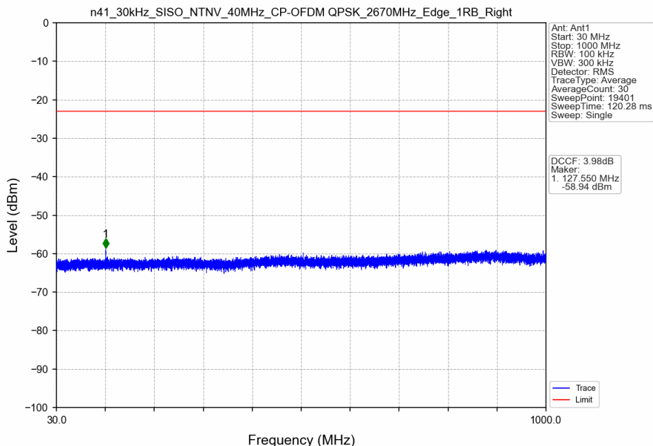
n41_30kHz_SISO_NTNV_40MHz_CP-OFDM QPSK_2670MHz_Edge_1RB_Right
