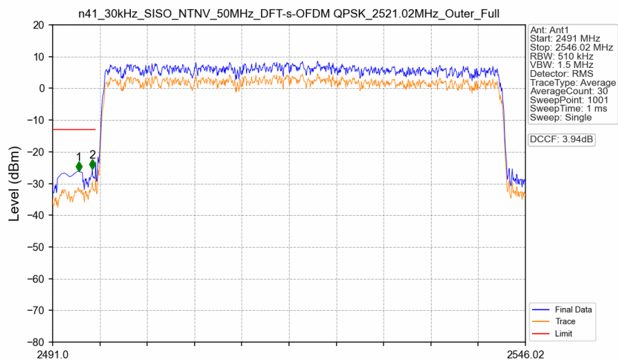
n41_30kHz_SISO_NTNV_50MHz_DFT-s-OFDM QPSK_2521.02MHz_Outer_Full
