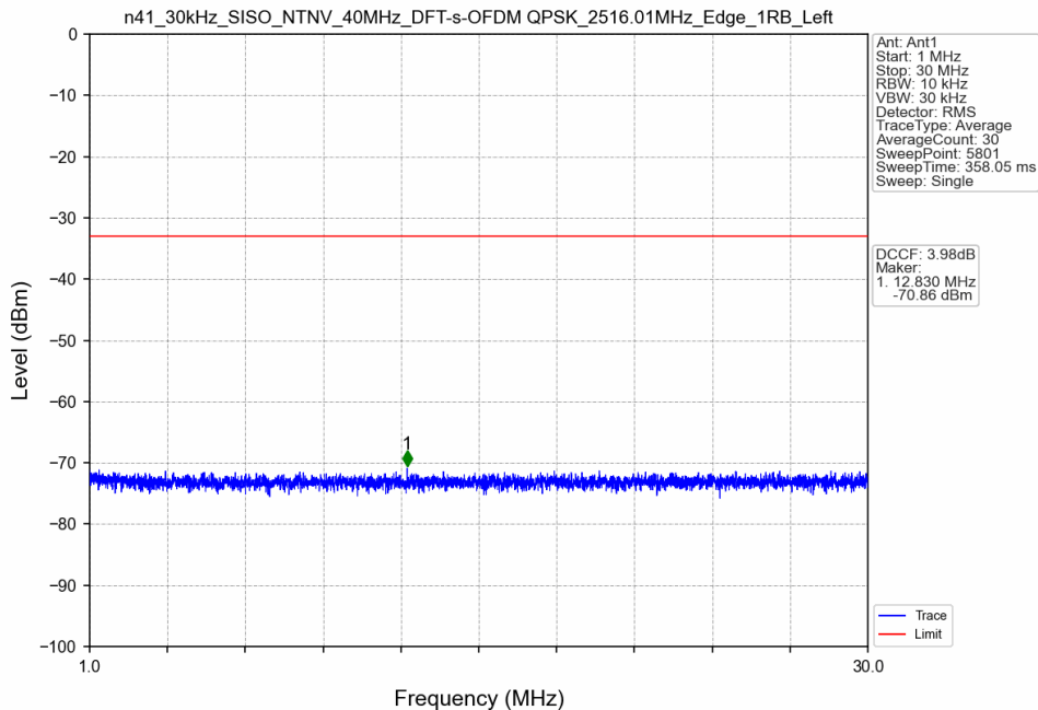
n41_30kHz_SISO_NTNV_40MHz_DFT-s-OFDM QPSK_2516.01MHz_Edge_1RB_Left
