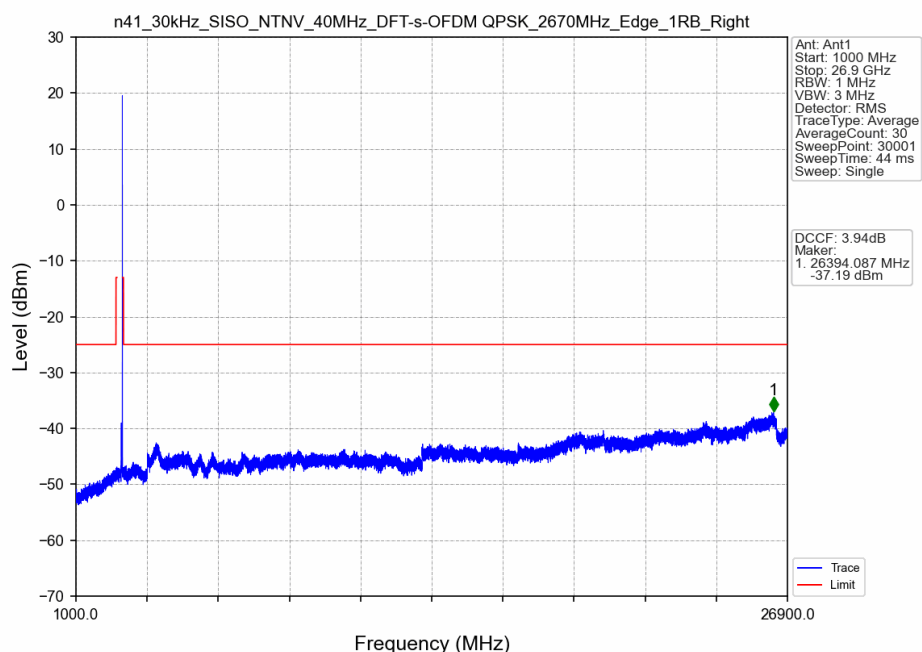
n41_30kHz_SISO_NTNV_40MHz_DFT-s-OFDM QPSK_2670MHz_Edge_1RB_Right
