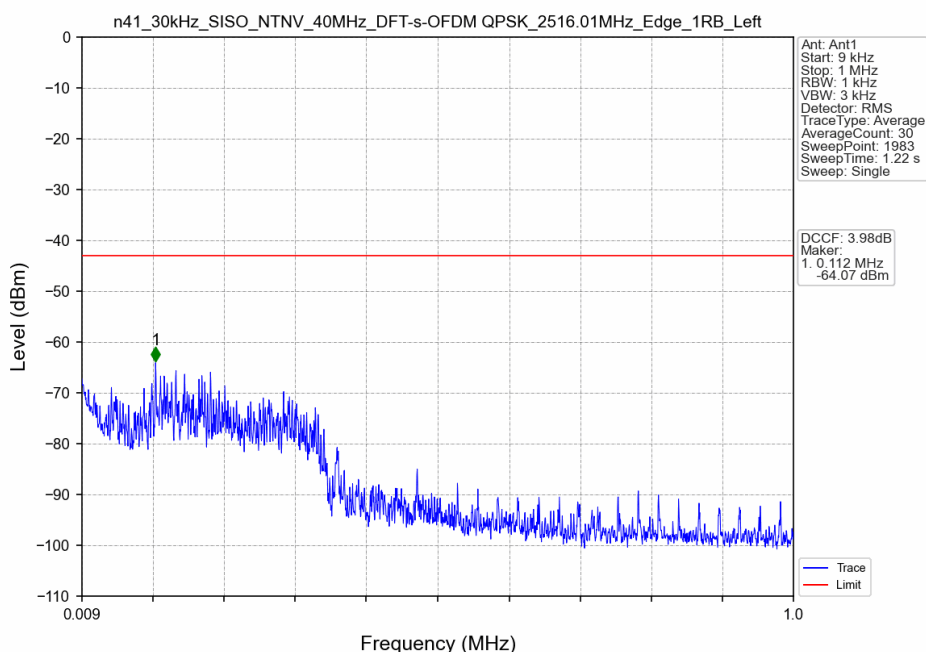
n41_30kHz_SISO_NTNV_40MHz_DFT-s-OFDM QPSK_2516.01MHz_Edge_1RB_Left
