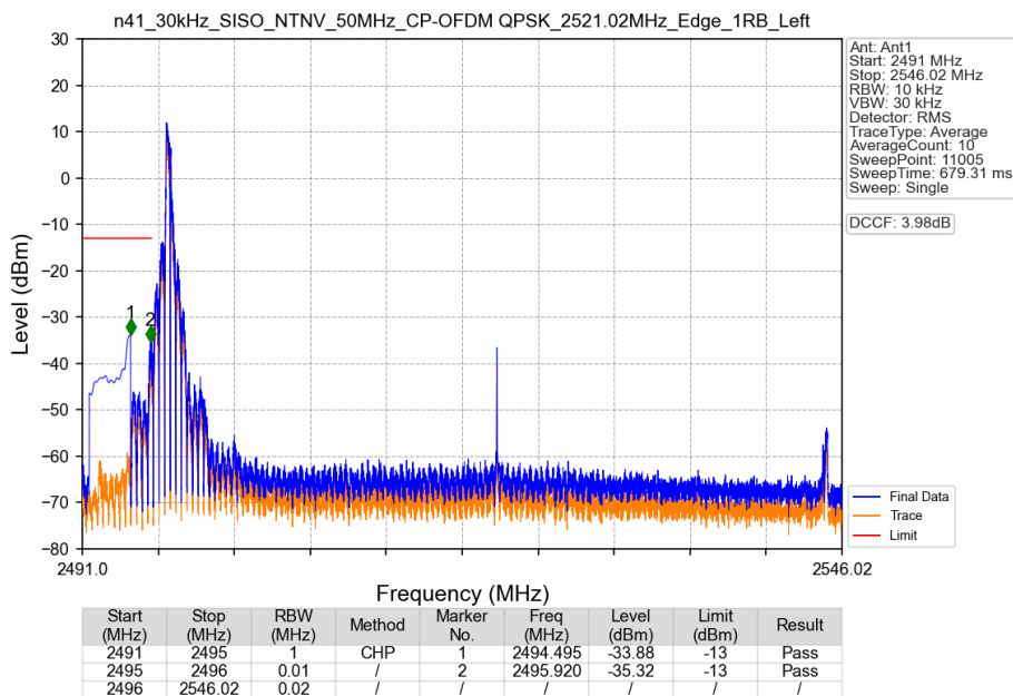
n41_30kHz_SISO_NTNV_50MHz_CP-OFDM QPSK_2521.02MHz_Edge_1RB_Left
