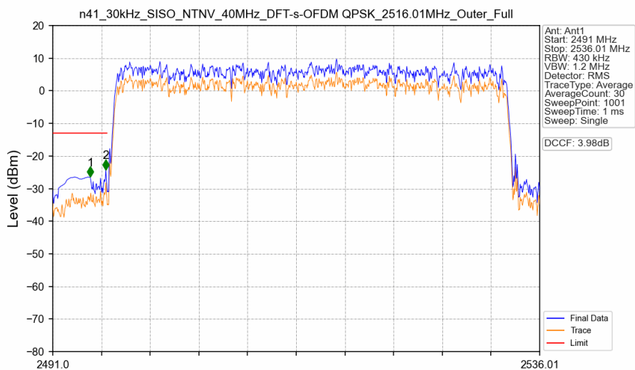
n41_30kHz_SISO_NTNV_40MHz_DFT-s-OFDM QPSK_2516.01MHz_Outer_Full
