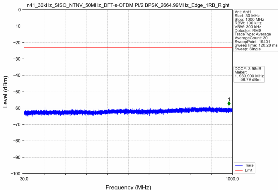
n41_30kHz_SISO_NTNV_50MHz_DFT-s-OFDM PI/2 BPSK_2664.99MHz_Edge_1RB_Right
