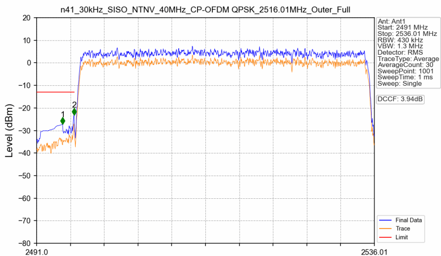
n41_30kHz_SISO_NTNV_40MHz_CP-OFDM QPSK_2516.01MHz_Outer_Full
