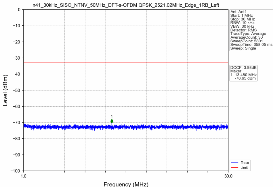
n41_30kHz_SISO_NTNV_50MHz_DFT-s-OFDM QPSK_2521.02MHz_Edge_1RB_Left
