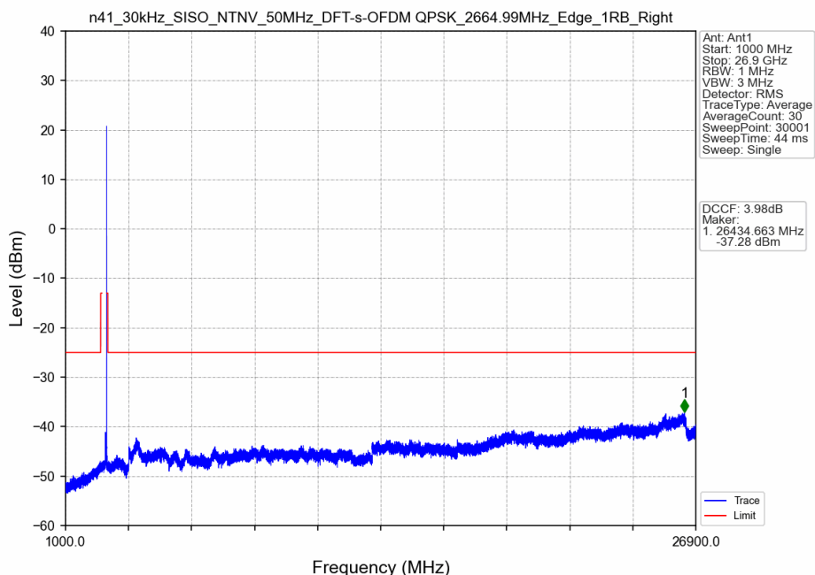
n41_30kHz_SISO_NTNV_50MHz_DFT-s-OFDM QPSK_2664.99MHz_Edge_1RB_Right
