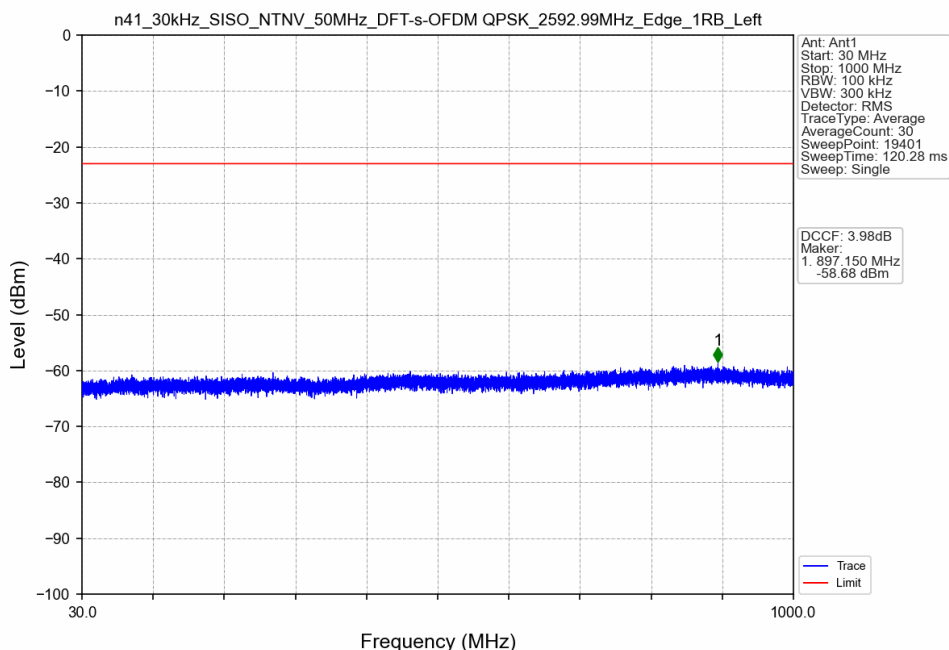
n41_30kHz_SISO_NTNV_50MHz_DFT-s-OFDM QPSK_2592.99MHz_Edge_1RB_Left
