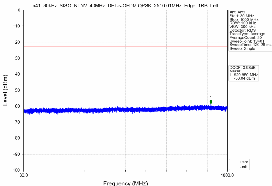
n41_30kHz_SISO_NTNV_40MHz_DFT-s-OFDM QPSK_2516.01MHz_Edge_1RB_Left
