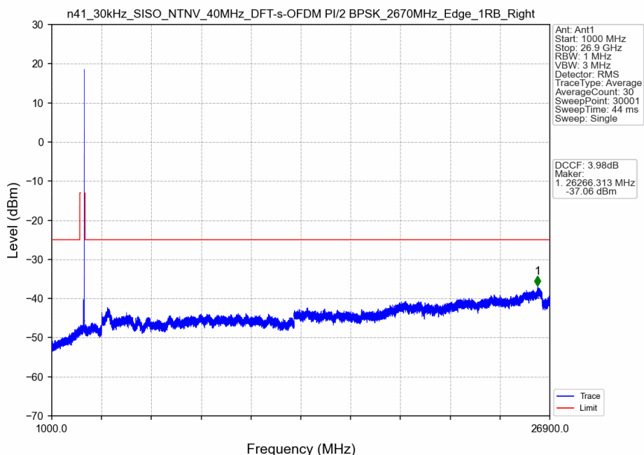
n41_30kHz_SISO_NTNV_40MHz_DFT-s-OFDM PI/2 BPSK_2670MHz_Edge_1RB_Right
