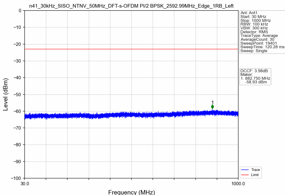
n41_30kHz_SISO_NTNV_50MHz_DFT-s-OFDM PI/2 BPSK_2592.99MHz_Edge_1RB_Left
