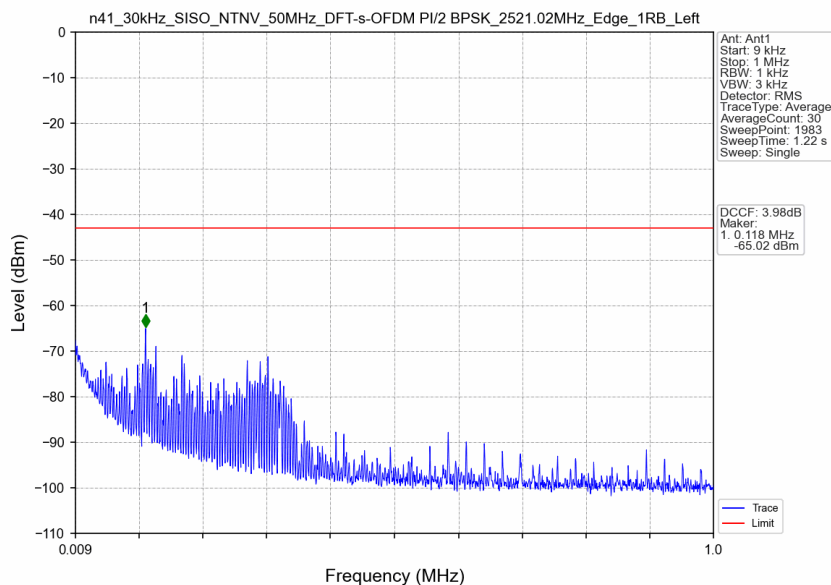
n41_30kHz_SISO_NTNV_50MHz_DFT-s-OFDM PI/2 BPSK_2521.02MHz_Edge_1RB_Left
