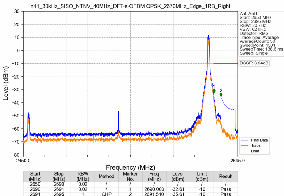
n41_30kHz_SISO_NTNV_40MHz_DFT-s-OFDM QPSK_2670MHz_Edge_1RB_Right
