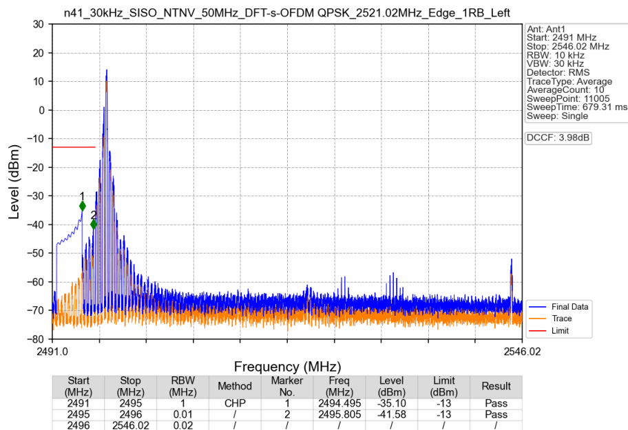
n41_30kHz_SISO_NTNV_50MHz_DFT-s-OFDM QPSK_2521.02MHz_Edge_1RB_Left
