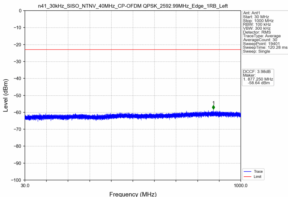
n41_30kHz_SISO_NTNV_40MHz_CP-OFDM QPSK_2592.99MHz_Edge_1RB_Left
