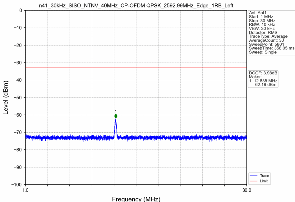
n41_30kHz_SISO_NTNV_40MHz_CP-OFDM QPSK_2592.99MHz_Edge_1RB_Left
