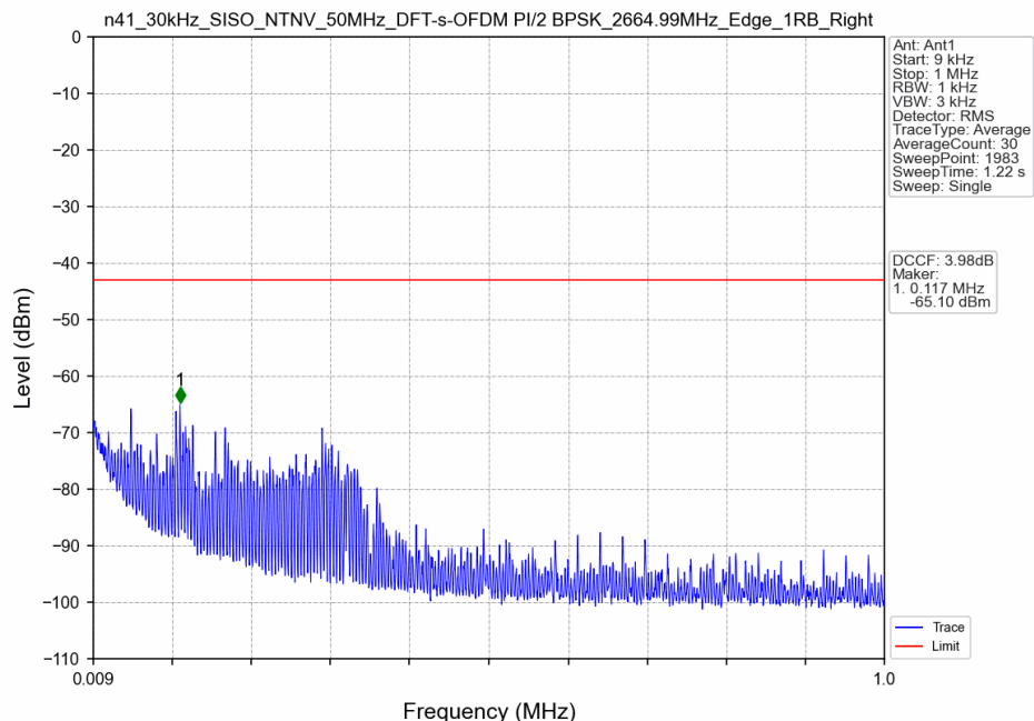
n41_30kHz_SISO_NTNV_50MHz_DFT-s-OFDM PI/2 BPSK_2664.99MHz_Edge_1RB_Right
