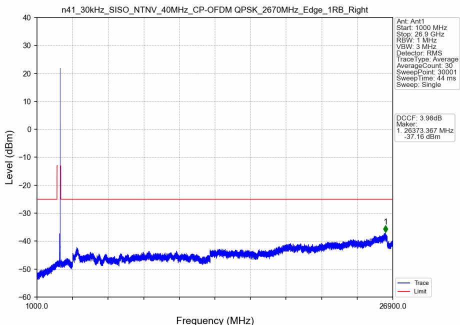
n41_30kHz_SISO_NTNV_40MHz_CP-OFDM QPSK_2670MHz_Edge_1RB_Right
