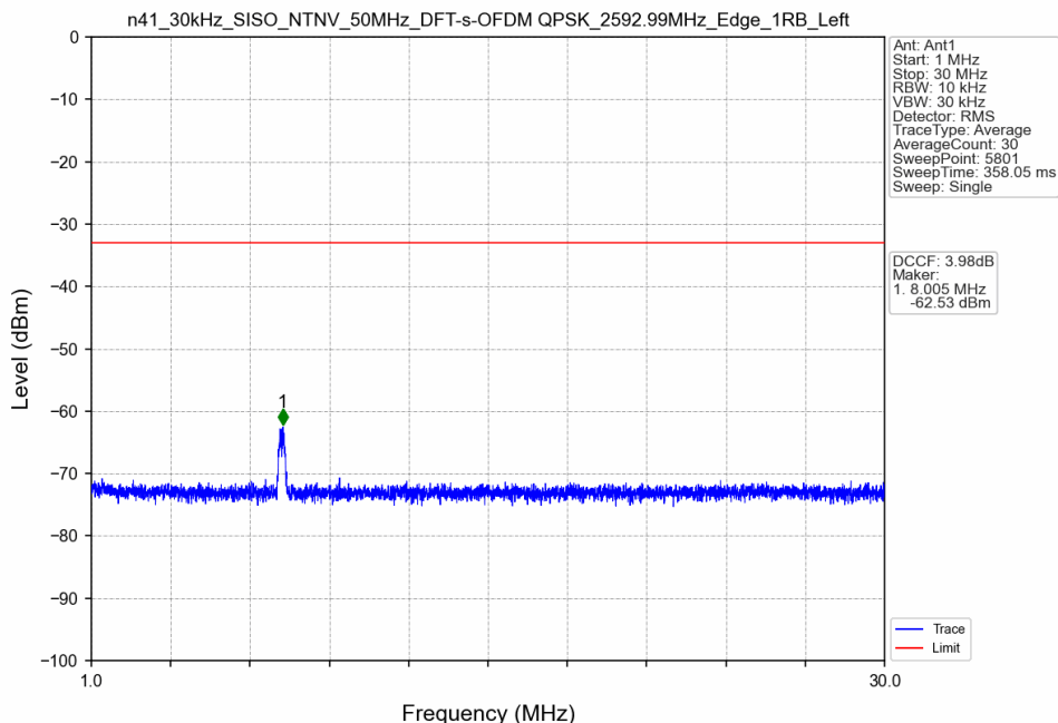
n41_30kHz_SISO_NTNV_50MHz_DFT-s-OFDM QPSK_2592.99MHz_Edge_1RB_Left
