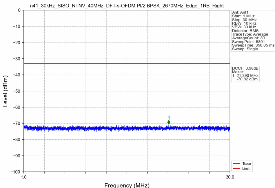
n41_30kHz_SISO_NTNV_40MHz_DFT-s-OFDM PI/2 BPSK_2670MHz_Edge_1RB_Right
