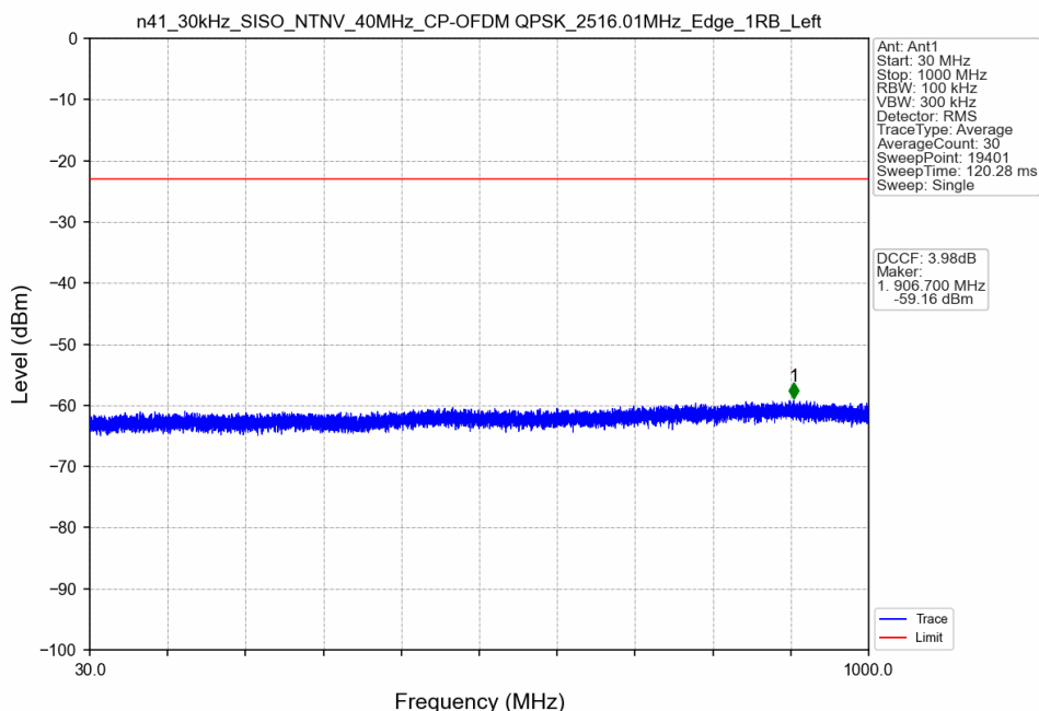
n41_30kHz_SISO_NTNV_40MHz_CP-OFDM QPSK_2516.01MHz_Edge_1RB_Left
