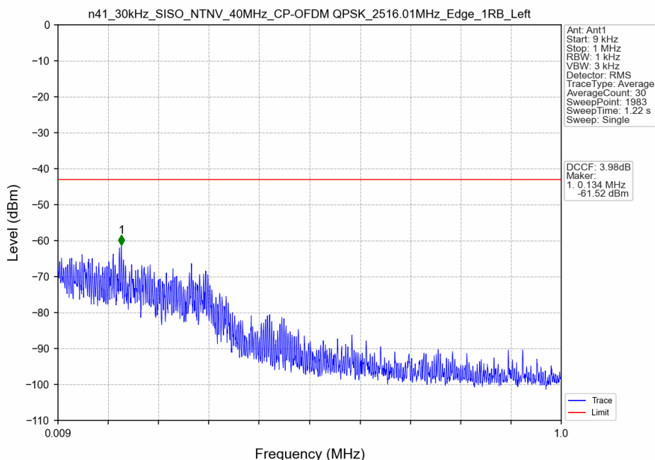
n41_30kHz_SISO_NTNV_40MHz_CP-OFDM QPSK_2516.01MHz_Edge_1RB_Left
