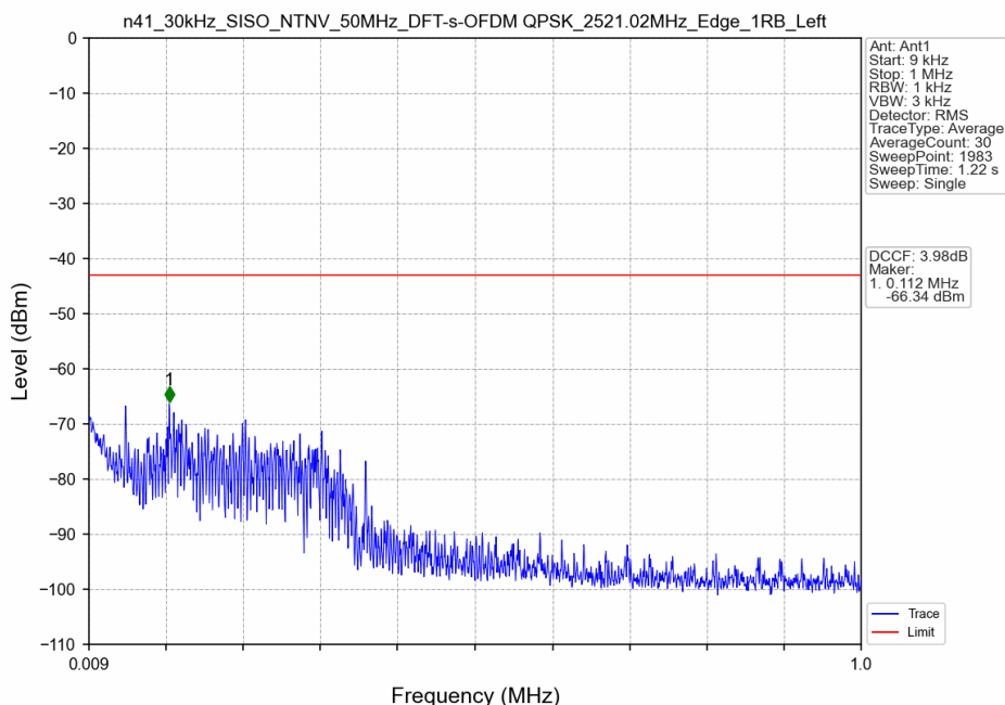
n41_30kHz_SISO_NTNV_50MHz_DFT-s-OFDM QPSK_2521.02MHz_Edge_1RB_Left
