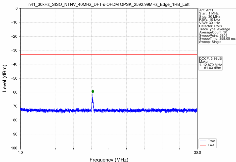
n41_30kHz_SISO_NTNV_40MHz_DFT-s-OFDM QPSK_2592.99MHz_Edge_1RB_Left
