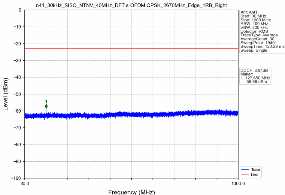
n41_30kHz_SISO_NTNV_40MHz_DFT-s-OFDM QPSK_2670MHz_Edge_1RB_Right
