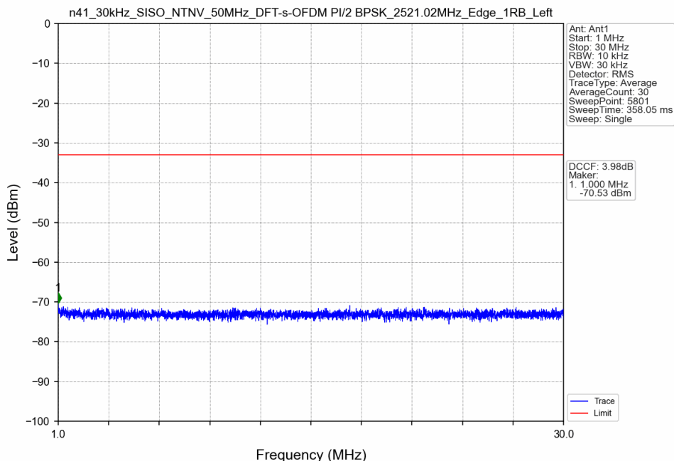
n41_30kHz_SISO_NTNV_50MHz_DFT-s-OFDM PI/2 BPSK_2521.02MHz_Edge_1RB_Left
