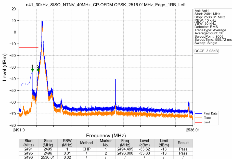
n41_30kHz_SISO_NTNV_40MHz_CP-OFDM QPSK_2516.01MHz_Edge_1RB_Left
