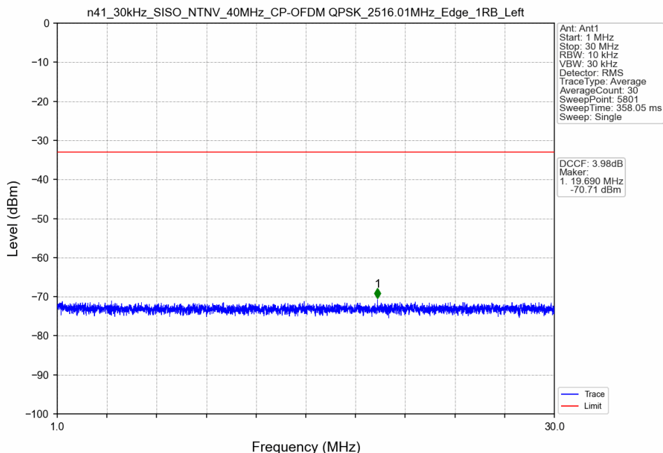
n41_30kHz_SISO_NTNV_40MHz_CP-OFDM QPSK_2516.01MHz_Edge_1RB_Left
