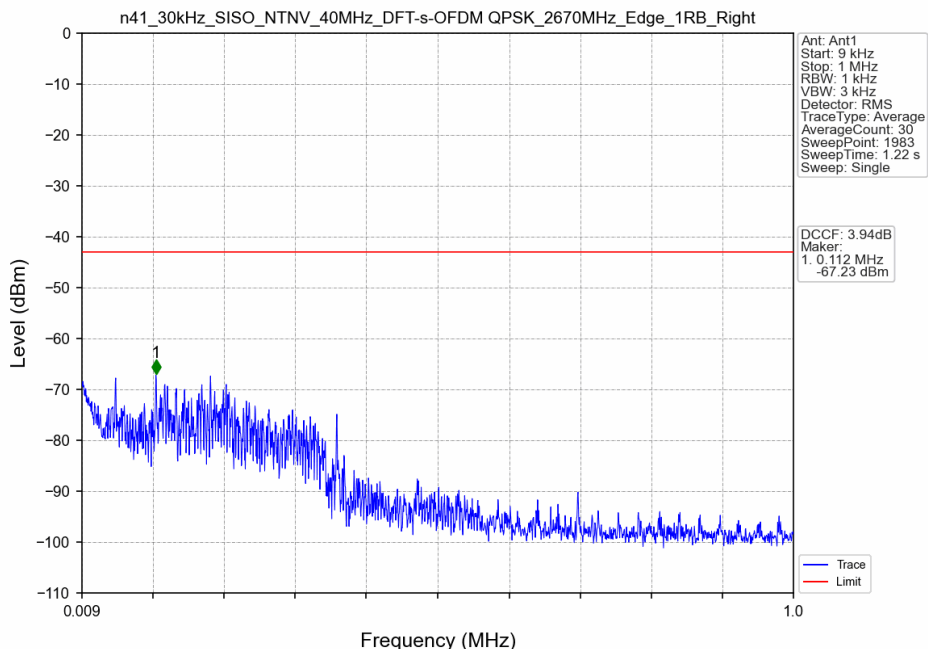
n41_30kHz_SISO_NTNV_40MHz_DFT-s-OFDM QPSK_2670MHz_Edge_1RB_Right
