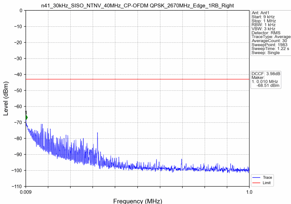
n41_30kHz_SISO_NTNV_40MHz_CP-OFDM QPSK_2670MHz_Edge_1RB_Right
