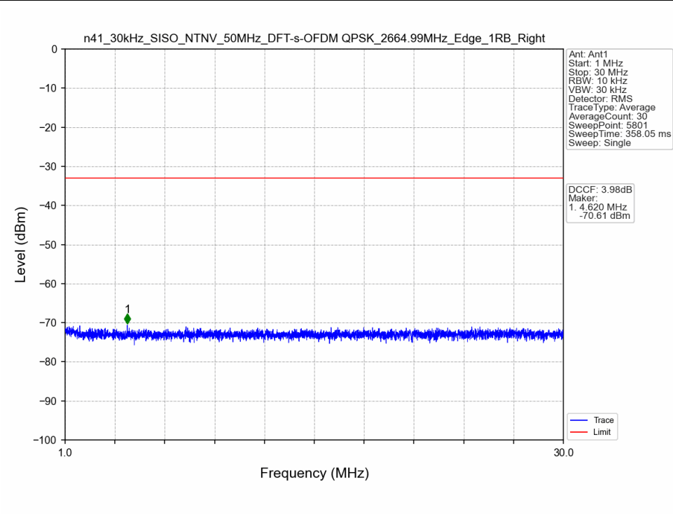
n41_30kHz_SISO_NTNV_50MHz_DFT-s-OFDM QPSK_2664.99MHz_Edge_1RB_Right
