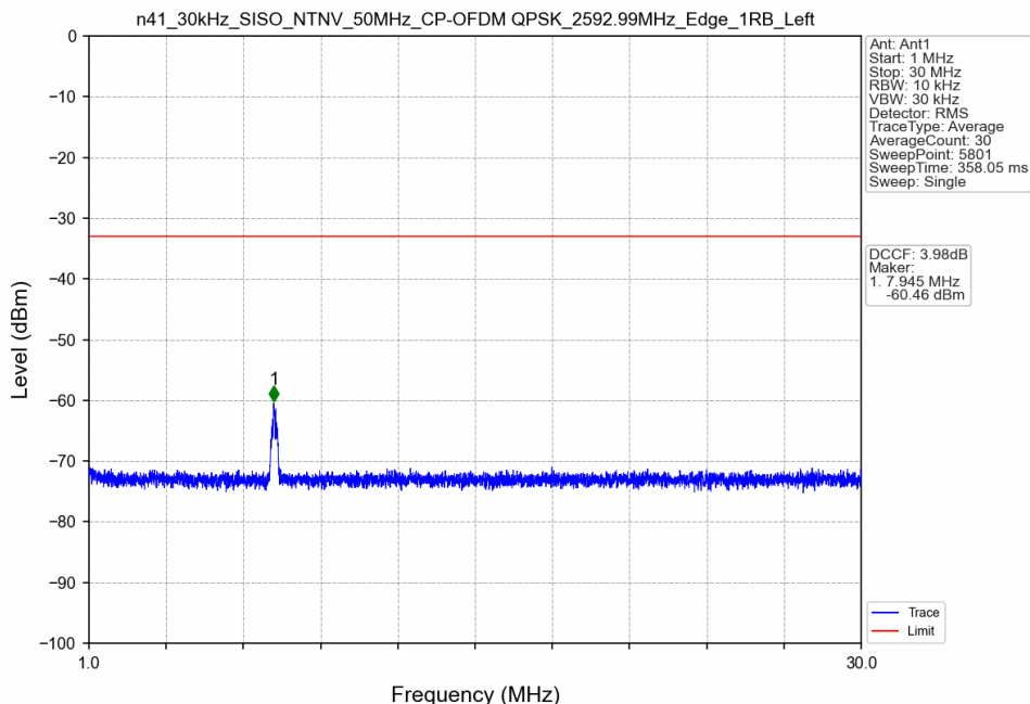
n41_30kHz_SISO_NTNV_50MHz_CP-OFDM QPSK_2592.99MHz_Edge_1RB_Left
