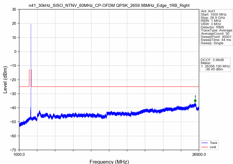
n41_30kHz_SISO_NTNV_60MHz_CP-OFDM QPSK_2659.98MHz_Edge_1RB_Right
