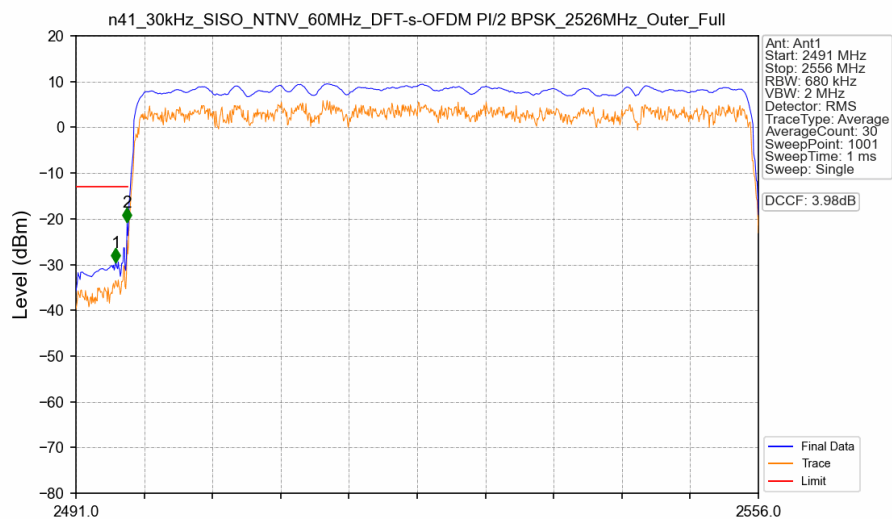
n41_30kHz_SISO_NTNV_60MHz_DFT-s-OFDM PI/2 BPSK_2526MHz_Outer_Full
