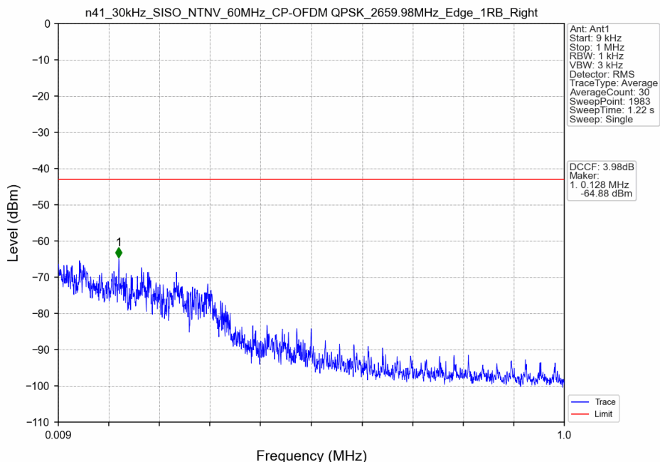
n41_30kHz_SISO_NTNV_60MHz_CP-OFDM QPSK_2659.98MHz_Edge_1RB_Right
