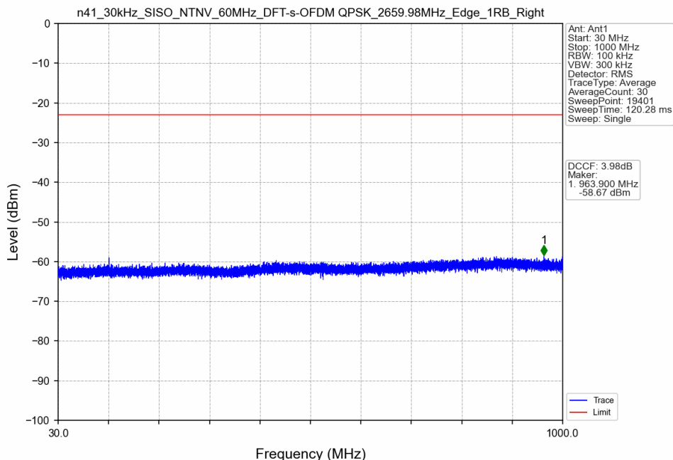
n41_30kHz_SISO_NTNV_60MHz_DFT-s-OFDM QPSK_2659.98MHz_Edge_1RB_Right
