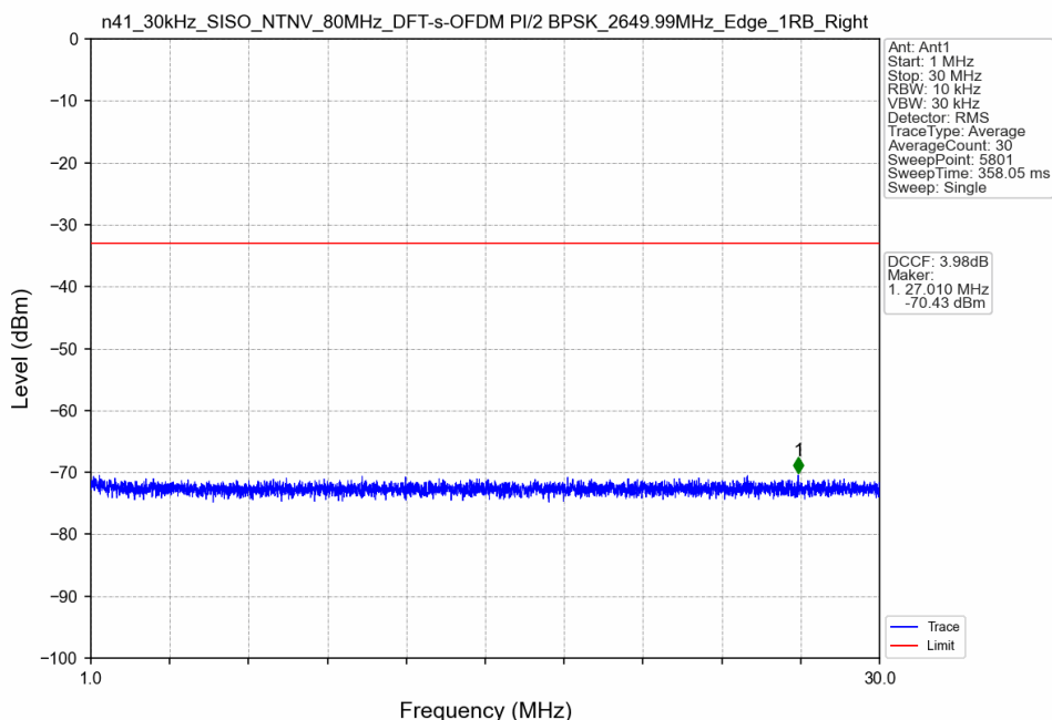
n41_30kHz_SISO_NTNV_80MHz_DFT-s-OFDM PI/2 BPSK_2649.99MHz_Edge_1RB_Right
