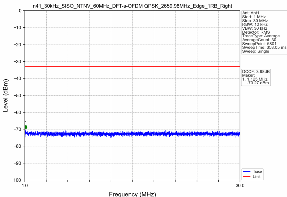
n41_30kHz_SISO_NTNV_60MHz_DFT-s-OFDM QPSK_2659.98MHz_Edge_1RB_Right
