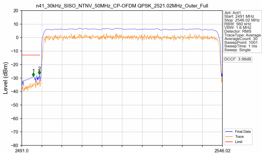
n41_30kHz_SISO_NTNV_50MHz_CP-OFDM QPSK_2521.02MHz_Outer_Full
