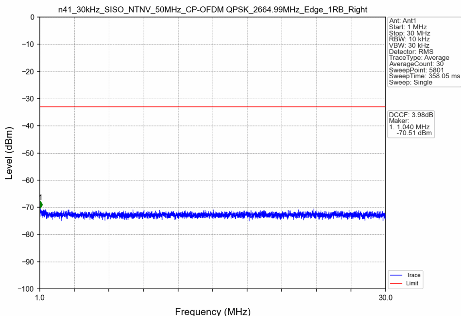
n41_30kHz_SISO_NTNV_50MHz_CP-OFDM QPSK_2664.99MHz_Edge_1RB_Right
