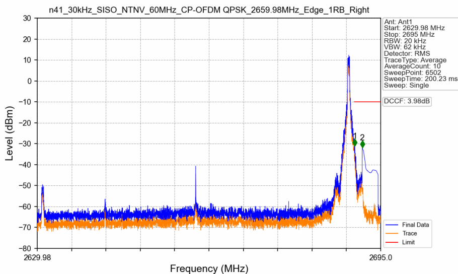
n41_30kHz_SISO_NTNV_60MHz_CP-OFDM QPSK_2659.98MHz_Edge_1RB_Right
