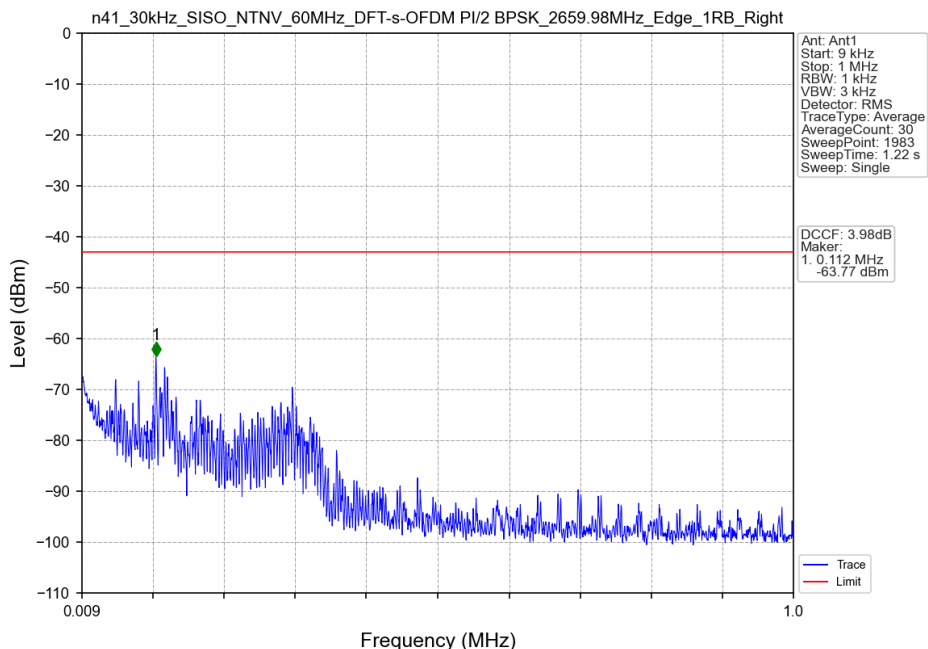
n41_30kHz_SISO_NTNV_60MHz_DFT-s-OFDM PI/2 BPSK_2659.98MHz_Edge_1RB_Right
