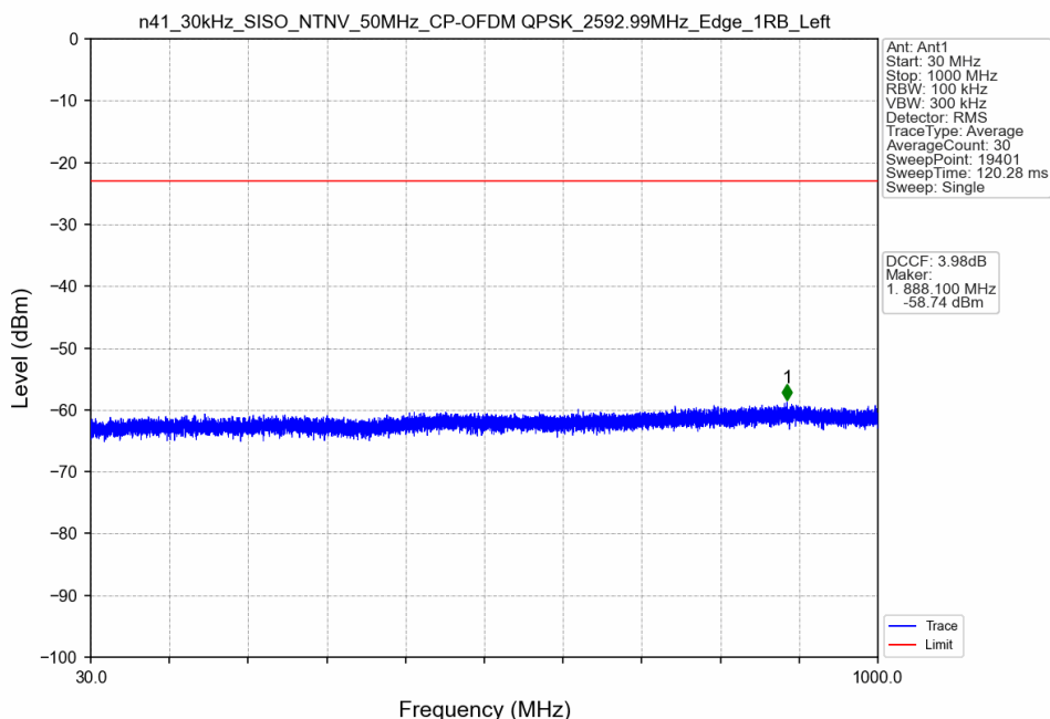
n41_30kHz_SISO_NTNV_50MHz_CP-OFDM QPSK_2592.99MHz_Edge_1RB_Left
