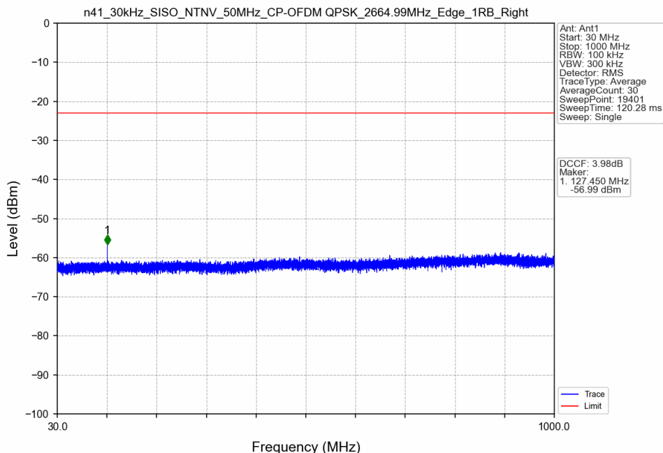
n41_30kHz_SISO_NTNV_50MHz_CP-OFDM QPSK_2664.99MHz_Edge_1RB_Right
