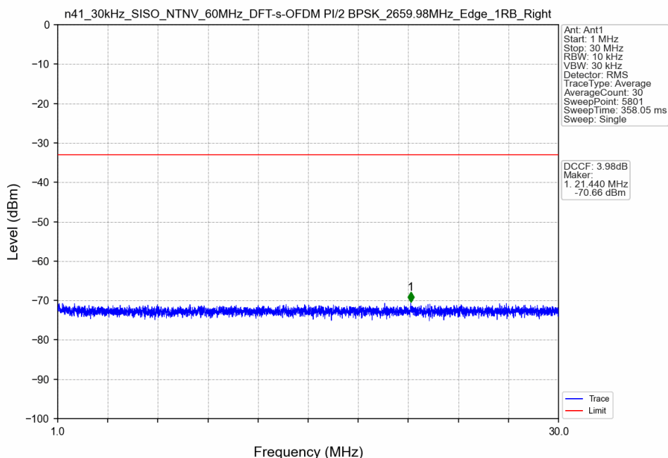
n41_30kHz_SISO_NTNV_60MHz_DFT-s-OFDM PI/2 BPSK_2659.98MHz_Edge_1RB_Right
