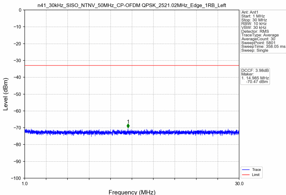
n41_30kHz_SISO_NTNV_50MHz_CP-OFDM QPSK_2521.02MHz_Edge_1RB_Left
