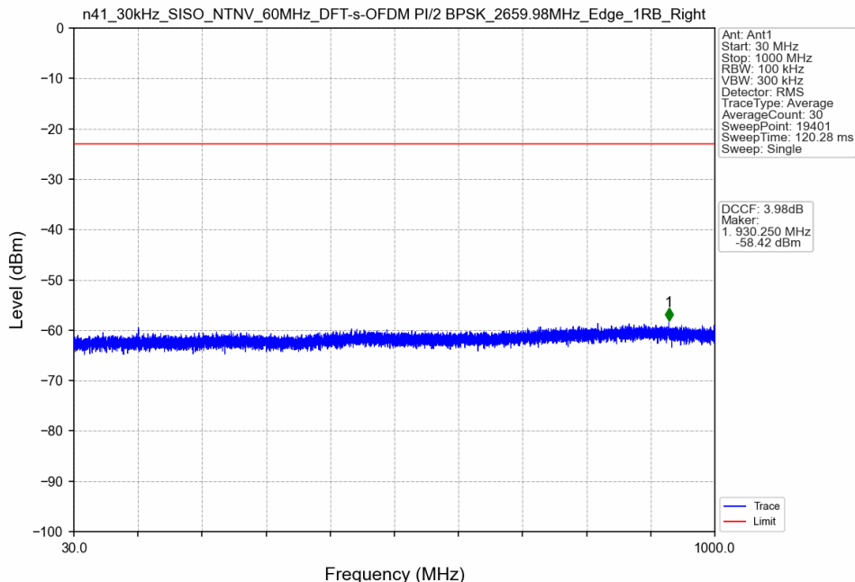
n41_30kHz_SISO_NTNV_60MHz_DFT-s-OFDM PI/2 BPSK_2659.98MHz_Edge_1RB_Right
