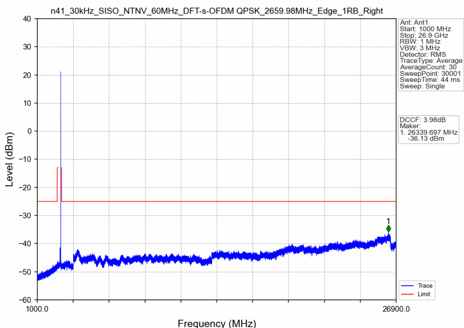
n41_30kHz_SISO_NTNV_60MHz_DFT-s-OFDM QPSK_2659.98MHz_Edge_1RB_Right
