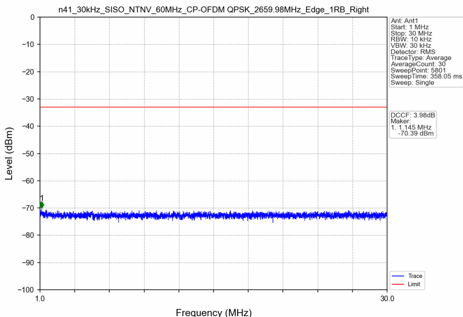
n41_30kHz_SISO_NTNV_60MHz_CP-OFDM QPSK_2659.98MHz_Edge_1RB_Right
