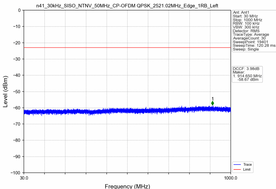
n41_30kHz_SISO_NTNV_50MHz_CP-OFDM QPSK_2521.02MHz_Edge_1RB_Left
