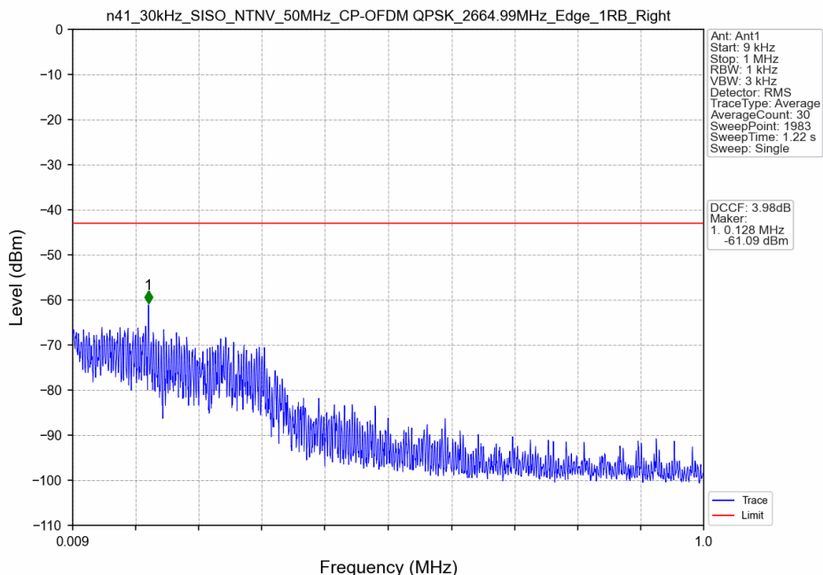
n41_30kHz_SISO_NTNV_50MHz_CP-OFDM QPSK_2664.99MHz_Edge_1RB_Right
