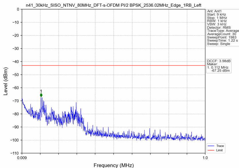
n41_30kHz_SISO_NTNV_80MHz_DFT-s-OFDM PI/2 BPSK_2536.02MHz_Edge_1RB_Left
