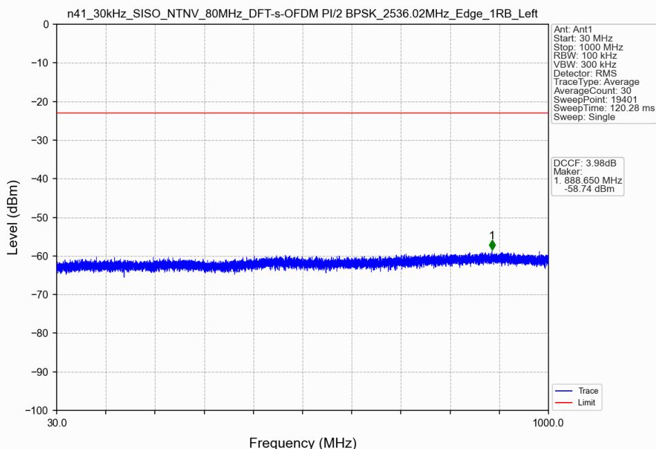
n41_30kHz_SISO_NTNV_80MHz_DFT-s-OFDM PI/2 BPSK_2536.02MHz_Edge_1RB_Left
