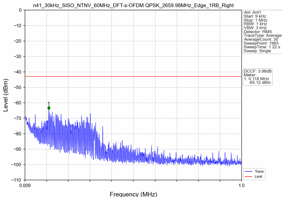
n41_30kHz_SISO_NTNV_60MHz_DFT-s-OFDM QPSK_2659.98MHz_Edge_1RB_Right
