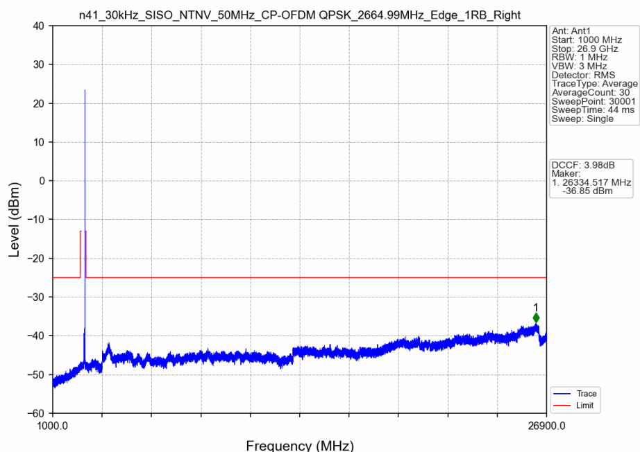
n41_30kHz_SISO_NTNV_50MHz_CP-OFDM QPSK_2664.99MHz_Edge_1RB_Right
