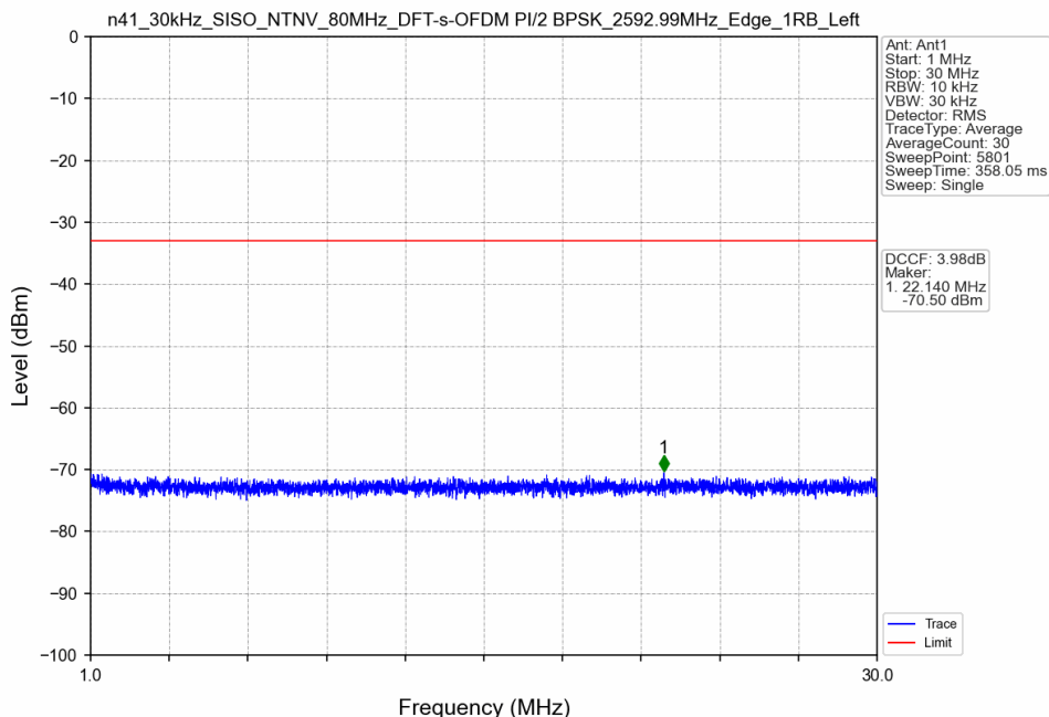
n41_30kHz_SISO_NTNV_80MHz_DFT-s-OFDM PI/2 BPSK_2592.99MHz_Edge_1RB_Left
