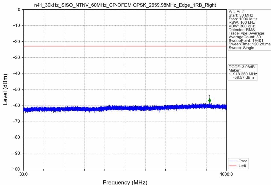
n41_30kHz_SISO_NTNV_60MHz_CP-OFDM QPSK_2659.98MHz_Edge_1RB_Right
