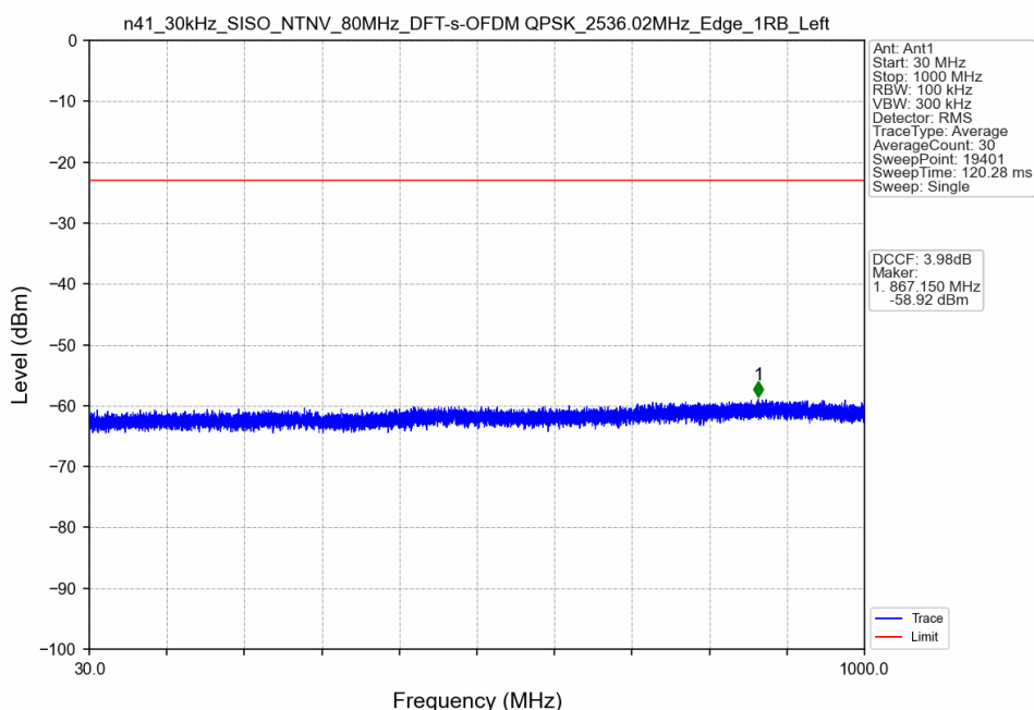
n41_30kHz_SISO_NTNV_80MHz_DFT-s-OFDM QPSK_2536.02MHz_Edge_1RB_Left
