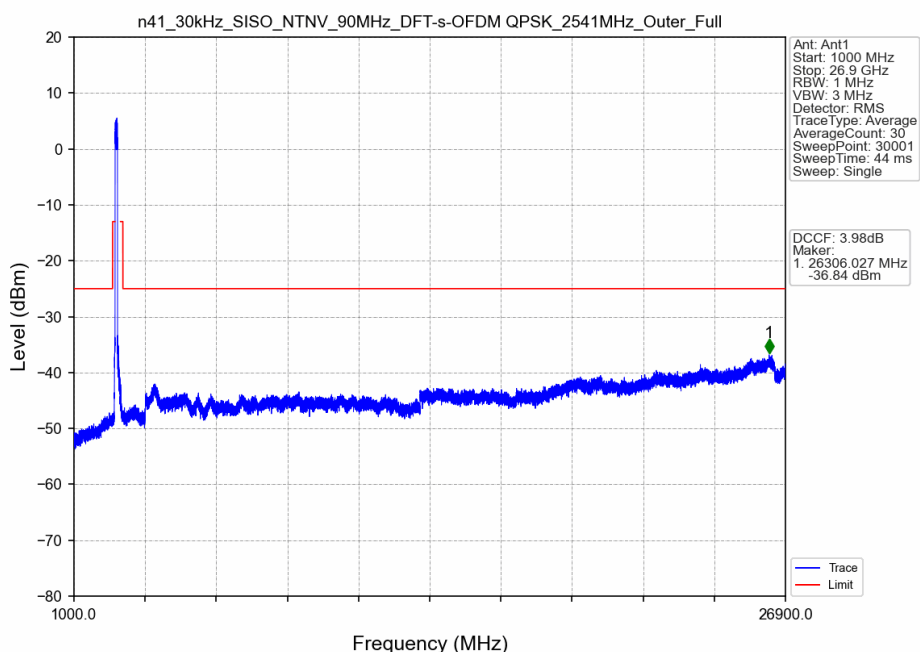
n41_30kHz_SISO_NTNV_90MHz_DFT-s-OFDM QPSK_2541MHz_Outer_Full
