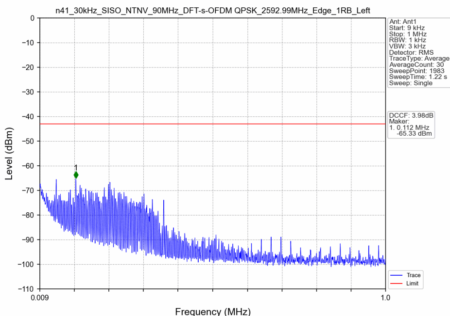
n41_30kHz_SISO_NTNV_90MHz_DFT-s-OFDM QPSK_2592.99MHz_Edge_1RB_Left
