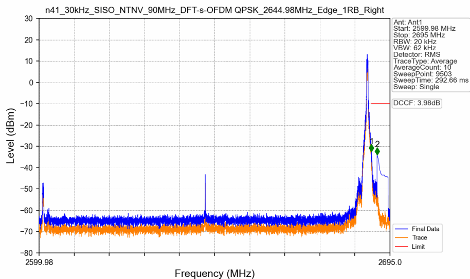
n41_30kHz_SISO_NTNV_90MHz_DFT-s-OFDM QPSK_2644.98MHz_Edge_1RB_Right
