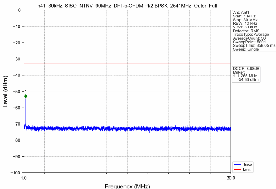
n41_30kHz_SISO_NTNV_90MHz_DFT-s-OFDM PI/2 BPSK_2541MHz_Outer_Full
