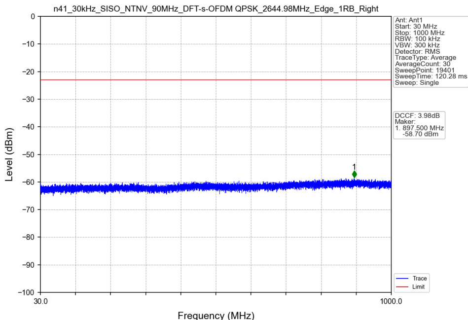
n41_30kHz_SISO_NTNV_90MHz_DFT-s-OFDM QPSK_2644.98MHz_Edge_1RB_Right
