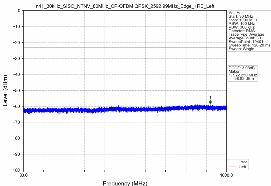
n41_30kHz_SISO_NTNV_80MHz_CP-OFDM QPSK_2592.99MHz_Edge_1RB_Left
