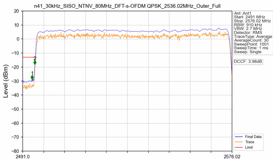
n41_30kHz_SISO_NTNV_80MHz_DFT-s-OFDM QPSK_2536.02MHz_Outer_Full
