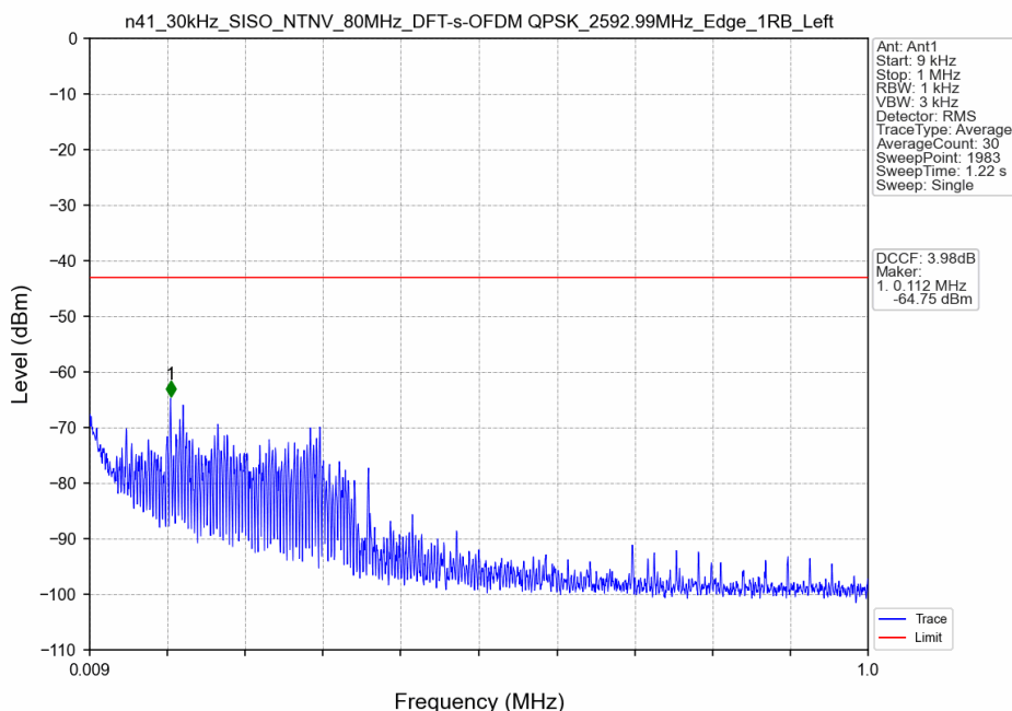
n41_30kHz_SISO_NTNV_80MHz_DFT-s-OFDM QPSK_2592.99MHz_Edge_1RB_Left
