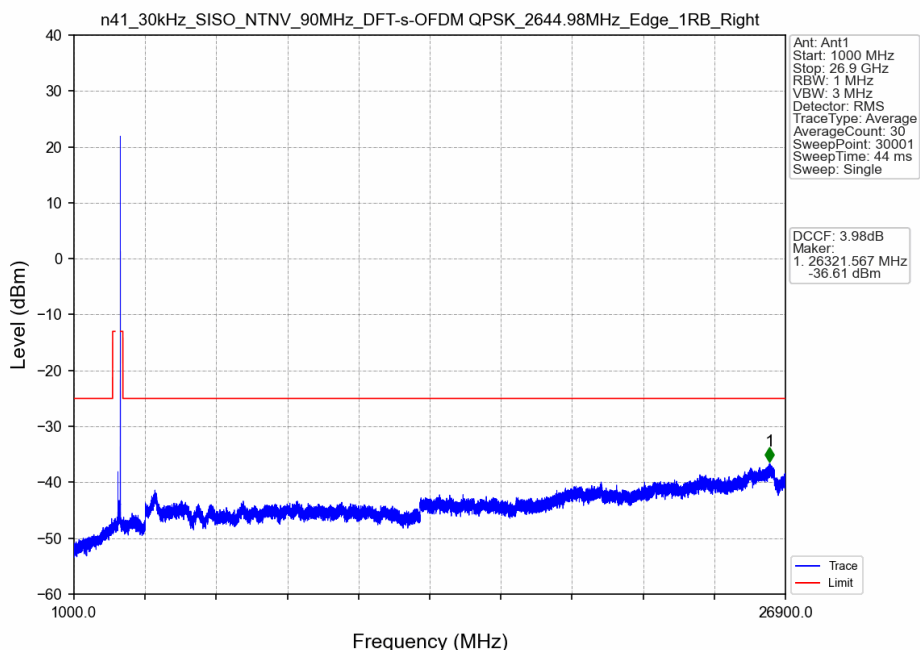
n41_30kHz_SISO_NTNV_90MHz_DFT-s-OFDM QPSK_2644.98MHz_Edge_1RB_Right
