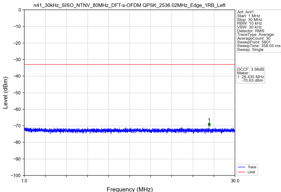
n41_30kHz_SISO_NTNV_80MHz_DFT-s-OFDM QPSK_2536.02MHz_Edge_1RB_Left
