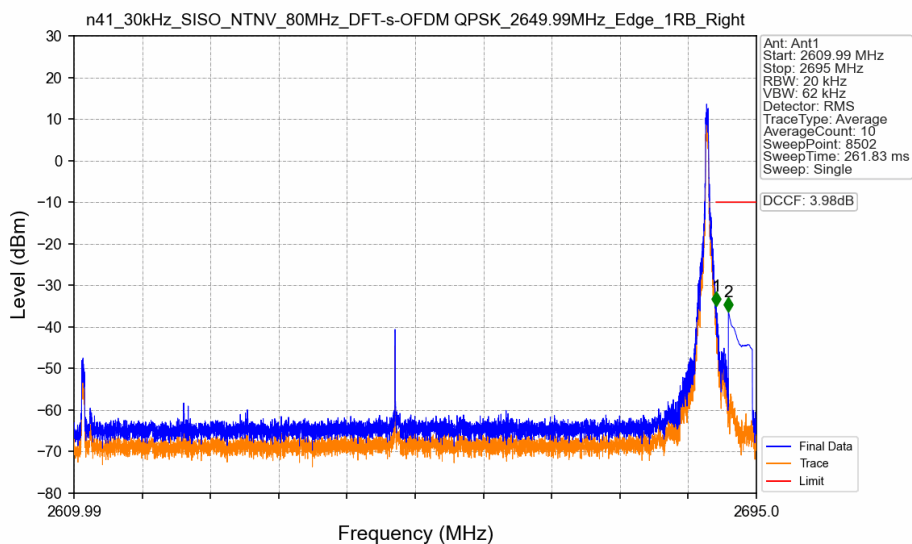
n41_30kHz_SISO_NTNV_80MHz_DFT-s-OFDM QPSK_2649.99MHz_Edge_1RB_Right
