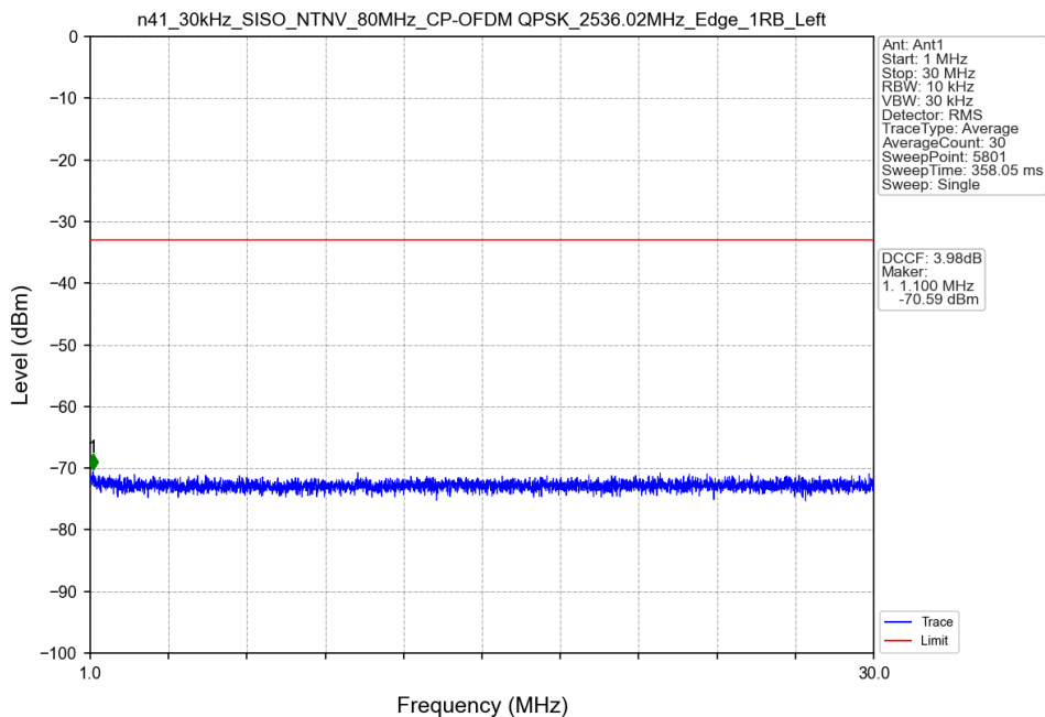
n41_30kHz_SISO_NTNV_80MHz_CP-OFDM QPSK_2536.02MHz_Edge_1RB_Left
