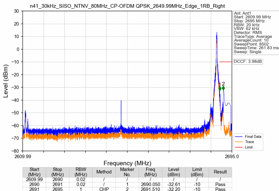
n41_30kHz_SISO_NTNV_80MHz_CP-OFDM QPSK_2649.99MHz_Edge_1RB_Right
