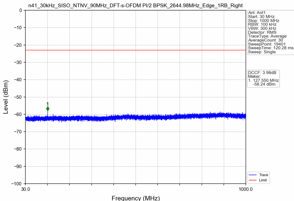
n41_30kHz_SISO_NTNV_90MHz_DFT-s-OFDM PI/2 BPSK_2644.98MHz_Edge_1RB_Right
