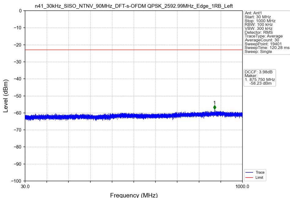
n41_30kHz_SISO_NTNV_90MHz_DFT-s-OFDM QPSK_2592.99MHz_Edge_1RB_Left
