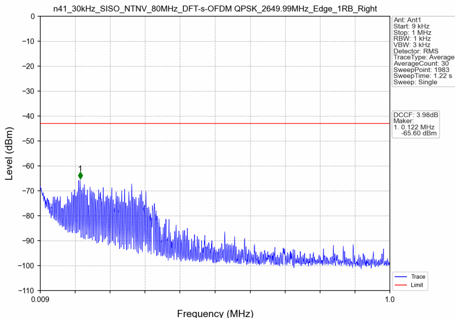
n41_30kHz_SISO_NTNV_80MHz_DFT-s-OFDM QPSK_2649.99MHz_Edge_1RB_Right
