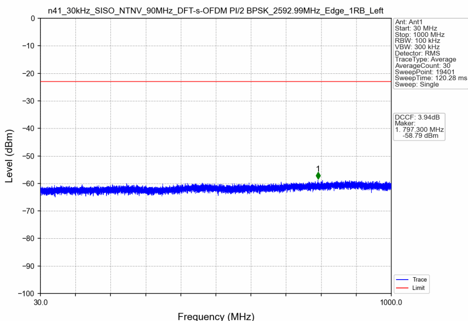
n41_30kHz_SISO_NTNV_90MHz_DFT-s-OFDM PI/2 BPSK_2592.99MHz_Edge_1RB_Left
