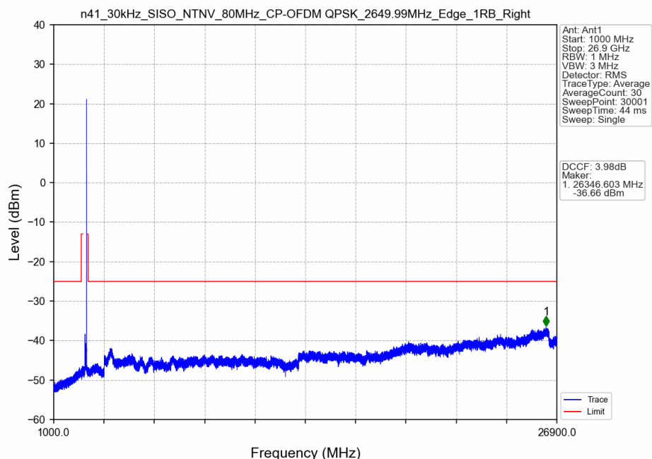
n41_30kHz_SISO_NTNV_80MHz_CP-OFDM QPSK_2649.99MHz_Edge_1RB_Right
