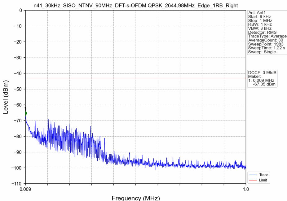
n41_30kHz_SISO_NTNV_90MHz_DFT-s-OFDM QPSK_2644.98MHz_Edge_1RB_Right
