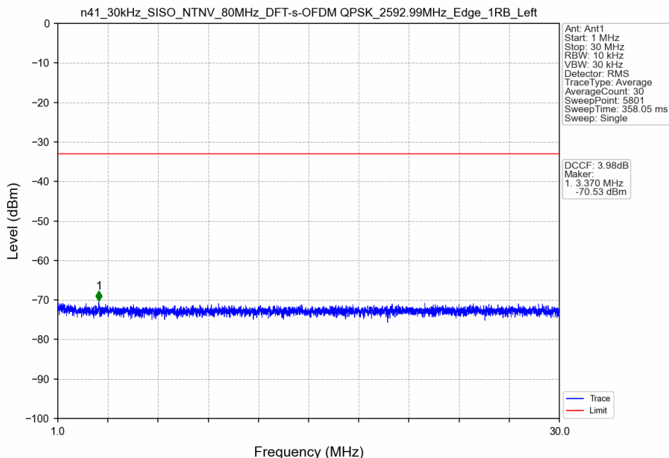
n41_30kHz_SISO_NTNV_80MHz_DFT-s-OFDM QPSK_2592.99MHz_Edge_1RB_Left
