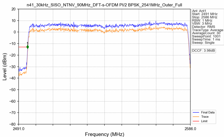
n41_30kHz_SISO_NTNV_90MHz_DFT-s-OFDM PI/2 BPSK_2541MHz_Outer_Full
