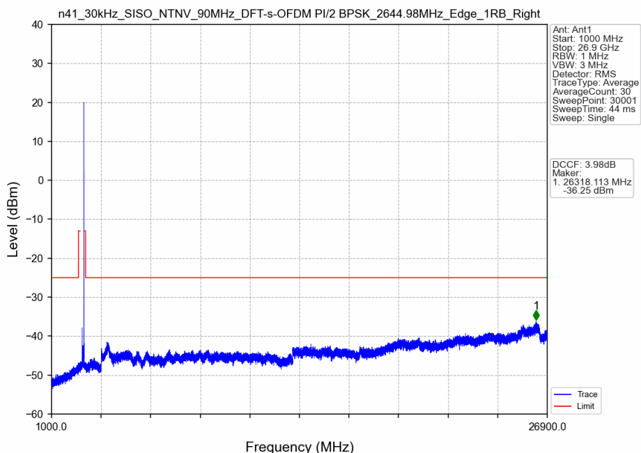
n41_30kHz_SISO_NTNV_90MHz_DFT-s-OFDM PI/2 BPSK_2644.98MHz_Edge_1RB_Right
