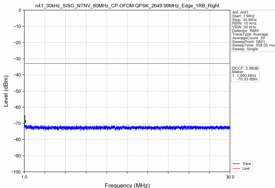
n41_30kHz_SISO_NTNV_80MHz_CP-OFDM QPSK_2649.99MHz_Edge_1RB_Right
