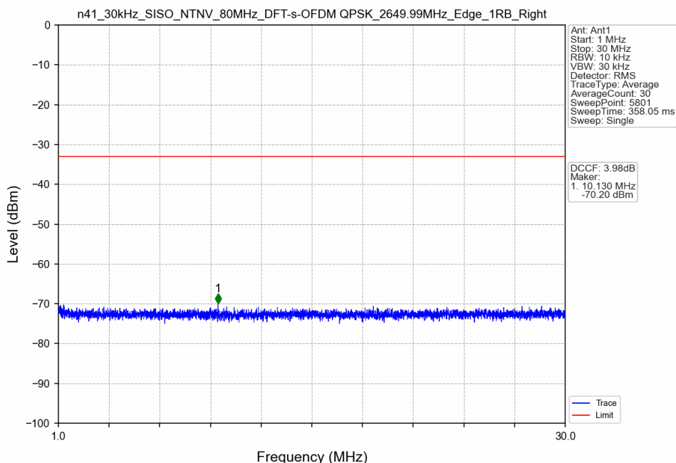
n41_30kHz_SISO_NTNV_80MHz_DFT-s-OFDM QPSK_2649.99MHz_Edge_1RB_Right
