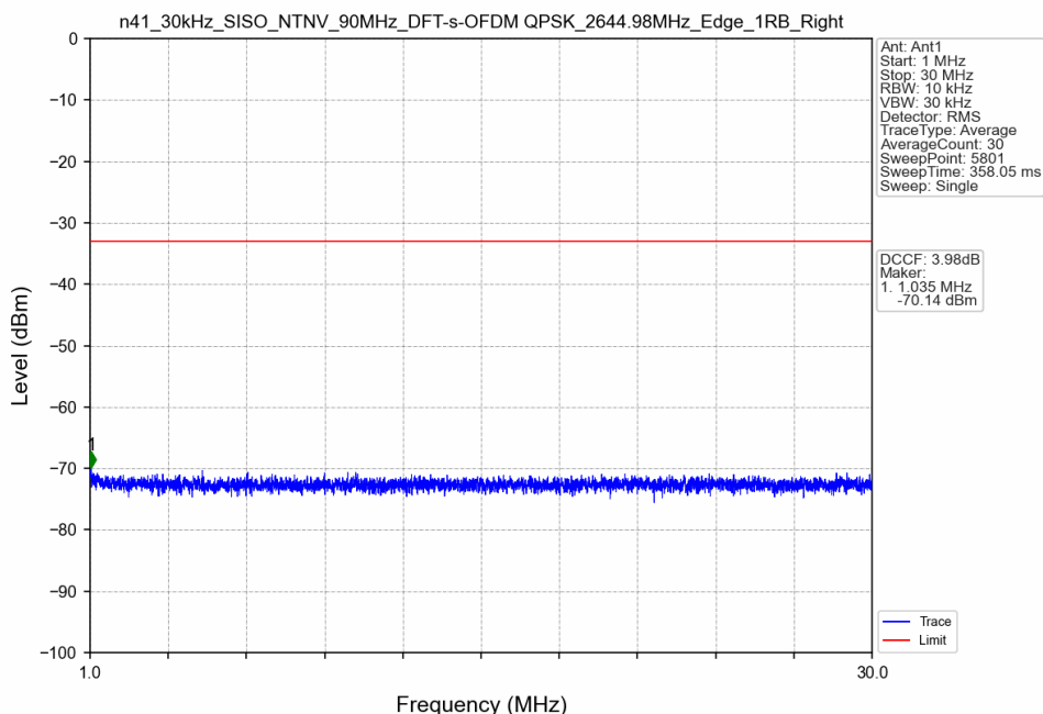
n41_30kHz_SISO_NTNV_90MHz_DFT-s-OFDM QPSK_2644.98MHz_Edge_1RB_Right
