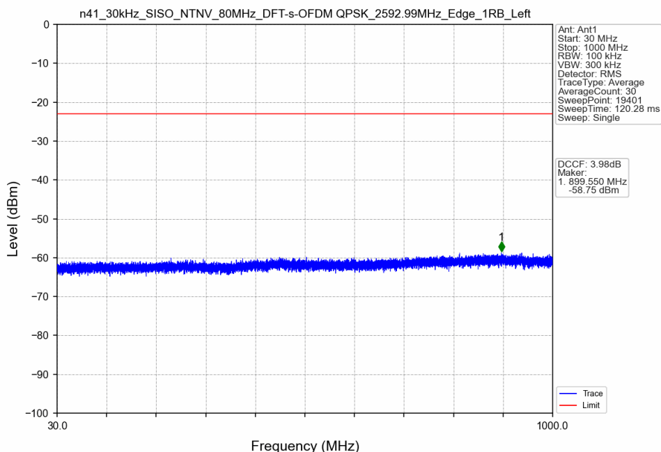
n41_30kHz_SISO_NTNV_80MHz_DFT-s-OFDM QPSK_2592.99MHz_Edge_1RB_Left
