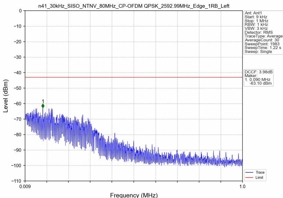
n41_30kHz_SISO_NTNV_80MHz_CP-OFDM QPSK_2592.99MHz_Edge_1RB_Left
