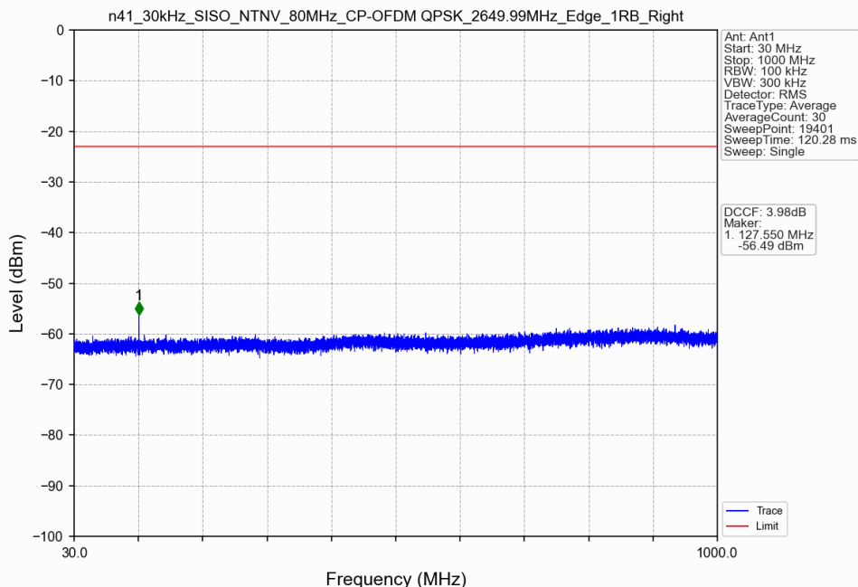
n41_30kHz_SISO_NTNV_80MHz_CP-OFDM QPSK_2649.99MHz_Edge_1RB_Right
