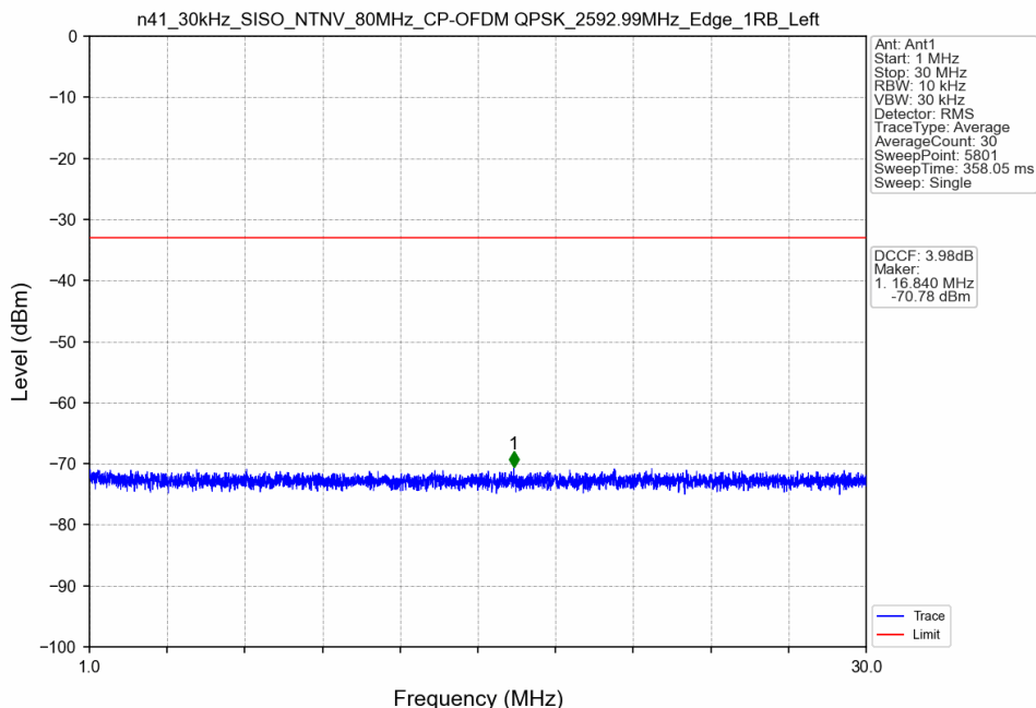
n41_30kHz_SISO_NTNV_80MHz_CP-OFDM QPSK_2592.99MHz_Edge_1RB_Left
