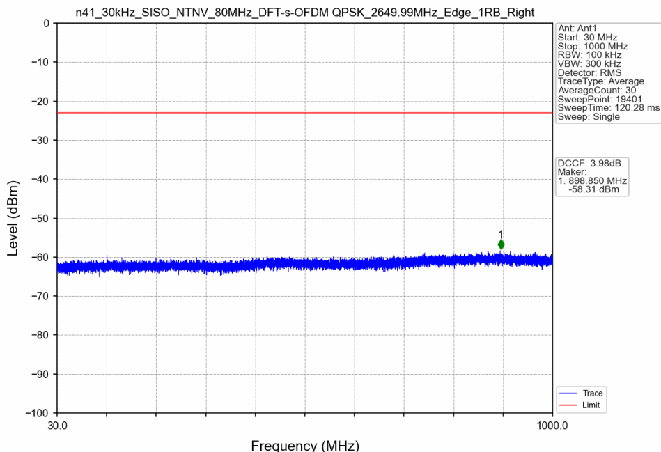
n41_30kHz_SISO_NTNV_80MHz_DFT-s-OFDM QPSK_2649.99MHz_Edge_1RB_Right
