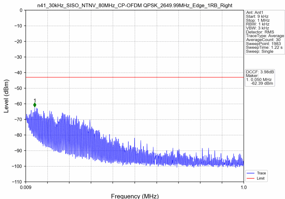
n41_30kHz_SISO_NTNV_80MHz_CP-OFDM QPSK_2649.99MHz_Edge_1RB_Right
