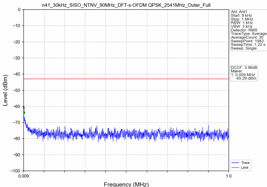
n41_30kHz_SISO_NTNV_90MHz_DFT-s-OFDM QPSK_2541MHz_Outer_Full
