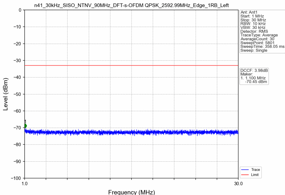
n41_30kHz_SISO_NTNV_90MHz_DFT-s-OFDM QPSK_2592.99MHz_Edge_1RB_Left
