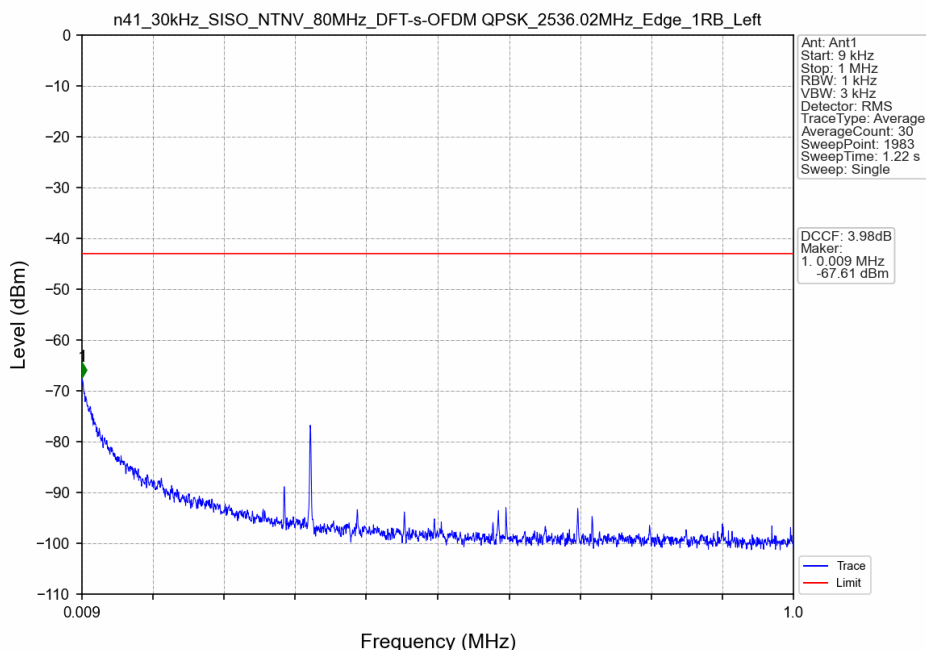
n41_30kHz_SISO_NTNV_80MHz_DFT-s-OFDM QPSK_2536.02MHz_Edge_1RB_Left
