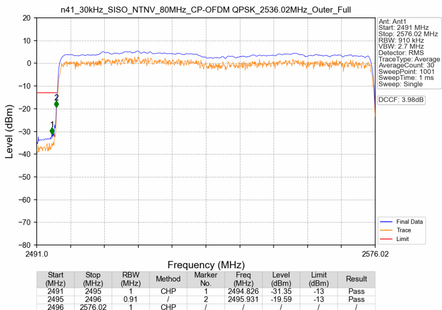
n41_30kHz_SISO_NTNV_80MHz_CP-OFDM QPSK_2536.02MHz_Outer_Full
