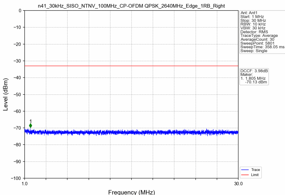
n41_30kHz_SISO_NTNV_100MHz_CP-OFDM QPSK_2640MHz_Edge_1RB_Right
