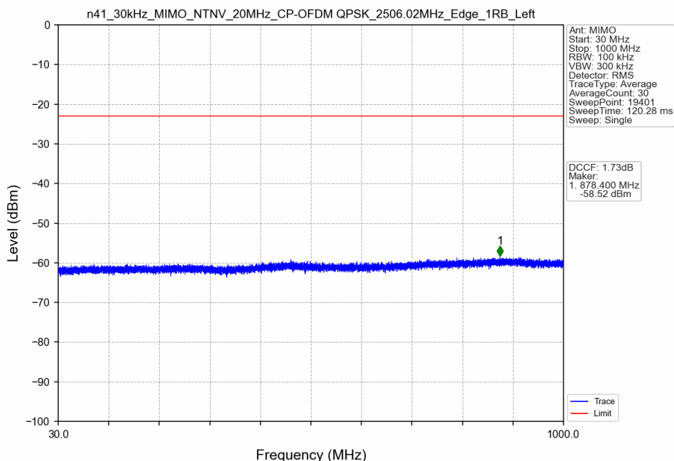
n41_30kHz_MIMO_NTNV_20MHz_CP-OFDM QPSK_2506.02MHz_Edge_1RB_Left
