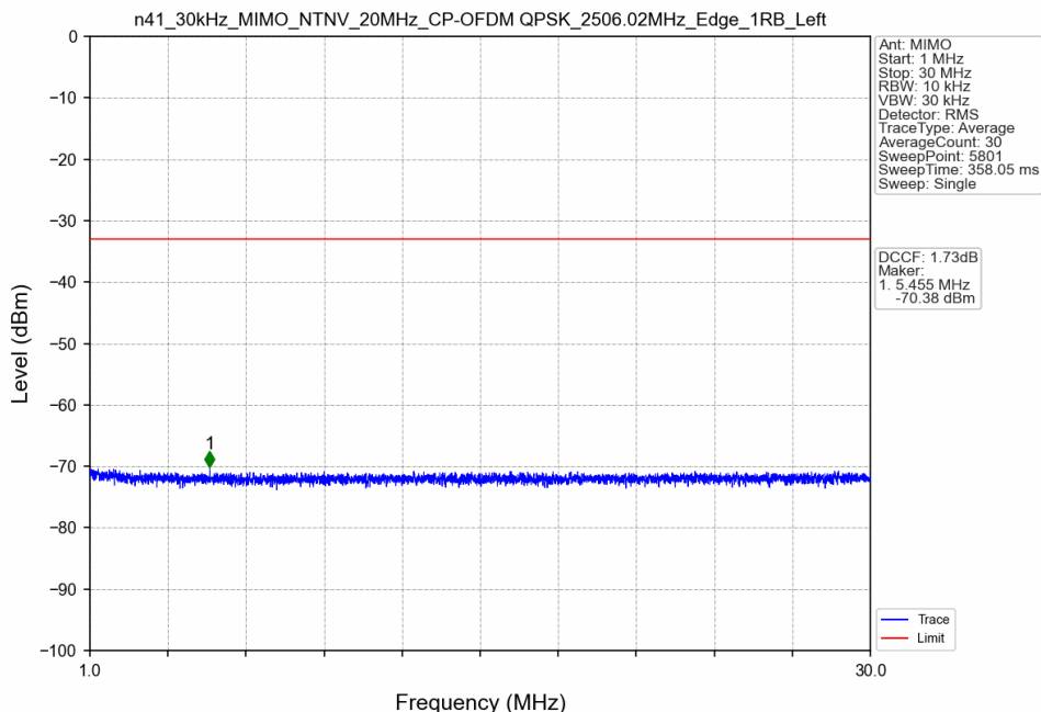
n41_30kHz_MIMO_NTNV_20MHz_CP-OFDM QPSK_2506.02MHz_Edge_1RB_Left
