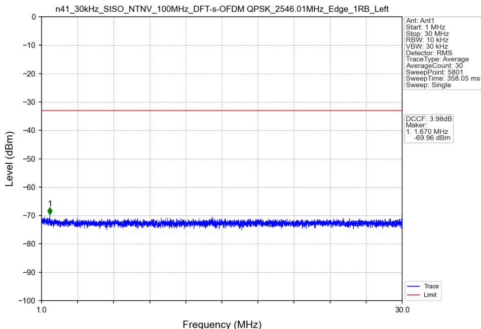
n41_30kHz_SISO_NTNV_100MHz_DFT-s-OFDM QPSK_2546.01MHz_Edge_1RB_Left
