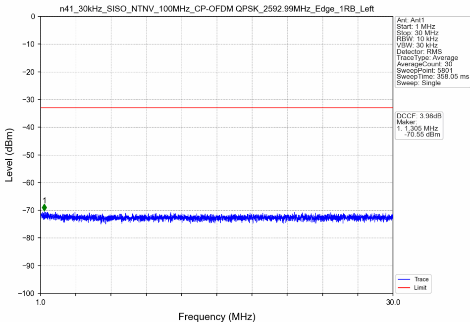
n41_30kHz_SISO_NTNV_100MHz_CP-OFDM QPSK_2592.99MHz_Edge_1RB_Left
