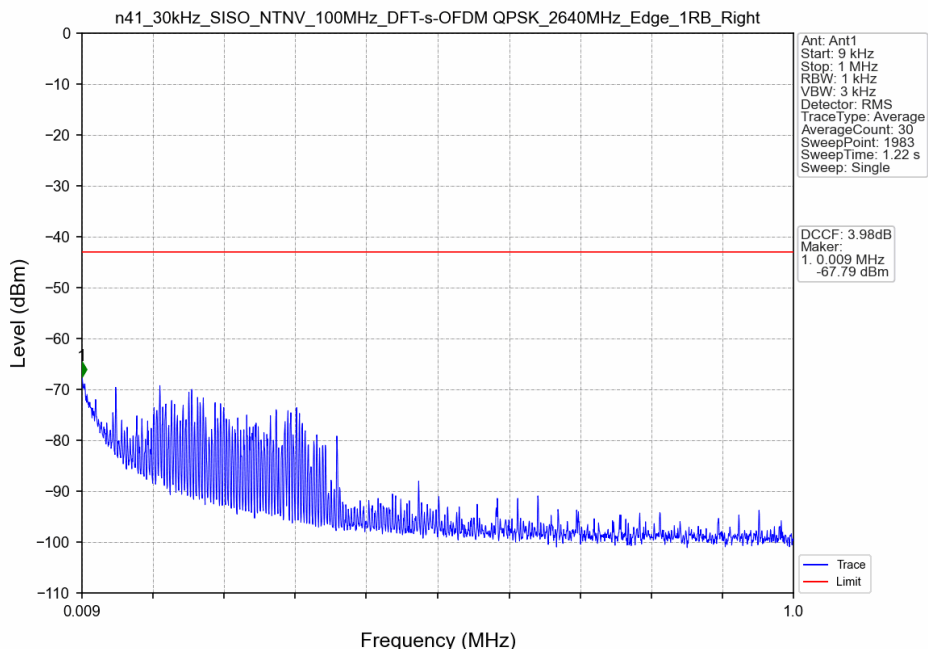
n41_30kHz_SISO_NTNV_100MHz_DFT-s-OFDM QPSK_2640MHz_Edge_1RB_Right
