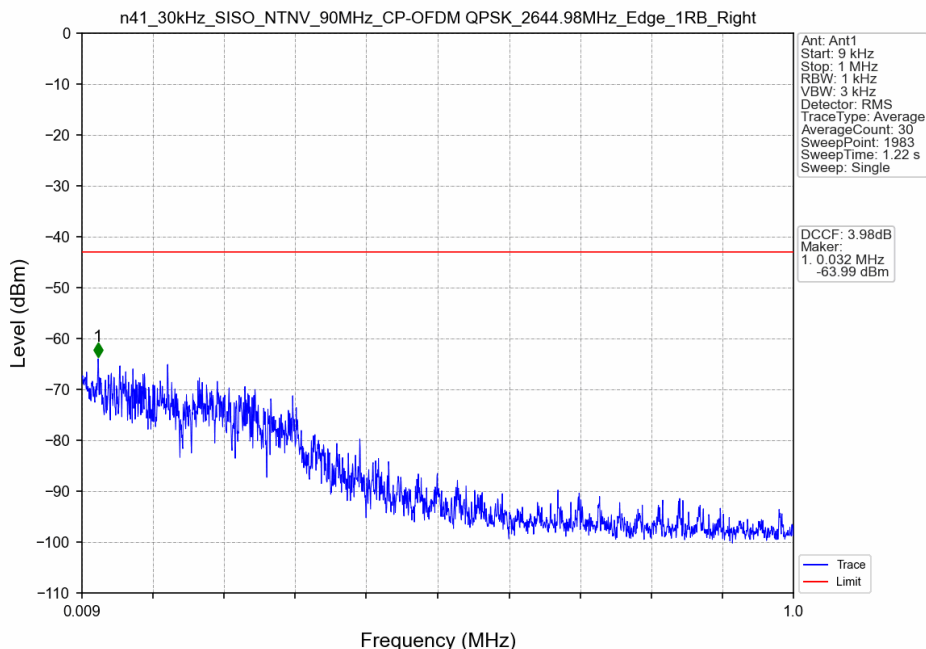
n41_30kHz_SISO_NTNV_90MHz_CP-OFDM QPSK_2644.98MHz_Edge_1RB_Right
