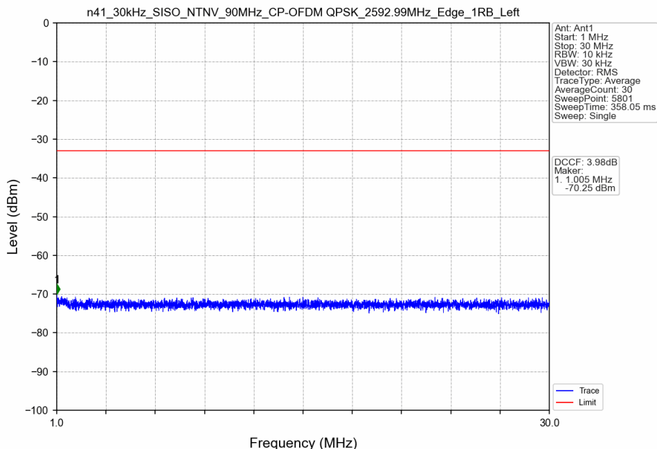
n41_30kHz_SISO_NTNV_90MHz_CP-OFDM QPSK_2592.99MHz_Edge_1RB_Left
