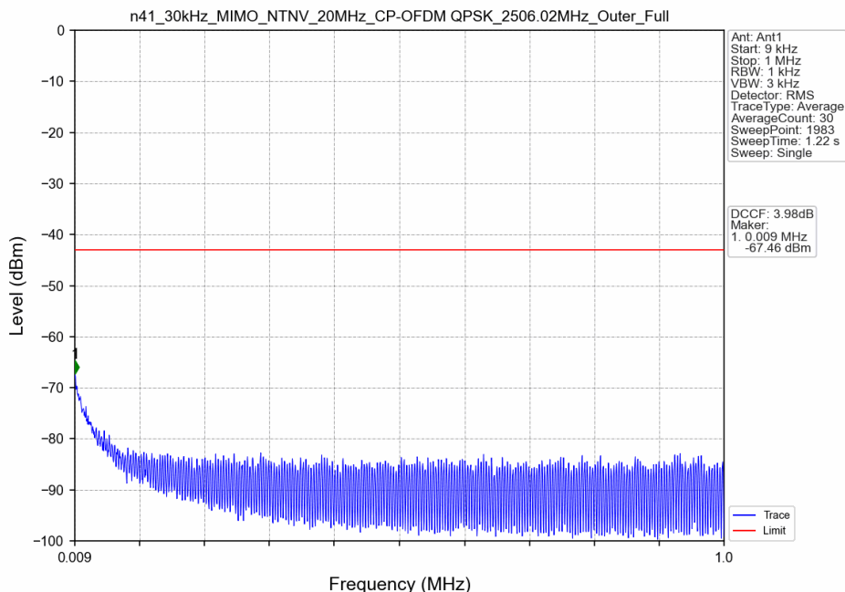
n41_30kHz_MIMO_NTNV_20MHz_CP-OFDM QPSK_2506.02MHz_Outer_Full
