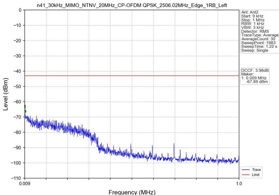
n41_30kHz_MIMO_NTNV_20MHz_CP-OFDM QPSK_2506.02MHz_Edge_1RB_Left
