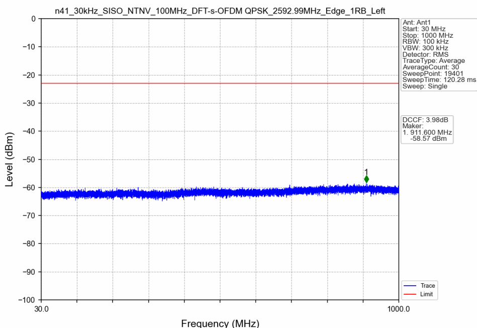
n41_30kHz_SISO_NTNV_100MHz_DFT-s-OFDM QPSK_2592.99MHz_Edge_1RB_Left
