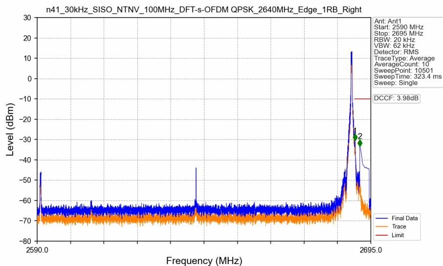
n41_30kHz_SISO_NTNV_100MHz_DFT-s-OFDM QPSK_2640MHz_Edge_1RB_Right
