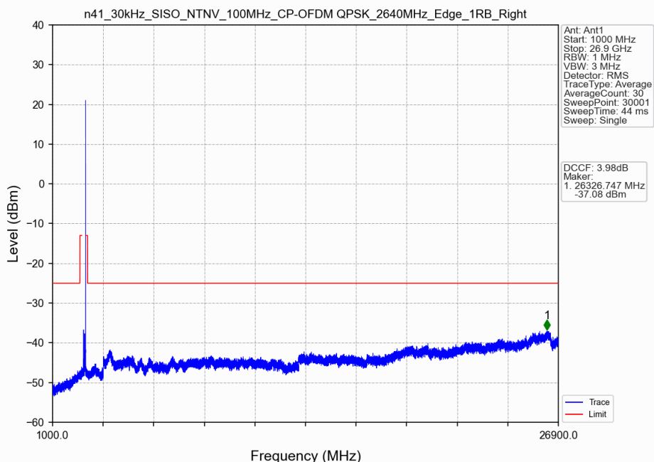
n41_30kHz_SISO_NTNV_100MHz_CP-OFDM QPSK_2640MHz_Edge_1RB_Right
