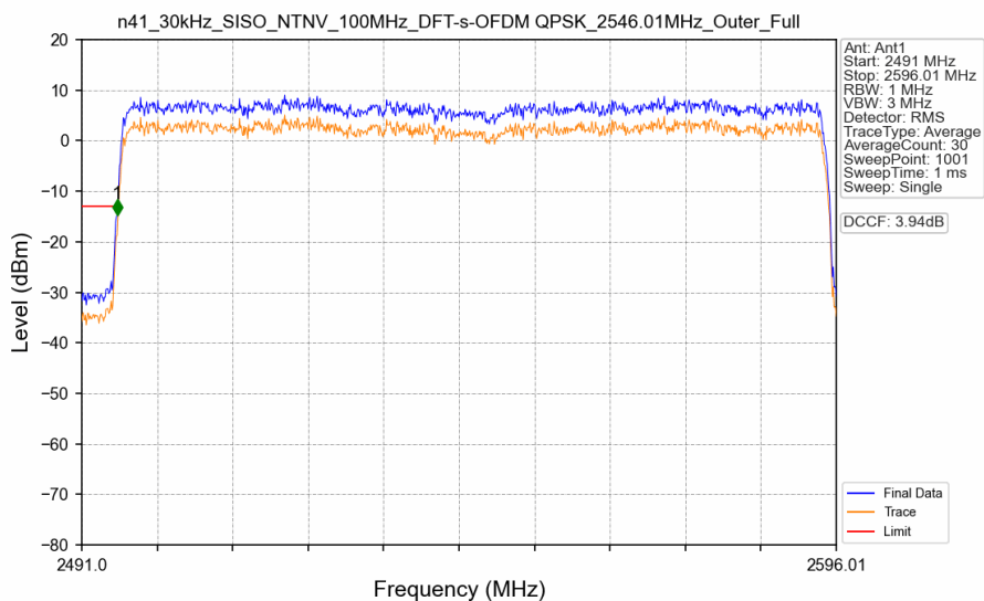
n41_30kHz_SISO_NTNV_100MHz_DFT-s-OFDM QPSK_2546.01MHz_Outer_Full
