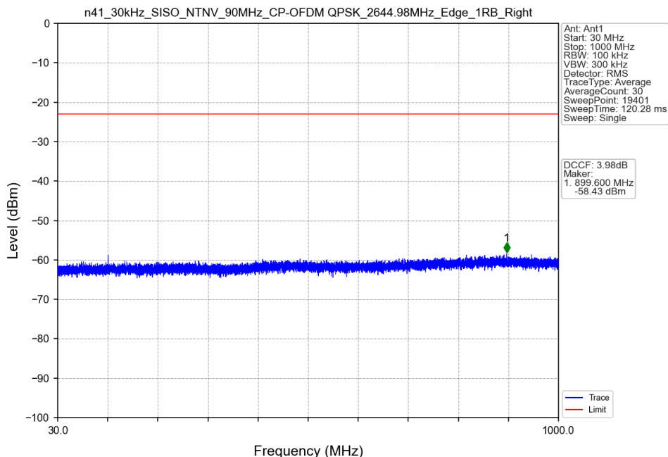
n41_30kHz_SISO_NTNV_90MHz_CP-OFDM QPSK_2644.98MHz_Edge_1RB_Right
