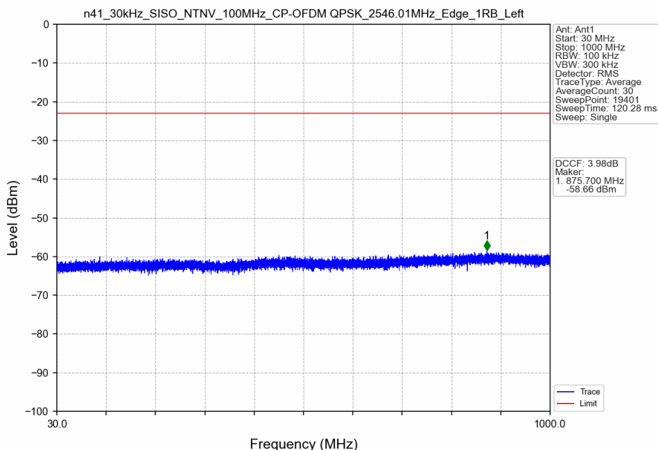
n41_30kHz_SISO_NTNV_100MHz_CP-OFDM QPSK_2546.01MHz_Edge_1RB_Left
