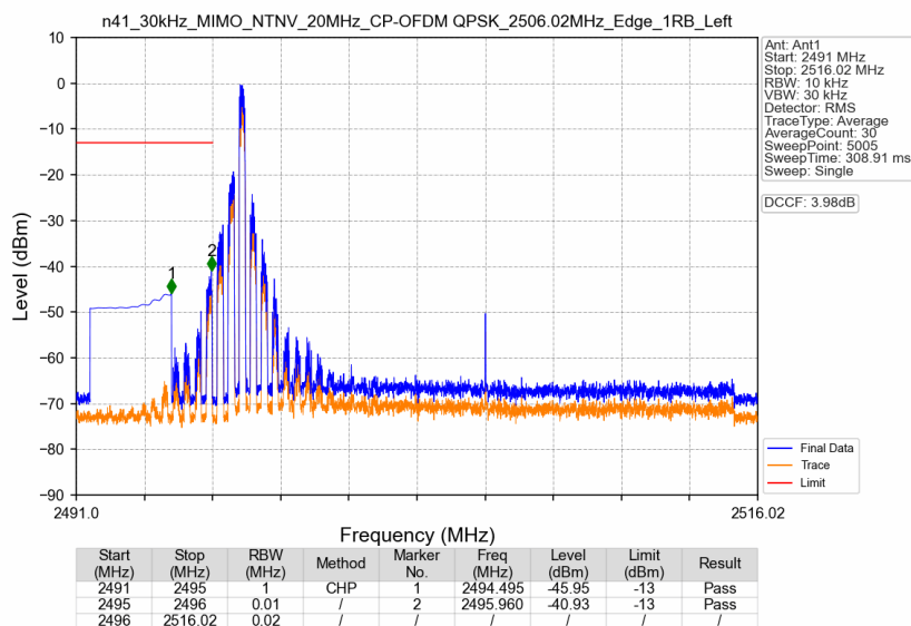
n41_30kHz_MIMO_NTNV_20MHz_CP-OFDM QPSK_2506.02MHz_Edge_1RB_Left
