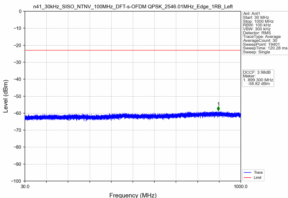
n41_30kHz_SISO_NTNV_100MHz_DFT-s-OFDM QPSK_2546.01MHz_Edge_1RB_Left
