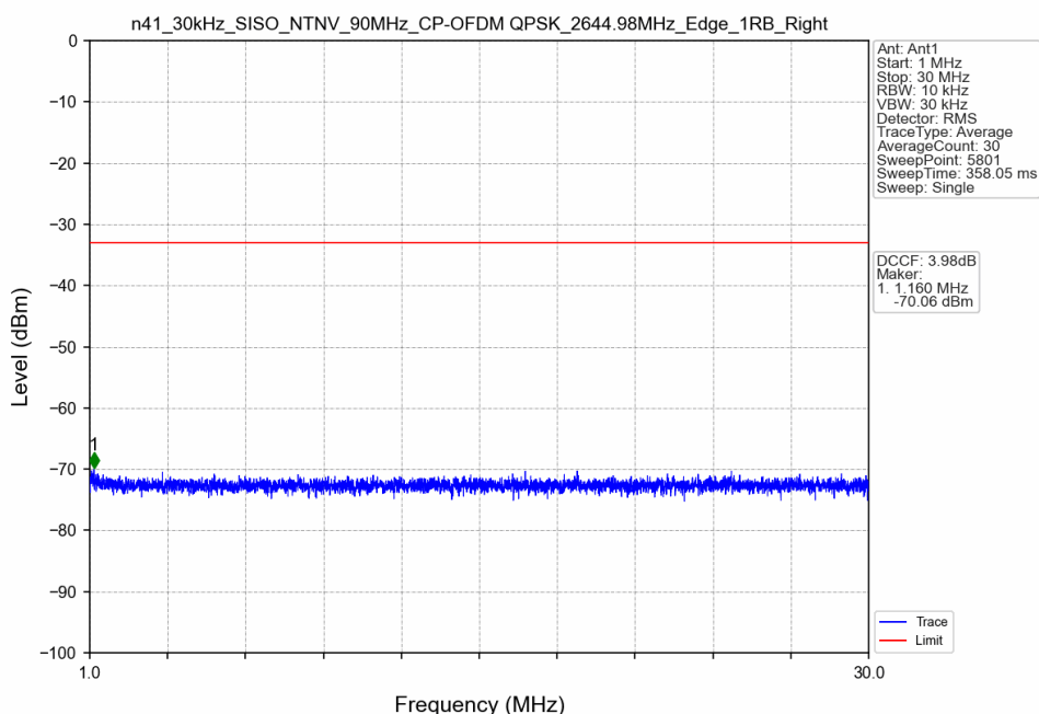
n41_30kHz_SISO_NTNV_90MHz_CP-OFDM QPSK_2644.98MHz_Edge_1RB_Right
