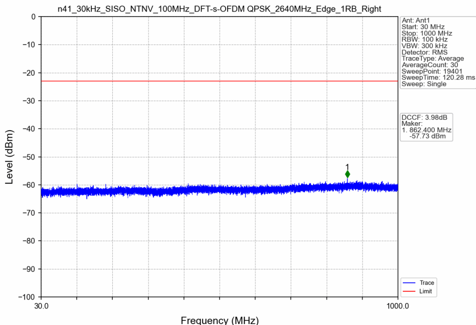
n41_30kHz_SISO_NTNV_100MHz_DFT-s-OFDM QPSK_2640MHz_Edge_1RB_Right
