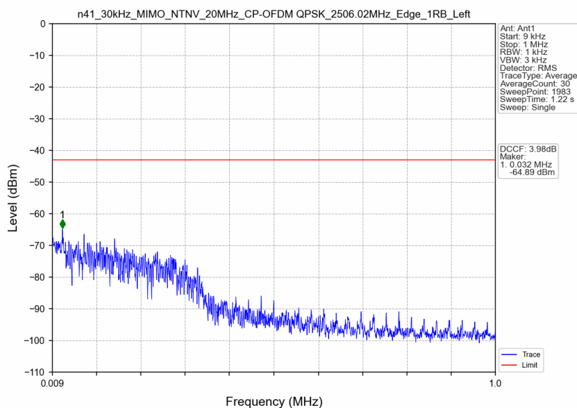
n41_30kHz_MIMO_NTNV_20MHz_CP-OFDM QPSK_2506.02MHz_Edge_1RB_Left
