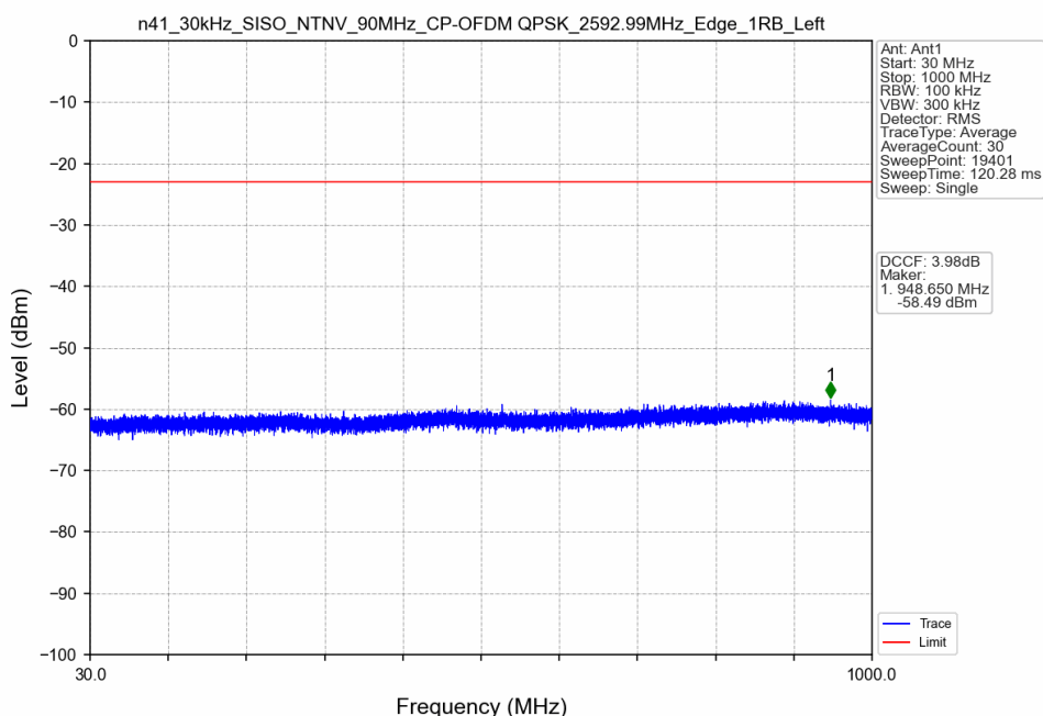
n41_30kHz_SISO_NTNV_90MHz_CP-OFDM QPSK_2592.99MHz_Edge_1RB_Left
