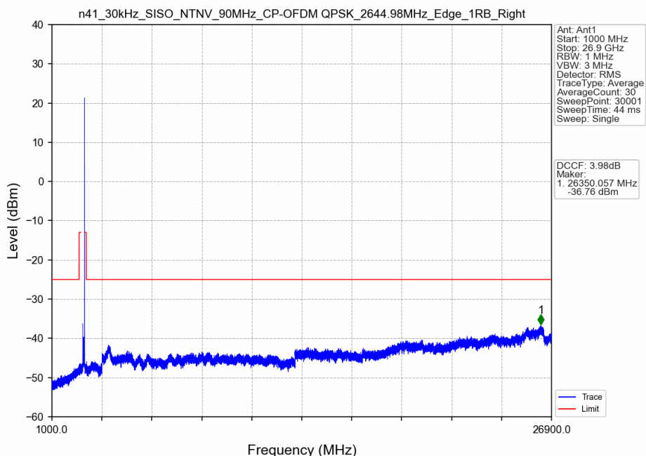
n41_30kHz_SISO_NTNV_90MHz_CP-OFDM QPSK_2644.98MHz_Edge_1RB_Right
