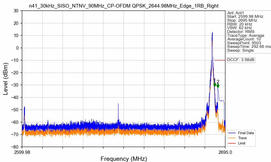
n41_30kHz_SISO_NTNV_90MHz_CP-OFDM QPSK_2644.98MHz_Edge_1RB_Right
