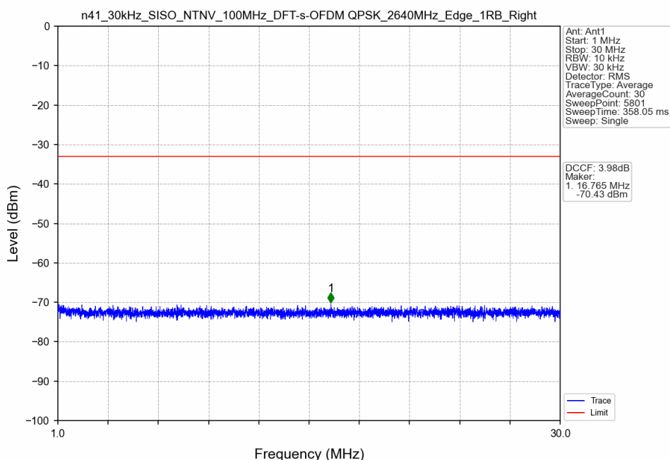
n41_30kHz_SISO_NTNV_100MHz_DFT-s-OFDM QPSK_2640MHz_Edge_1RB_Right
