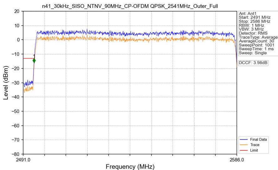
n41_30kHz_SISO_NTNV_90MHz_CP-OFDM QPSK_2541MHz_Outer_Full
