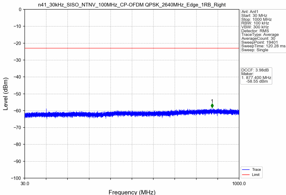
n41_30kHz_SISO_NTNV_100MHz_CP-OFDM QPSK_2640MHz_Edge_1RB_Right
