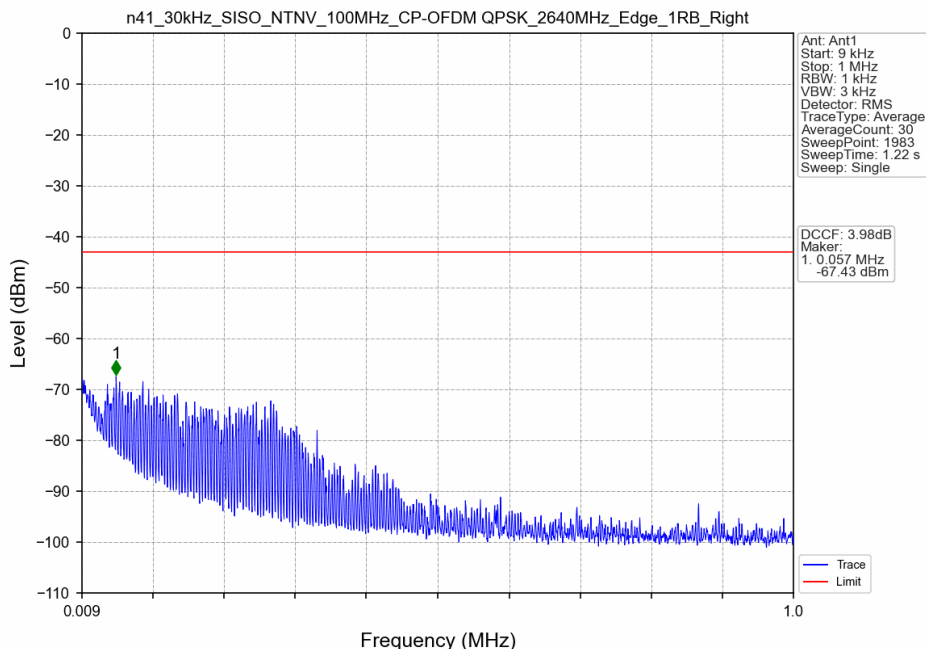
n41_30kHz_SISO_NTNV_100MHz_CP-OFDM QPSK_2640MHz_Edge_1RB_Right
