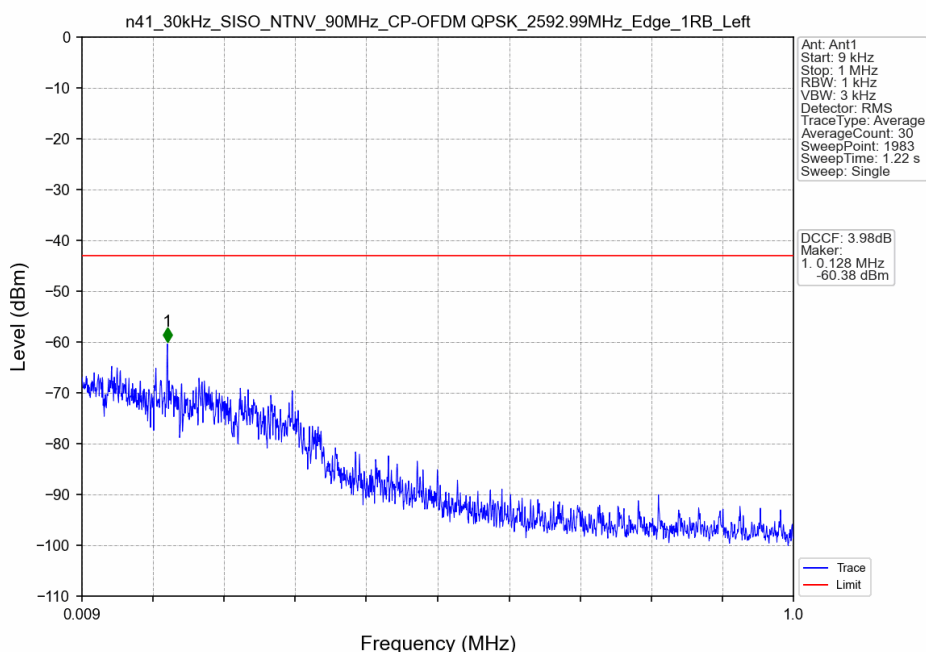
n41_30kHz_SISO_NTNV_90MHz_CP-OFDM QPSK_2592.99MHz_Edge_1RB_Left
