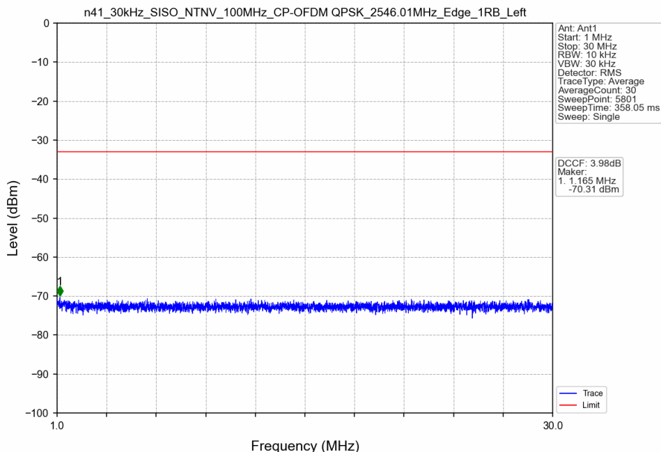
n41_30kHz_SISO_NTNV_100MHz_CP-OFDM QPSK_2546.01MHz_Edge_1RB_Left
