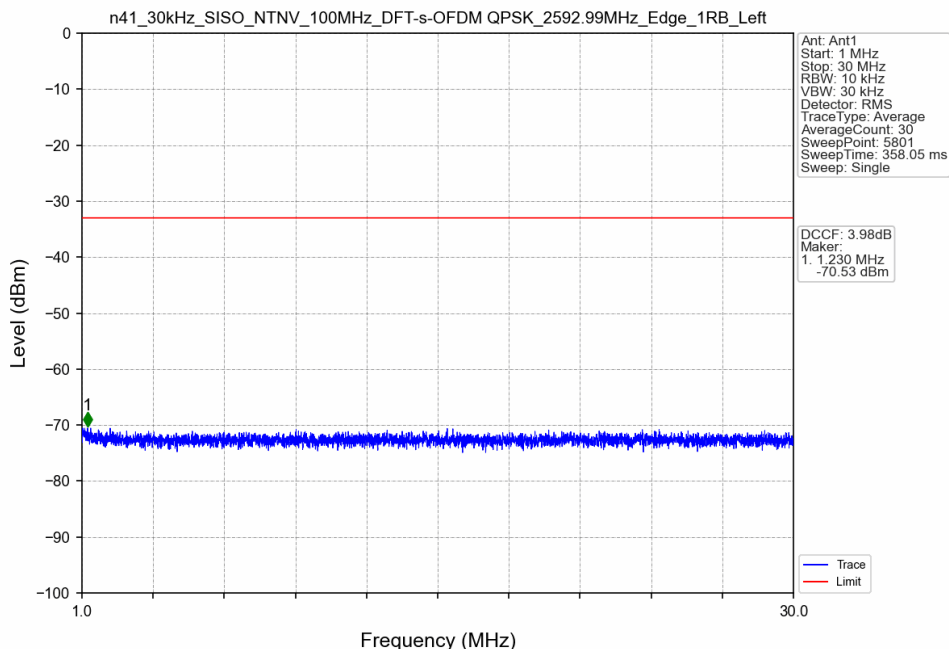
n41_30kHz_SISO_NTNV_100MHz_DFT-s-OFDM QPSK_2592.99MHz_Edge_1RB_Left
