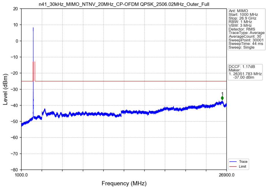
n41_30kHz_MIMO_NTNV_20MHz_CP-OFDM QPSK_2506.02MHz_Outer_Full
