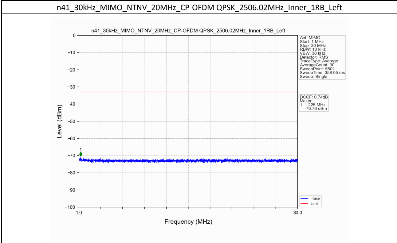
n41_30kHz_MIMO_NTNV_20MHz_CP-OFDM QPSK_2506.02MHz_Inner_1RB_Left
