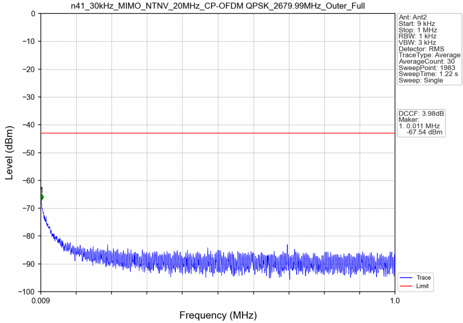
n41_30kHz_MIMO_NTNV_20MHz_CP-OFDM QPSK_2679.99MHz_Outer_Full
