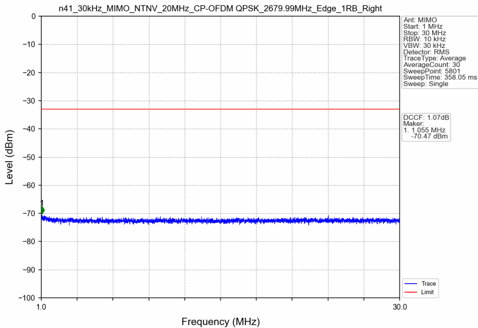
n41_30kHz_MIMO_NTNV_20MHz_CP-OFDM QPSK_2679.99MHz_Edge_1RB_Right
