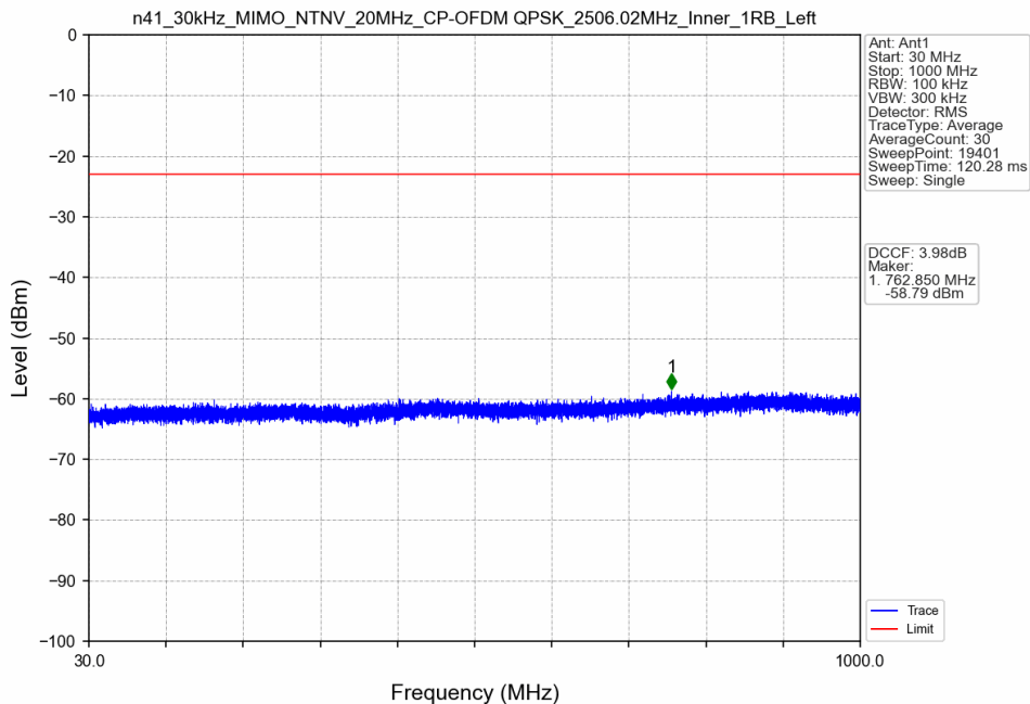
n41_30kHz_MIMO_NTNV_20MHz_CP-OFDM QPSK_2506.02MHz_Inner_1RB_Left
