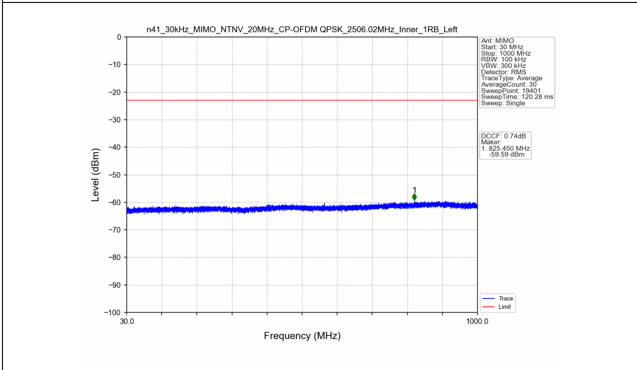
n41_30kHz_MIMO_NTNV_20MHz_CP-OFDM QPSK_2506.02MHz_Inner_1RB_Left
