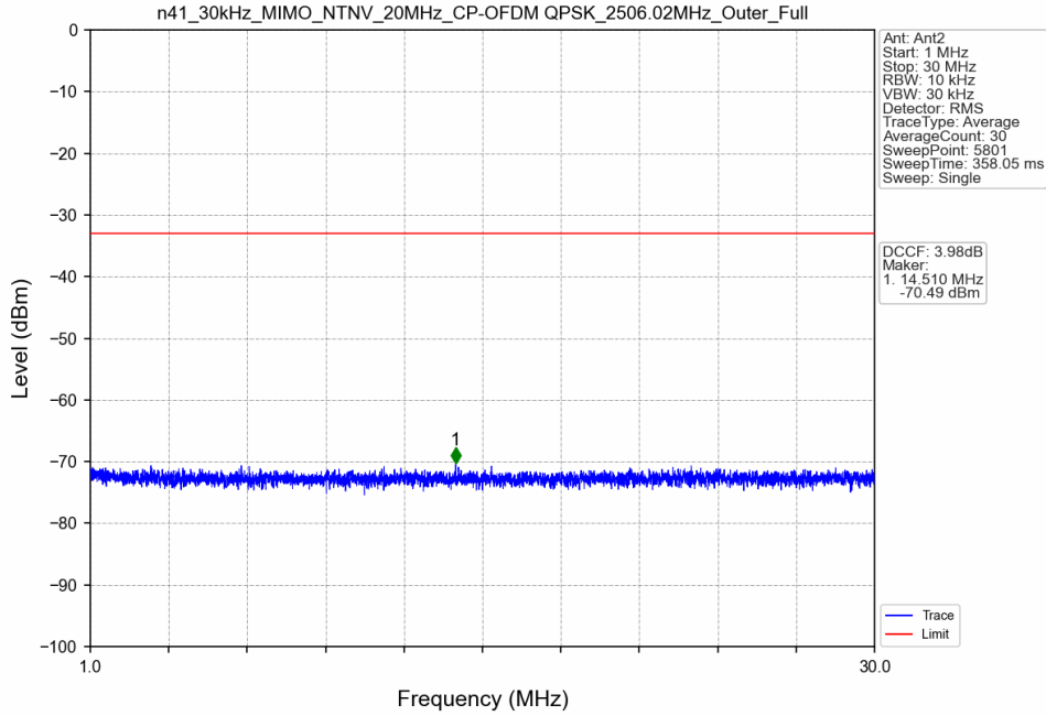
n41_30kHz_MIMO_NTNV_20MHz_CP-OFDM QPSK_2506.02MHz_Outer_Full
