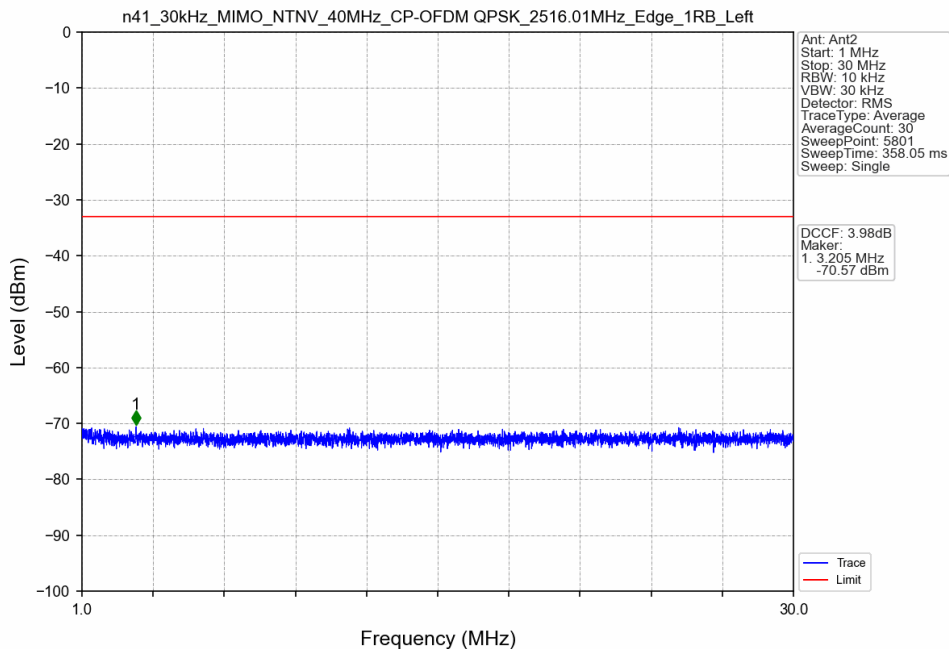
n41_30kHz_MIMO_NTNV_40MHz_CP-OFDM QPSK_2516.01MHz_Edge_1RB_Left
