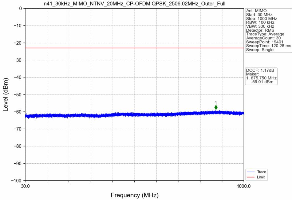
n41_30kHz_MIMO_NTNV_20MHz_CP-OFDM QPSK_2506.02MHz_Outer_Full
