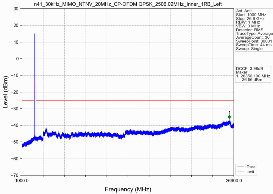
n41_30kHz_MIMO_NTNV_20MHz_CP-OFDM QPSK_2506.02MHz_Inner_1RB_Left
