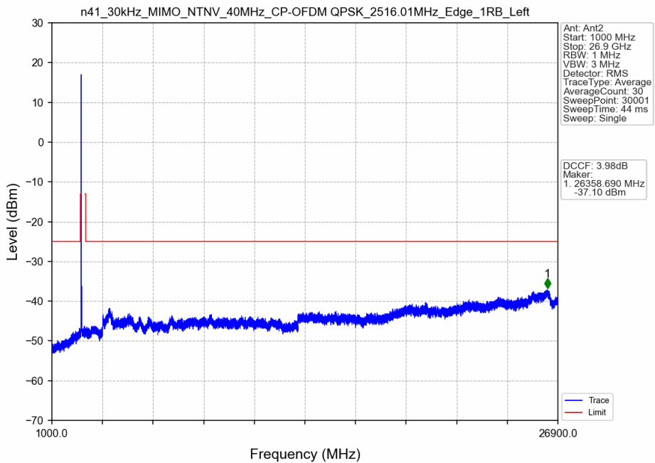
n41_30kHz_MIMO_NTNV_40MHz_CP-OFDM QPSK_2516.01MHz_Edge_1RB_Left
