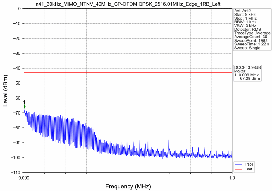
n41_30kHz_MIMO_NTNV_40MHz_CP-OFDM QPSK_2516.01MHz_Edge_1RB_Left
