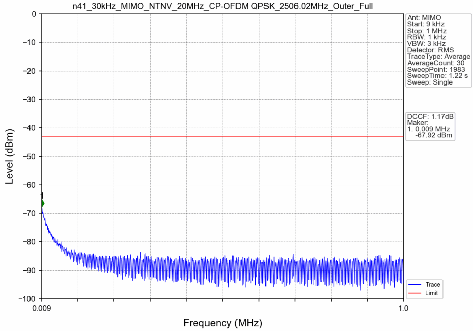
n41_30kHz_MIMO_NTNV_20MHz_CP-OFDM QPSK_2506.02MHz_Outer_Full
