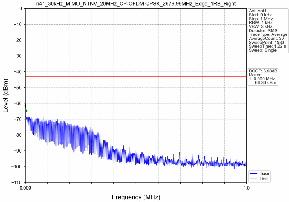
n41_30kHz_MIMO_NTNV_20MHz_CP-OFDM QPSK_2679.99MHz_Edge_1RB_Right
