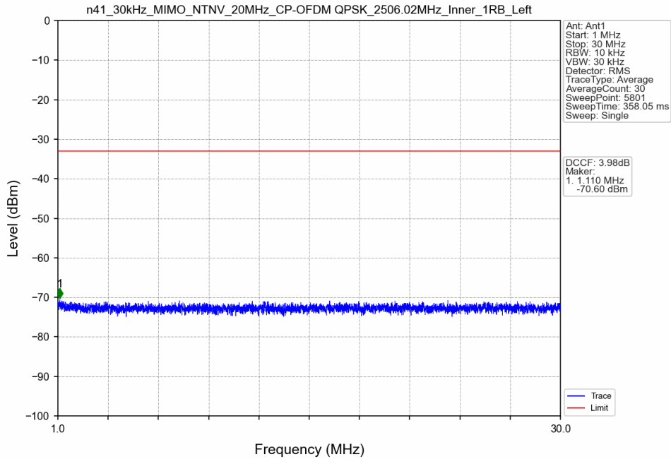
n41_30kHz_MIMO_NTNV_20MHz_CP-OFDM QPSK_2506.02MHz_Inner_1RB_Left
