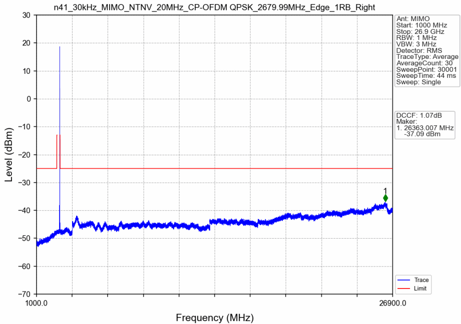
n41_30kHz_MIMO_NTNV_20MHz_CP-OFDM QPSK_2679.99MHz_Edge_1RB_Right
