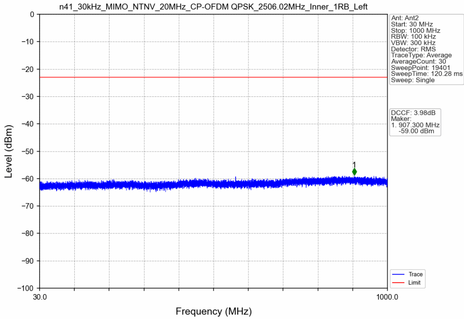
n41_30kHz_MIMO_NTNV_20MHz_CP-OFDM_QPSK_2506.02MHz_Inner_1RB_Left
