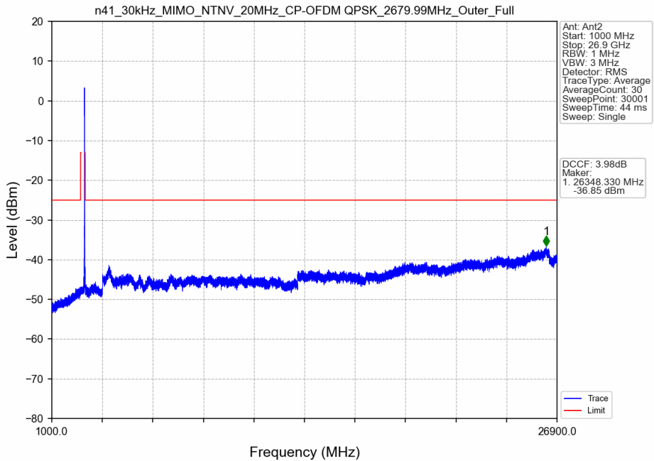
n41_30kHz_MIMO_NTNV_20MHz_CP-OFDM QPSK_2679.99MHz_Outer_Full
