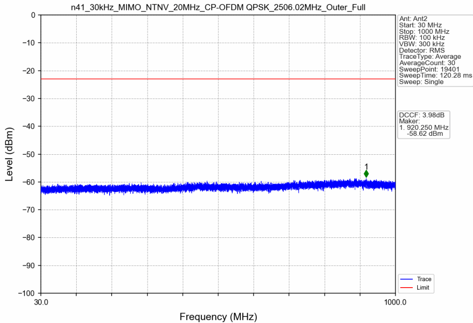
n41_30kHz_MIMO_NTNV_20MHz_CP-OFDM QPSK_2506.02MHz_Outer_Full
