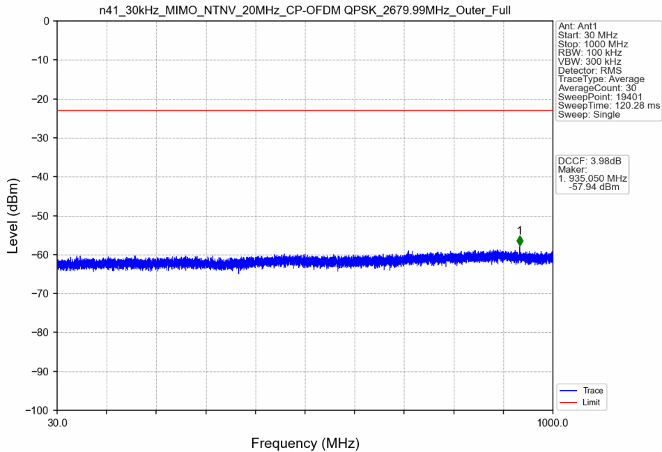
n41_30kHz_MIMO_NTNV_20MHz_CP-OFDM QPSK_2679.99MHz_Outer_Full
