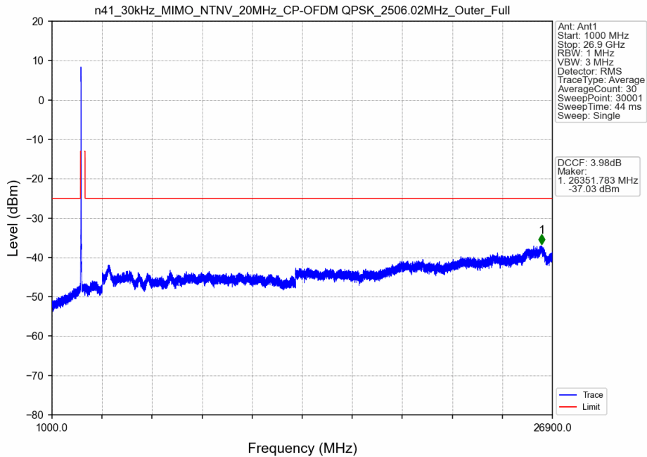
n41_30kHz_MIMO_NTNV_20MHz_CP-OFDM QPSK_2506.02MHz_Outer_Full
