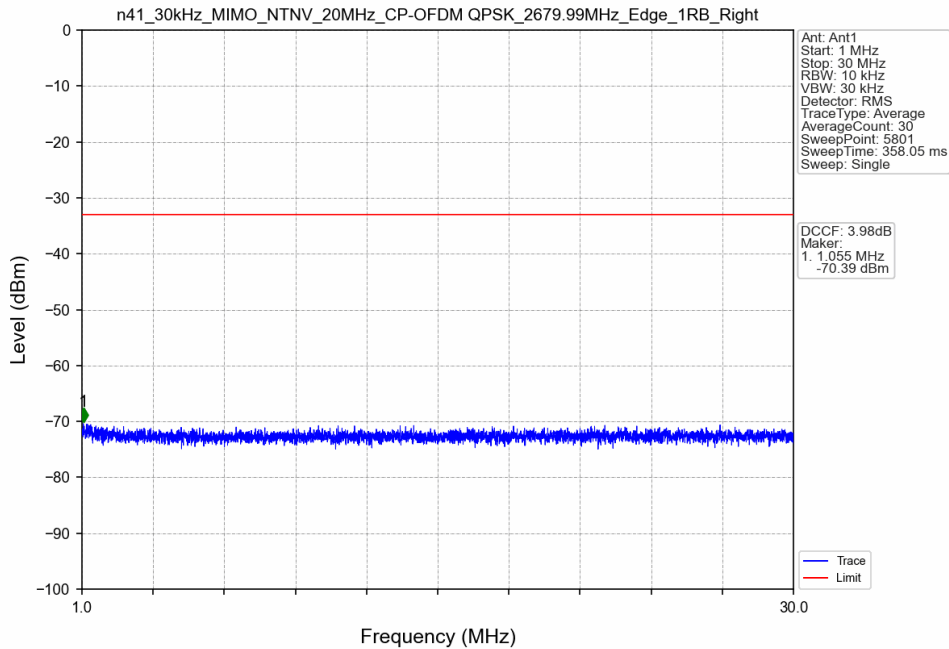
n41_30kHz_MIMO_NTNV_20MHz_CP-OFDM QPSK_2679.99MHz_Edge_1RB_Right
