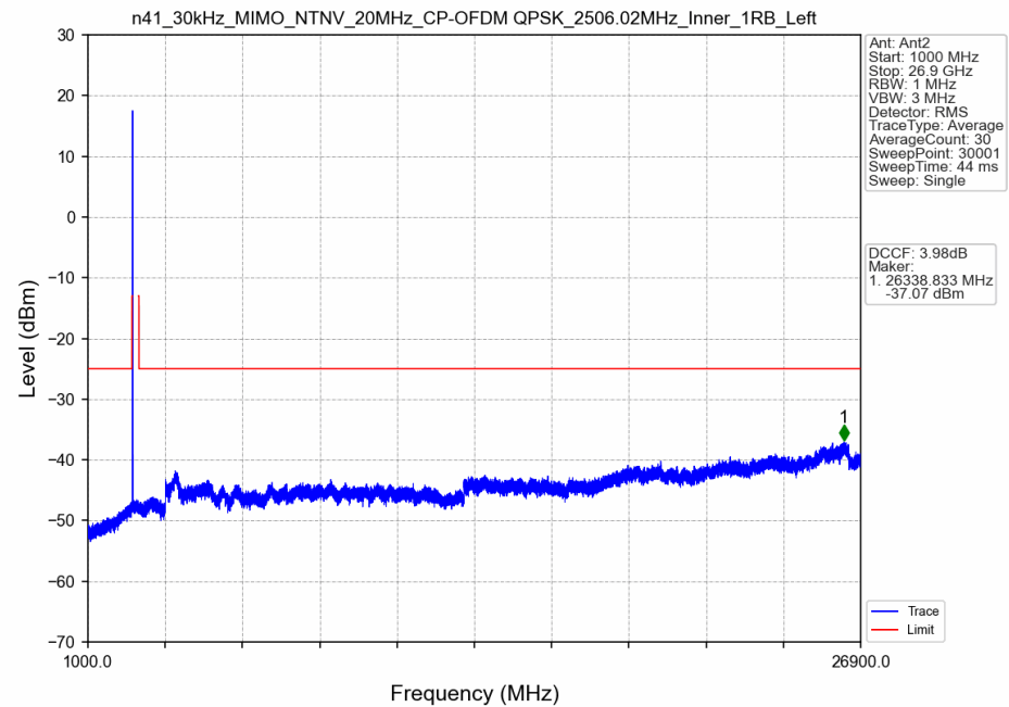
n41_30kHz_MIMO_NTNV_20MHz_CP-OFDM_QPSK_2506.02MHz_Inner_1RB_Left
