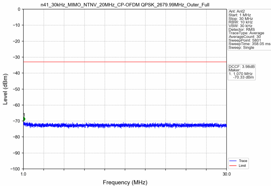
n41_30kHz_MIMO_NTNV_20MHz_CP-OFDM QPSK_2679.99MHz_Outer_Full
