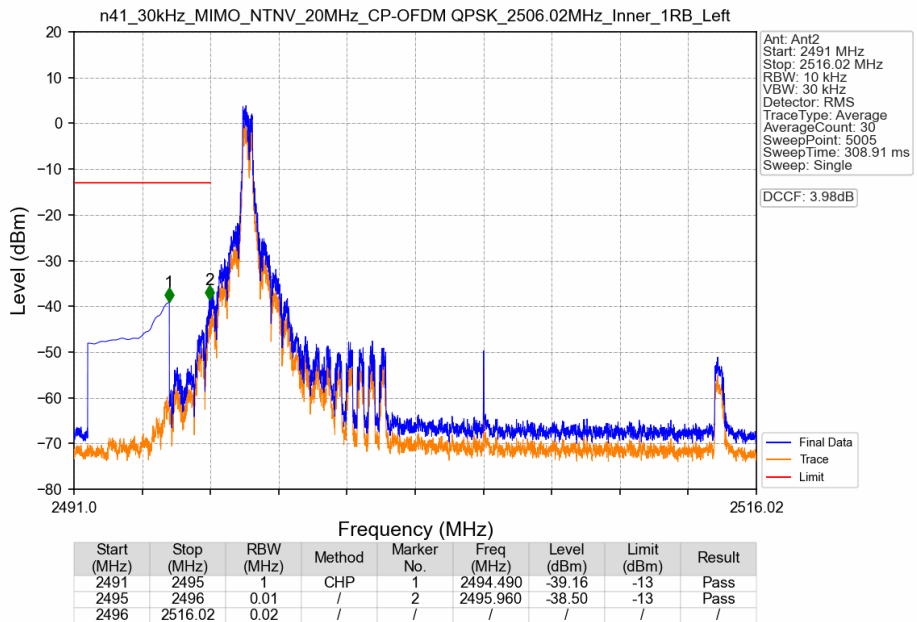
n41_30kHz_MIMO_NTNV_20MHz_CP-OFDM QPSK_2506.02MHz_Inner_1RB_Left
