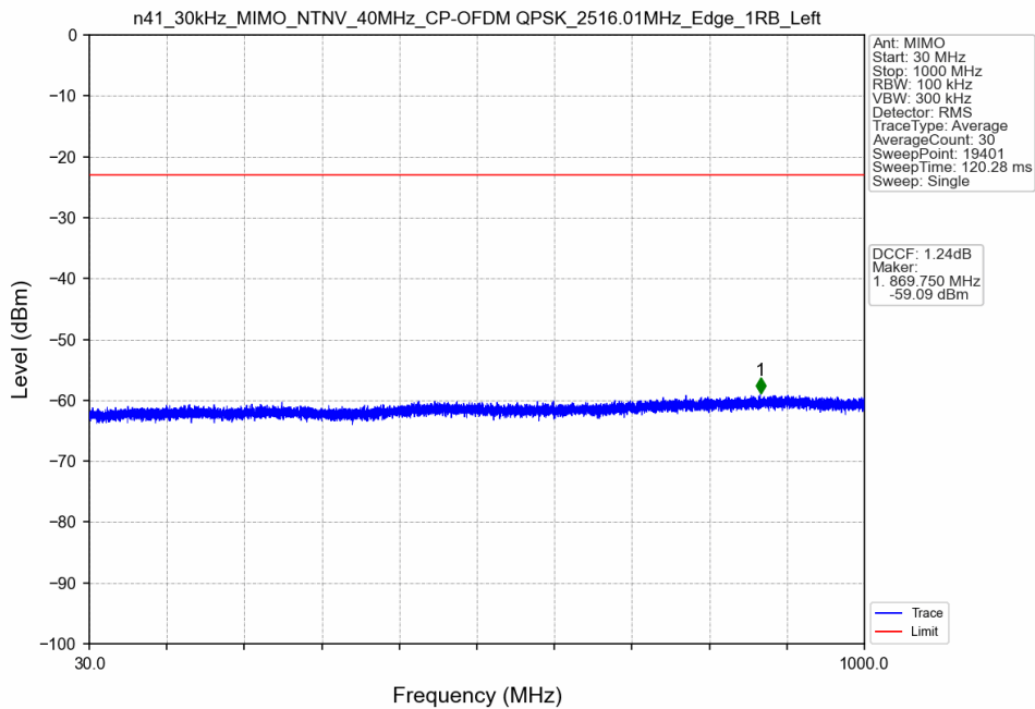
n41_30kHz_MIMO_NTNV_40MHz_CP-OFDM QPSK_2516.01MHz_Edge_1RB_Left
