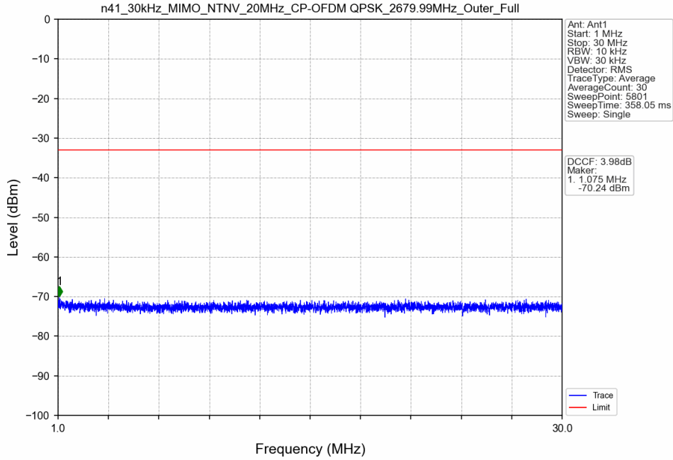
n41_30kHz_MIMO_NTNV_20MHz_CP-OFDM QPSK_2679.99MHz_Outer_Full
