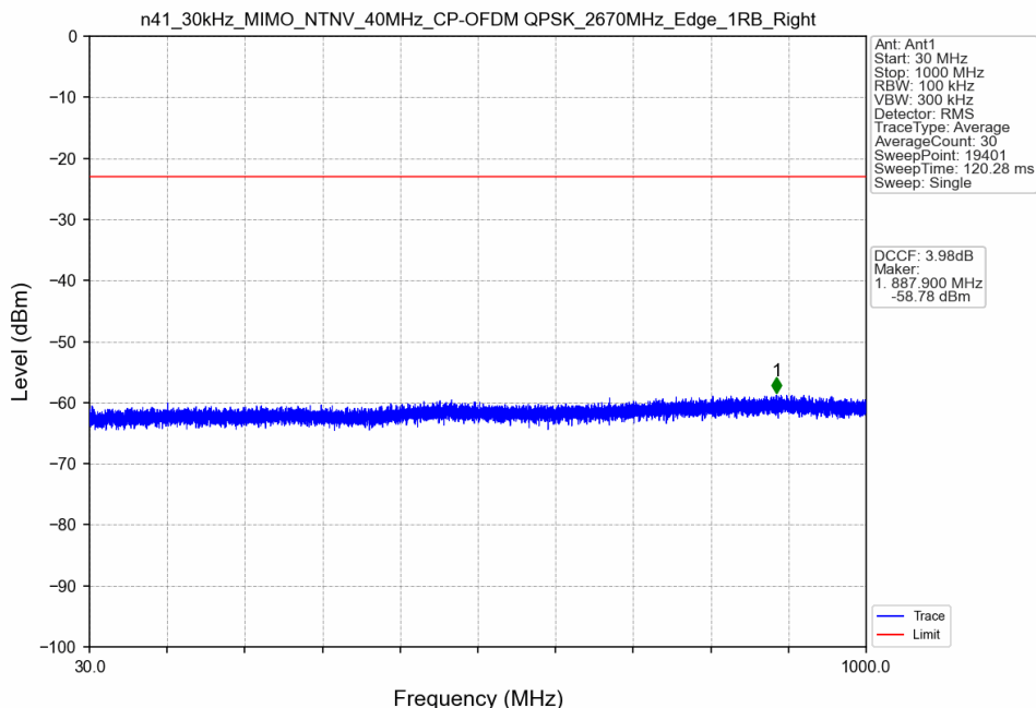
n41_30kHz_MIMO_NTNV_40MHz_CP-OFDM QPSK_2670MHz_Edge_1RB_Right
