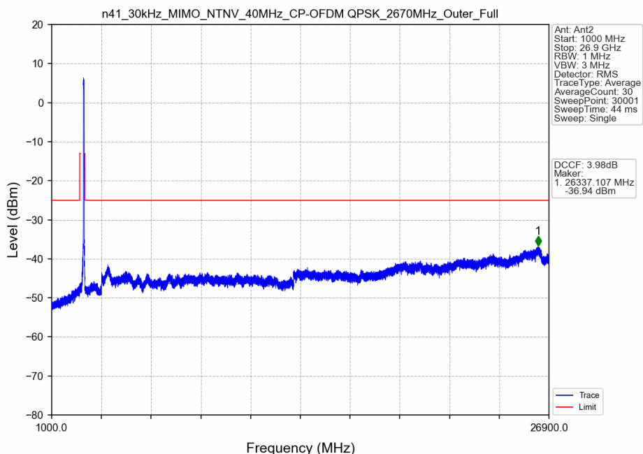
n41_30kHz_MIMO_NTNV_40MHz_CP-OFDM QPSK_2670MHz_Outer_Full
