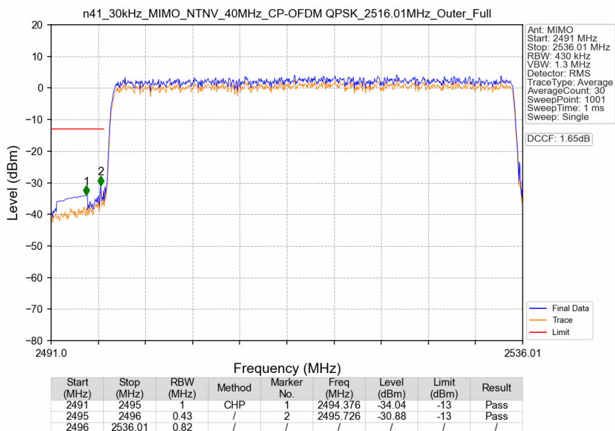
n41_30kHz_MIMO_NTNV_40MHz_CP-OFDM QPSK_2516.01MHz_Outer_Full
