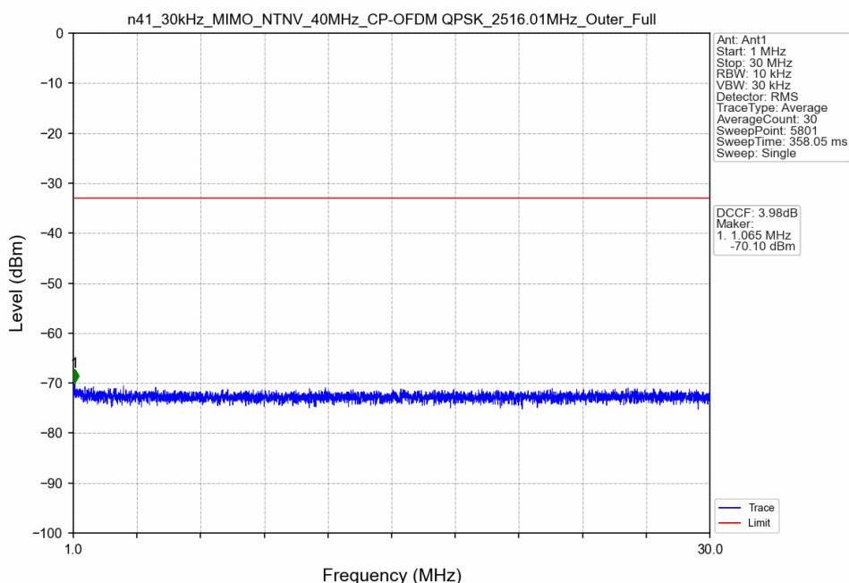
n41_30kHz_MIMO_NTNV_40MHz_CP-OFDM QPSK_2516.01MHz_Outer_Full
