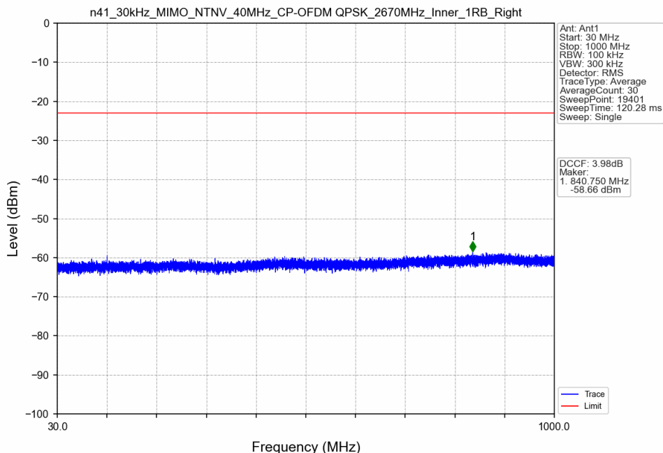
n41_30kHz_MIMO_NTNV_40MHz_CP-OFDM QPSK_2670MHz_Inner_1RB_Right
