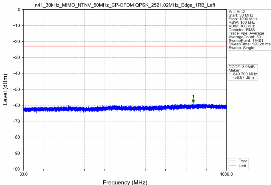
n41_30kHz_MIMO_NTNV_50MHz_CP-OFDM QPSK_2521.02MHz_Edge_1RB_Left
