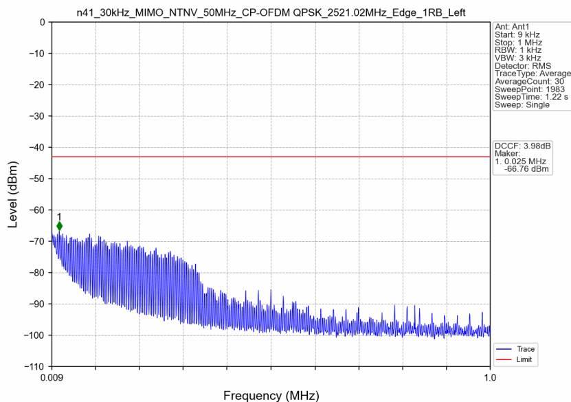
n41_30kHz_MIMO_NTNV_50MHz_CP-OFDM QPSK_2521.02MHz_Edge_1RB_Left
