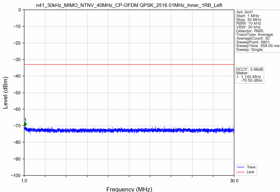
n41_30kHz_MIMO_NTNV_40MHz_CP-OFDM QPSK_2516.01MHz_Inner_1RB_Left
