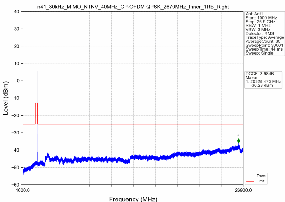
n41_30kHz_MIMO_NTNV_40MHz_CP-OFDM QPSK_2670MHz_Inner_1RB_Right
