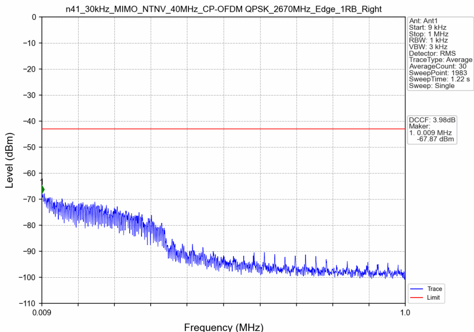
n41_30kHz_MIMO_NTNV_40MHz_CP-OFDM QPSK_2670MHz_Edge_1RB_Right
