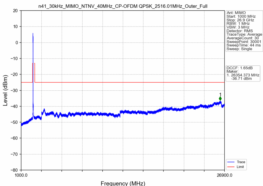
n41_30kHz_MIMO_NTNV_40MHz_CP-OFDM QPSK_2516.01MHz_Outer_Full
