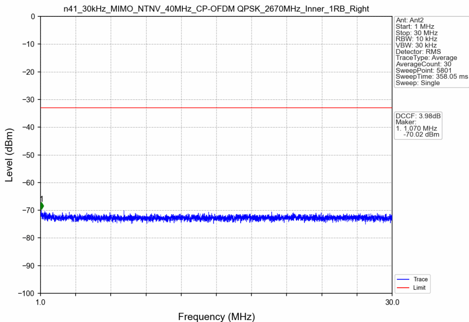
n41_30kHz_MIMO_NTNV_40MHz_CP-OFDM QPSK_2670MHz_Inner_1RB_Right
