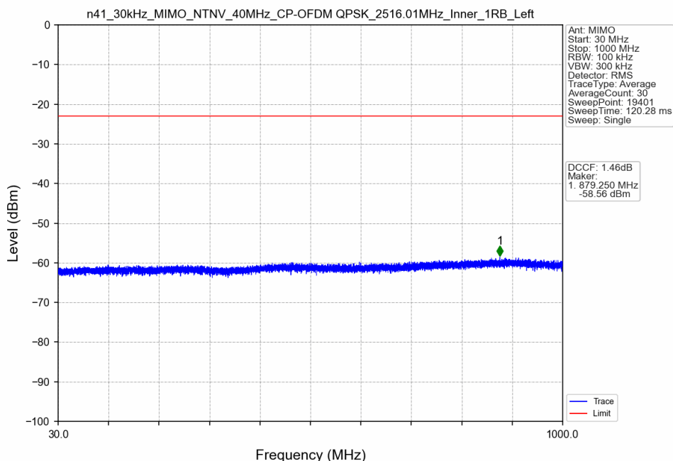
n41_30kHz_MIMO_NTNV_40MHz_CP-OFDM QPSK_2516.01MHz_Inner_1RB_Left
