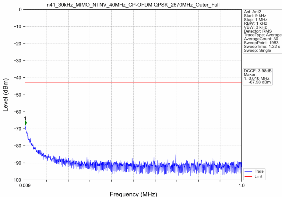
n41_30kHz_MIMO_NTNV_40MHz_CP-OFDM QPSK_2670MHz_Outer_Full
