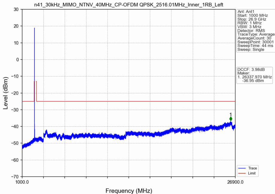
n41_30kHz_MIMO_NTNV_40MHz_CP-OFDM QPSK_2516.01MHz_Inner_1RB_Left
