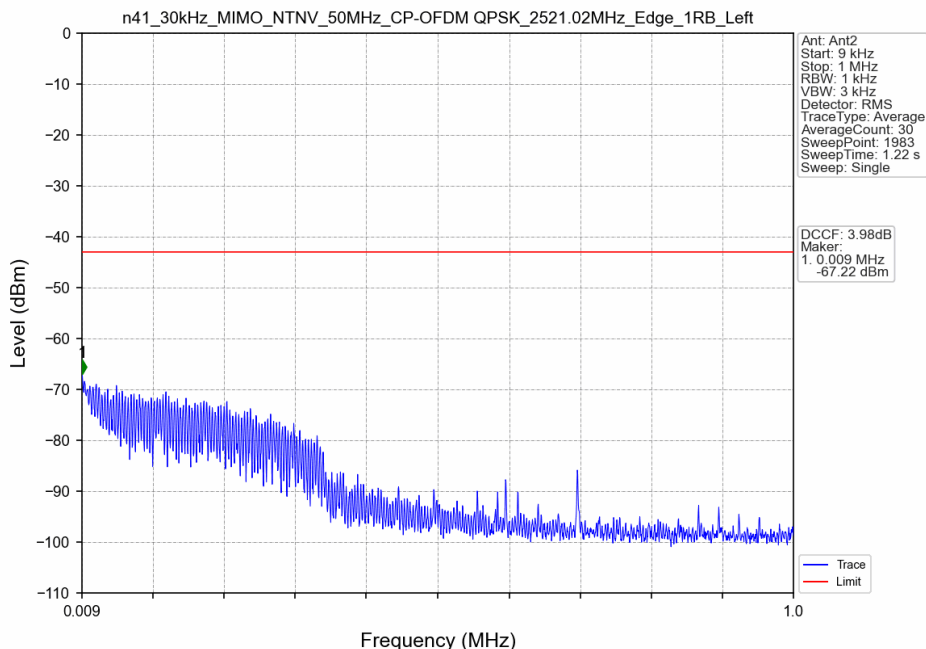
n41_30kHz_MIMO_NTNV_50MHz_CP-OFDM QPSK_2521.02MHz_Edge_1RB_Left
