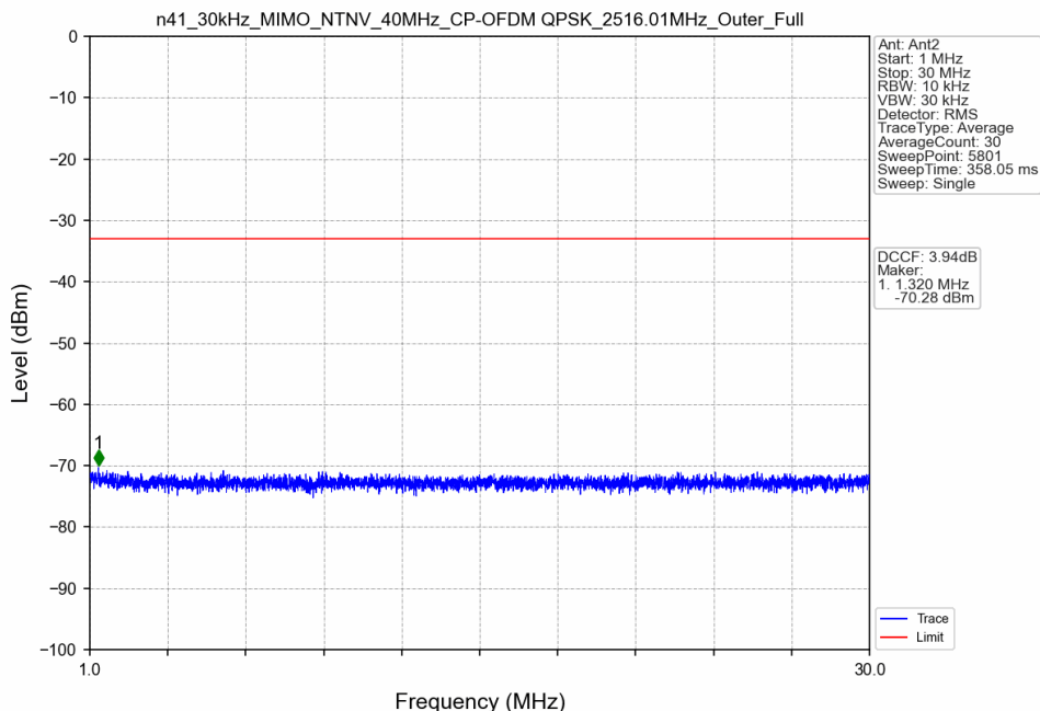
n41_30kHz_MIMO_NTNV_40MHz_CP-OFDM QPSK_2516.01MHz_Outer_Full
