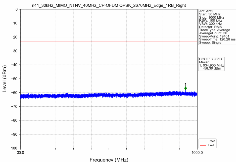
n41_30kHz_MIMO_NTNV_40MHz_CP-OFDM QPSK_2670MHz_Edge_1RB_Right
