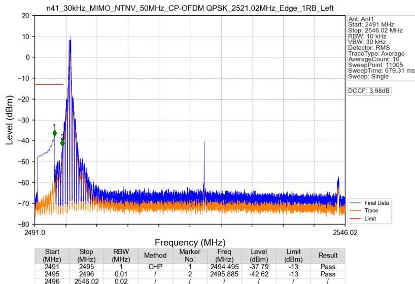
n41_30kHz_MIMO_NTNV_50MHz_CP-OFDM QPSK_2521.02MHz_Edge_1RB_Left
