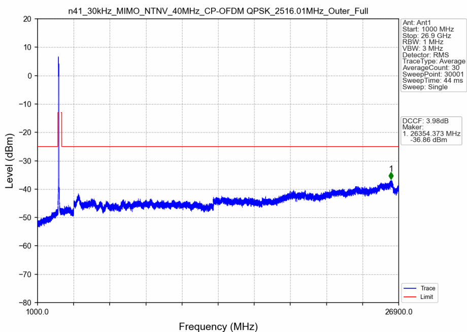
n41_30kHz_MIMO_NTNV_40MHz_CP-OFDM QPSK_2516.01MHz_Outer_Full
