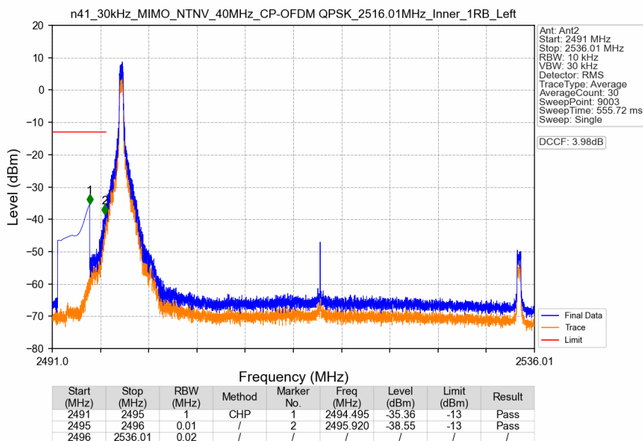
n41_30kHz_MIMO_NTNV_40MHz_CP-OFDM QPSK_2516.01MHz_Inner_1RB_Left
