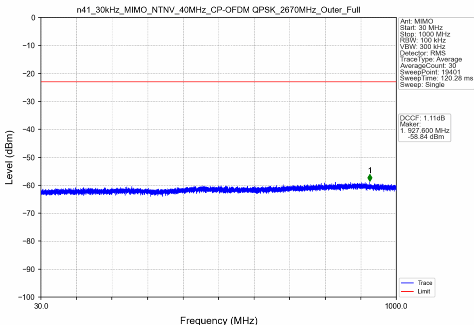
n41_30kHz_MIMO_NTNV_40MHz_CP-OFDM QPSK_2670MHz_Outer_Full
