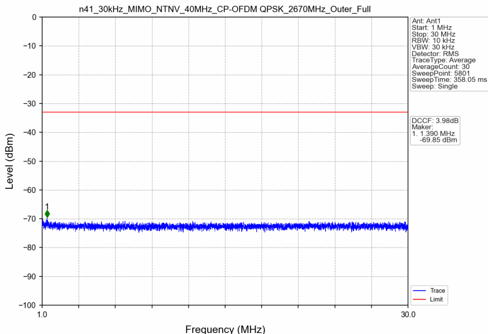
n41_30kHz_MIMO_NTNV_40MHz_CP-OFDM QPSK_2670MHz_Outer_Full
