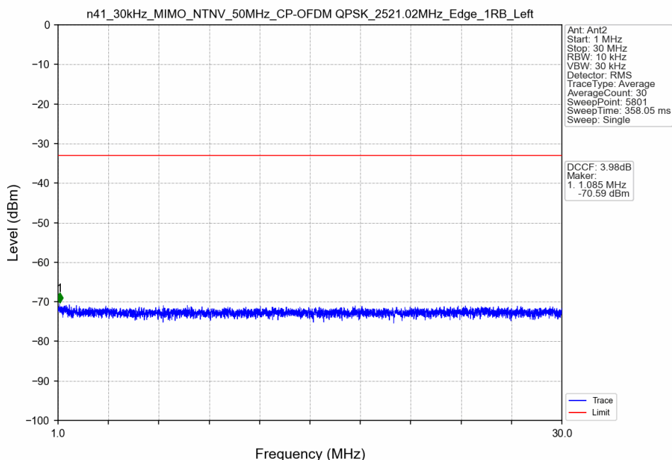
n41_30kHz_MIMO_NTNV_50MHz_CP-OFDM QPSK_2521.02MHz_Edge_1RB_Left
