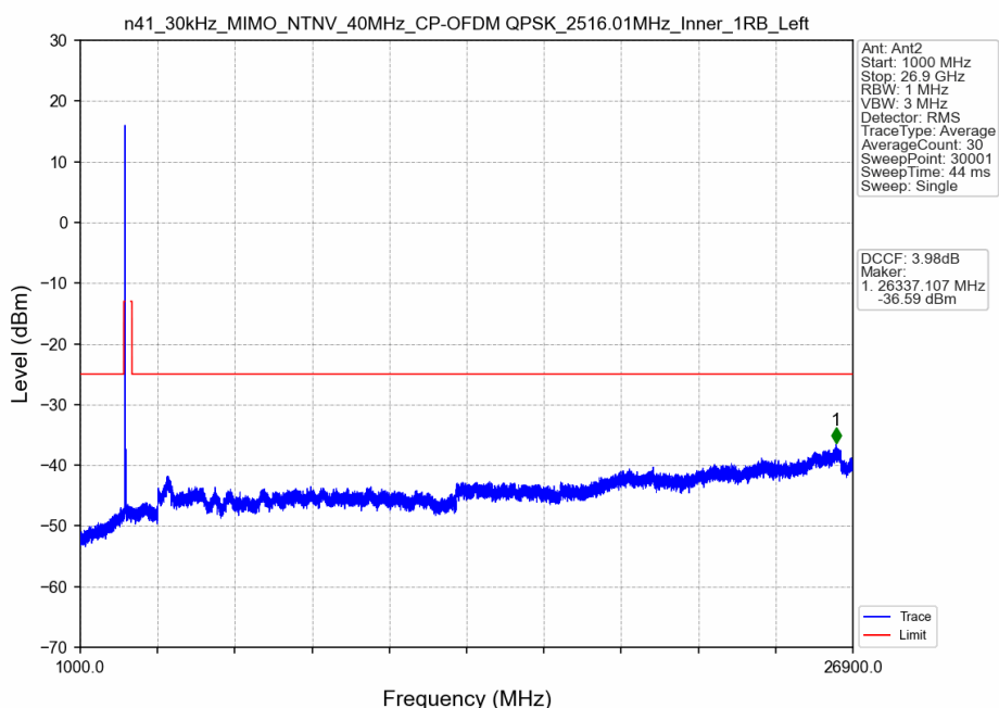
n41_30kHz_MIMO_NTNV_40MHz_CP-OFDM QPSK_2516.01MHz_Inner_1RB_Left
