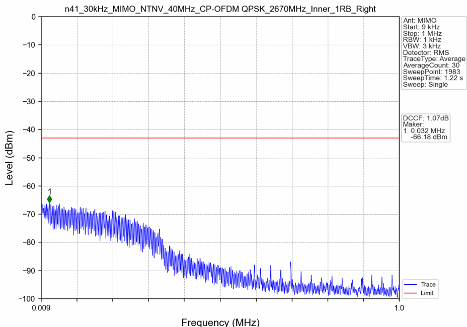
n41_30kHz_MIMO_NTNV_40MHz_CP-OFDM QPSK_2670MHz_Inner_1RB_Right
