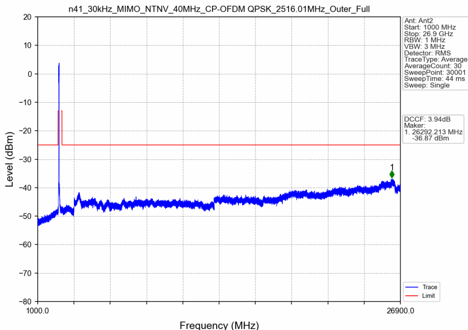
n41_30kHz_MIMO_NTNV_40MHz_CP-OFDM QPSK_2516.01MHz_Outer_Full
