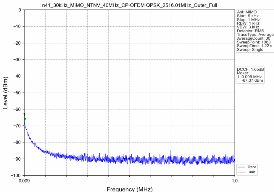
n41_30kHz_MIMO_NTNV_40MHz_CP-OFDM QPSK_2516.01MHz_Outer_Full
