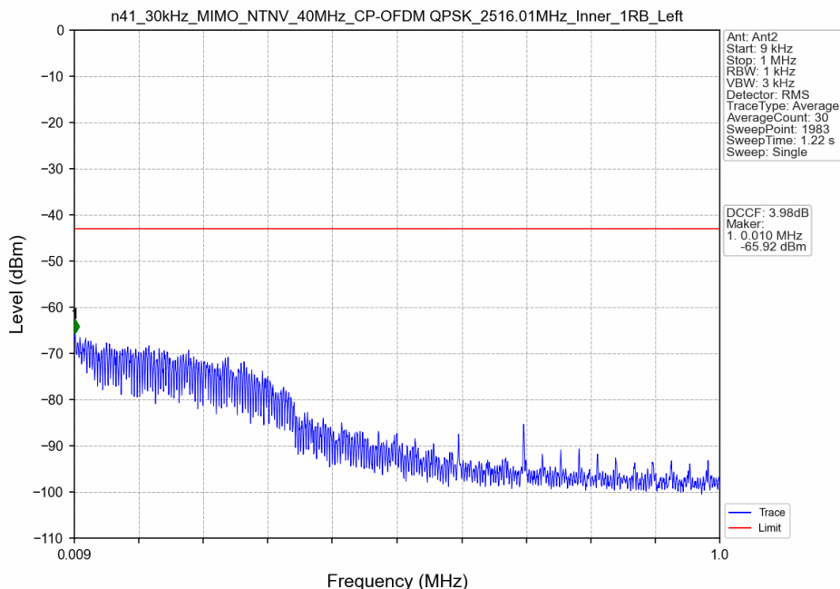
n41_30kHz_MIMO_NTNV_40MHz_CP-OFDM QPSK_2516.01MHz_Inner_1RB_Left
