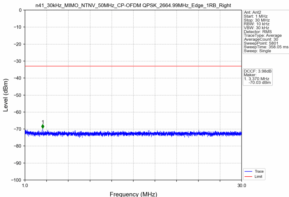
n41_30kHz_MIMO_NTNV_50MHz_CP-OFDM QPSK_2664.99MHz_Edge_1RB_Right
