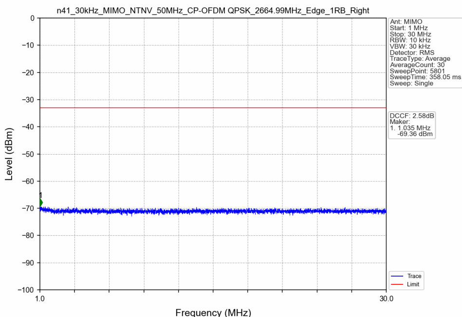
n41_30kHz_MIMO_NTNV_50MHz_CP-OFDM QPSK_2664.99MHz_Edge_1RB_Right
