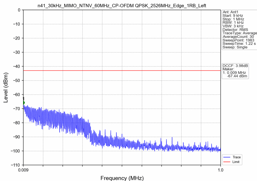
n41_30kHz_MIMO_NTNV_60MHz_CP-OFDM QPSK_2526MHz_Edge_1RB_Left
