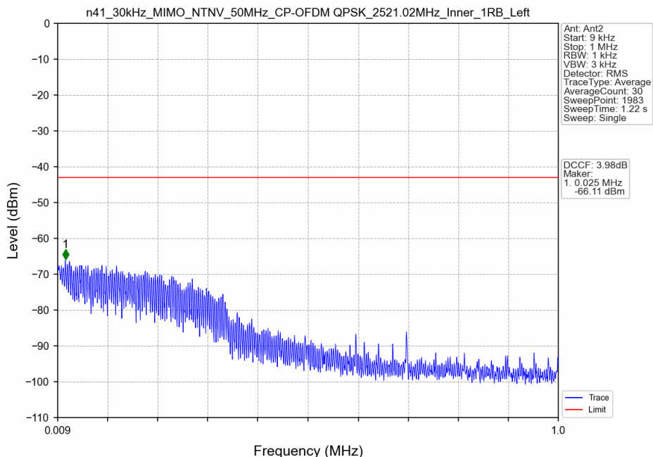
n41_30kHz_MIMO_NTNV_50MHz_CP-OFDM QPSK_2521.02MHz_Inner_1RB_Left
