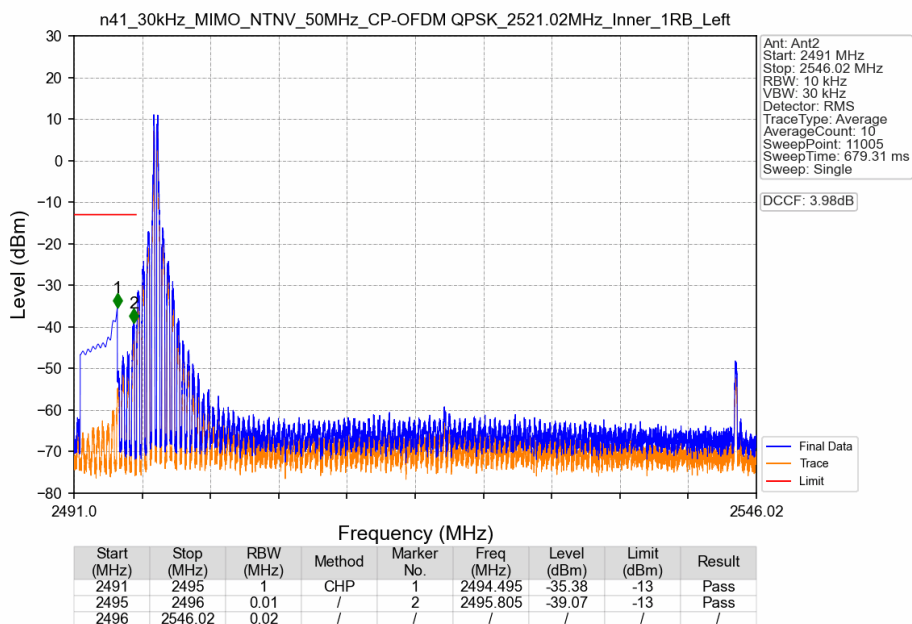
n41_30kHz_MIMO_NTNV_50MHz_CP-OFDM QPSK_2521.02MHz_Inner_1RB_Left
