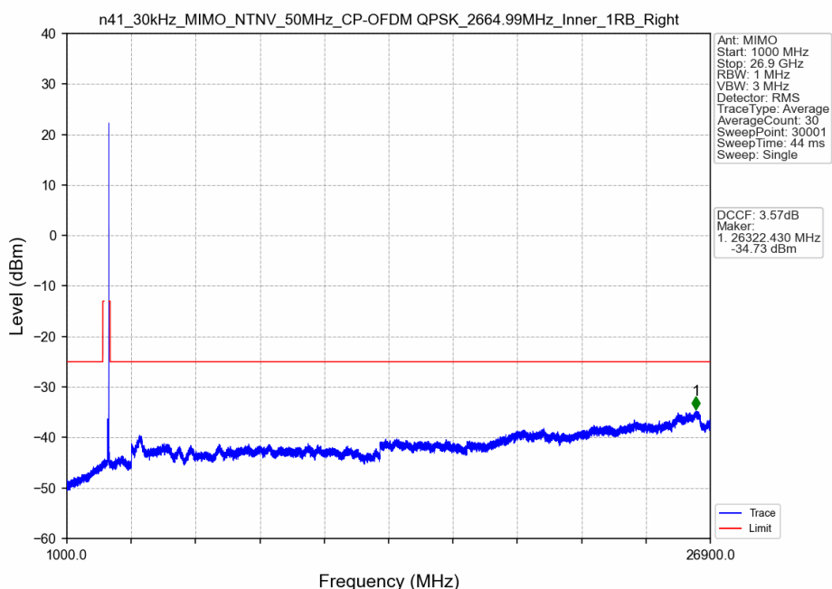
n41_30kHz_MIMO_NTNV_50MHz_CP-OFDM QPSK_2664.99MHz_Inner_1RB_Right
