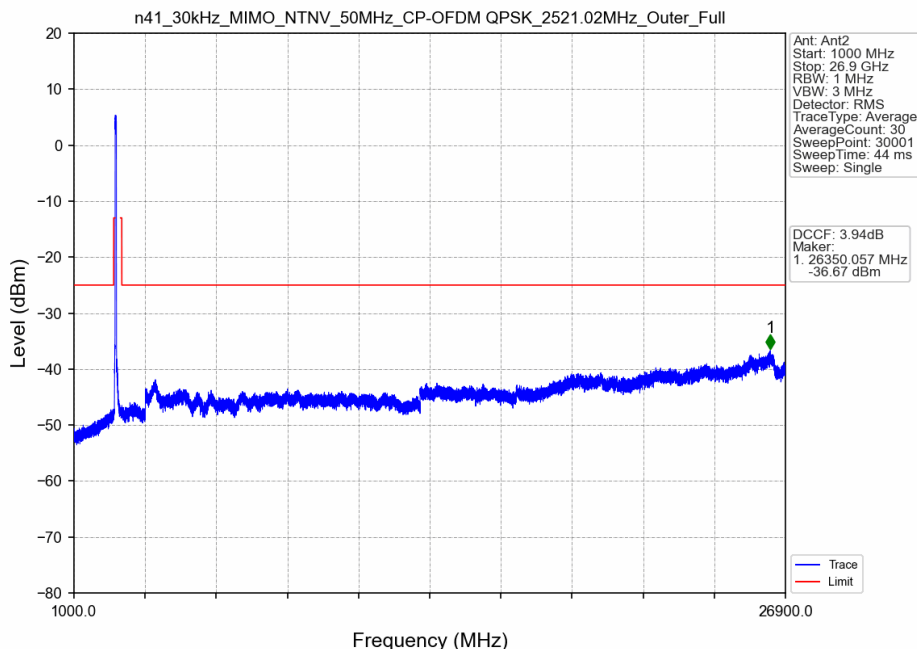
n41_30kHz_MIMO_NTNV_50MHz_CP-OFDM QPSK_2521.02MHz_Outer_Full
