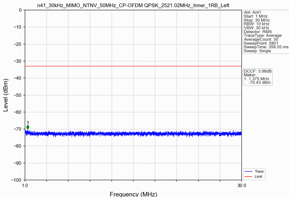
n41_30kHz_MIMO_NTNV_50MHz_CP-OFDM QPSK_2521.02MHz_Inner_1RB_Left
