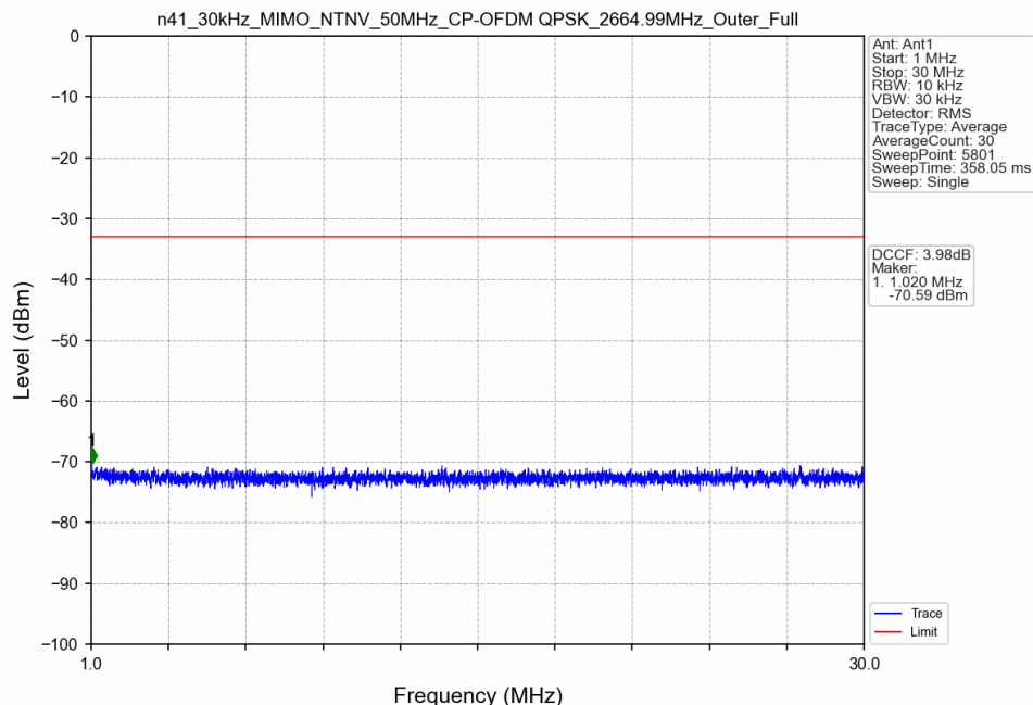
n41_30kHz_MIMO_NTNV_50MHz_CP-OFDM QPSK_2664.99MHz_Outer_Full
