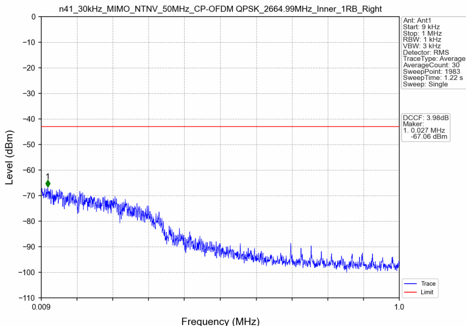
n41_30kHz_MIMO_NTNV_50MHz_CP-OFDM QPSK_2664.99MHz_Inner_1RB_Right
