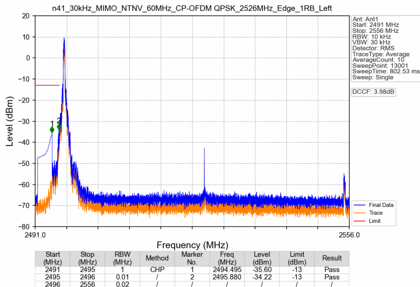
n41_30kHz_MIMO_NTNV_60MHz_CP-OFDM QPSK_2526MHz_Edge_1RB_Left
