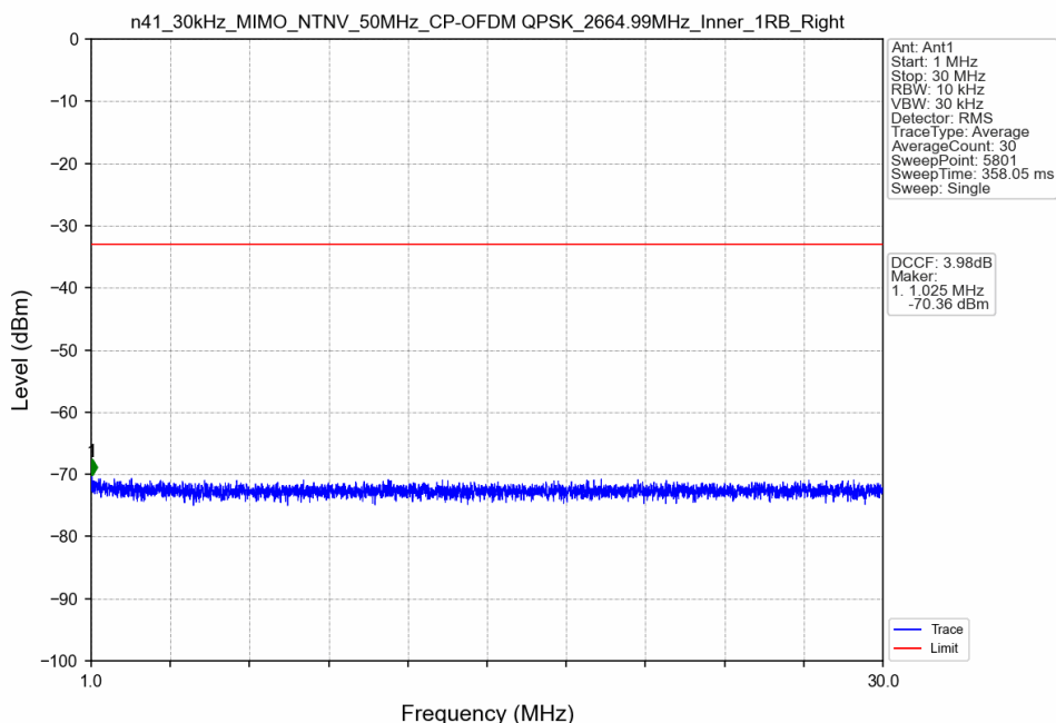
n41_30kHz_MIMO_NTNV_50MHz_CP-OFDM QPSK_2664.99MHz_Inner_1RB_Right
