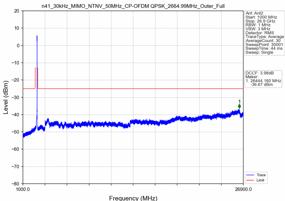
n41_30kHz_MIMO_NTNV_50MHz_CP-OFDM QPSK_2664.99MHz_Outer_Full
