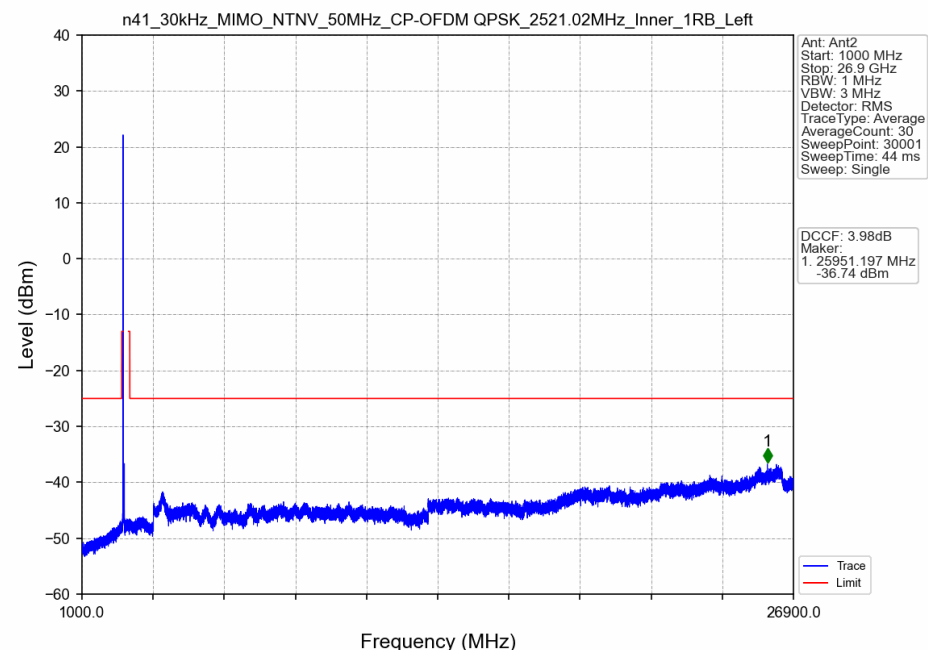
n41_30kHz_MIMO_NTNV_50MHz_CP-OFDM QPSK_2521.02MHz_Inner_1RB_Left
