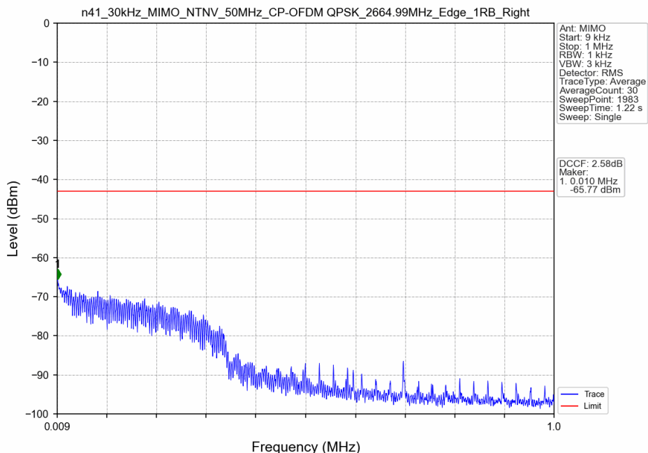
n41_30kHz_MIMO_NTNV_50MHz_CP-OFDM QPSK_2664.99MHz_Edge_1RB_Right
