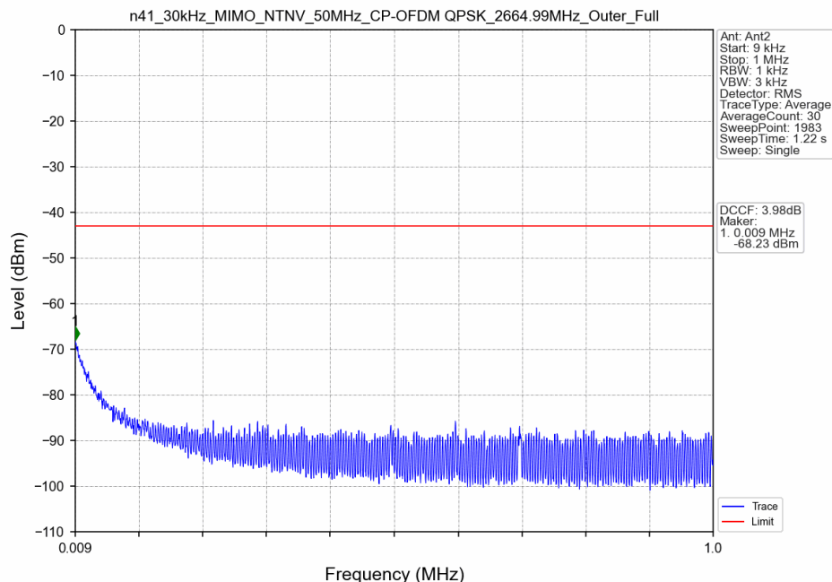
n41_30kHz_MIMO_NTNV_50MHz_CP-OFDM QPSK_2664.99MHz_Outer_Full
