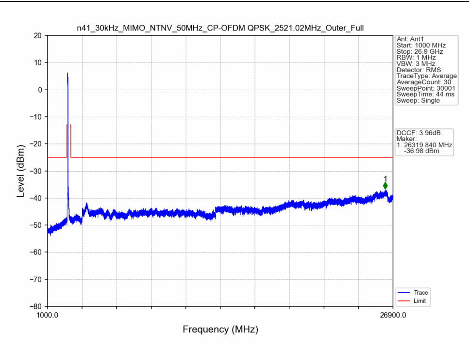
n41_30kHz_MIMO_NTNV_50MHz_CP-OFDM QPSK_2521.02MHz_Outer_Full
