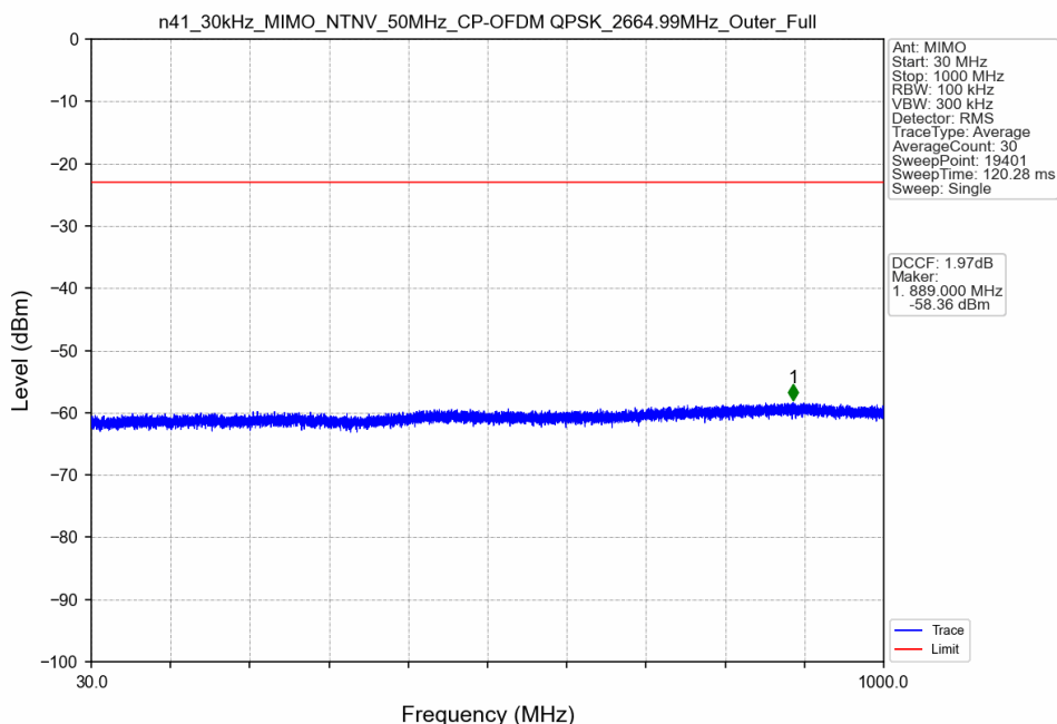
n41_30kHz_MIMO_NTNV_50MHz_CP-OFDM QPSK_2664.99MHz_Outer_Full
