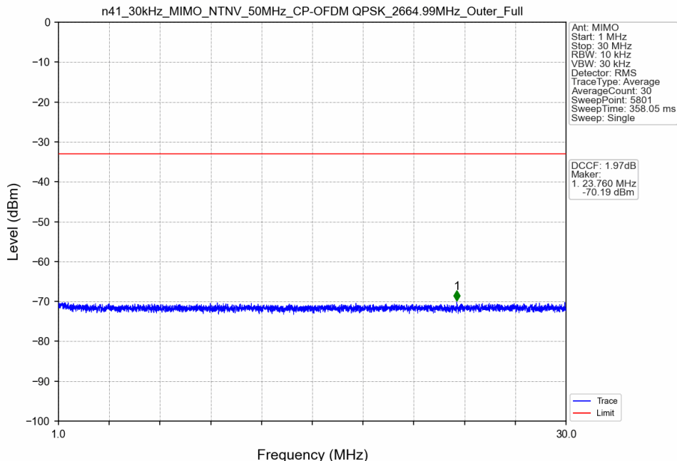
n41_30kHz_MIMO_NTNV_50MHz_CP-OFDM QPSK_2664.99MHz_Outer_Full
