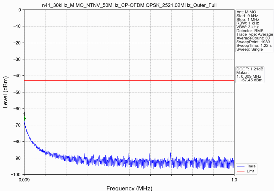
n41_30kHz_MIMO_NTNV_50MHz_CP-OFDM QPSK_2521.02MHz_Outer_Full
