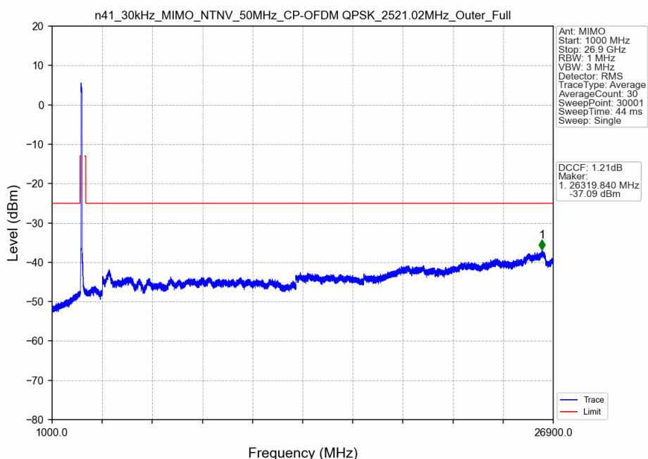
n41_30kHz_MIMO_NTNV_50MHz_CP-OFDM QPSK_2521.02MHz_Outer_Full
