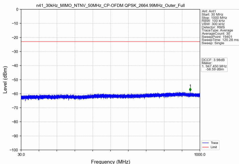
n41_30kHz_MIMO_NTNV_50MHz_CP-OFDM QPSK_2664.99MHz_Outer_Full
