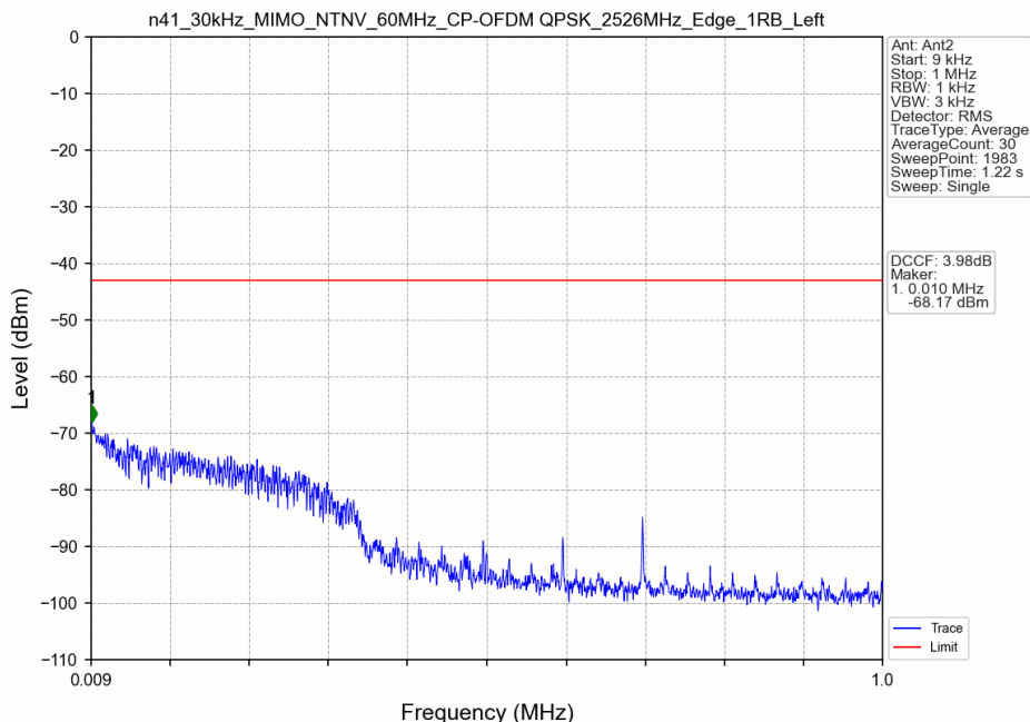
n41_30kHz_MIMO_NTNV_60MHz_CP-OFDM QPSK_2526MHz_Edge_1RB_Left
