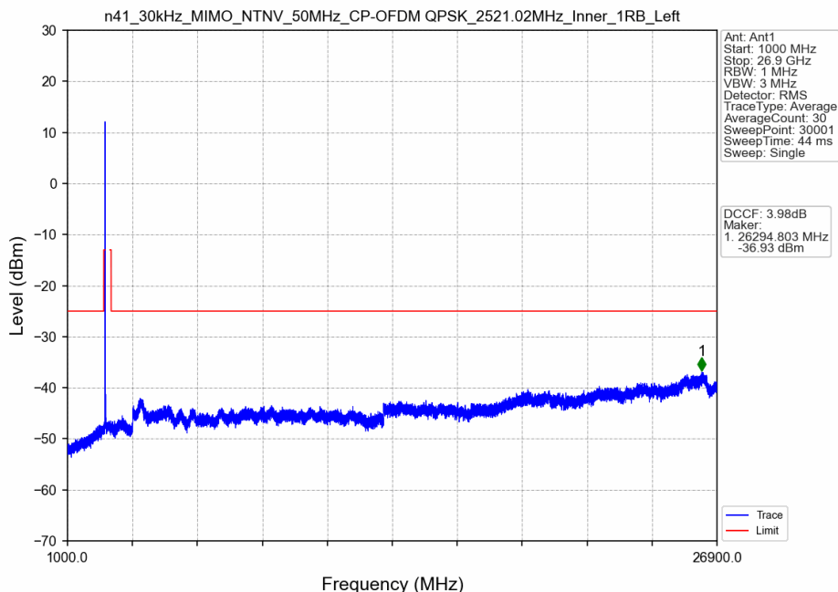
n41_30kHz_MIMO_NTNV_50MHz_CP-OFDM QPSK_2521.02MHz_Inner_1RB_Left
