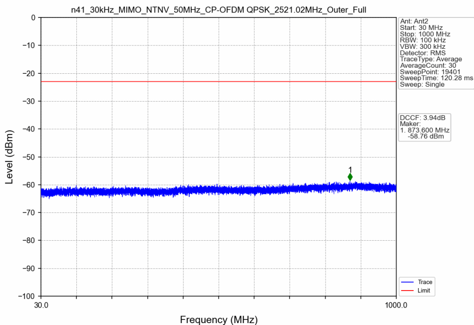
n41_30kHz_MIMO_NTNV_50MHz_CP-OFDM QPSK_2521.02MHz_Outer_Full
