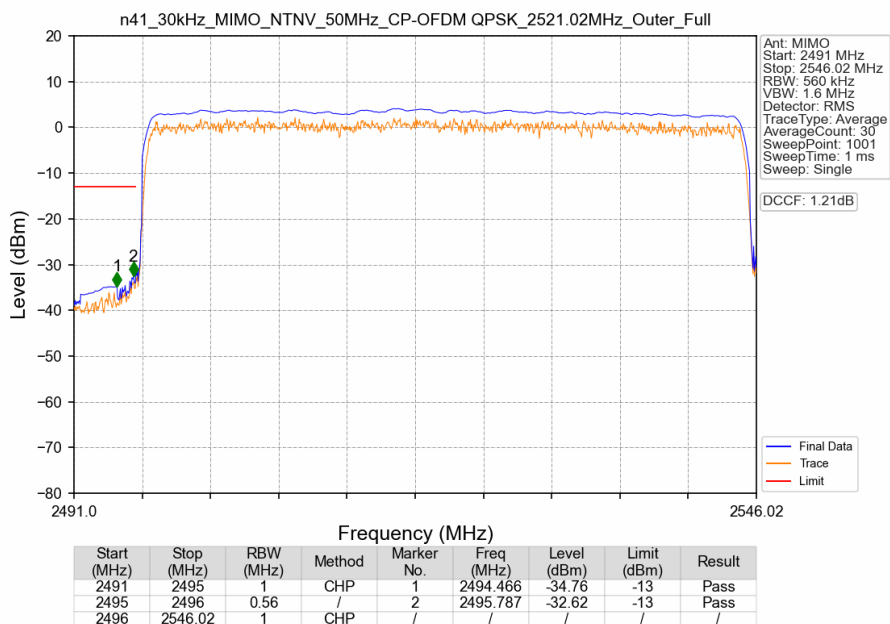
n41_30kHz_MIMO_NTNV_50MHz_CP-OFDM QPSK_2521.02MHz_Outer_Full
