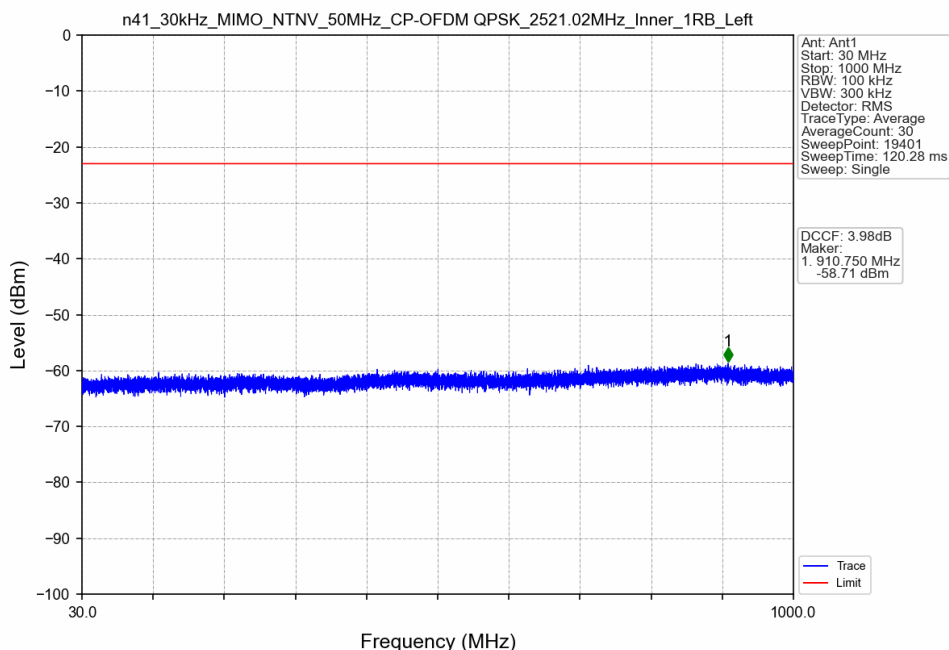
n41_30kHz_MIMO_NTNV_50MHz_CP-OFDM QPSK_2521.02MHz_Inner_1RB_Left
