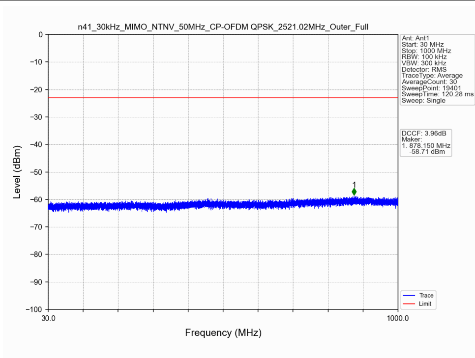
n41_30kHz_MIMO_NTNV_50MHz_CP-OFDM QPSK_2521.02MHz_Outer_Full
