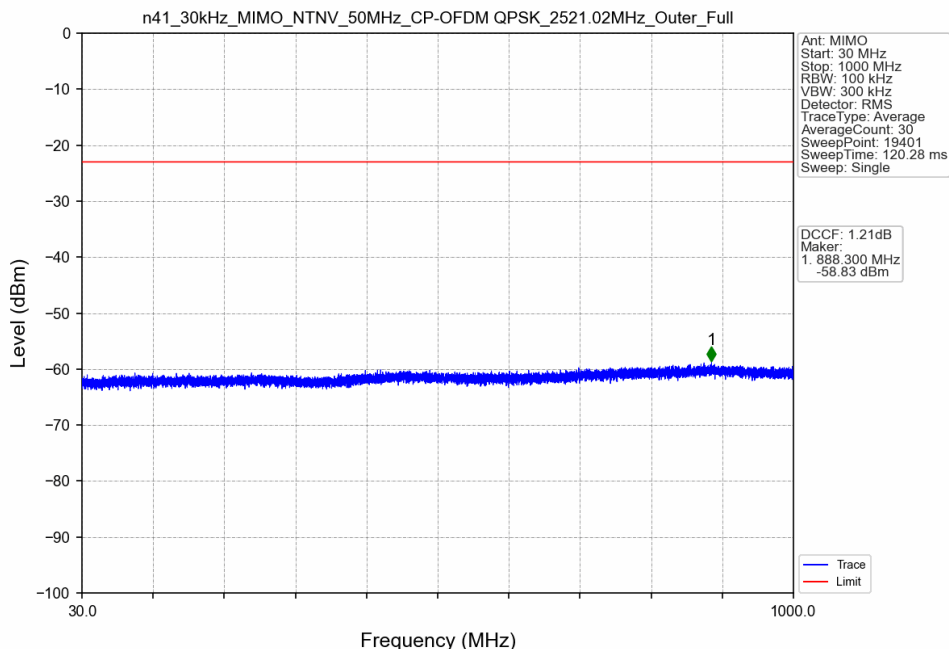
n41_30kHz_MIMO_NTNV_50MHz_CP-OFDM QPSK_2521.02MHz_Outer_Full
