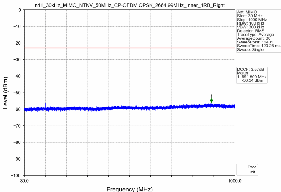
n41_30kHz_MIMO_NTNV_50MHz_CP-OFDM QPSK_2664.99MHz_Inner_1RB_Right
