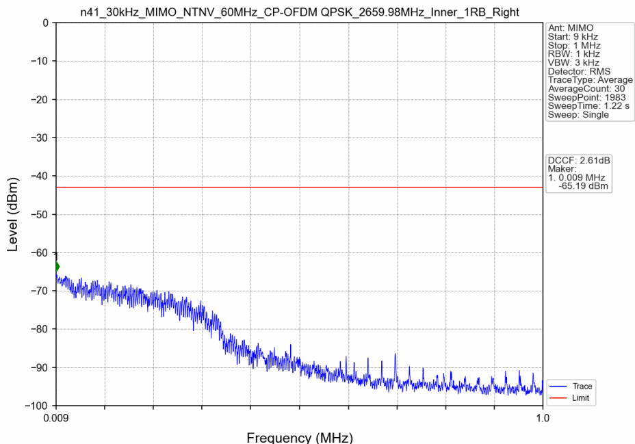
n41_30kHz_MIMO_NTNV_60MHz_CP-OFDM QPSK_2659.98MHz_Inner_1RB_Right
