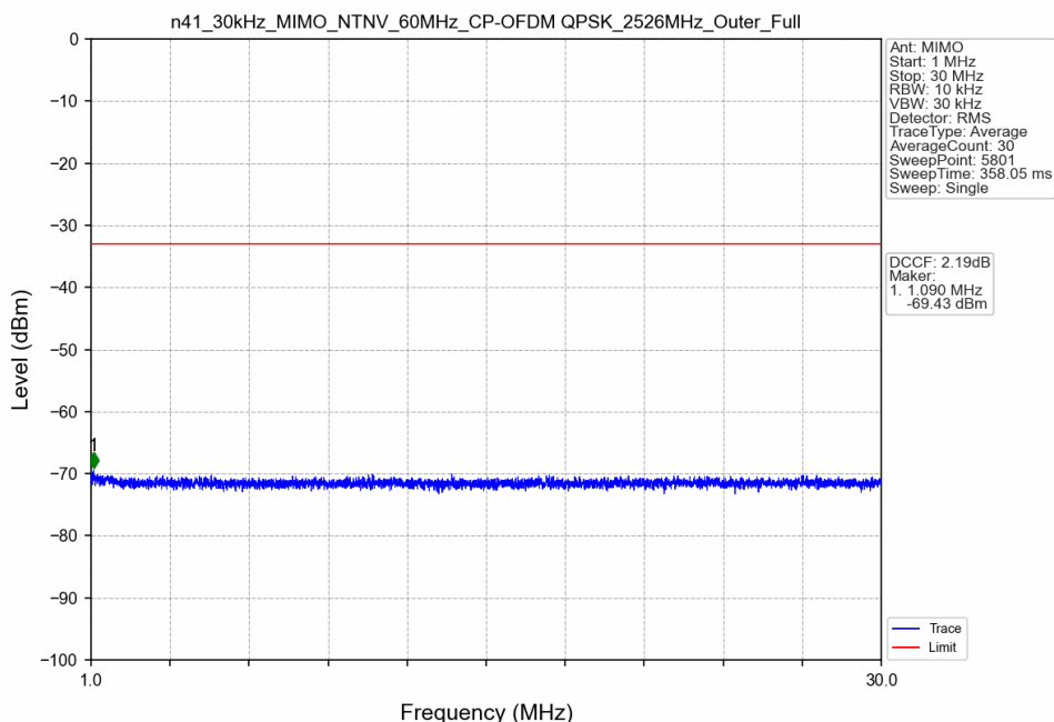
n41_30kHz_MIMO_NTNV_60MHz_CP-OFDM QPSK_2526MHz_Outer_Full
