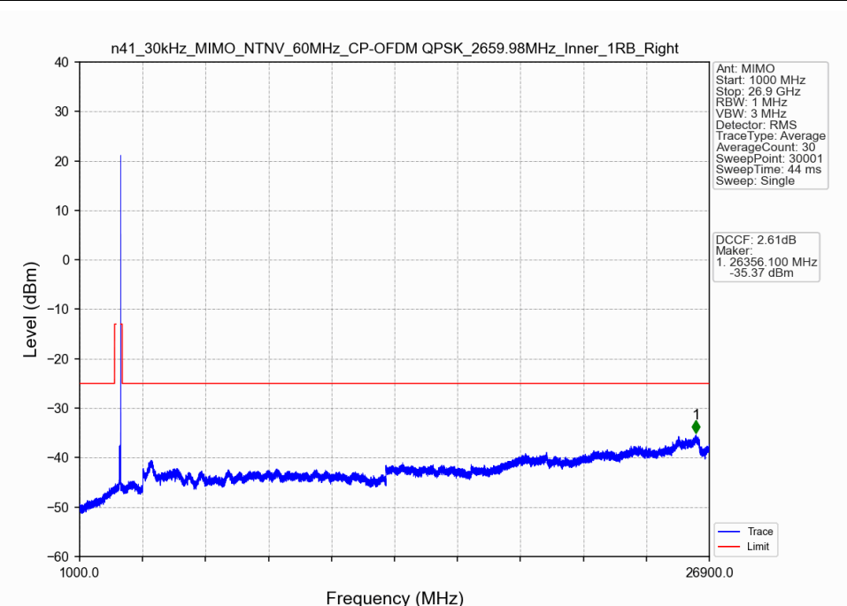
n41_30kHz_MIMO_NTNV_60MHz_CP-OFDM QPSK_2659.98MHz_Inner_1RB_Right
