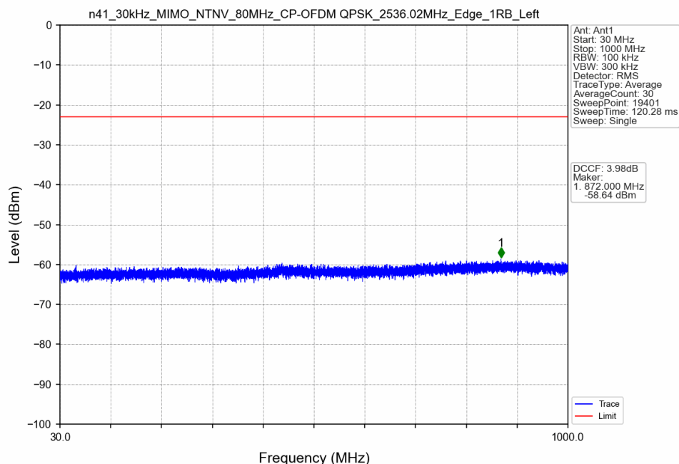
n41_30kHz_MIMO_NTNV_80MHz_CP-OFDM QPSK_2536.02MHz_Edge_1RB_Left
