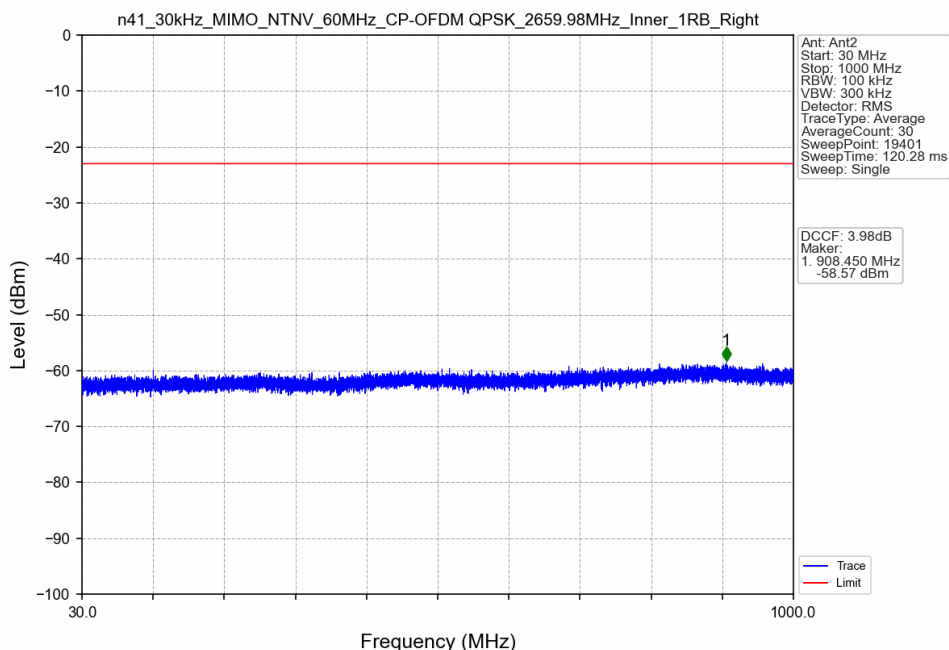
n41_30kHz_MIMO_NTNV_60MHz_CP-OFDM QPSK_2659.98MHz_Inner_1RB_Right
