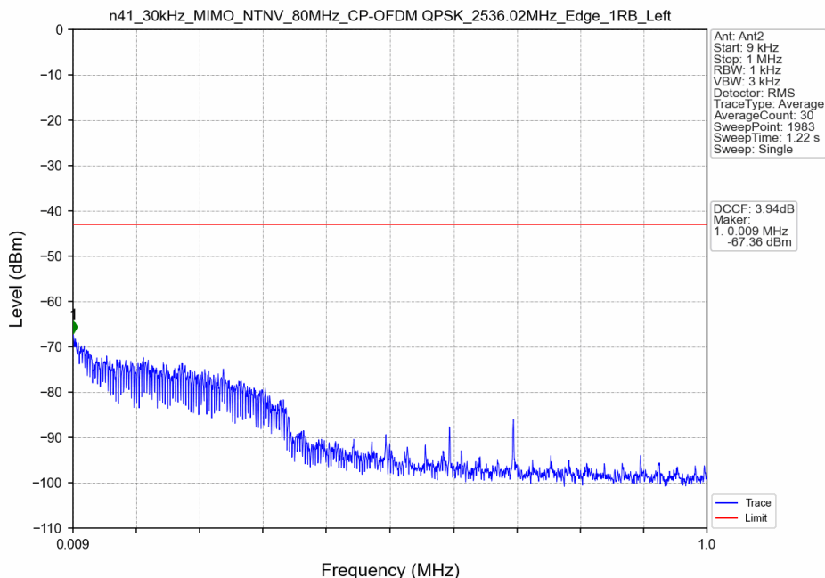
n41_30kHz_MIMO_NTNV_80MHz_CP-OFDM QPSK_2536.02MHz_Edge_1RB_Left
