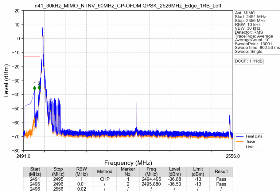
n41_30kHz_MIMO_NTNV_60MHz_CP-OFDM QPSK_2526MHz_Edge_1RB_Left
