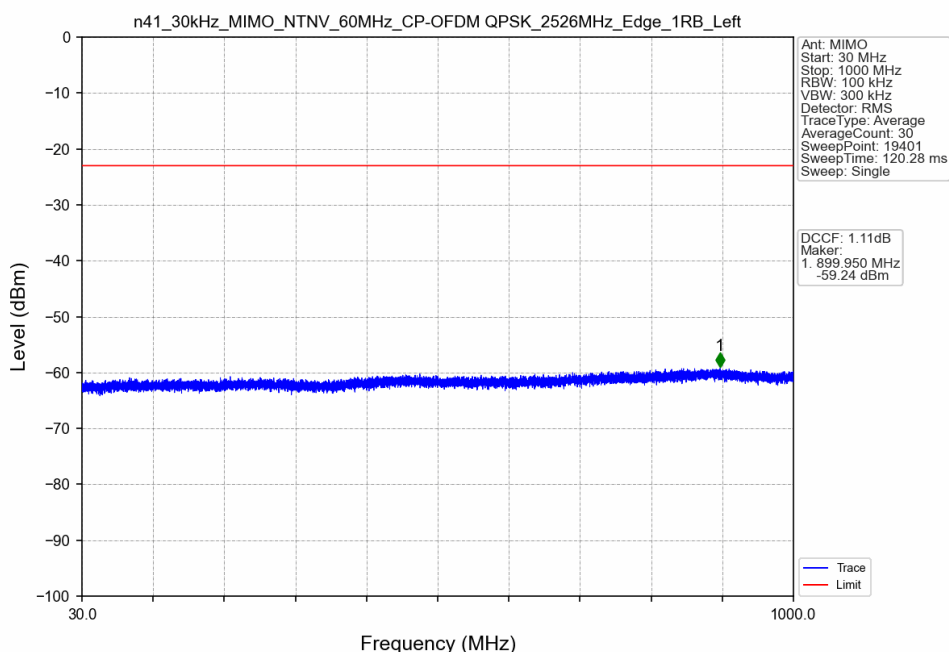
n41_30kHz_MIMO_NTNV_60MHz_CP-OFDM QPSK_2526MHz_Edge_1RB_Left
