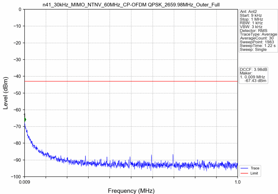
n41_30kHz_MIMO_NTNV_60MHz_CP-OFDM QPSK_2659.98MHz_Outer_Full
