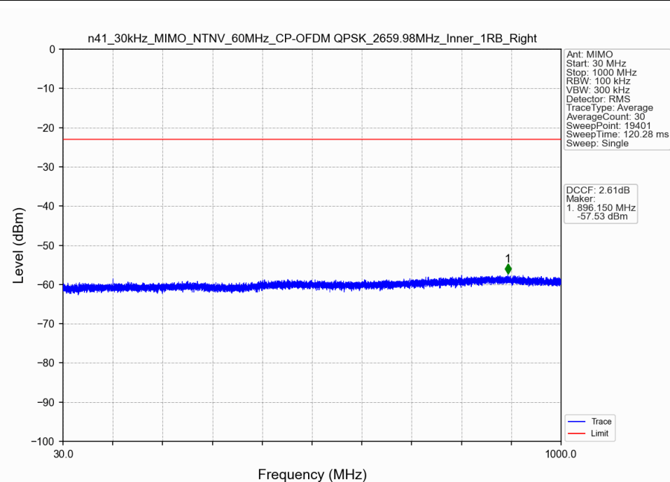
n41_30kHz_MIMO_NTNV_60MHz_CP-OFDM QPSK_2659.98MHz_Inner_1RB_Right
