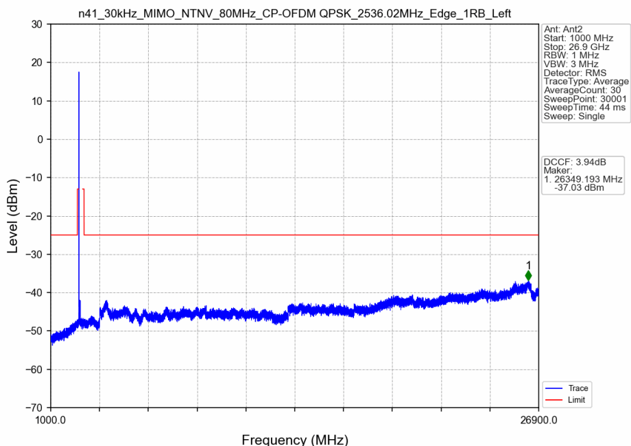
n41_30kHz_MIMO_NTNV_80MHz_CP-OFDM QPSK_2536.02MHz_Edge_1RB_Left
