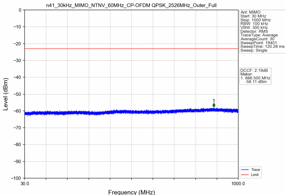
n41_30kHz_MIMO_NTNV_60MHz_CP-OFDM QPSK_2526MHz_Outer_Full
