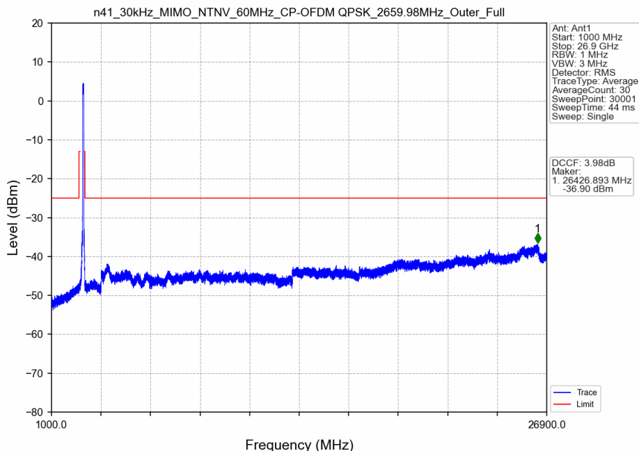
n41_30kHz_MIMO_NTNV_60MHz_CP-OFDM QPSK_2659.98MHz_Outer_Full
