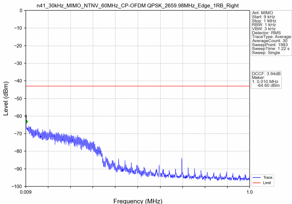
n41_30kHz_MIMO_NTNV_60MHz_CP-OFDM QPSK_2659.98MHz_Edge_1RB_Right
