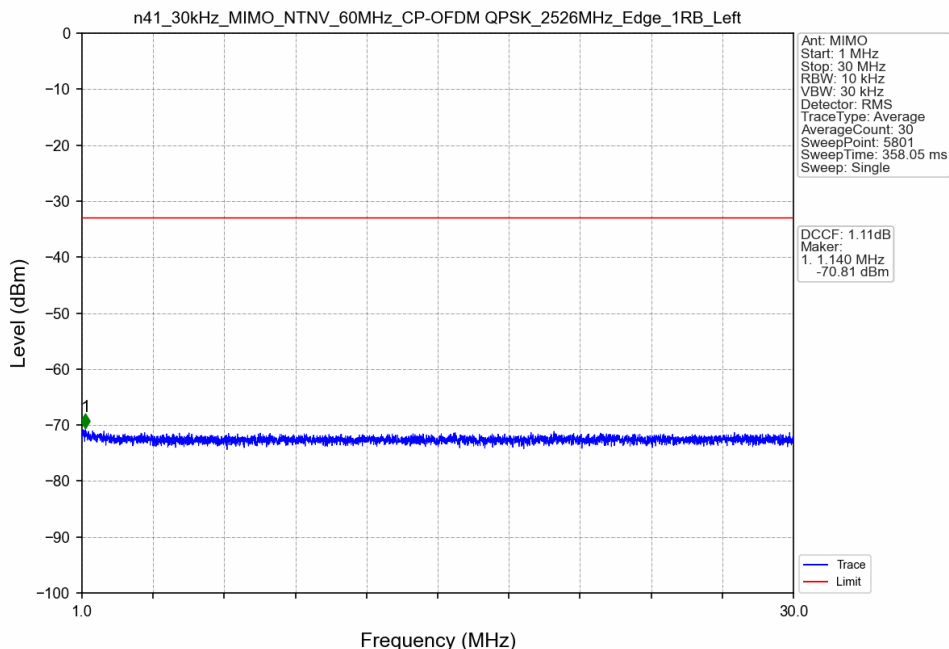
n41_30kHz_MIMO_NTNV_60MHz_CP-OFDM QPSK_2526MHz_Edge_1RB_Left
