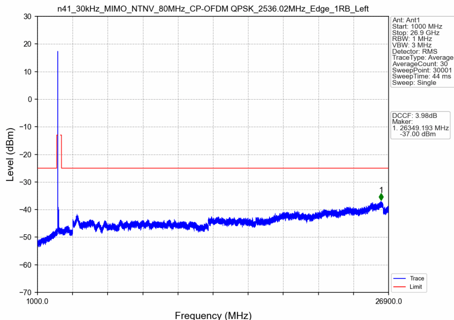
n41_30kHz_MIMO_NTNV_80MHz_CP-OFDM QPSK_2536.02MHz_Edge_1RB_Left
