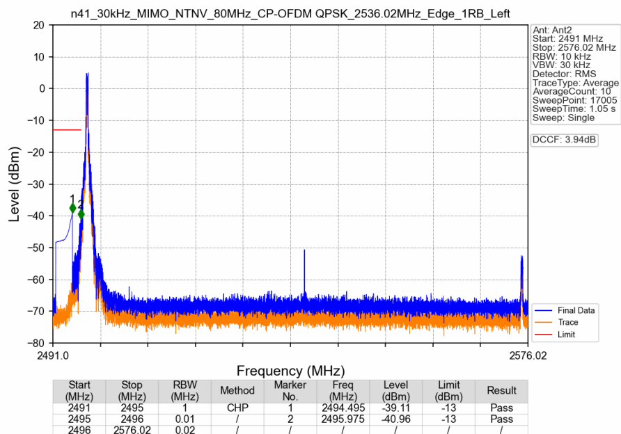
n41_30kHz_MIMO_NTNV_80MHz_CP-OFDM QPSK_2536.02MHz_Edge_1RB_Left
