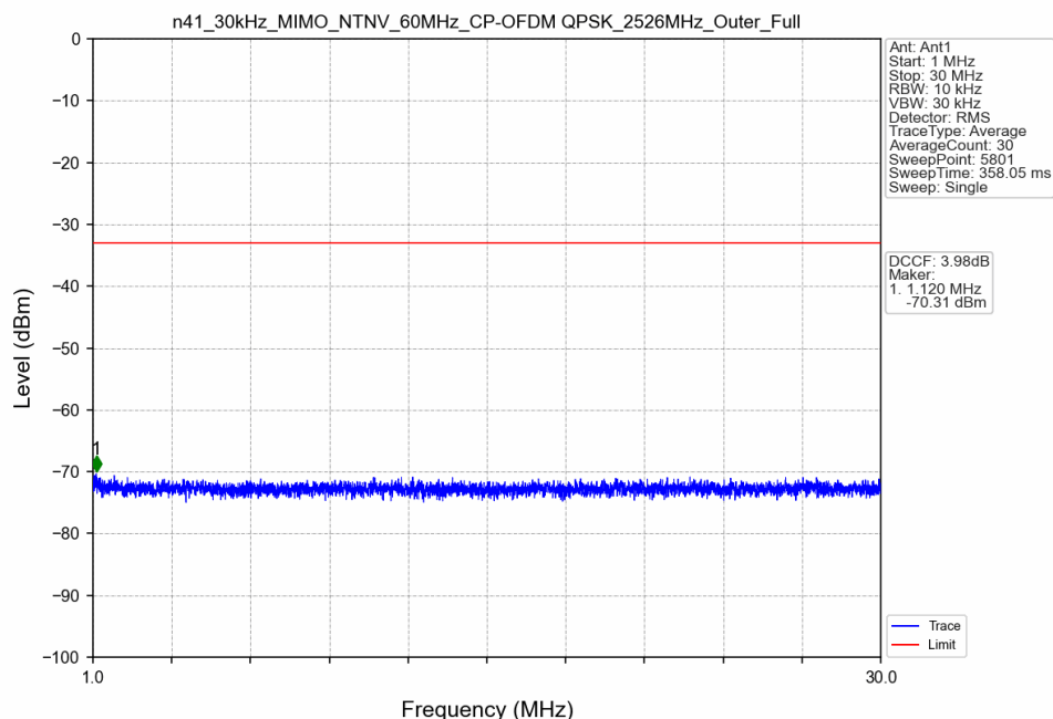
n41_30kHz_MIMO_NTNV_60MHz_CP-OFDM QPSK_2526MHz_Outer_Full
