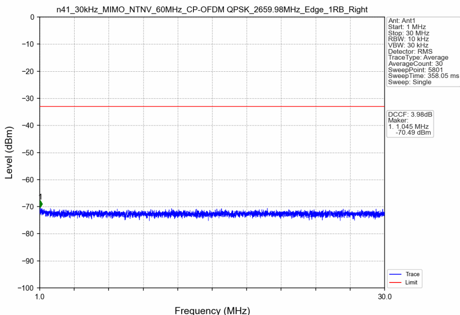
n41_30kHz_MIMO_NTNV_60MHz_CP-OFDM QPSK_2659.98MHz_Edge_1RB_Right
