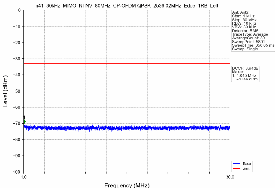
n41_30kHz_MIMO_NTNV_80MHz_CP-OFDM QPSK_2536.02MHz_Edge_1RB_Left
