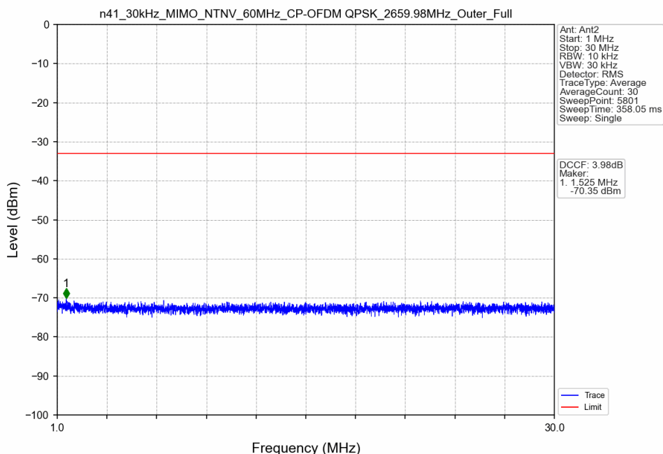
n41_30kHz_MIMO_NTNV_60MHz_CP-OFDM QPSK_2659.98MHz_Outer_Full
