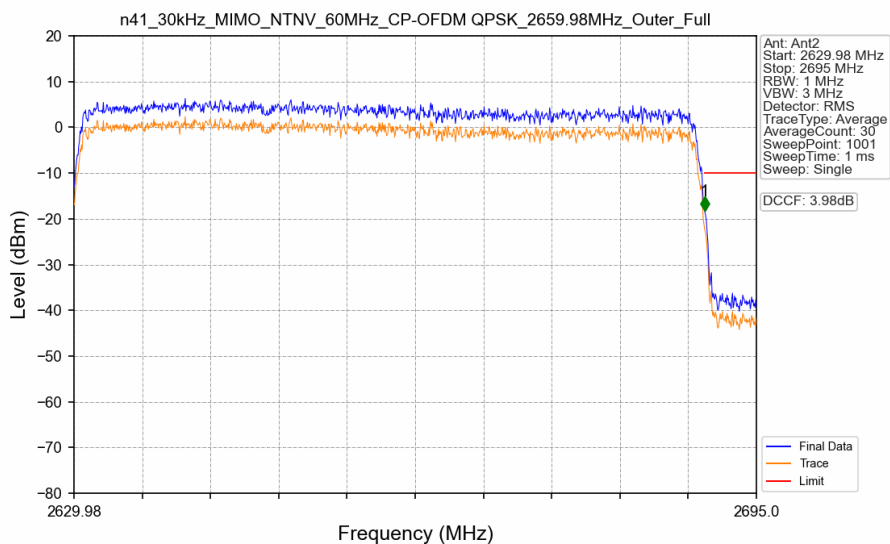
n41_30kHz_MIMO_NTNV_60MHz_CP-OFDM QPSK_2659.98MHz_Outer_Full
