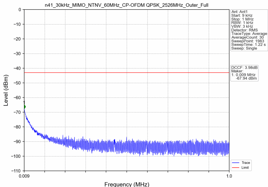
n41_30kHz_MIMO_NTNV_60MHz_CP-OFDM QPSK_2526MHz_Outer_Full
