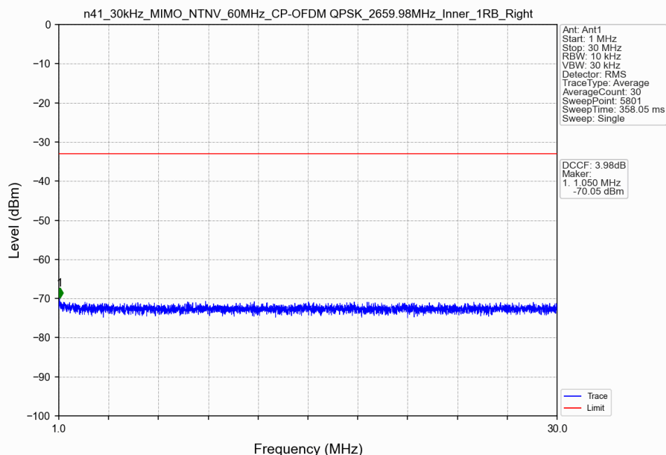
n41_30kHz_MIMO_NTNV_60MHz_CP-OFDM QPSK_2659.98MHz_Inner_1RB_Right
