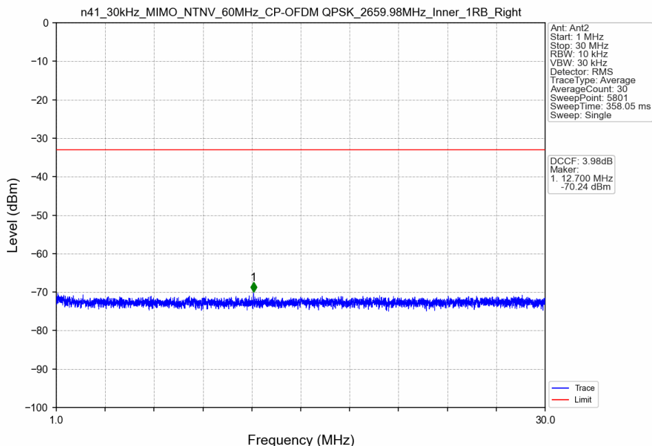
n41_30kHz_MIMO_NTNV_60MHz_CP-OFDM QPSK_2659.98MHz_Inner_1RB_Right
