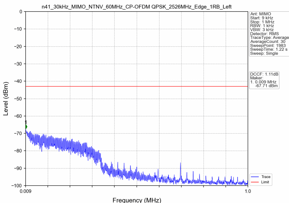
n41_30kHz_MIMO_NTNV_60MHz_CP-OFDM QPSK_2526MHz_Edge_1RB_Left
