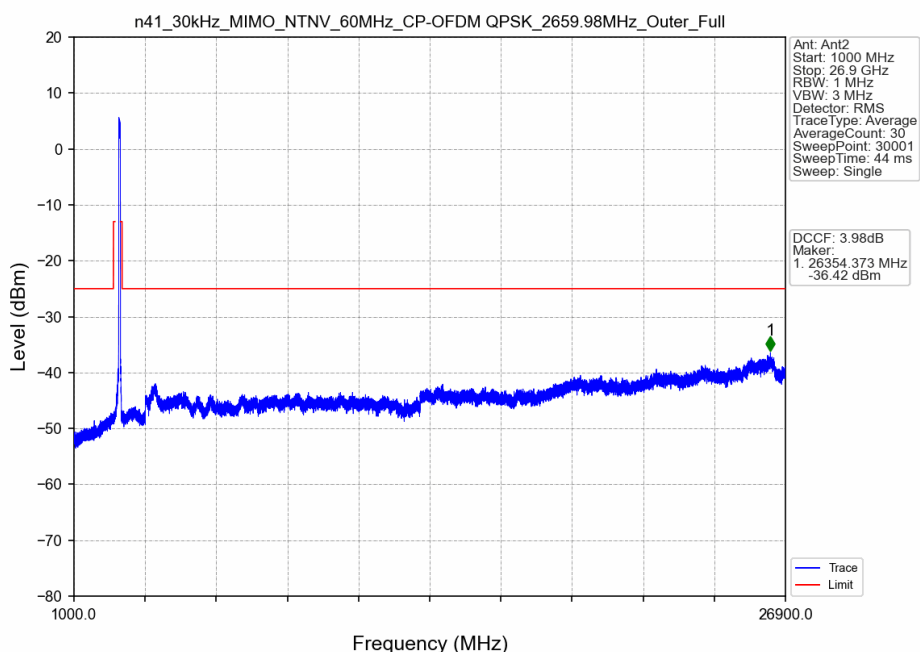
n41_30kHz_MIMO_NTNV_60MHz_CP-OFDM QPSK_2659.98MHz_Outer_Full
