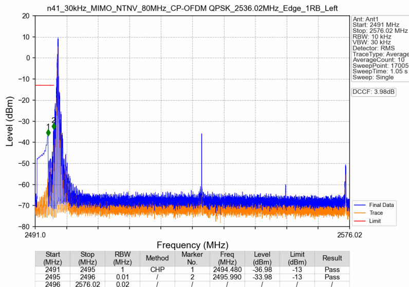
n41_30kHz_MIMO_NTNV_80MHz_CP-OFDM QPSK_2536.02MHz_Edge_1RB_Left
