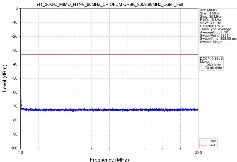
n41_30kHz_MIMO_NTNV_60MHz_CP-OFDM QPSK_2659.98MHz_Outer_Full
