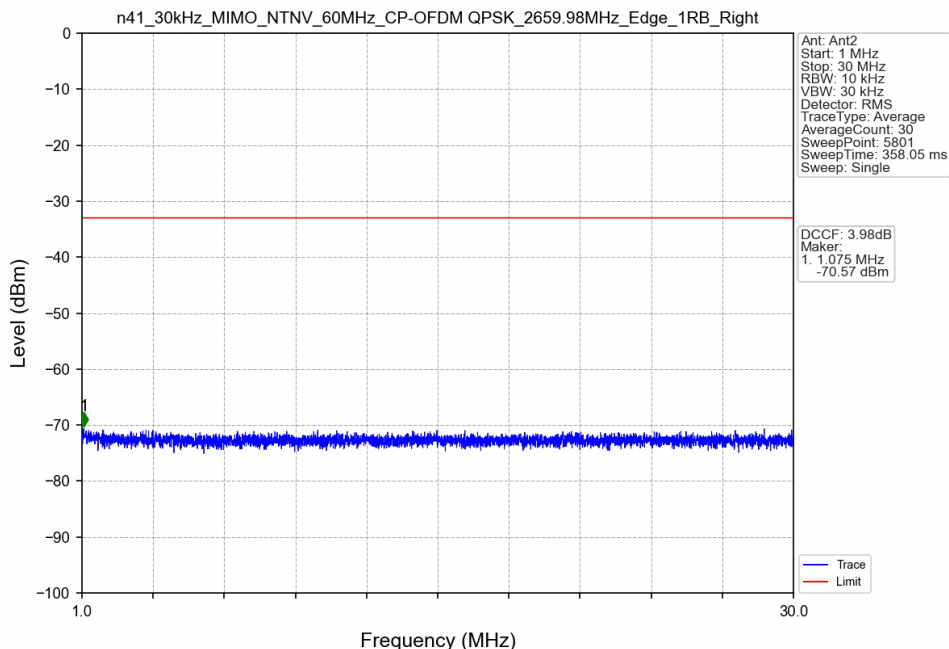
n41_30kHz_MIMO_NTNV_60MHz_CP-OFDM QPSK_2659.98MHz_Edge_1RB_Right
