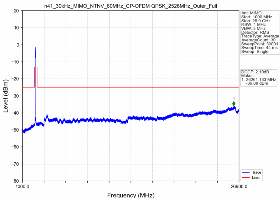
n41_30kHz_MIMO_NTNV_60MHz_CP-OFDM QPSK_2526MHz_Outer_Full
