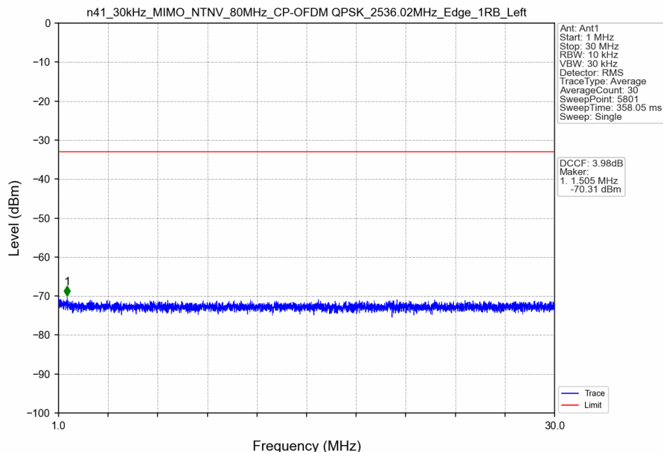
n41_30kHz_MIMO_NTNV_80MHz_CP-OFDM QPSK_2536.02MHz_Edge_1RB_Left
