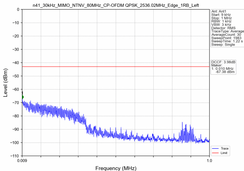
n41_30kHz_MIMO_NTNV_80MHz_CP-OFDM QPSK_2536.02MHz_Edge_1RB_Left
