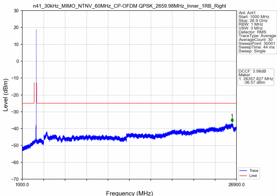
n41_30kHz_MIMO_NTNV_60MHz_CP-OFDM QPSK_2659.98MHz_Inner_1RB_Right
