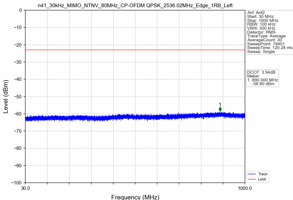
n41_30kHz_MIMO_NTNV_80MHz_CP-OFDM QPSK_2536.02MHz_Edge_1RB_Left
