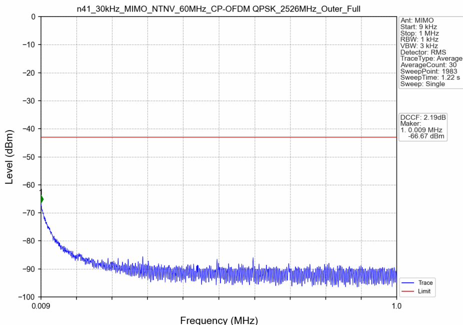
n41_30kHz_MIMO_NTNV_60MHz_CP-OFDM QPSK_2526MHz_Outer_Full
