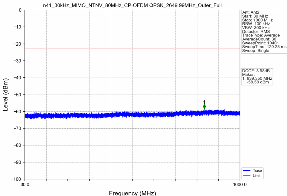
n41_30kHz_MIMO_NTNV_80MHz_CP-OFDM QPSK_2649.99MHz_Outer_Full
