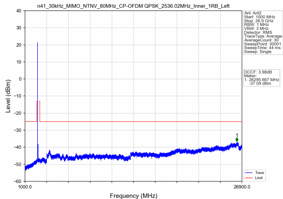
n41_30kHz_MIMO_NTNV_80MHz_CP-OFDM QPSK_2536.02MHz_Inner_1RB_Left
