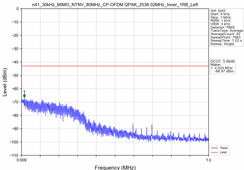
n41_30kHz_MIMO_NTNV_80MHz_CP-OFDM QPSK_2536.02MHz_Inner_1RB_Left
