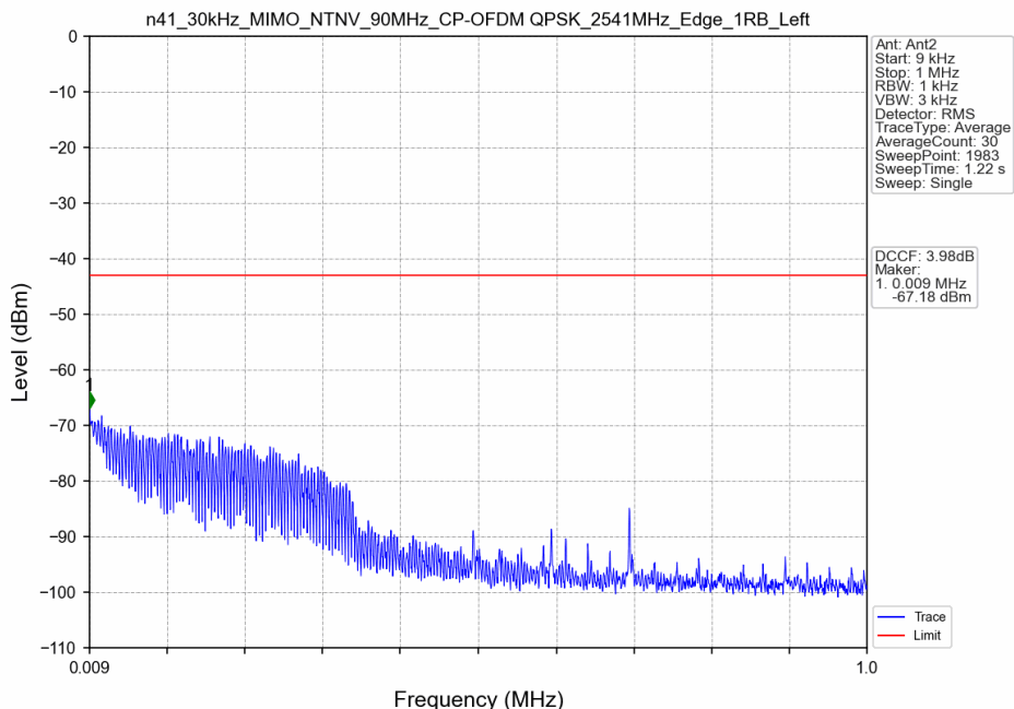
n41_30kHz_MIMO_NTNV_90MHz_CP-OFDM QPSK_2541MHz_Edge_1RB_Left
