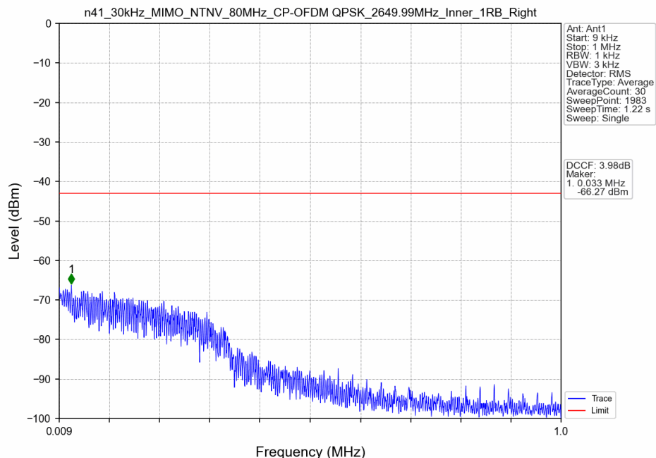
n41_30kHz_MIMO_NTNV_80MHz_CP-OFDM QPSK_2649.99MHz_Inner_1RB_Right
