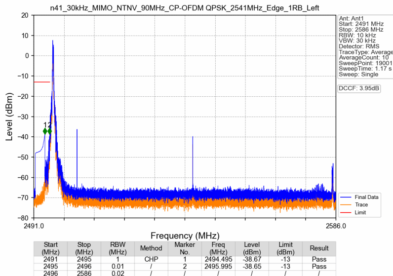
n41_30kHz_MIMO_NTNV_90MHz_CP-OFDM QPSK_2541MHz_Edge_1RB_Left
