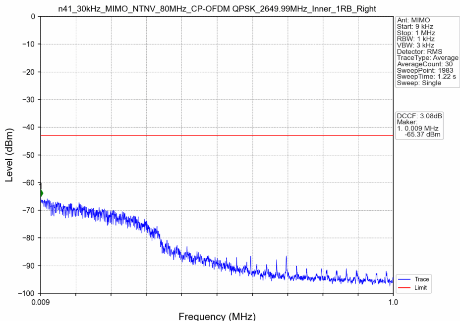
n41_30kHz_MIMO_NTNV_80MHz_CP-OFDM QPSK_2649.99MHz_Inner_1RB_Right
