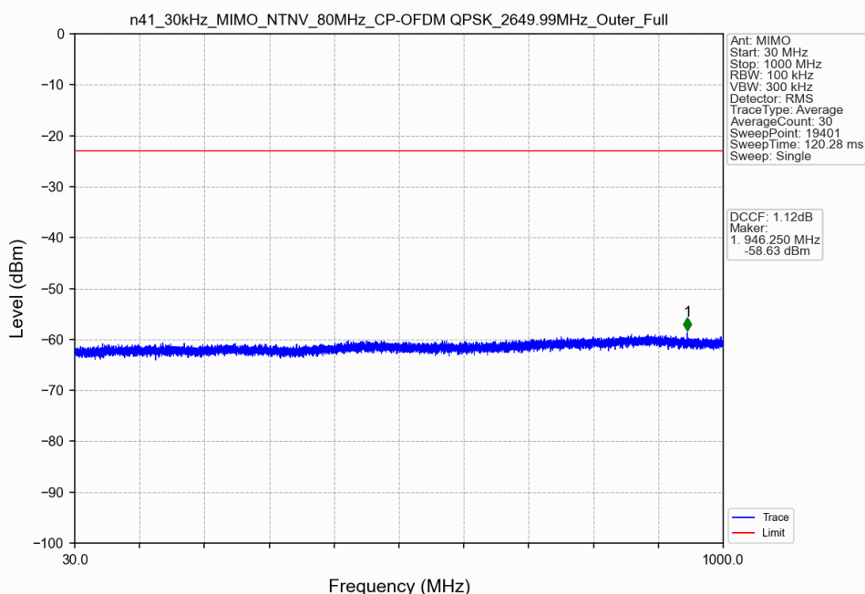
n41_30kHz_MIMO_NTNV_80MHz_CP-OFDM QPSK_2649.99MHz_Outer_Full
