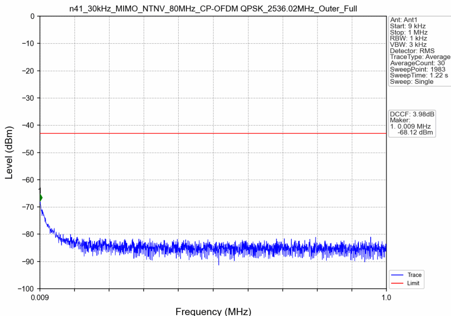
n41_30kHz_MIMO_NTNV_80MHz_CP-OFDM QPSK_2536.02MHz_Outer_Full
