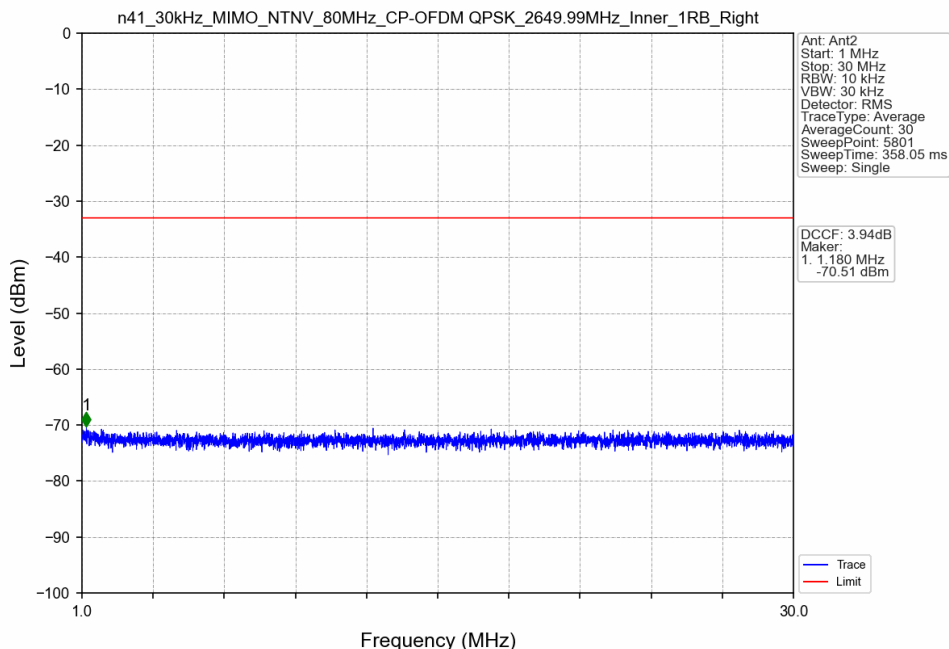
n41_30kHz_MIMO_NTNV_80MHz_CP-OFDM QPSK_2649.99MHz_Inner_1RB_Right
