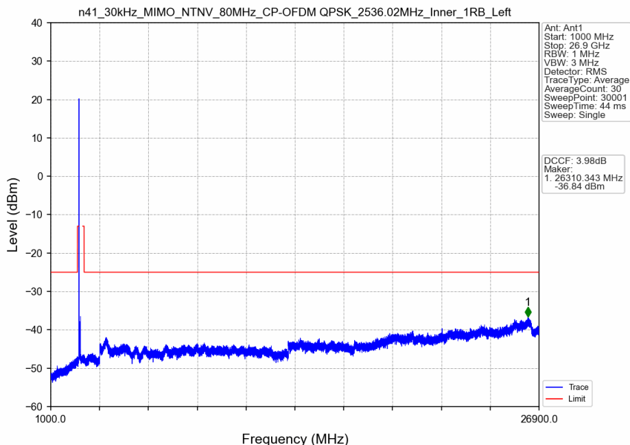
n41_30kHz_MIMO_NTNV_80MHz_CP-OFDM QPSK_2536.02MHz_Inner_1RB_Left
