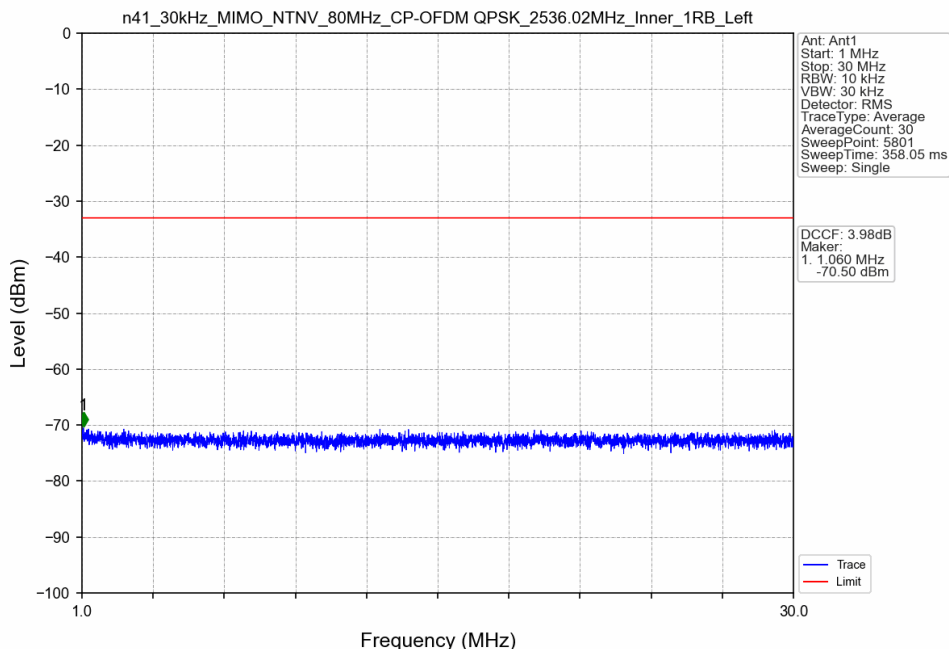
n41_30kHz_MIMO_NTNV_80MHz_CP-OFDM QPSK_2536.02MHz_Inner_1RB_Left
