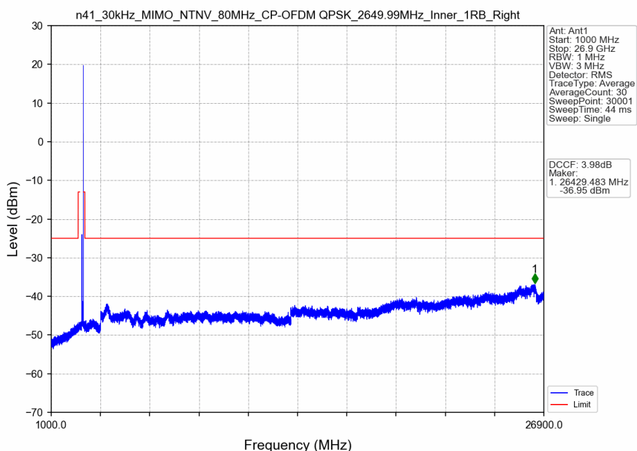
n41_30kHz_MIMO_NTNV_80MHz_CP-OFDM QPSK_2649.99MHz_Inner_1RB_Right
