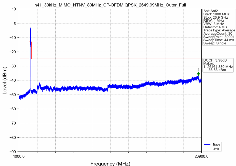
n41_30kHz_MIMO_NTNV_80MHz_CP-OFDM QPSK_2649.99MHz_Outer_Full
