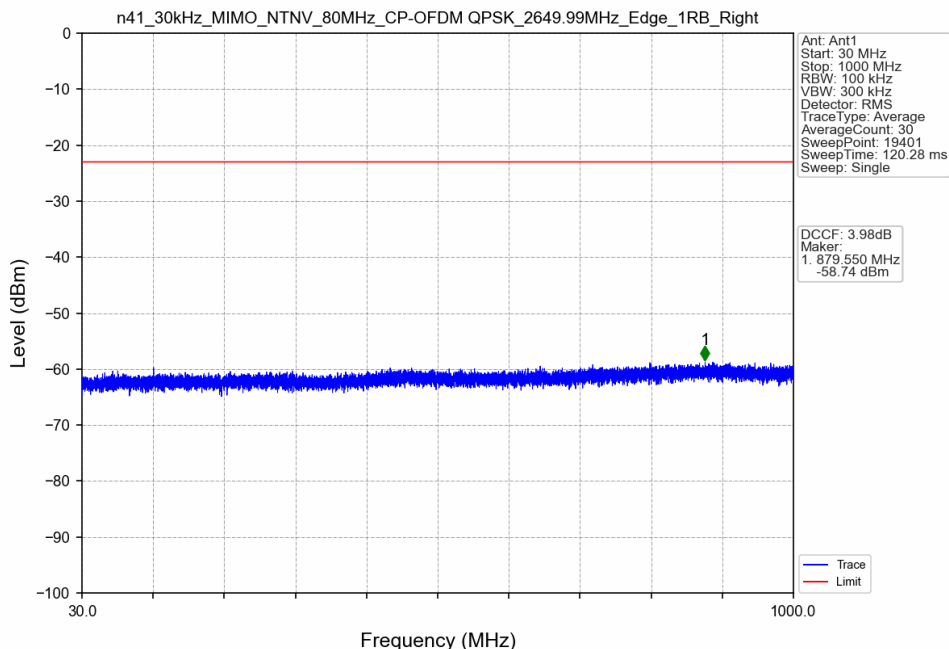
n41_30kHz_MIMO_NTNV_80MHz_CP-OFDM QPSK_2649.99MHz_Edge_1RB_Right
