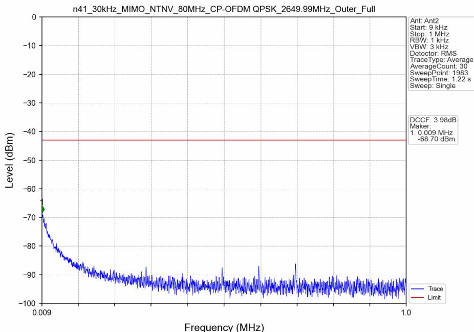
n41_30kHz_MIMO_NTNV_80MHz_CP-OFDM QPSK_2649.99MHz_Outer_Full
