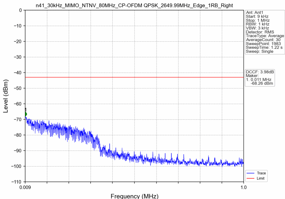
n41_30kHz_MIMO_NTNV_80MHz_CP-OFDM QPSK_2649.99MHz_Edge_1RB_Right
