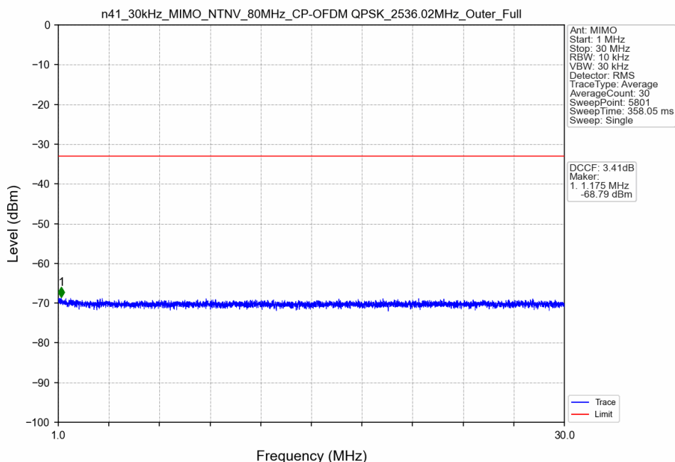
n41_30kHz_MIMO_NTNV_80MHz_CP-OFDM QPSK_2536.02MHz_Outer_Full
