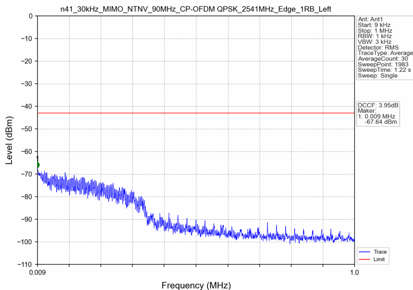
n41_30kHz_MIMO_NTNV_90MHz_CP-OFDM QPSK_2541MHz_Edge_1RB_Left
