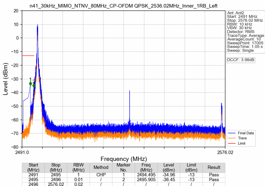
n41_30kHz_MIMO_NTNV_80MHz_CP-OFDM QPSK_2536.02MHz_Inner_1RB_Left
