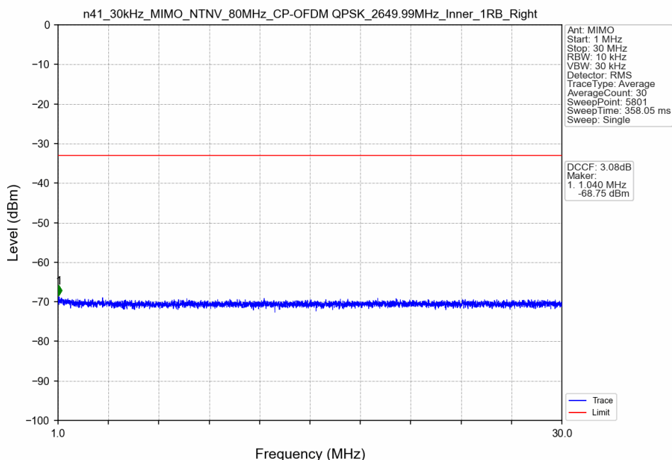
n41_30kHz_MIMO_NTNV_80MHz_CP-OFDM QPSK_2649.99MHz_Inner_1RB_Right
