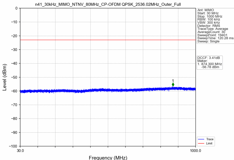
n41_30kHz_MIMO_NTNV_80MHz_CP-OFDM QPSK_2536.02MHz_Outer_Full
