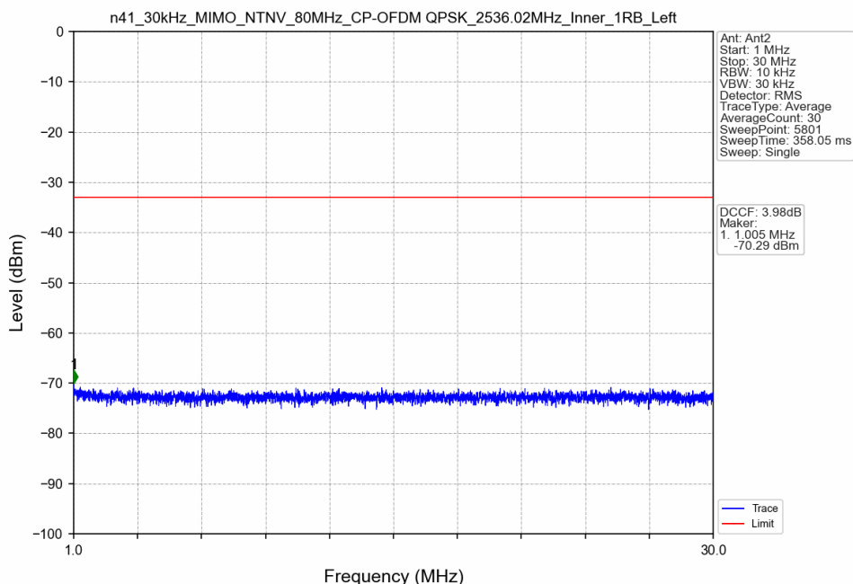
n41_30kHz_MIMO_NTNV_80MHz_CP-OFDM QPSK_2536.02MHz_Inner_1RB_Left
