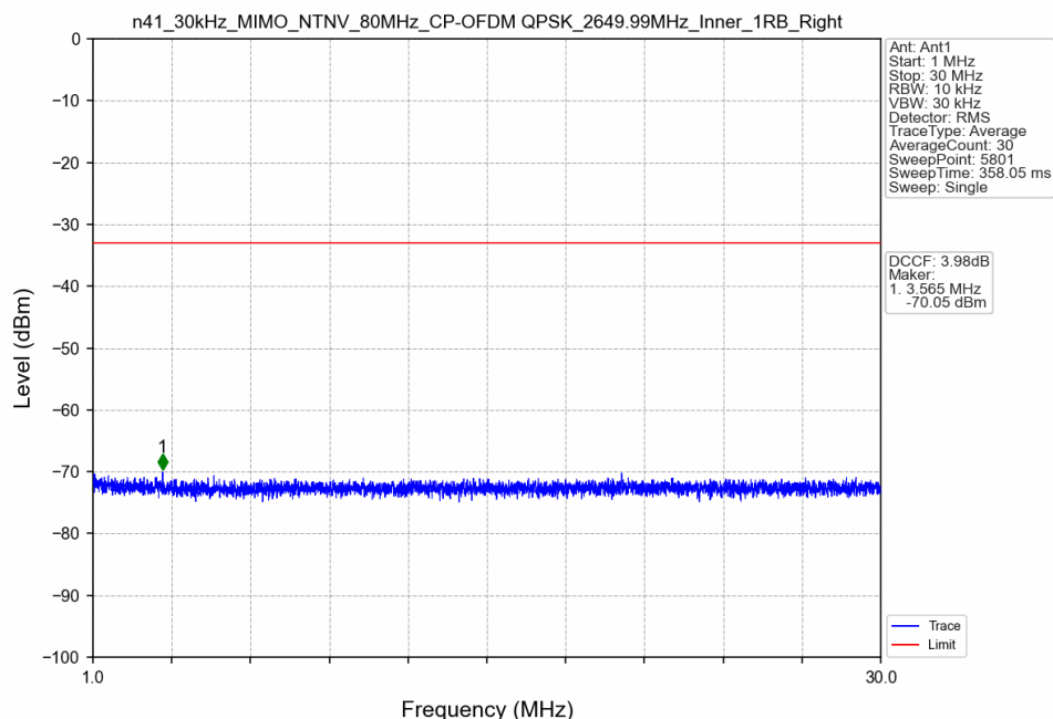
n41_30kHz_MIMO_NTNV_80MHz_CP-OFDM QPSK_2649.99MHz_Inner_1RB_Right
