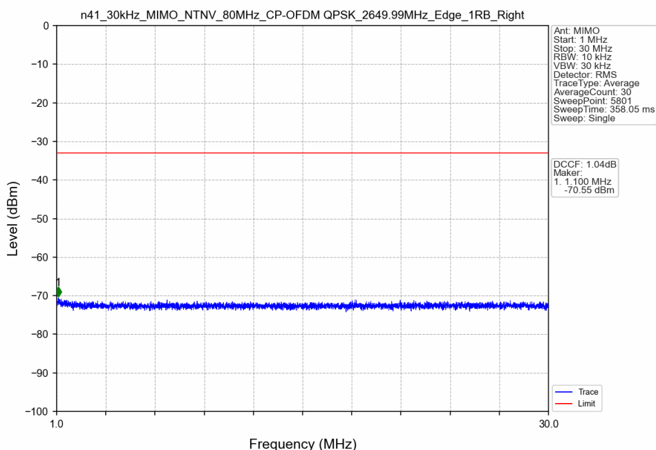
n41_30kHz_MIMO_NTNV_80MHz_CP-OFDM QPSK_2649.99MHz_Edge_1RB_Right
