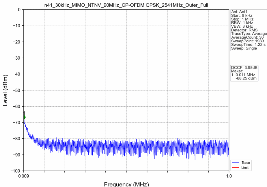
n41_30kHz_MIMO_NTNV_90MHz_CP-OFDM QPSK_2541MHz_Outer_Full
