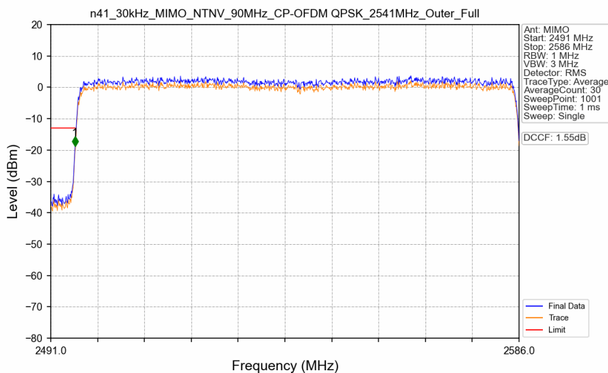
n41_30kHz_MIMO_NTNV_90MHz_CP-OFDM QPSK_2541MHz_Outer_Full
