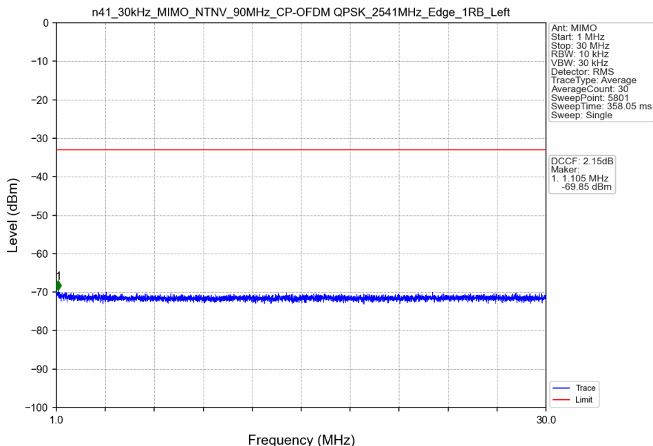
n41_30kHz_MIMO_NTNV_90MHz_CP-OFDM QPSK_2541MHz_Edge_1RB_Left
