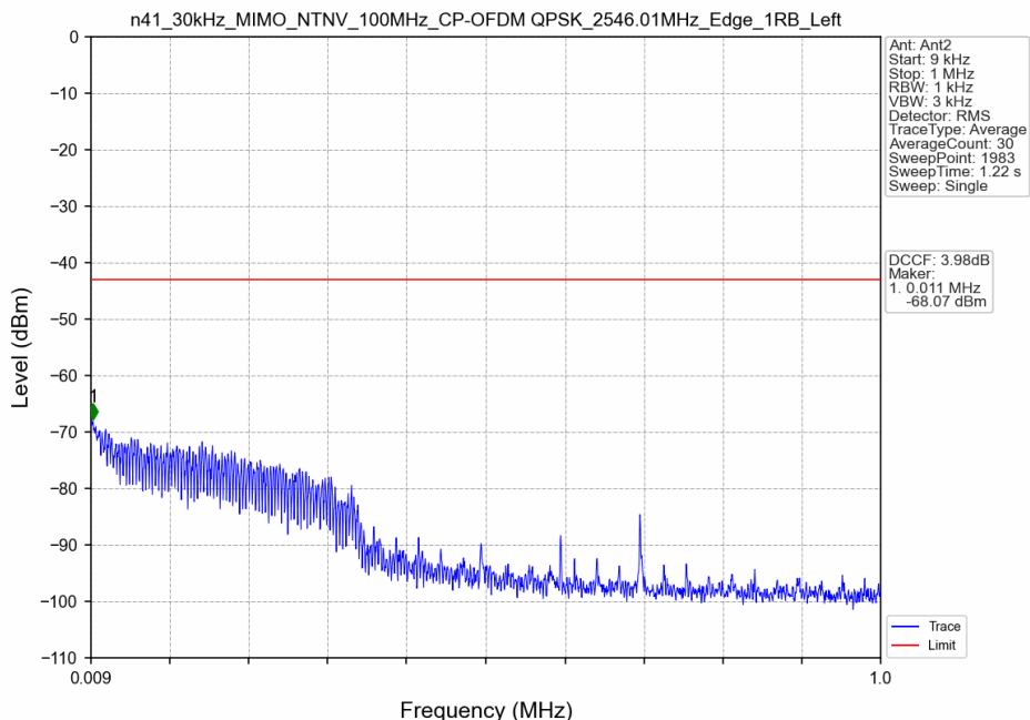
n41_30kHz_MIMO_NTNV_100MHz_CP-OFDM QPSK_2546.01MHz_Edge_1RB_Left
