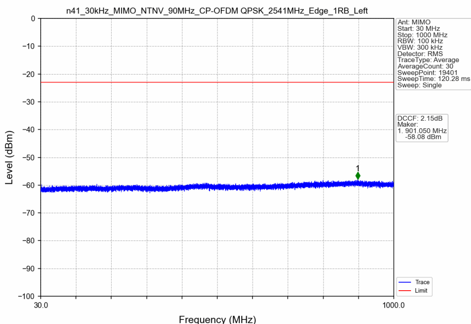
n41_30kHz_MIMO_NTNV_90MHz_CP-OFDM QPSK_2541MHz_Edge_1RB_Left
