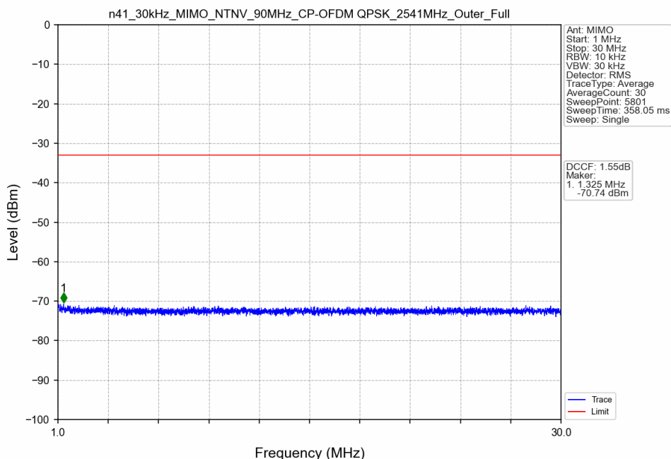
n41_30kHz_MIMO_NTNV_90MHz_CP-OFDM QPSK_2541MHz_Outer_Full
