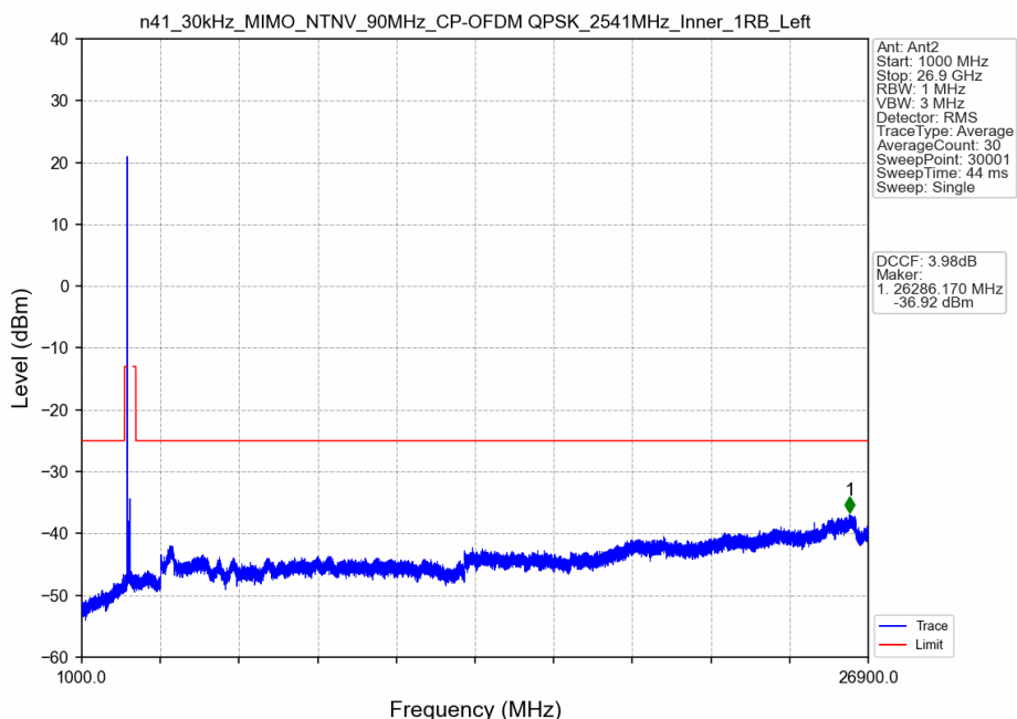
n41_30kHz_MIMO_NTNV_90MHz_CP-OFDM QPSK_2541MHz_Inner_1RB_Left
