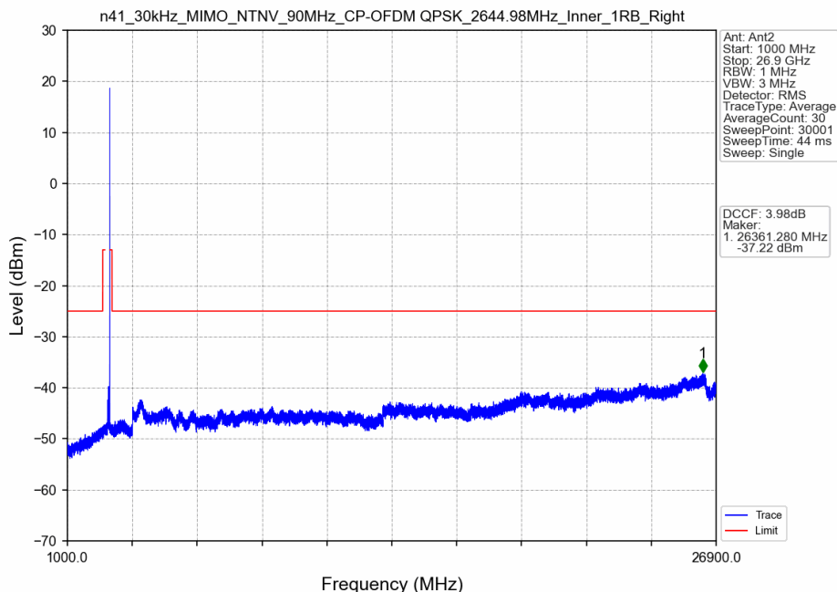
n41_30kHz_MIMO_NTNV_90MHz_CP-OFDM QPSK_2644.98MHz_Inner_1RB_Right
