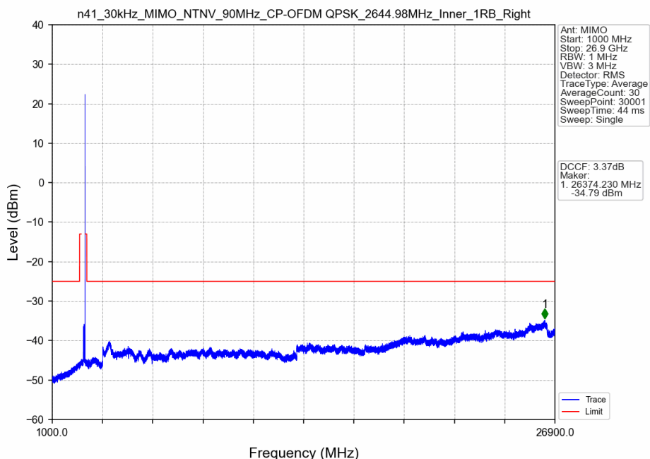
n41_30kHz_MIMO_NTNV_90MHz_CP-OFDM QPSK_2644.98MHz_Inner_1RB_Right
