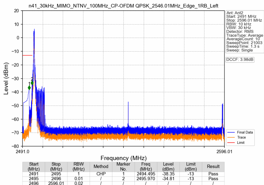
n41_30kHz_MIMO_NTNV_100MHz_CP-OFDM QPSK_2546.01MHz_Edge_1RB_Left
