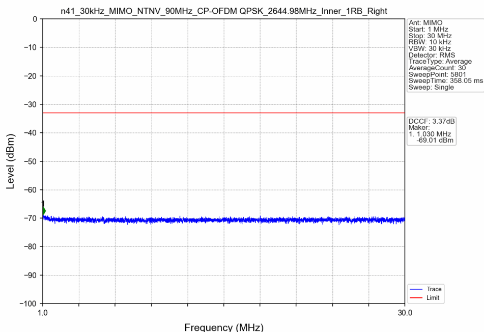
n41_30kHz_MIMO_NTNV_90MHz_CP-OFDM QPSK_2644.98MHz_Inner_1RB_Right
