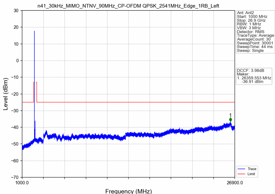
n41_30kHz_MIMO_NTNV_90MHz_CP-OFDM QPSK_2541MHz_Edge_1RB_Left
