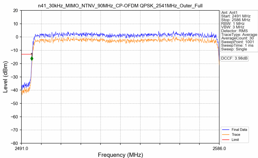
n41_30kHz_MIMO_NTNV_90MHz_CP-OFDM QPSK_2541MHz_Outer_Full
