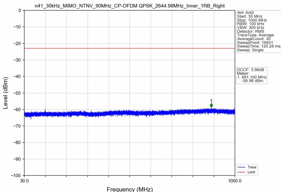
n41_30kHz_MIMO_NTNV_90MHz_CP-OFDM QPSK_2644.98MHz_Inner_1RB_Right
