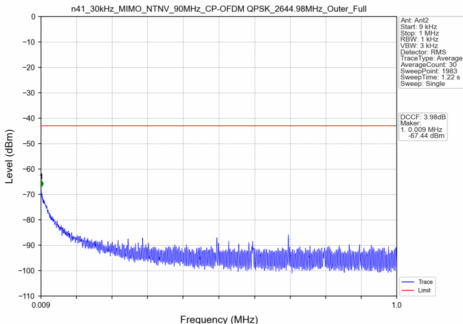
n41_30kHz_MIMO_NTNV_90MHz_CP-OFDM QPSK_2644.98MHz_Outer_Full
