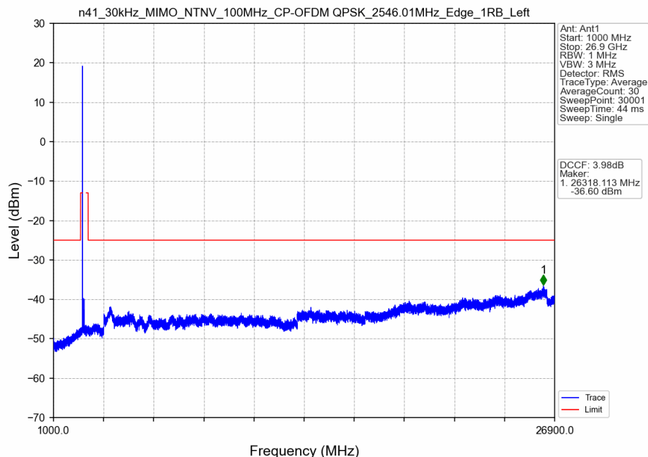
n41_30kHz_MIMO_NTNV_100MHz_CP-OFDM QPSK_2546.01MHz_Edge_1RB_Left
