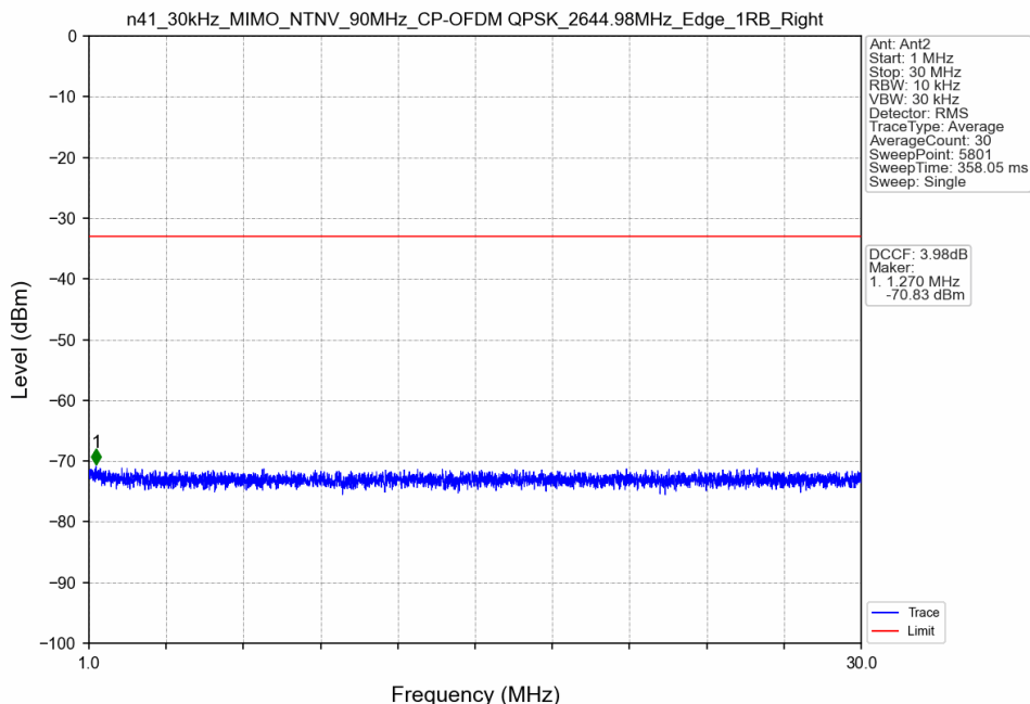
n41_30kHz_MIMO_NTNV_90MHz_CP-OFDM QPSK_2644.98MHz_Edge_1RB_Right
