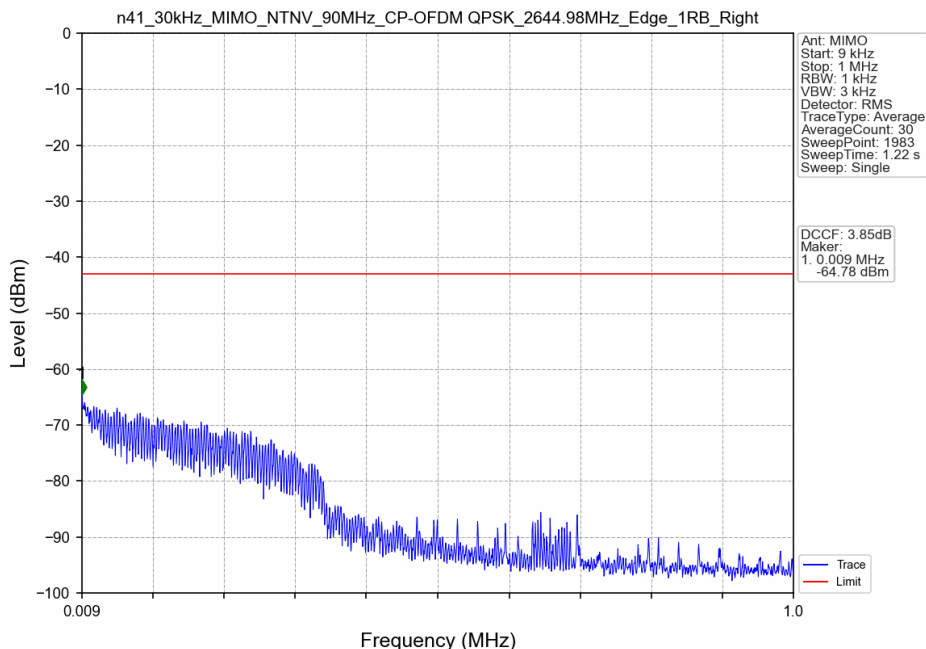
n41_30kHz_MIMO_NTNV_90MHz_CP-OFDM QPSK_2644.98MHz_Edge_1RB_Right
