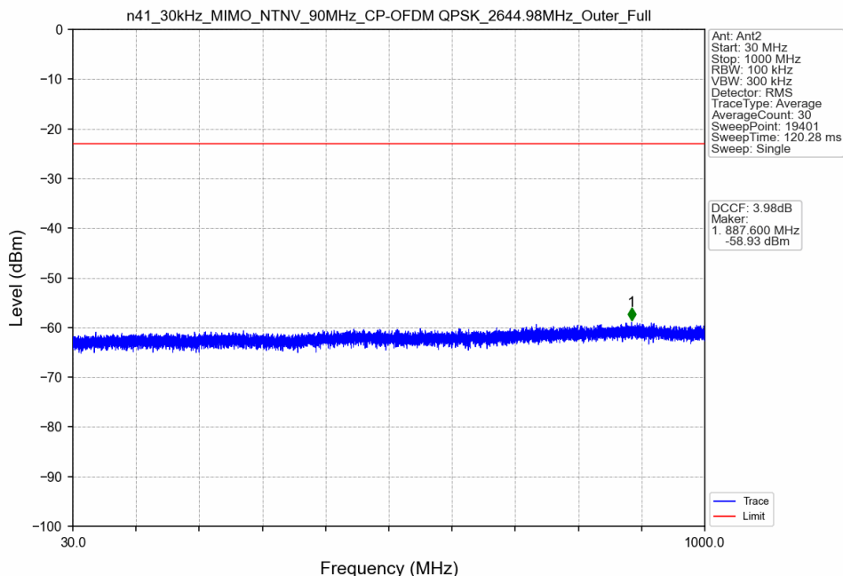
n41_30kHz_MIMO_NTNV_90MHz_CP-OFDM QPSK_2644.98MHz_Outer_Full
