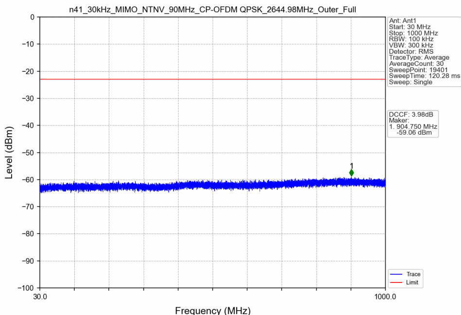
n41_30kHz_MIMO_NTNV_90MHz_CP-OFDM QPSK_2644.98MHz_Outer_Full
