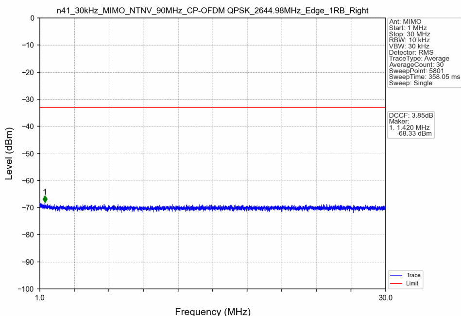
n41_30kHz_MIMO_NTNV_90MHz_CP-OFDM QPSK_2644.98MHz_Edge_1RB_Right
