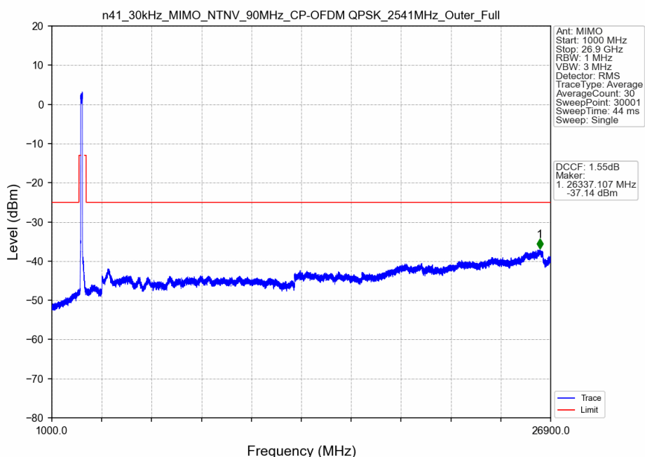
n41_30kHz_MIMO_NTNV_90MHz_CP-OFDM QPSK_2541MHz_Outer_Full
