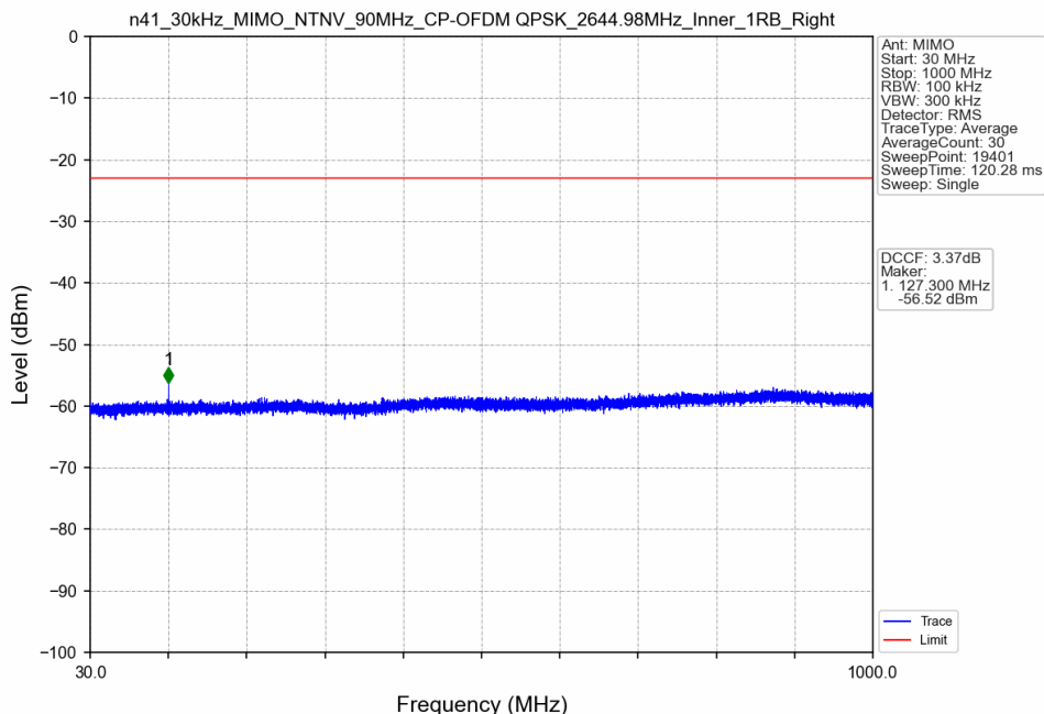
n41_30kHz_MIMO_NTNV_90MHz_CP-OFDM QPSK_2644.98MHz_Inner_1RB_Right
