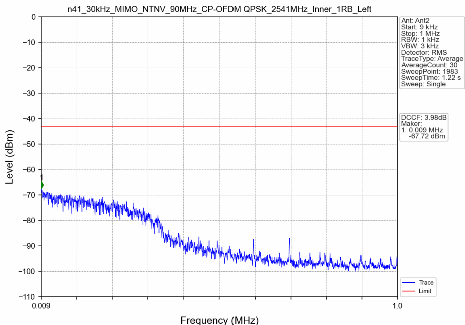
n41_30kHz_MIMO_NTNV_90MHz_CP-OFDM QPSK_2541MHz_Inner_1RB_Left
