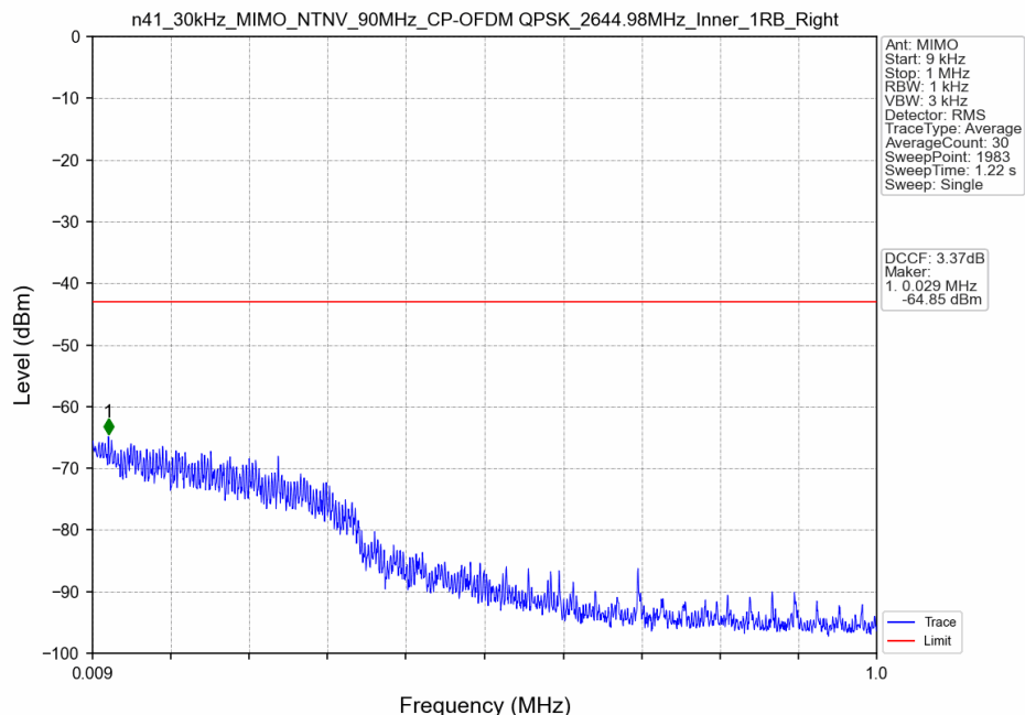
n41_30kHz_MIMO_NTNV_90MHz_CP-OFDM QPSK_2644.98MHz_Inner_1RB_Right
