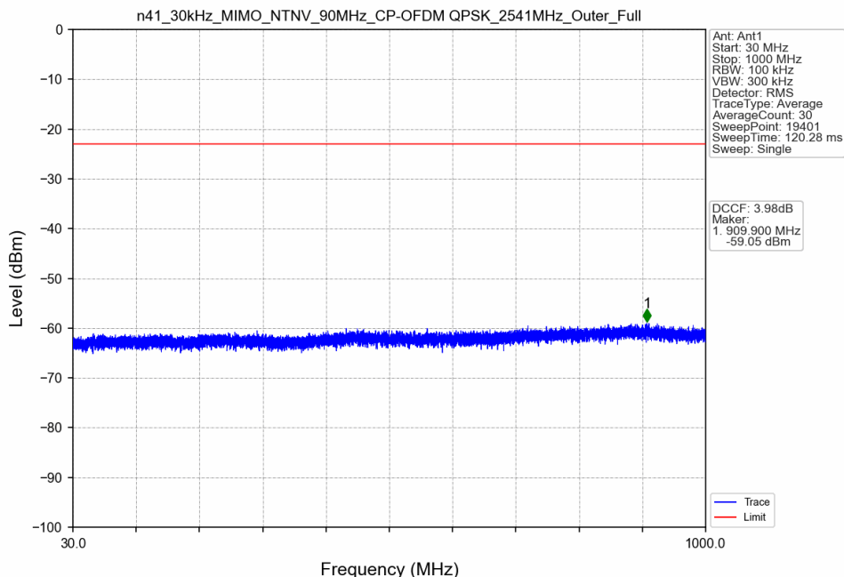
n41_30kHz_MIMO_NTNV_90MHz_CP-OFDM QPSK_2541MHz_Outer_Full
