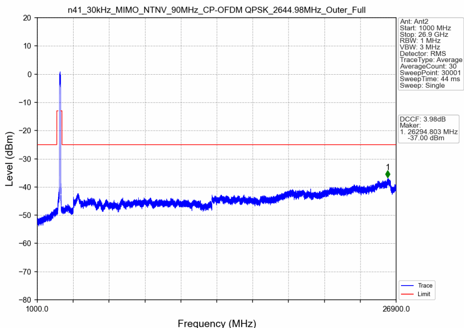
n41_30kHz_MIMO_NTNV_90MHz_CP-OFDM QPSK_2644.98MHz_Outer_Full
