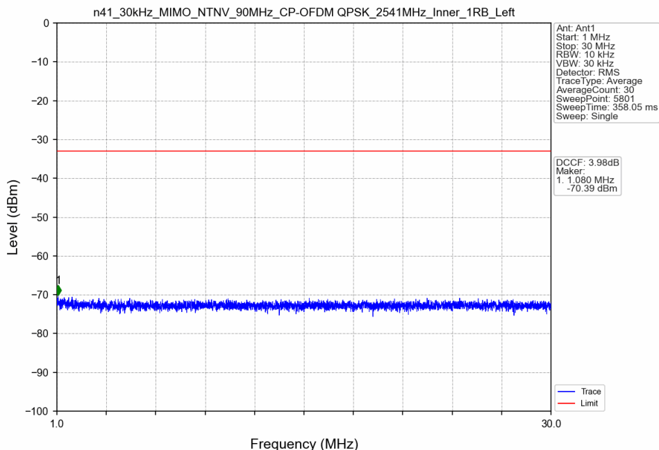
n41_30kHz_MIMO_NTNV_90MHz_CP-OFDM QPSK_2541MHz_Inner_1RB_Left
