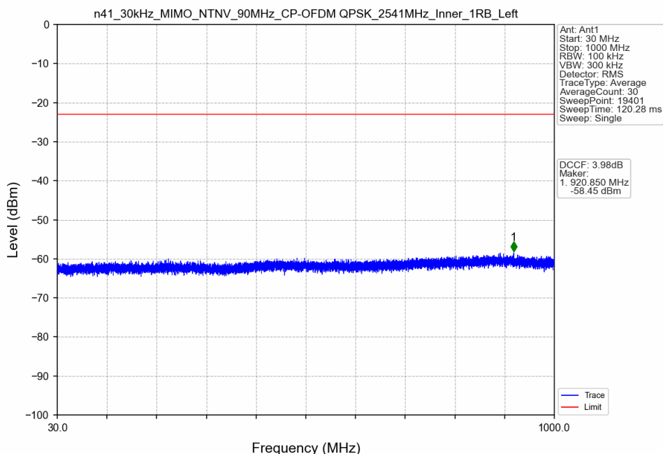
n41_30kHz_MIMO_NTNV_90MHz_CP-OFDM QPSK_2541MHz_Inner_1RB_Left
