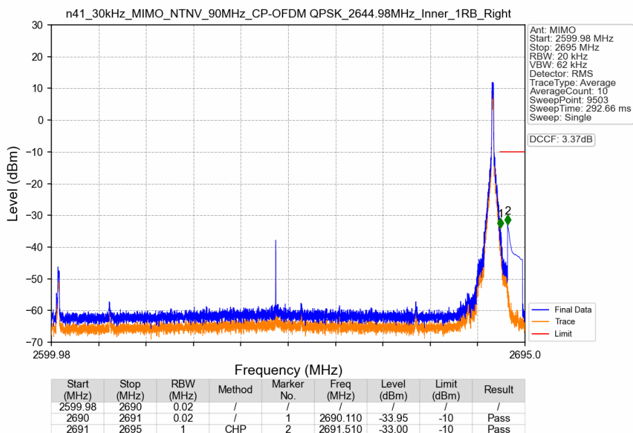
n41_30kHz_MIMO_NTNV_90MHz_CP-OFDM QPSK_2644.98MHz_Inner_1RB_Right
