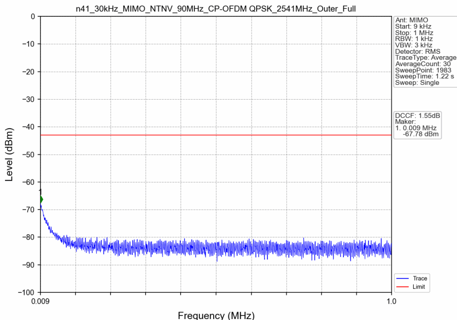
n41_30kHz_MIMO_NTNV_90MHz_CP-OFDM QPSK_2541MHz_Outer_Full
