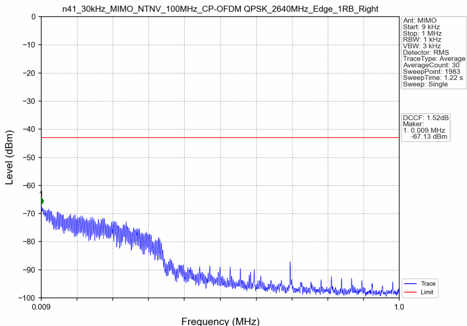
n41_30kHz_MIMO_NTNV_100MHz_CP-OFDM QPSK_2640MHz_Edge_1RB_Right
