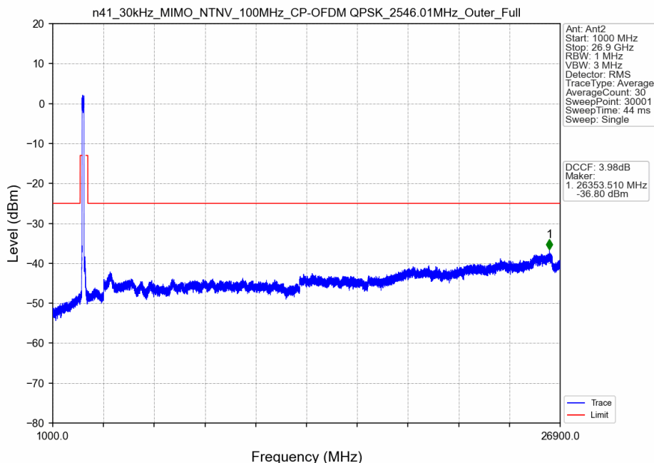
n41_30kHz_MIMO_NTNV_100MHz_CP-OFDM QPSK_2546.01MHz_Outer_Full
