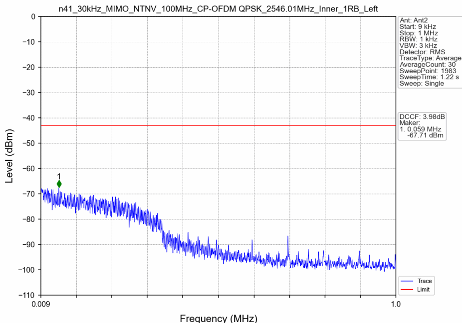
n41_30kHz_MIMO_NTNV_100MHz_CP-OFDM QPSK_2546.01MHz_Inner_1RB_Left
