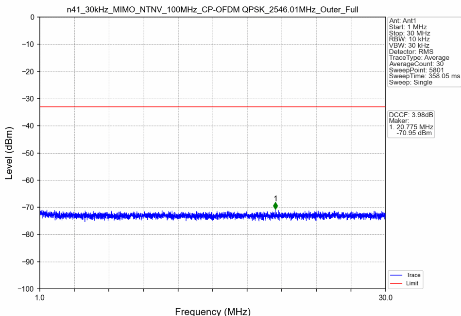
n41_30kHz_MIMO_NTNV_100MHz_CP-OFDM QPSK_2546.01MHz_Outer_Full
