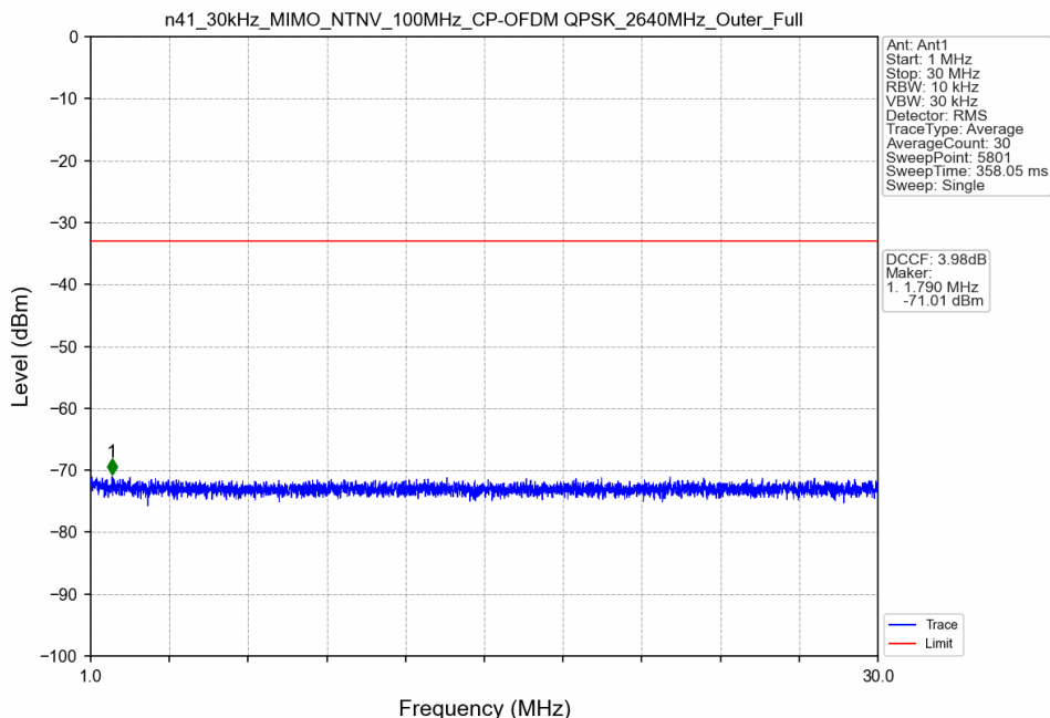
n41_30kHz_MIMO_NTNV_100MHz_CP-OFDM QPSK_2640MHz_Outer_Full
