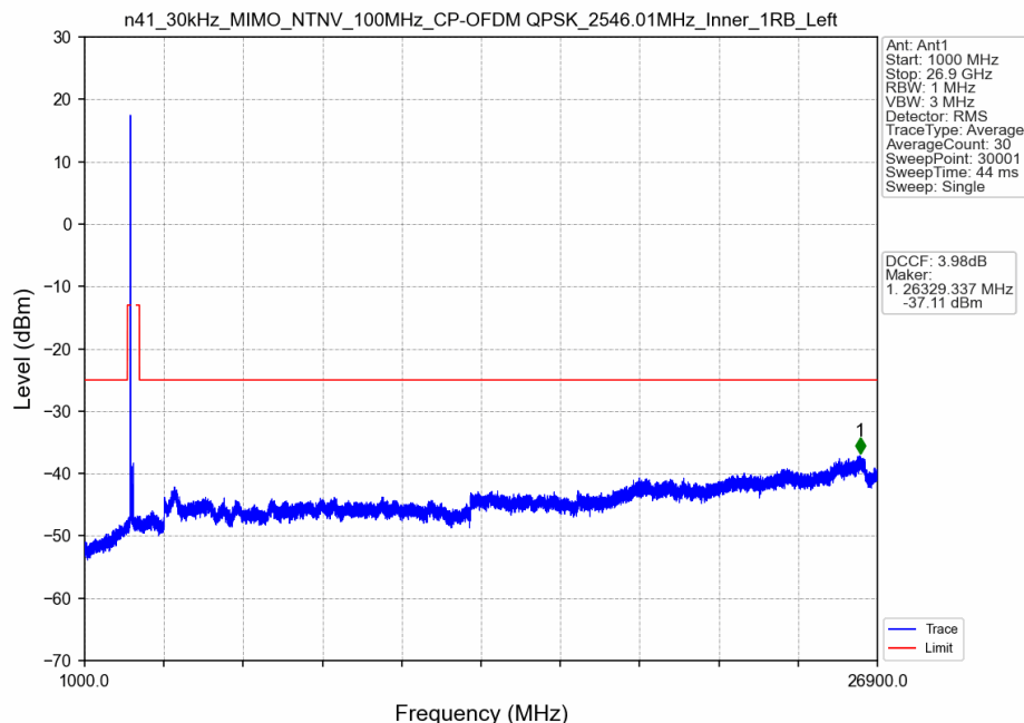
n41_30kHz_MIMO_NTNV_100MHz_CP-OFDM QPSK_2546.01MHz_Inner_1RB_Left
