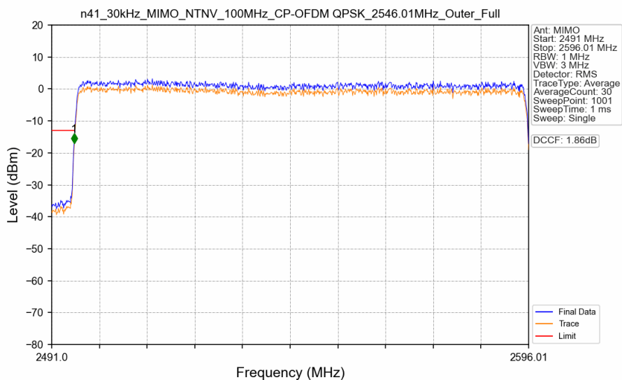
n41_30kHz_MIMO_NTNV_100MHz_CP-OFDM QPSK_2546.01MHz_Outer_Full
