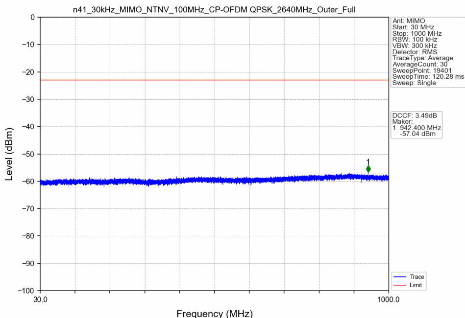
n41_30kHz_MIMO_NTNV_100MHz_CP-OFDM QPSK_2640MHz_Outer_Full
