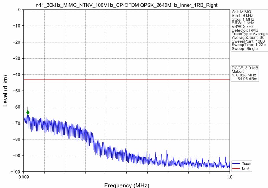
n41_30kHz_MIMO_NTNV_100MHz_CP-OFDM QPSK_2640MHz_Inner_1RB_Right
