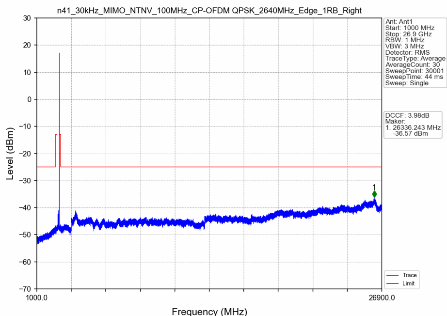
n41_30kHz_MIMO_NTNV_100MHz_CP-OFDM QPSK_2640MHz_Edge_1RB_Right
