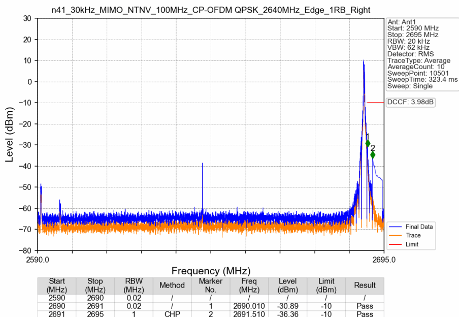
n41_30kHz_MIMO_NTNV_100MHz_CP-OFDM QPSK_2640MHz_Edge_1RB_Right
