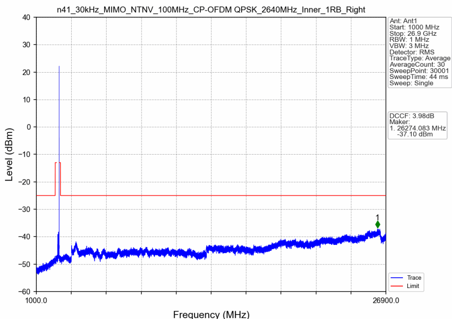
n41_30kHz_MIMO_NTNV_100MHz_CP-OFDM QPSK_2640MHz_Inner_1RB_Right
