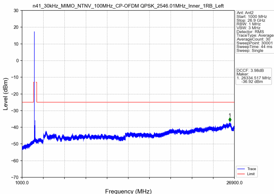
n41_30kHz_MIMO_NTNV_100MHz_CP-OFDM QPSK_2546.01MHz_Inner_1RB_Left
