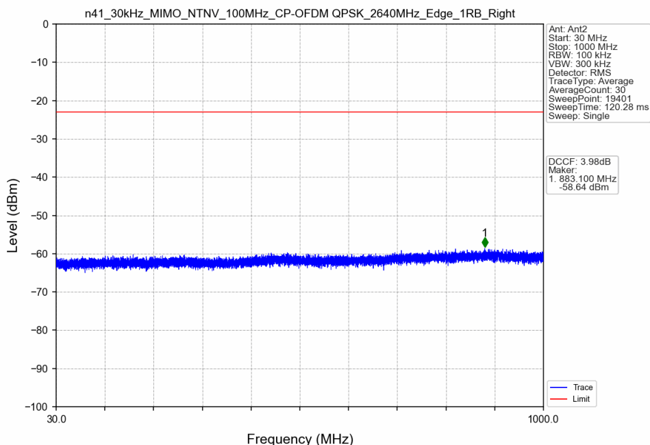
n41_30kHz_MIMO_NTNV_100MHz_CP-OFDM QPSK_2640MHz_Edge_1RB_Right
