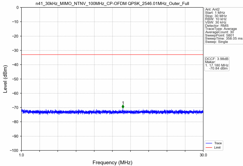
n41_30kHz_MIMO_NTNV_100MHz_CP-OFDM QPSK_2546.01MHz_Outer_Full
