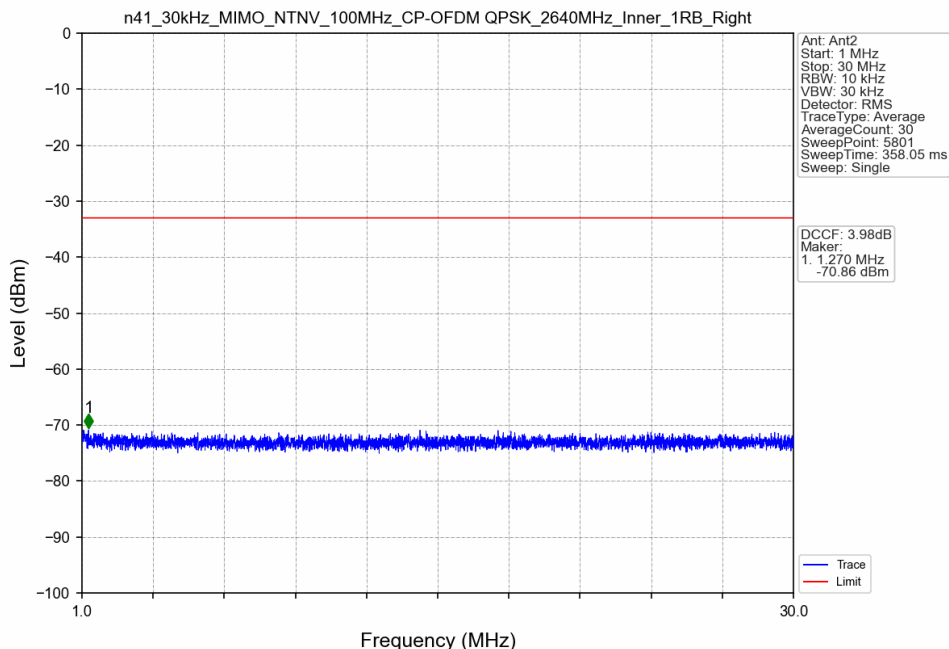
n41_30kHz_MIMO_NTNV_100MHz_CP-OFDM QPSK_2640MHz_Inner_1RB_Right
