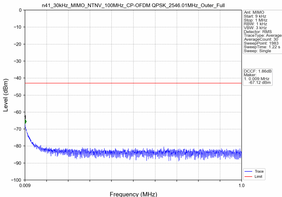
n41_30kHz_MIMO_NTNV_100MHz_CP-OFDM QPSK_2546.01MHz_Outer_Full
