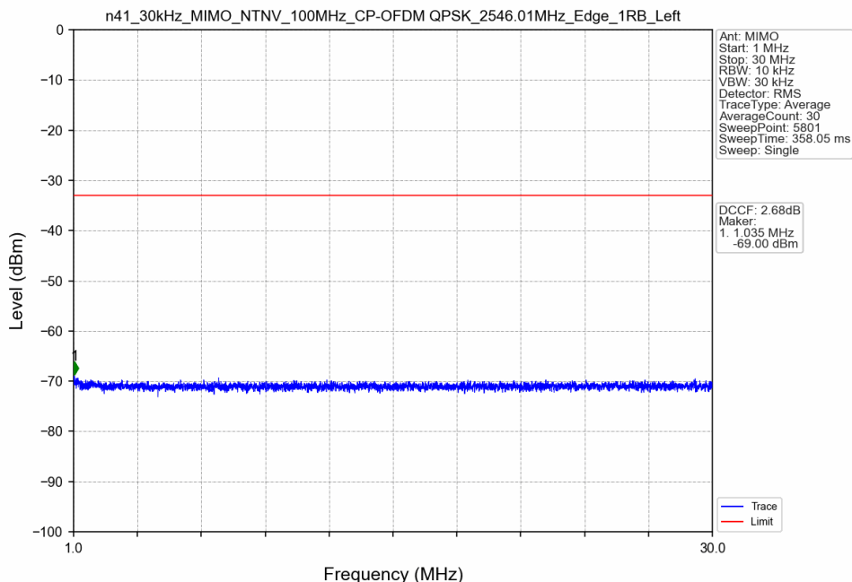
n41_30kHz_MIMO_NTNV_100MHz_CP-OFDM QPSK_2546.01MHz_Edge_1RB_Left
