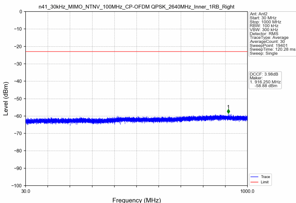
n41_30kHz_MIMO_NTNV_100MHz_CP-OFDM QPSK_2640MHz_Inner_1RB_Right
