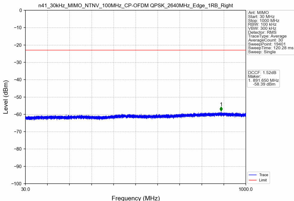
n41_30kHz_MIMO_NTNV_100MHz_CP-OFDM QPSK_2640MHz_Edge_1RB_Right
