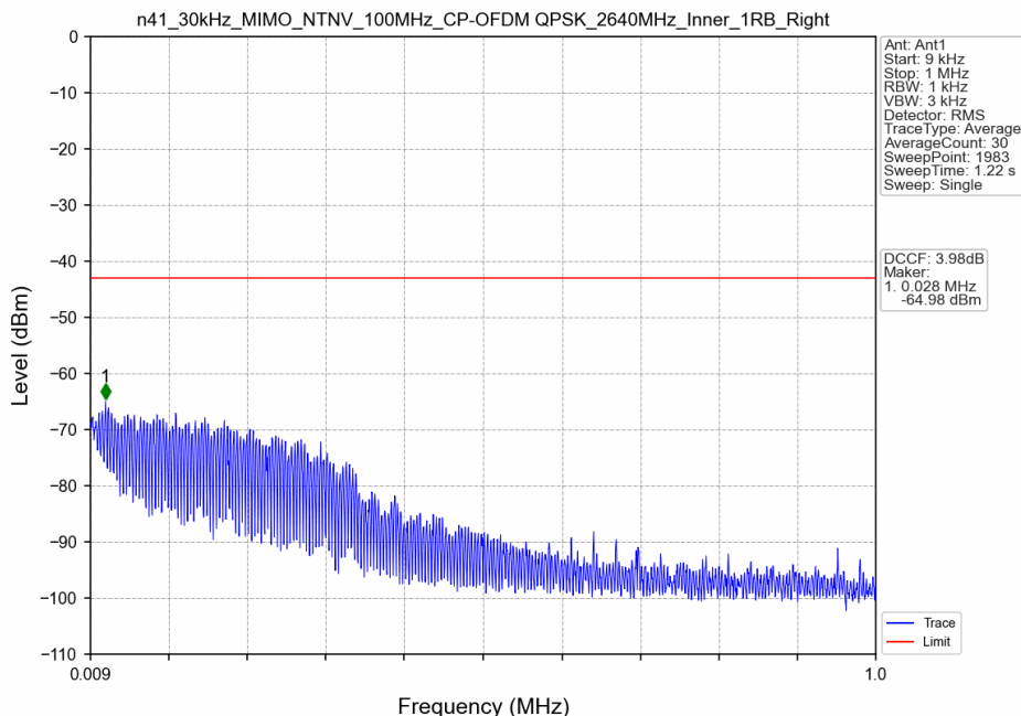
n41_30kHz_MIMO_NTNV_100MHz_CP-OFDM QPSK_2640MHz_Inner_1RB_Right
