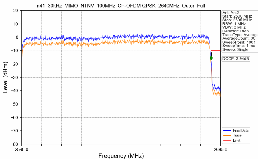
n41_30kHz_MIMO_NTNV_100MHz_CP-OFDM QPSK_2640MHz_Outer_Full
