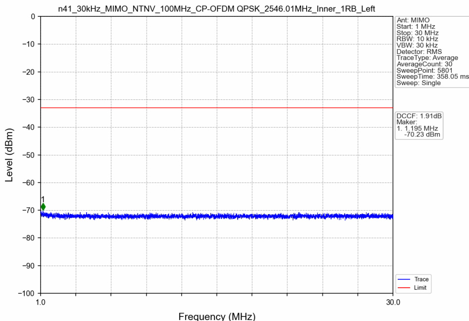
n41_30kHz_MIMO_NTNV_100MHz_CP-OFDM QPSK_2546.01MHz_Inner_1RB_Left
