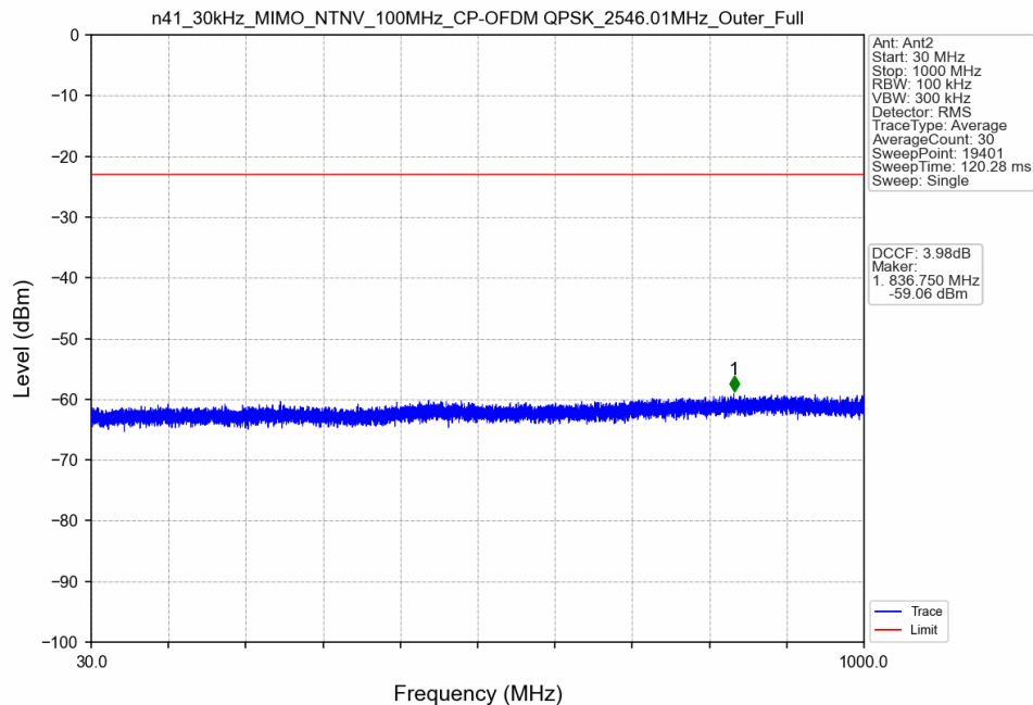
n41_30kHz_MIMO_NTNV_100MHz_CP-OFDM QPSK_2546.01MHz_Outer_Full
