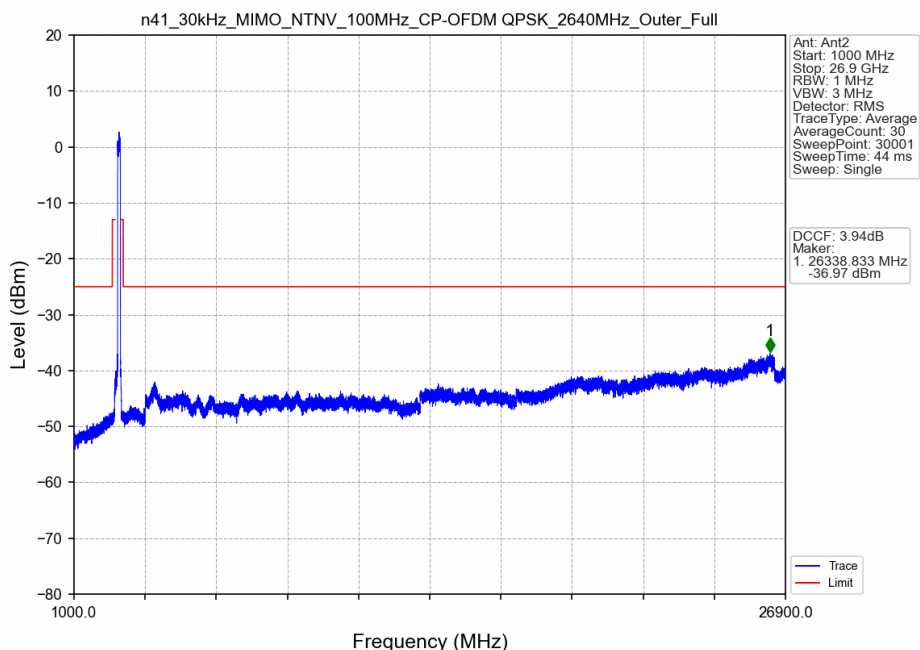
n41_30kHz_MIMO_NTNV_100MHz_CP-OFDM QPSK_2640MHz_Outer_Full
