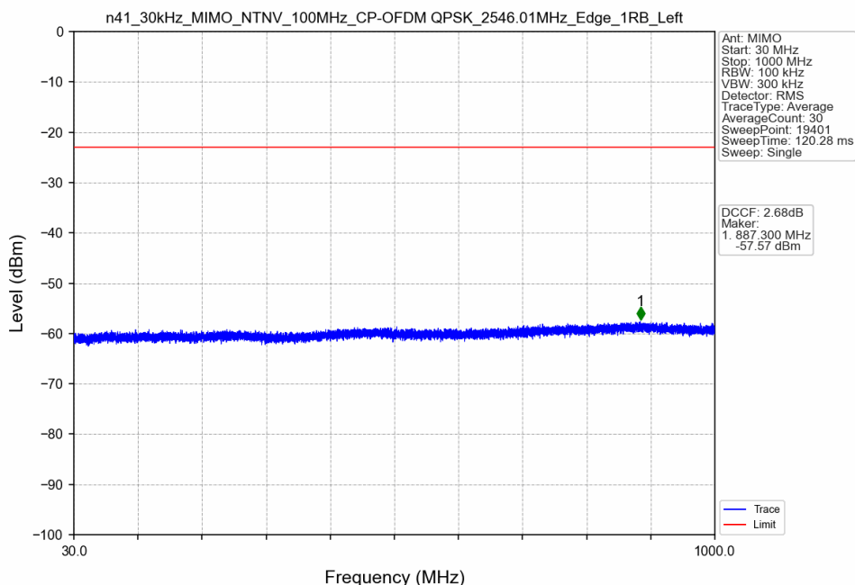
n41_30kHz_MIMO_NTNV_100MHz_CP-OFDM QPSK_2546.01MHz_Edge_1RB_Left
