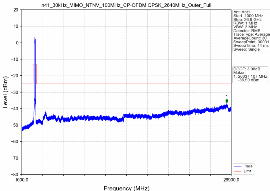
n41_30kHz_MIMO_NTNV_100MHz_CP-OFDM QPSK_2640MHz_Outer_Full
