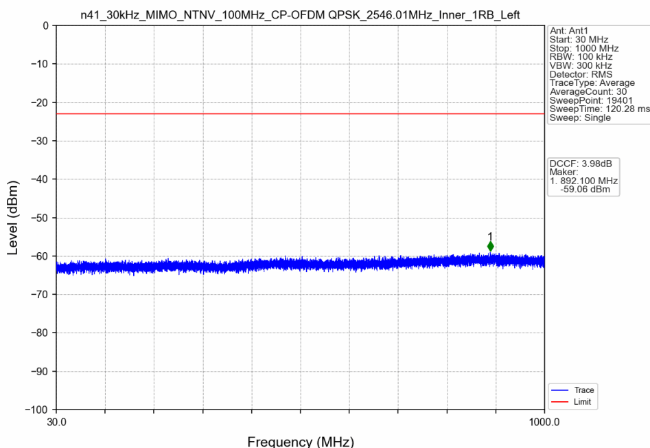
n41_30kHz_MIMO_NTNV_100MHz_CP-OFDM QPSK_2546.01MHz_Inner_1RB_Left
