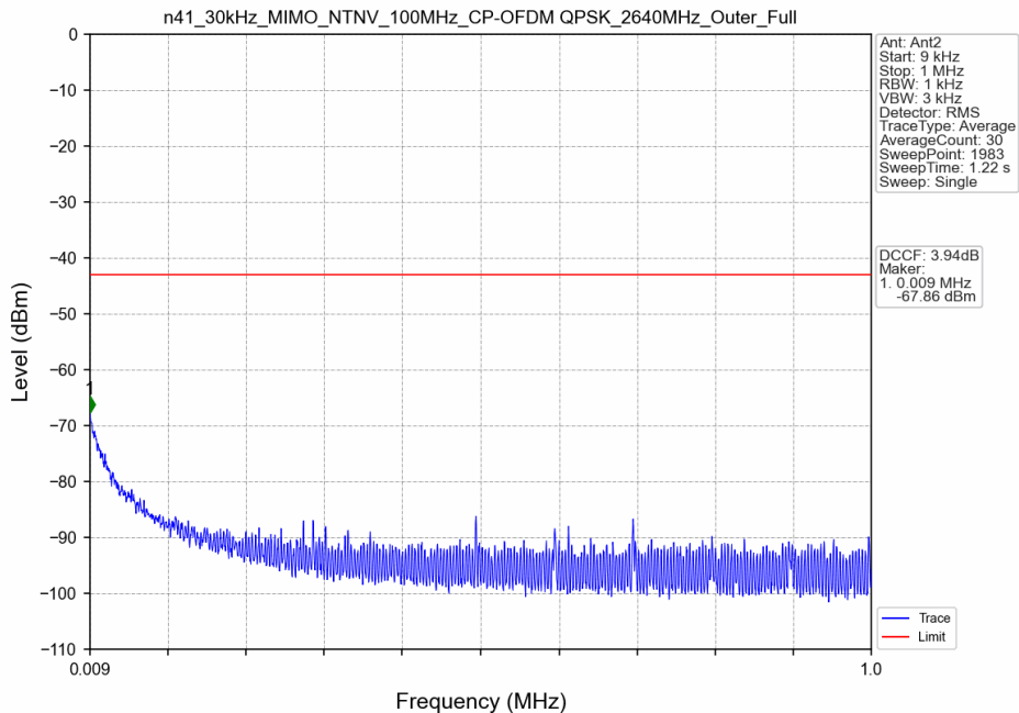
n41_30kHz_MIMO_NTNV_100MHz_CP-OFDM QPSK_2640MHz_Outer_Full
