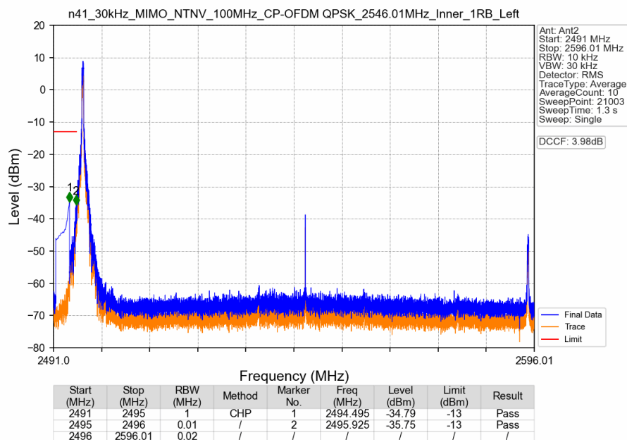
n41_30kHz_MIMO_NTNV_100MHz_CP-OFDM QPSK_2546.01MHz_Inner_1RB_Left
