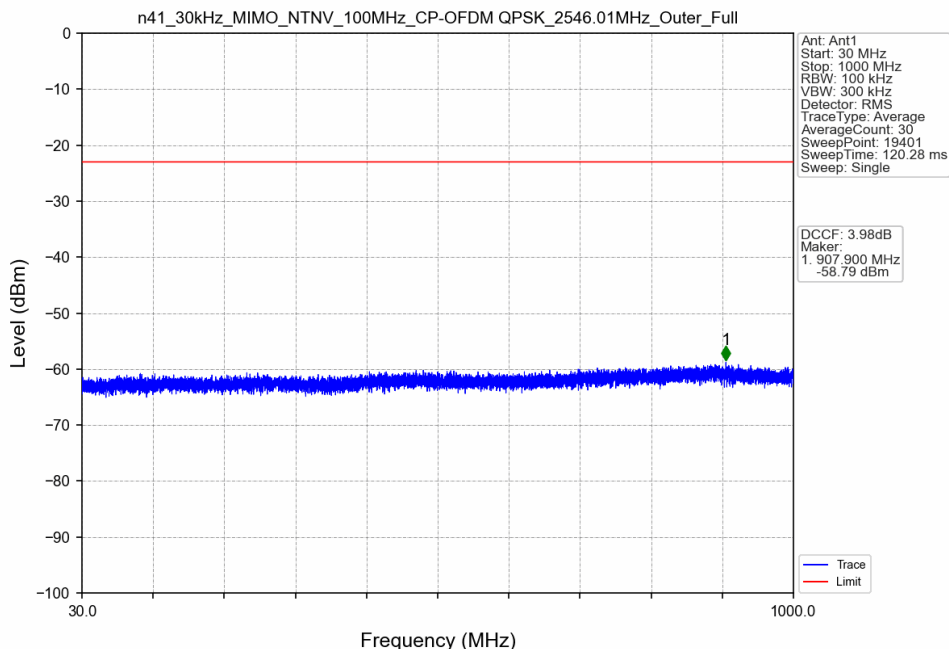
n41_30kHz_MIMO_NTNV_100MHz_CP-OFDM QPSK_2546.01MHz_Outer_Full
