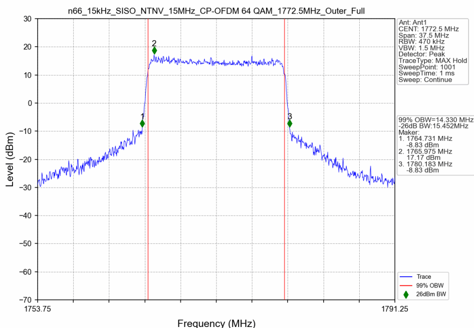
n66_15kHz_SISO_NTNV_15MHz_CP-OFDM 64 QAM_1772.5MHz_Outer_Full
