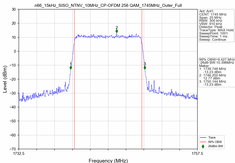
n66_15kHz_SISO_NTNV_10MHz_CP-OFDM 256 QAM_1745MHz_Outer_Full
