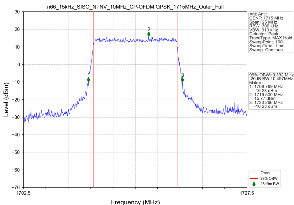
n66_15kHz_SISO_NTNV_10MHz_CP-OFDM QPSK_1715MHz_Outer_Full
