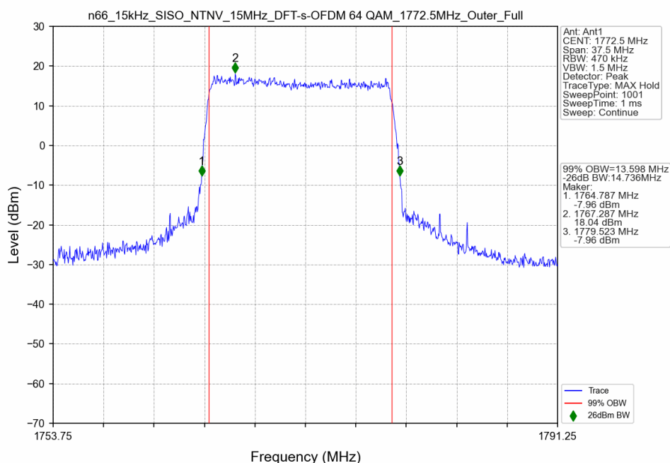
n66_15kHz_SISO_NTNV_15MHz_DFT-s-OFDM 64 QAM_1772.5MHz_Outer_Full
