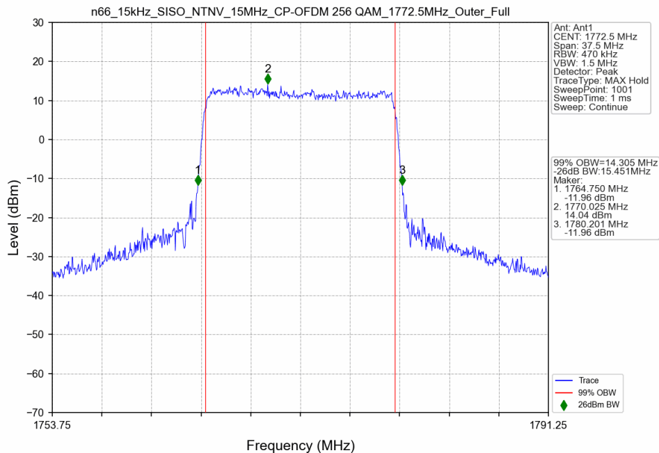
n66_15kHz_SISO_NTNV_15MHz_CP-OFDM 256 QAM_1772.5MHz_Outer_Full
