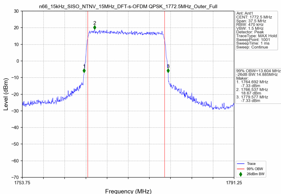
n66_15kHz_SISO_NTNV_15MHz_DFT-s-OFDM QPSK_1772.5MHz_Outer_Full
