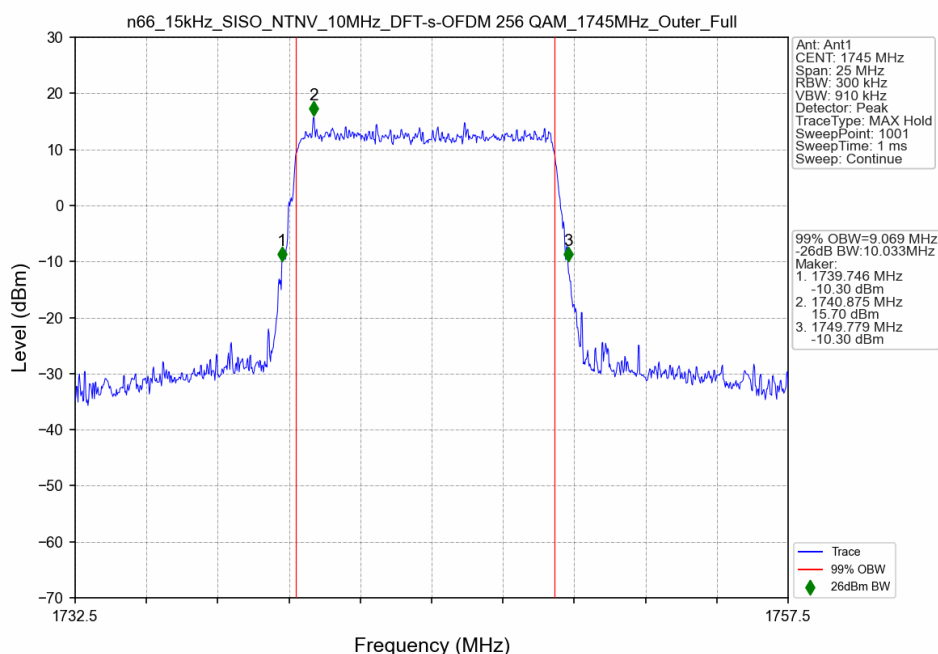
n66_15kHz_SISO_NTNV_10MHz_DFT-s-OFDM 256 QAM_1745MHz_Outer_Full
