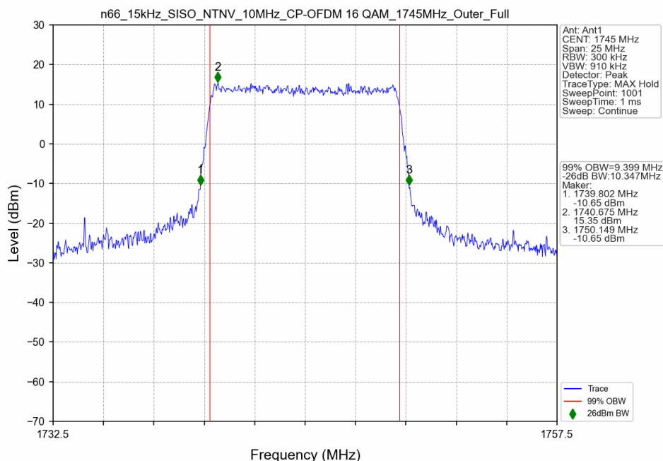
n66_15kHz_SISO_NTNV_10MHz_CP-OFDM 16 QAM_1745MHz_Outer_Full
