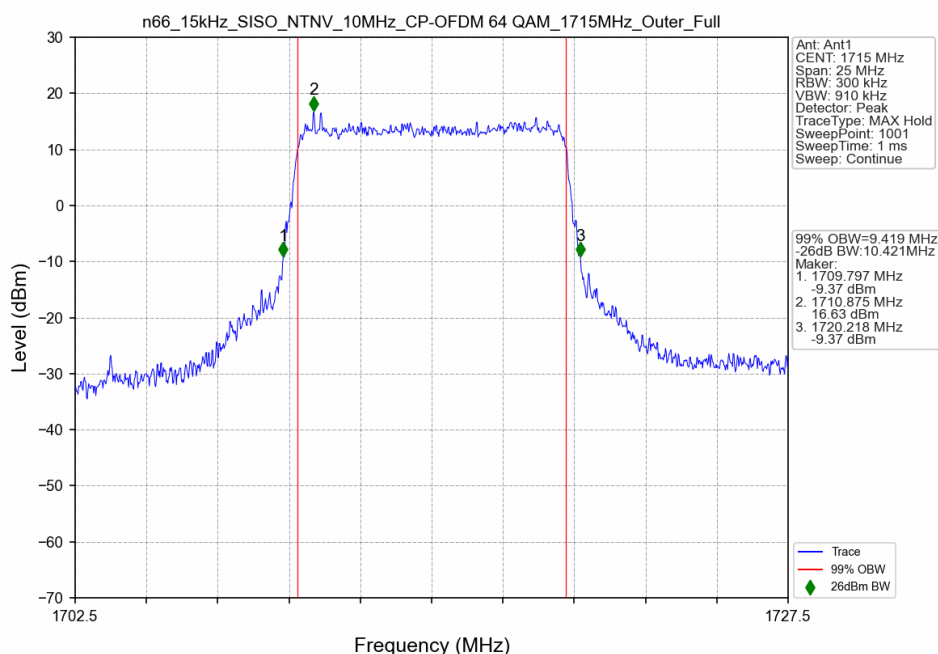
n66_15kHz_SISO_NTNV_10MHz_CP-OFDM 64 QAM_1715MHz_Outer_Full
