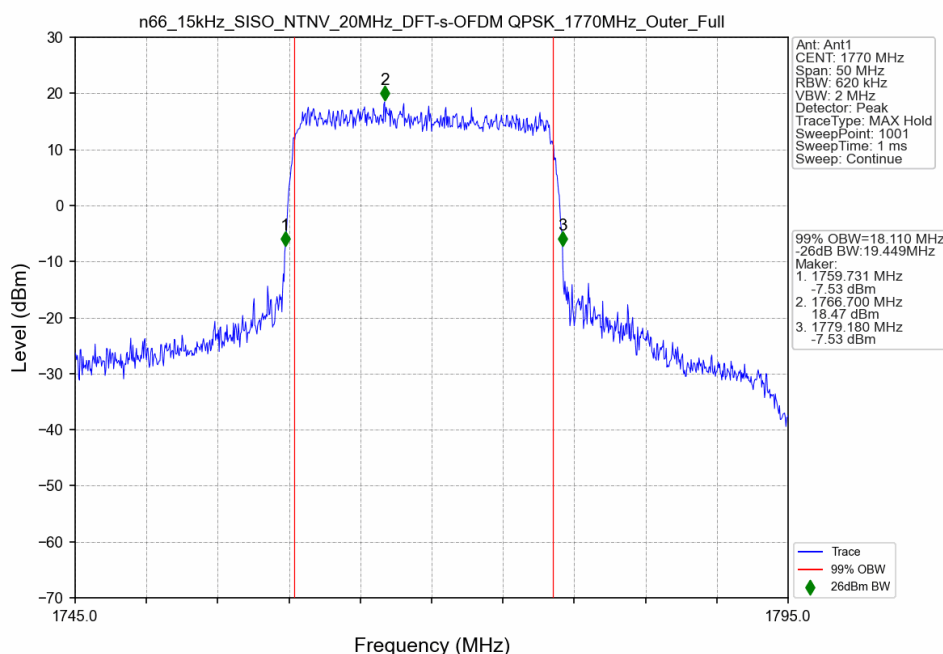
n66_15kHz_SISO_NTNV_20MHz_DFT-s-OFDM QPSK_1770MHz_Outer_Full
