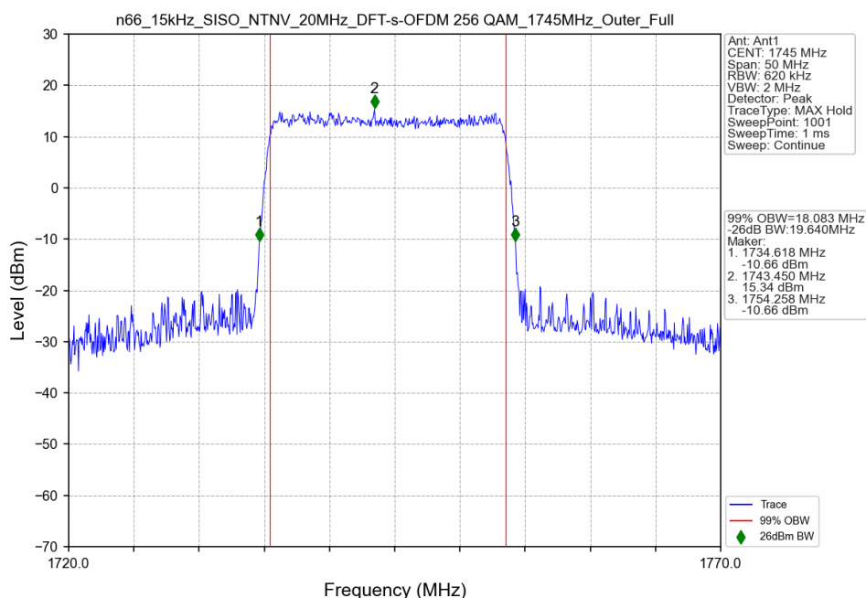
n66_15kHz_SISO_NTNV_20MHz_DFT-s-OFDM 256 QAM_1745MHz_Outer_Full
