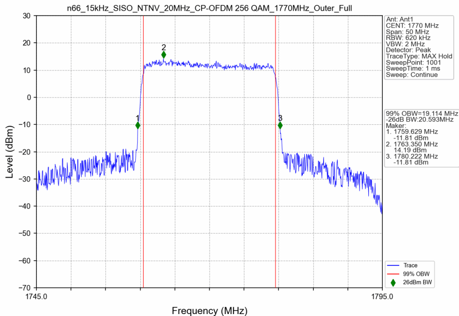
n66_15kHz_SISO_NTNV_20MHz_CP-OFDM 256 QAM_1770MHz_Outer_Full
