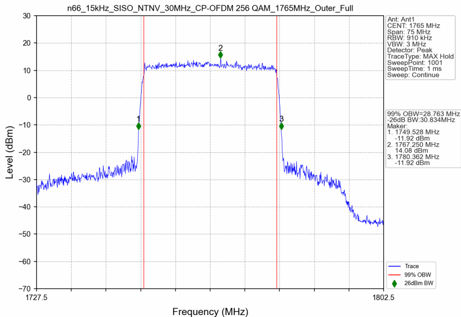
n66_15kHz_SISO_NTNV_30MHz_CP-OFDM 256 QAM_1765MHz_Outer_Full
