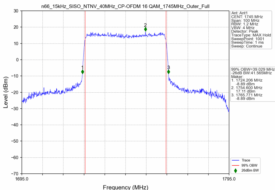
n66_15kHz_SISO_NTNV_40MHz_CP-OFDM 16 QAM_1745MHz_Outer_Full
