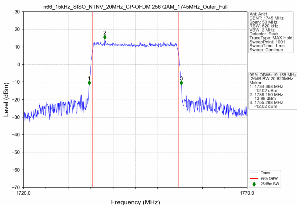
n66_15kHz_SISO_NTNV_20MHz_CP-OFDM 256 QAM_1745MHz_Outer_Full
