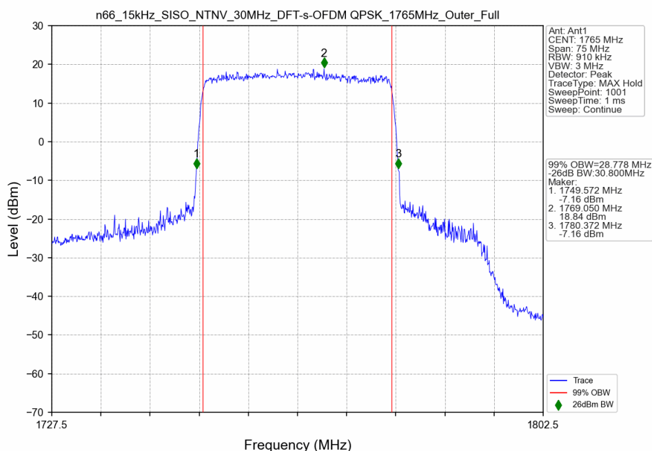
n66_15kHz_SISO_NTNV_30MHz_DFT-s-OFDM QPSK_1765MHz_Outer_Full
