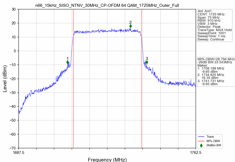
n66_15kHz_SISO_NTNV_30MHz_CP-OFDM 64 QAM_1725MHz_Outer_Full
