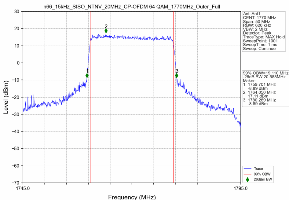
n66_15kHz_SISO_NTNV_20MHz_CP-OFDM 64 QAM_1770MHz_Outer_Full
