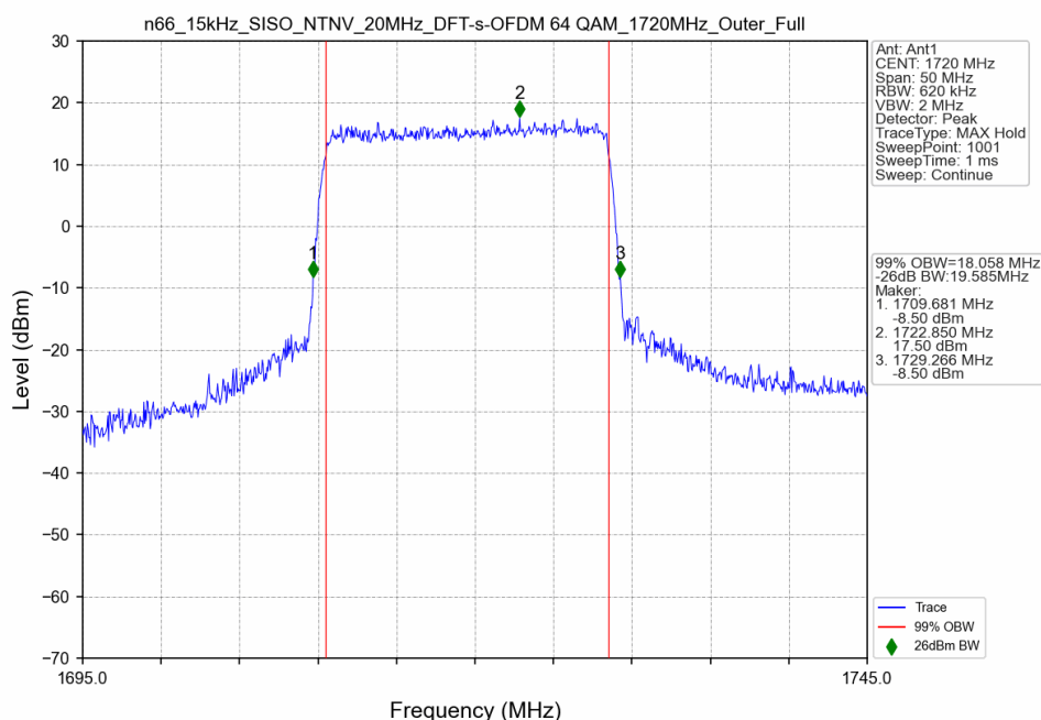
n66_15kHz_SISO_NTNV_20MHz_DFT-s-OFDM 64 QAM_1720MHz_Outer_Full
