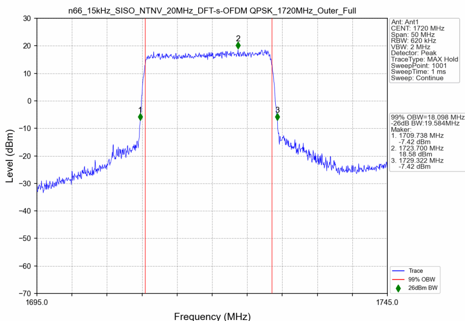
n66_15kHz_SISO_NTNV_20MHz_DFT-s-OFDM QPSK_1720MHz_Outer_Full
