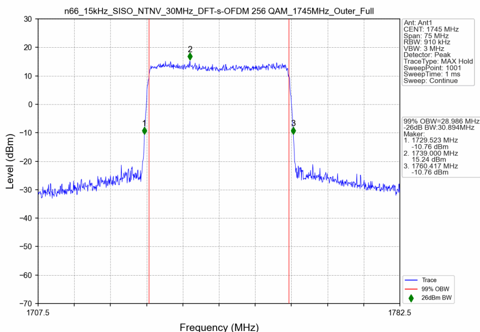
n66_15kHz_SISO_NTNV_30MHz_DFT-s-OFDM 256 QAM_1745MHz_Outer_Full
