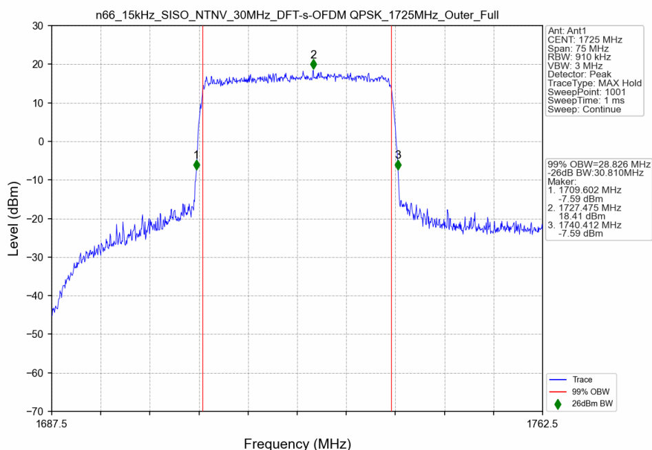
n66_15kHz_SISO_NTNV_30MHz_DFT-s-OFDM QPSK_1725MHz_Outer_Full
