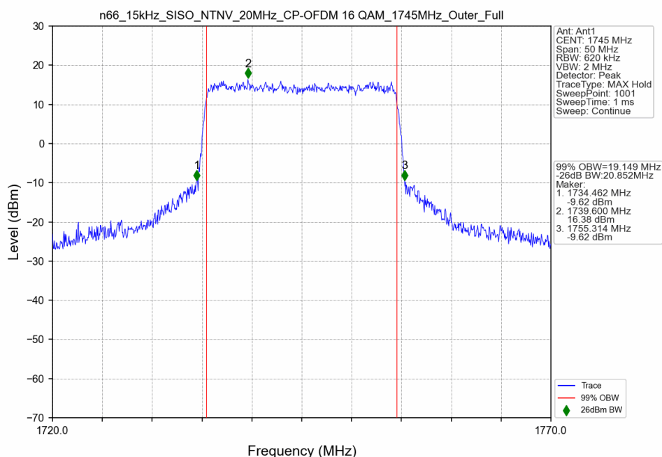
n66_15kHz_SISO_NTNV_20MHz_CP-OFDM 16 QAM_1745MHz_Outer_Full
