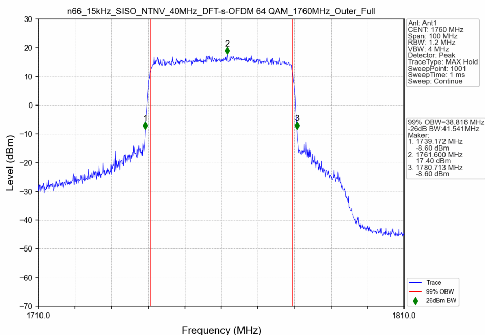
n66_15kHz_SISO_NTNV_40MHz_DFT-s-OFDM 64 QAM_1760MHz_Outer_Full
