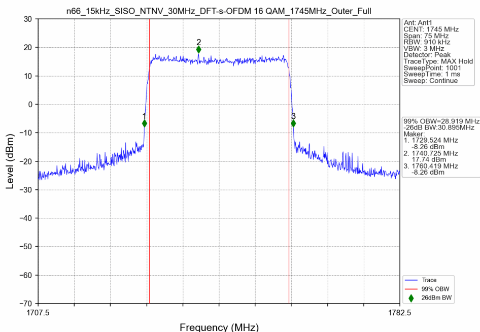
n66_15kHz_SISO_NTNV_30MHz_DFT-s-OFDM 16 QAM_1745MHz_Outer_Full
