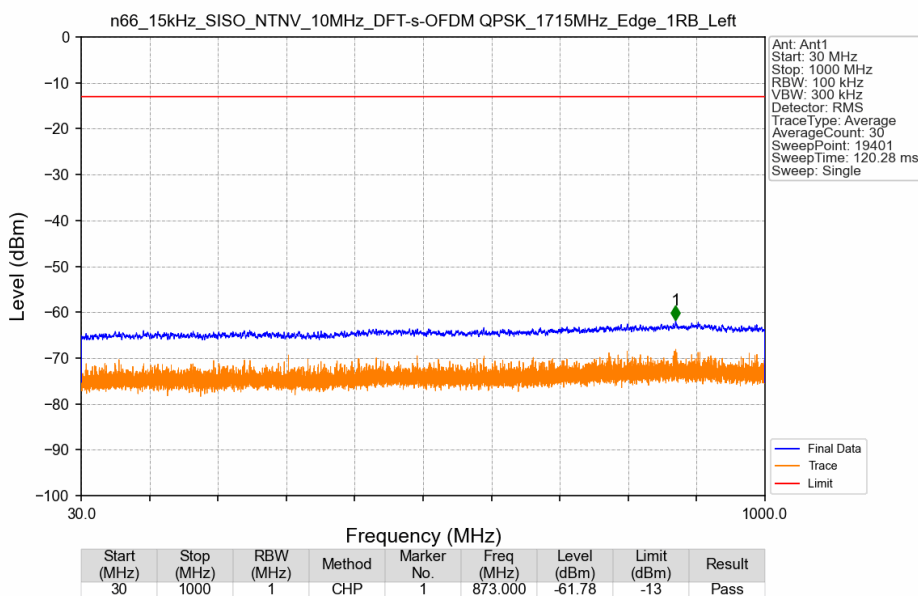
n66_15kHz_SISO_NTNV_10MHz_DFT-s-OFDM QPSK_1715MHz_Edge_1RB_Left
