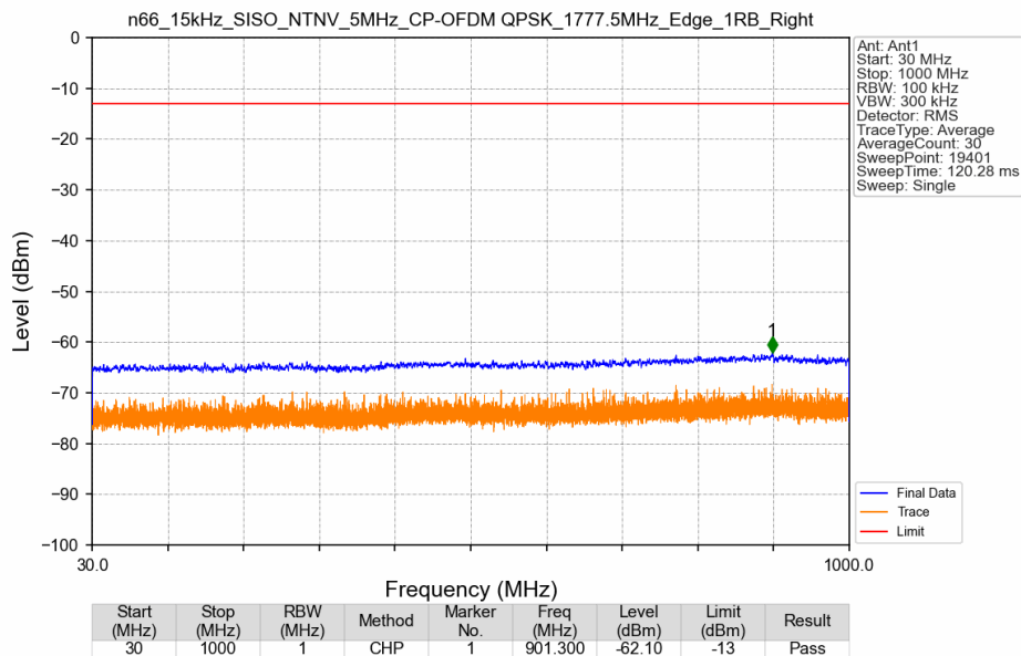
n66_15kHz_SISO_NTNV_5MHz_CP-OFDM QPSK_1777.5MHz_Edge_1RB_Right
