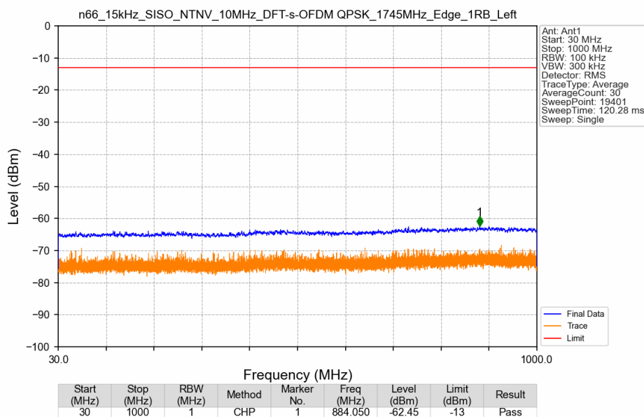
n66_15kHz_SISO_NTNV_10MHz_DFT-s-OFDM QPSK_1745MHz_Edge_1RB_Left
