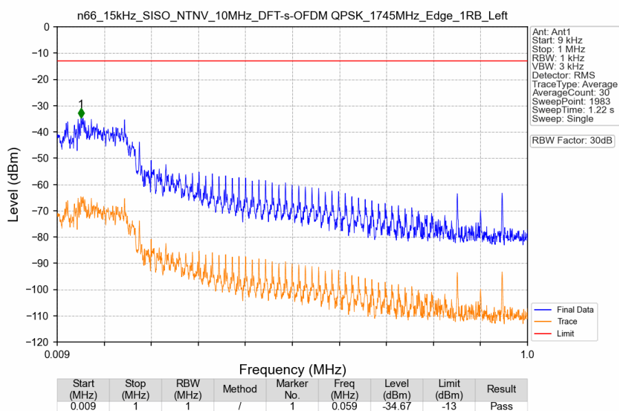
n66_15kHz_SISO_NTNV_10MHz_DFT-s-OFDM QPSK_1745MHz_Edge_1RB_Left
