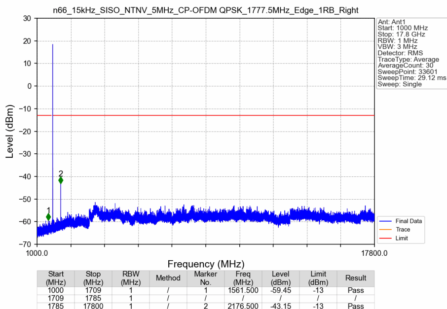
n66_15kHz_SISO_NTNV_5MHz_CP-OFDM QPSK_1777.5MHz_Edge_1RB_Right
