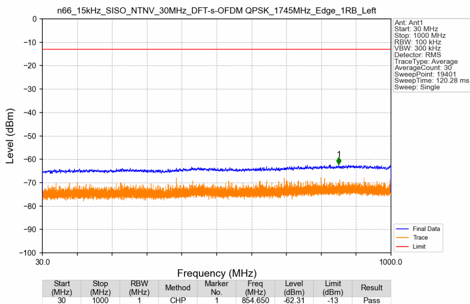
n66_15kHz_SISO_NTNV_30MHz_DFT-s-OFDM QPSK_1745MHz_Edge_1RB_Left
