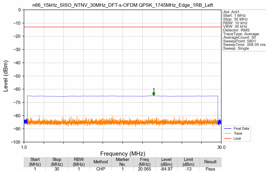
n66_15kHz_SISO_NTNV_30MHz_DFT-s-OFDM QPSK_1745MHz_Edge_1RB_Left
