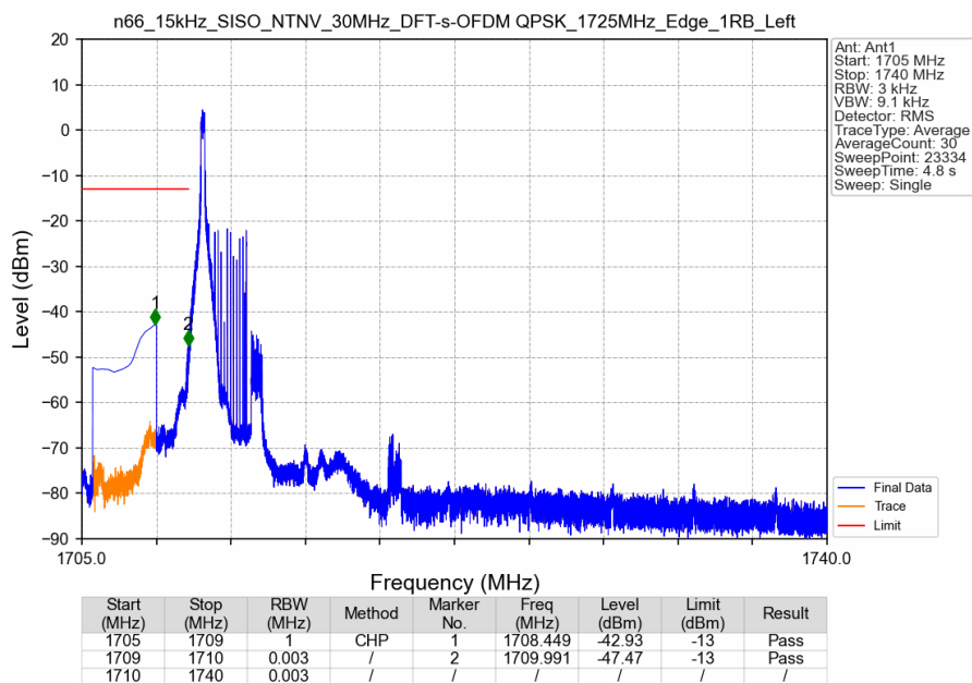
n66_15kHz_SISO_NTNV_30MHz_DFT-s-OFDM QPSK_1725MHz_Edge_1RB_Left
