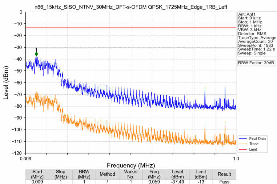
n66_15kHz_SISO_NTNV_30MHz_DFT-s-OFDM QPSK_1725MHz_Edge_1RB_Left
