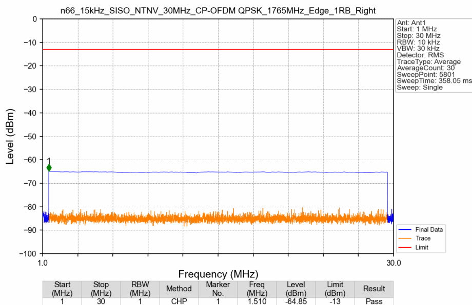
n66_15kHz_SISO_NTNV_30MHz_CP-OFDM QPSK_1765MHz_Edge_1RB_Right
