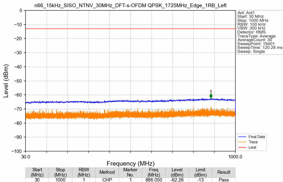
n66_15kHz_SISO_NTNV_30MHz_DFT-s-OFDM QPSK_1725MHz_Edge_1RB_Left
