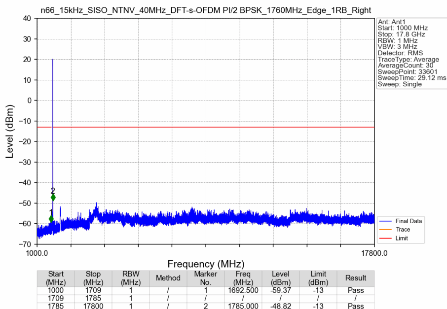
n66_15kHz_SISO_NTNV_40MHz_DFT-s-OFDM PI/2 BPSK_1760MHz_Edge_1RB_Right
