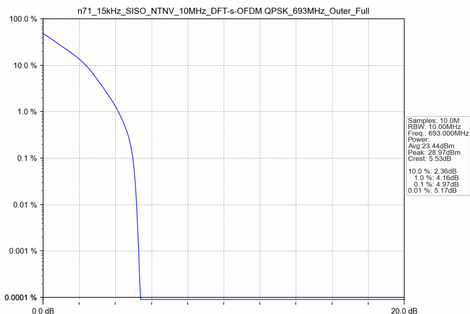
n71_15kHz_SISO_NTNV_10MHz_DFT-s-OFDM QPSK_693MHz_Outer_Full
