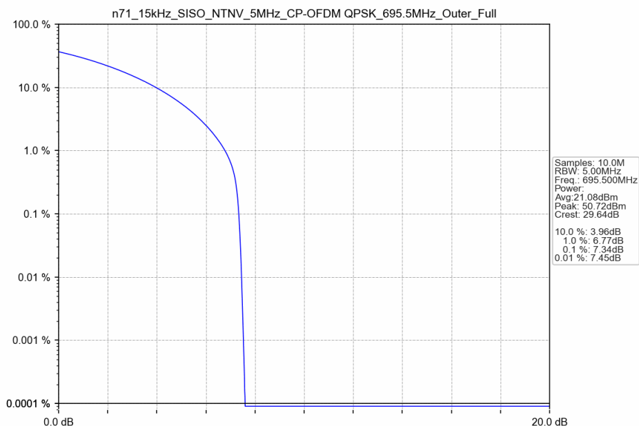
n71_15kHz_SISO_NTNV_5MHz_CP-OFDM QPSK_695.5MHz_Outer_Full
