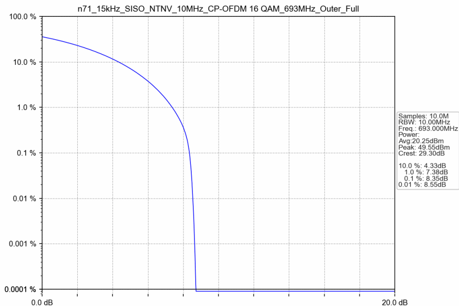
n71_15kHz_SISO_NTNV_10MHz_CP-OFDM 16 QAM_693MHz_Outer_Full
