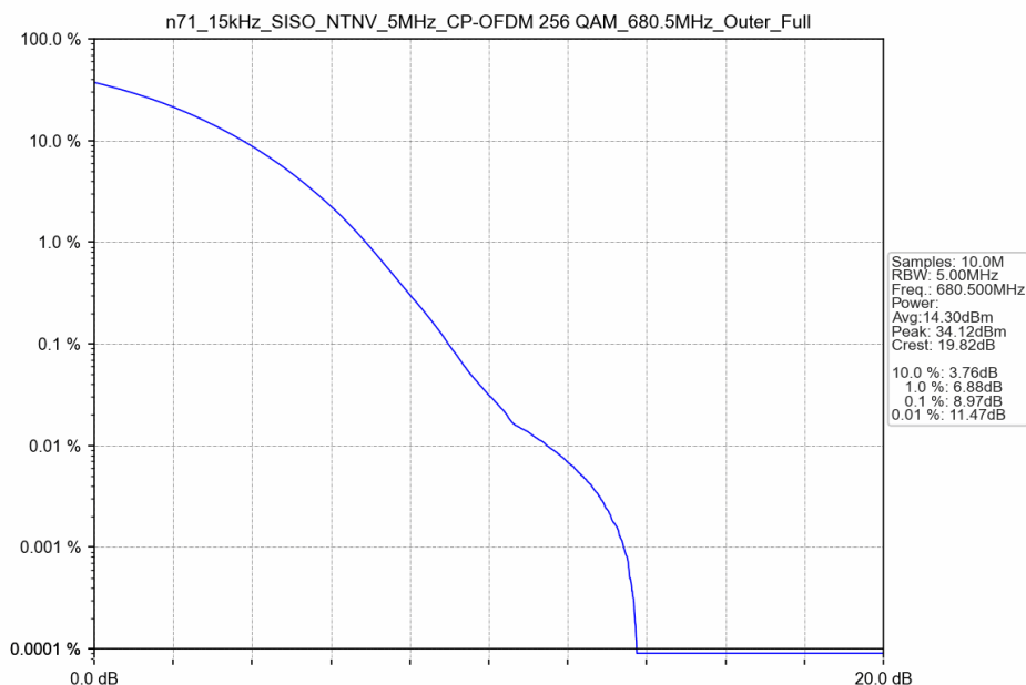
n71_15kHz_SISO_NTNV_5MHz_CP-OFDM 256 QAM_680.5MHz_Outer_Full
