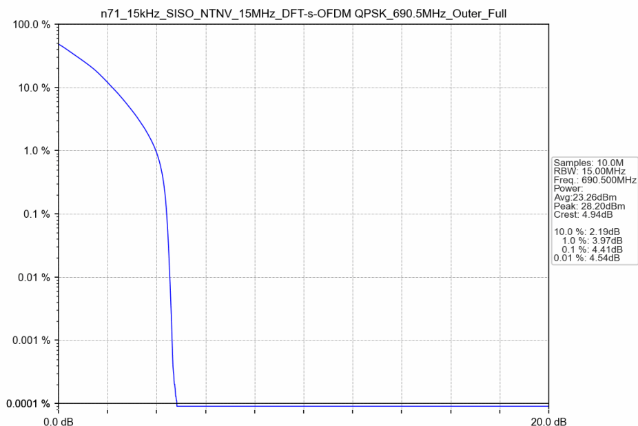
n71_15kHz_SISO_NTNV_15MHz_DFT-s-OFDM QPSK_690.5MHz_Outer_Full
