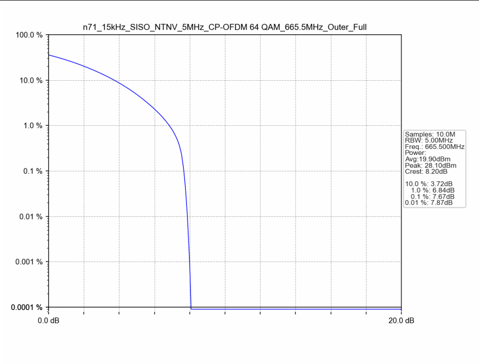
n71_15kHz_SISO_NTNV_5MHz_CP-OFDM 64 QAM_665.5MHz_Outer_Full
