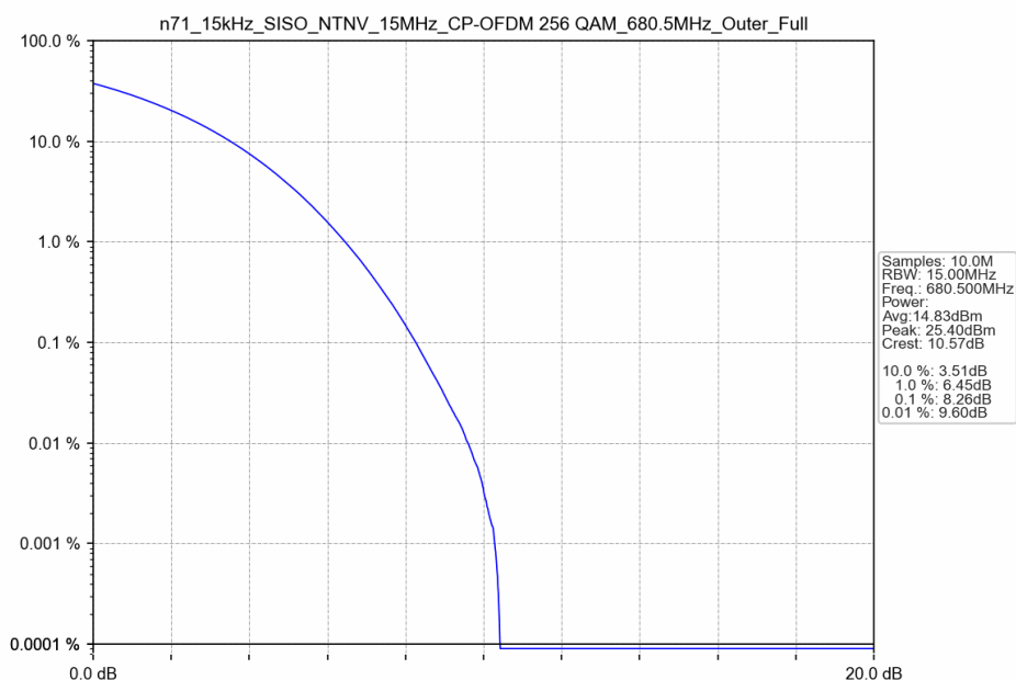
n71_15kHz_SISO_NTNV_15MHz_CP-OFDM 256 QAM_680.5MHz_Outer_Full
