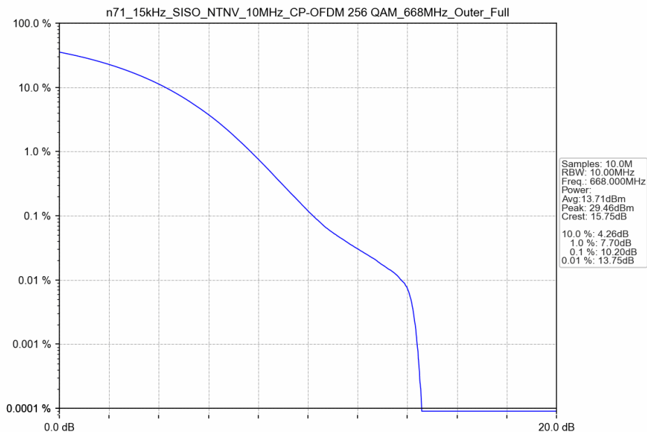
n71_15kHz_SISO_NTNV_10MHz_CP-OFDM 256 QAM_668MHz_Outer_Full
