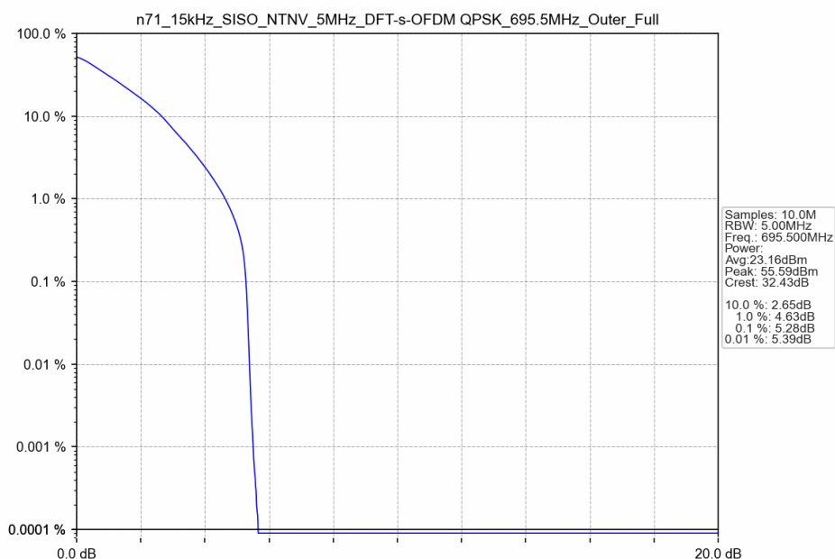
n71_15kHz_SISO_NTNV_5MHz_DFT-s-OFDM QPSK_695.5MHz_Outer_Full
