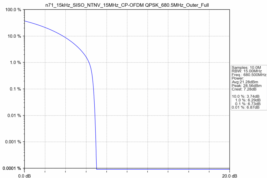
n71_15kHz_SISO_NTNV_15MHz_CP-OFDM QPSK_680.5MHz_Outer_Full
