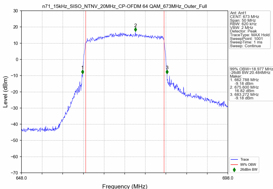
n71_15kHz_SISO_NTNV_20MHz_CP-OFDM 64 QAM_673MHz_Outer_Full
