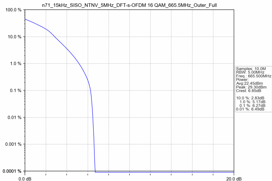
n71_15kHz_SISO_NTNV_5MHz_DFT-s-OFDM 16 QAM_665.5MHz_Outer_Full
