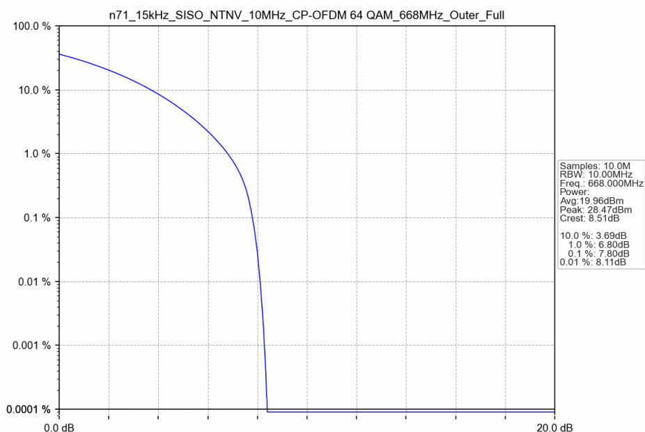
n71_15kHz_SISO_NTNV_10MHz_CP-OFDM 64 QAM_668MHz_Outer_Full
