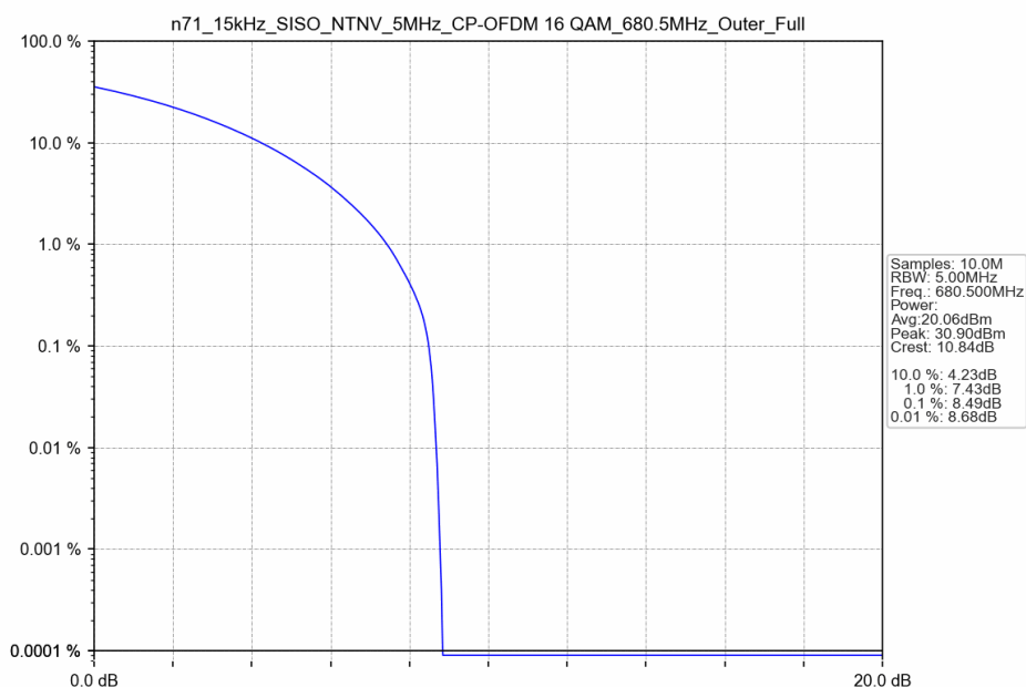
n71_15kHz_SISO_NTNV_5MHz_CP-OFDM 16 QAM_680.5MHz_Outer_Full
