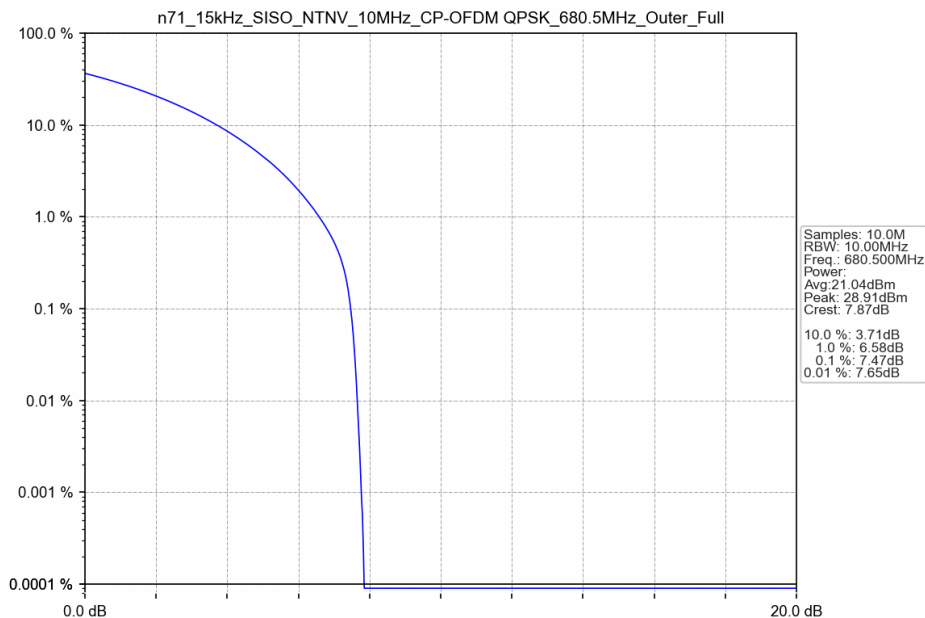
n71_15kHz_SISO_NTNV_10MHz_CP-OFDM QPSK_680.5MHz_Outer_Full
