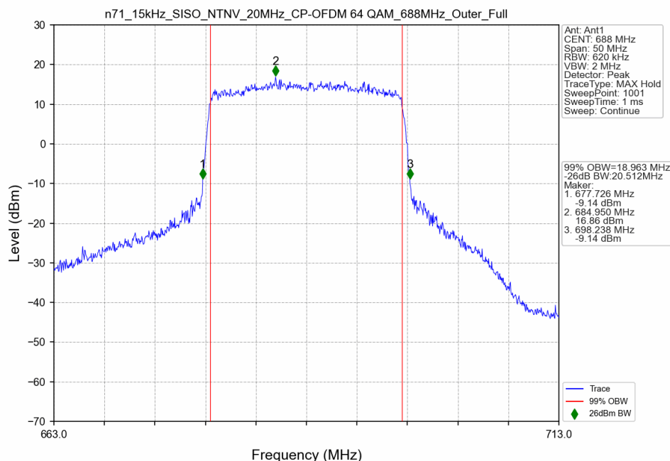
n71_15kHz_SISO_NTNV_20MHz_CP-OFDM 64 QAM_688MHz_Outer_Full
