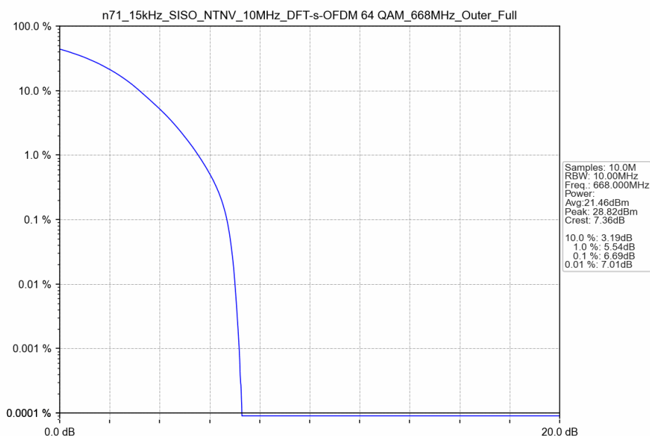
n71_15kHz_SISO_NTNV_10MHz_DFT-s-OFDM 64 QAM_668MHz_Outer_Full
