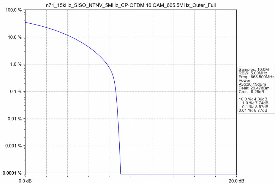
n71_15kHz_SISO_NTNV_5MHz_CP-OFDM 16 QAM_665.5MHz_Outer_Full
