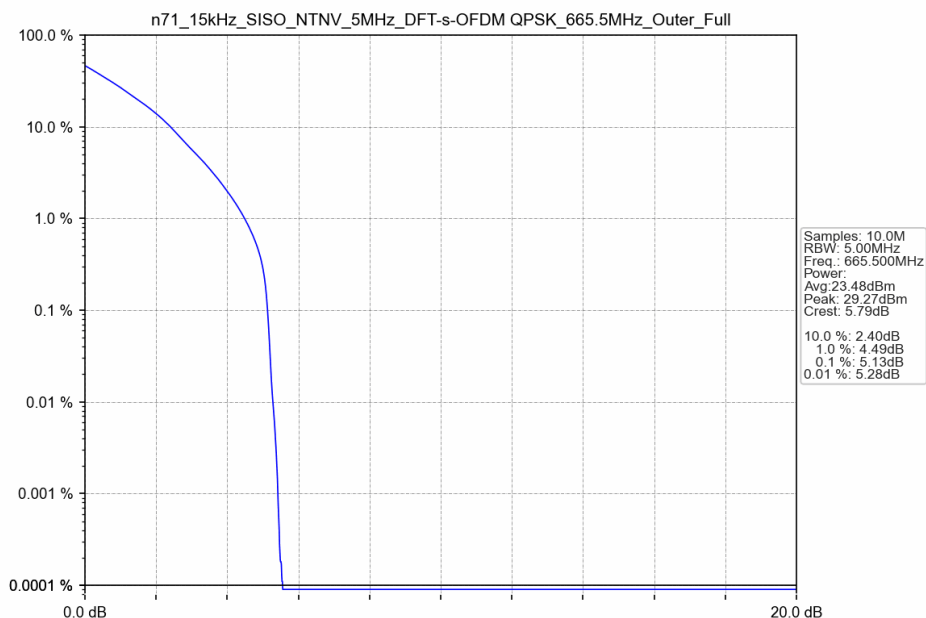
n71_15kHz_SISO_NTNV_5MHz_DFT-s-OFDM QPSK_665.5MHz_Outer_Full
