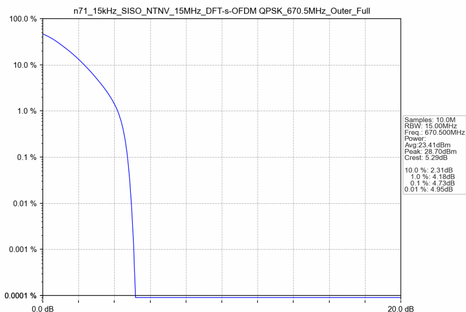
n71_15kHz_SISO_NTNV_15MHz_DFT-s-OFDM QPSK_670.5MHz_Outer_Full
