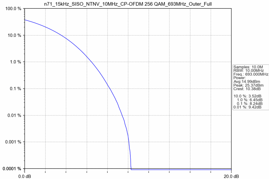
n71_15kHz_SISO_NTNV_10MHz_CP-OFDM 256 QAM_693MHz_Outer_Full
