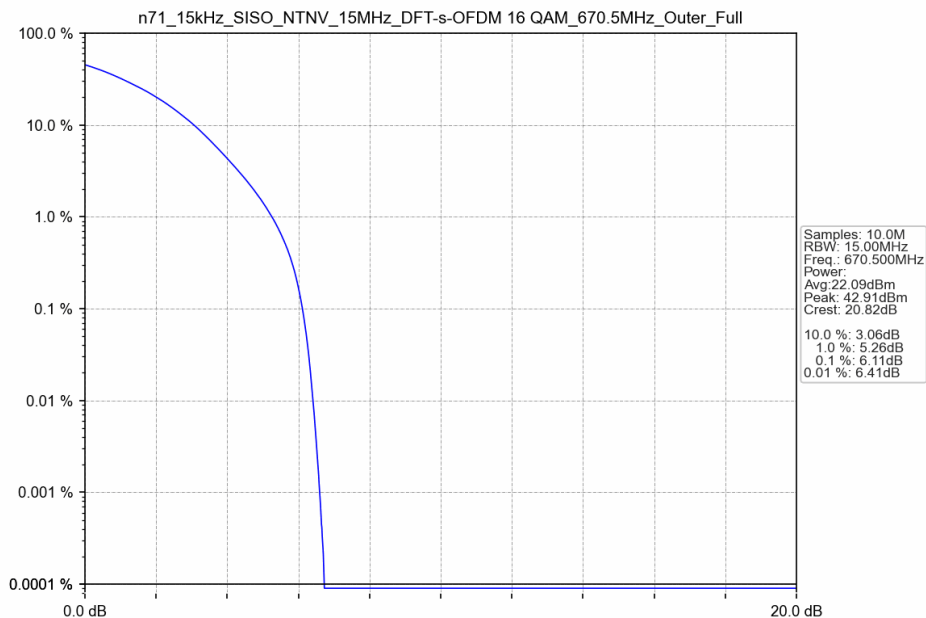
n71_15kHz_SISO_NTNV_15MHz_DFT-s-OFDM 16 QAM_670.5MHz_Outer_Full
