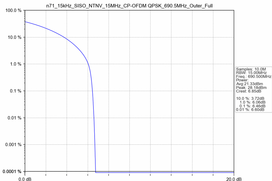
n71_15kHz_SISO_NTNV_15MHz_CP-OFDM QPSK_690.5MHz_Outer_Full
