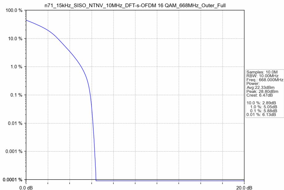
n71_15kHz_SISO_NTNV_10MHz_DFT-s-OFDM 16 QAM_668MHz_Outer_Full
