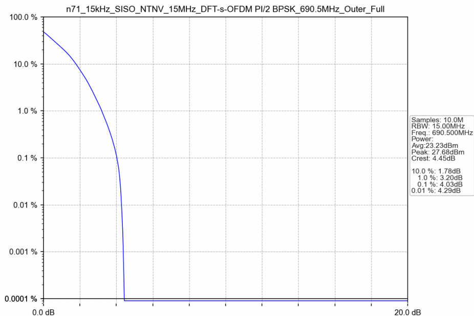
n71_15kHz_SISO_NTNV_15MHz_DFT-s-OFDM PI/2 BPSK_690.5MHz_Outer_Full
