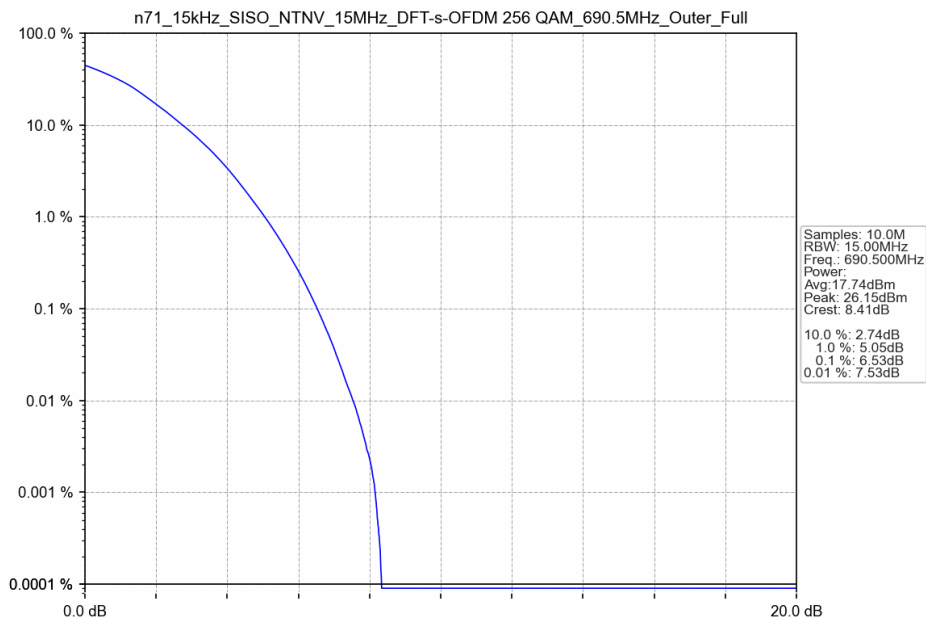
n71_15kHz_SISO_NTNV_15MHz_DFT-s-OFDM 256 QAM_690.5MHz_Outer_Full
