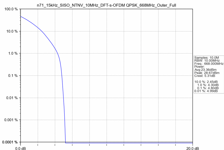
n71_15kHz_SISO_NTNV_10MHz_DFT-s-OFDM QPSK_668MHz_Outer_Full
