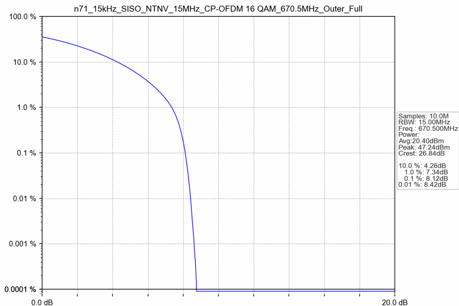
n71_15kHz_SISO_NTNV_15MHz_CP-OFDM 16 QAM_670.5MHz_Outer_Full
