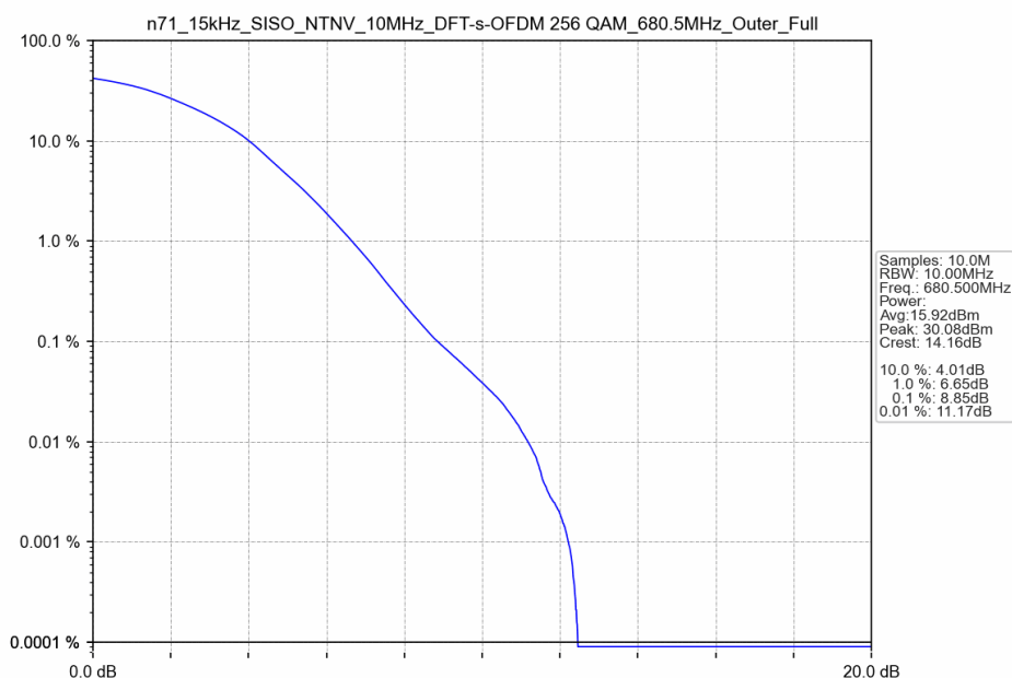
n71_15kHz_SISO_NTNV_10MHz_DFT-s-OFDM 256 QAM_680.5MHz_Outer_Full
