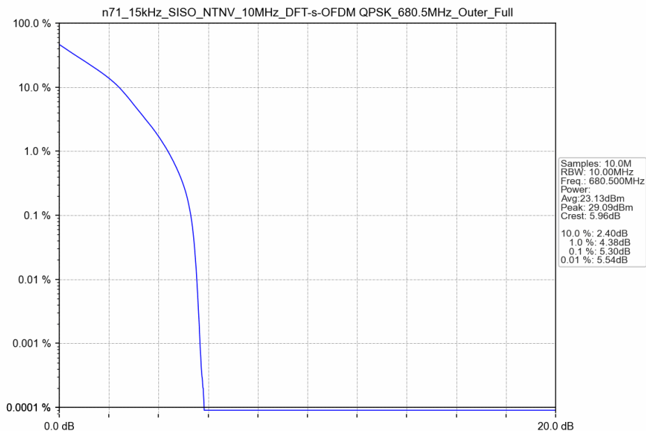
n71_15kHz_SISO_NTNV_10MHz_DFT-s-OFDM QPSK_680.5MHz_Outer_Full
