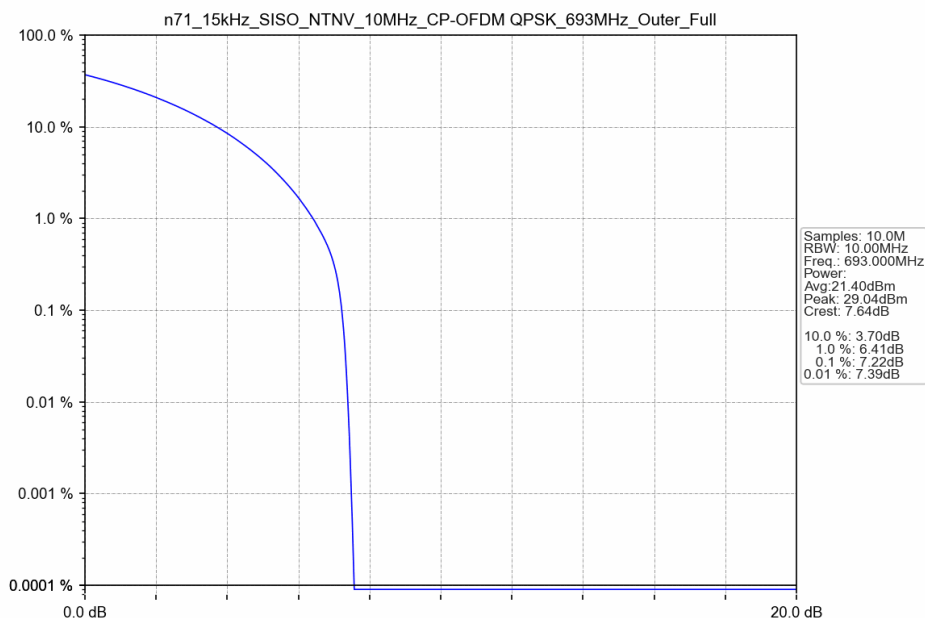
n71_15kHz_SISO_NTNV_10MHz_CP-OFDM QPSK_693MHz_Outer_Full
