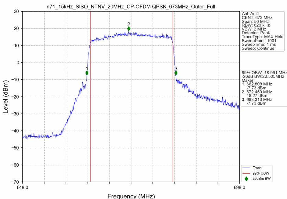
n71_15kHz_SISO_NTNV_20MHz_CP-OFDM QPSK_673MHz_Outer_Full
