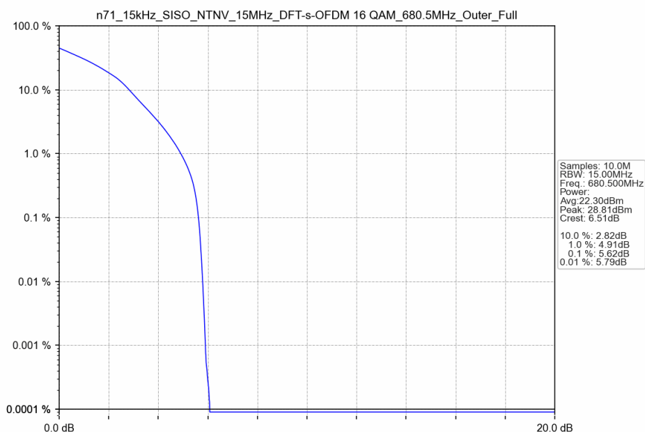
n71_15kHz_SISO_NTNV_15MHz_DFT-s-OFDM 16 QAM_680.5MHz_Outer_Full
