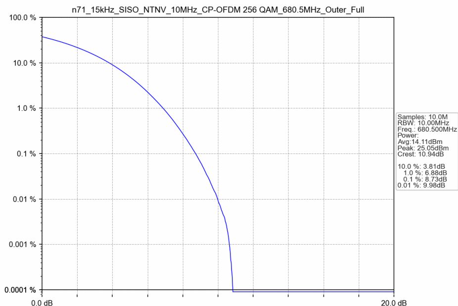
n71_15kHz_SISO_NTNV_10MHz_CP-OFDM 256 QAM_680.5MHz_Outer_Full
