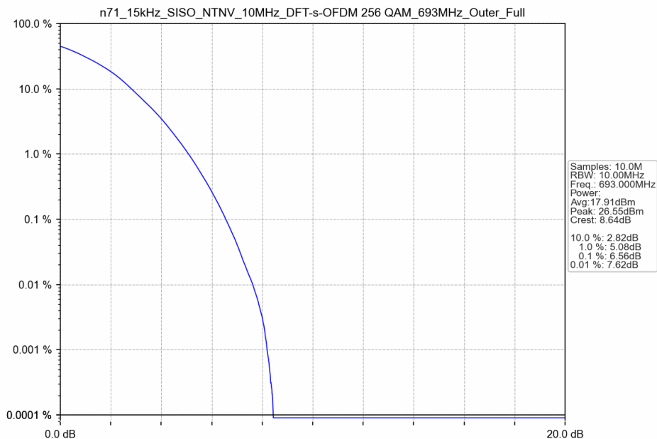
n71_15kHz_SISO_NTNV_10MHz_DFT-s-OFDM 256 QAM_693MHz_Outer_Full
