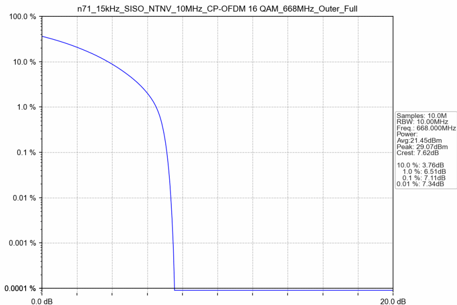
n71_15kHz_SISO_NTNV_10MHz_CP-OFDM 16 QAM_668MHz_Outer_Full
