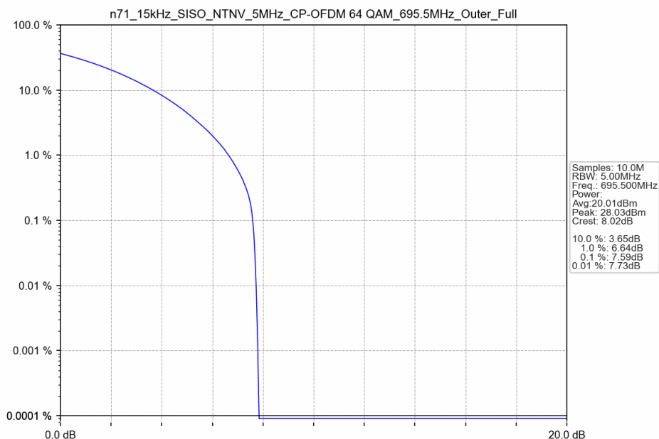
n71_15kHz_SISO_NTNV_5MHz_CP-OFDM 64 QAM_695.5MHz_Outer_Full
