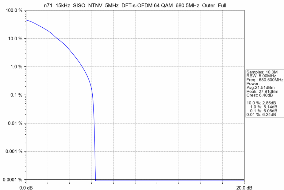
n71_15kHz_SISO_NTNV_5MHz_DFT-s-OFDM 64 QAM_680.5MHz_Outer_Full
