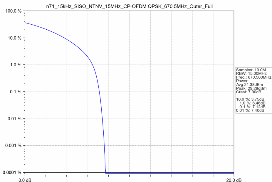
n71_15kHz_SISO_NTNV_15MHz_CP-OFDM QPSK_670.5MHz_Outer_Full
