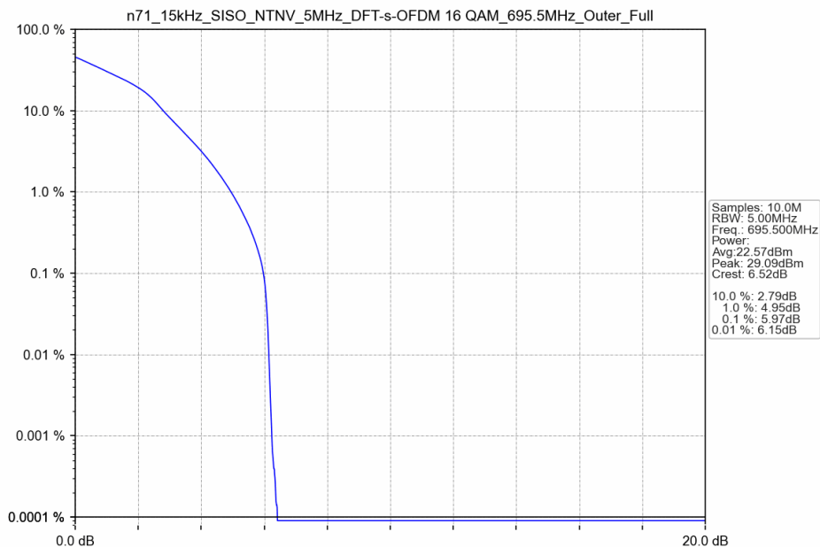
n71_15kHz_SISO_NTNV_5MHz_DFT-s-OFDM 16 QAM_695.5MHz_Outer_Full
