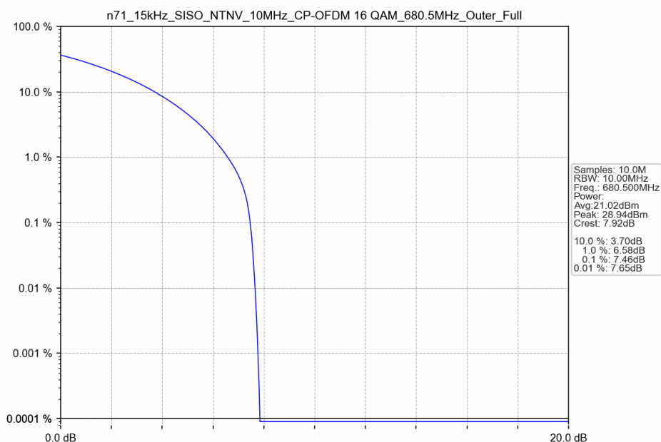
n71_15kHz_SISO_NTNV_10MHz_CP-OFDM 16 QAM_680.5MHz_Outer_Full
