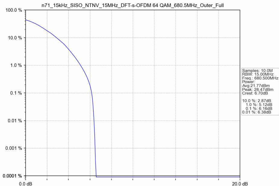
n71_15kHz_SISO_NTNV_15MHz_DFT-s-OFDM 64 QAM_680.5MHz_Outer_Full
