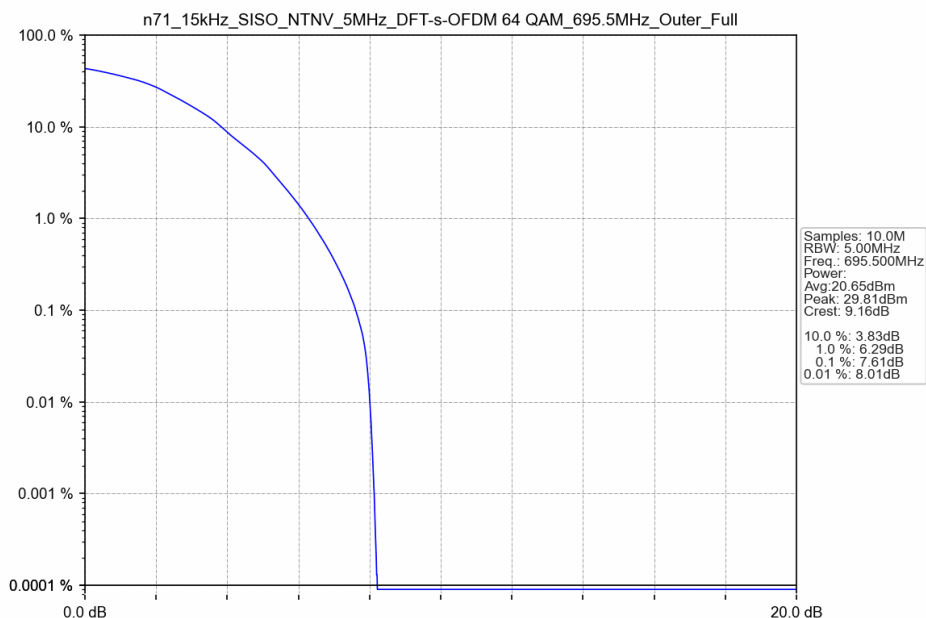
n71_15kHz_SISO_NTNV_5MHz_DFT-s-OFDM 64 QAM_695.5MHz_Outer_Full
