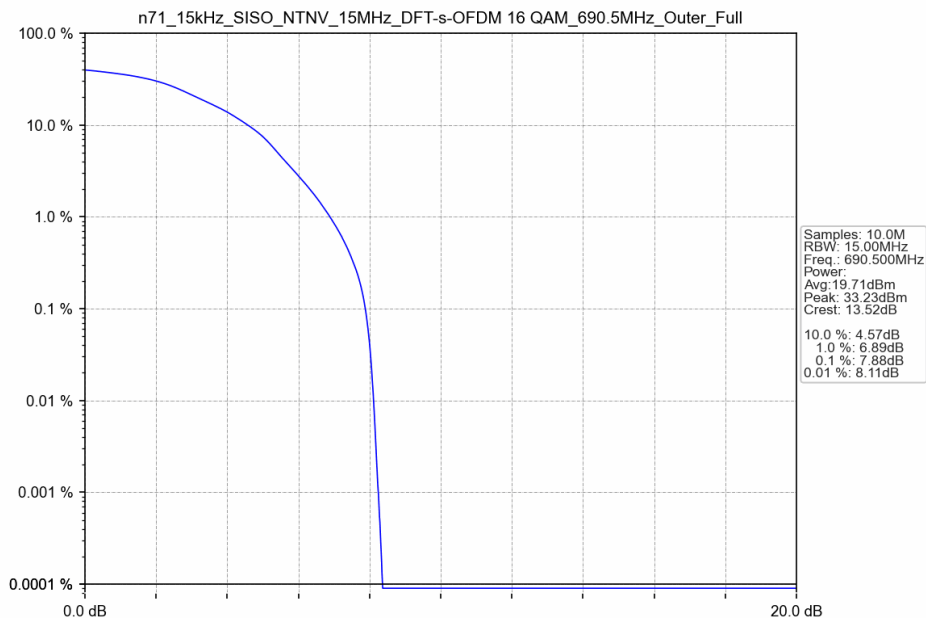
n71_15kHz_SISO_NTNV_15MHz_DFT-s-OFDM 16 QAM_690.5MHz_Outer_Full
