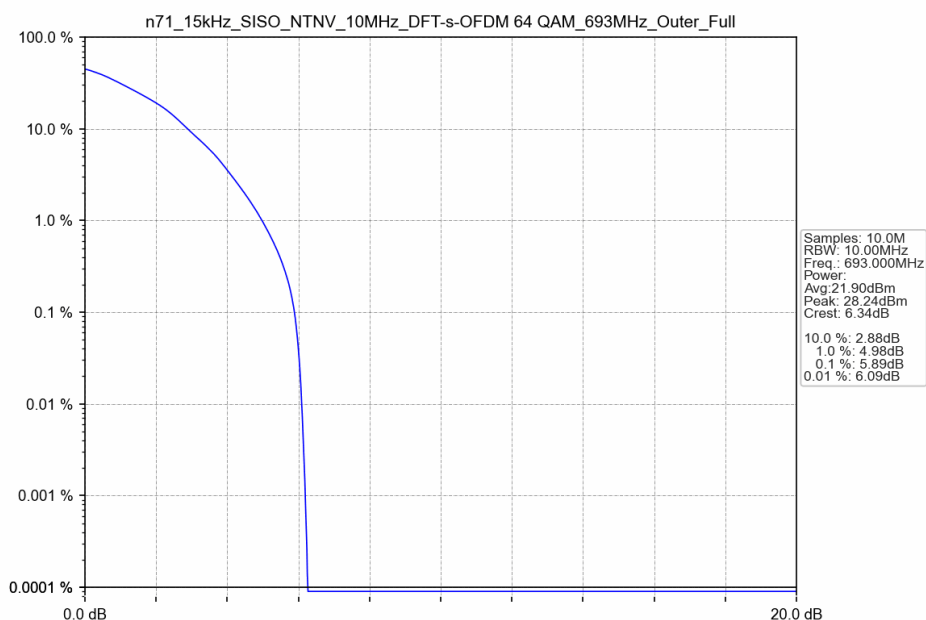
n71_15kHz_SISO_NTNV_10MHz_DFT-s-OFDM 64 QAM_693MHz_Outer_Full
