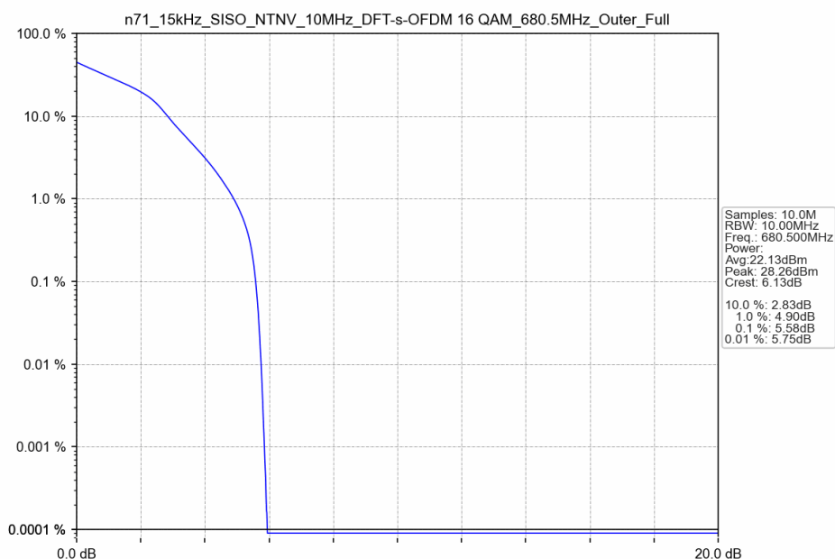
n71_15kHz_SISO_NTNV_10MHz_DFT-s-OFDM 16 QAM_680.5MHz_Outer_Full
