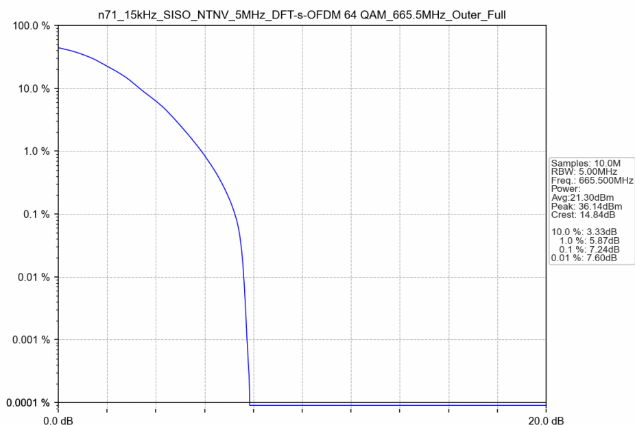
n71_15kHz_SISO_NTNV_5MHz_DFT-s-OFDM 64 QAM_665.5MHz_Outer_Full
