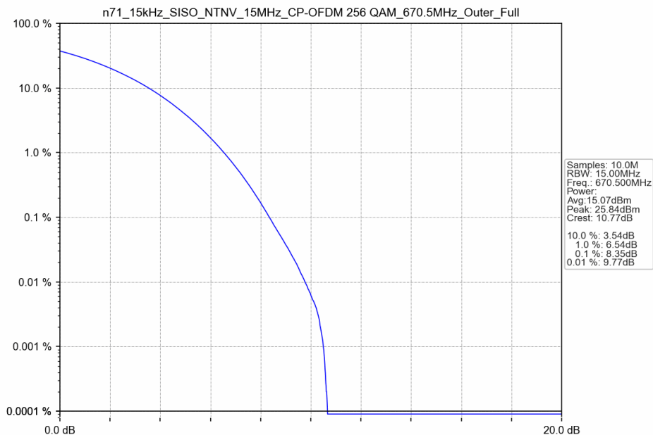
n71_15kHz_SISO_NTNV_15MHz_CP-OFDM 256 QAM_670.5MHz_Outer_Full
