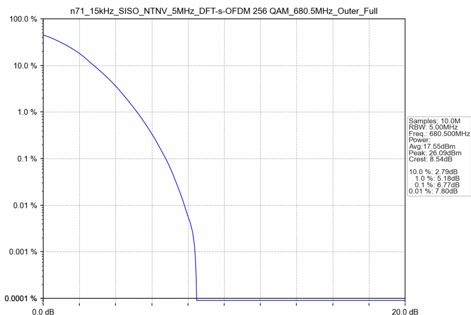
n71_15kHz_SISO_NTNV_5MHz_DFT-s-OFDM 256 QAM_680.5MHz_Outer_Full
