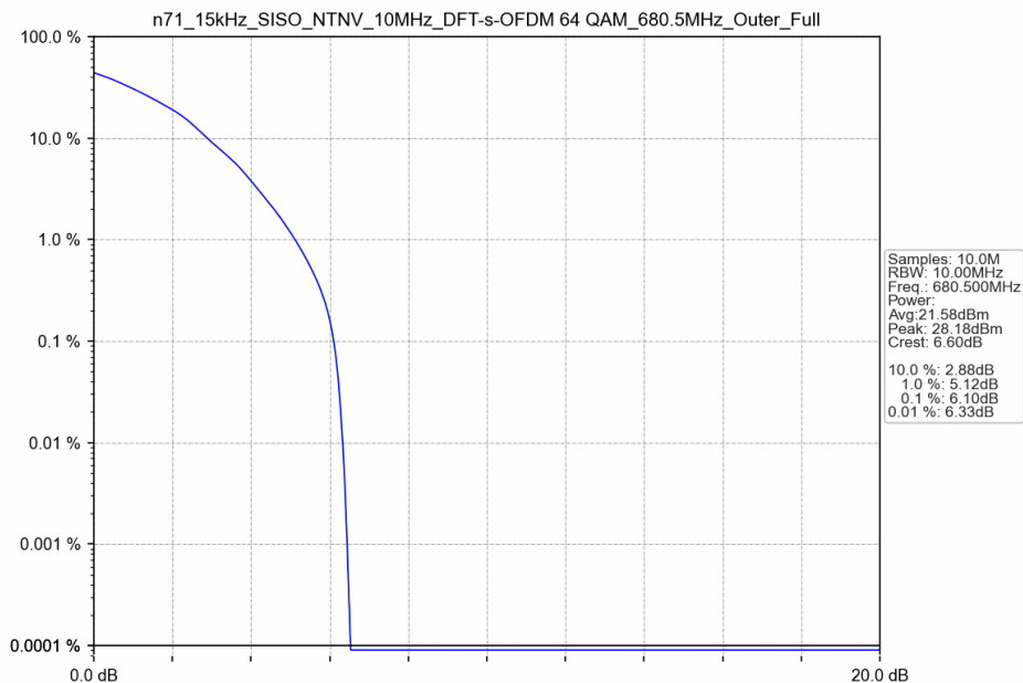
n71_15kHz_SISO_NTNV_10MHz_DFT-s-OFDM 64 QAM_680.5MHz_Outer_Full
