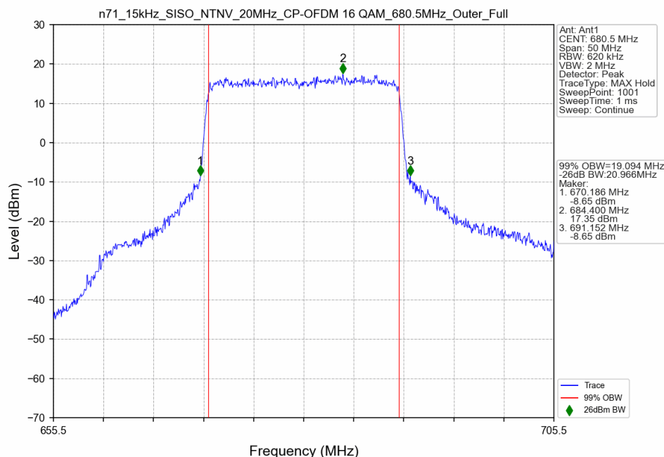
n71_15kHz_SISO_NTNV_20MHz_CP-OFDM 16 QAM_680.5MHz_Outer_Full
