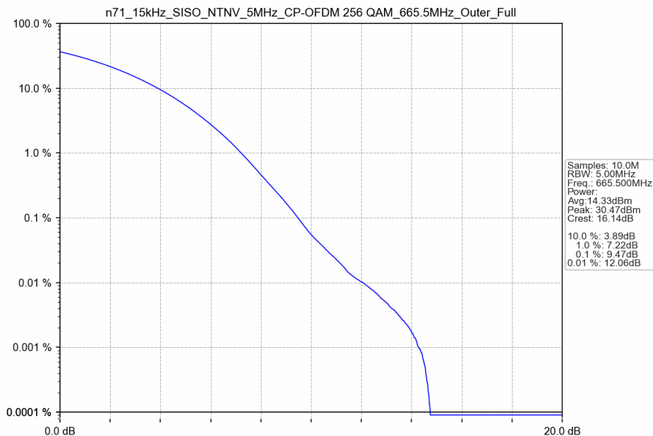
n71_15kHz_SISO_NTNV_5MHz_CP-OFDM 256 QAM_665.5MHz_Outer_Full
