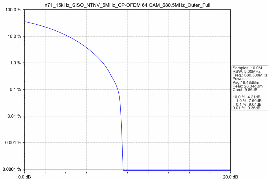
n71_15kHz_SISO_NTNV_5MHz_CP-OFDM 64 QAM_680.5MHz_Outer_Full
