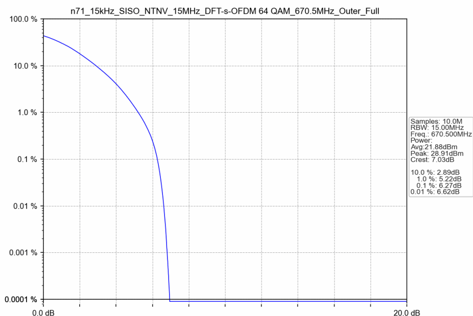
n71_15kHz_SISO_NTNV_15MHz_DFT-s-OFDM 64 QAM_670.5MHz_Outer_Full
