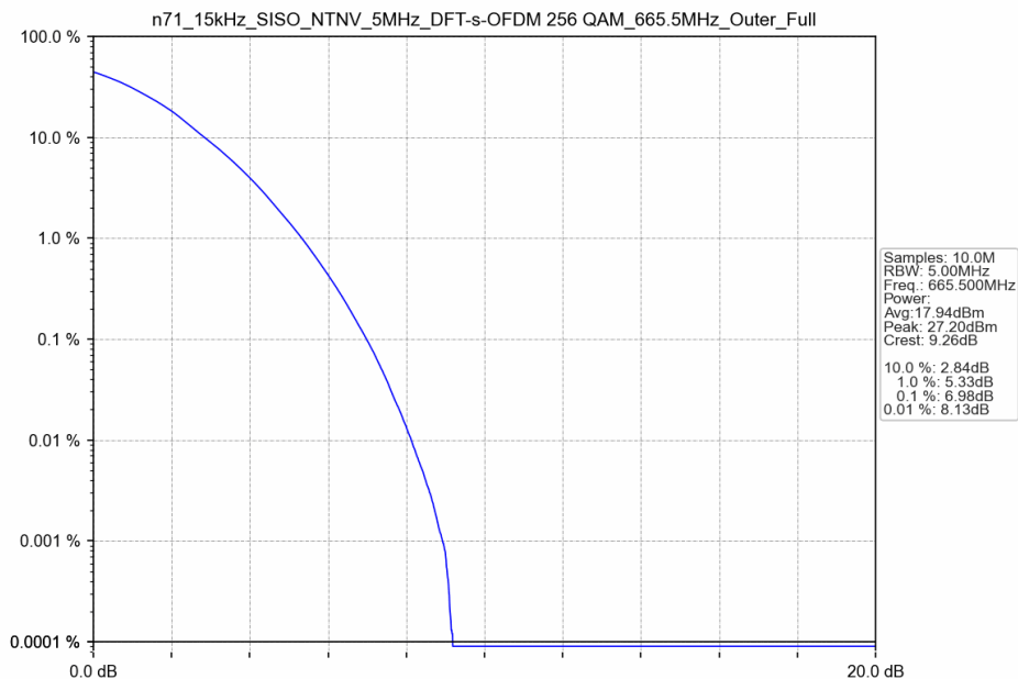
n71_15kHz_SISO_NTNV_5MHz_DFT-s-OFDM 256 QAM_665.5MHz_Outer_Full
