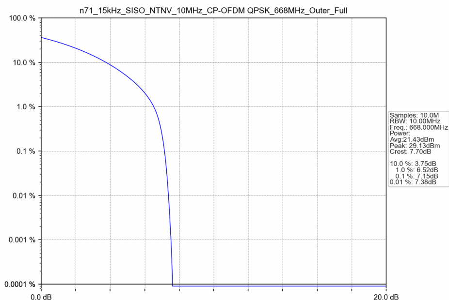
n71_15kHz_SISO_NTNV_10MHz_CP-OFDM QPSK_668MHz_Outer_Full
