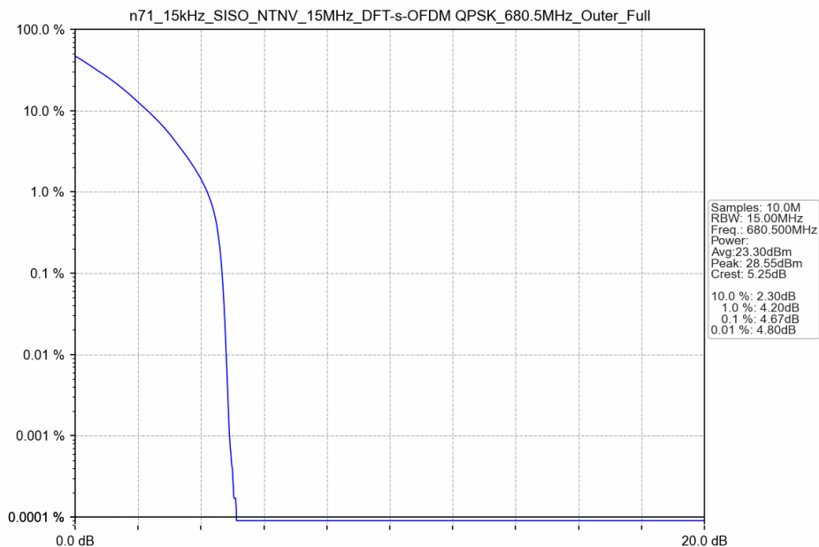
n71_15kHz_SISO_NTNV_15MHz_DFT-s-OFDM QPSK_680.5MHz_Outer_Full
