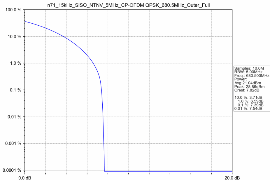
n71_15kHz_SISO_NTNV_5MHz_CP-OFDM QPSK_680.5MHz_Outer_Full
