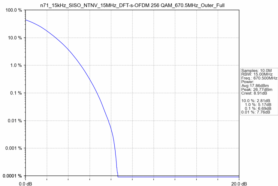
n71_15kHz_SISO_NTNV_15MHz_DFT-s-OFDM 256 QAM_670.5MHz_Outer_Full
