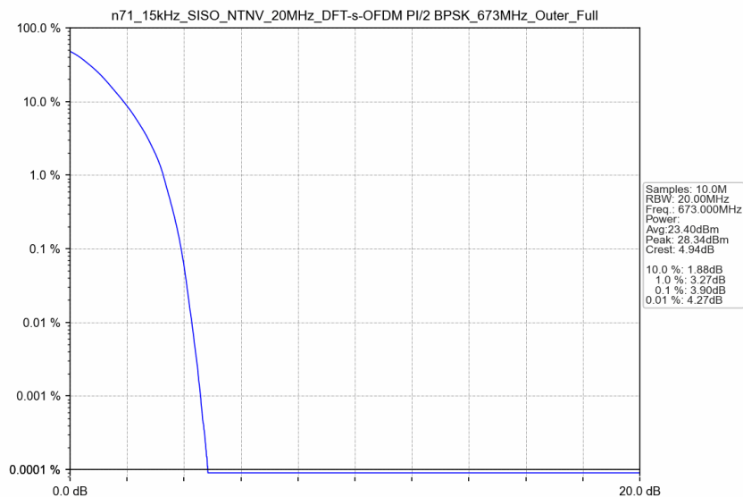
n71_15kHz_SISO_NTNV_20MHz_DFT-s-OFDM PI/2 BPSK_673MHz_Outer_Full
