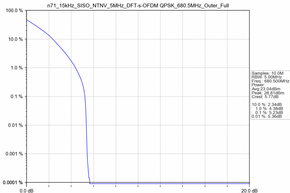
n71_15kHz_SISO_NTNV_5MHz_DFT-s-OFDM QPSK_680.5MHz_Outer_Full
