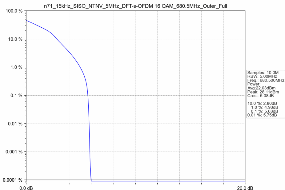
n71_15kHz_SISO_NTNV_5MHz_DFT-s-OFDM 16 QAM_680.5MHz_Outer_Full
