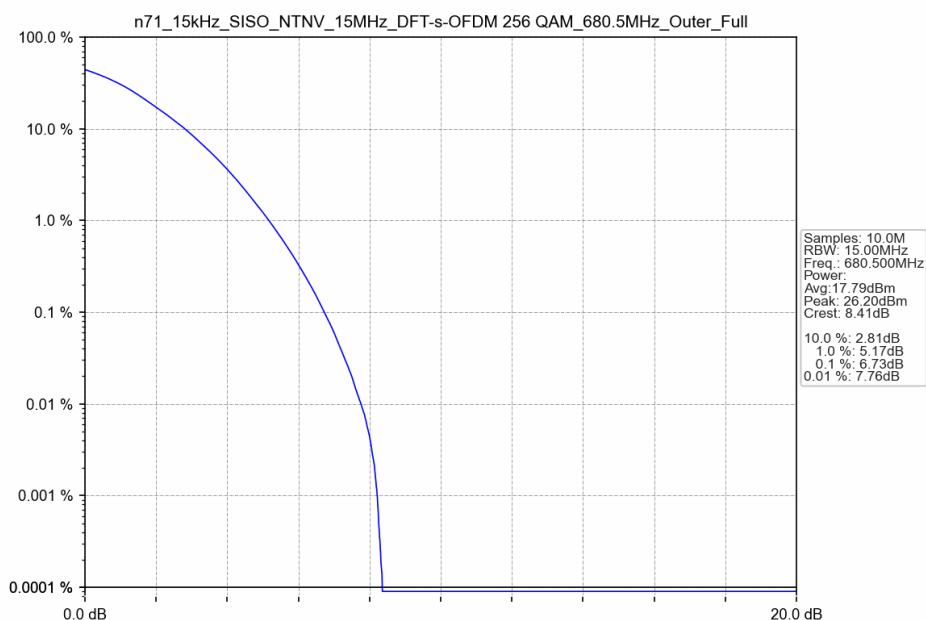
n71_15kHz_SISO_NTNV_15MHz_DFT-s-OFDM 256 QAM_680.5MHz_Outer_Full
