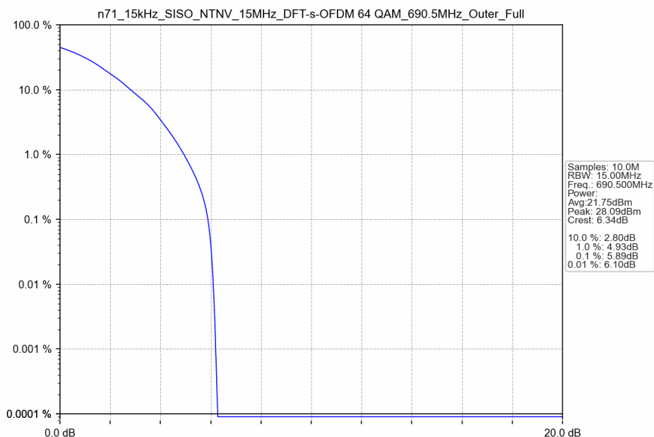
n71_15kHz_SISO_NTNV_15MHz_DFT-s-OFDM 64 QAM_690.5MHz_Outer_Full
