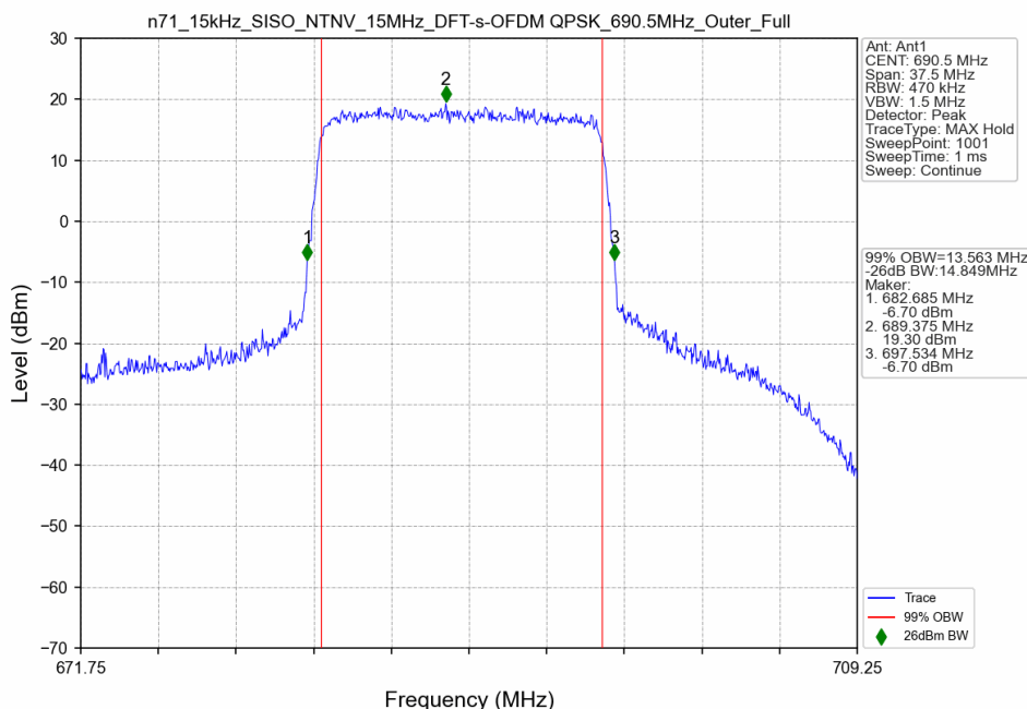
n71_15kHz_SISO_NTNV_15MHz_DFT-s-OFDM QPSK_690.5MHz_Outer_Full
