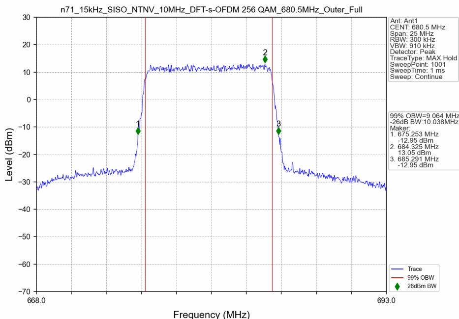
n71_15kHz_SISO_NTNV_10MHz_DFT-s-OFDM 256 QAM_680.5MHz_Outer_Full
