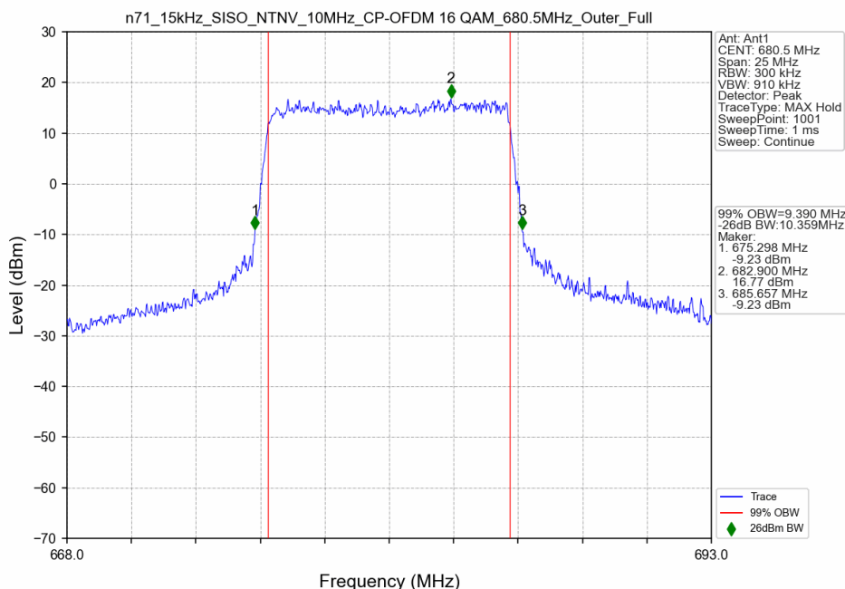
n71_15kHz_SISO_NTNV_10MHz_CP-OFDM 16 QAM_680.5MHz_Outer_Full
