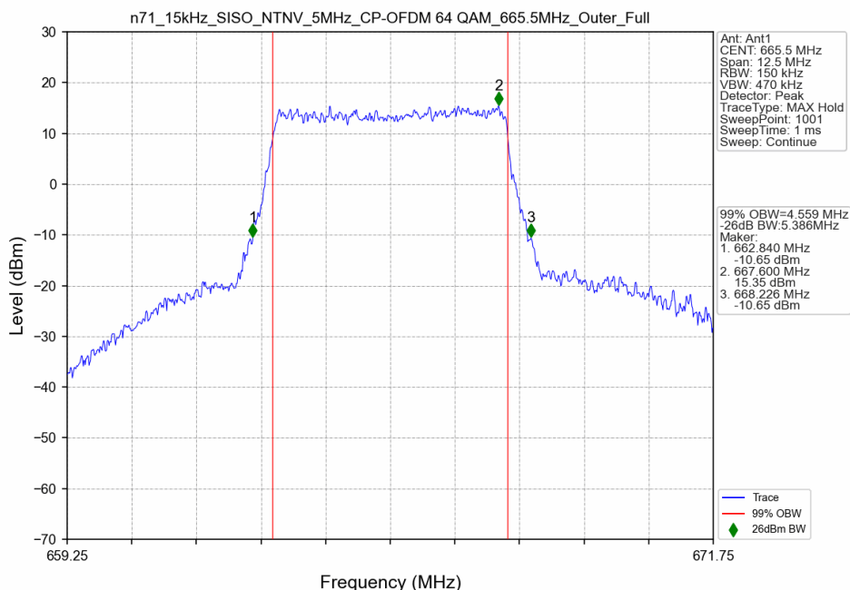
n71_15kHz_SISO_NTNV_5MHz_CP-OFDM 64 QAM_665.5MHz_Outer_Full
