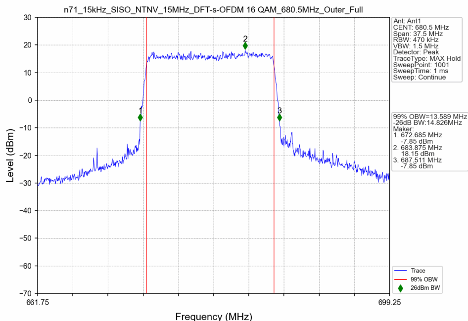
n71_15kHz_SISO_NTNV_15MHz_DFT-s-OFDM 16 QAM_680.5MHz_Outer_Full
