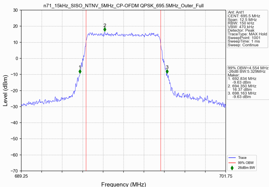
n71_15kHz_SISO_NTNV_5MHz_CP-OFDM QPSK_695.5MHz_Outer_Full
