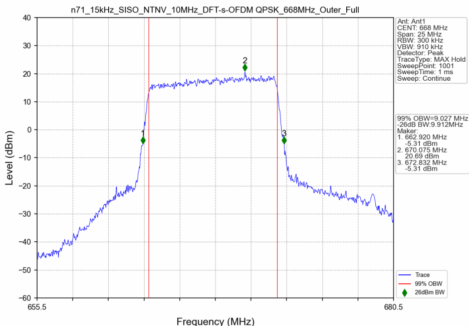
n71_15kHz_SISO_NTNV_10MHz_DFT-s-OFDM QPSK_668MHz_Outer_Full
