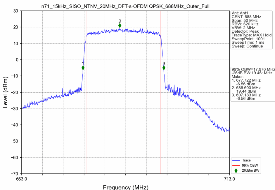
n71_15kHz_SISO_NTNV_20MHz_DFT-s-OFDM QPSK_688MHz_Outer_Full
