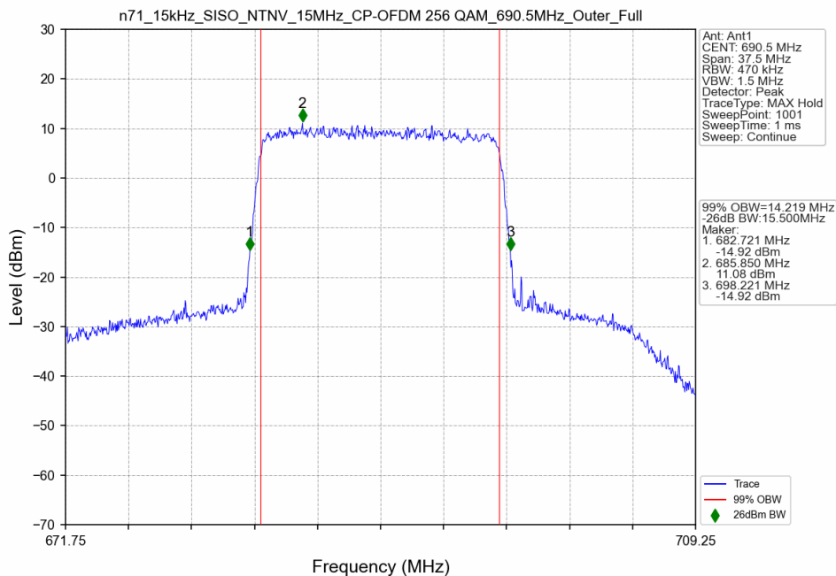
n71_15kHz_SISO_NTNV_15MHz_CP-OFDM 256 QAM_690.5MHz_Outer_Full
