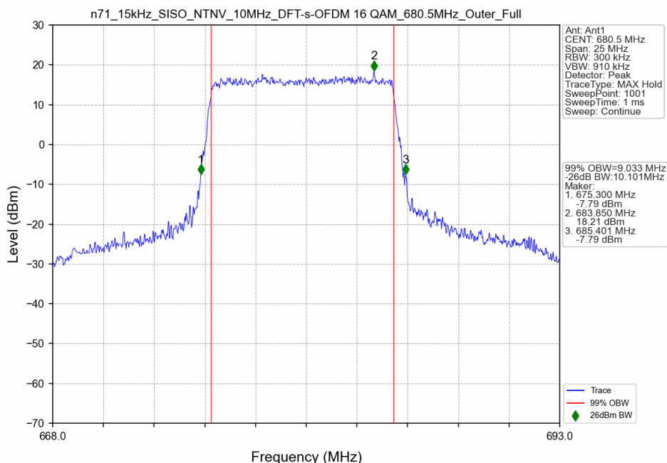
n71_15kHz_SISO_NTNV_10MHz_DFT-s-OFDM 16 QAM_680.5MHz_Outer_Full
