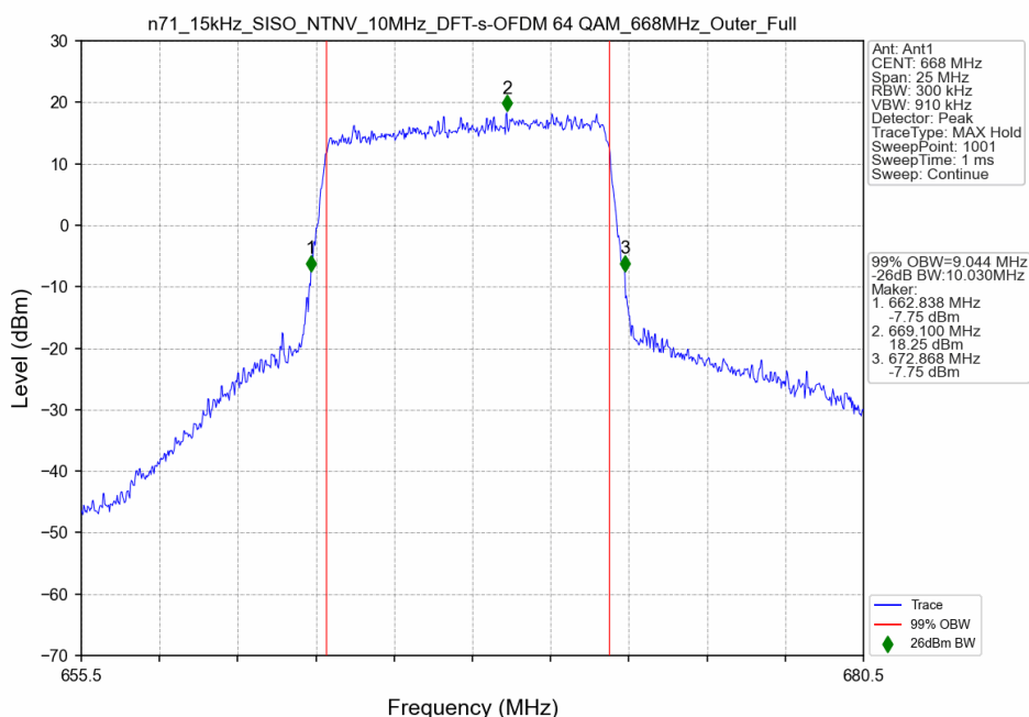
n71_15kHz_SISO_NTNV_10MHz_DFT-s-OFDM 64 QAM_668MHz_Outer_Full
