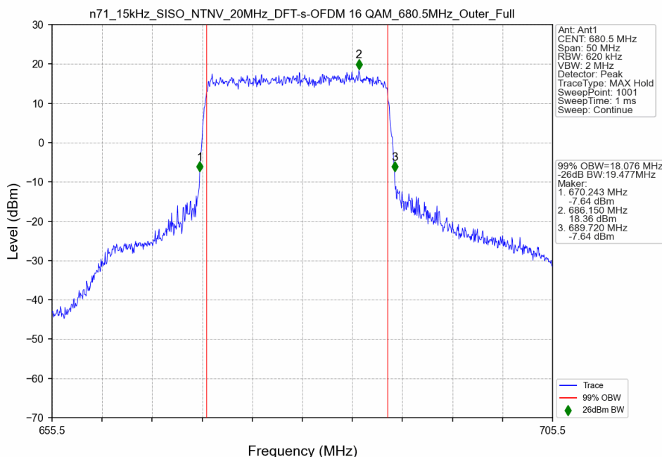
n71_15kHz_SISO_NTNV_20MHz_DFT-s-OFDM 16 QAM_680.5MHz_Outer_Full
