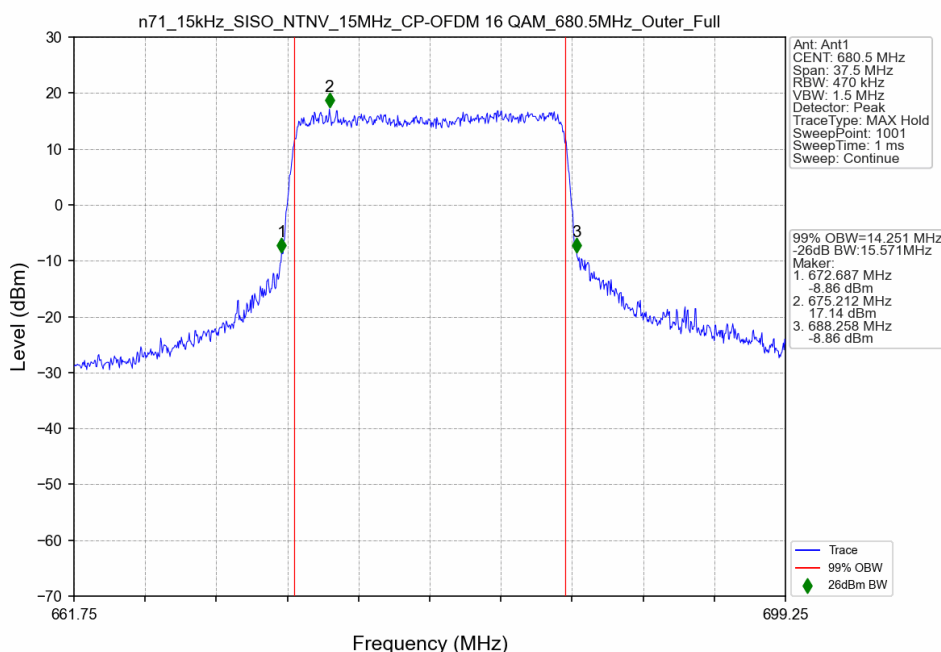
n71_15kHz_SISO_NTNV_15MHz_CP-OFDM 16 QAM_680.5MHz_Outer_Full
