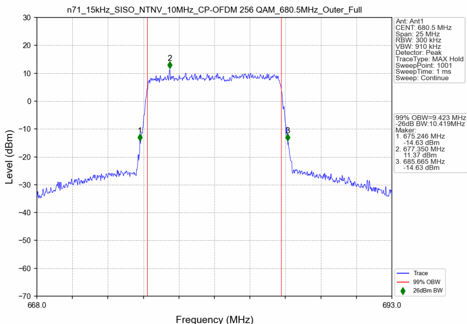
n71_15kHz_SISO_NTNV_10MHz_CP-OFDM 256 QAM_680.5MHz_Outer_Full
