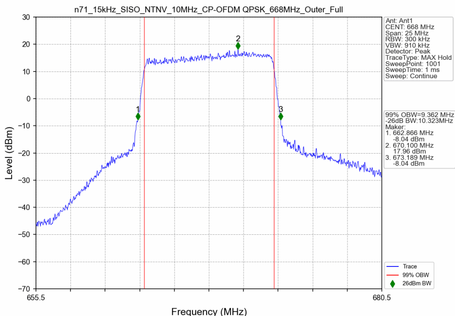
n71_15kHz_SISO_NTNV_10MHz_CP-OFDM QPSK_668MHz_Outer_Full
