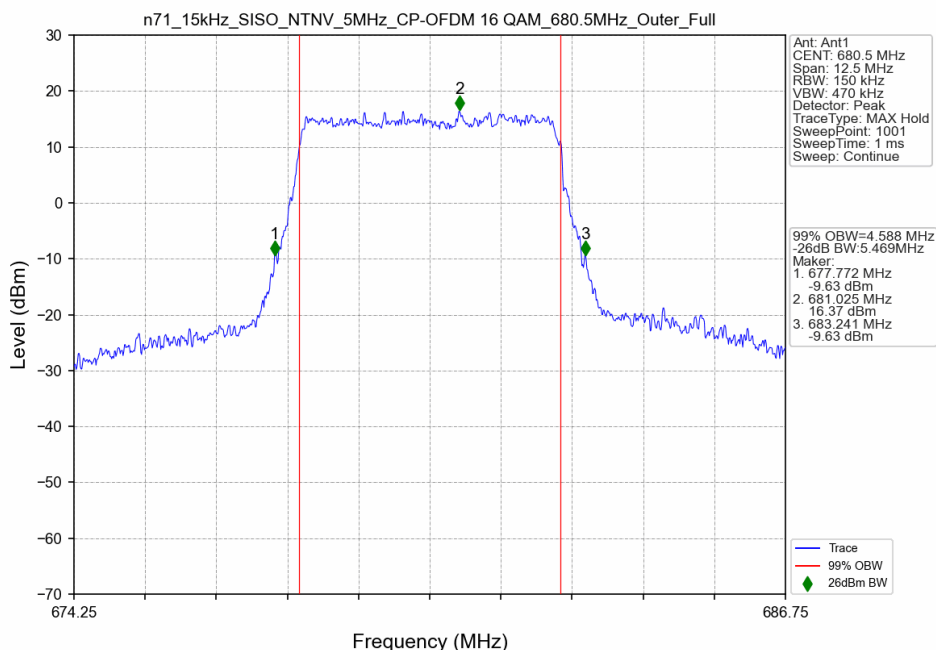
n71_15kHz_SISO_NTNV_5MHz_CP-OFDM 16 QAM_680.5MHz_Outer_Full
