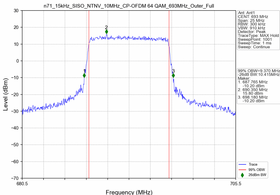
n71_15kHz_SISO_NTNV_10MHz_CP-OFDM 64 QAM_693MHz_Outer_Full
