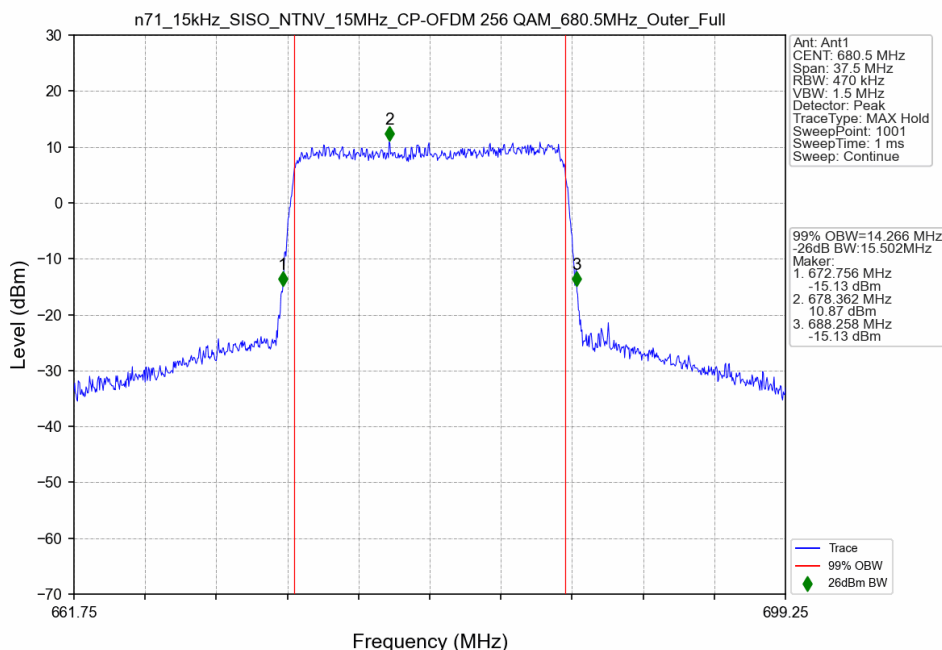
n71_15kHz_SISO_NTNV_15MHz_CP-OFDM 256 QAM_680.5MHz_Outer_Full
