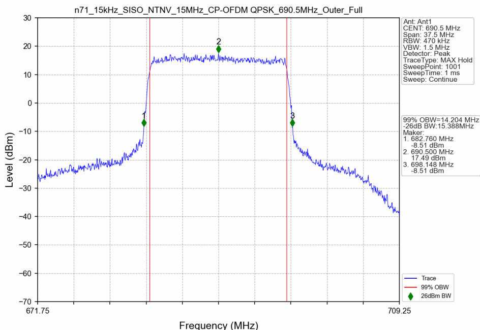
n71_15kHz_SISO_NTNV_15MHz_CP-OFDM QPSK_690.5MHz_Outer_Full
