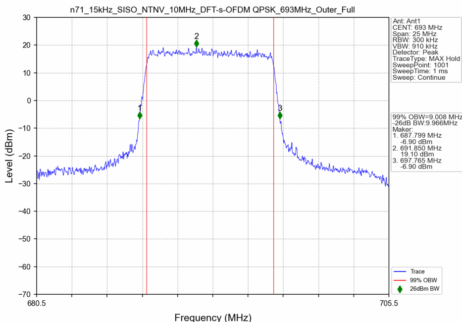
n71_15kHz_SISO_NTNV_10MHz_DFT-s-OFDM QPSK_693MHz_Outer_Full
