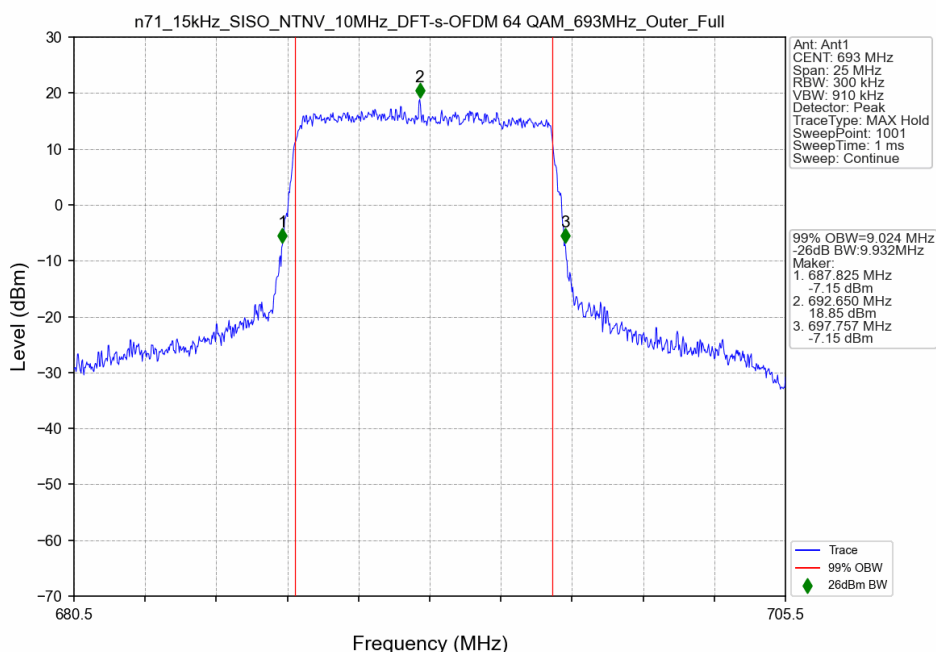
n71_15kHz_SISO_NTNV_10MHz_DFT-s-OFDM 64 QAM_693MHz_Outer_Full
