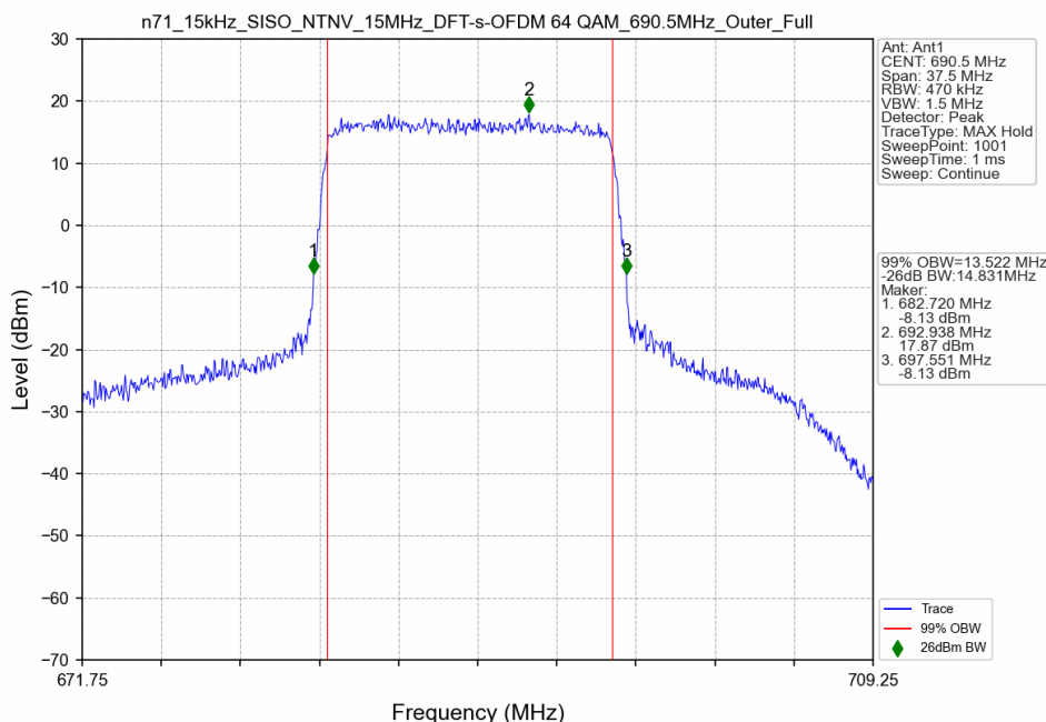
n71_15kHz_SISO_NTNV_15MHz_DFT-s-OFDM 64 QAM_690.5MHz_Outer_Full
