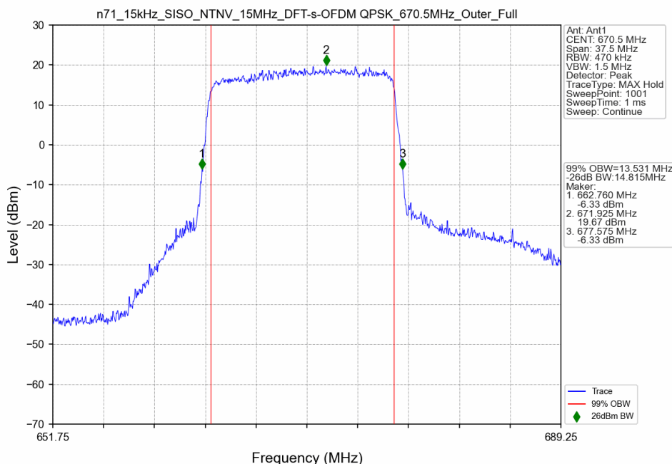
n71_15kHz_SISO_NTNV_15MHz_DFT-s-OFDM QPSK_670.5MHz_Outer_Full
