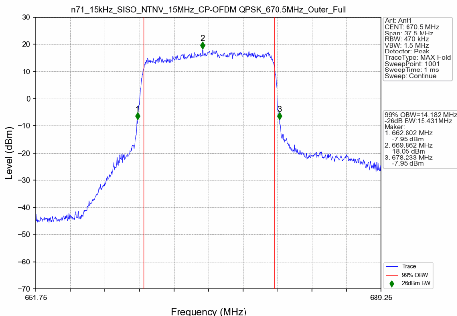
n71_15kHz_SISO_NTNV_15MHz_CP-OFDM QPSK_670.5MHz_Outer_Full
