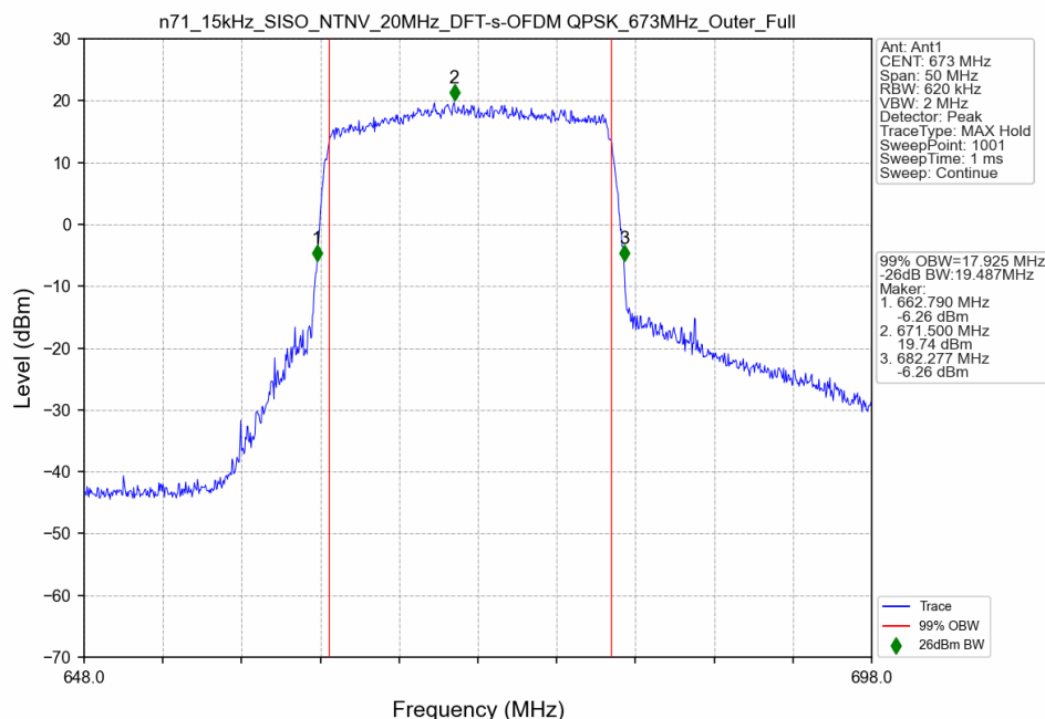
n71_15kHz_SISO_NTNV_20MHz_DFT-s-OFDM QPSK_673MHz_Outer_Full
