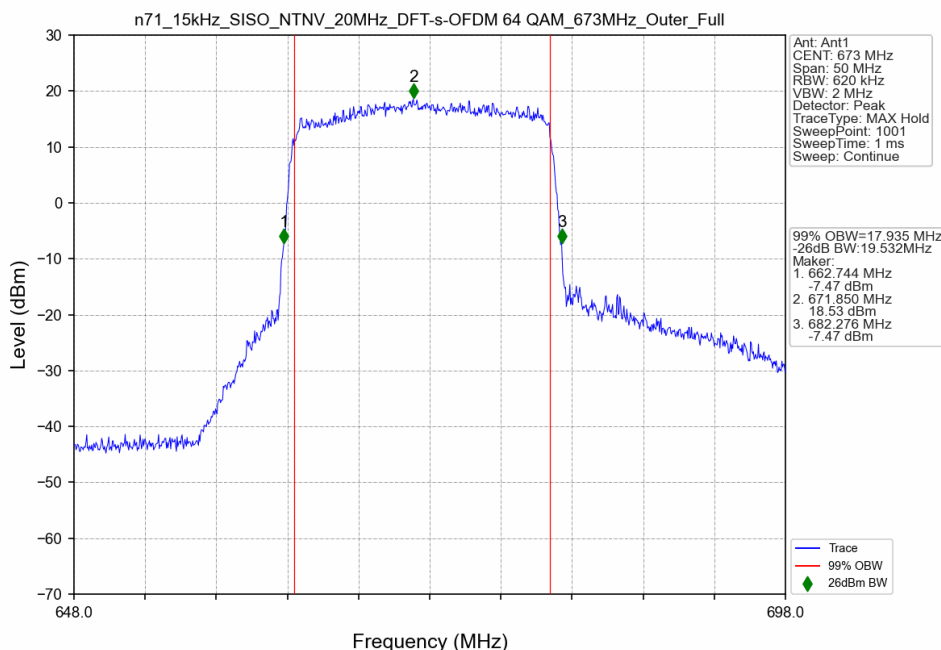
n71_15kHz_SISO_NTNV_20MHz_DFT-s-OFDM 64 QAM_673MHz_Outer_Full
