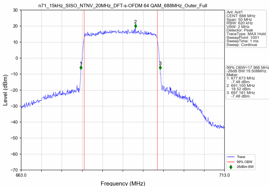
n71_15kHz_SISO_NTNV_20MHz_DFT-s-OFDM 64 QAM_688MHz_Outer_Full
