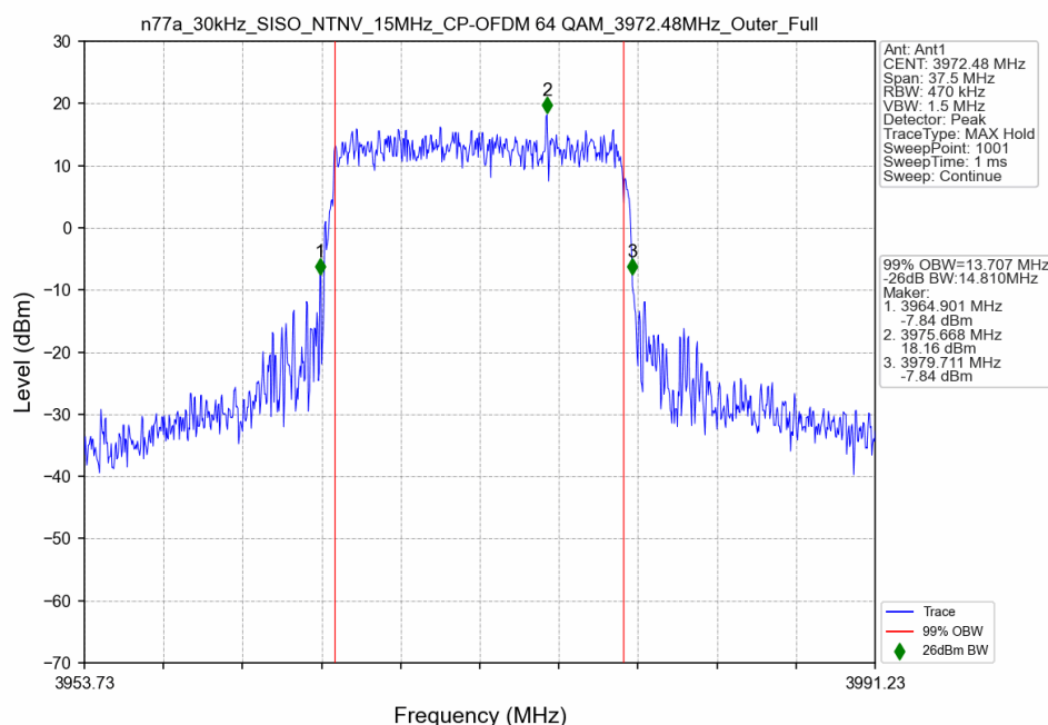
n77a_30kHz_SISO_NTNV_15MHz_CP-OFDM 64 QAM_3972.48MHz_Outer_Full
