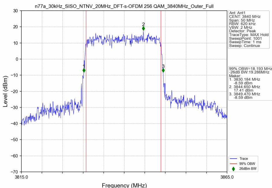
n77a_30kHz_SISO_NTNV_20MHz_DFT-s-OFDM 256 QAM_3840MHz_Outer_Full
