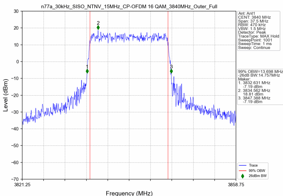
n77a_30kHz_SISO_NTNV_15MHz_CP-OFDM 16 QAM_3840MHz_Outer_Full
