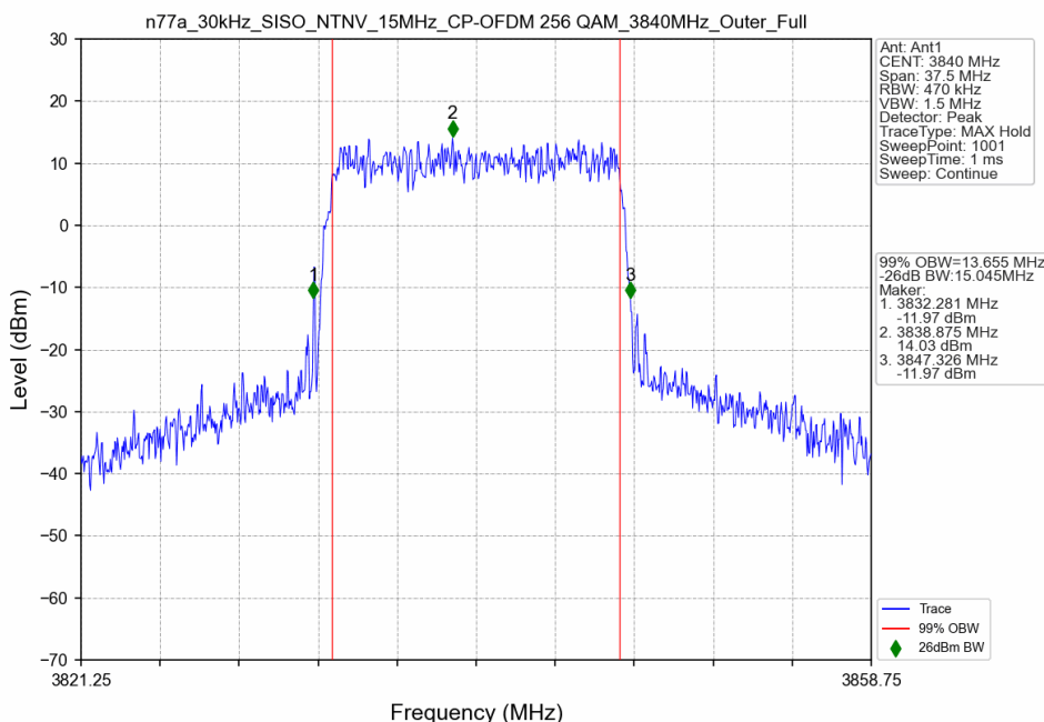
n77a_30kHz_SISO_NTNV_15MHz_CP-OFDM 256 QAM_3840MHz_Outer_Full
