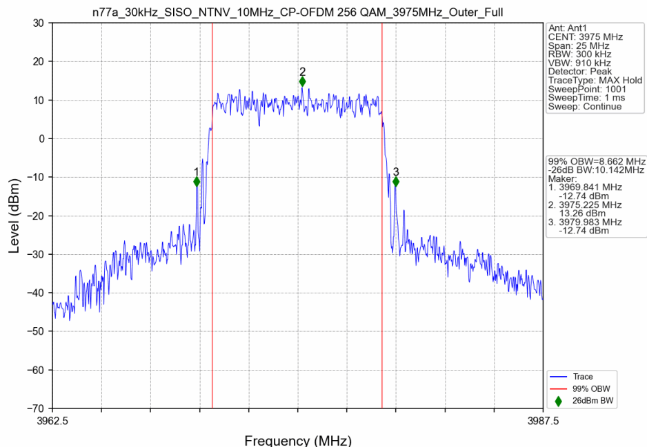
n77a_30kHz_SISO_NTNV_10MHz_CP-OFDM 256 QAM_3975MHz_Outer_Full
