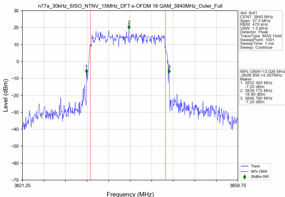
n77a_30kHz_SISO_NTNV_15MHz_DFT-s-OFDM 16 QAM_3840MHz_Outer_Full
