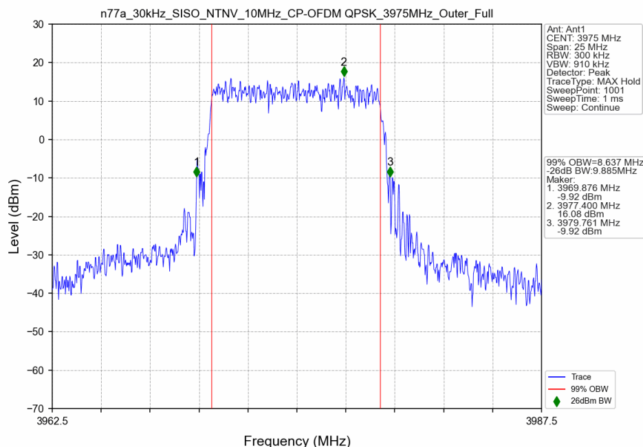
n77a_30kHz_SISO_NTNV_10MHz_CP-OFDM QPSK_3975MHz_Outer_Full
