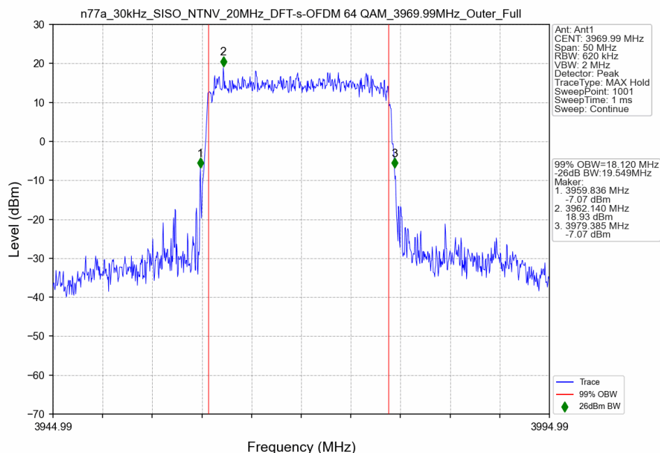
n77a_30kHz_SISO_NTNV_20MHz_DFT-s-OFDM 64 QAM_3969.99MHz_Outer_Full
