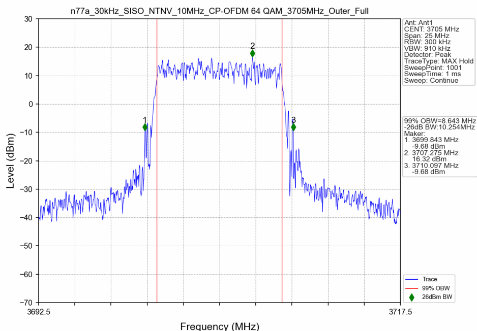
n77a_30kHz_SISO_NTNV_10MHz_CP-OFDM 64 QAM_3705MHz_Outer_Full
