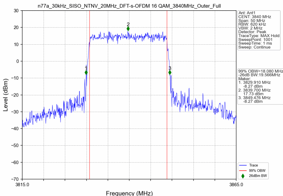
n77a_30kHz_SISO_NTNV_20MHz_DFT-s-OFDM 16 QAM_3840MHz_Outer_Full
