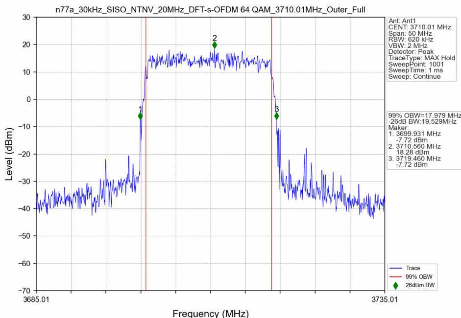
n77a_30kHz_SISO_NTNV_20MHz_DFT-s-OFDM 64 QAM_3710.01MHz_Outer_Full
