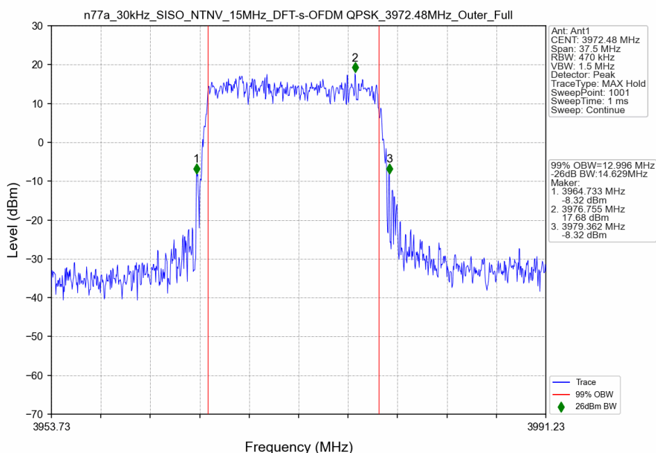
n77a_30kHz_SISO_NTNV_15MHz_DFT-s-OFDM QPSK_3972.48MHz_Outer_Full
