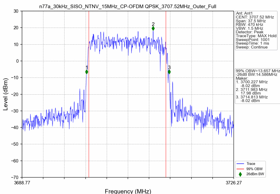
n77a_30kHz_SISO_NTNV_15MHz_CP-OFDM QPSK_3707.52MHz_Outer_Full
