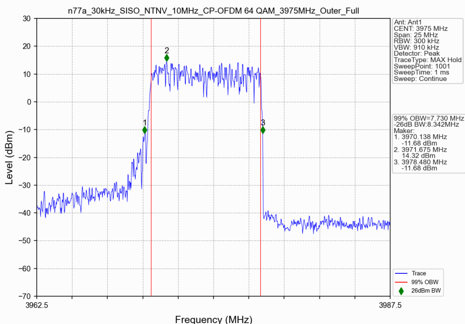
n77a_30kHz_SISO_NTNV_10MHz_CP-OFDM 64 QAM_3975MHz_Outer_Full
