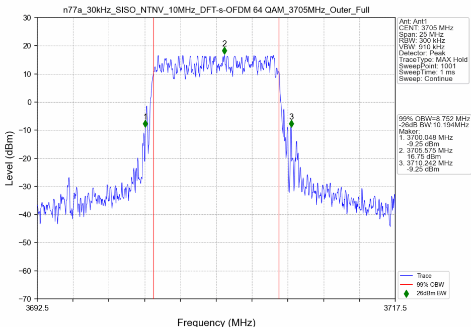
n77a_30kHz_SISO_NTNV_10MHz_DFT-s-OFDM 64 QAM_3705MHz_Outer_Full
