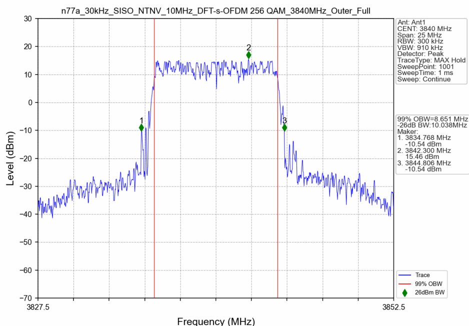
n77a_30kHz_SISO_NTNV_10MHz_DFT-s-OFDM 256 QAM_3840MHz_Outer_Full
