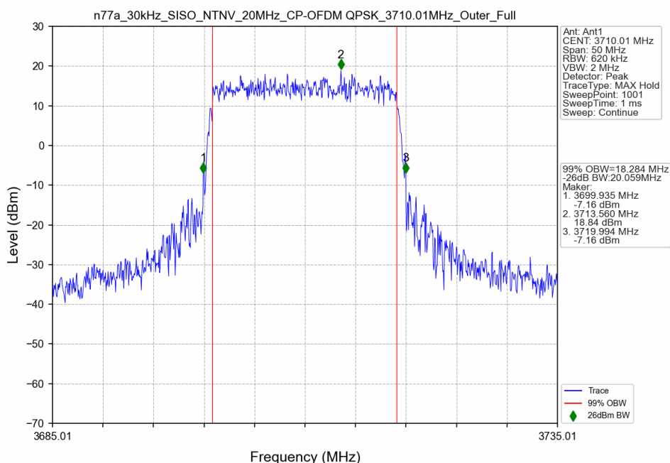
n77a_30kHz_SISO_NTNV_20MHz_CP-OFDM QPSK_3710.01MHz_Outer_Full
