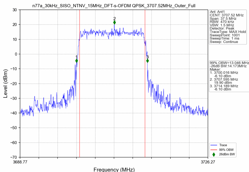
n77a_30kHz_SISO_NTNV_15MHz_DFT-s-OFDM QPSK_3707.52MHz_Outer_Full
