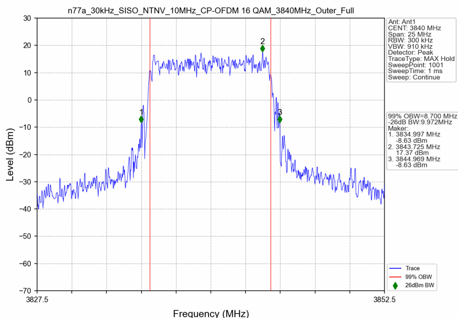
n77a_30kHz_SISO_NTNV_10MHz_CP-OFDM 16 QAM_3840MHz_Outer_Full
