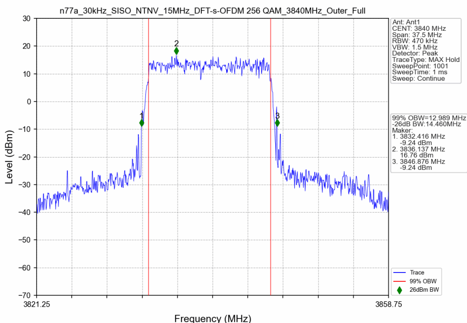
n77a_30kHz_SISO_NTNV_15MHz_DFT-s-OFDM 256 QAM_3840MHz_Outer_Full
