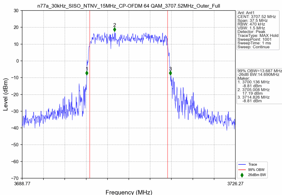
n77a_30kHz_SISO_NTNV_15MHz_CP-OFDM 64 QAM_3707.52MHz_Outer_Full
