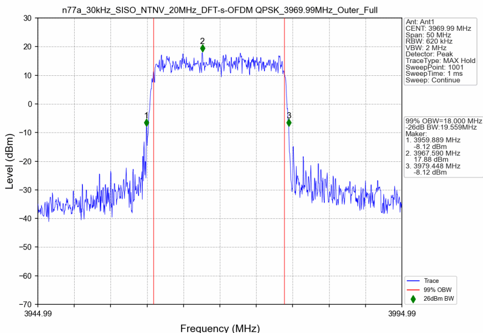
n77a_30kHz_SISO_NTNV_20MHz_DFT-s-OFDM QPSK_3969.99MHz_Outer_Full
