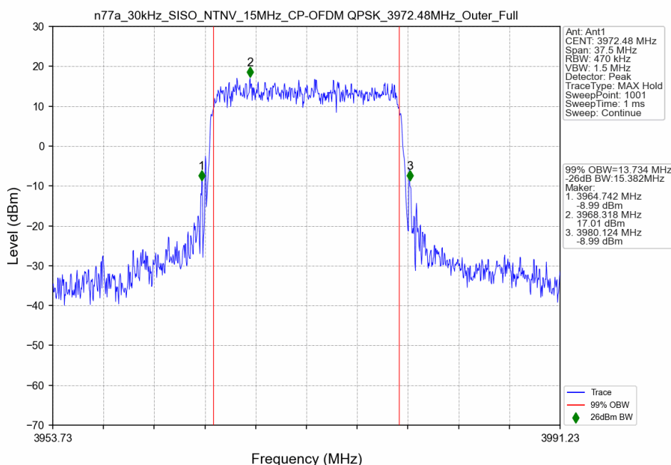
n77a_30kHz_SISO_NTNV_15MHz_CP-OFDM QPSK_3972.48MHz_Outer_Full
