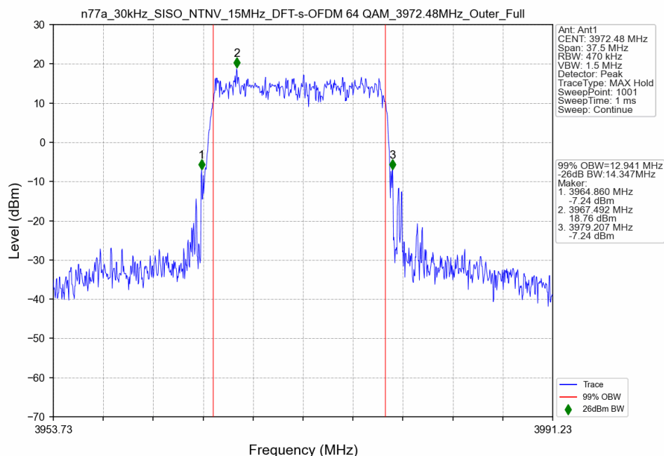
n77a_30kHz_SISO_NTNV_15MHz_DFT-s-OFDM 64 QAM_3972.48MHz_Outer_Full
