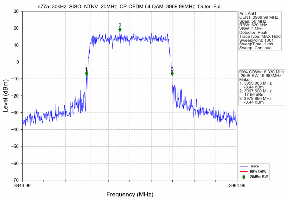
n77a_30kHz_SISO_NTNV_20MHz_CP-OFDM 64 QAM_3969.99MHz_Outer_Full
