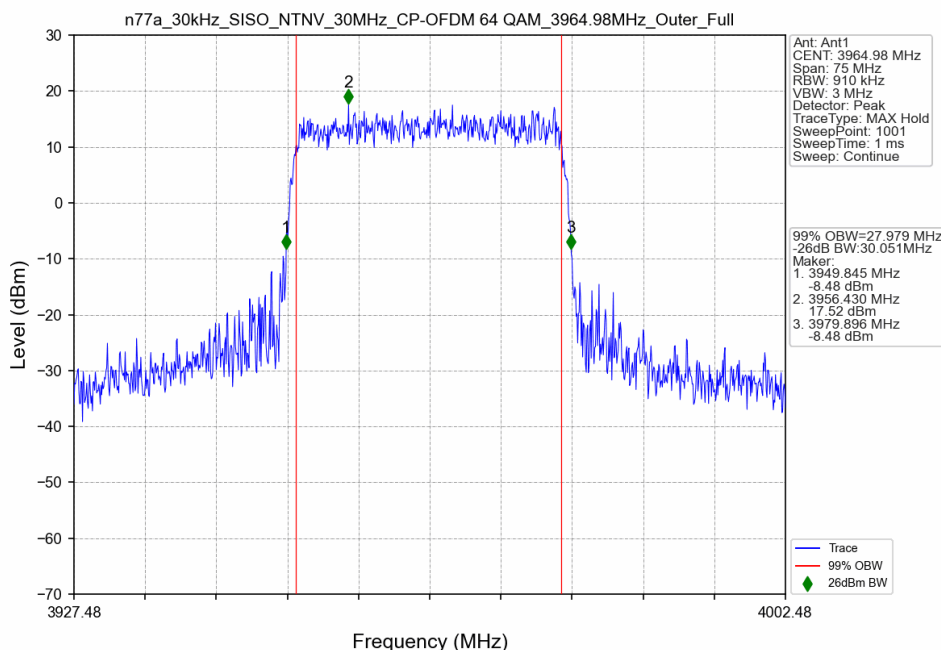
n77a_30kHz_SISO_NTNV_30MHz_CP-OFDM 64 QAM_3964.98MHz_Outer_Full
