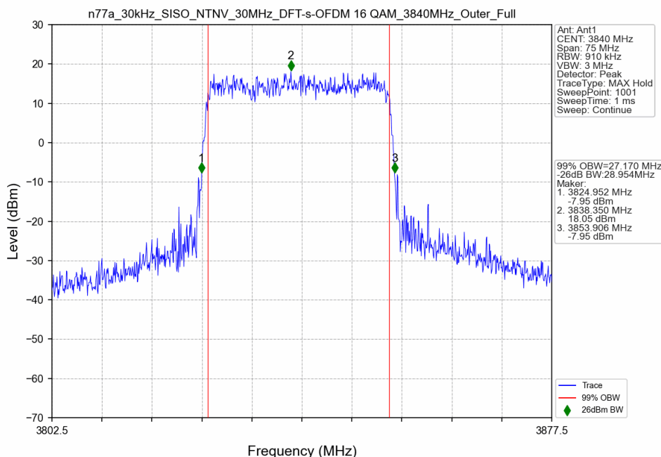
n77a_30kHz_SISO_NTNV_30MHz_DFT-s-OFDM 16 QAM_3840MHz_Outer_Full
