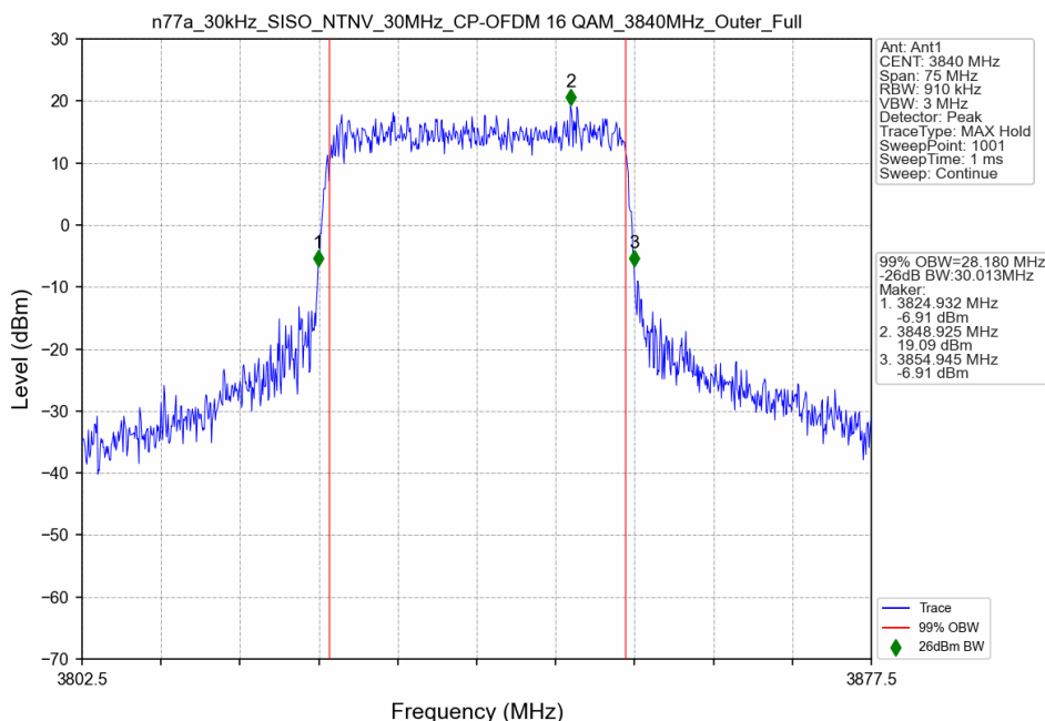
n77a_30kHz_SISO_NTNV_30MHz_CP-OFDM 16 QAM_3840MHz_Outer_Full
