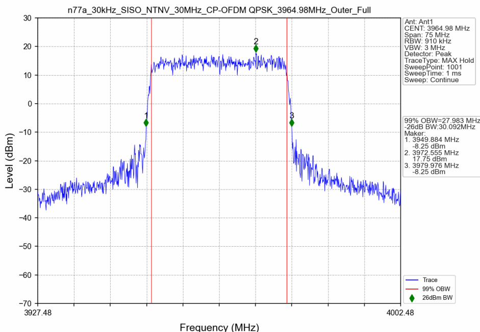
n77a_30kHz_SISO_NTNV_30MHz_CP-OFDM QPSK_3964.98MHz_Outer_Full
