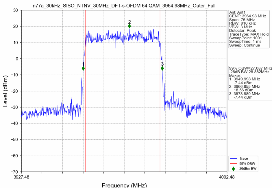
n77a_30kHz_SISO_NTNV_30MHz_DFT-s-OFDM 64 QAM_3964.98MHz_Outer_Full
