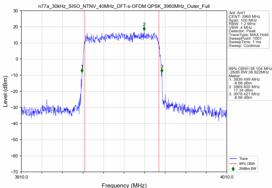
n77a_30kHz_SISO_NTNV_40MHz_DFT-s-OFDM QPSK_3960MHz_Outer_Full
