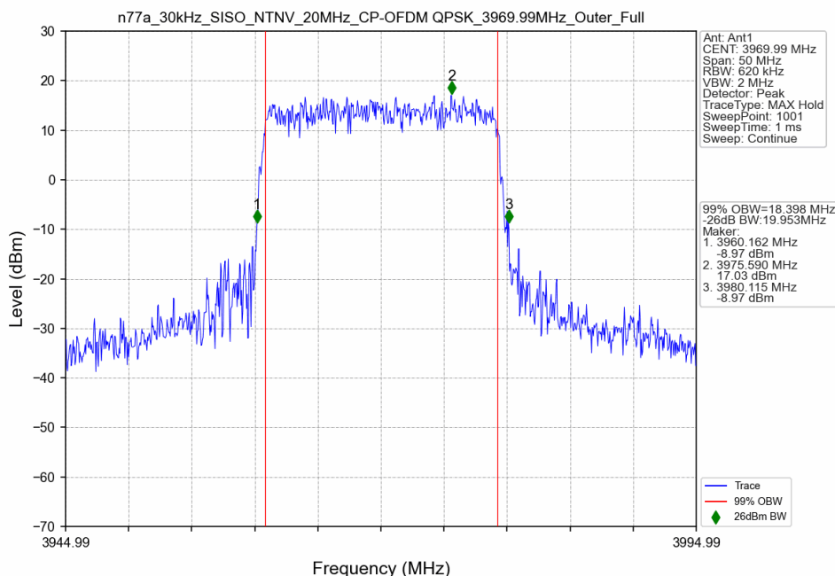
n77a_30kHz_SISO_NTNV_20MHz_CP-OFDM QPSK_3969.99MHz_Outer_Full
