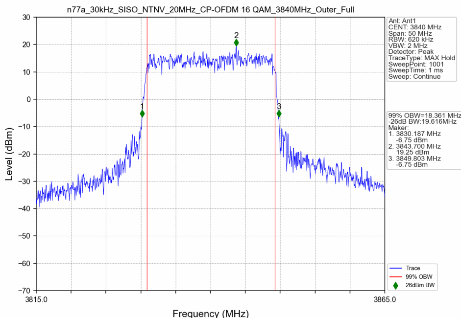
n77a_30kHz_SISO_NTNV_20MHz_CP-OFDM 16 QAM_3840MHz_Outer_Full
