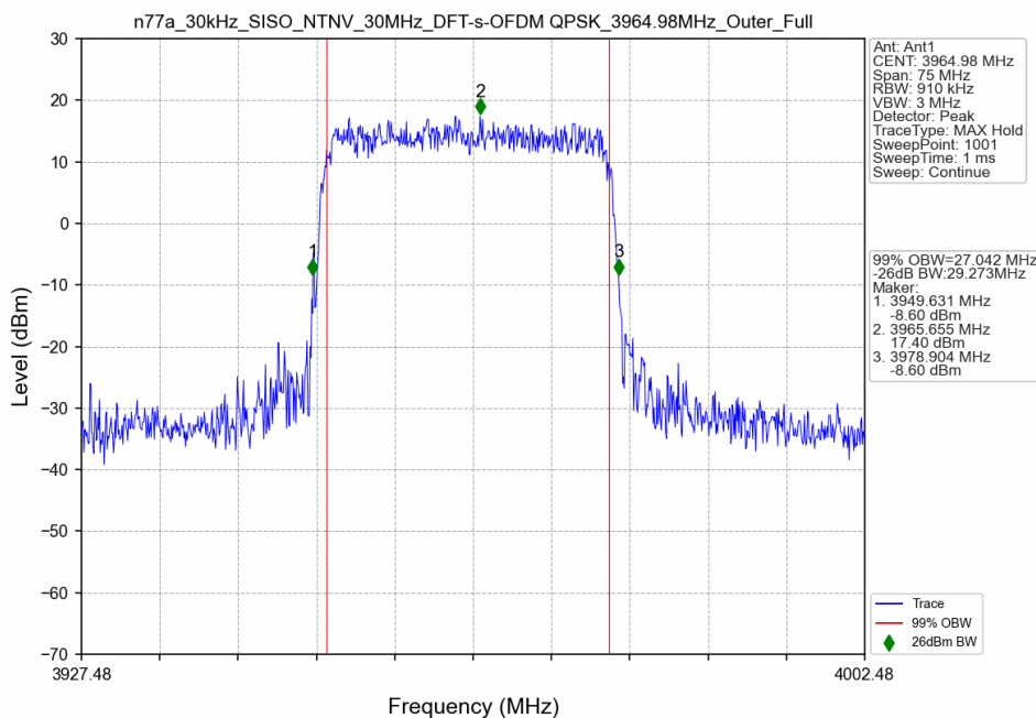
n77a_30kHz_SISO_NTNV_30MHz_DFT-s-OFDM QPSK_3964.98MHz_Outer_Full
