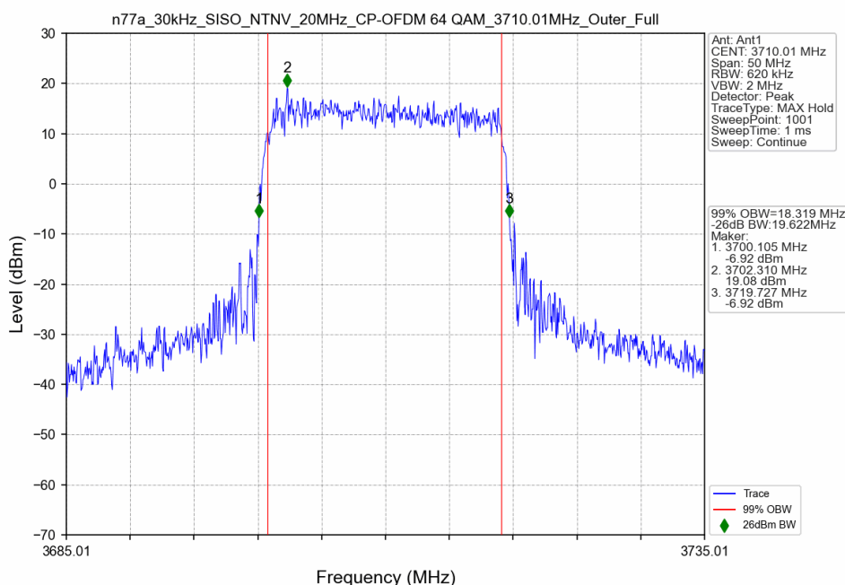
n77a_30kHz_SISO_NTNV_20MHz_CP-OFDM 64 QAM_3710.01MHz_Outer_Full
