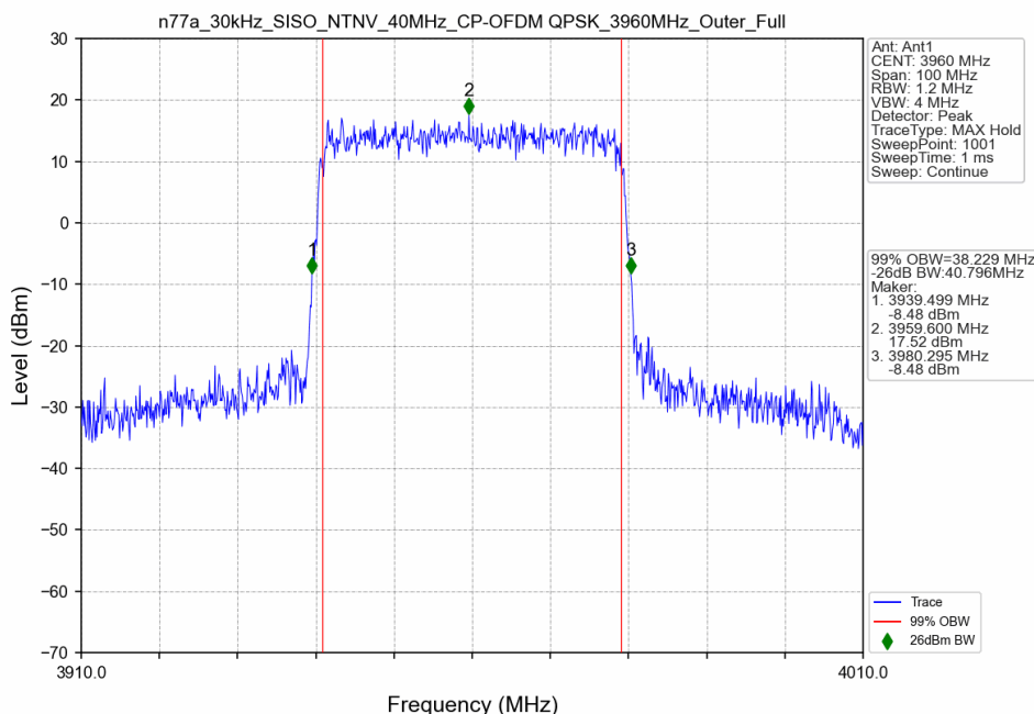
n77a_30kHz_SISO_NTNV_40MHz_CP-OFDM QPSK_3960MHz_Outer_Full
