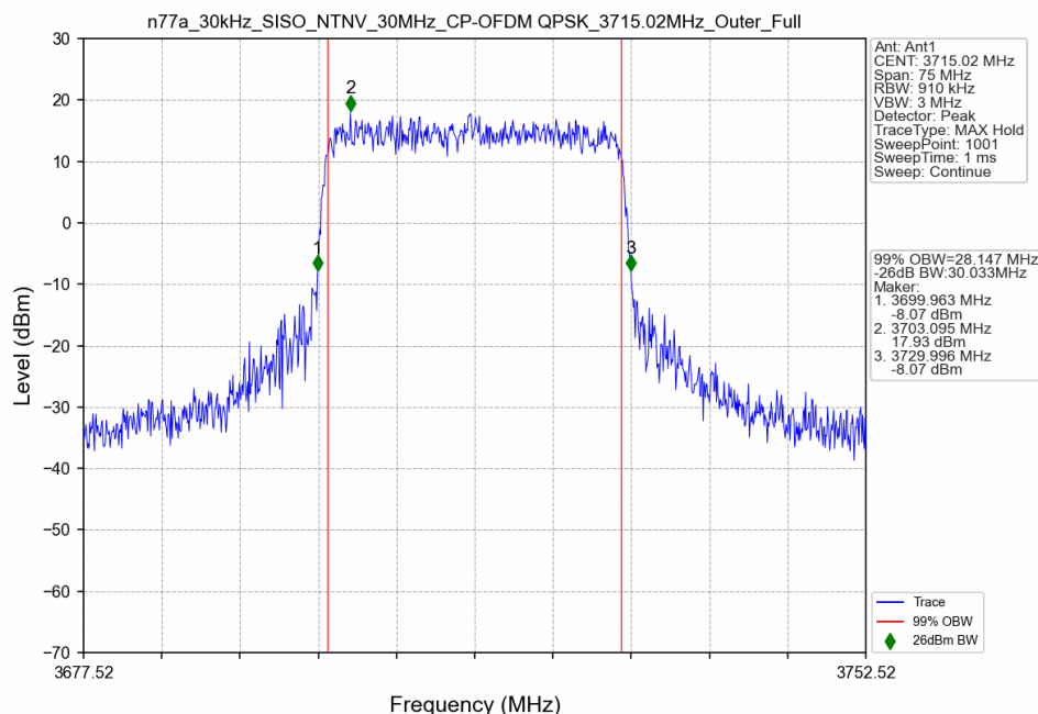
n77a_30kHz_SISO_NTNV_30MHz_CP-OFDM QPSK_3715.02MHz_Outer_Full
