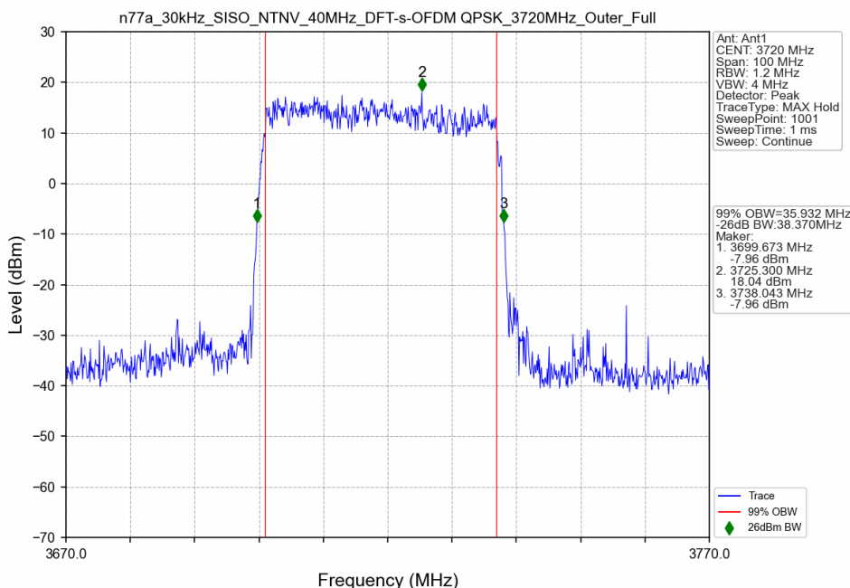
n77a_30kHz_SISO_NTNV_40MHz_DFT-s-OFDM QPSK_3720MHz_Outer_Full
