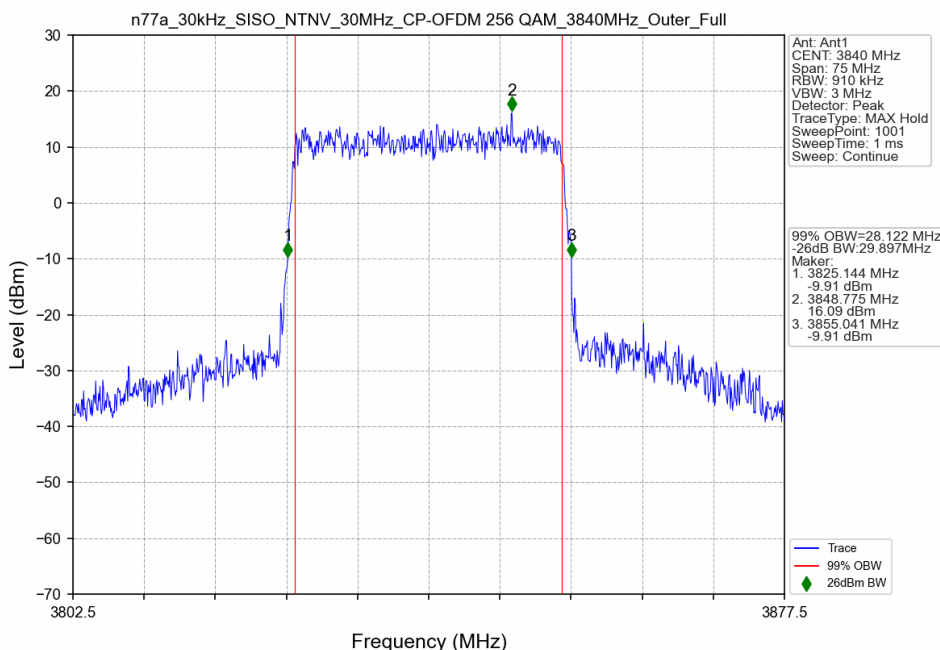
n77a_30kHz_SISO_NTNV_30MHz_CP-OFDM 256 QAM_3840MHz_Outer_Full
