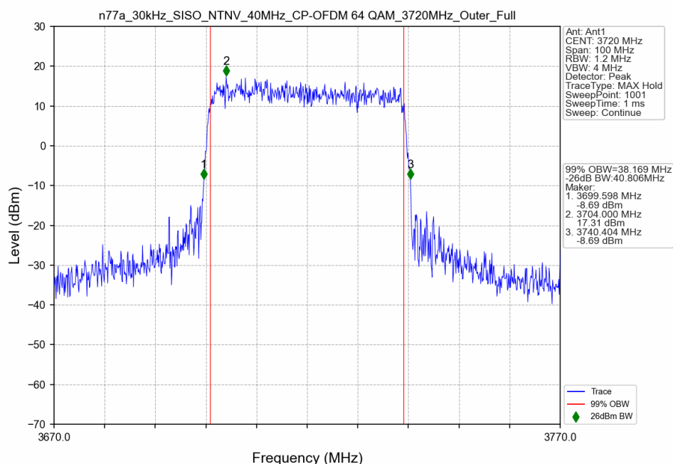
n77a_30kHz_SISO_NTNV_40MHz_CP-OFDM 64 QAM_3720MHz_Outer_Full
