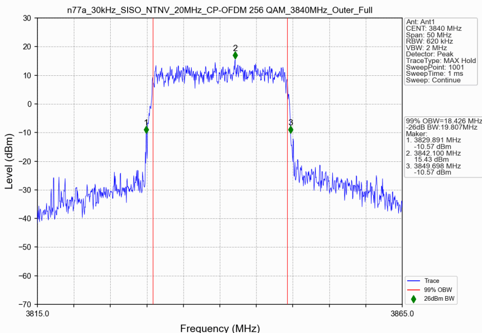
n77a_30kHz_SISO_NTNV_20MHz_CP-OFDM 256 QAM_3840MHz_Outer_Full
