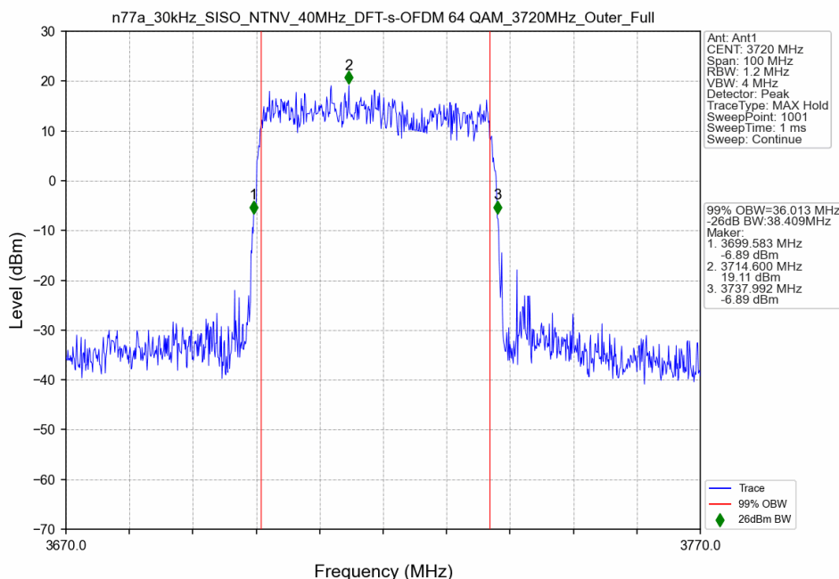
n77a_30kHz_SISO_NTNV_40MHz_DFT-s-OFDM 64 QAM_3720MHz_Outer_Full
