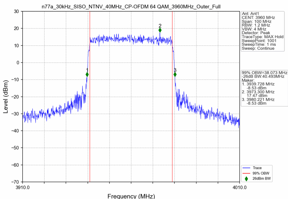
n77a_30kHz_SISO_NTNV_40MHz_CP-OFDM 64 QAM_3960MHz_Outer_Full
