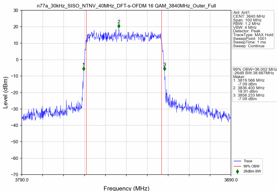
n77a_30kHz_SISO_NTNV_40MHz_DFT-s-OFDM 16 QAM_3840MHz_Outer_Full
