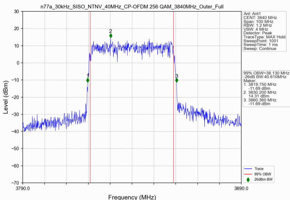
n77a_30kHz_SISO_NTNV_40MHz_CP-OFDM 256 QAM_3840MHz_Outer_Full
