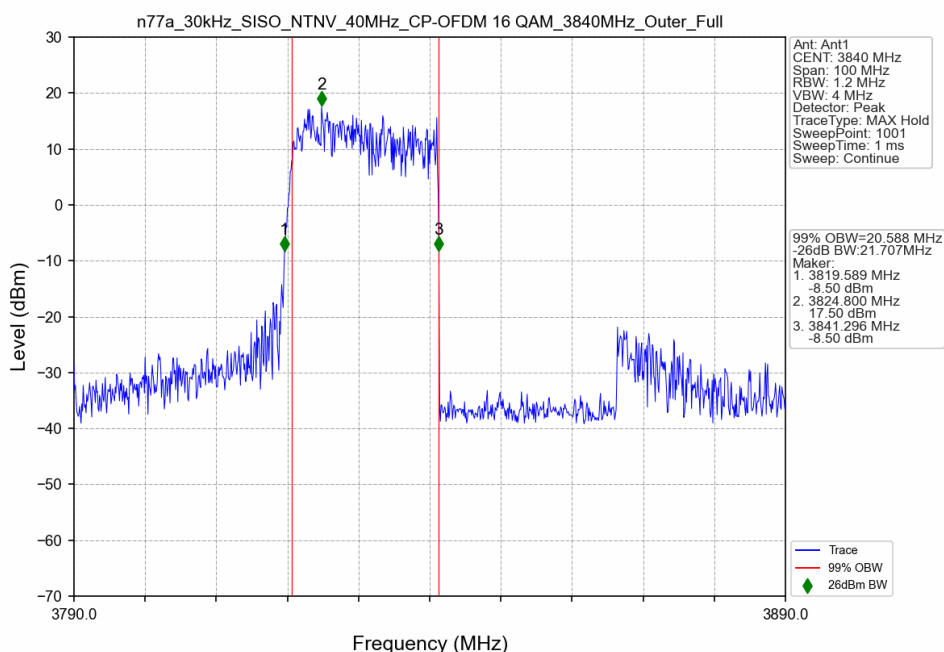
n77a_30kHz_SISO_NTNV_40MHz_CP-OFDM 16 QAM_3840MHz_Outer_Full
