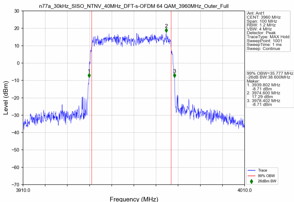
n77a_30kHz_SISO_NTNV_40MHz_DFT-s-OFDM 64 QAM_3960MHz_Outer_Full
