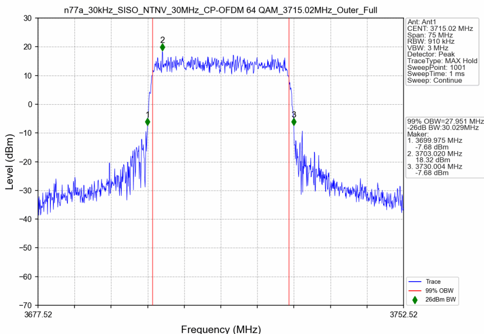
n77a_30kHz_SISO_NTNV_30MHz_CP-OFDM 64 QAM_3715.02MHz_Outer_Full
