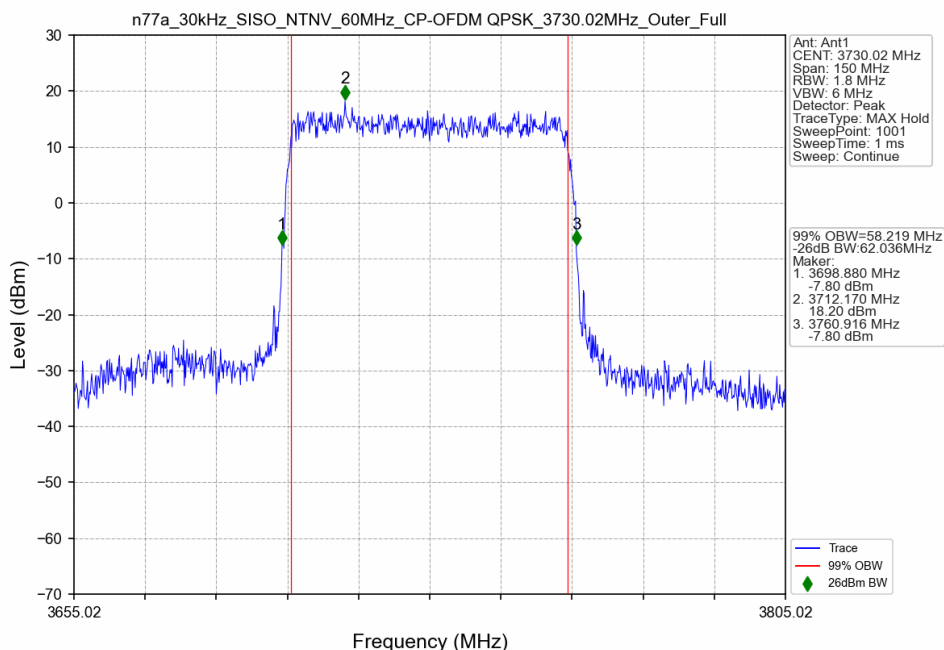
n77a_30kHz_SISO_NTNV_60MHz_CP-OFDM QPSK_3730.02MHz_Outer_Full
