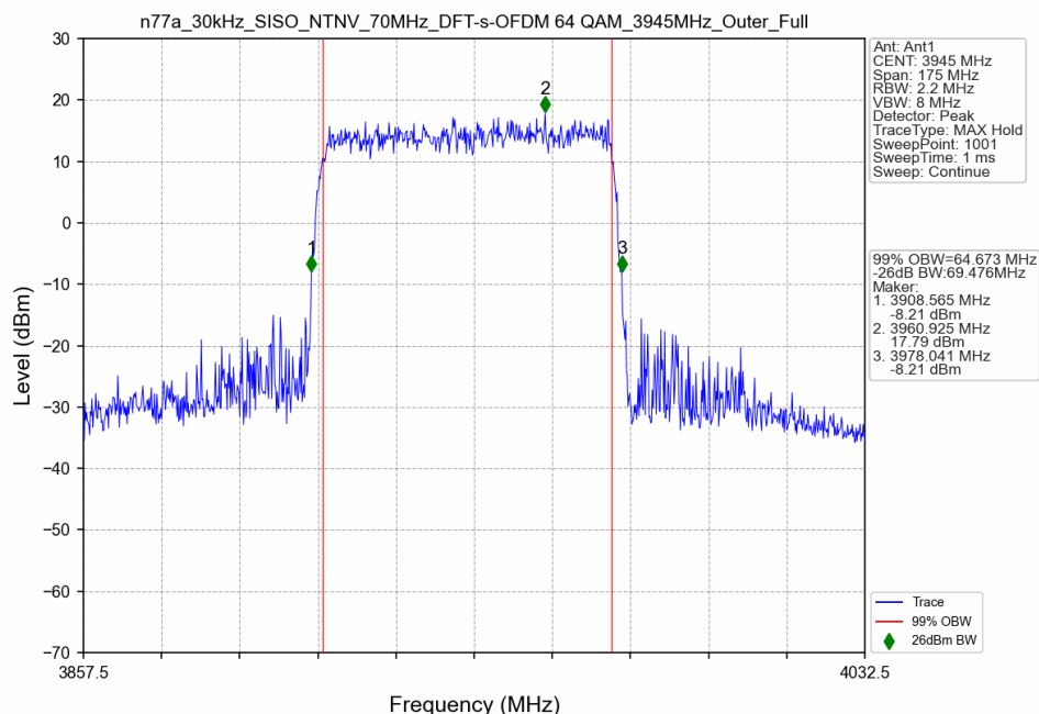
n77a_30kHz_SISO_NTNV_70MHz_DFT-s-OFDM 64 QAM_3945MHz_Outer_Full
