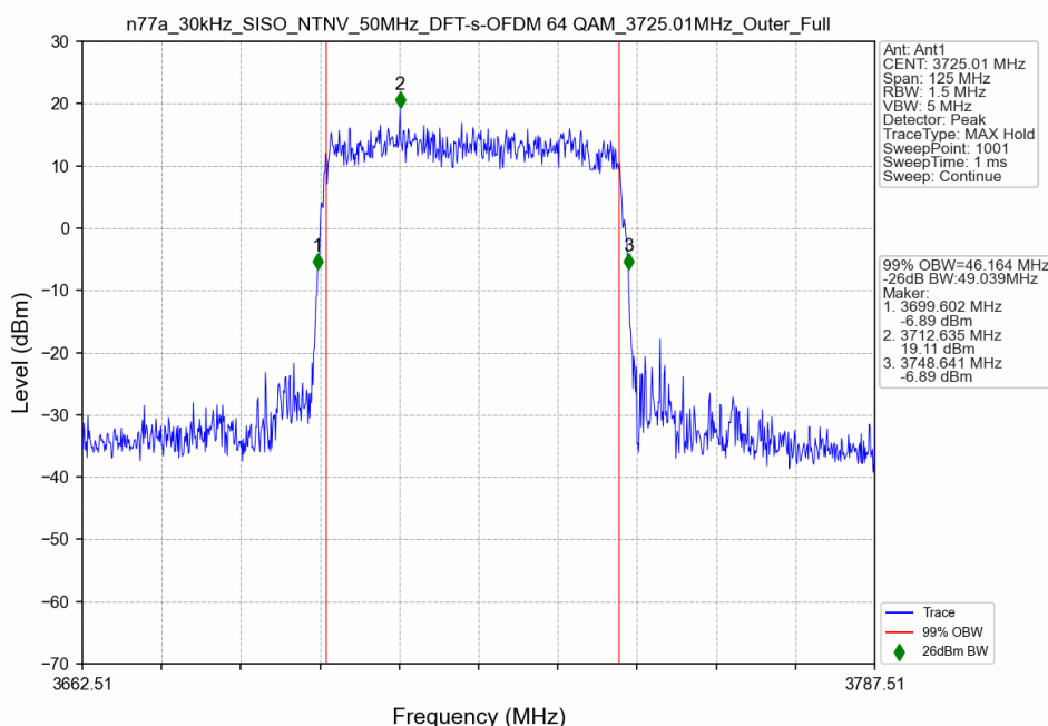
n77a_30kHz_SISO_NTNV_50MHz_DFT-s-OFDM 64 QAM_3725.01MHz_Outer_Full
