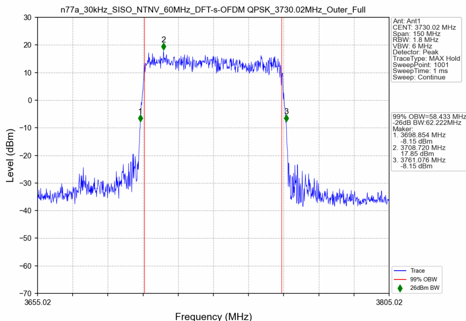
n77a_30kHz_SISO_NTNV_60MHz_DFT-s-OFDM QPSK_3730.02MHz_Outer_Full
