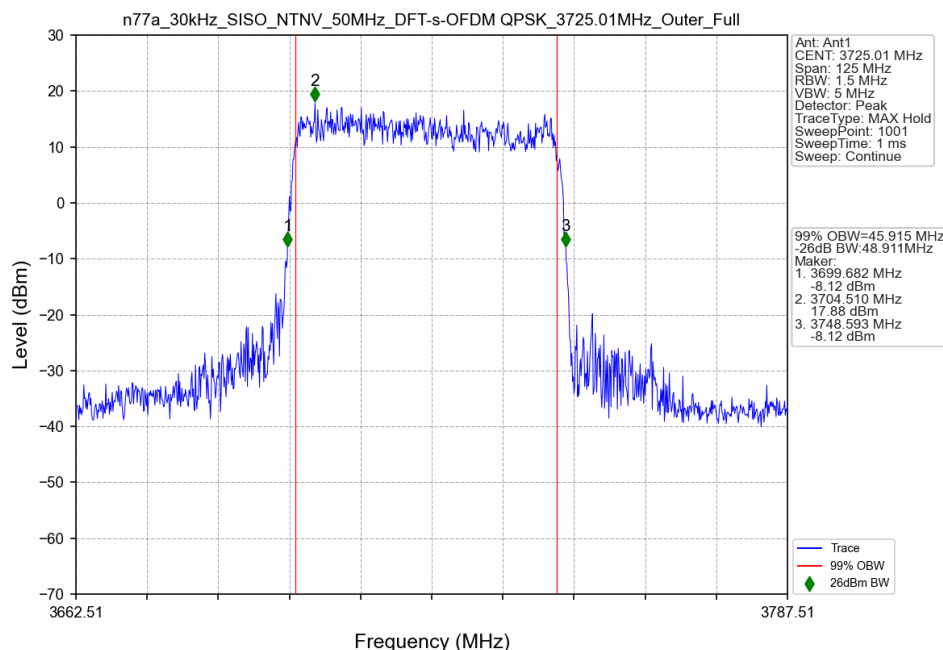
n77a_30kHz_SISO_NTNV_50MHz_DFT-s-OFDM QPSK_3725.01MHz_Outer_Full
