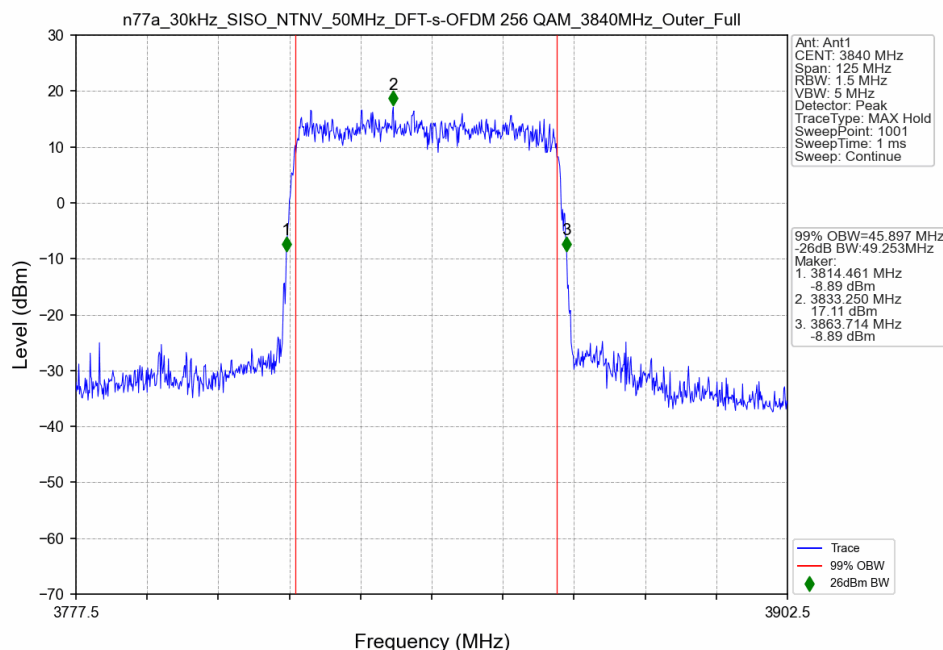
n77a_30kHz_SISO_NTNV_50MHz_DFT-s-OFDM 256 QAM_3840MHz_Outer_Full
