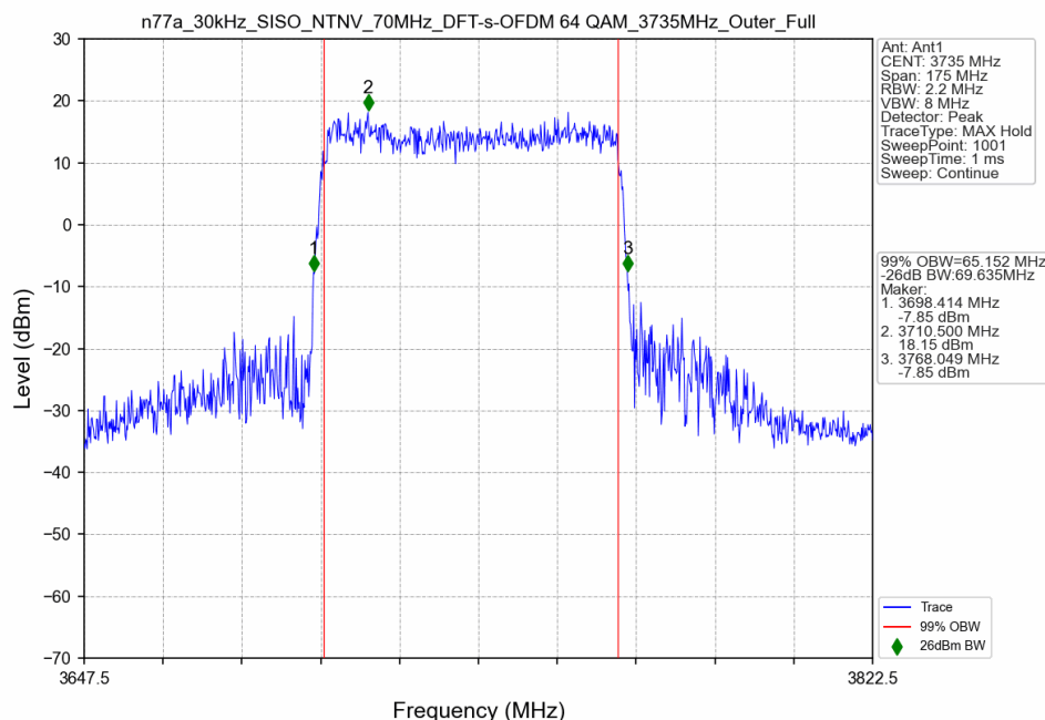
n77a_30kHz_SISO_NTNV_70MHz_DFT-s-OFDM 64 QAM_3735MHz_Outer_Full
