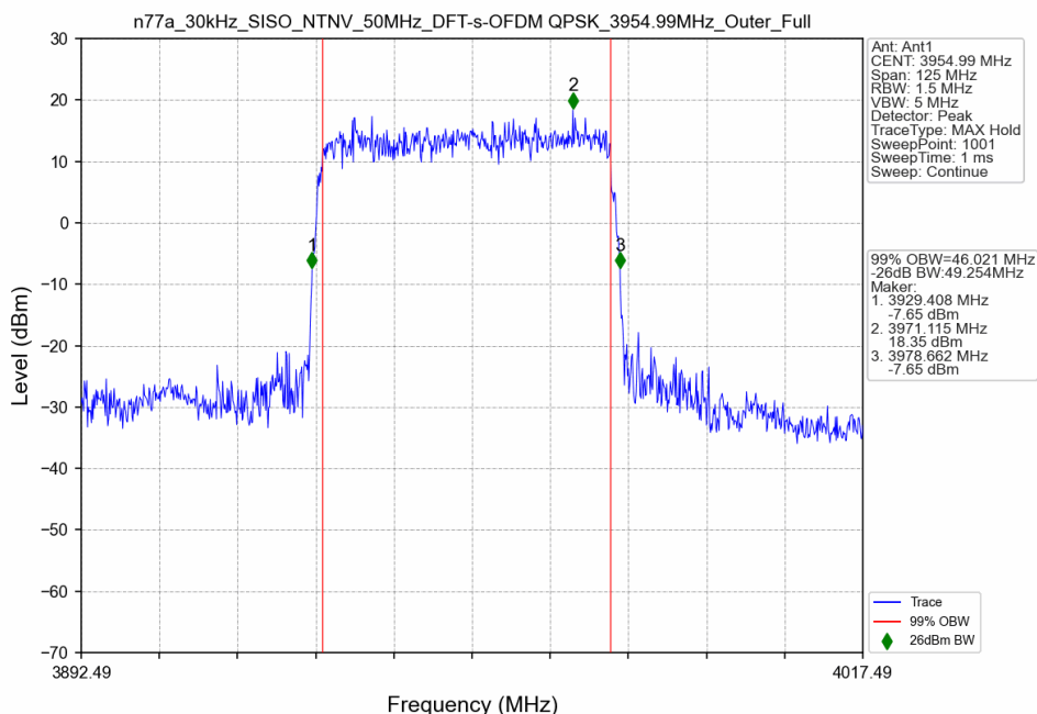
n77a_30kHz_SISO_NTNV_50MHz_DFT-s-OFDM QPSK_3954.99MHz_Outer_Full
