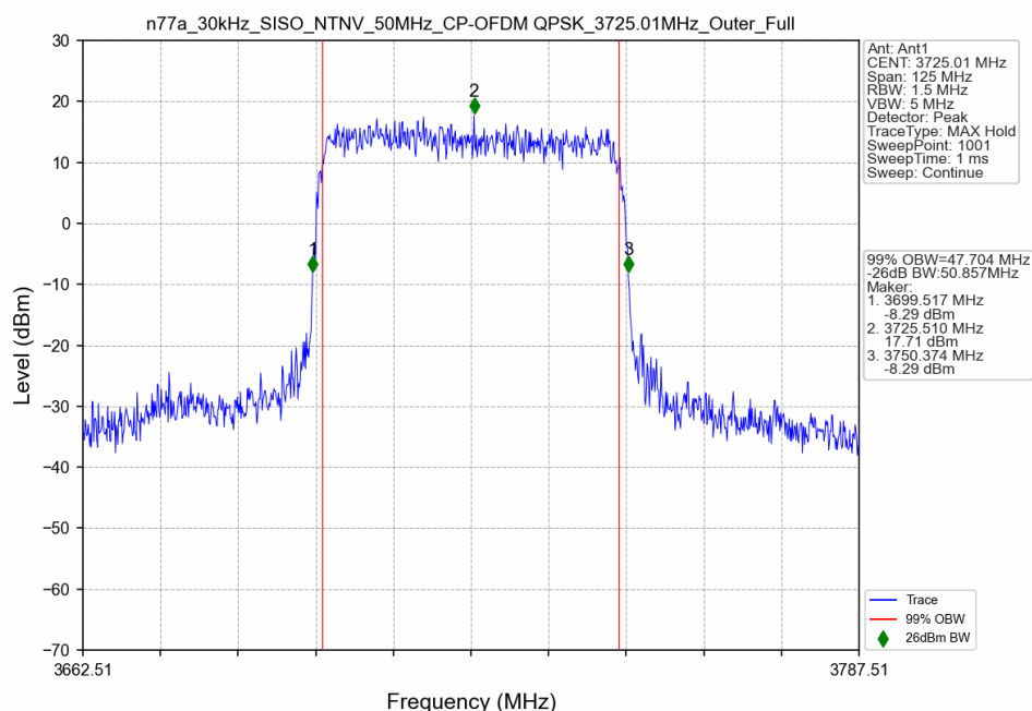
n77a_30kHz_SISO_NTNV_50MHz_CP-OFDM QPSK_3725.01MHz_Outer_Full
