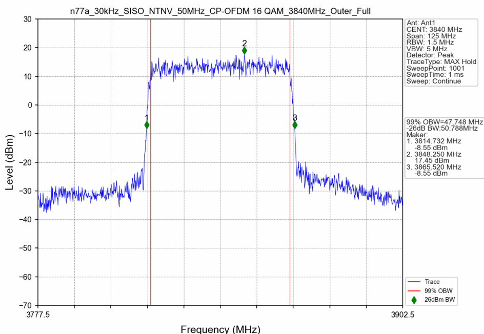
n77a_30kHz_SISO_NTNV_50MHz_CP-OFDM 16 QAM_3840MHz_Outer_Full
