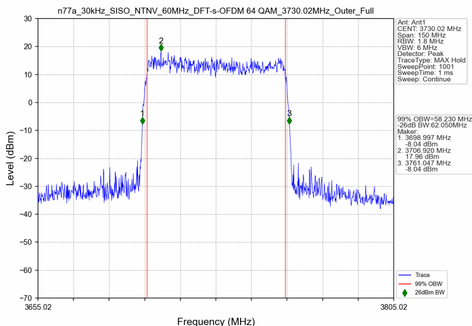
n77a_30kHz_SISO_NTNV_60MHz_DFT-s-OFDM 64 QAM_3730.02MHz_Outer_Full
