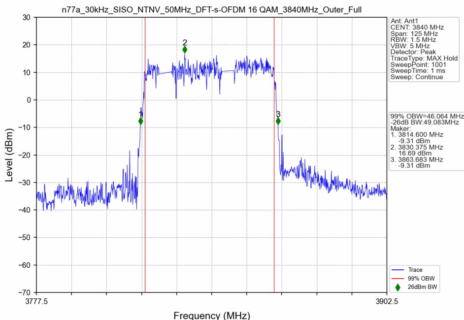
n77a_30kHz_SISO_NTNV_50MHz_DFT-s-OFDM 16 QAM_3840MHz_Outer_Full
