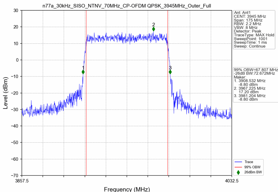
n77a_30kHz_SISO_NTNV_70MHz_CP-OFDM QPSK_3945MHz_Outer_Full
