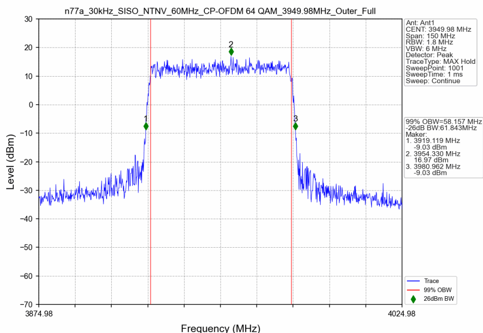
n77a_30kHz_SISO_NTNV_60MHz_CP-OFDM 64 QAM_3949.98MHz_Outer_Full
