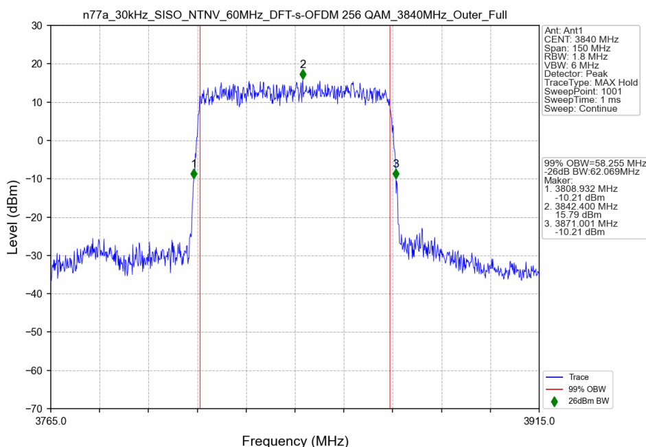
n77a_30kHz_SISO_NTNV_60MHz_DFT-s-OFDM 256 QAM_3840MHz_Outer_Full
