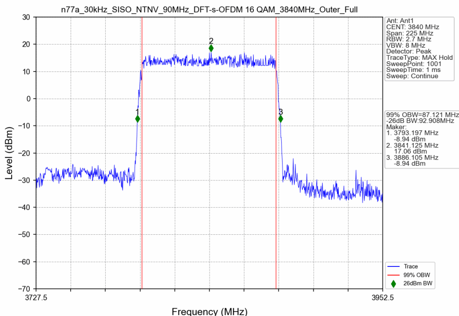
n77a_30kHz_SISO_NTNV_90MHz_DFT-s-OFDM 16 QAM_3840MHz_Outer_Full
