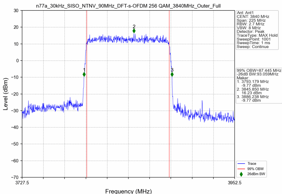
n77a_30kHz_SISO_NTNV_90MHz_DFT-s-OFDM 256 QAM_3840MHz_Outer_Full
