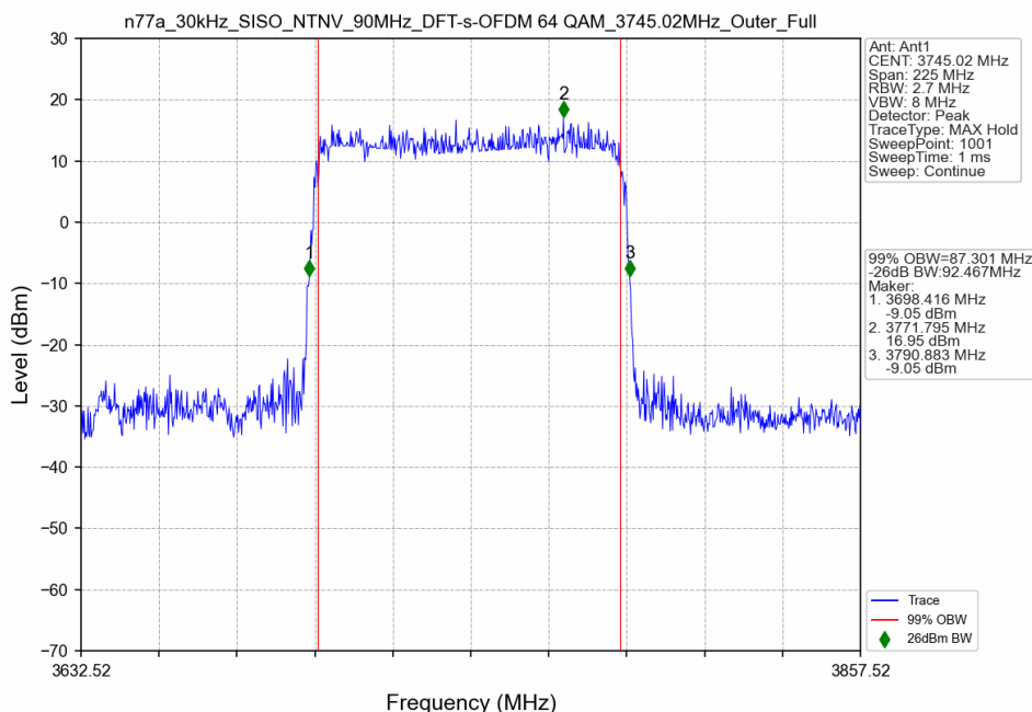
n77a_30kHz_SISO_NTNV_90MHz_DFT-s-OFDM 64 QAM_3745.02MHz_Outer_Full
