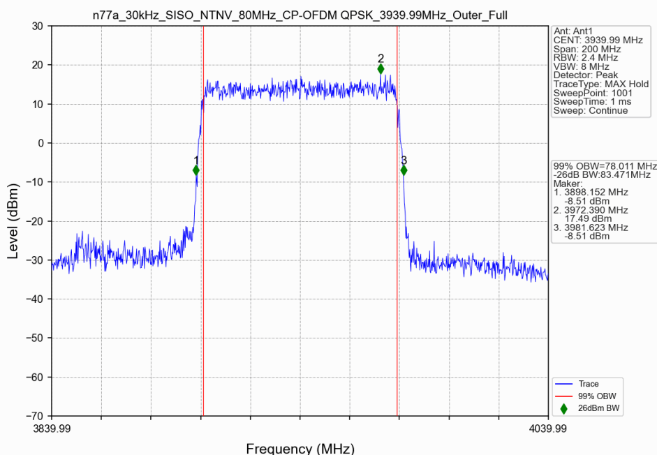
n77a_30kHz_SISO_NTNV_80MHz_CP-OFDM QPSK_3939.99MHz_Outer_Full
