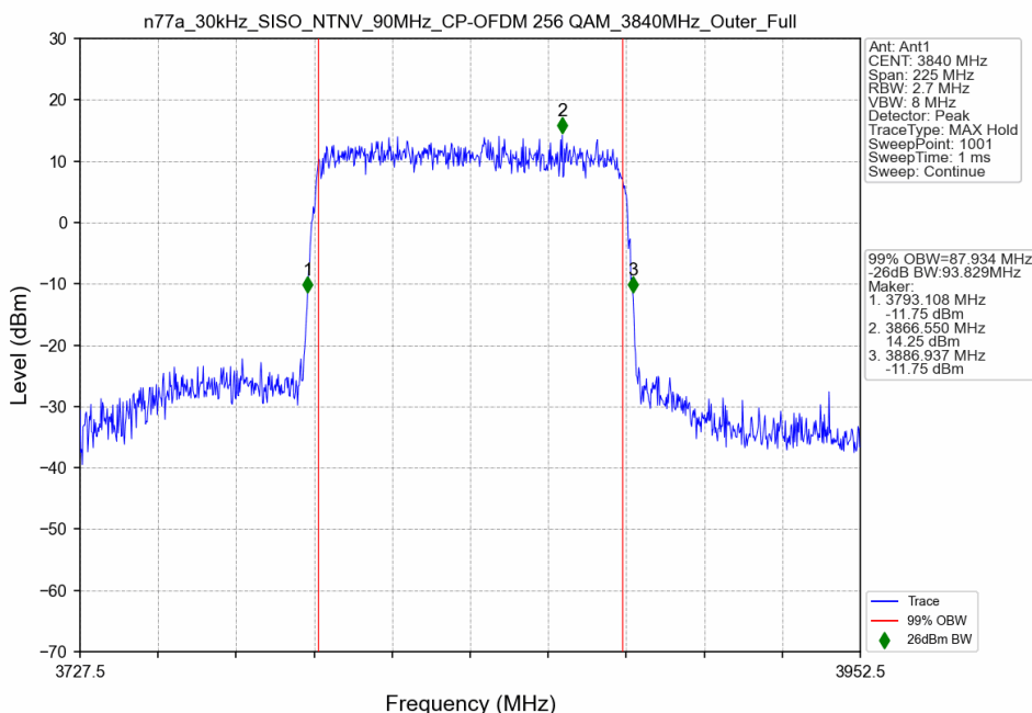
n77a_30kHz_SISO_NTNV_90MHz_CP-OFDM 256 QAM_3840MHz_Outer_Full
