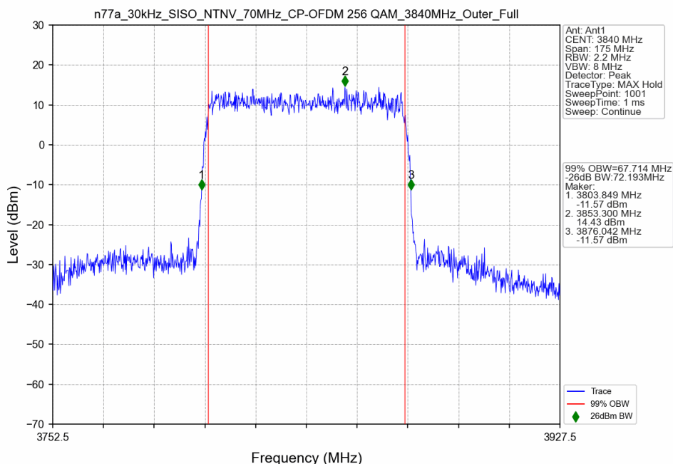
n77a_30kHz_SISO_NTNV_70MHz_CP-OFDM 256 QAM_3840MHz_Outer_Full
