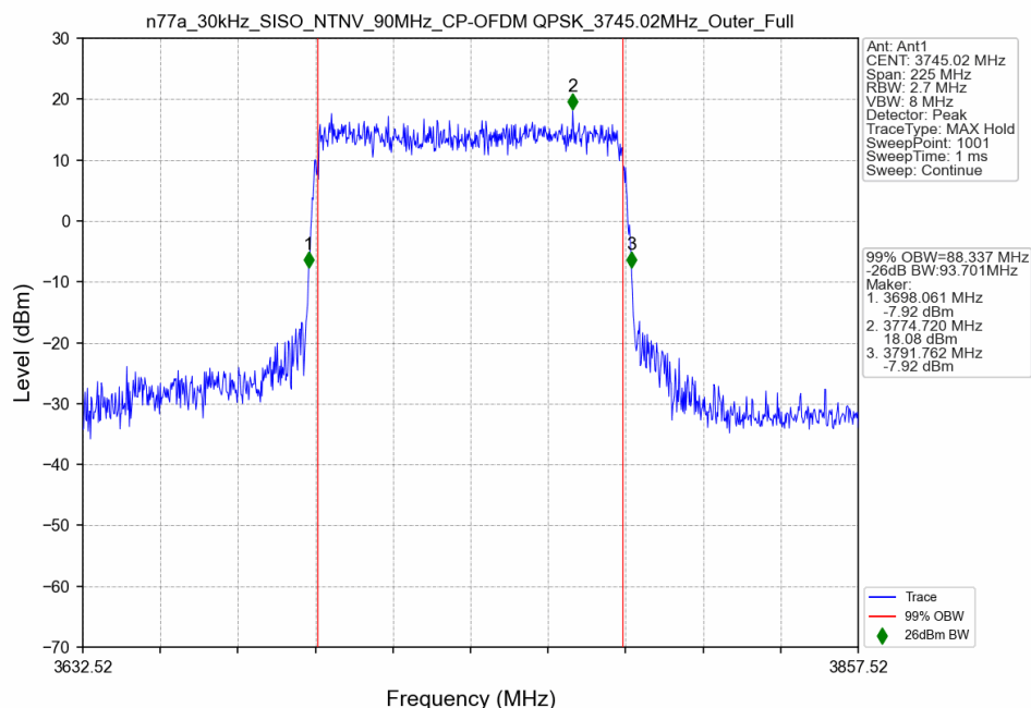
n77a_30kHz_SISO_NTNV_90MHz_CP-OFDM QPSK_3745.02MHz_Outer_Full
