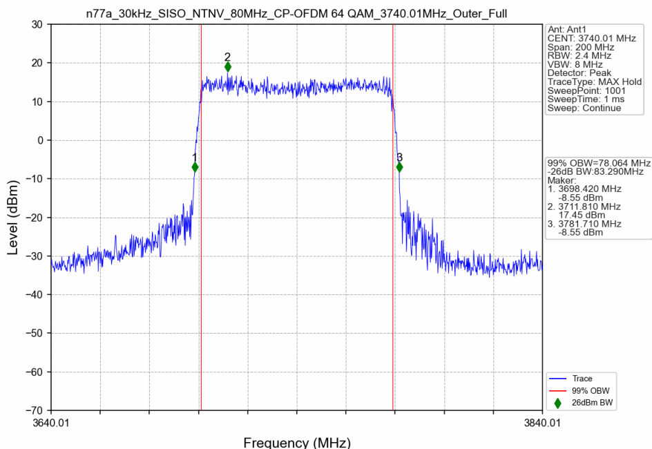
n77a_30kHz_SISO_NTNV_80MHz_CP-OFDM 64 QAM_3740.01MHz_Outer_Full
