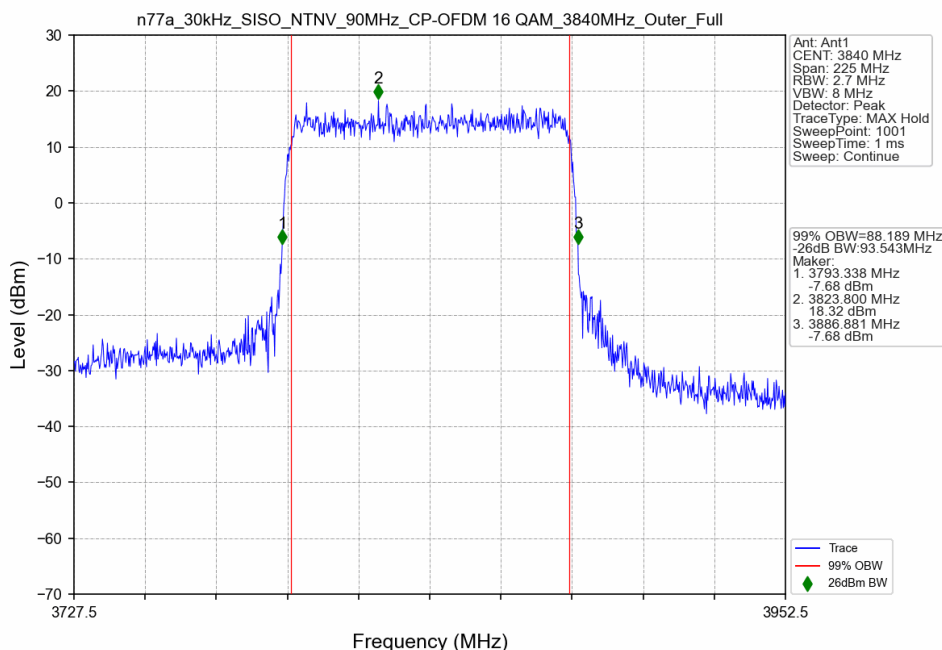
n77a_30kHz_SISO_NTNV_90MHz_CP-OFDM 16 QAM_3840MHz_Outer_Full
