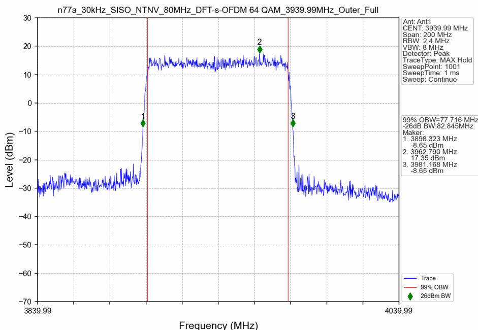
n77a_30kHz_SISO_NTNV_80MHz_DFT-s-OFDM 64 QAM_3939.99MHz_Outer_Full
