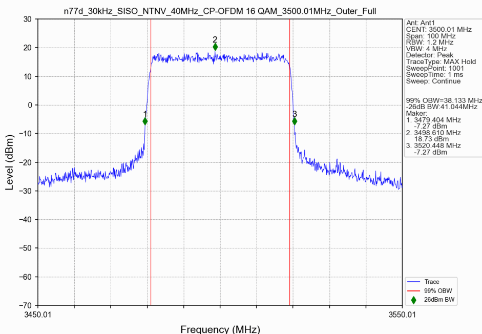
n77d_30kHz_SISO_NTNV_40MHz_CP-OFDM 16 QAM_3500.01MHz_Outer_Full
