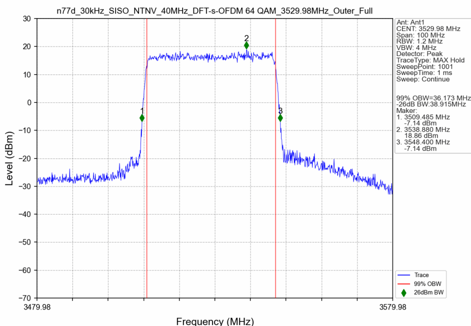
n77d_30kHz_SISO_NTNV_40MHz_DFT-s-OFDM 64 QAM_3529.98MHz_Outer_Full
