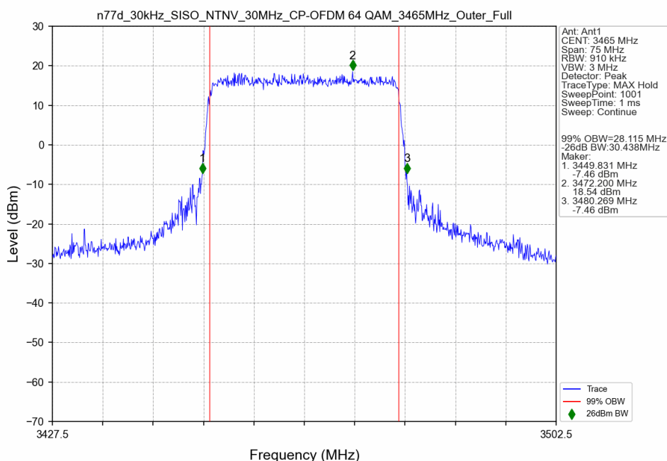
n77d_30kHz_SISO_NTNV_30MHz_CP-OFDM 64 QAM_3465MHz_Outer_Full
