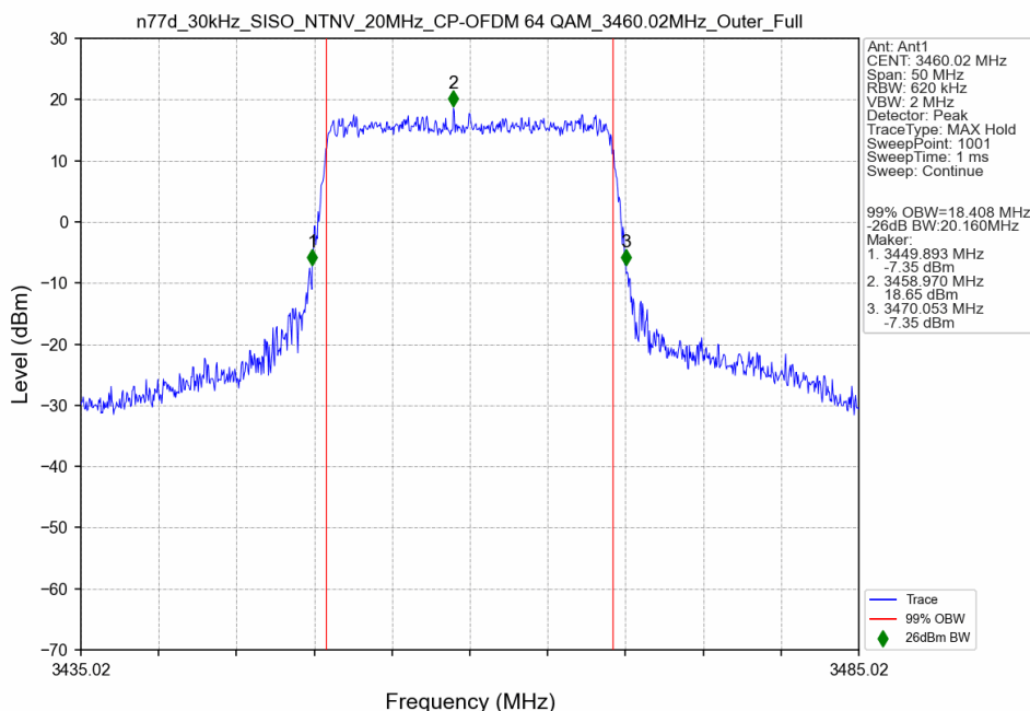
n77d_30kHz_SISO_NTNV_20MHz_CP-OFDM 64 QAM_3460.02MHz_Outer_Full
