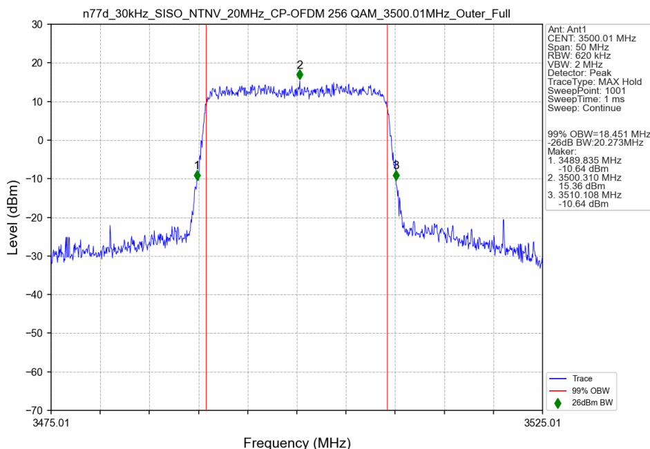
n77d_30kHz_SISO_NTNV_20MHz_CP-OFDM 256 QAM_3500.01MHz_Outer_Full
