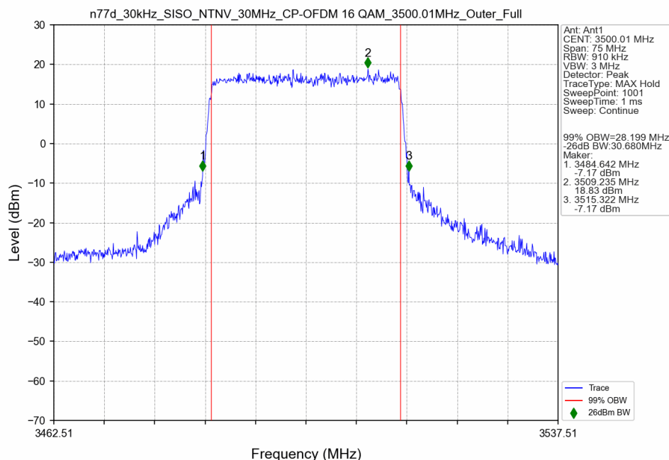
n77d_30kHz_SISO_NTNV_30MHz_CP-OFDM 16 QAM_3500.01MHz_Outer_Full
