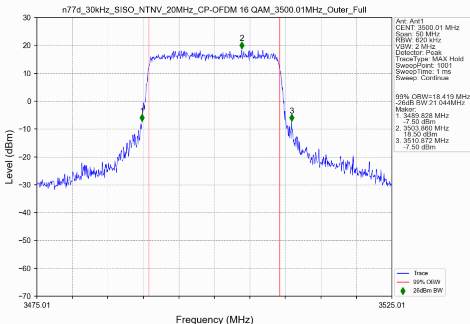
n77d_30kHz_SISO_NTNV_20MHz_CP-OFDM 16 QAM_3500.01MHz_Outer_Full
