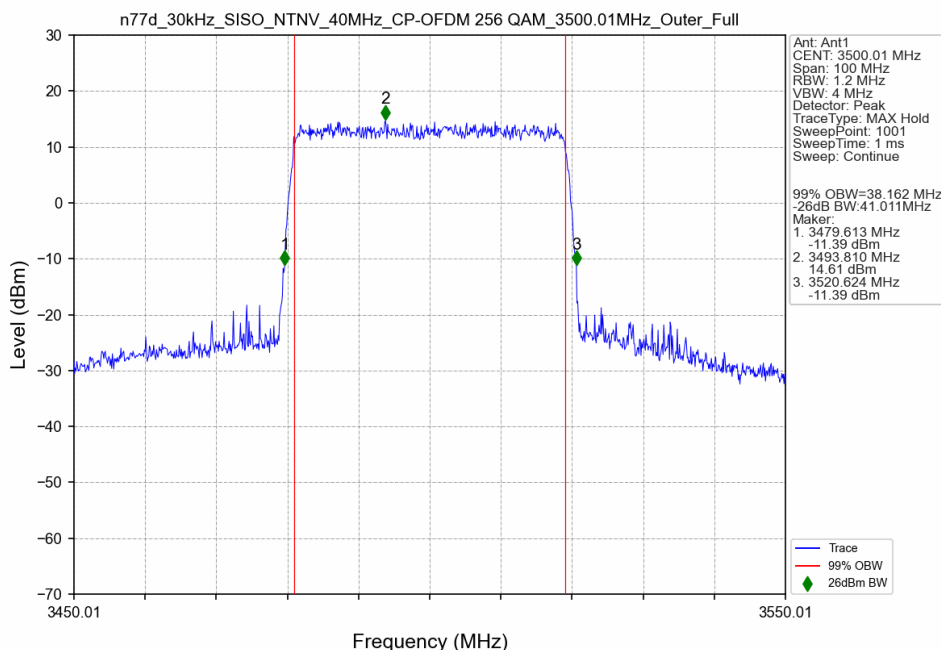
n77d_30kHz_SISO_NTNV_40MHz_CP-OFDM 256 QAM_3500.01MHz_Outer_Full
