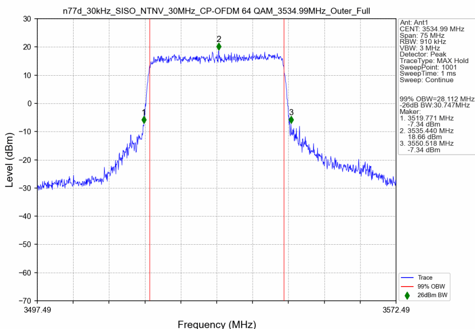
n77d_30kHz_SISO_NTNV_30MHz_CP-OFDM 64 QAM_3534.99MHz_Outer_Full
