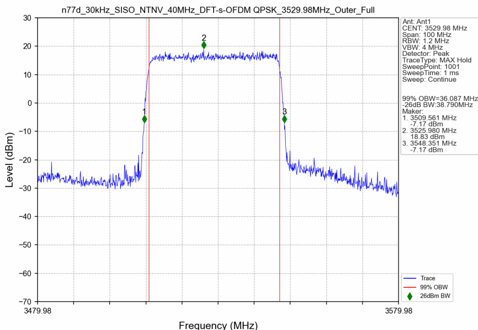
n77d_30kHz_SISO_NTNV_40MHz_DFT-s-OFDM QPSK_3529.98MHz_Outer_Full
