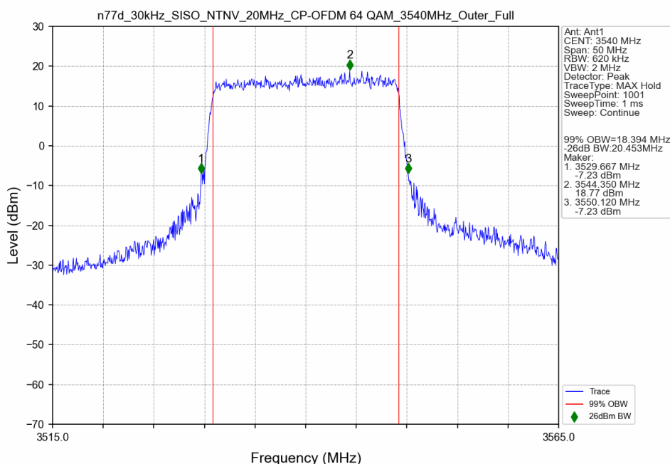
n77d_30kHz_SISO_NTNV_20MHz_CP-OFDM 64 QAM_3540MHz_Outer_Full
