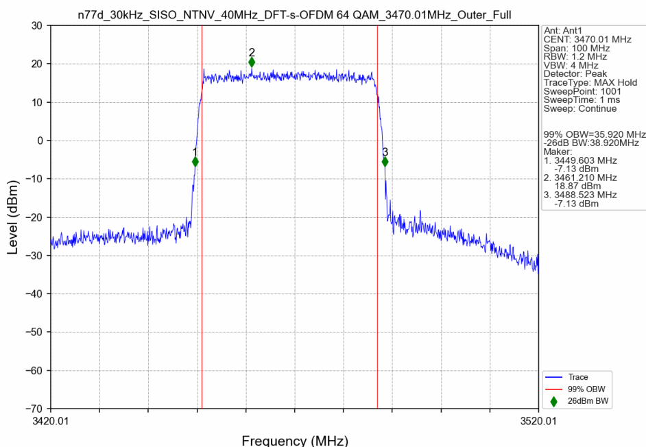
n77d_30kHz_SISO_NTNV_40MHz_DFT-s-OFDM 64 QAM_3470.01MHz_Outer_Full
