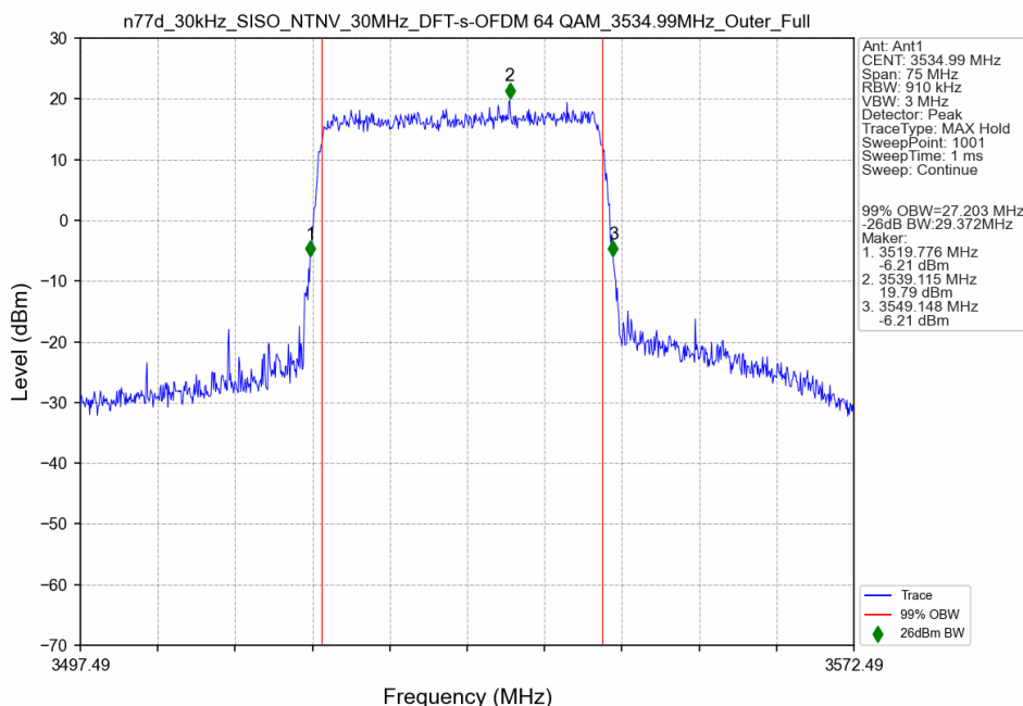
n77d_30kHz_SISO_NTNV_30MHz_DFT-s-OFDM 64 QAM_3534.99MHz_Outer_Full
