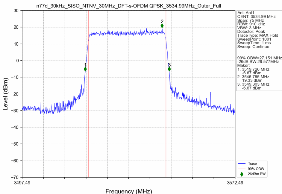
n77d_30kHz_SISO_NTNV_30MHz_DFT-s-OFDM QPSK_3534.99MHz_Outer_Full
