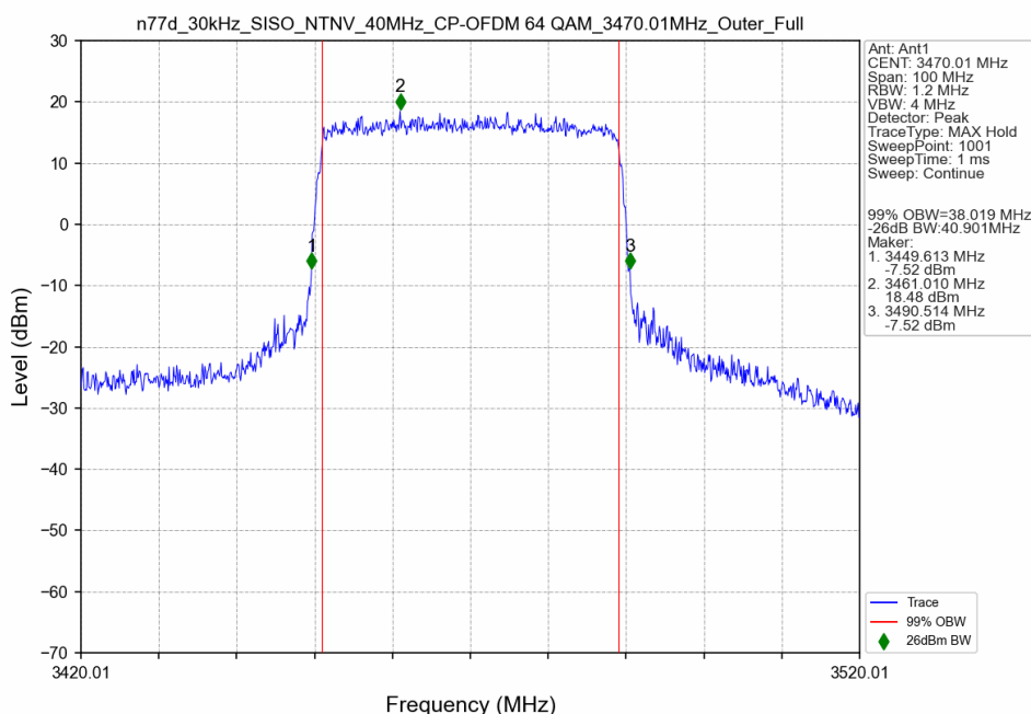
n77d_30kHz_SISO_NTNV_40MHz_CP-OFDM 64 QAM_3470.01MHz_Outer_Full
