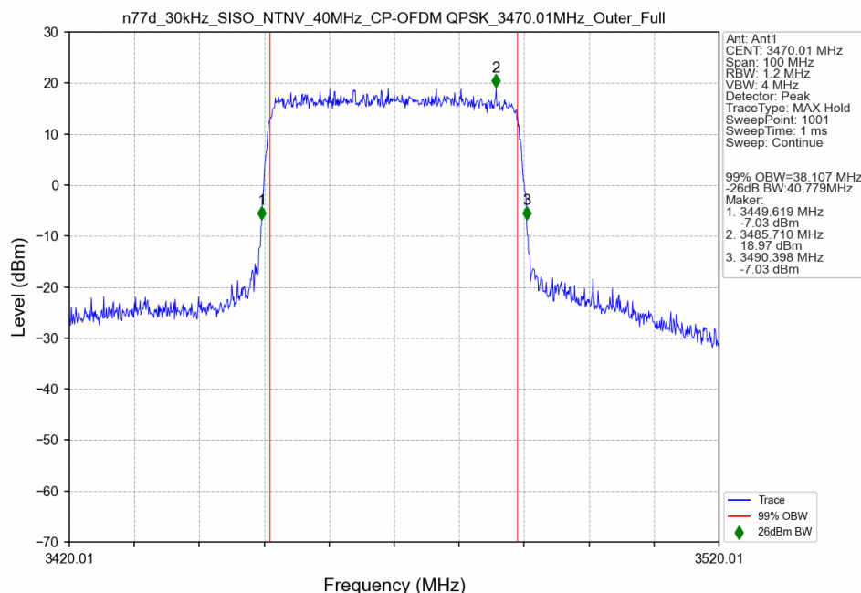
n77d_30kHz_SISO_NTNV_40MHz_CP-OFDM QPSK_3470.01MHz_Outer_Full
