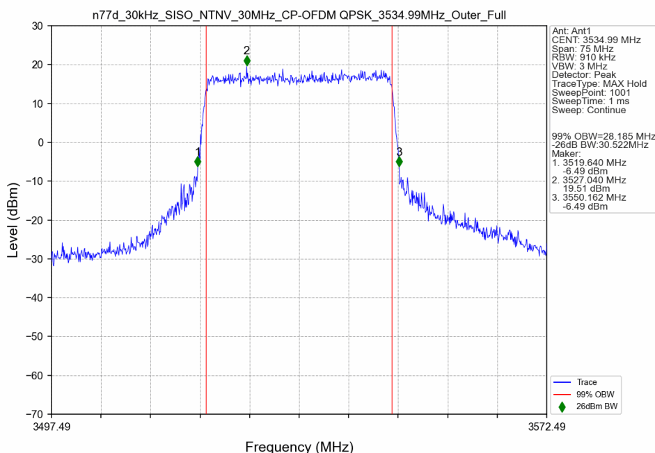
n77d_30kHz_SISO_NTNV_30MHz_CP-OFDM QPSK_3534.99MHz_Outer_Full
