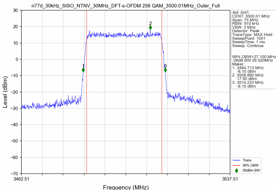
n77d_30kHz_SISO_NTNV_30MHz_DFT-s-OFDM 256 QAM_3500.01MHz_Outer_Full
