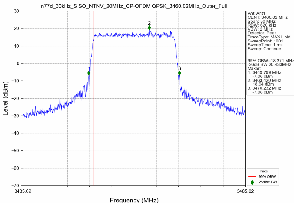
n77d_30kHz_SISO_NTNV_20MHz_CP-OFDM QPSK_3460.02MHz_Outer_Full
