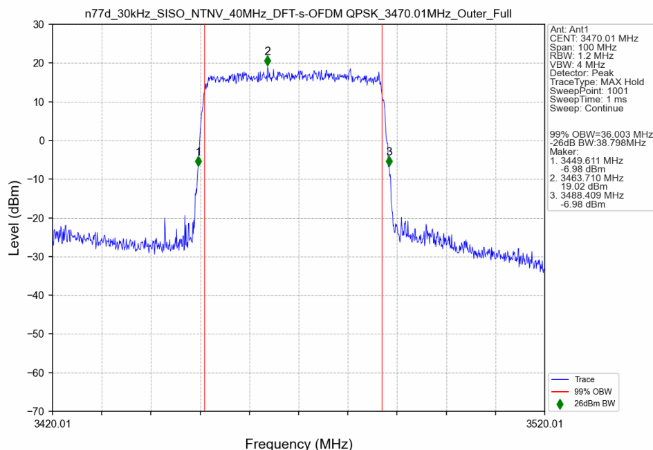
n77d_30kHz_SISO_NTNV_40MHz_DFT-s-OFDM QPSK_3470.01MHz_Outer_Full
