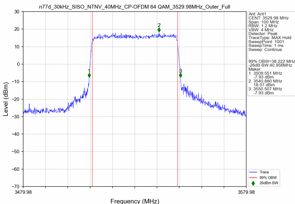
n77d_30kHz_SISO_NTNV_40MHz_CP-OFDM 64 QAM_3529.98MHz_Outer_Full
