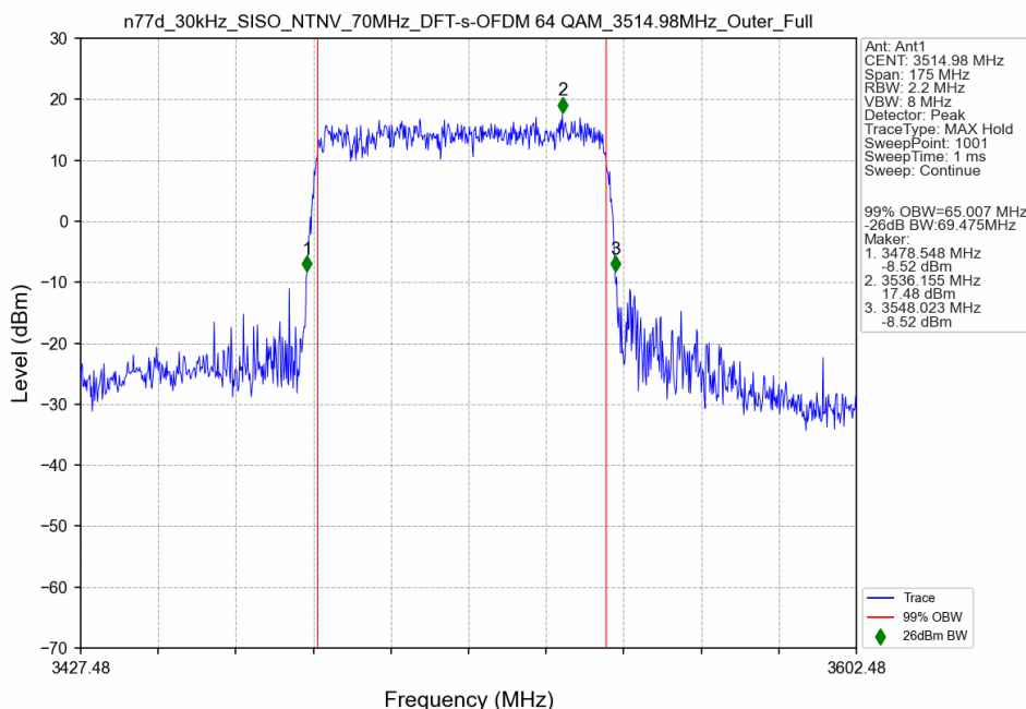
n77d_30kHz_SISO_NTNV_70MHz_DFT-s-OFDM 64 QAM_3514.98MHz_Outer_Full
