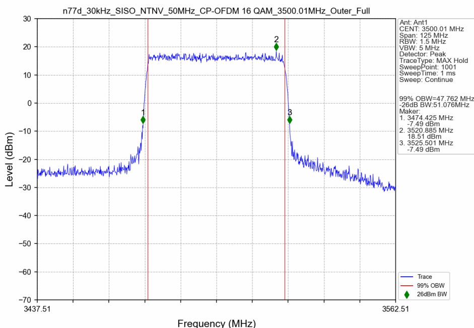
n77d_30kHz_SISO_NTNV_50MHz_CP-OFDM 16 QAM_3500.01MHz_Outer_Full
