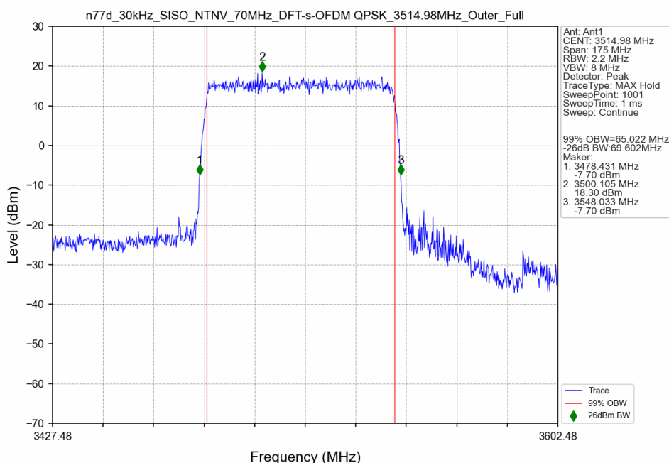
n77d_30kHz_SISO_NTNV_70MHz_DFT-s-OFDM QPSK_3514.98MHz_Outer_Full
