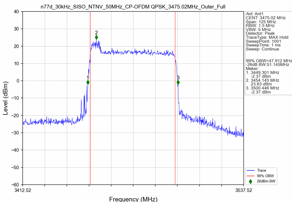
n77d_30kHz_SISO_NTNV_50MHz_CP-OFDM QPSK_3475.02MHz_Outer_Full
