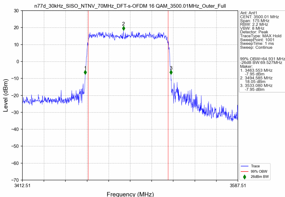
n77d_30kHz_SISO_NTNV_70MHz_DFT-s-OFDM 16 QAM_3500.01MHz_Outer_Full
