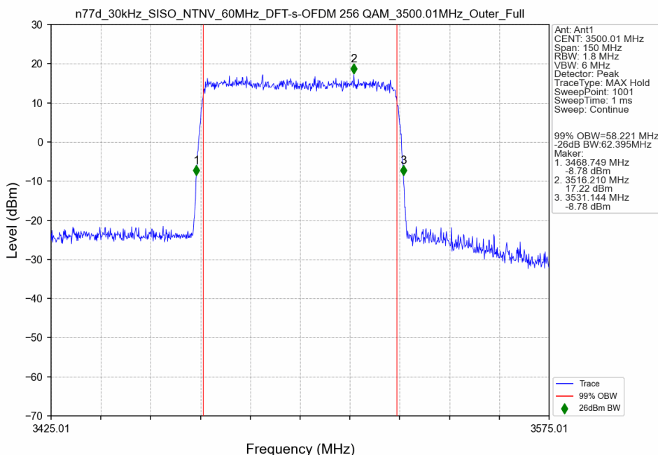
n77d_30kHz_SISO_NTNV_60MHz_DFT-s-OFDM 256 QAM_3500.01MHz_Outer_Full
