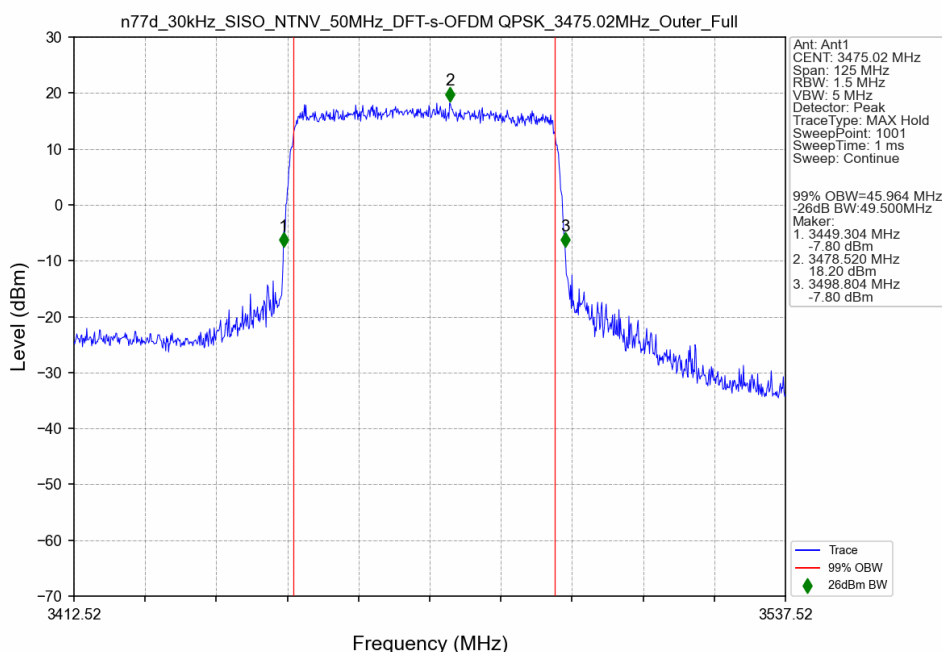
n77d_30kHz_SISO_NTNV_50MHz_DFT-s-OFDM QPSK_3475.02MHz_Outer_Full
