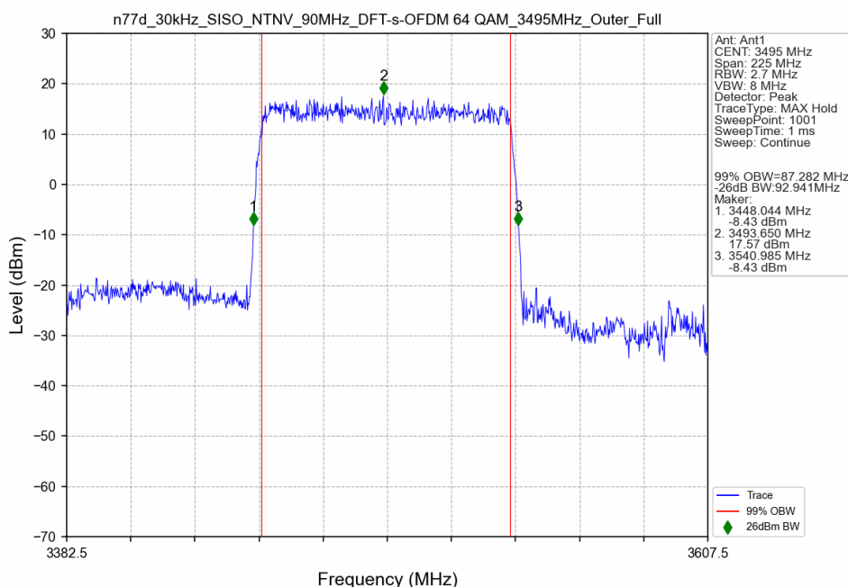
n77d_30kHz_SISO_NTNV_90MHz_DFT-s-OFDM 64 QAM_3495MHz_Outer_Full
