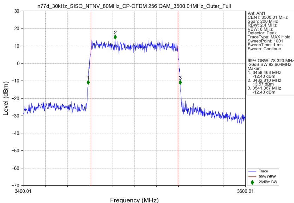
n77d_30kHz_SISO_NTNV_80MHz_CP-OFDM 256 QAM_3500.01MHz_Outer_Full
