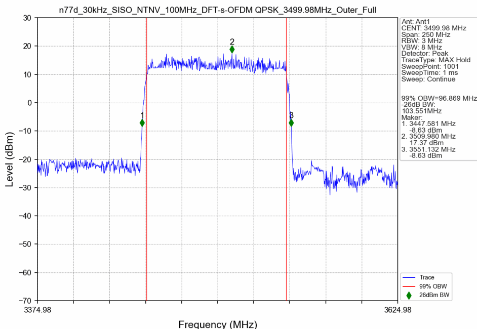
n77d_30kHz_SISO_NTNV_100MHz_DFT-s-OFDM QPSK_3499.98MHz_Outer_Full
