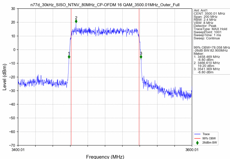
n77d_30kHz_SISO_NTNV_80MHz_CP-OFDM 16 QAM_3500.01MHz_Outer_Full
