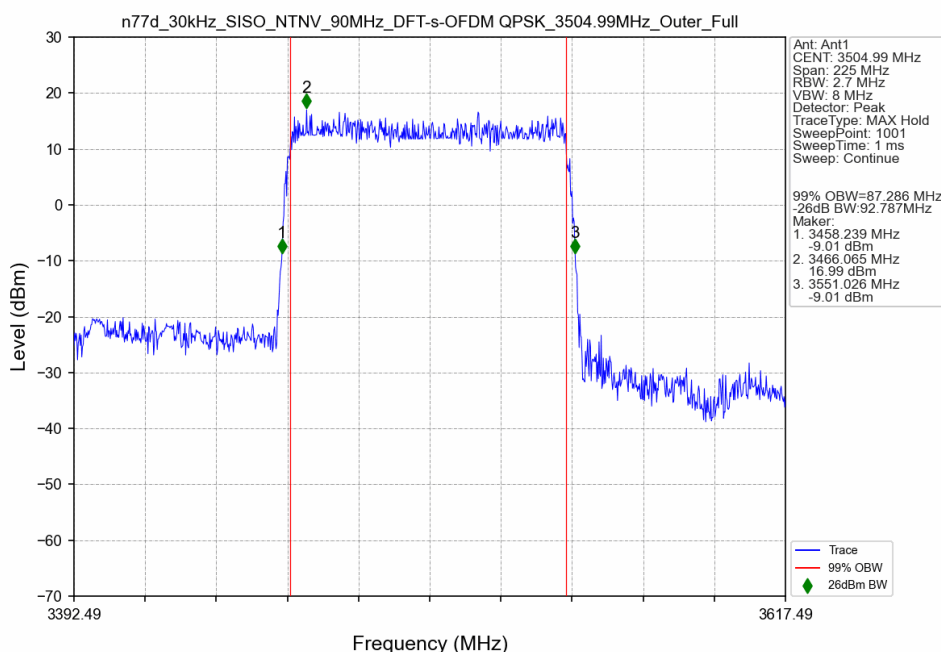
n77d_30kHz_SISO_NTNV_90MHz_DFT-s-OFDM QPSK_3504.99MHz_Outer_Full
