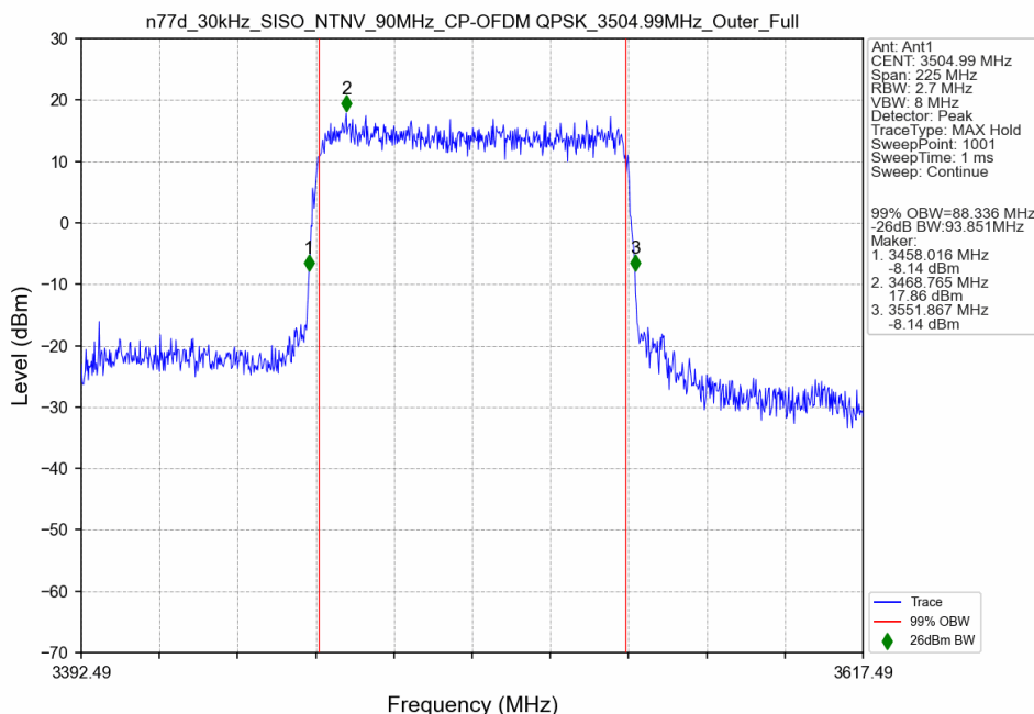
n77d_30kHz_SISO_NTNV_90MHz_CP-OFDM QPSK_3504.99MHz_Outer_Full
