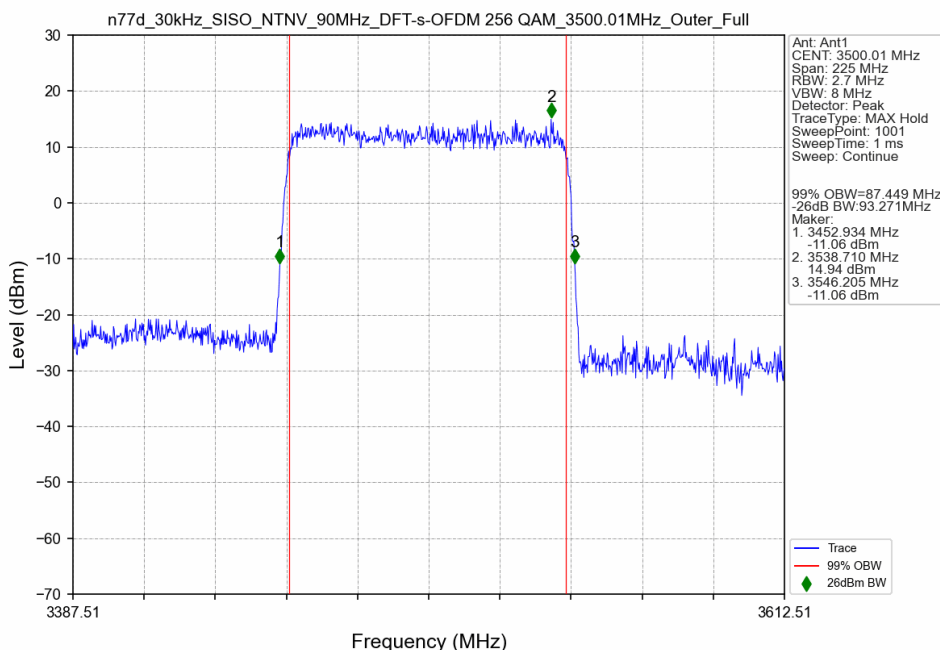
n77d_30kHz_SISO_NTNV_90MHz_DFT-s-OFDM 256 QAM_3500.01MHz_Outer_Full
