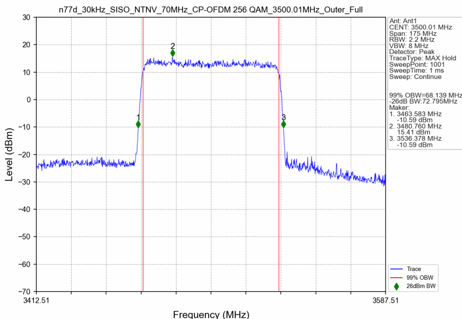
n77d_30kHz_SISO_NTNV_70MHz_CP-OFDM 256 QAM_3500.01MHz_Outer_Full
