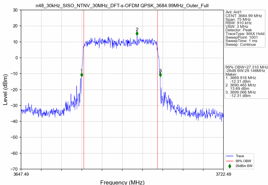
n48_30kHz_SISO_NTNV_30MHz_DFT-s-OFDM QPSK_3684.99MHz_Outer_Full
