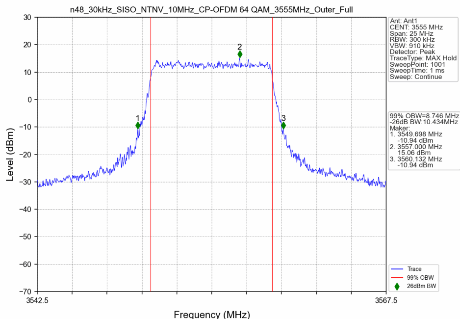
n48_30kHz_SISO_NTNV_10MHz_CP-OFDM 64 QAM_3555MHz_Outer_Full
