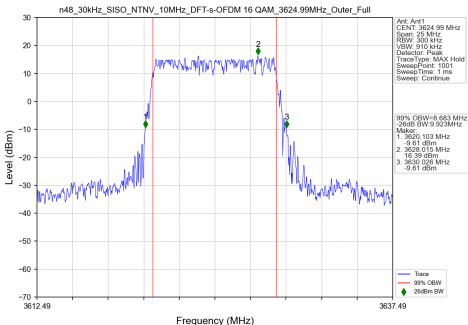
n48_30kHz_SISO_NTNV_10MHz_DFT-s-OFDM 16 QAM_3624.99MHz_Outer_Full
