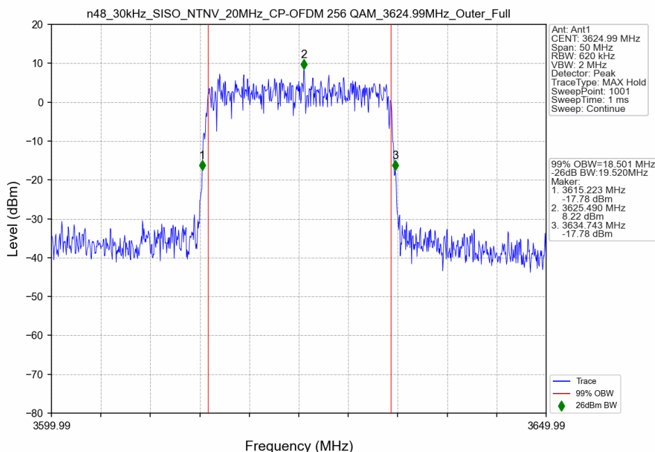
n48_30kHz_SISO_NTNV_20MHz_CP-OFDM 256 QAM_3624.99MHz_Outer_Full
