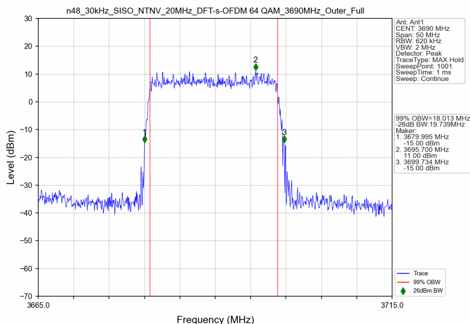
n48_30kHz_SISO_NTNV_20MHz_DFT-s-OFDM 64 QAM_3690MHz_Outer_Full
