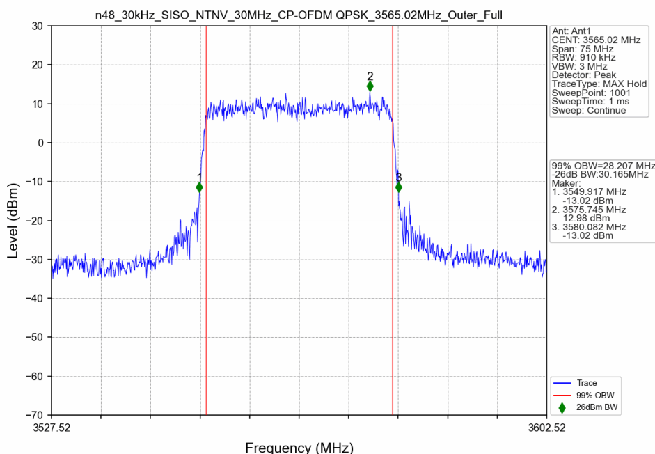
n48_30kHz_SISO_NTNV_30MHz_CP-OFDM QPSK_3565.02MHz_Outer_Full
