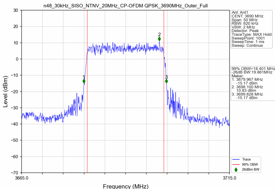
n48_30kHz_SISO_NTNV_20MHz_CP-OFDM QPSK_3690MHz_Outer_Full
