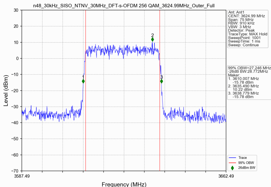
n48_30kHz_SISO_NTNV_30MHz_DFT-s-OFDM 256 QAM_3624.99MHz_Outer_Full
