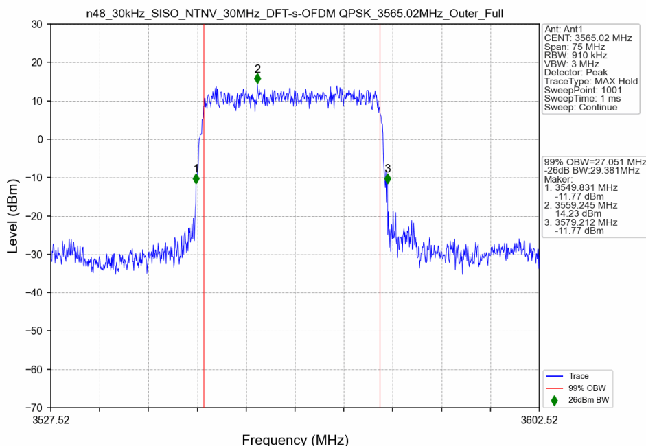
n48_30kHz_SISO_NTNV_30MHz_DFT-s-OFDM QPSK_3565.02MHz_Outer_Full
