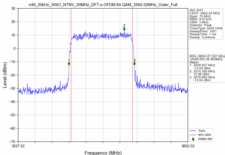
n48_30kHz_SISO_NTNV_30MHz_DFT-s-OFDM 64 QAM_3565.02MHz_Outer_Full
