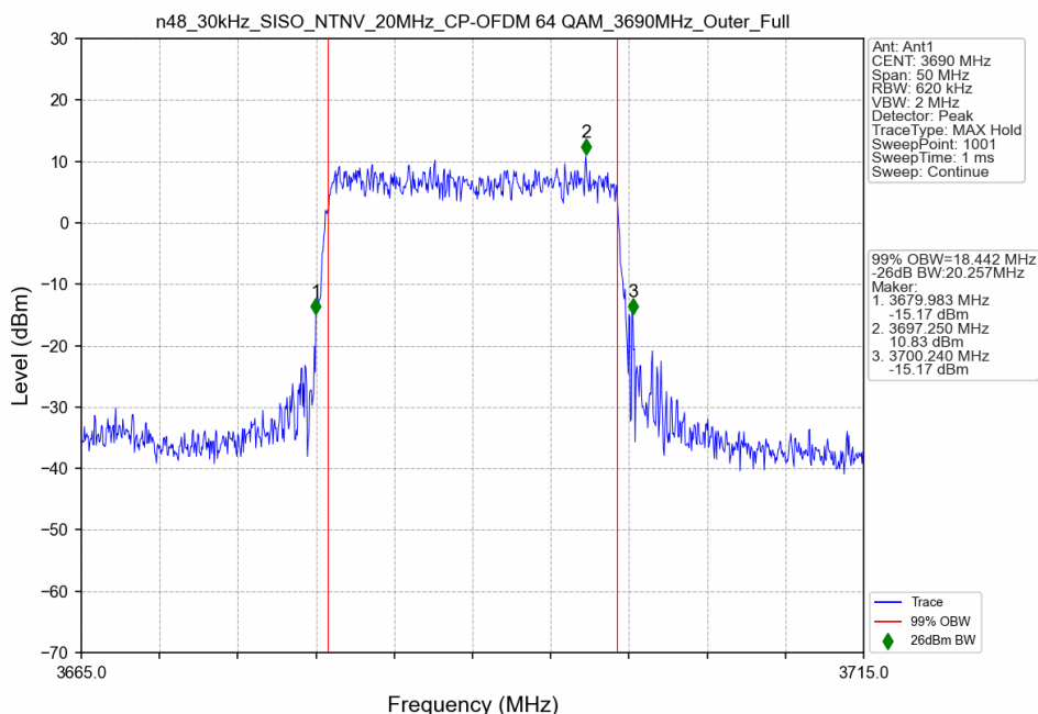
n48_30kHz_SISO_NTNV_20MHz_CP-OFDM 64 QAM_3690MHz_Outer_Full
