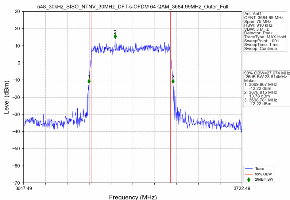
n48_30kHz_SISO_NTNV_30MHz_DFT-s-OFDM 64 QAM_3684.99MHz_Outer_Full
