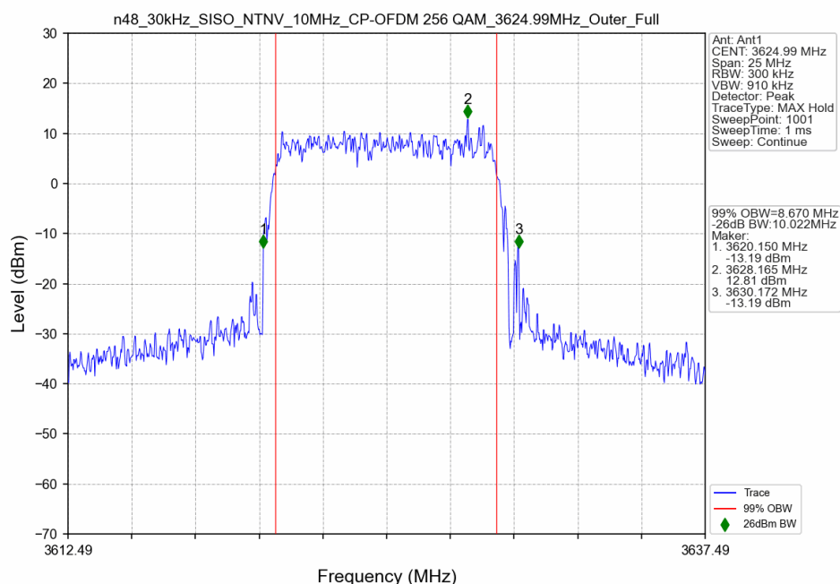
n48_30kHz_SISO_NTNV_10MHz_CP-OFDM 256 QAM_3624.99MHz_Outer_Full
