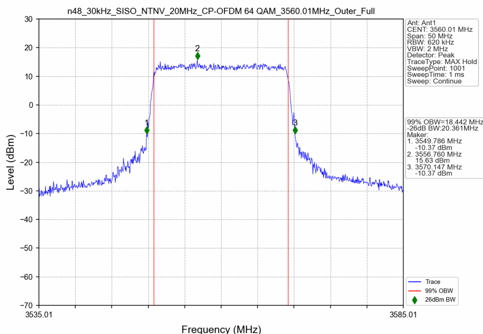
n48_30kHz_SISO_NTNV_20MHz_CP-OFDM 64 QAM_3560.01MHz_Outer_Full
