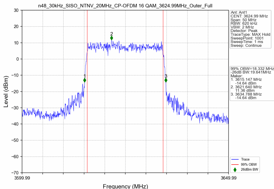
n48_30kHz_SISO_NTNV_20MHz_CP-OFDM 16 QAM_3624.99MHz_Outer_Full
