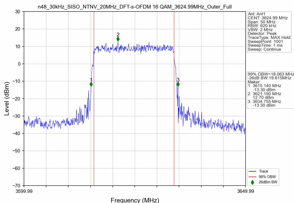
n48_30kHz_SISO_NTNV_20MHz_DFT-s-OFDM 16 QAM_3624.99MHz_Outer_Full
