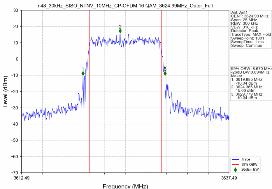
n48_30kHz_SISO_NTNV_10MHz_CP-OFDM 16 QAM_3624.99MHz_Outer_Full
