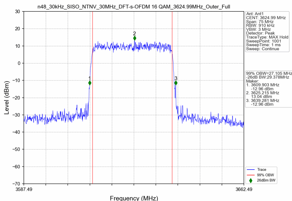
n48_30kHz_SISO_NTNV_30MHz_DFT-s-OFDM 16 QAM_3624.99MHz_Outer_Full
