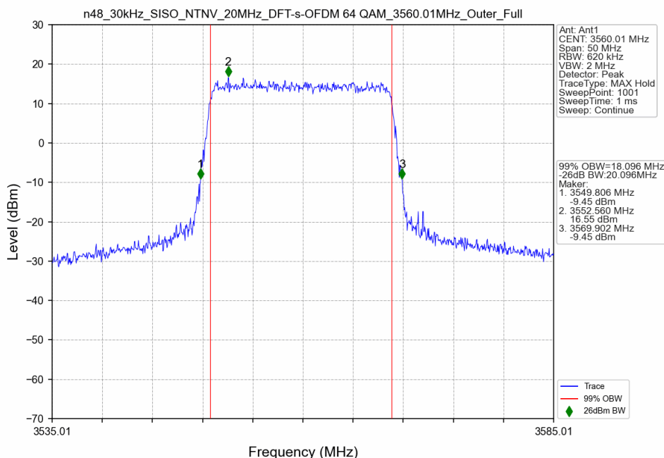
n48_30kHz_SISO_NTNV_20MHz_DFT-s-OFDM 64 QAM_3560.01MHz_Outer_Full
