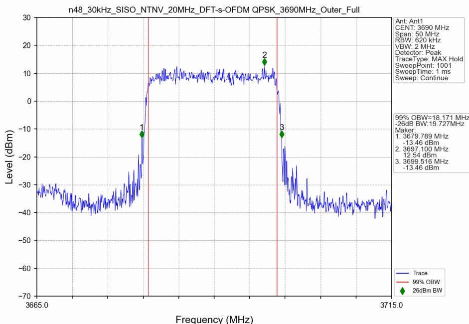
n48_30kHz_SISO_NTNV_20MHz_DFT-s-OFDM QPSK_3690MHz_Outer_Full
