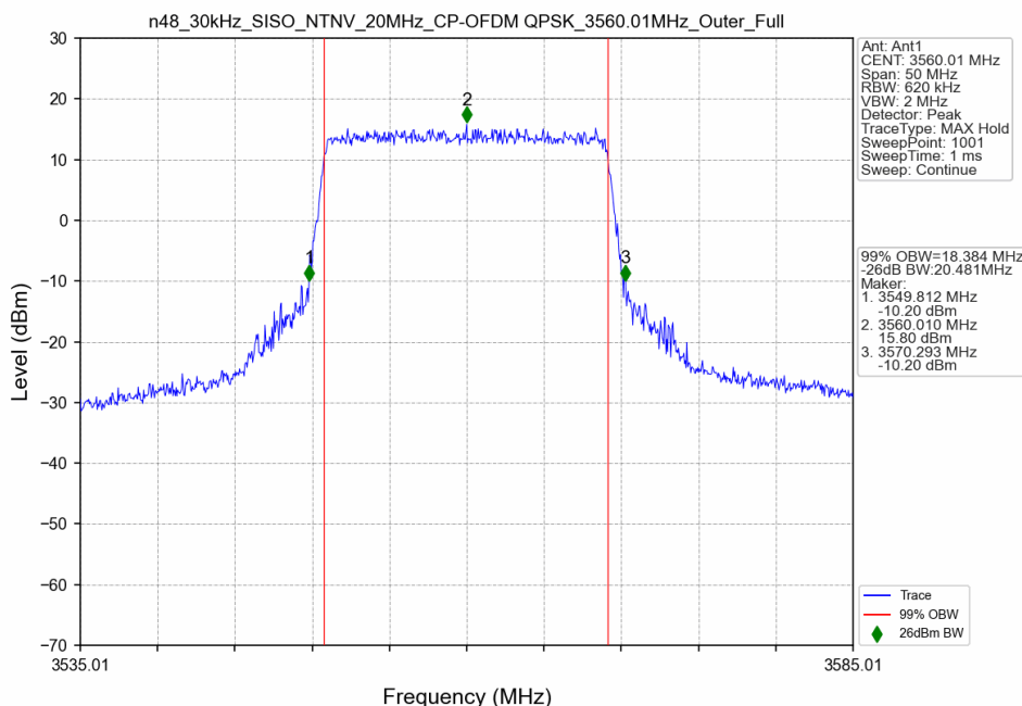
n48_30kHz_SISO_NTNV_20MHz_CP-OFDM QPSK_3560.01MHz_Outer_Full
