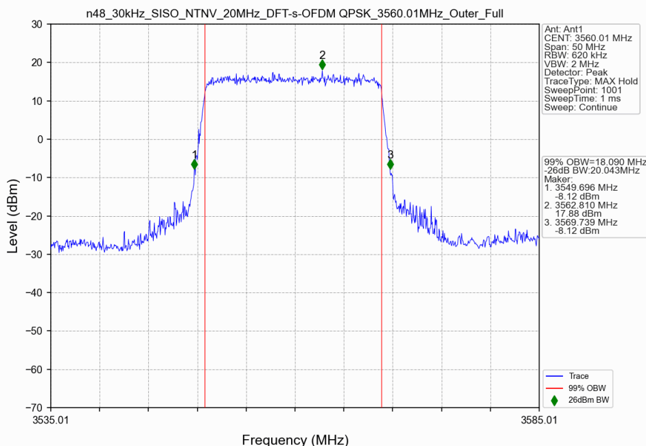
n48_30kHz_SISO_NTNV_20MHz_DFT-s-OFDM QPSK_3560.01MHz_Outer_Full
