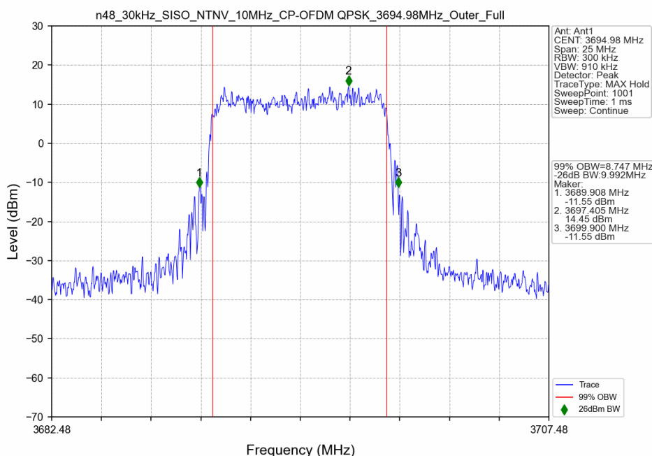
n48_30kHz_SISO_NTNV_10MHz_CP-OFDM QPSK_3694.98MHz_Outer_Full
