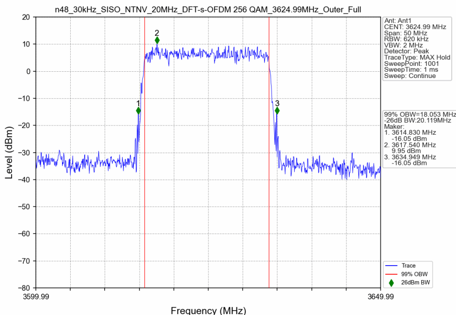
n48_30kHz_SISO_NTNV_20MHz_DFT-s-OFDM 256 QAM_3624.99MHz_Outer_Full
