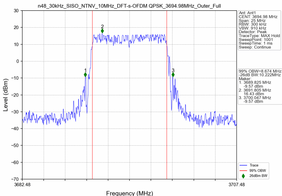
n48_30kHz_SISO_NTNV_10MHz_DFT-s-OFDM QPSK_3694.98MHz_Outer_Full
