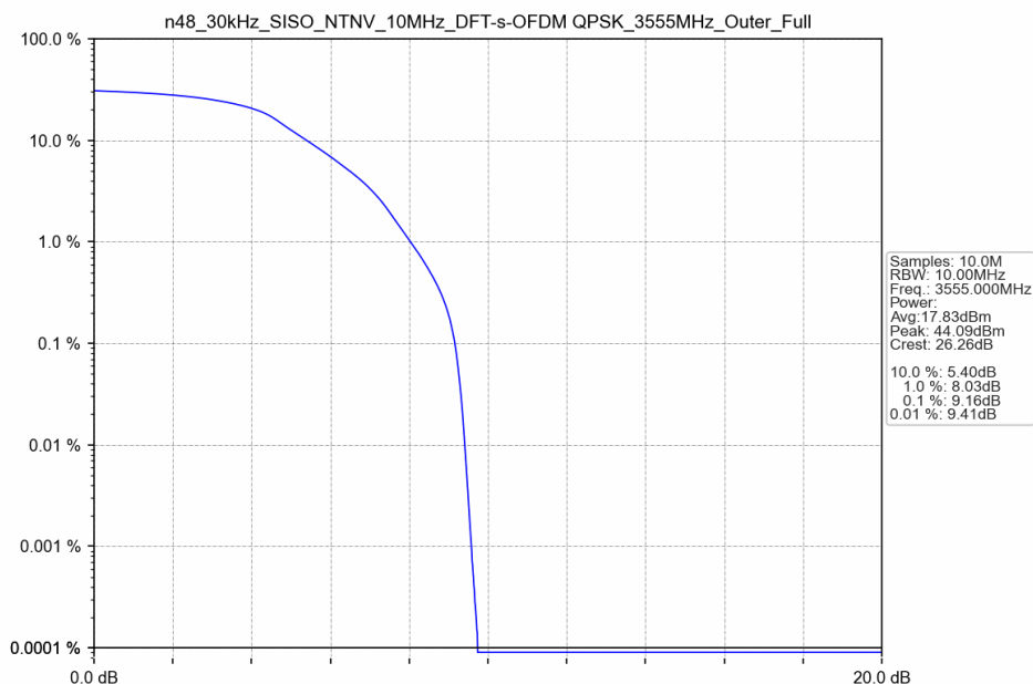
n48_30kHz_SISO_NTNV_10MHz_DFT-s-OFDM QPSK_3555MHz_Outer_Full
