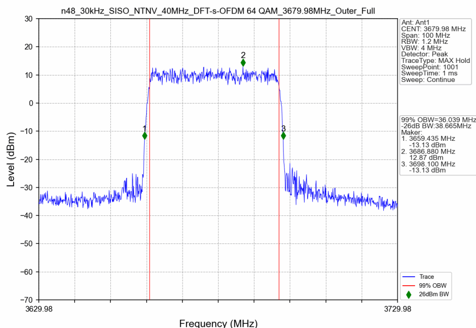
n48_30kHz_SISO_NTNV_40MHz_DFT-s-OFDM 64 QAM_3679.98MHz_Outer_Full
