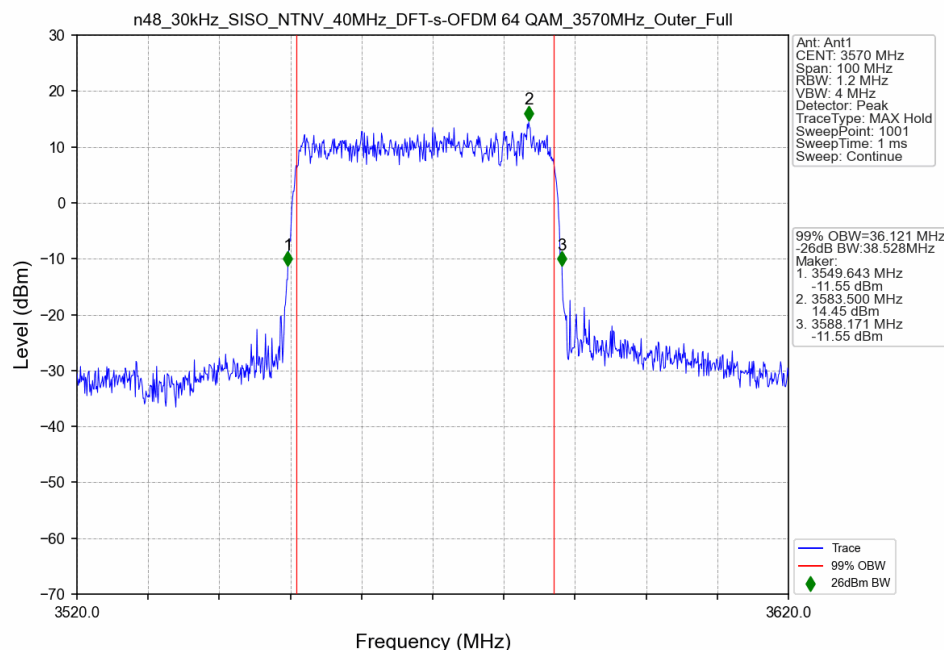
n48_30kHz_SISO_NTNV_40MHz_DFT-s-OFDM 64 QAM_3570MHz_Outer_Full
