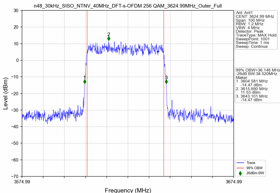
n48_30kHz_SISO_NTNV_40MHz_DFT-s-OFDM 256 QAM_3624.99MHz_Outer_Full
