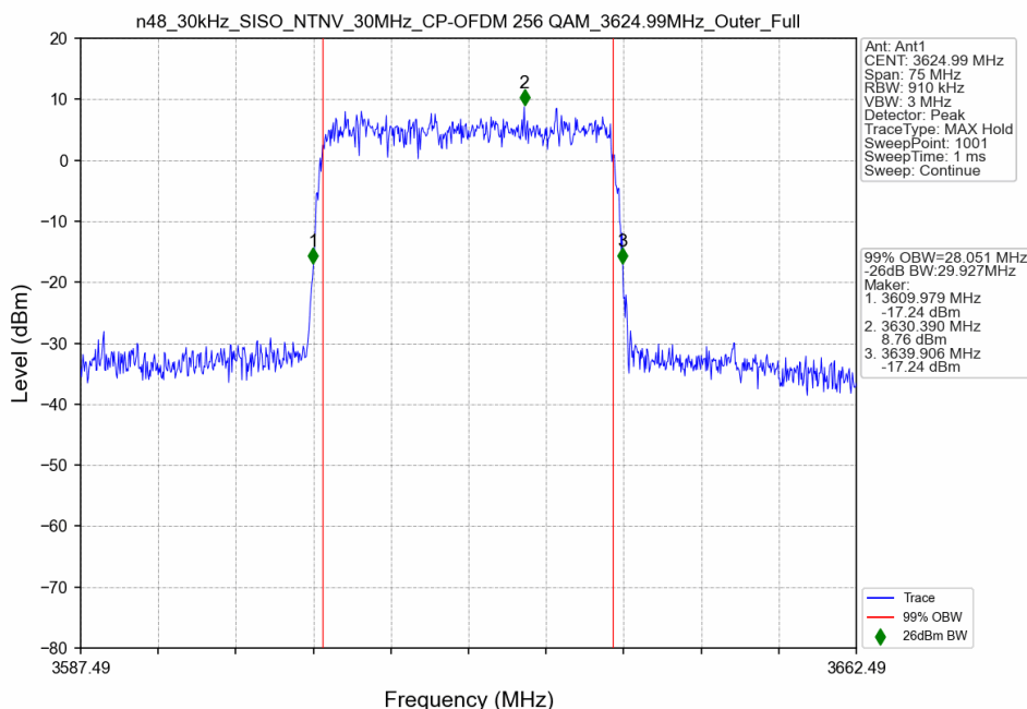
n48_30kHz_SISO_NTNV_30MHz_CP-OFDM 256 QAM_3624.99MHz_Outer_Full
