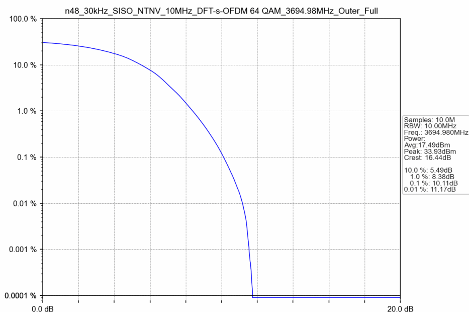
n48_30kHz_SISO_NTNV_10MHz_DFT-s-OFDM 64 QAM_3694.98MHz_Outer_Full
