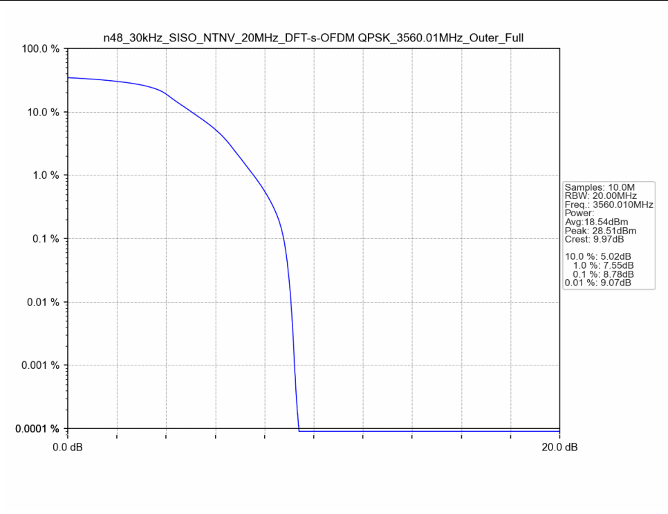
n48_30kHz_SISO_NTNV_20MHz_DFT-s-OFDM QPSK_3560.01MHz_Outer_Full
