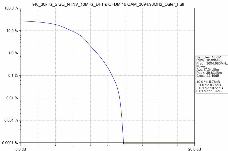
n48_30kHz_SISO_NTNV_10MHz_DFT-s-OFDM 16 QAM_3694.98MHz_Outer_Full
