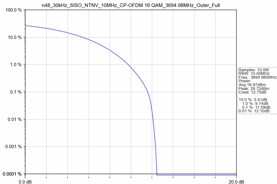
n48_30kHz_SISO_NTNV_10MHz_CP-OFDM 16 QAM_3694.98MHz_Outer_Full
