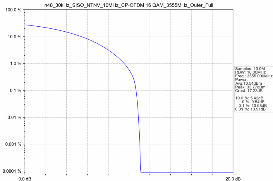
n48_30kHz_SISO_NTNV_10MHz_CP-OFDM 16 QAM_3555MHz_Outer_Full
