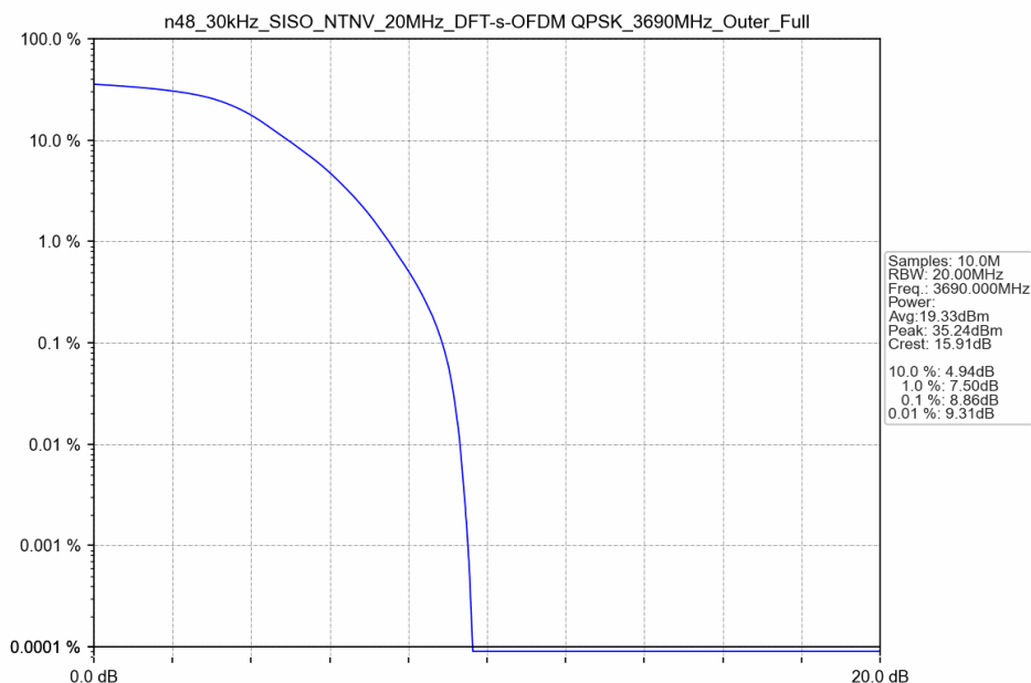
n48_30kHz_SISO_NTNV_20MHz_DFT-s-OFDM QPSK_3690MHz_Outer_Full
