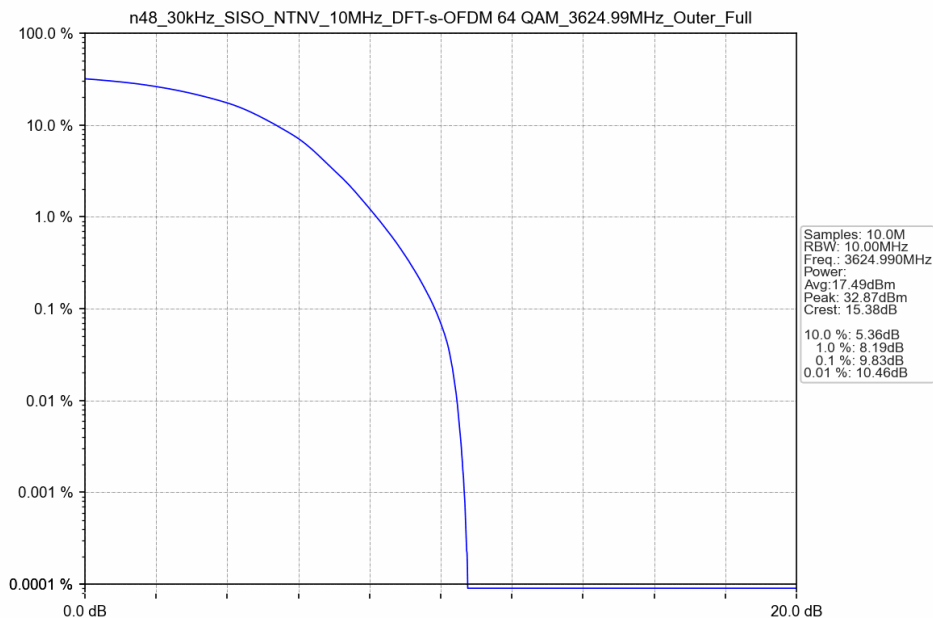
n48_30kHz_SISO_NTNV_10MHz_DFT-s-OFDM 64 QAM_3624.99MHz_Outer_Full
