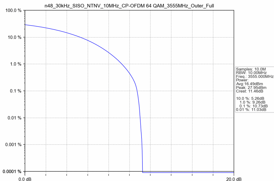
n48_30kHz_SISO_NTNV_10MHz_CP-OFDM 64 QAM_3555MHz_Outer_Full
