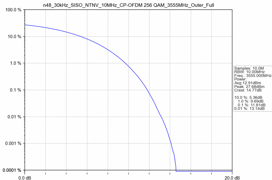
n48_30kHz_SISO_NTNV_10MHz_CP-OFDM 256 QAM_3555MHz_Outer_Full
