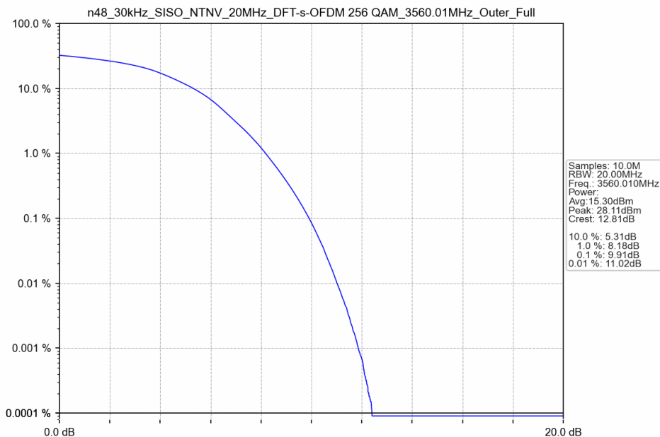
n48_30kHz_SISO_NTNV_20MHz_DFT-s-OFDM 256 QAM_3560.01MHz_Outer_Full
