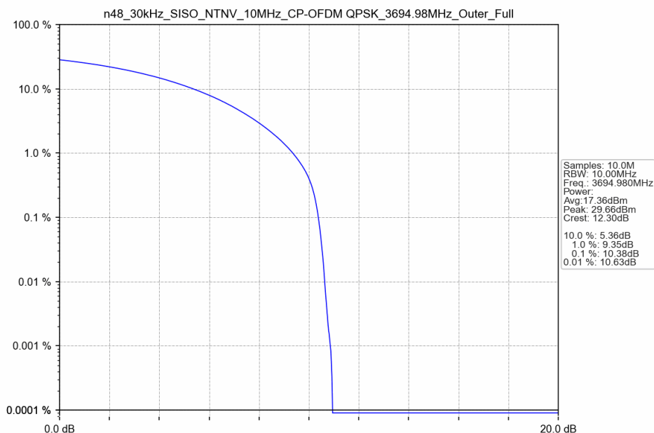
n48_30kHz_SISO_NTNV_10MHz_CP-OFDM QPSK_3694.98MHz_Outer_Full
