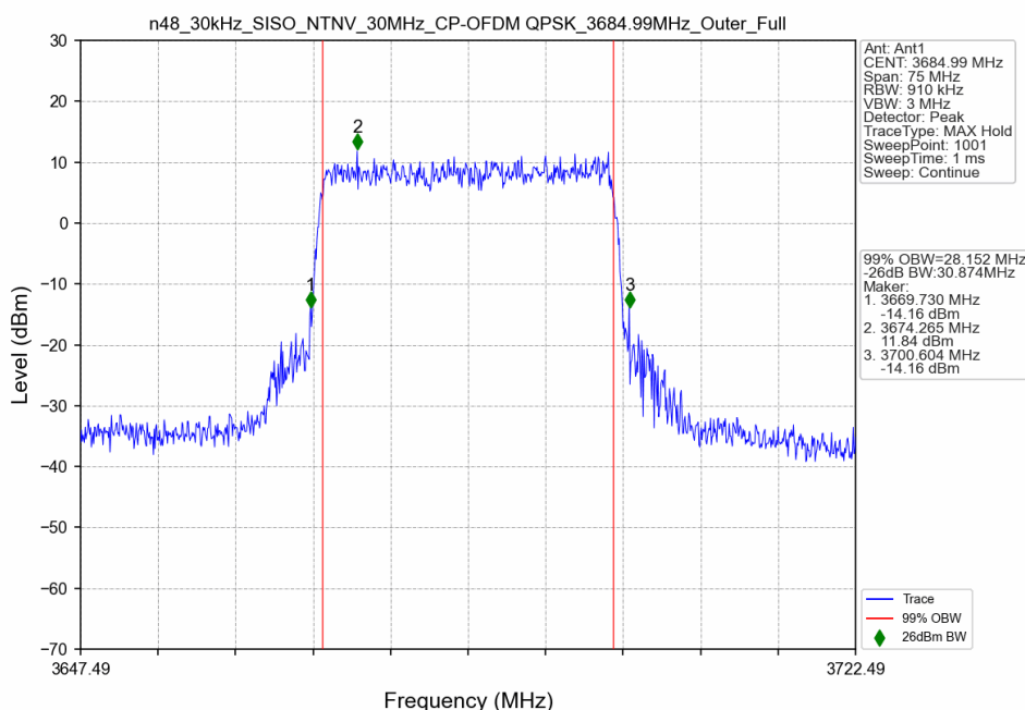
n48_30kHz_SISO_NTNV_30MHz_CP-OFDM QPSK_3684.99MHz_Outer_Full
