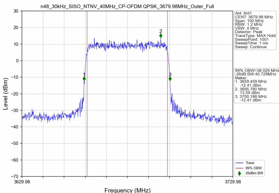
n48_30kHz_SISO_NTNV_40MHz_CP-OFDM QPSK_3679.98MHz_Outer_Full
