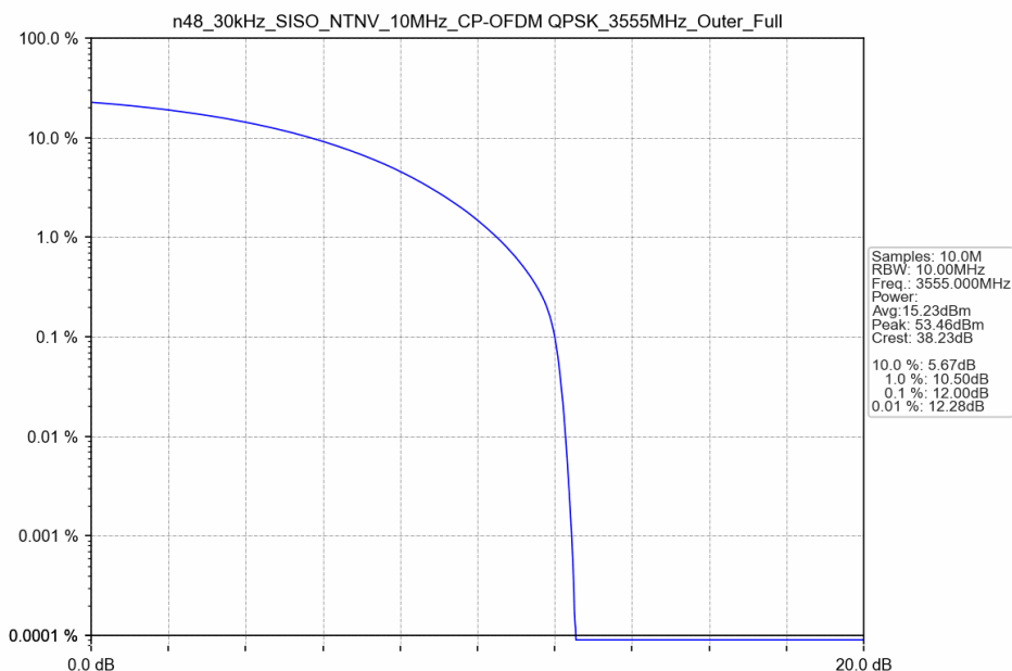
n48_30kHz_SISO_NTNV_10MHz_CP-OFDM QPSK_3555MHz_Outer_Full
