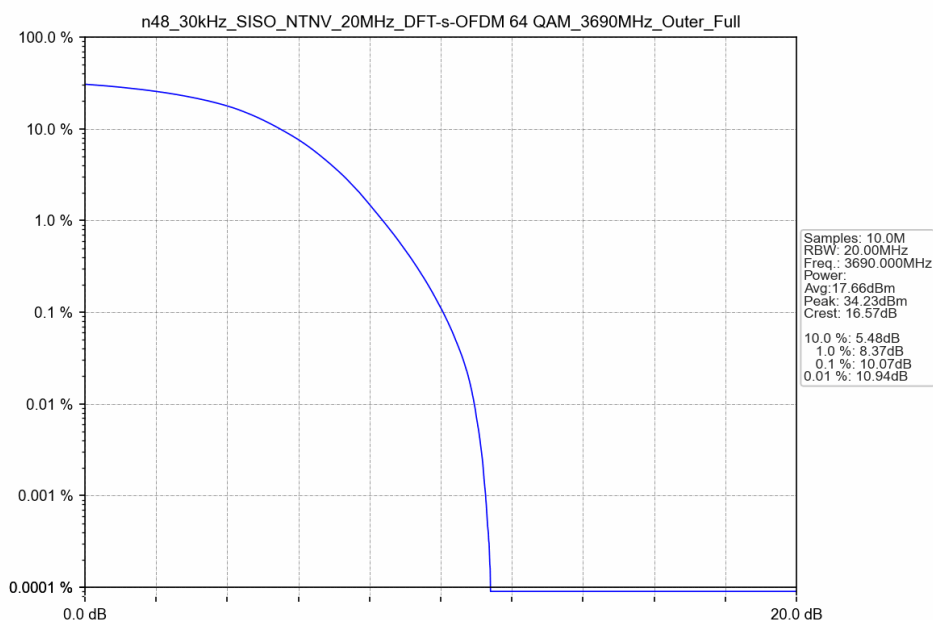
n48_30kHz_SISO_NTNV_20MHz_DFT-s-OFDM 64 QAM_3690MHz_Outer_Full
