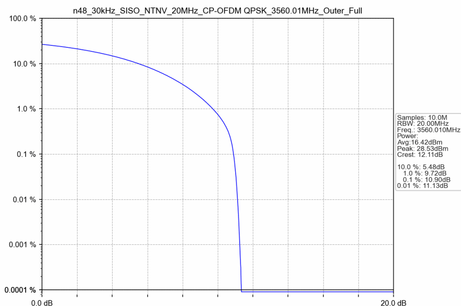
n48_30kHz_SISO_NTNV_20MHz_CP-OFDM QPSK_3560.01MHz_Outer_Full
