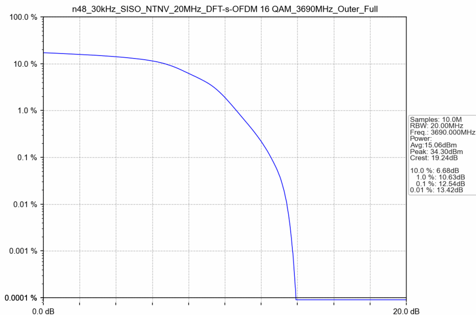
n48_30kHz_SISO_NTNV_20MHz_DFT-s-OFDM 16 QAM_3690MHz_Outer_Full
