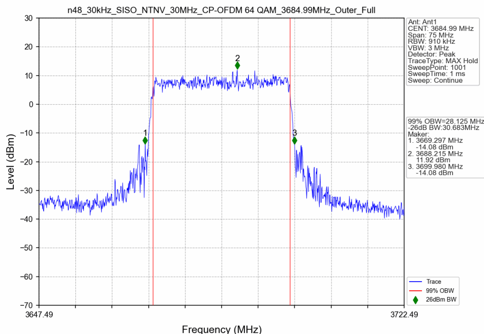
n48_30kHz_SISO_NTNV_30MHz_CP-OFDM 64 QAM_3684.99MHz_Outer_Full
