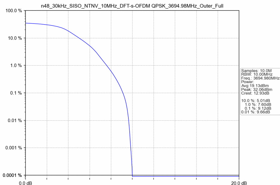
n48_30kHz_SISO_NTNV_10MHz_DFT-s-OFDM QPSK_3694.98MHz_Outer_Full
