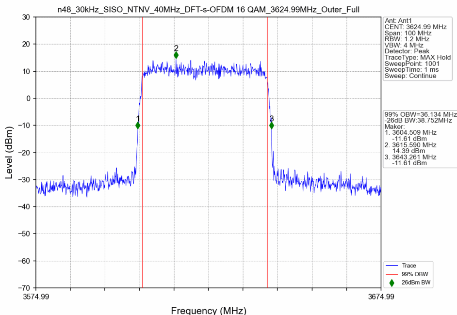
n48_30kHz_SISO_NTNV_40MHz_DFT-s-OFDM 16 QAM_3624.99MHz_Outer_Full
