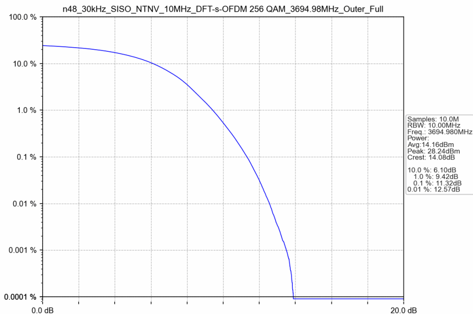
n48_30kHz_SISO_NTNV_10MHz_DFT-s-OFDM 256 QAM_3694.98MHz_Outer_Full
