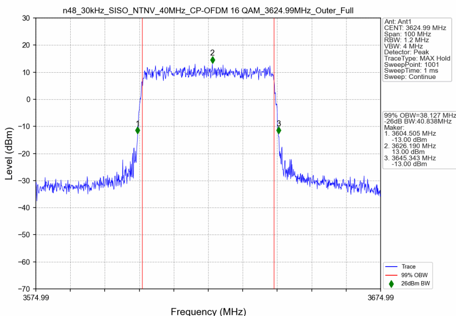
n48_30kHz_SISO_NTNV_40MHz_CP-OFDM 16 QAM_3624.99MHz_Outer_Full
