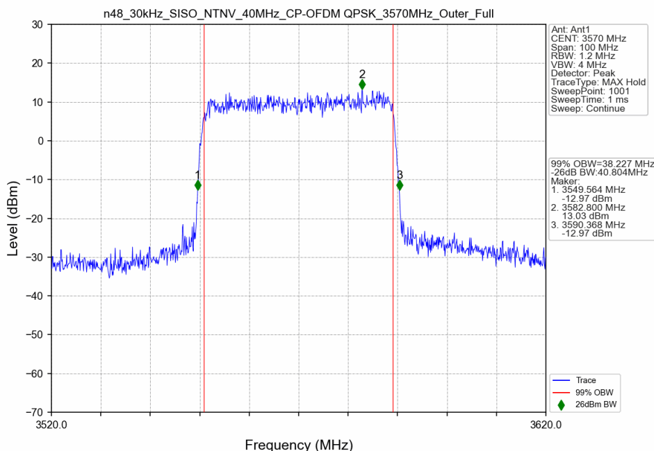
n48_30kHz_SISO_NTNV_40MHz_CP-OFDM QPSK_3570MHz_Outer_Full
