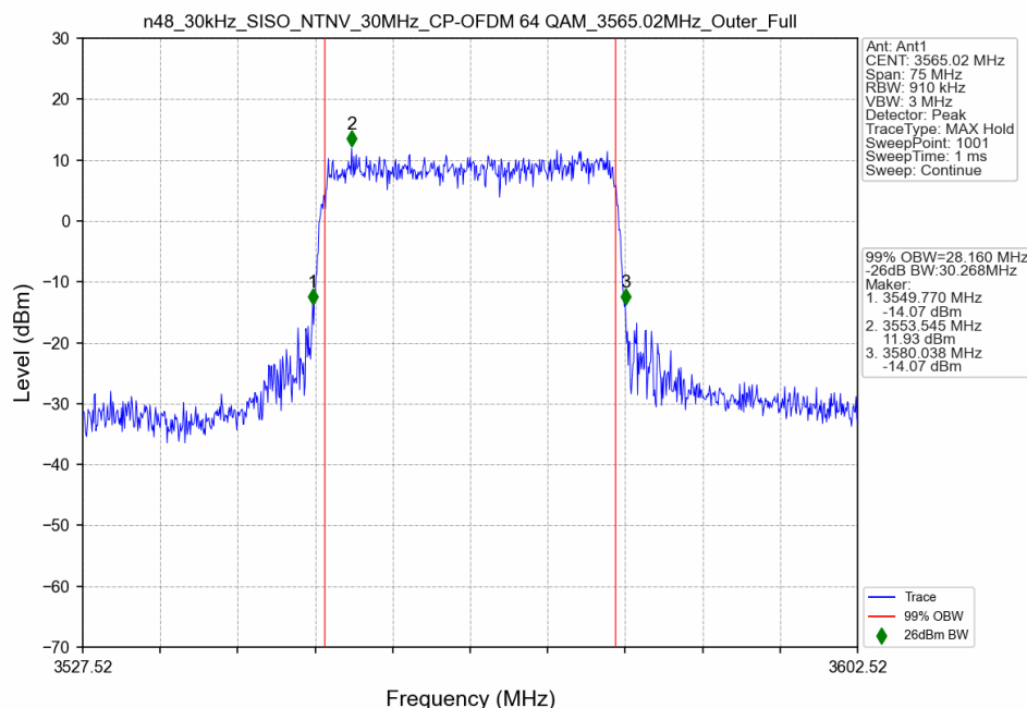
n48_30kHz_SISO_NTNV_30MHz_CP-OFDM 64 QAM_3565.02MHz_Outer_Full
