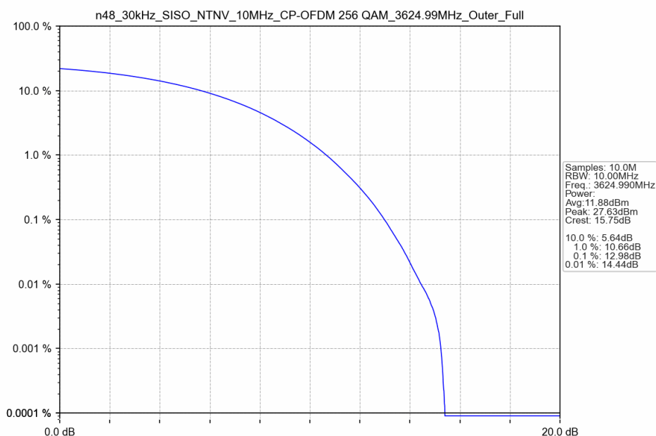
n48_30kHz_SISO_NTNV_10MHz_CP-OFDM 256 QAM_3624.99MHz_Outer_Full
