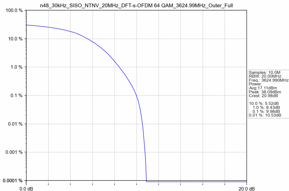
n48_30kHz_SISO_NTNV_20MHz_DFT-s-OFDM 64 QAM_3624.99MHz_Outer_Full
