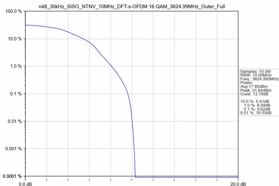
n48_30kHz_SISO_NTNV_10MHz_DFT-s-OFDM 16 QAM_3624.99MHz_Outer_Full
