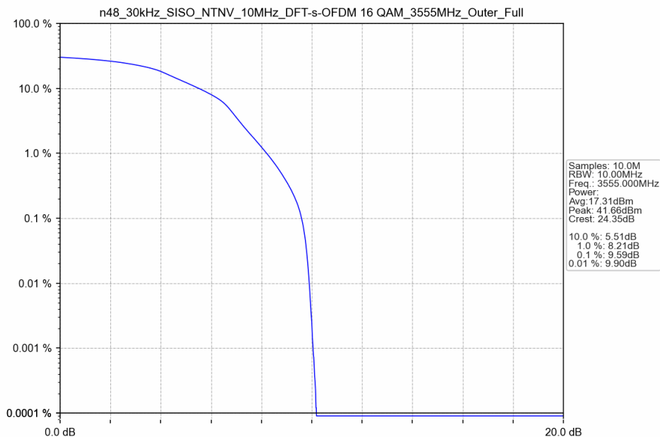
n48_30kHz_SISO_NTNV_10MHz_DFT-s-OFDM 16 QAM_3555MHz_Outer_Full
