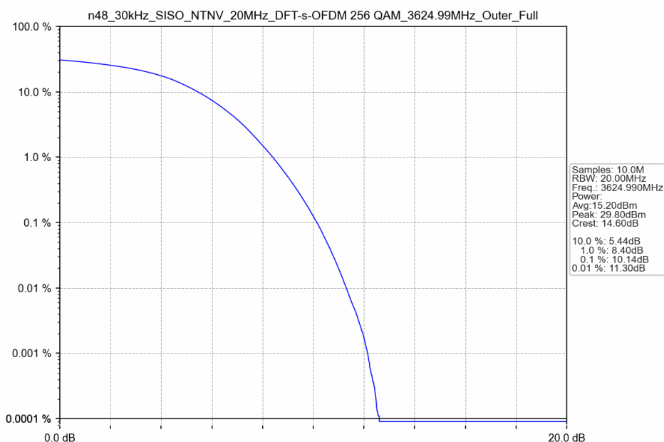
n48_30kHz_SISO_NTNV_20MHz_DFT-s-OFDM 256 QAM_3624.99MHz_Outer_Full
