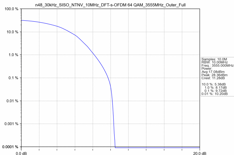
n48_30kHz_SISO_NTNV_10MHz_DFT-s-OFDM 64 QAM_3555MHz_Outer_Full
