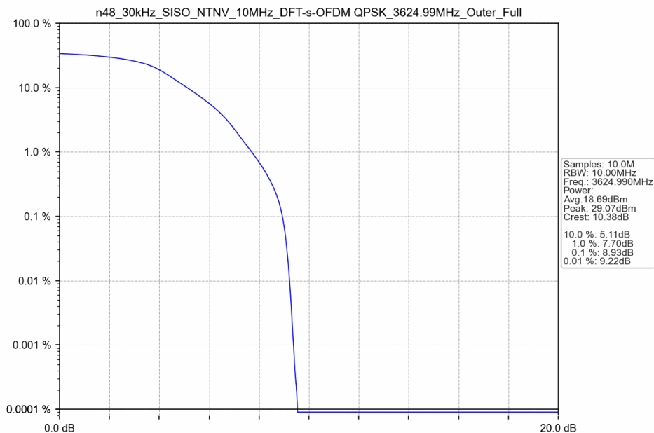
n48_30kHz_SISO_NTNV_10MHz_DFT-s-OFDM QPSK_3624.99MHz_Outer_Full
