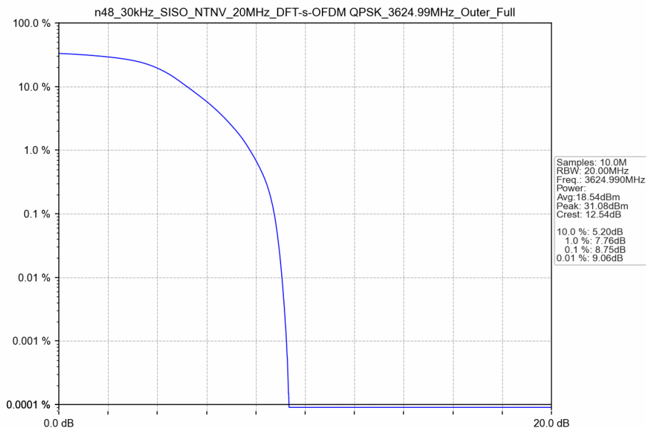
n48_30kHz_SISO_NTNV_20MHz_DFT-s-OFDM QPSK_3624.99MHz_Outer_Full
