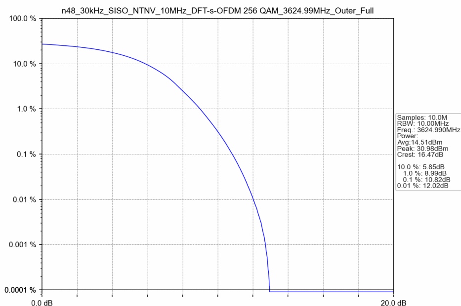
n48_30kHz_SISO_NTNV_10MHz_DFT-s-OFDM 256 QAM_3624.99MHz_Outer_Full
