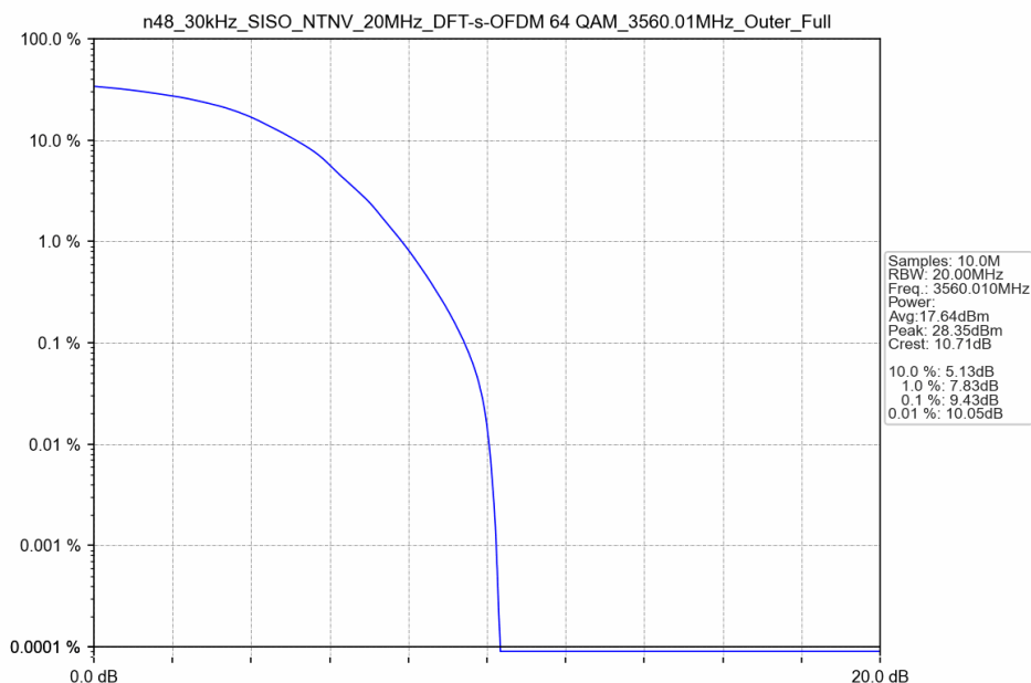
n48_30kHz_SISO_NTNV_20MHz_DFT-s-OFDM 64 QAM_3560.01MHz_Outer_Full
