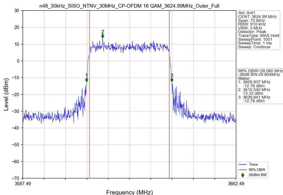
n48_30kHz_SISO_NTNV_30MHz_CP-OFDM 16 QAM_3624.99MHz_Outer_Full
