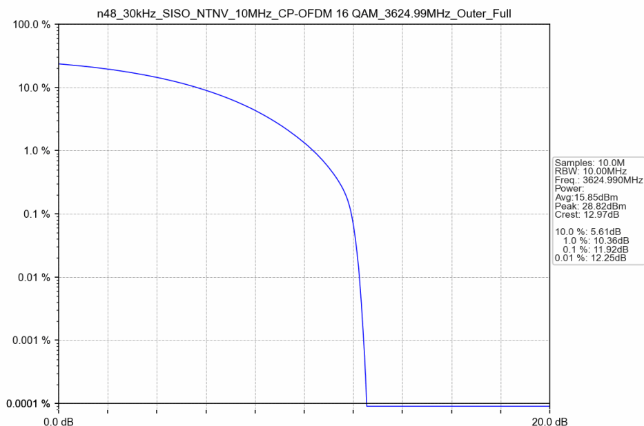
n48_30kHz_SISO_NTNV_10MHz_CP-OFDM 16 QAM_3624.99MHz_Outer_Full
