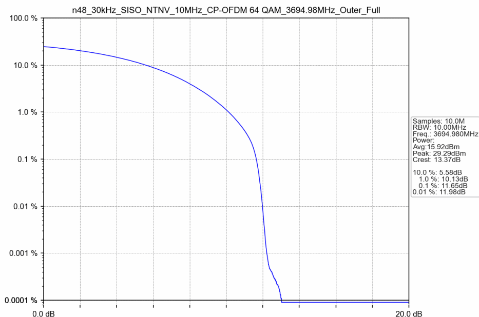
n48_30kHz_SISO_NTNV_10MHz_CP-OFDM 64 QAM_3694.98MHz_Outer_Full
