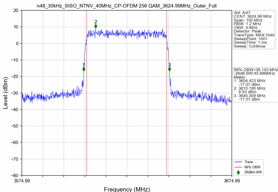
n48_30kHz_SISO_NTNV_40MHz_CP-OFDM 256 QAM_3624.99MHz_Outer_Full
