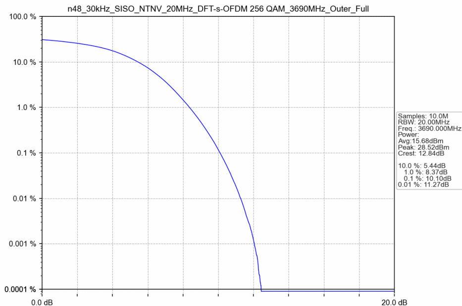
n48_30kHz_SISO_NTNV_20MHz_DFT-s-OFDM 256 QAM_3690MHz_Outer_Full
