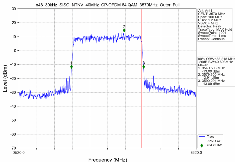
n48_30kHz_SISO_NTNV_40MHz_CP-OFDM 64 QAM_3570MHz_Outer_Full
