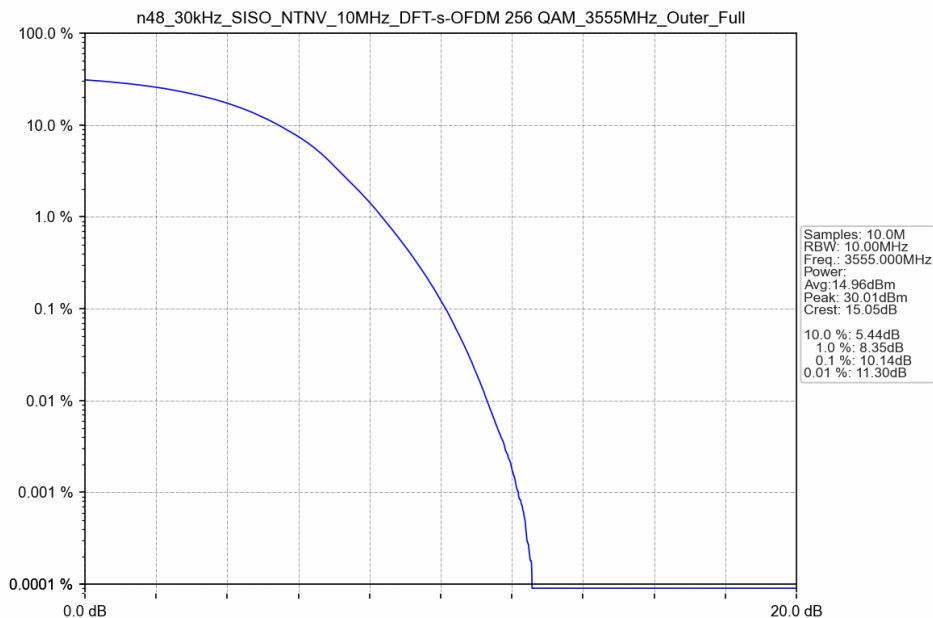
n48_30kHz_SISO_NTNV_10MHz_DFT-s-OFDM 256 QAM_3555MHz_Outer_Full
