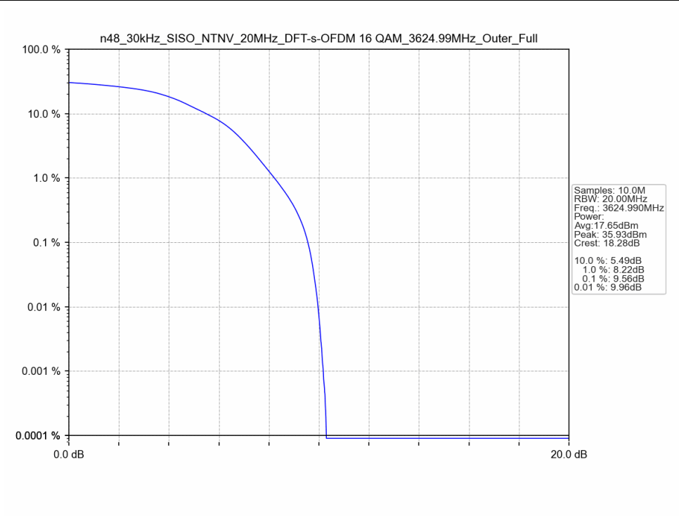
n48_30kHz_SISO_NTNV_20MHz_DFT-s-OFDM 16 QAM_3624.99MHz_Outer_Full
