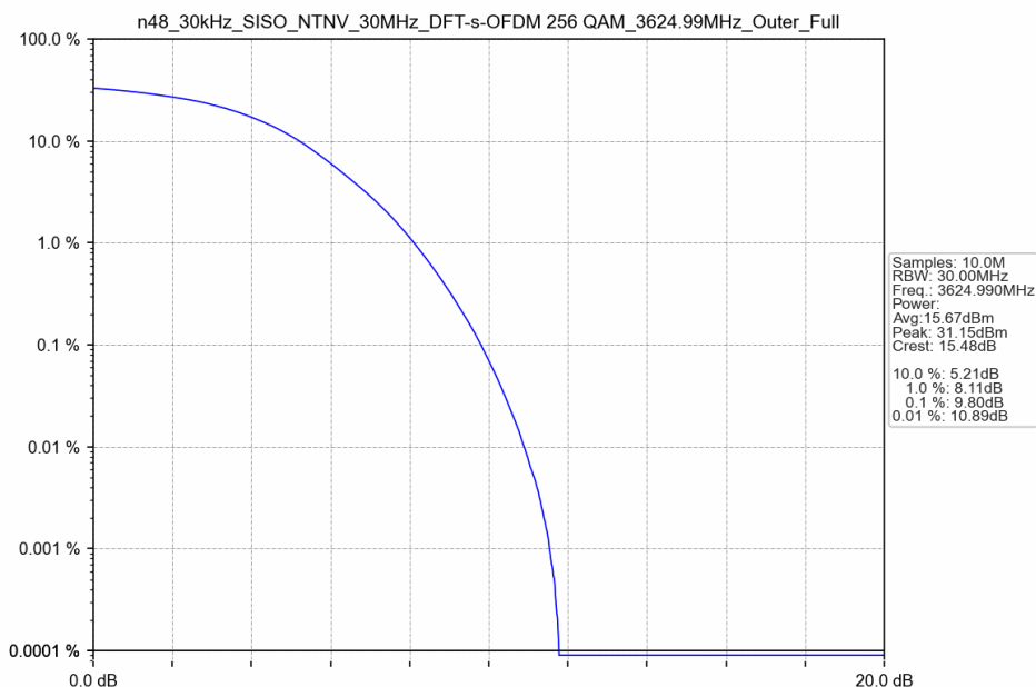
n48_30kHz_SISO_NTNV_30MHz_DFT-s-OFDM 256 QAM_3624.99MHz_Outer_Full
