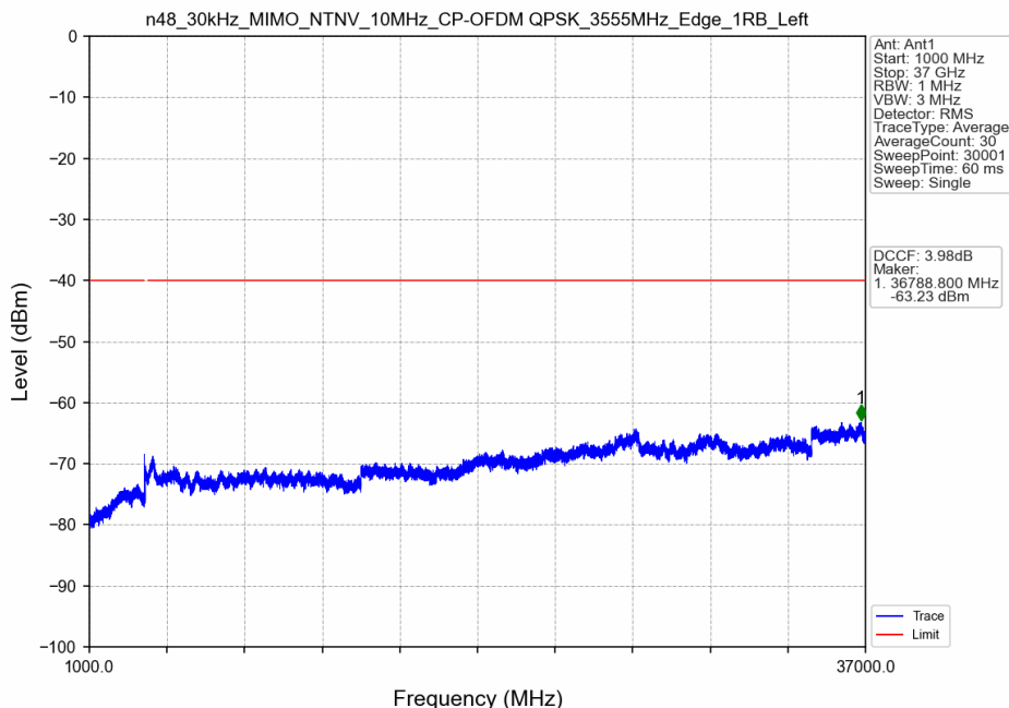
n48_30kHz_MIMO_NTNV_10MHz_CP-OFDM QPSK_3555MHz_Edge_1RB_Left
