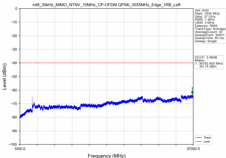
n48_30kHz_MIMO_NTNV_10MHz_CP-OFDM QPSK_3555MHz_Edge_1RB_Left
