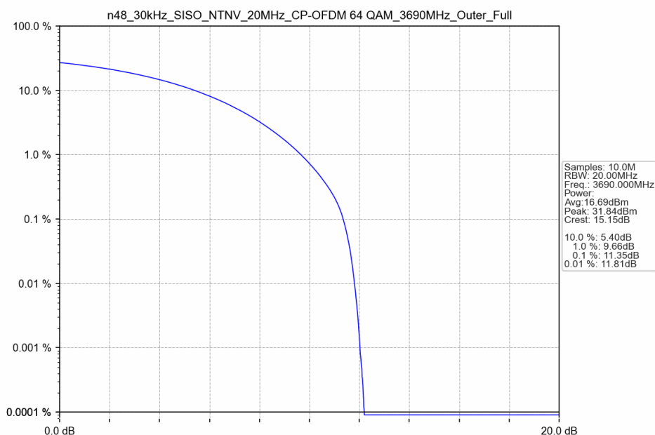
n48_30kHz_SISO_NTNV_20MHz_CP-OFDM 64 QAM_3690MHz_Outer_Full
