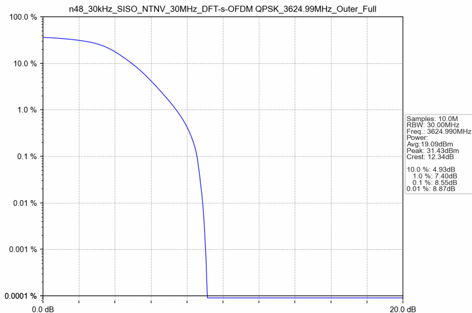
n48_30kHz_SISO_NTNV_30MHz_DFT-s-OFDM QPSK_3624.99MHz_Outer_Full
