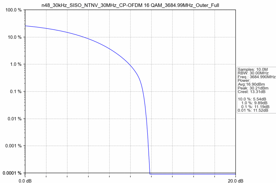
n48_30kHz_SISO_NTNV_30MHz_CP-OFDM 16 QAM_3684.99MHz_Outer_Full
