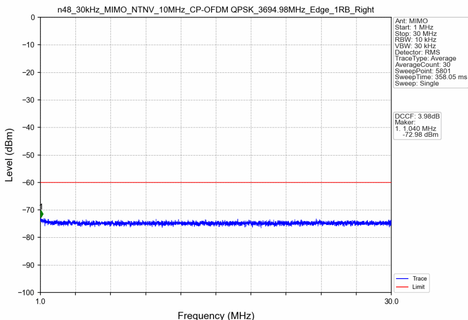
n48_30kHz_MIMO_NTNV_10MHz_CP-OFDM QPSK_3694.98MHz_Edge_1RB_Right
