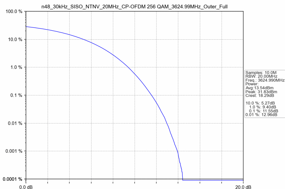
n48_30kHz_SISO_NTNV_20MHz_CP-OFDM 256 QAM_3624.99MHz_Outer_Full
