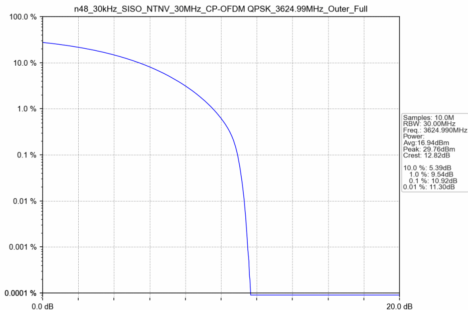
n48_30kHz_SISO_NTNV_30MHz_CP-OFDM QPSK_3624.99MHz_Outer_Full
