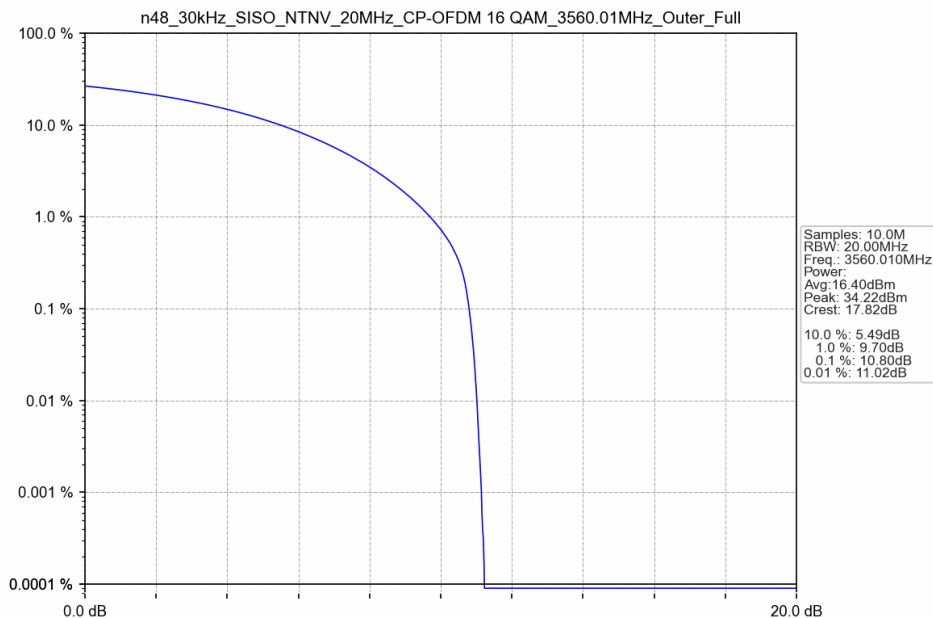
n48_30kHz_SISO_NTNV_20MHz_CP-OFDM 16 QAM_3560.01MHz_Outer_Full
