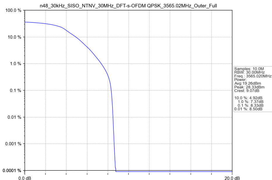
n48_30kHz_SISO_NTNV_30MHz_DFT-s-OFDM QPSK_3565.02MHz_Outer_Full
