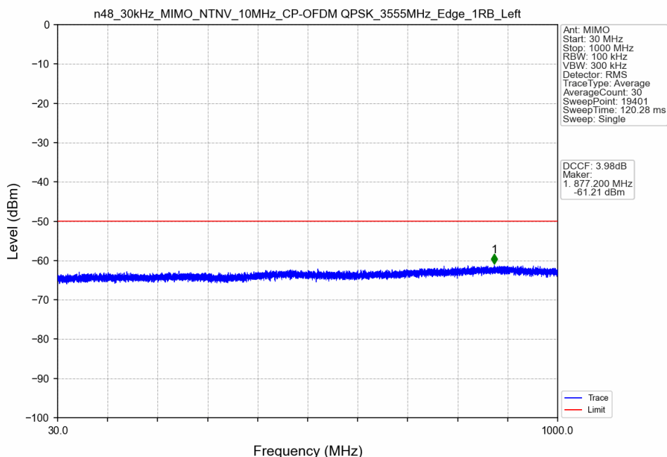
n48_30kHz_MIMO_NTNV_10MHz_CP-OFDM QPSK_3555MHz_Edge_1RB_Left
