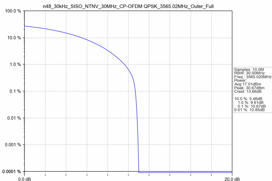
n48_30kHz_SISO_NTNV_30MHz_CP-OFDM QPSK_3565.02MHz_Outer_Full
