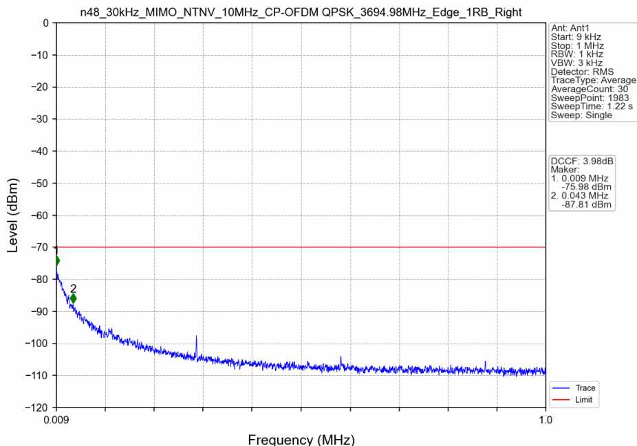
n48_30kHz_MIMO_NTNV_10MHz_CP-OFDM QPSK_3694.98MHz_Edge_1RB_Right
