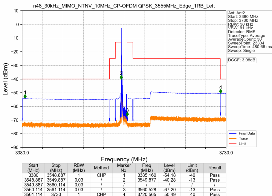
n48_30kHz_MIMO_NTNV_10MHz_CP-OFDM QPSK_3555MHz_Edge_1RB_Left
