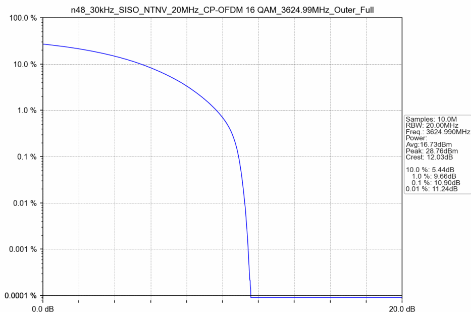
n48_30kHz_SISO_NTNV_20MHz_CP-OFDM 16 QAM_3624.99MHz_Outer_Full
