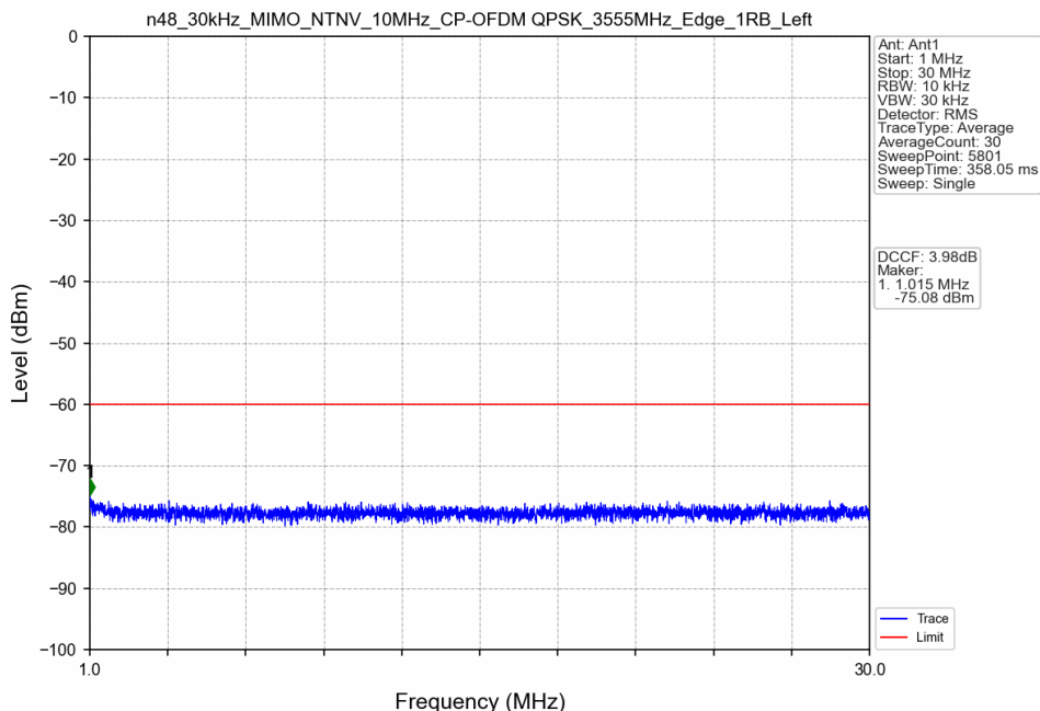
n48_30kHz_MIMO_NTNV_10MHz_CP-OFDM QPSK_3555MHz_Edge_1RB_Left
