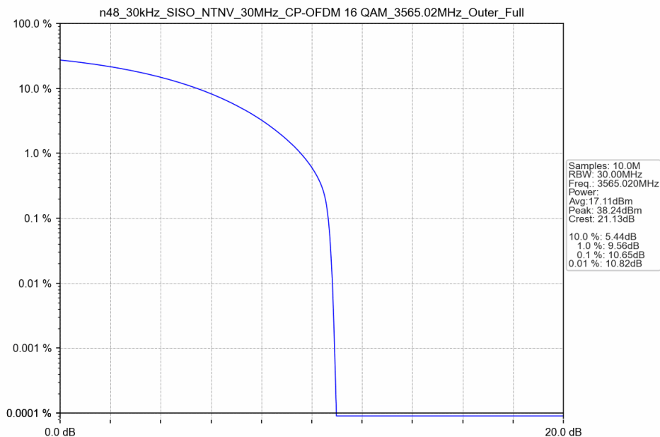
n48_30kHz_SISO_NTNV_30MHz_CP-OFDM 16 QAM_3565.02MHz_Outer_Full
