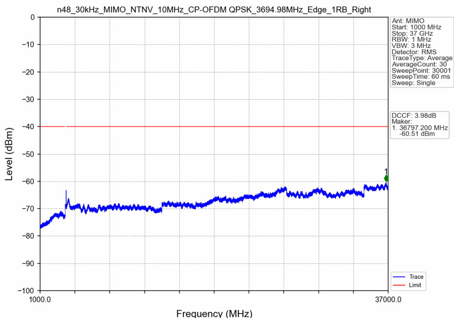
n48_30kHz_MIMO_NTNV_10MHz_CP-OFDM QPSK_3694.98MHz_Edge_1RB_Right
