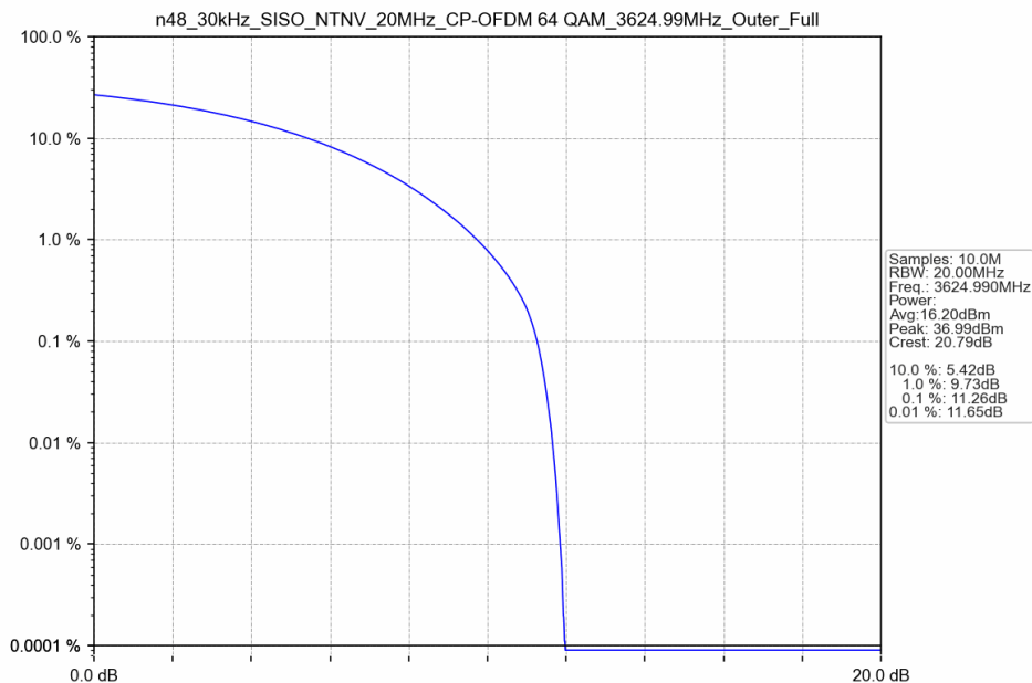
n48_30kHz_SISO_NTNV_20MHz_CP-OFDM 64 QAM_3624.99MHz_Outer_Full
