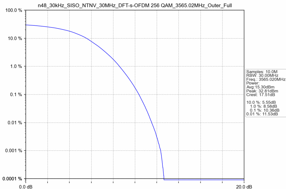
n48_30kHz_SISO_NTNV_30MHz_DFT-s-OFDM 256 QAM_3565.02MHz_Outer_Full
