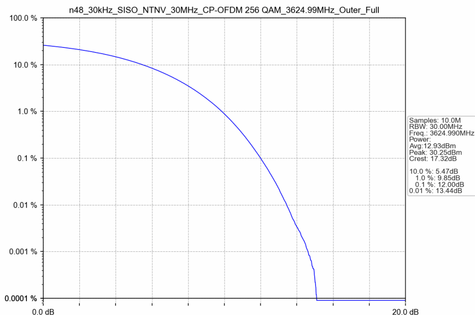
n48_30kHz_SISO_NTNV_30MHz_CP-OFDM 256 QAM_3624.99MHz_Outer_Full
