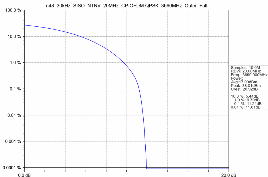
n48_30kHz_SISO_NTNV_20MHz_CP-OFDM QPSK_3690MHz_Outer_Full
