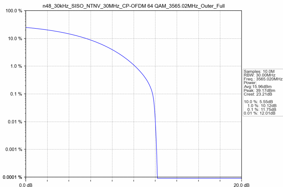
n48_30kHz_SISO_NTNV_30MHz_CP-OFDM 64 QAM_3565.02MHz_Outer_Full
