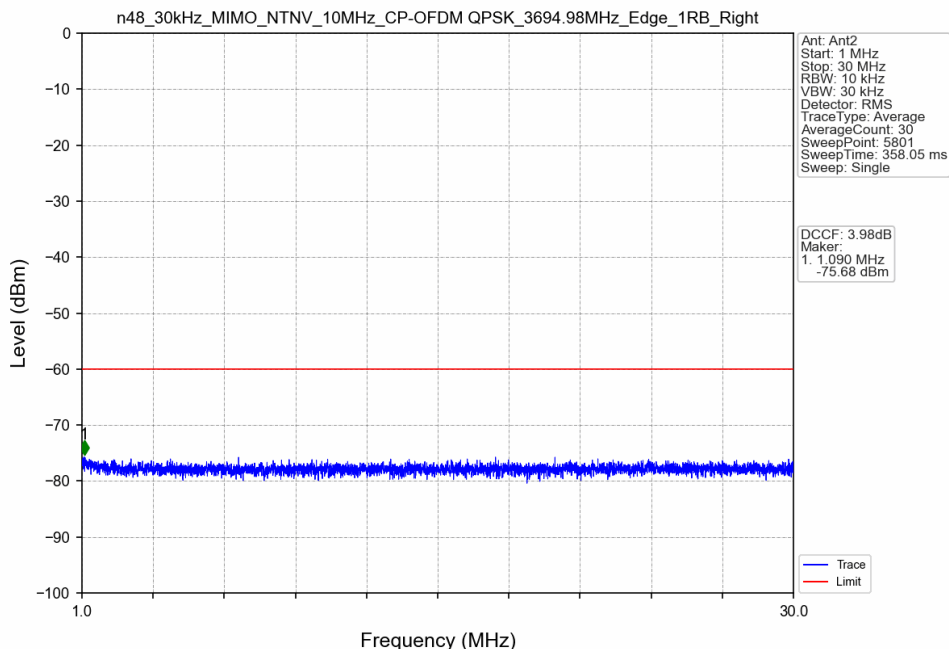
n48_30kHz_MIMO_NTNV_10MHz_CP-OFDM QPSK_3694.98MHz_Edge_1RB_Right
