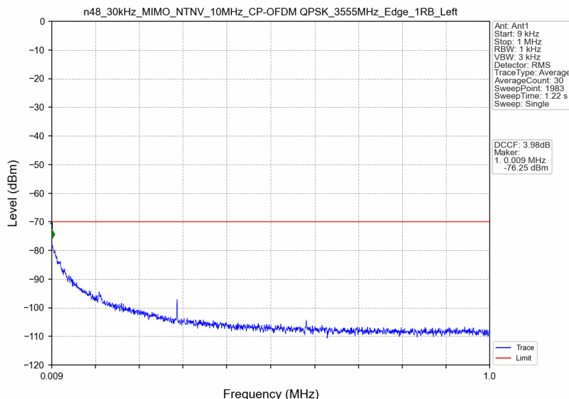
n48_30kHz_MIMO_NTNV_10MHz_CP-OFDM QPSK_3555MHz_Edge_1RB_Left
