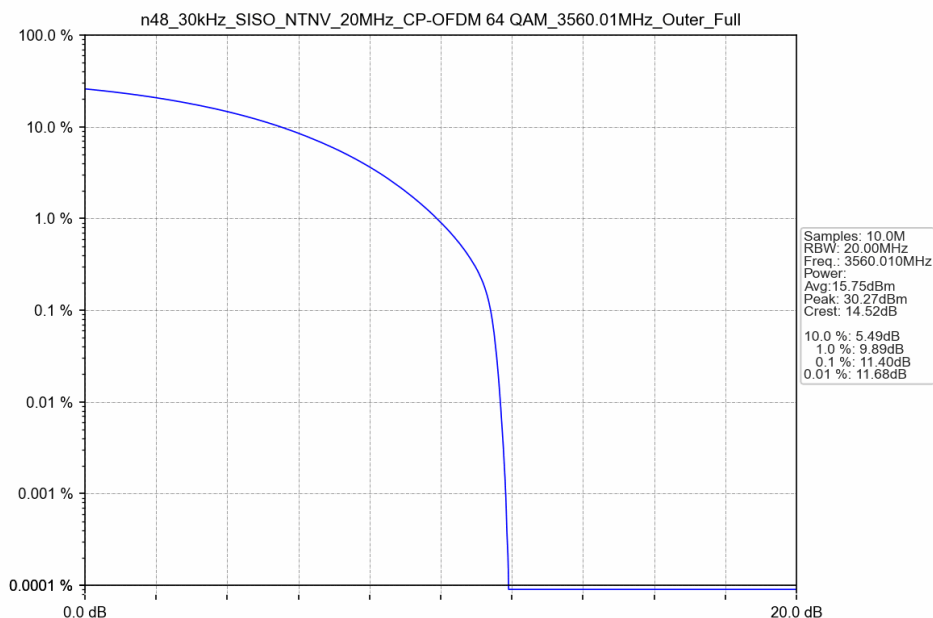
n48_30kHz_SISO_NTNV_20MHz_CP-OFDM 64 QAM_3560.01MHz_Outer_Full
