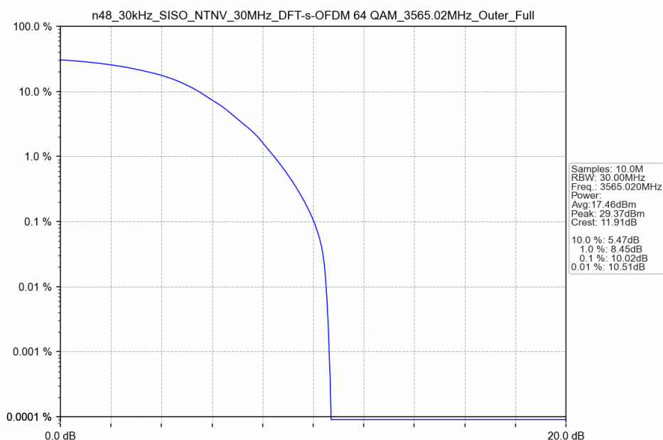
n48_30kHz_SISO_NTNV_30MHz_DFT-s-OFDM 64 QAM_3565.02MHz_Outer_Full
