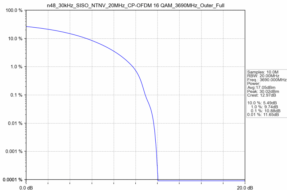
n48_30kHz_SISO_NTNV_20MHz_CP-OFDM 16 QAM_3690MHz_Outer_Full
