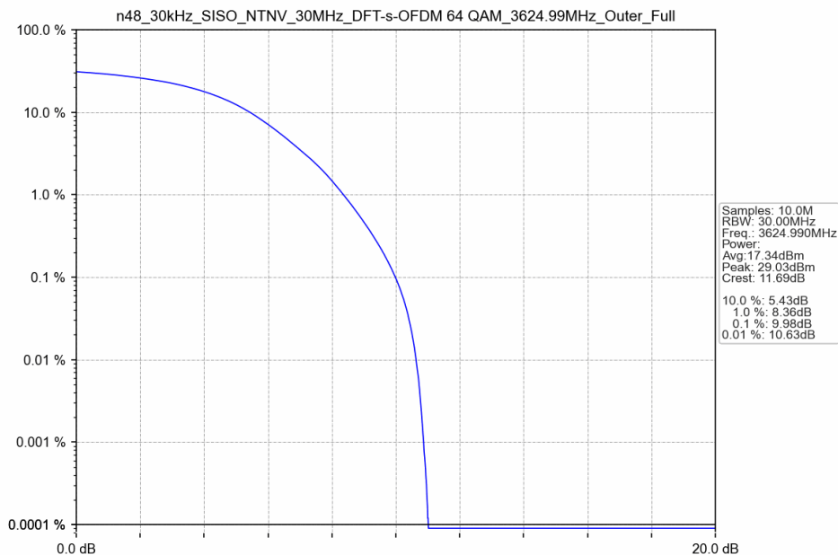
n48_30kHz_SISO_NTNV_30MHz_DFT-s-OFDM 64 QAM_3624.99MHz_Outer_Full
