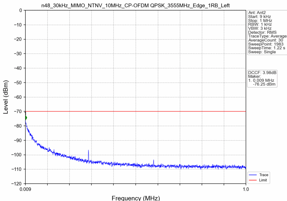
n48_30kHz_MIMO_NTNV_10MHz_CP-OFDM QPSK_3555MHz_Edge_1RB_Left
