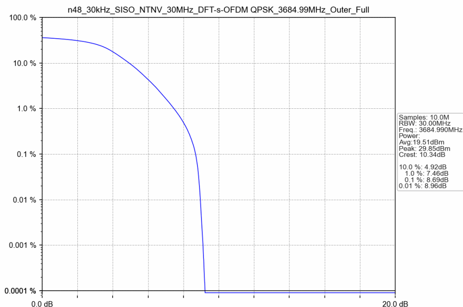
n48_30kHz_SISO_NTNV_30MHz_DFT-s-OFDM QPSK_3684.99MHz_Outer_Full
