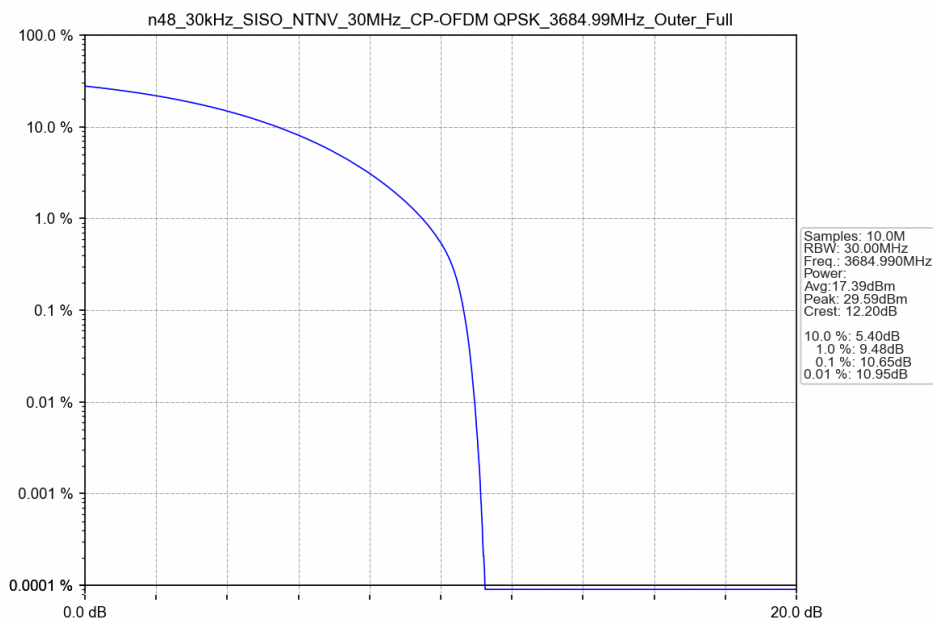
n48_30kHz_SISO_NTNV_30MHz_CP-OFDM QPSK_3684.99MHz_Outer_Full
