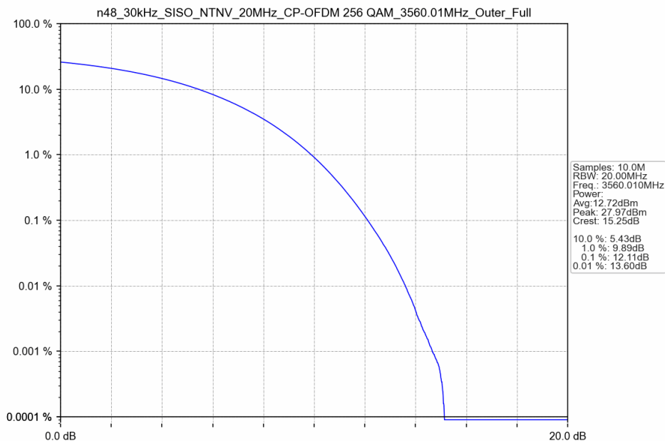
n48_30kHz_SISO_NTNV_20MHz_CP-OFDM 256 QAM_3560.01MHz_Outer_Full
