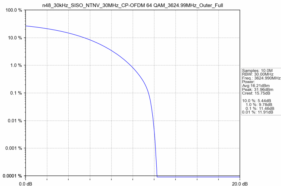
n48_30kHz_SISO_NTNV_30MHz_CP-OFDM 64 QAM_3624.99MHz_Outer_Full
