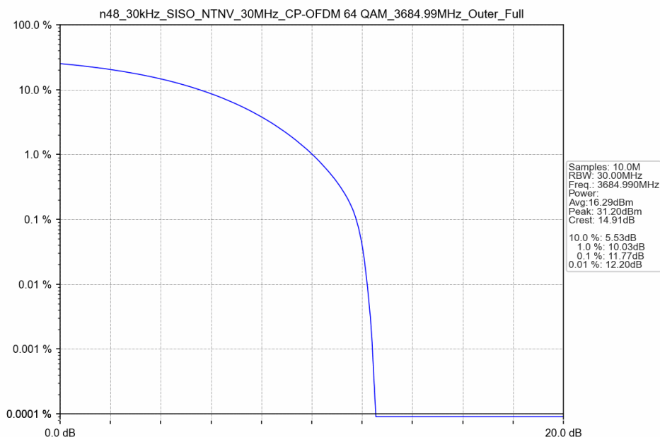
n48_30kHz_SISO_NTNV_30MHz_CP-OFDM 64 QAM_3684.99MHz_Outer_Full
