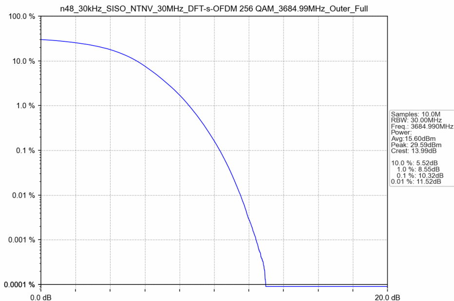
n48_30kHz_SISO_NTNV_30MHz_DFT-s-OFDM 256 QAM_3684.99MHz_Outer_Full
