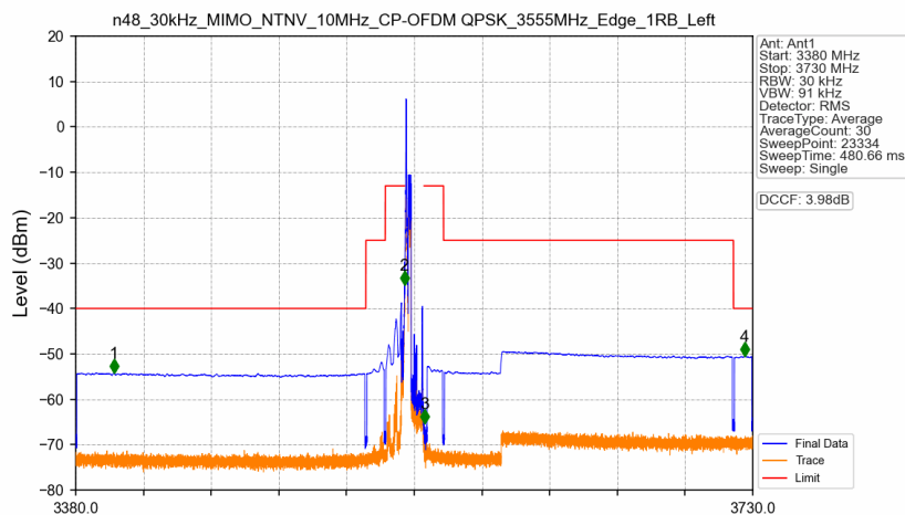
n48_30kHz_MIMO_NTNV_10MHz_CP-OFDM QPSK_3555MHz_Edge_1RB_Left
