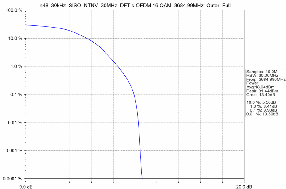
n48_30kHz_SISO_NTNV_30MHz_DFT-s-OFDM 16 QAM_3684.99MHz_Outer_Full
