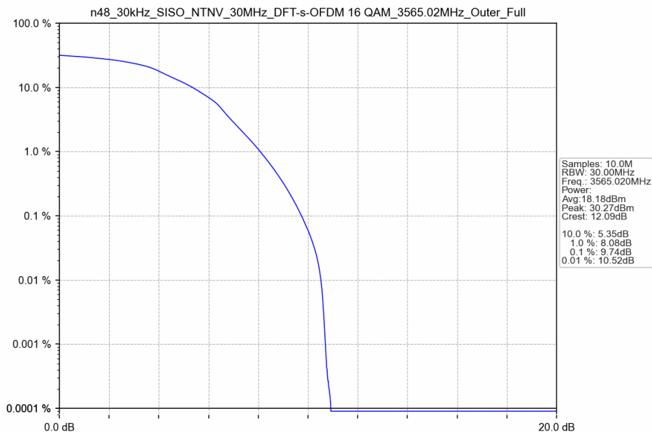
n48_30kHz_SISO_NTNV_30MHz_DFT-s-OFDM 16 QAM_3565.02MHz_Outer_Full
