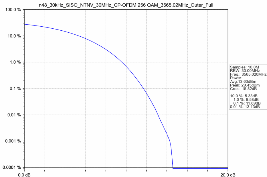
n48_30kHz_SISO_NTNV_30MHz_CP-OFDM 256 QAM_3565.02MHz_Outer_Full
