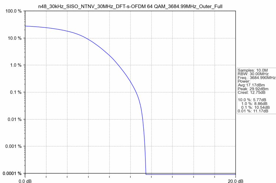
n48_30kHz_SISO_NTNV_30MHz_DFT-s-OFDM 64 QAM_3684.99MHz_Outer_Full
