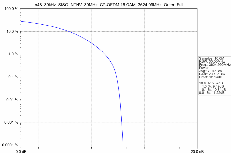
n48_30kHz_SISO_NTNV_30MHz_CP-OFDM 16 QAM_3624.99MHz_Outer_Full
