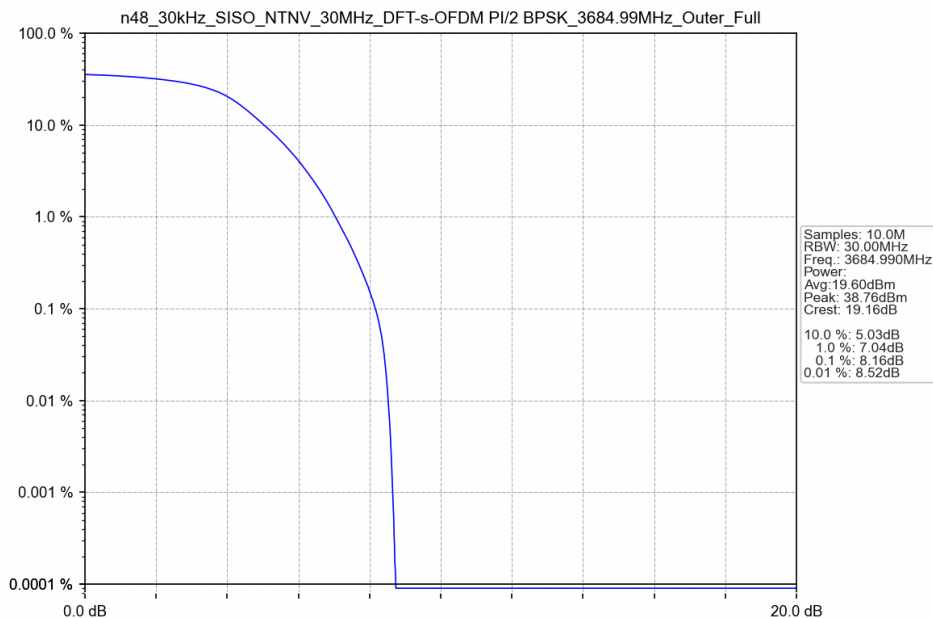
n48_30kHz_SISO_NTNV_30MHz_DFT-s-OFDM PI/2 BPSK_3684.99MHz_Outer_Full
