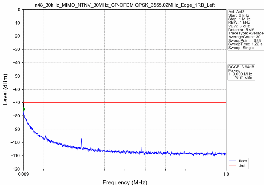
n48_30kHz_MIMO_NTNV_30MHz_CP-OFDM QPSK_3565.02MHz_Edge_1RB_Left
