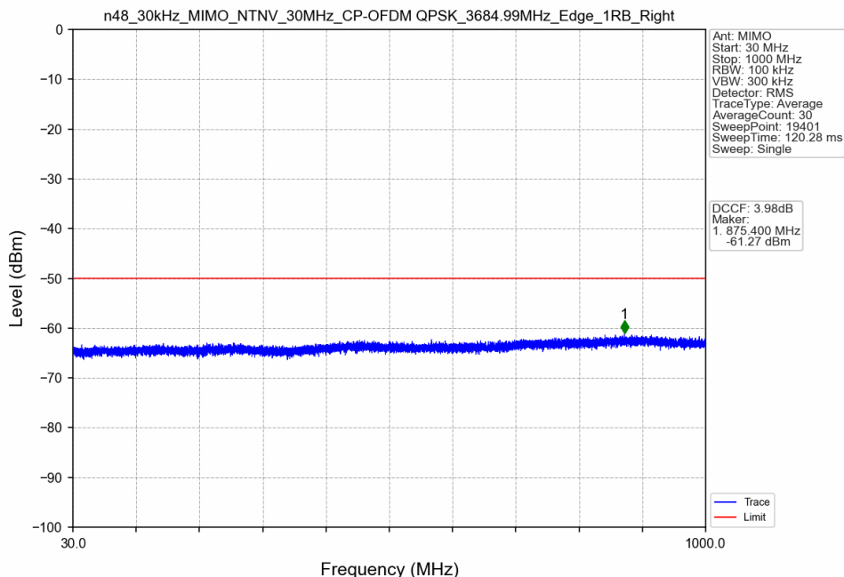
n48_30kHz_MIMO_NTNV_30MHz_CP-OFDM QPSK_3684.99MHz_Edge_1RB_Right
