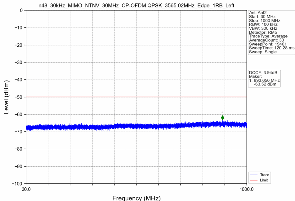
n48_30kHz_MIMO_NTNV_30MHz_CP-OFDM QPSK_3565.02MHz_Edge_1RB_Left
