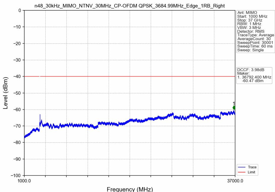
n48_30kHz_MIMO_NTNV_30MHz_CP-OFDM QPSK_3684.99MHz_Edge_1RB_Right
