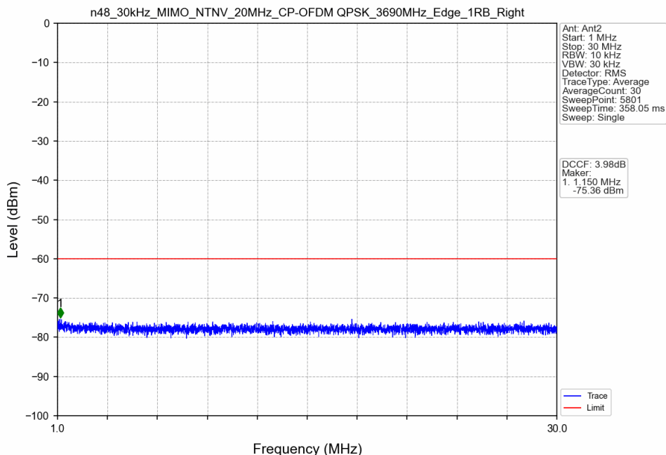
n48_30kHz_MIMO_NTNV_20MHz_CP-OFDM QPSK_3690MHz_Edge_1RB_Right
