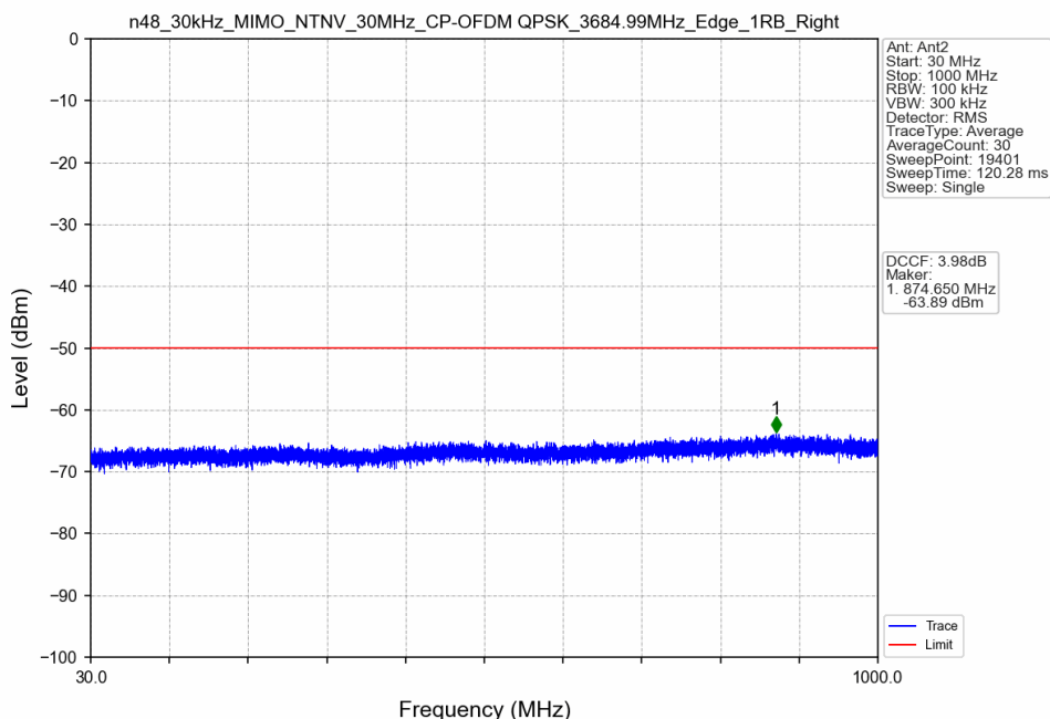
n48_30kHz_MIMO_NTNV_30MHz_CP-OFDM QPSK_3684.99MHz_Edge_1RB_Right
