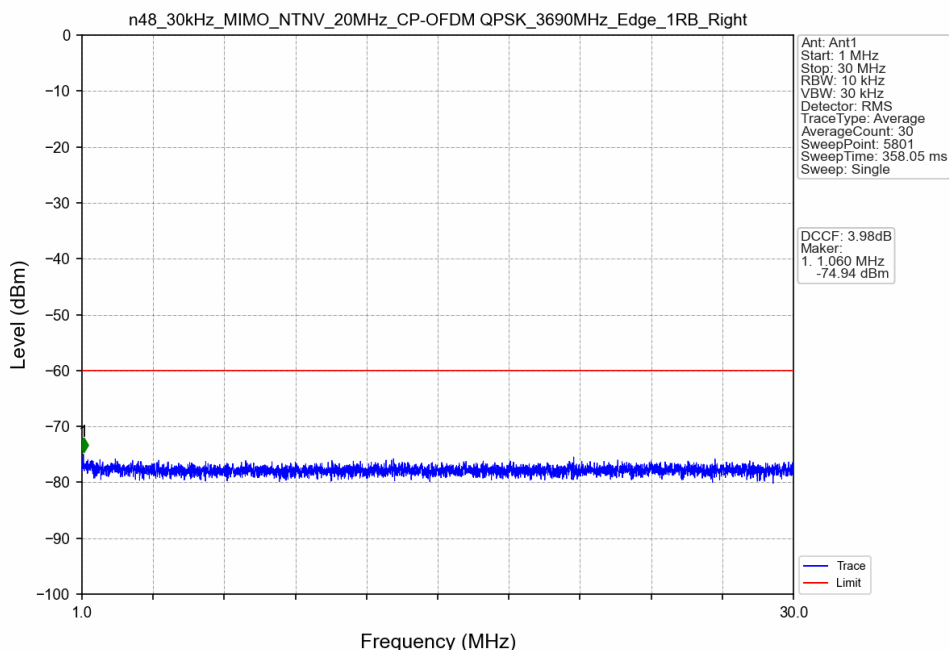
n48_30kHz_MIMO_NTNV_20MHz_CP-OFDM QPSK_3690MHz_Edge_1RB_Right
