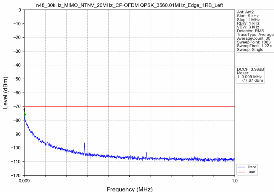
n48_30kHz_MIMO_NTNV_20MHz_CP-OFDM QPSK_3560.01MHz_Edge_1RB_Left
