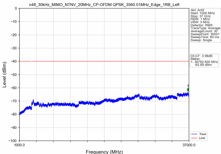
n48_30kHz_MIMO_NTNV_20MHz_CP-OFDM QPSK_3560.01MHz_Edge_1RB_Left
