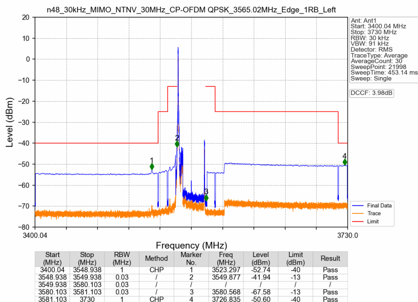
n48_30kHz_MIMO_NTNV_30MHz_CP-OFDM QPSK_3565.02MHz_Edge_1RB_Left
