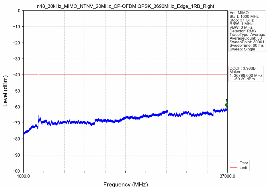
n48_30kHz_MIMO_NTNV_20MHz_CP-OFDM QPSK_3690MHz_Edge_1RB_Right
