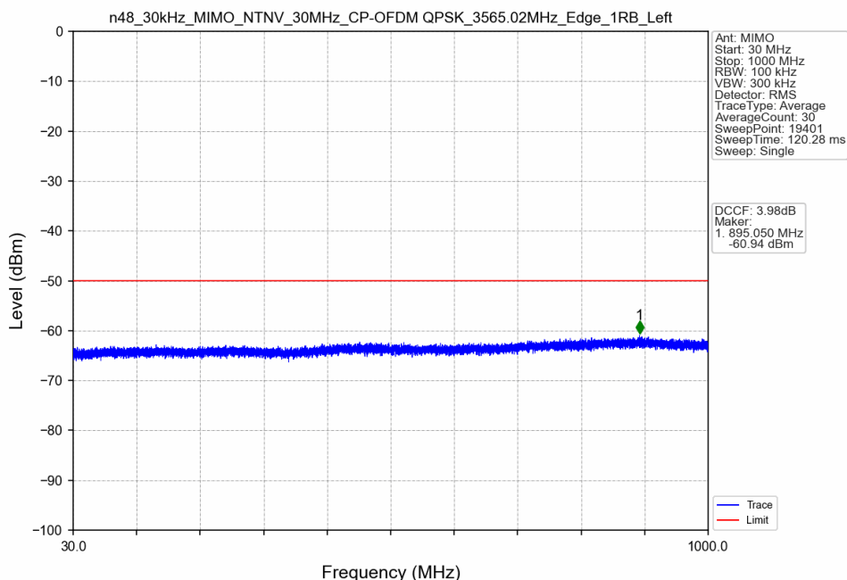
n48_30kHz_MIMO_NTNV_30MHz_CP-OFDM QPSK_3565.02MHz_Edge_1RB_Left
