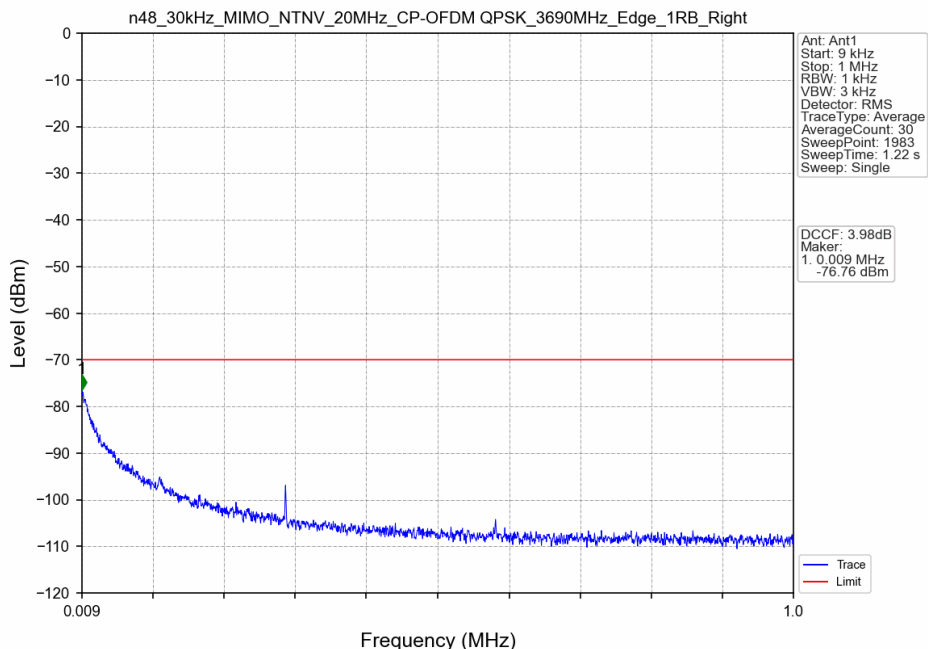
n48_30kHz_MIMO_NTNV_20MHz_CP-OFDM QPSK_3690MHz_Edge_1RB_Right
