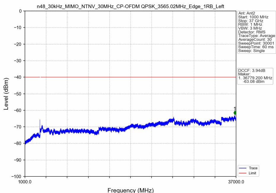
n48_30kHz_MIMO_NTNV_30MHz_CP-OFDM QPSK_3565.02MHz_Edge_1RB_Left
