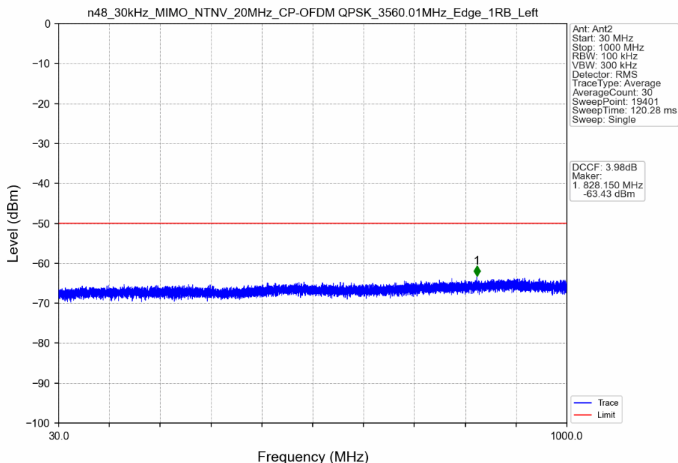
n48_30kHz_MIMO_NTNV_20MHz_CP-OFDM QPSK_3560.01MHz_Edge_1RB_Left
