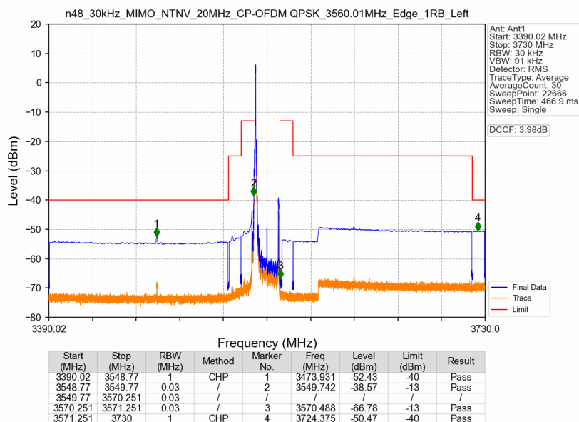
n48_30kHz_MIMO_NTNV_20MHz_CP-OFDM QPSK_3560.01MHz_Edge_1RB_Left
