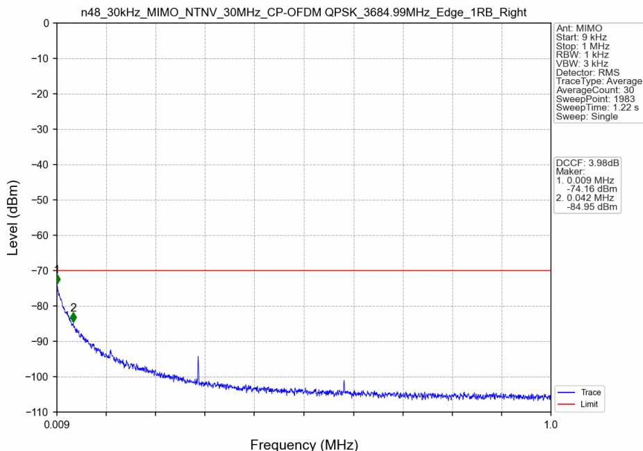
n48_30kHz_MIMO_NTNV_30MHz_CP-OFDM QPSK_3684.99MHz_Edge_1RB_Right
