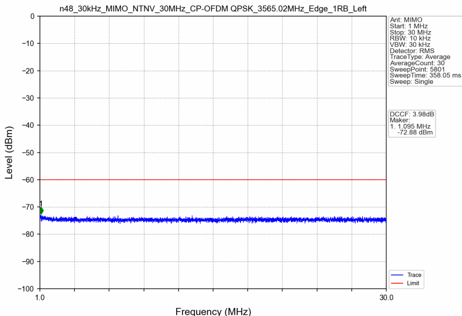
n48_30kHz_MIMO_NTNV_30MHz_CP-OFDM QPSK_3565.02MHz_Edge_1RB_Left
