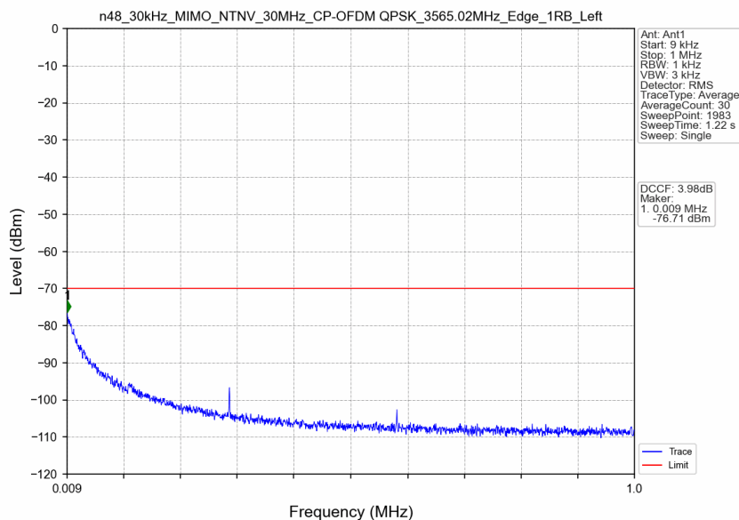
n48_30kHz_MIMO_NTNV_30MHz_CP-OFDM QPSK_3565.02MHz_Edge_1RB_Left
