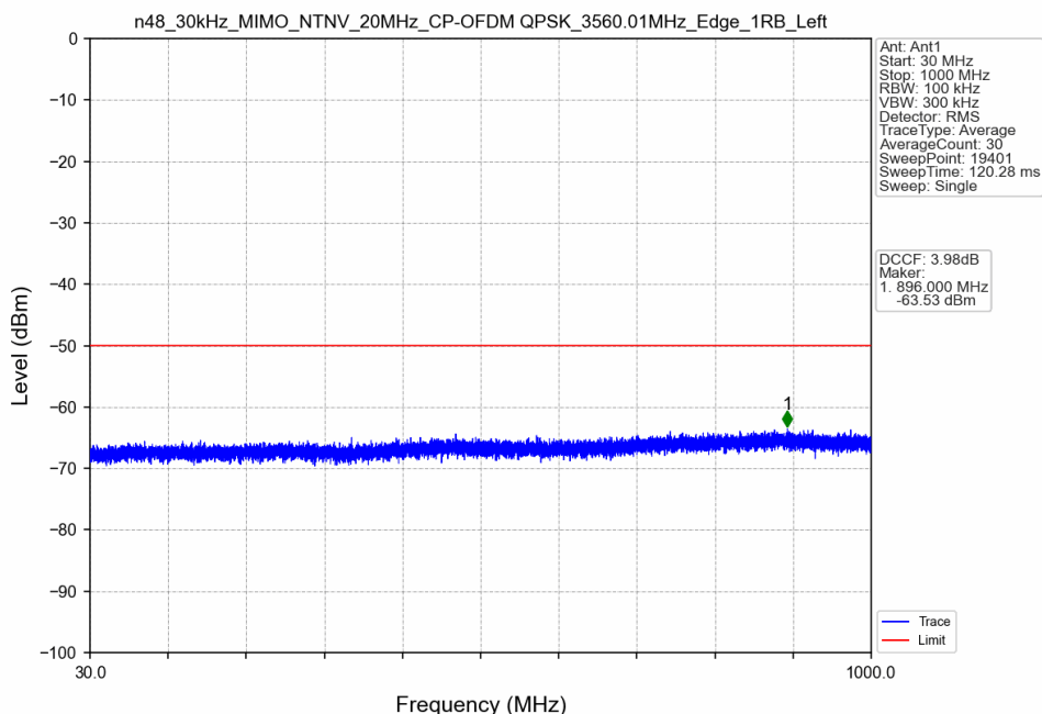
n48_30kHz_MIMO_NTNV_20MHz_CP-OFDM QPSK_3560.01MHz_Edge_1RB_Left
