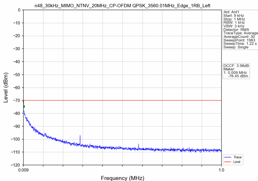
n48_30kHz_MIMO_NTNV_20MHz_CP-OFDM QPSK_3560.01MHz_Edge_1RB_Left
