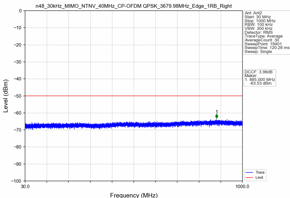
n48_30kHz_MIMO_NTNV_40MHz_CP-OFDM QPSK_3679.98MHz_Edge_1RB_Right
