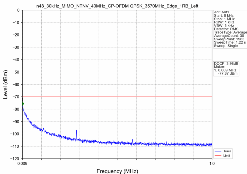
n48_30kHz_MIMO_NTNV_40MHz_CP-OFDM QPSK_3570MHz_Edge_1RB_Left
