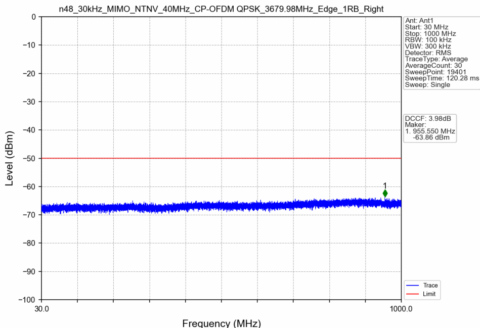
n48_30kHz_MIMO_NTNV_40MHz_CP-OFDM QPSK_3679.98MHz_Edge_1RB_Right
