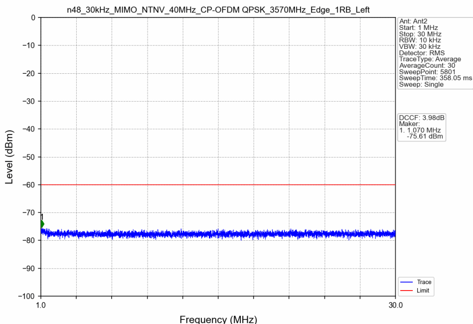
n48_30kHz_MIMO_NTNV_40MHz_CP-OFDM QPSK_3570MHz_Edge_1RB_Left
