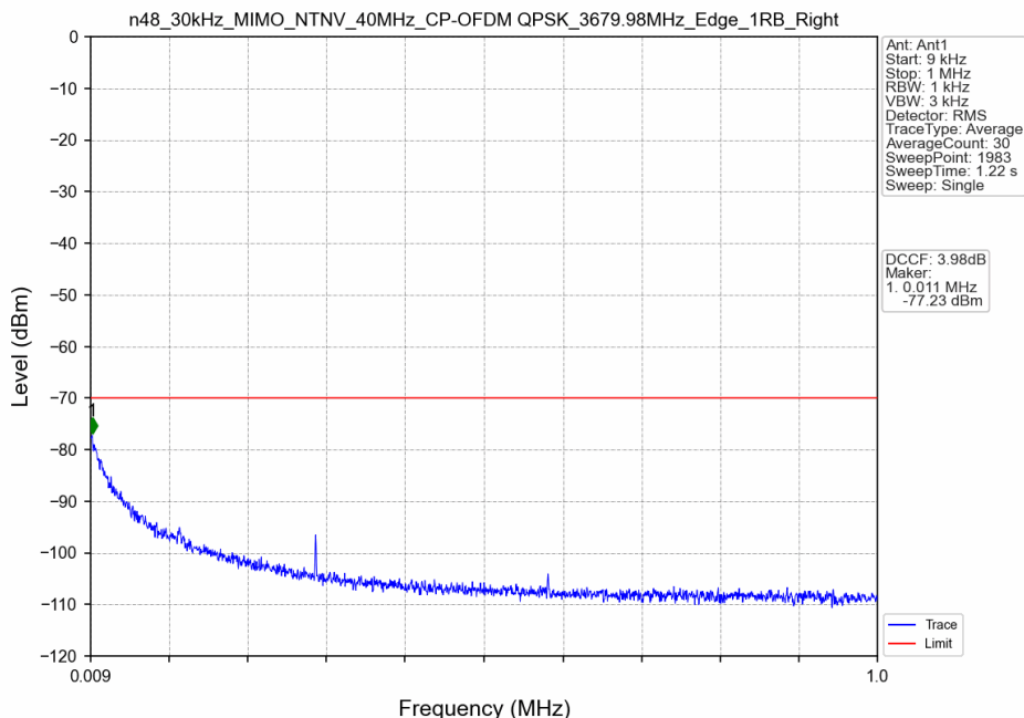
n48_30kHz_MIMO_NTNV_40MHz_CP-OFDM QPSK_3679.98MHz_Edge_1RB_Right
