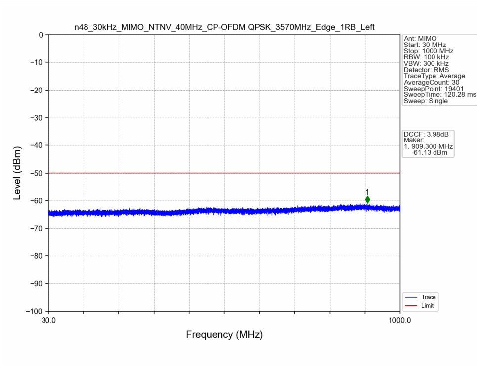
n48_30kHz_MIMO_NTNV_40MHz_CP-OFDM QPSK_3570MHz_Edge_1RB_Left
