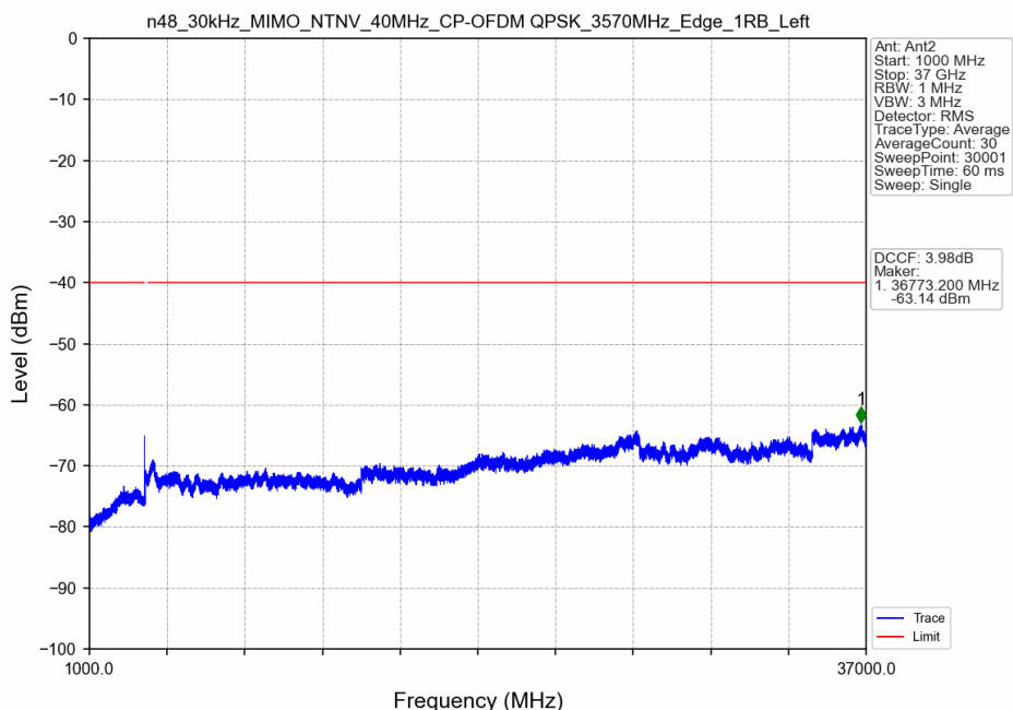
n48_30kHz_MIMO_NTNV_40MHz_CP-OFDM QPSK_3570MHz_Edge_1RB_Left
