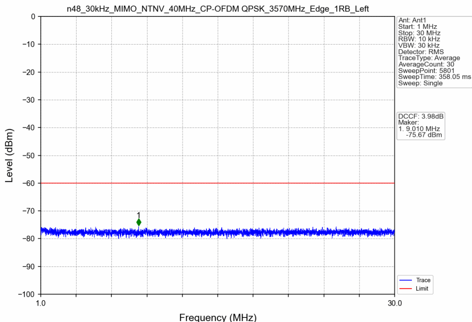
n48_30kHz_MIMO_NTNV_40MHz_CP-OFDM QPSK_3570MHz_Edge_1RB_Left
