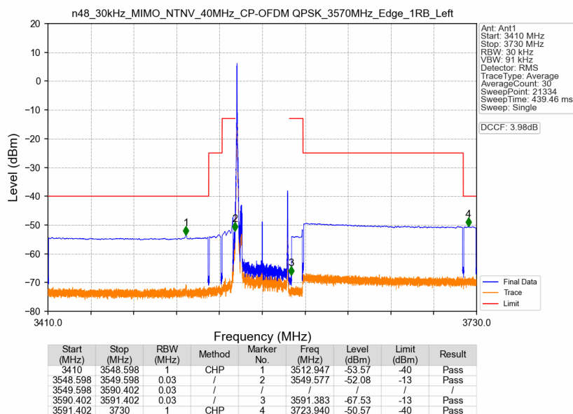
n48_30kHz_MIMO_NTNV_40MHz_CP-OFDM QPSK_3570MHz_Edge_1RB_Left
