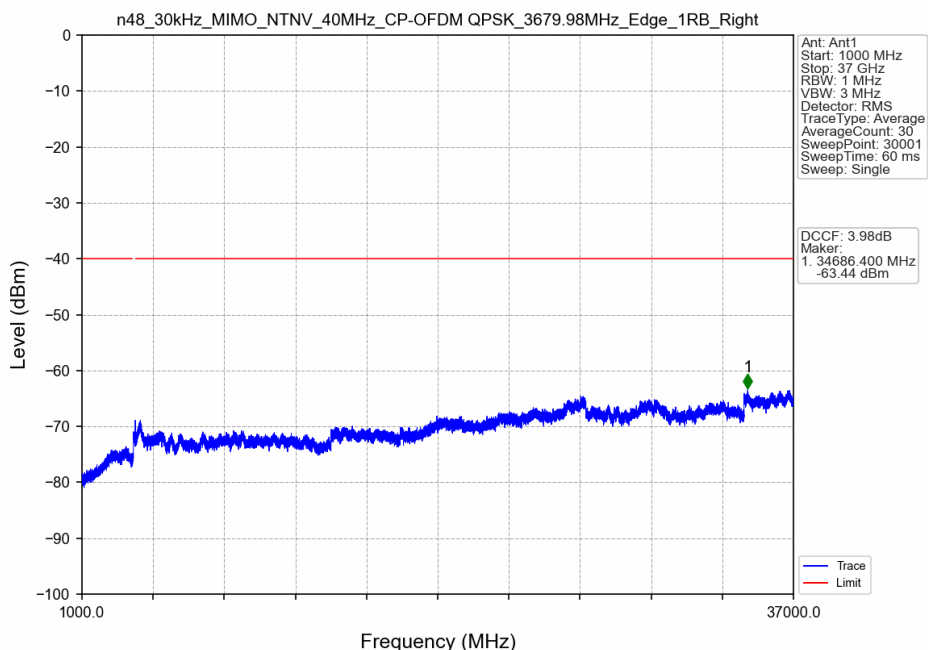
n48_30kHz_MIMO_NTNV_40MHz_CP-OFDM QPSK_3679.98MHz_Edge_1RB_Right
