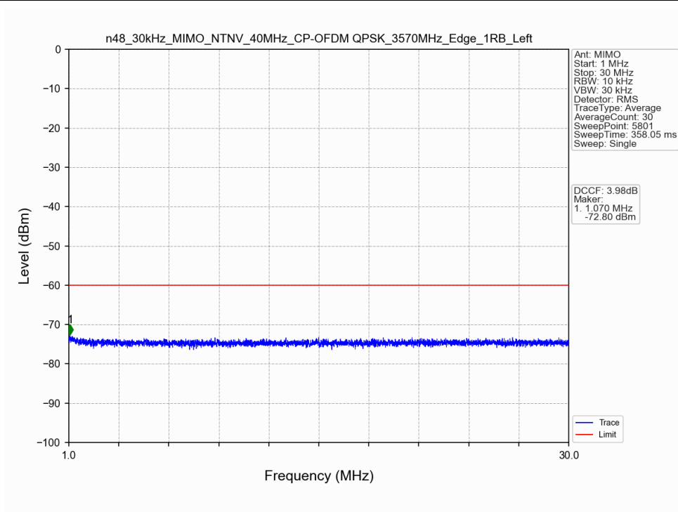
n48_30kHz_MIMO_NTNV_40MHz_CP-OFDM QPSK_3570MHz_Edge_1RB_Left
