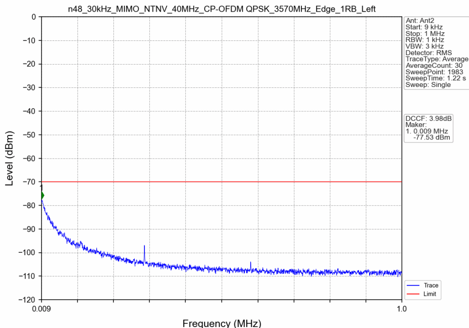
n48_30kHz_MIMO_NTNV_40MHz_CP-OFDM QPSK_3570MHz_Edge_1RB_Left
