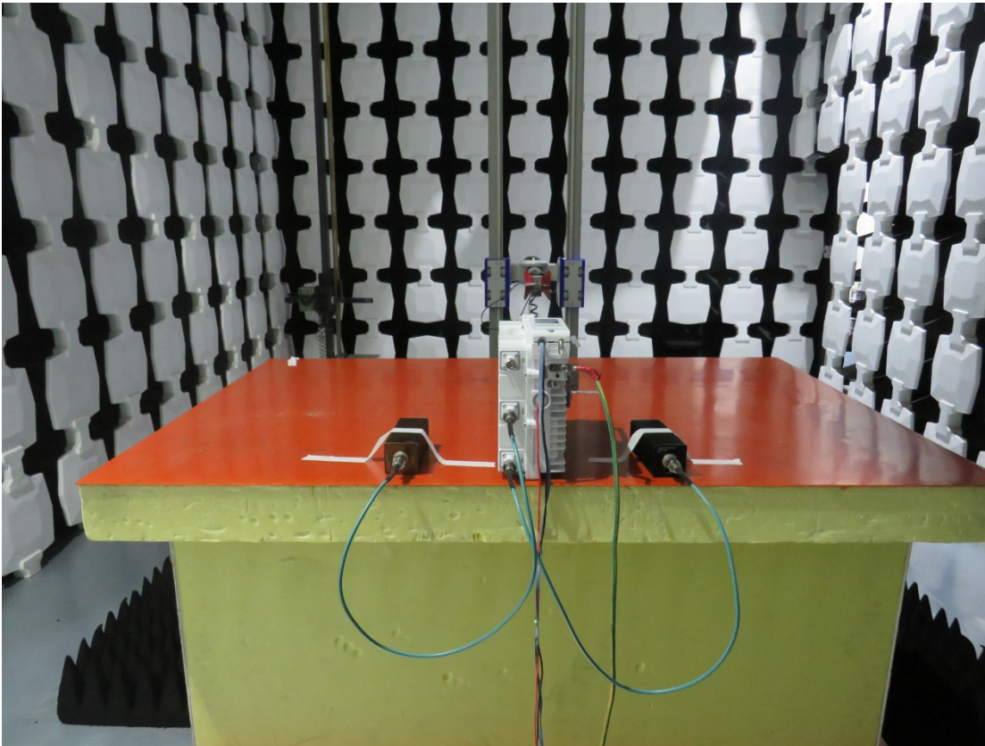
Part96 RSE test setup
