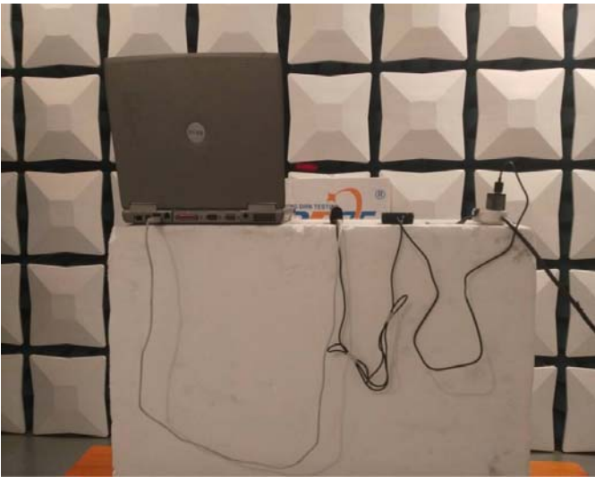
8.2 AC Power Line Conducted Emission
