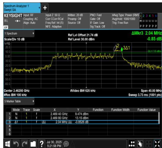
11AX20MIMO-Ant7-2462-52Tone-RU40-PASS
