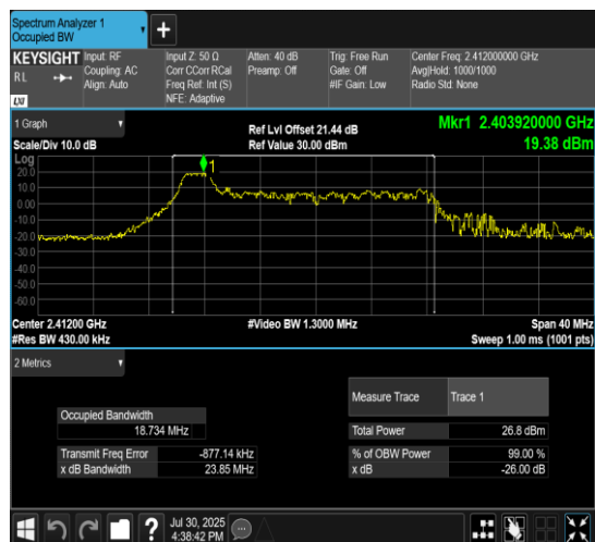
11AX20MIMO-Ant7-2412-52Tone-RU37
