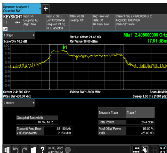
11AX20MIMO-Ant10-2412-106Tone-RU53
