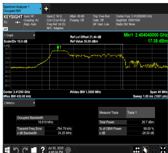
11AX20MIMO-Ant7-2412-106Tone-RU53
