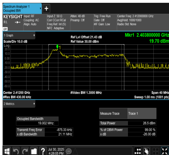
11AX20MIMO-Ant10-2412-52Tone-RU37
