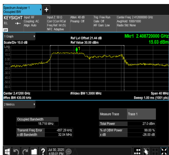
11AX20MIMO-Ant7-2412-106Tone-RU53
