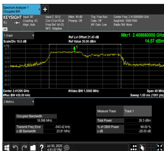
11AX20MIMO-Ant10-2412-106Tone-RU53
