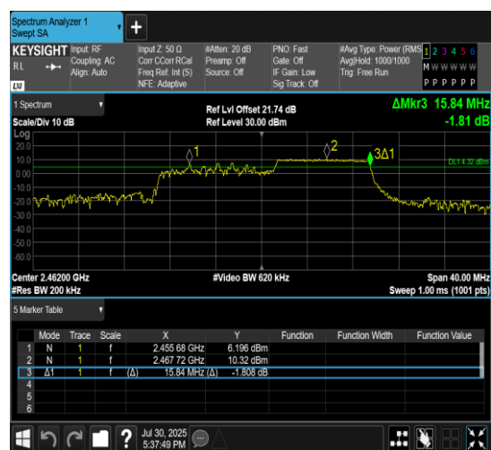
11AX20MIMO-Ant7-2462-106Tone-RU54-PASS
