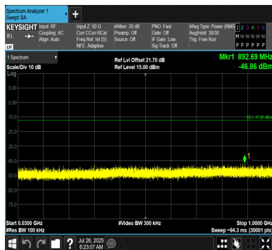
BLE_125K-Ant7-2480-30~1000-PASS
