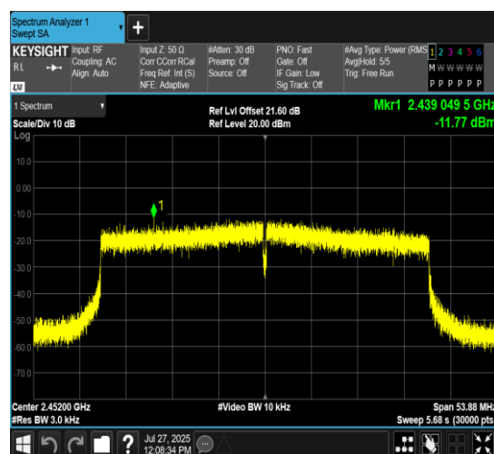
11AX40MIMO-Ant7-2452-PASS
