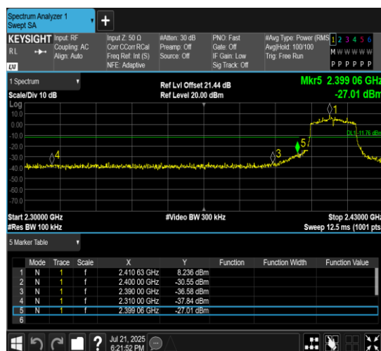
11G-CDD-Ant7-2412-PASS
