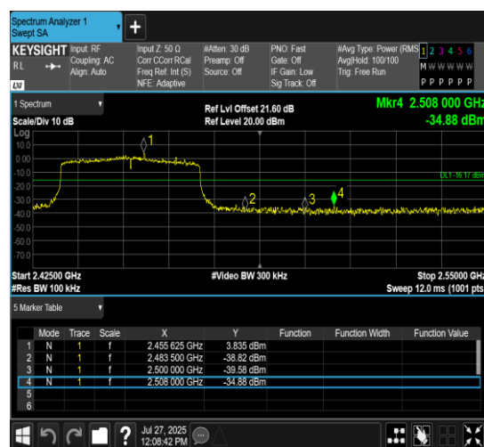
11AX40MIMO-Ant7-2452-PASS
