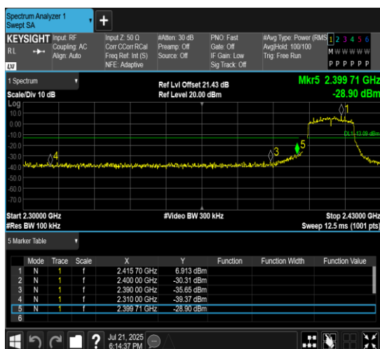
11G-CDD-Ant10-2412-PASS
