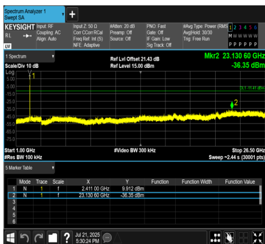
11B-CDD-Ant10-2412-1000~26500-PASS
