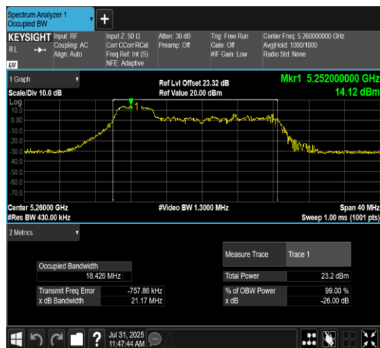
11AX20MIMO-Ant7-5260-106Tone-RU53
