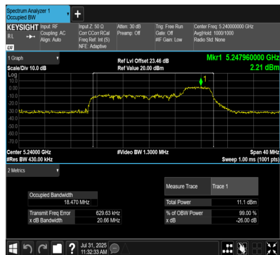
11AX20MIMO-Ant7-5240-106Tone-RU54
