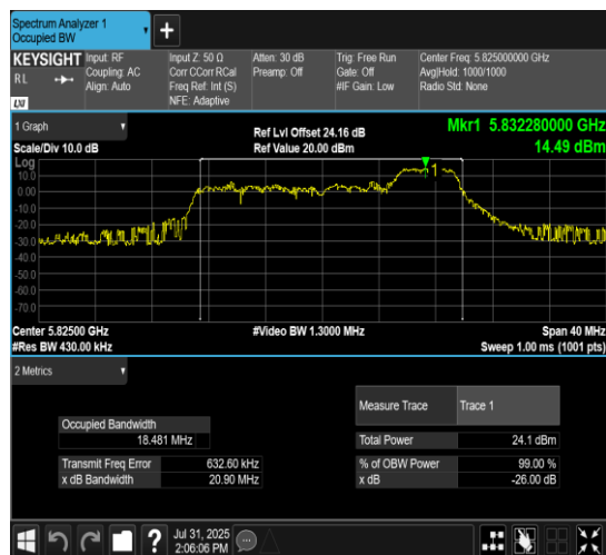
11AX20MIMO-Ant7-5825-106Tone-RU54
