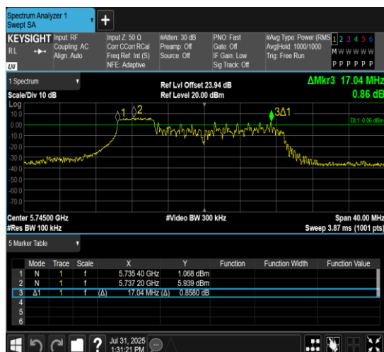
11AX20MIMO-Ant10-5745-106Tone-RU53-PASS
