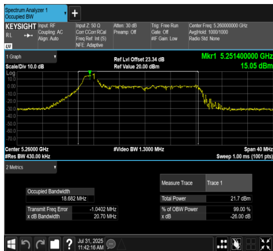
11AX20MIMO-Ant10-5260-52Tone-RU37
