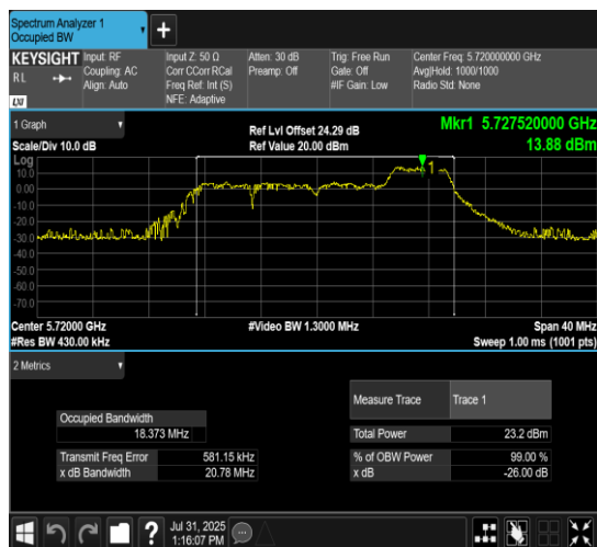
11AX20MIMO-Ant10-5720-106Tone-RU54
