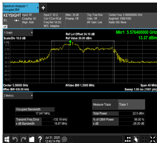
11AX20MIMO-Ant7-5580-106Tone-RU53
