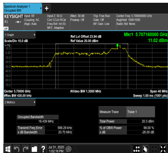
11AX20MIMO-Ant7-5700-106Tone-RU54
