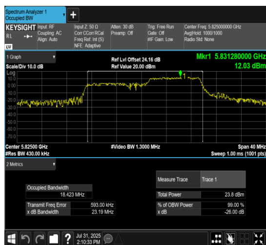
11AX20MIMO-Ant7-5825-106Tone-RU54
