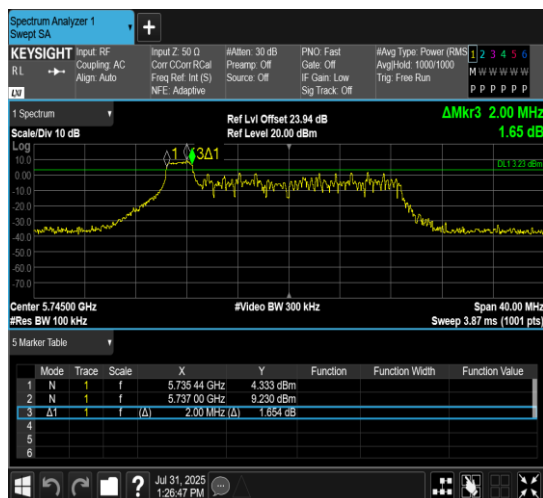
11AX20MIMO-Ant10-5745-52Tone-RU37-PASS
