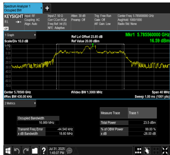
11AX20MIMO-Ant7-5785-52Tone-RU38
