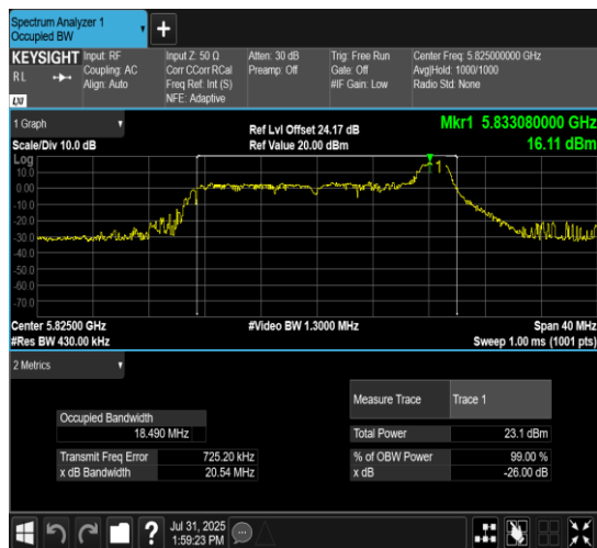
11AX20MIMO-Ant10-5825-52Tone-RU40
