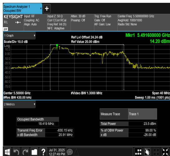
11AX20MIMO-Ant7-5500-106Tone-RU53
