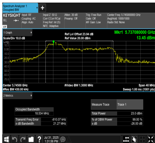
11AX20MIMO-Ant10-5745-106Tone-RU53
