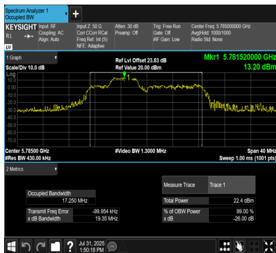
11AX20MIMO-Ant10-5785-106Tone-RU53
