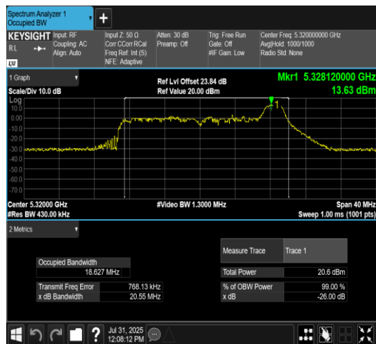
11AX20MIMO-Ant7-5320-52Tone-RU40
