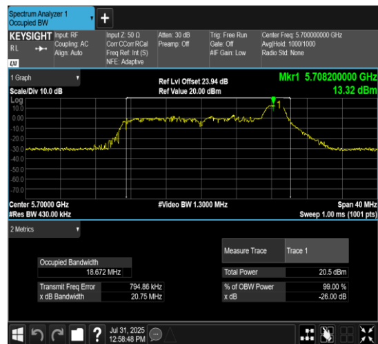
11AX20MIMO-Ant7-5700-52Tone-RU40
