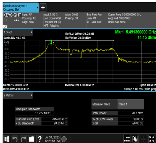
11AX20MIMO-Ant7-5500-52Tone-RU37
