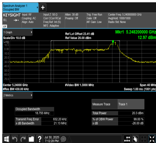
11AX20MIMO-Ant10-5240-52Tone-RU40
