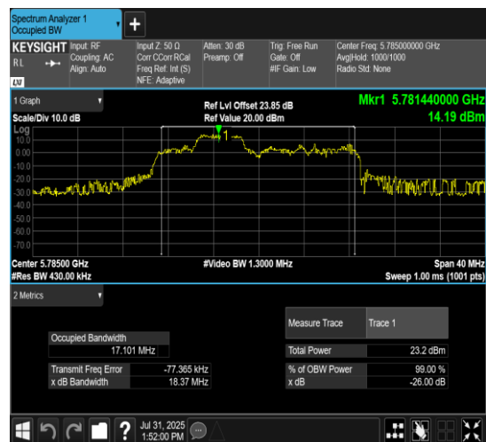
11AX20MIMO-Ant7-5785-106Tone-RU53
