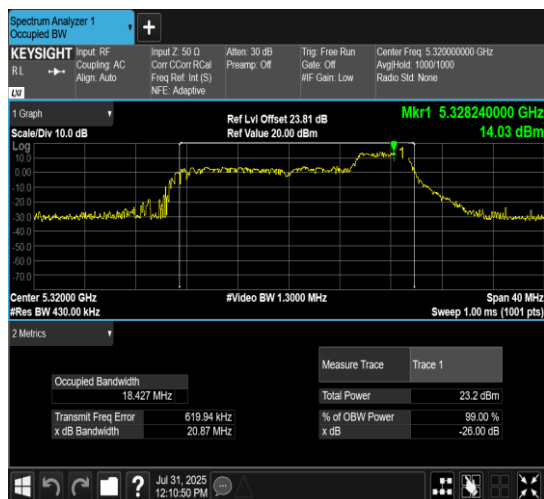
11AX20MIMO-Ant10-5320-106Tone-RU54
