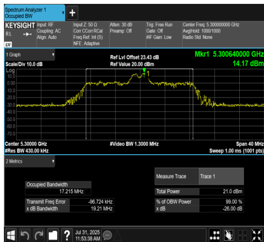
11AX20MIMO-Ant10-5300-52Tone-RU38
