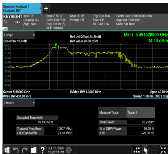
11AX20MIMO-Ant10-5500-106Tone-RU53
