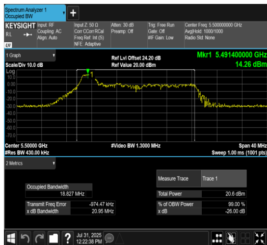
11AX20MIMO-Ant10-5500-52Tone-RU37
