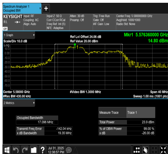
11AX20MIMO-Ant10-5580-106Tone-RU53
