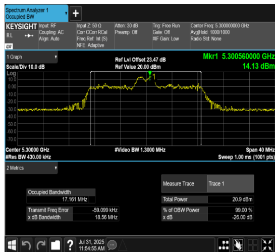
11AX20MIMO-Ant7-5300-52Tone-RU38
