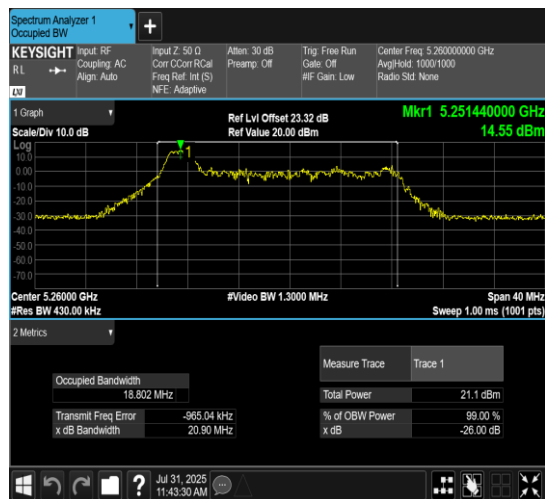
11AX20MIMO-Ant7-5260-52Tone-RU37
