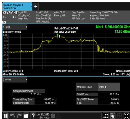
11AX20MIMO-Ant7-5300-106Tone-RU53
