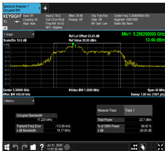
11AX20MIMO-Ant10-5300-106Tone-RU53
