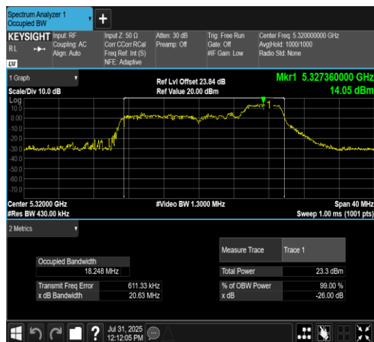
11AX20MIMO-Ant7-5320-106Tone-RU54
