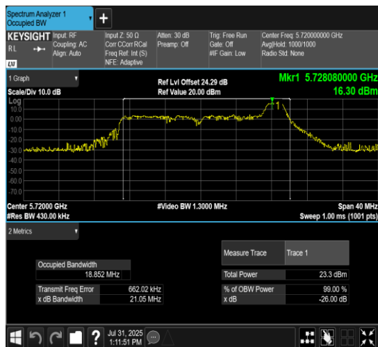
11AX20MIMO-Ant10-5720-52Tone-RU40
