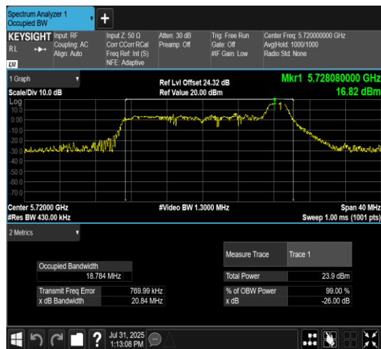
11AX20MIMO-Ant7-5720-52Tone-RU40
