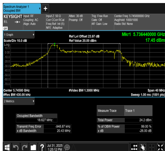
11AX20MIMO-Ant7-5745-52Tone-RU37
