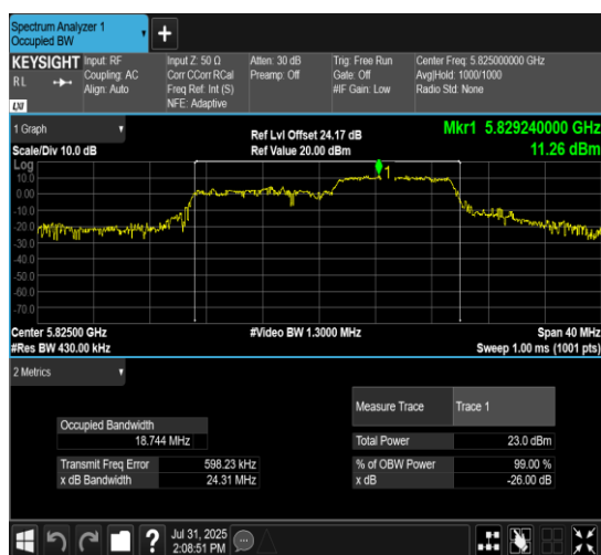
11AX20MIMO-Ant10-5825-106Tone-RU54
