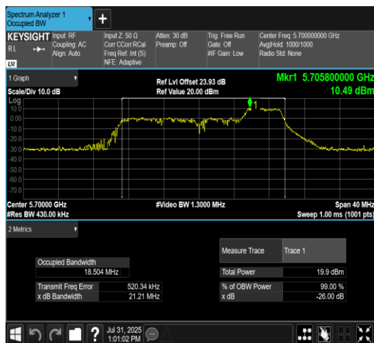
11AX20MIMO-Ant10-5700-106Tone-RU54
