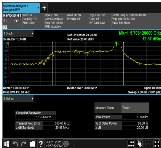
11AX20MIMO-Ant10-5700-52Tone-RU40
