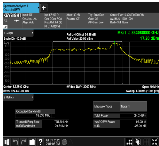
11AX20MIMO-Ant7-5825-52Tone-RU40
