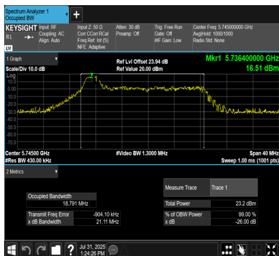
11AX20MIMO-Ant10-5745-52Tone-RU37
