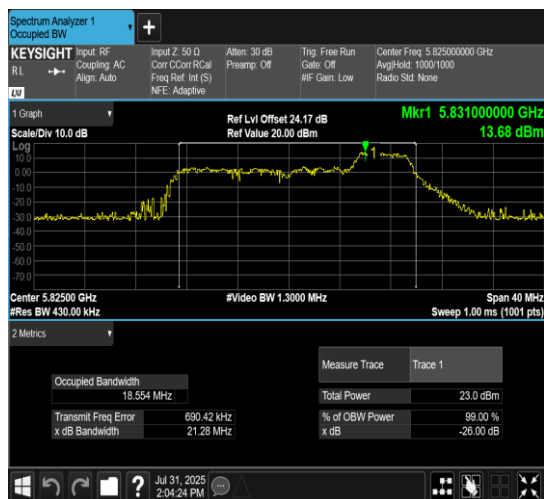
11AX20MIMO-Ant10-5825-106Tone-RU54
