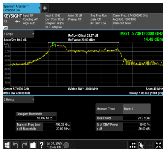
11AX20MIMO-Ant7-5745-106Tone-RU53
