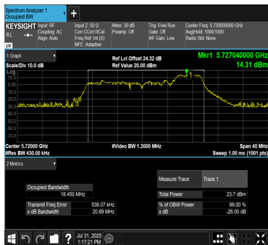
11AX20MIMO-Ant7-5720-106Tone-RU54
