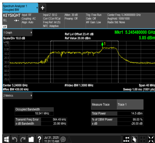
11AX20MIMO-Ant10-5240-106Tone-RU54
