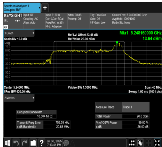
11AX20MIMO-Ant7-5240-52Tone-RU40
