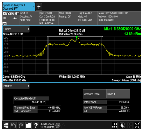
11AX20MIMO-Ant7-5580-52Tone-RU38
