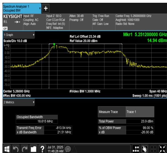
11AX20MIMO-Ant10-5260-106Tone-RU53
