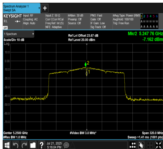
11AX160MIMO-Ant7-5250_UNII-2A-PASS
