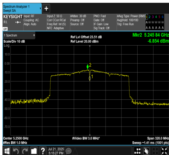
11AX160MIMO-Ant10-5250_UNII-2A-PASS
