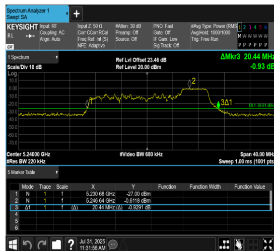
11AX20MIMO-Ant7-5240-106Tone-RU54
