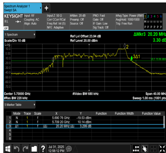
11AX20MIMO-Ant7-5700-52Tone-RU40
