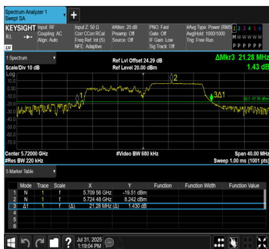
11AX20MIMO-Ant10-5720-106Tone-RU54
