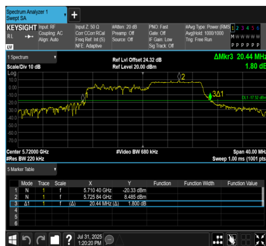
11AX20MIMO-Ant7-5720-106Tone-RU54
