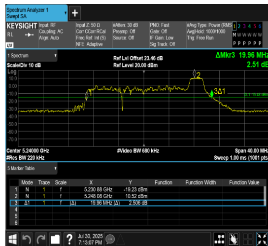
11AX20MIMO-Ant7-5240-52Tone-RU40
