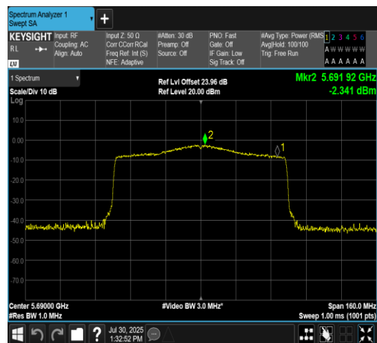
11AX80MIMO-Ant7-5690_UNII-3-PASS
