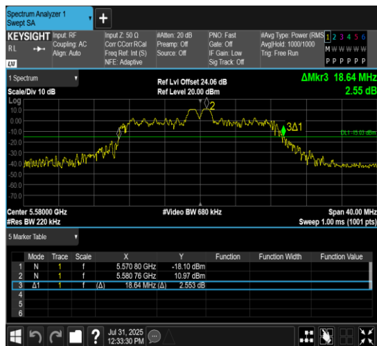
11AX20MIMO-Ant10-5580-52Tone-RU38
