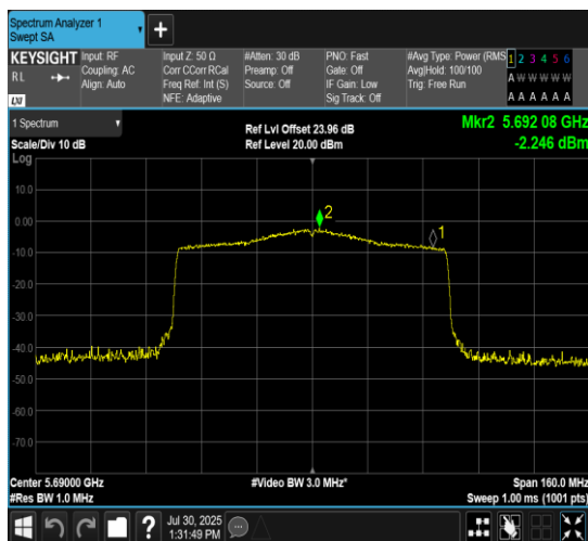
11AX80MIMO-Ant10-5690_UNII-3-PASS
