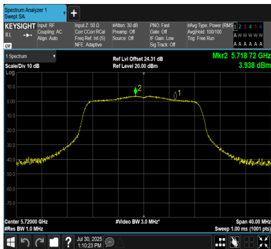
11N20MIMO-Ant10-5720_UNII-3-PASS
