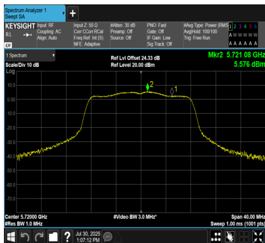
11A-CDD-Ant10-5720_UNII-3-PASS
