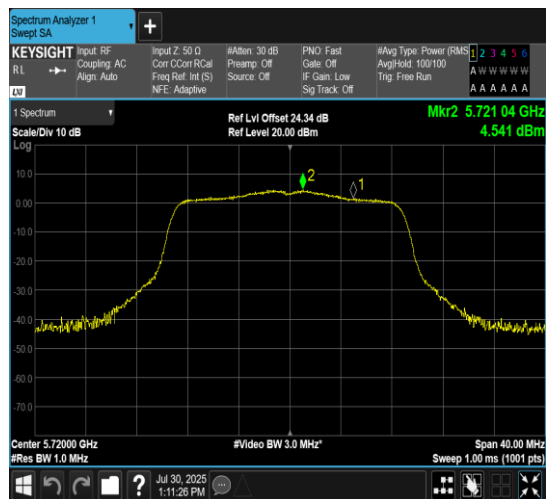
11N20MIMO-Ant7-5720_UNII-3-PASS
