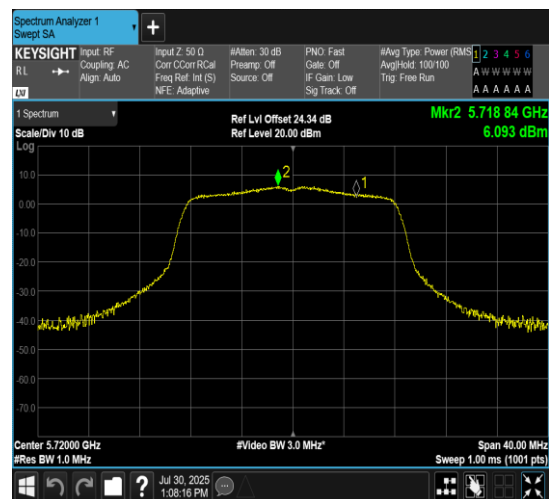
11A-CDD-Ant7-5720_UNII-3-PASS
